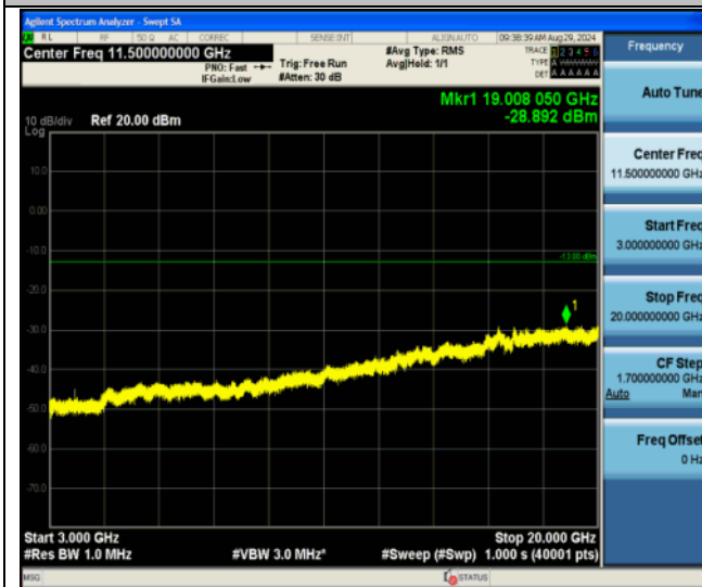
Band2-20MHz-QPSK-19100-1RB#0-3000~20000-PASS
