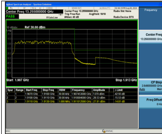
Band2-3MHz-QPSK-19185-15RB#0-PASS
