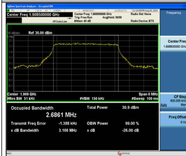
Band2-3MHz-QPSK-19185-15RB#0-PASS
