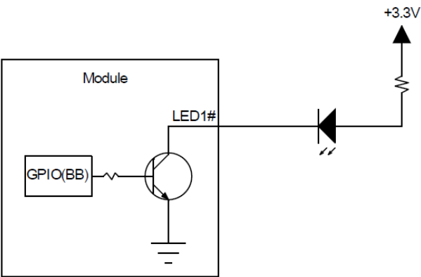
Figure 3-17 LED driving circuit
