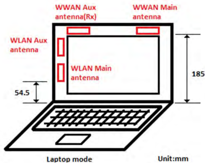
Fig.7 Antenna position of EUT(laptop mode)
