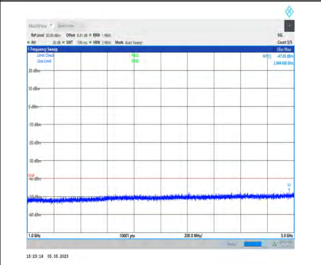
1-N48-PC3-30-40-H-1-DFT-PI2BPSK-Inner_1RB_Le ft-1@1-1000-3000-Ant1-2677.60--47.03--40-PASS
