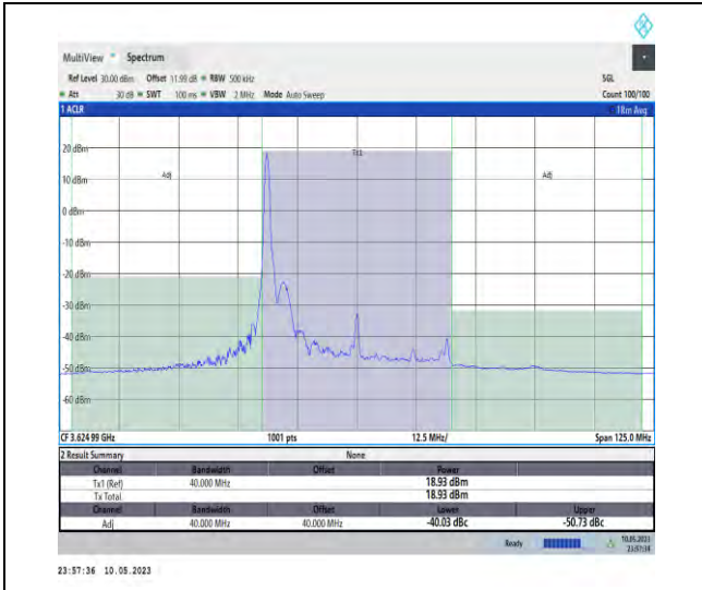
1-N48-PC3-30-40-M-CP-QPSK-Edge_1RB_Left-1 @0-Ant1-1--PASS-see graph
