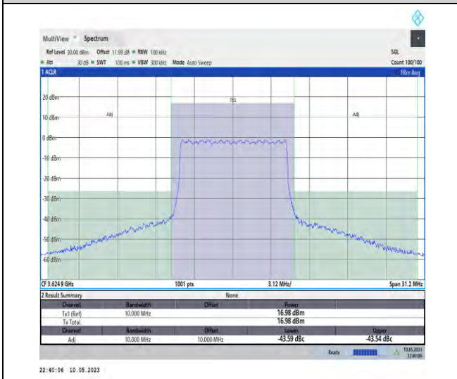
1-N48-PC3-30-10-M-CP-QPSK-Outer_Full-24@0-A nt1-1--PASS
