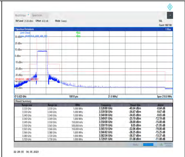
1-N48-PC3-30-15-L-3-DFT-PI2BPSK-Outer_Full-36@0-Ant1-1--PASS-see graph
