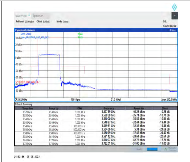
1-N48-PC3-30-30-L-3-DFT-PI2BPSK-Outer_Full-75@0-Ant1-1--PASS-see graph
