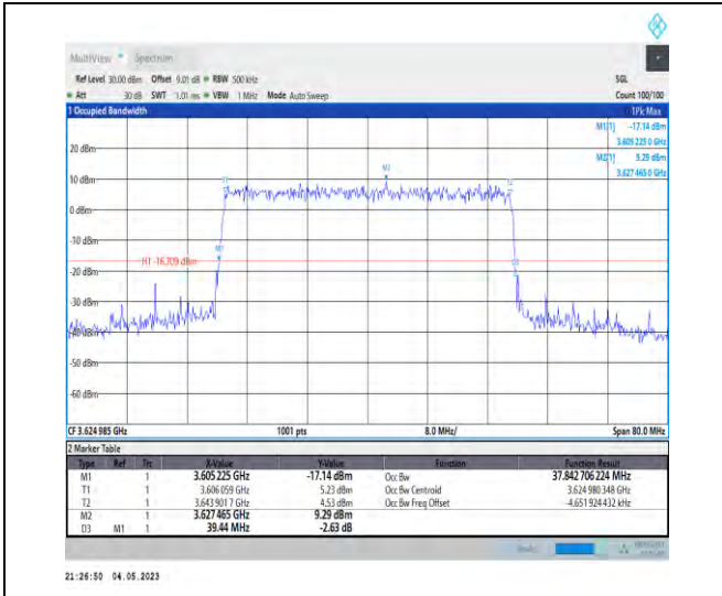
1-N48-PC3-30-40-M-8-CP-64QAM-Outer_Full-106@ 0-Ant1-37.843-39.440-<40-PASS
