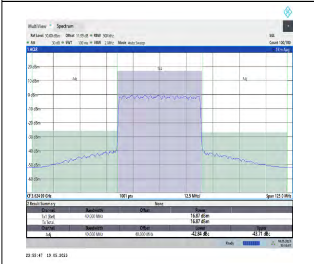
1-N48-PC3-30-40-M-CP-QPSK-Outer_Full-106@0- Ant1-1--PASS
