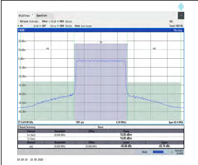
1-N48-PC3-30-20-M-CP-QPSK-Outer_Full-51@0-A nt1-1--PASS
