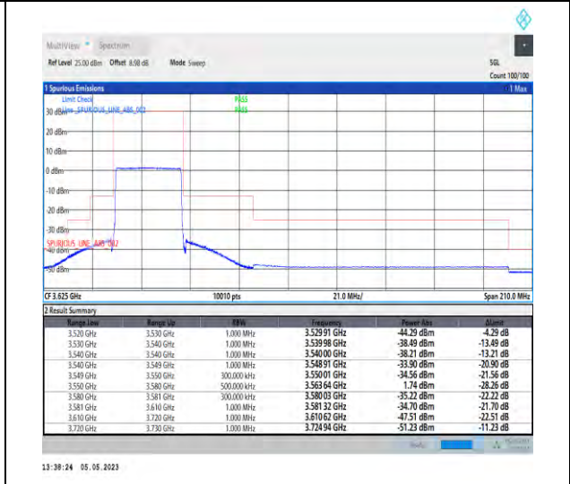
1-N48-PC3-30-30-L-6-CP-QPSK-Outer_Full-78@0-Ant1-1--PASS-see graph
