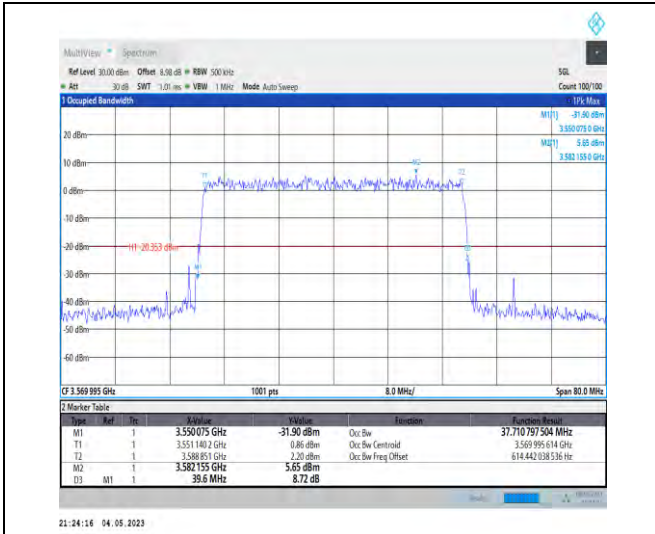
1-N48-PC3-30-40-L-9-CP-256QAM-Outer_Full-106 @0-Ant1-37.711-39.600-≤40-PASS
