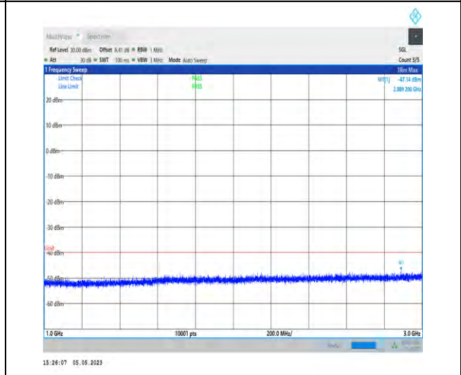
1-N48-PC3-30-40-M-1-DFT-PI2BPSK-Inner_1RB_Le ft-1@1-1000-3000-Ant1-2721.40--47.14--40-PASS
