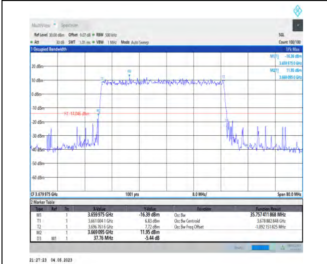
1-N48-PC3-30-40-H-1-DFT-QPSK-Outer_Full-100@ 0-Ant1-35.757-37.760-<40-PASS
