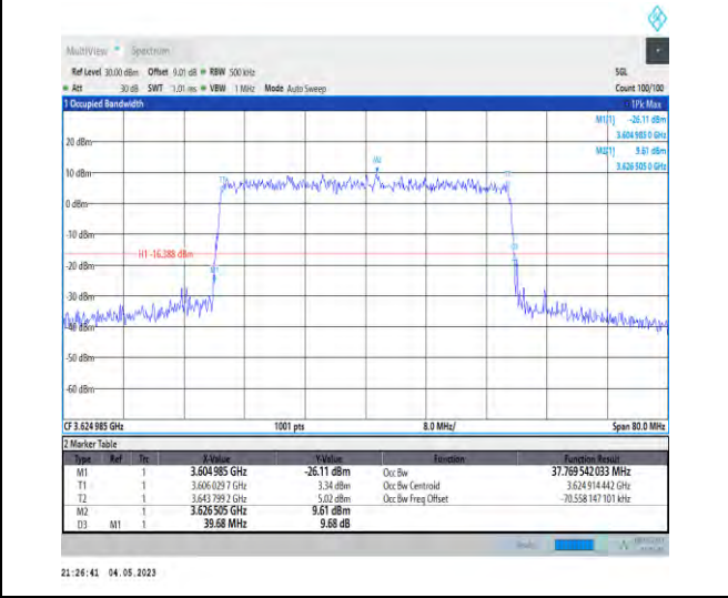
1-N48-PC3-30-40-M-7-CP-16QAM-Outer_Full-106@0 0-Ant1-37.77-39.680-<math>\leq 40</math>-PASS
