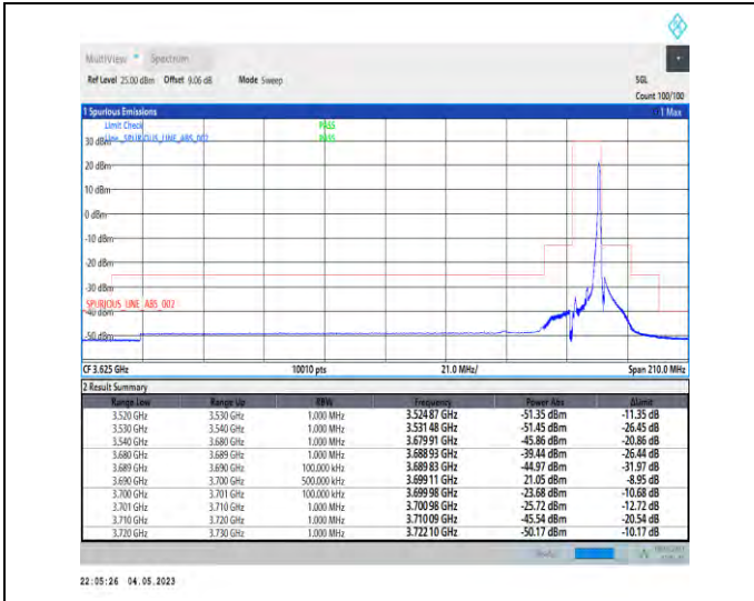
1-N48-PC3-30-10-H-2-DFT-PI2BPSK-Edge_1RB_Right-t1@23-Ant1-1--PASS-see graph
