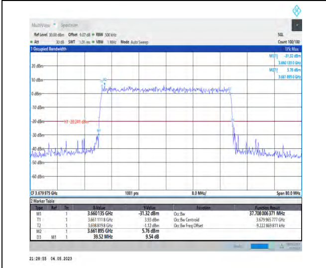
1-N48-PC3-30-40-H-9-CP-256QAM-Outer_Full-106 @0-Ant1-37.708-39.520-≤40-PASS
