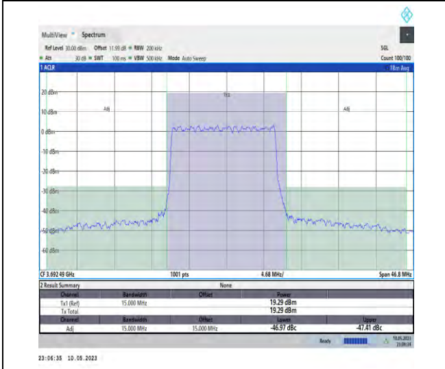
1-N48-PC3-30-15-H-DFT-PI2BPSK-Outer_Full-36@ 0-Ant1-1--PASS
