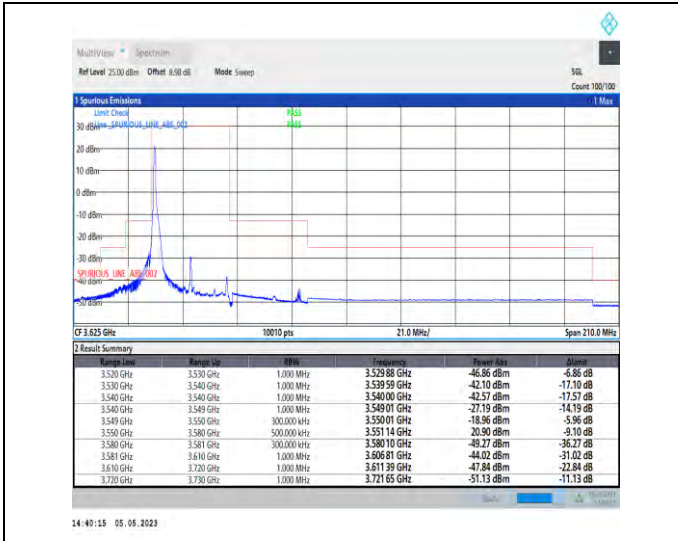
1-N48-PC3-30-30-L-1-DFT-PI2BPSK-Edge_1RB_Left-1@0-Ant1-1--PASS-see graph
