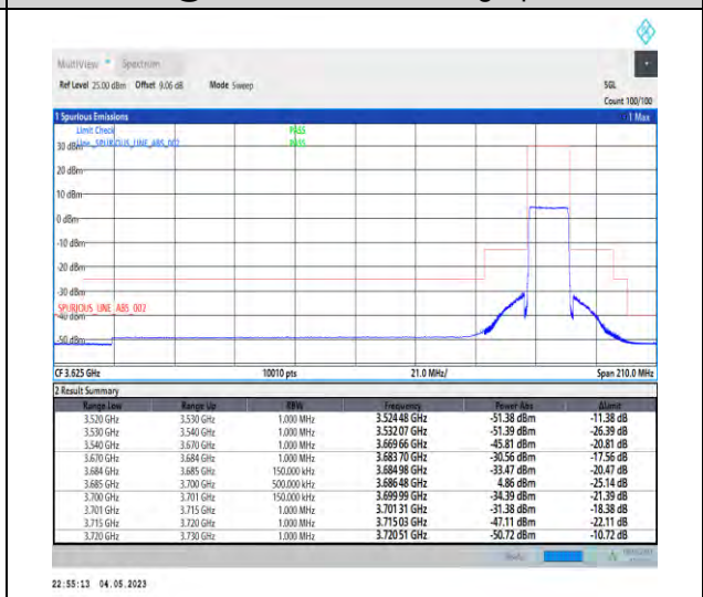
1-N48-PC3-30-15-H-6-CP-QPSK-Outer_Full-38@0-Ant1-1--PASS-see graph
