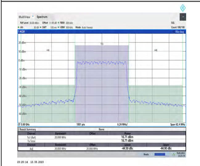
1-N48-PC3-30-20-H-CP-QPSK-Outer_Full-51@0-Ant t1-1--PASS
