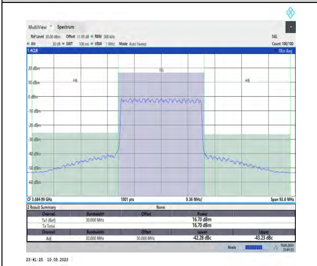
1-N48-PC3-30-30-H-CP-QPSK-Outer_Full-78@0-A nt1-1--PASS
