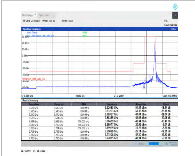
1-N48-PC3-30-15-H-2-DFT-PI2BPSK-Edge_1RB_Right-t1@37-Ant1-1--PASS-see graph
