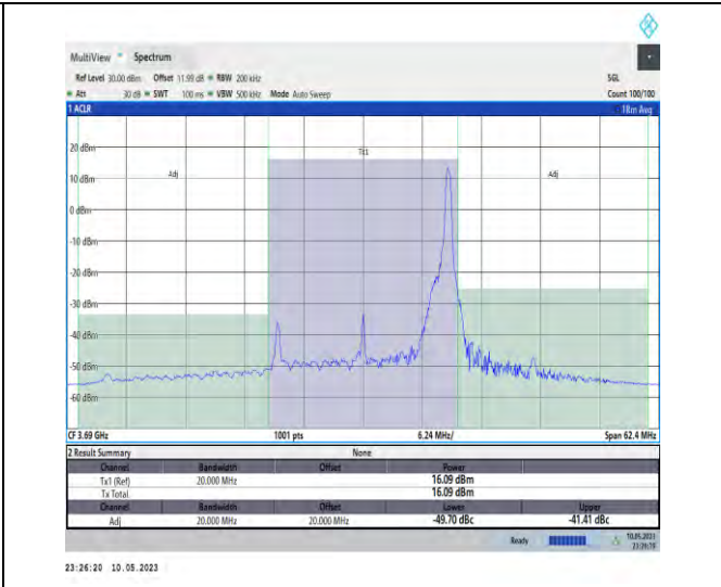
1-N48-PC3-30-20-H-CP-QPSK-Edge_1RB_Left-1@5 0-Ant1-1--PASS
