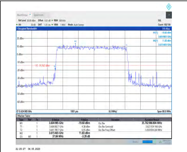
1-N48-PC3-30-40-M-1-DFT-QPSK-Outer_Full-100 @0-Ant1-35.703-37.840-≤40-PASS
