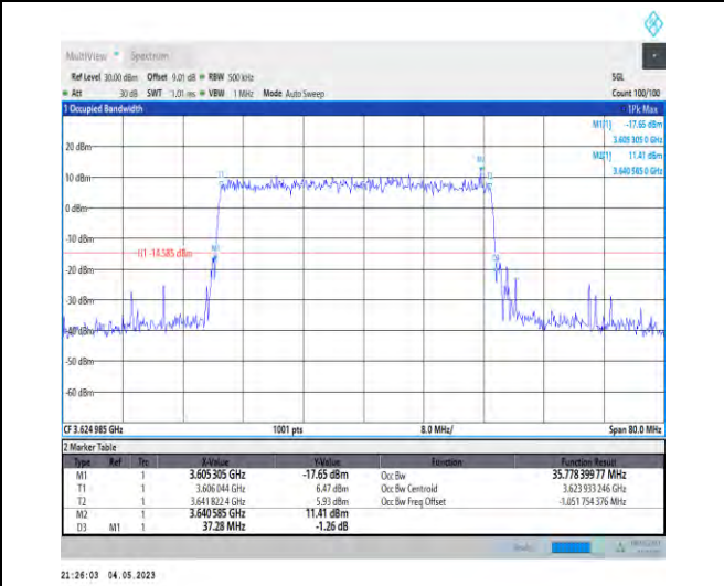
1-N48-PC3-30-40-M-3-DFT-16QAM-Outer_Full-100 @0-Ant1-35.778-37.280-≤40-PASS
