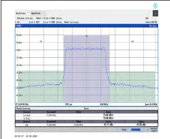
1-N48-PC3-30-15-M-DFT-PI2BPSK-Outer_Full-36@0-Ant1-1--PASS
