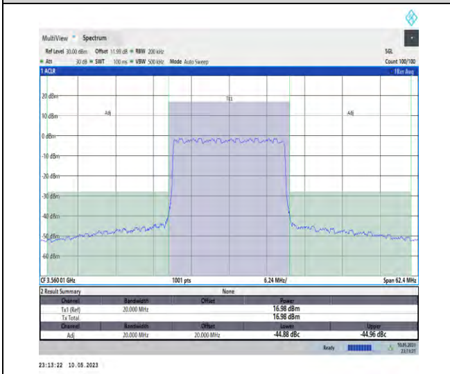
1-N48-PC3-30-20-L-CP-QPSK-Outer_Full-51@0-Ant t1-1--PASS
