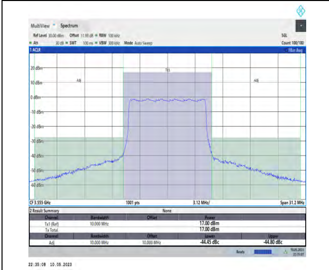
1-N48-PC3-30-10-L-CP-QPSK-Outer_Full-24@0-Ant t1-1--PASS
