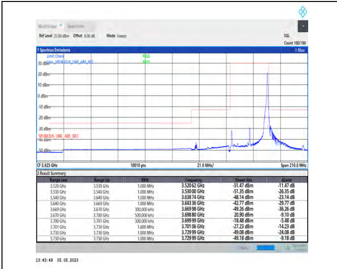
1-N48-PC3-30-30-H-2-DFT-PI2BPSK-Edge_1RB_Right-t1@77-Ant1-1--PASS-see graph
