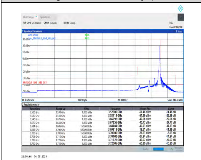
1-N48-PC3-30-15-H-5-CP-QPSK-Edge_1RB_Right-1@37-Ant1-1--PASS-see graph
