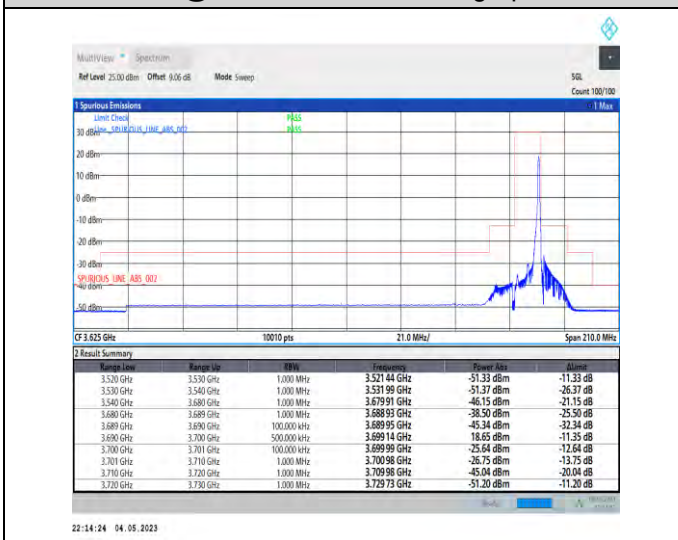
1-N48-PC3-30-10-H-5-CP-QPSK-Edge_1RB_Right-1@23-Ant1-1--PASS-see graph
