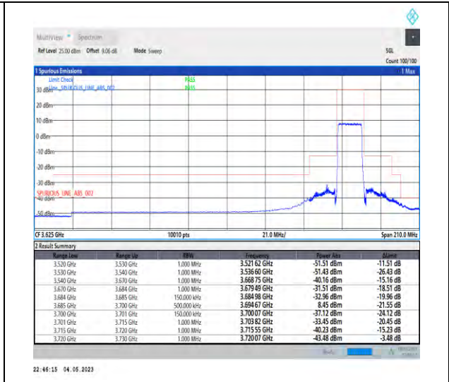
1-N48-PC3-30-15-H-3-DFT-PI2BPSK-Outer_Full-36@0-Ant1-1--PASS-see graph
