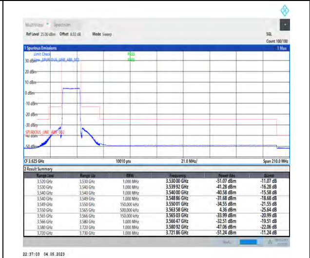
1-N48-PC3-30-15-L-6-CP-QPSK-Outer_Full-38@0-Ant1-1--PASS-see graph
