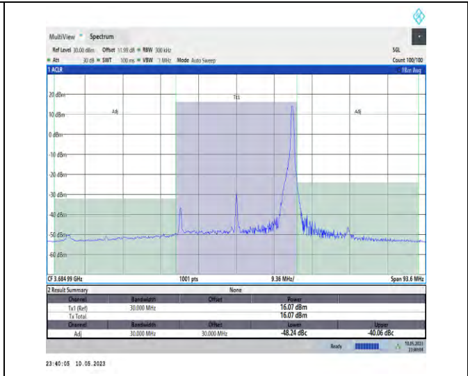
1-N48-PC3-30-30-H-CP-QPSK-Edge_1RB_Left-1@ 7-Ant1-1--PASS
