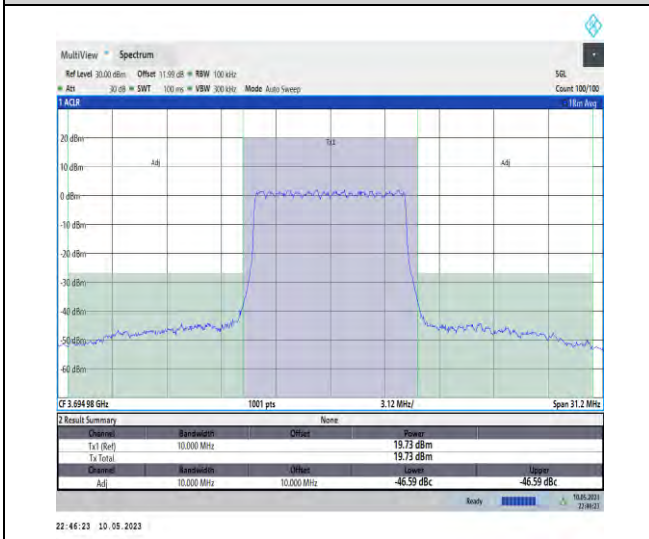
1-N48-PC3-30-10-H-DFT-PI2BPSK-Outer_Full-24@ 0-Ant1-1--PASS
