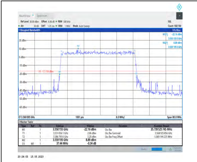
1-N48-PC3-30-40-L-5-DFT-256QAM-Outer_Full-100 @0-Ant1-35.74-37.440-≤40-PASS
