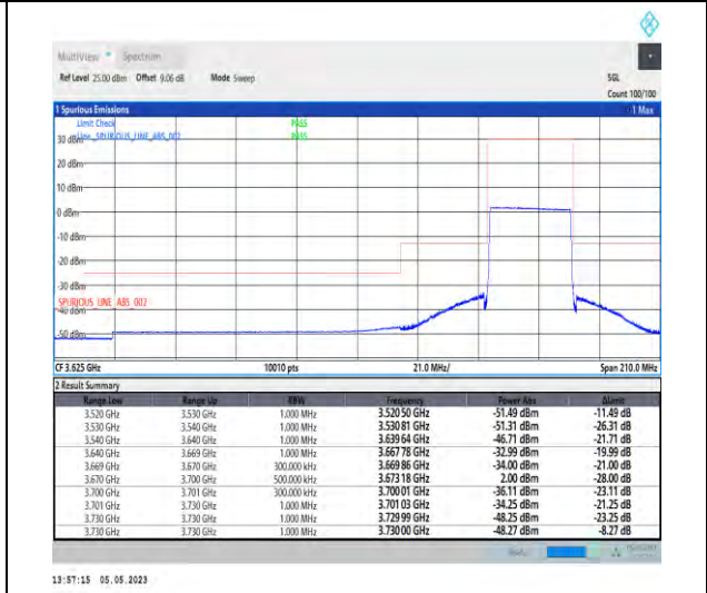
1-N48-PC3-30-30-H-6-CP-QPSK-Outer_Full-78@0-Ant1-1--PASS-see graph
