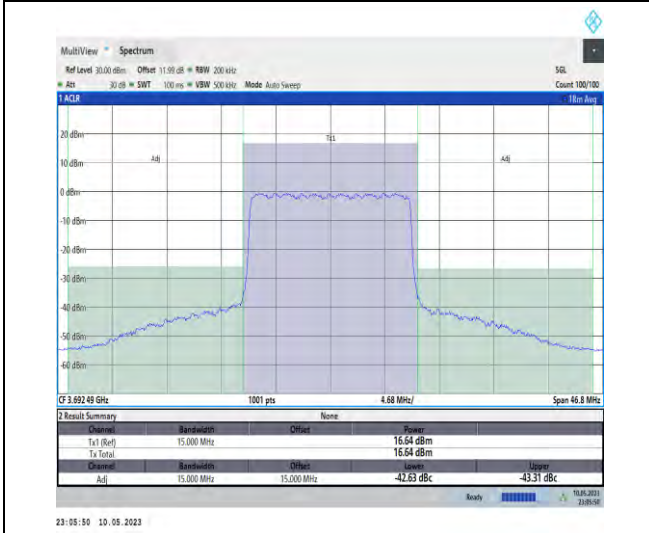
1-N48-PC3-30-15-H-CP-QPSK-Outer_Full-36@0-Ant t1-1--PASS
