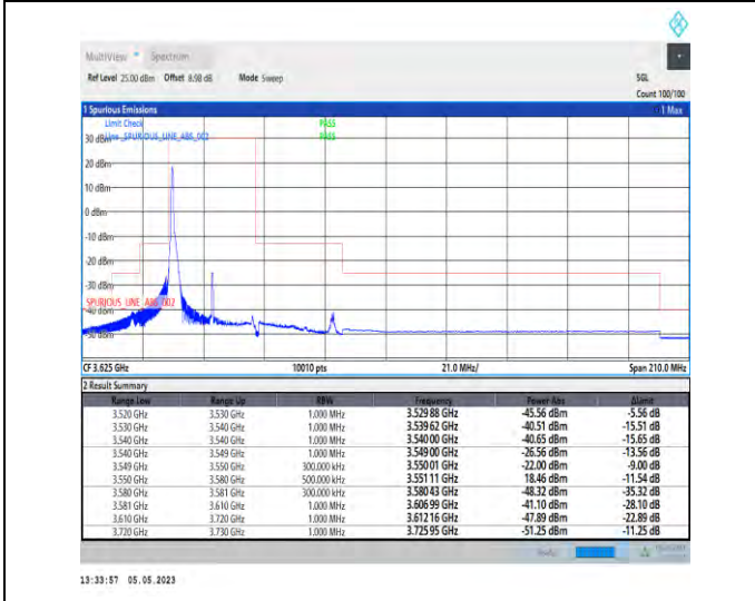
1-N48-PC3-30-30-L-4-CP-QPSK-Edge_1RB_Left-1@0-Ant1-1--PASS-see graph
