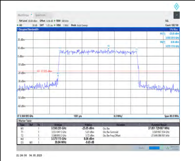
1-N48-PC3-30-40-L-8-CP-64QAM-Outer_Full-106@0-Ant1-37.852-39.840-≤40-PASS
