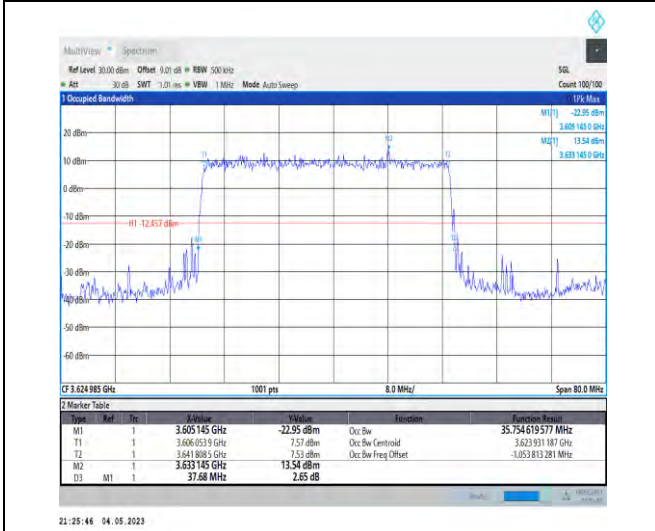
1-N48-PC3-30-40-M-2-DFT-PI2BPSK-Outer_Full-10 @0-Ant1-35.755-37.680-≤40-PASS
