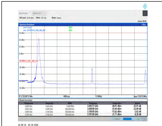
1-N77-3700-3980--30-60-L-4-CP-QPSK-Edge_1RB_Le ft-1@0-Ant2-PASS-see graph
