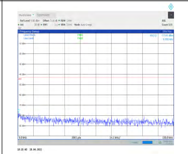
1-N77-3700-3980--30-100-M-1-DFT-QPSK-Edge_1R B_Left-1@0-0.009-0.15-Ant2--77.81--43-PASS
