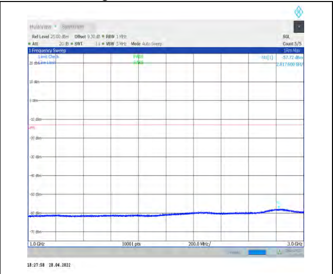
1-N77-3700-3980--30-100-H-1-DFT-QPSK-Edge_1R B_Left-1@0-1000-3000-Ant2--57.72--13-PASS
