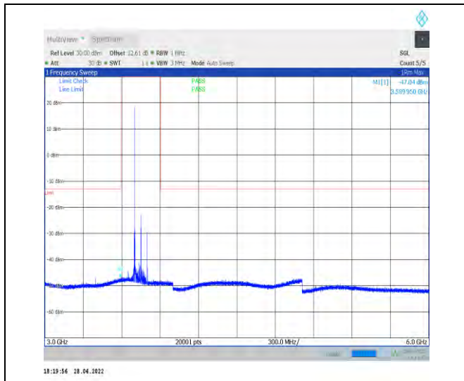
1-N77-3700-3980--30-100-L-1-DFT-QPSK-Edge_1R B_Left-1@0-3000-6000-Ant1--47.04--13-PASS
