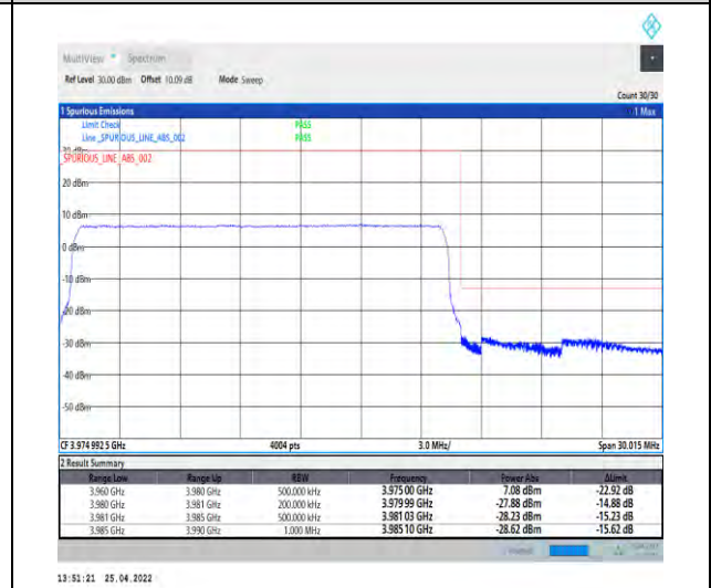
1-N77-3700-3980--30-20-H-6-CP-QPSK-Outer_Fu ll-51@0-Ant2-PASS-see graph
