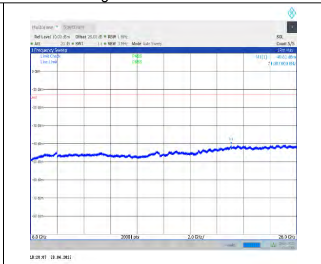
1-N77-3700-3980--30-100-L-1-DFT-QPSK-Edge_1R B_Left-1@0-6000-26000-Ant1--40.61--13-PASS
