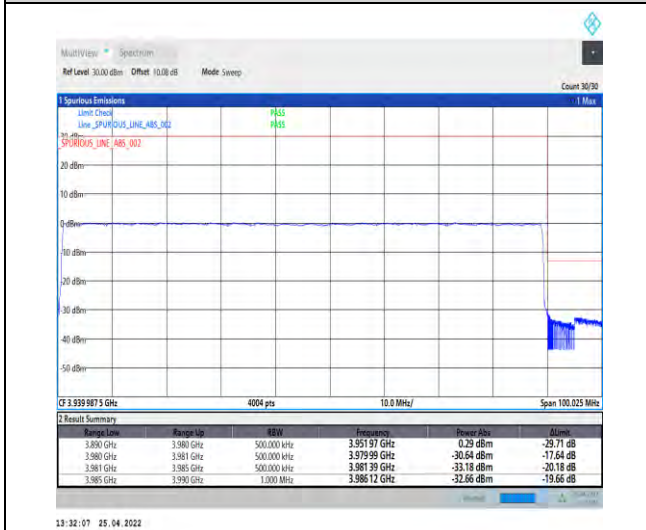
1-N77-3700-3980--30-90-H-6-CP-QPSK-Outer_Full-245@0-Ant1-PASS-see graph
