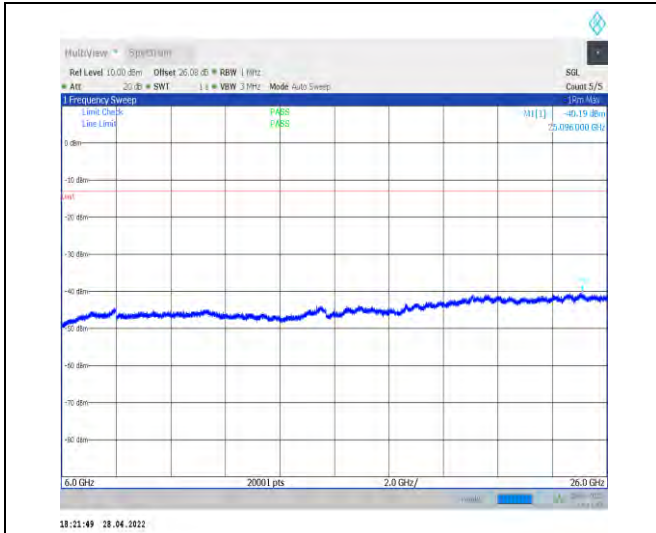
1-N77-3700-3980--30-100-M-1-DFT-QPSK-Edge_1R B_Left-1@0-6000-26000-Ant1--40.19--13-PASS
