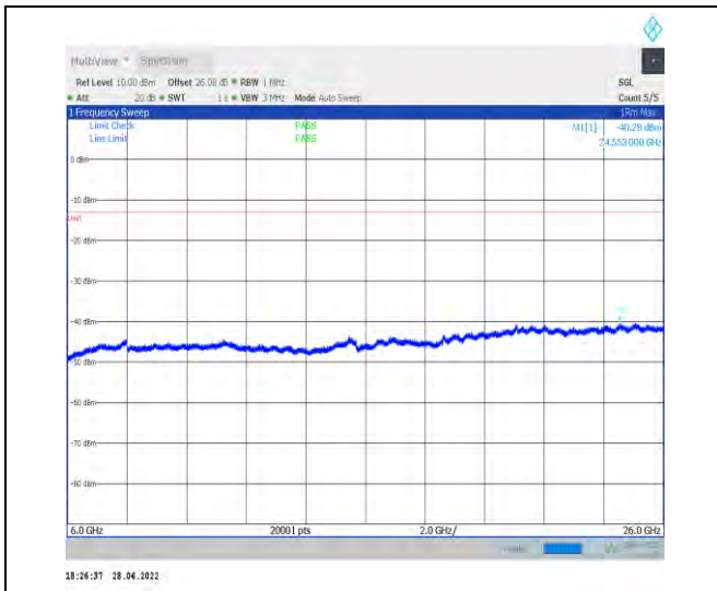
1-N77-3700-3980--30-100-M-1-DFT-QPSK-Edge_1R B_Left-1@0-6000-26000-Ant2--40.28--13-PASS
