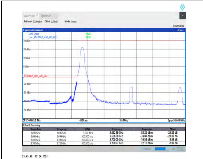
1-N77-3700-3980--30-20-L-4-CP-QPSK-Edge_1RB_Le ft-1@0-Ant2-PASS-see graph
