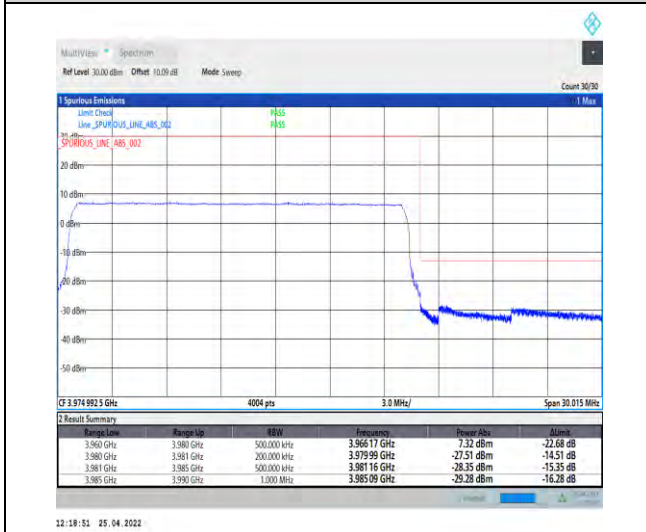
1-N77-3700-3980--30-20-H-6-CP-QPSK-Outer_Full-51@0-Ant1-PASS-see graph
