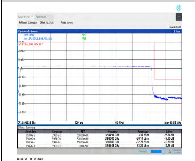
1-N77-3700-3980--30-50-H-6-CP-QPSK-Outer_Full-133@0-Ant1-PASS-see graph
