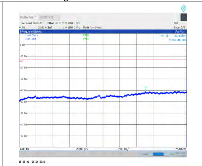
1-N77-3700-3980--30-100-L-1-DFT-QPSK-Edge_1R B_Left-1@0-6000-26000-Ant2--40.46--13-PASS
