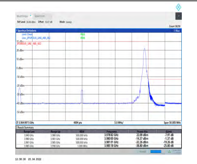
1-N77-3700-3980--30-40-H-5-CP-QPSK-Edge_1RB_Right-1@105-Ant1-PASS-see graph
