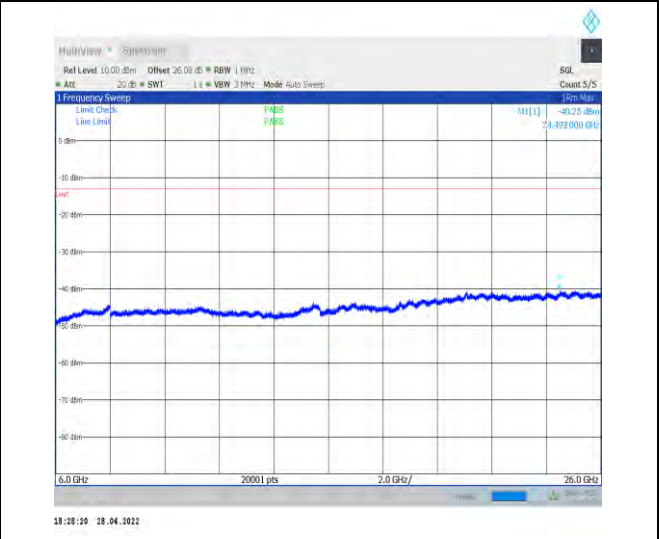
1-N77-3700-3980--30-100-H-1-DFT-QPSK-Edge_1R B_Left-1@0-6000-26000-Ant2--40.25--13-PASS
