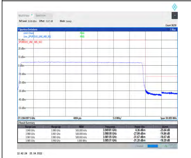
1-N77-3700-3980--30-40-H-6-CP-QPSK-Outer_Full-106@0-Ant1-PASS-see graph
