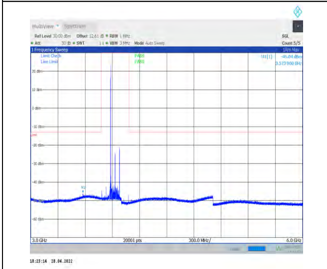
1-N77-3700-3980--30-100-H-1-DFT-QPSK-Edge_1R B_Left-1@0-3000-6000-Ant1--46.04--13-PASS
