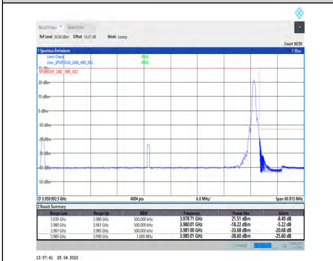
1-N77-3700-3980--30-50-H-5-CP-QPSK-Edge_1RB_Ri ght-1@132-Ant2-PASS-see graph
