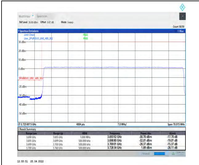
1-N77-3700-3980--30-60-L-6-CP-QPSK-Outer_Full-162@0-Ant1-PASS-see graph
