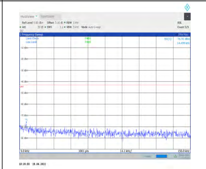
1-N77-3700-3980--30-100-M-1-DFT-QPSK-Edge_1R B_Left-1@0-0.009-0.15-Ant1--76.91--43-PASS
