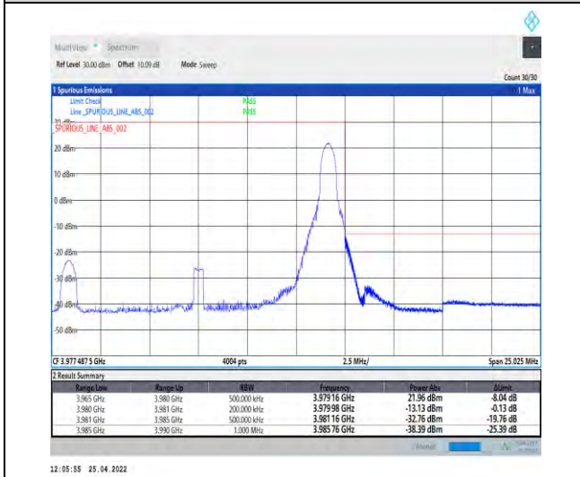
1-N77-3700-3980--30-15-H-5-CP-QPSK-Edge_1RB _Right-1@37-Ant1-PASS-see graph
