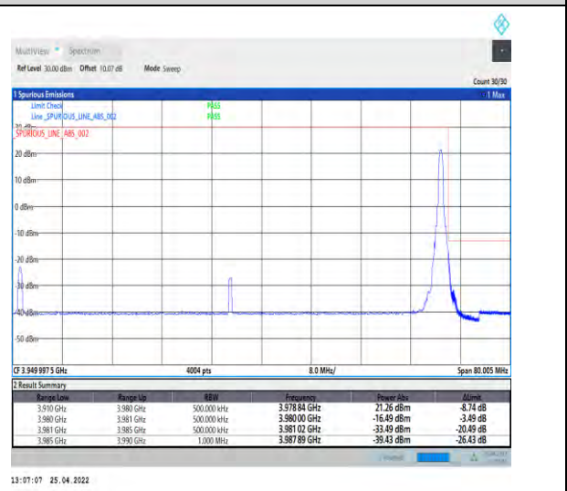
1-N77-3700-3980--30-70-H-5-CP-QPSK-Edge_1RB_Right-1@188-Ant1-PASS-see graph
