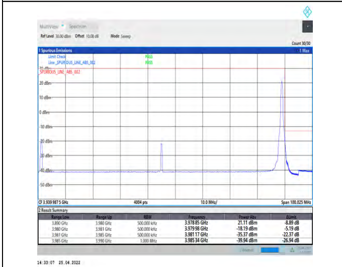
1-N77-3700-3980--30-90-H-5-CP-QPSK-Edge_1RB_Ri ght-1@244-Ant2-PASS-see graph
