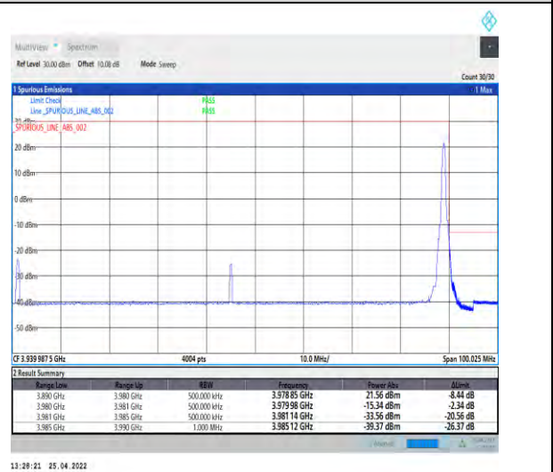
1-N77-3700-3980--30-90-H-5-CP-QPSK-Edge_1RB_Right-1@244-Ant1-PASS-see graph
