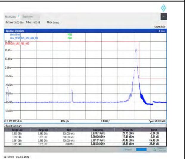
1-N77-3700-3980--30-50-H-5-CP-QPSK-Edge_1RB_Right-1@132-Ant1-PASS-see graph
