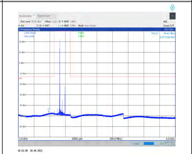
1-N77-3700-3980--30-100-M-1-DFT-QPSK-Edge_1R B_Left-1@0-3000-6000-Ant1--46.61--13-PASS
