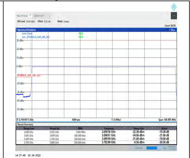
1-N77-3700-3980--30-100-L-6-CP-QPSK-Outer_Full-273@0-Ant2-PASS-see graph
