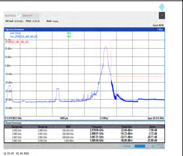
1-N77-3700-3980--30-20-H-5-CP-QPSK-Edge_1RB_Right-1@50-Ant1-PASS-see graph
