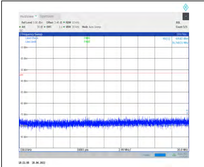
1-N77-3700-3980--30-100-M-1-DFT-QPSK-Edge_1R B_Left-1@0-15-30-Ant1--69.82--33-PASS
