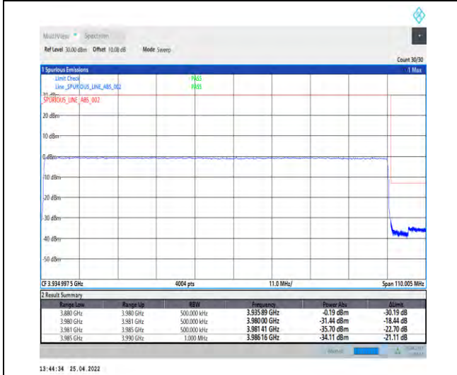
1-N77-3700-3980--30-100-H-6-CP-QPSK-Outer_Ful I-273@0-Ant1-PASS-see graph
