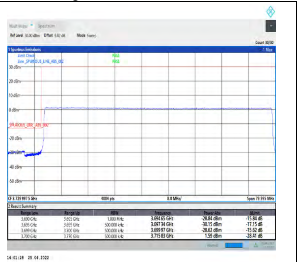
1-N77-3700-3980--30-70-L-6-CP-QPSK-Outer_Ful I-189@0-Ant2-PASS-see graph
