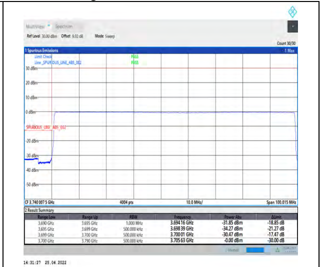
1-N77-3700-3980--30-90-L-6-CP-QPSK-Outer_Ful I-245@0-Ant2-PASS-see graph
