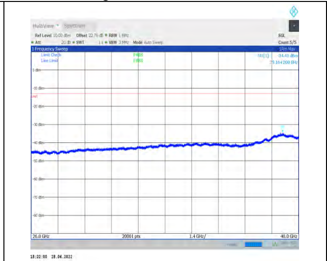
1-N77-3700-3980--30-100-M-1-DFT-QPSK-Edge_1R B_Left-1@0-26000-40000-Ant1--34.41--13-PASS
