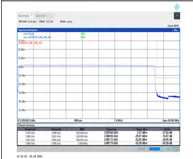
1-N77-3700-3980--30-60-H-6-CP-QPSK-Outer_Full-162@0-Ant1-PASS-see graph
