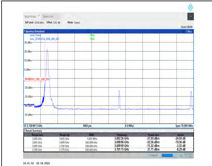
1-N77-3700-3980--30-70-L-4-CP-QPSK-Edge_1RB_Le ft-1@0-Ant2-PASS-see graph
