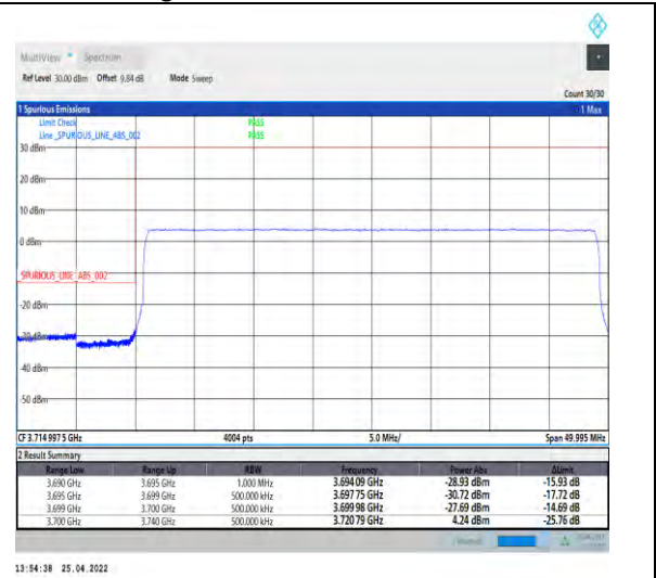
1-N77-3700-3980--30-40-L-6-CP-QPSK-Outer_Ful I-106@0-Ant2-PASS-see graph
