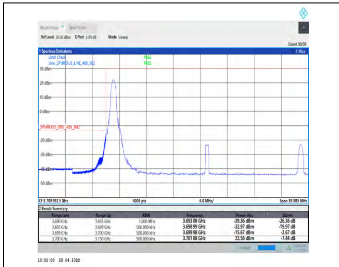
1-N77-3700-3980--30-30-L-4-CP-QPSK-Edge_1RB_Le ft-1@0-Ant2-PASS-see graph
