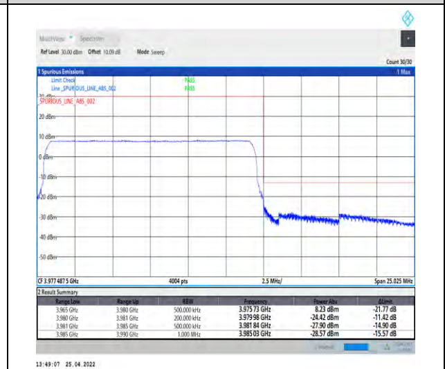
1-N77-3700-3980--30-15-H-6-CP-QPSK-Outer_Fu ll-38@0-Ant2-PASS-see graph
