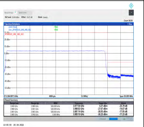
1-N77-3700-3980--30-40-H-6-CP-QPSK-Outer_Fu ll-106@0-Ant2-PASS-see graph
