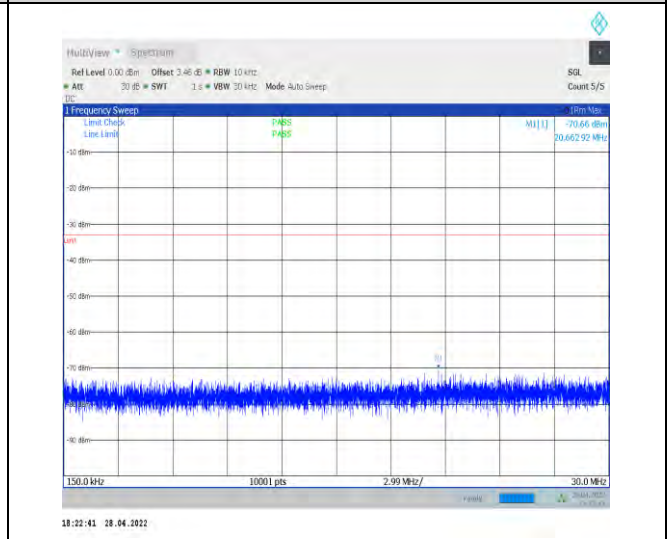
1-N77-3700-3980--30-100-H-1-DFT-QPSK-Edge_1R B_Left-1@0-0.15-30-Ant1--70.66--33-PASS
