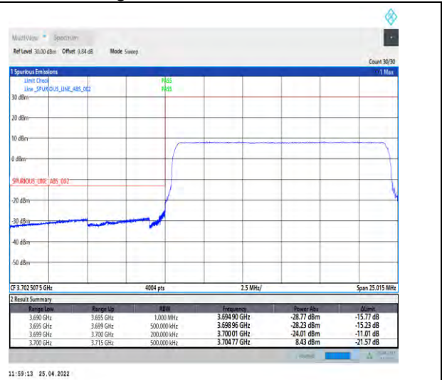
1-N77-3700-3980--30-15-L-6-CP-QPSK-Outer_Full-3 _8@0-Ant1-PASS-see graph
