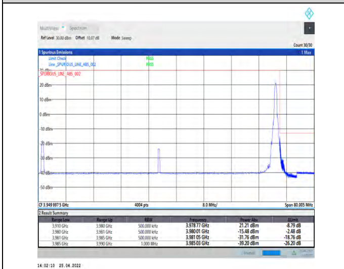
1-N77-3700-3980--30-70-H-5-CP-QPSK-Edge_1RB_Ri ght-1@188-Ant2-PASS-see graph
