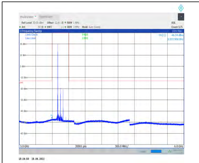
1-N77-3700-3980--30-100-L-1-DFT-QPSK-Edge_1R B_Left-1@0-3000-6000-Ant2--46.94--13-PASS
