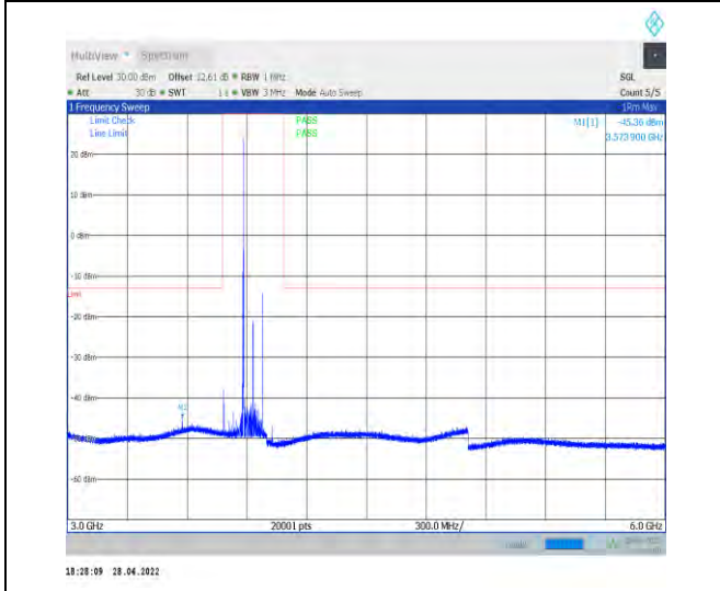
1-N77-3700-3980--30-100-H-1-DFT-QPSK-Edge_1R B_Left-1@0-3000-6000-Ant2--45.36--13-PASS
