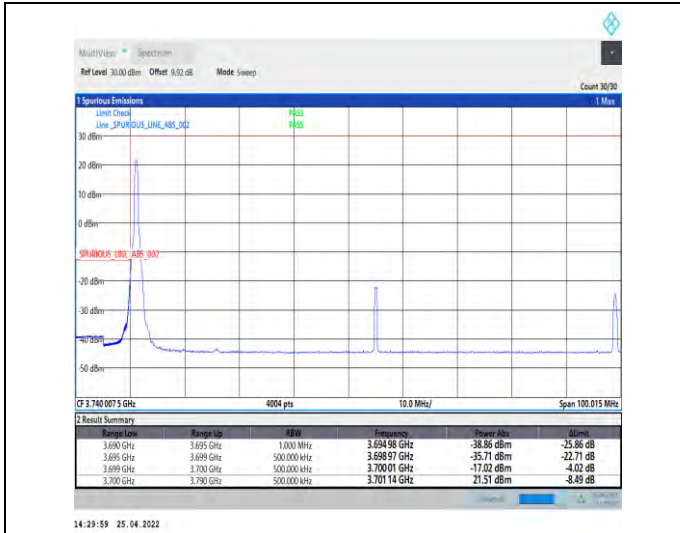
1-N77-3700-3980--30-90-L-4-CP-QPSK-Edge_1RB_Le ft-1@0-Ant2-PASS-see graph
