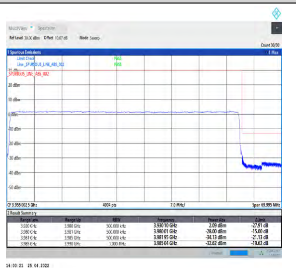
1-N77-3700-3980--30-60-H-6-CP-QPSK-Outer_Fu ll-162@0-Ant2-PASS-see graph
