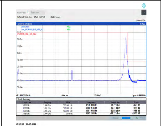
1-N77-3700-3980--30-60-H-5-CP-QPSK-Edge_1RB_Right-1@161-Ant1-PASS-see graph
