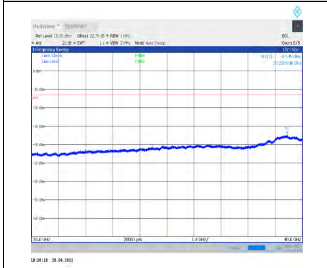
1-N77-3700-3980--30-100-L-1-DFT-QPSK-Edge_1R B_Left-1@0-26000-40000-Ant1--34.49--13-PASS
