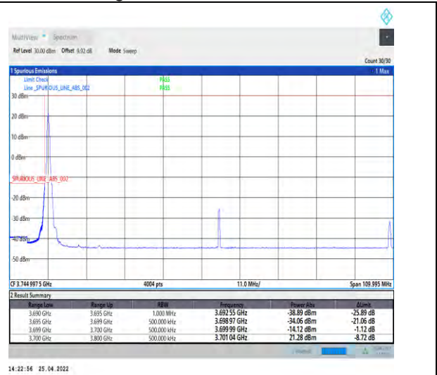
1-N77-3700-3980--30-100-L-4-CP-QPSK-Edge_1RB _Left-1@0-Ant1-PASS-see graph
