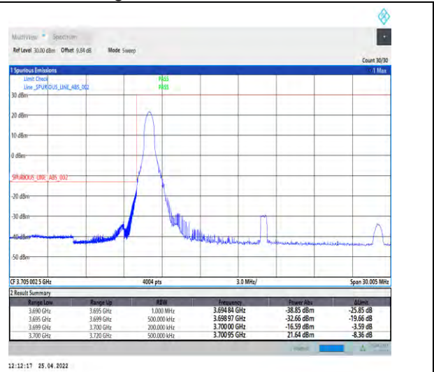
1-N77-3700-3980--30-20-L-4-CP-QPSK-Edge_1RB_Left-1@0-Ant1-PASS-see graph
