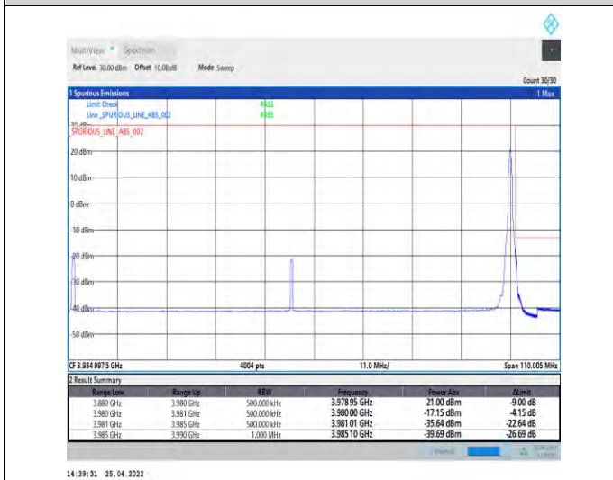
1-N77-3700-3980--30-100-H-5-CP-QPSK-Edge_1RB_Right-1@272-Ant2-PASS-see graph
