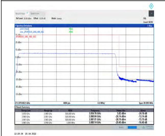
1-N77-3700-3980--30-30-H-6-CP-QPSK-Outer_Full-78@0-Ant1-PASS-see graph
