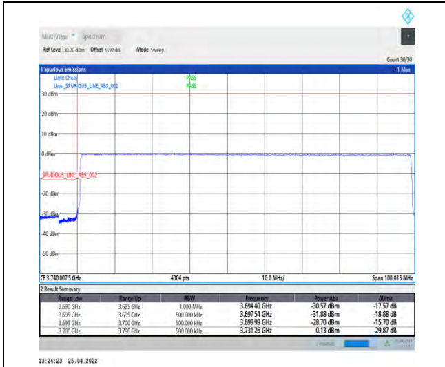
1-N77-3700-3980--30-90-L-6-CP-QPSK-Outer_Full-245@0-Ant1-PASS-see graph
