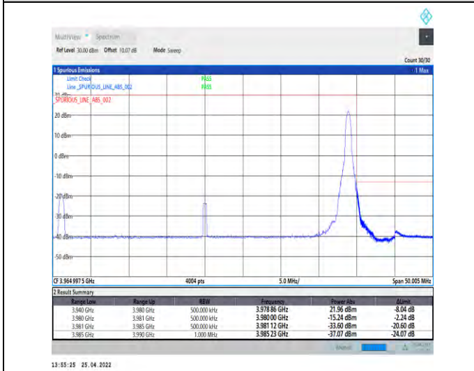
1-N77-3700-3980--30-40-H-5-CP-QPSK-Edge_1RB_Ri ght-1@105-Ant2-PASS-see graph
