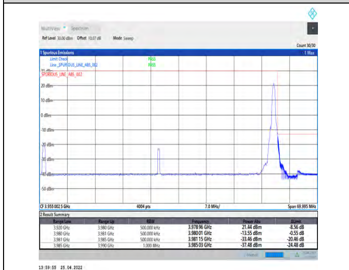
1-N77-3700-3980--30-60-H-5-CP-QPSK-Edge_1RB_Ri ght-1@161-Ant2-PASS-see graph
