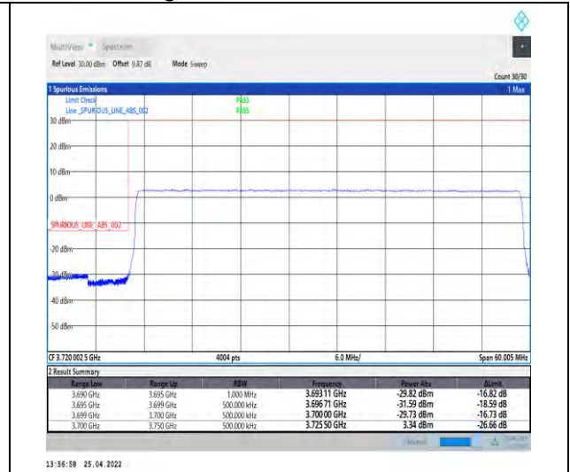
1-N77-3700-3980--30-50-L-6-CP-QPSK-Outer_Ful I-133@0-Ant2-PASS-see graph
