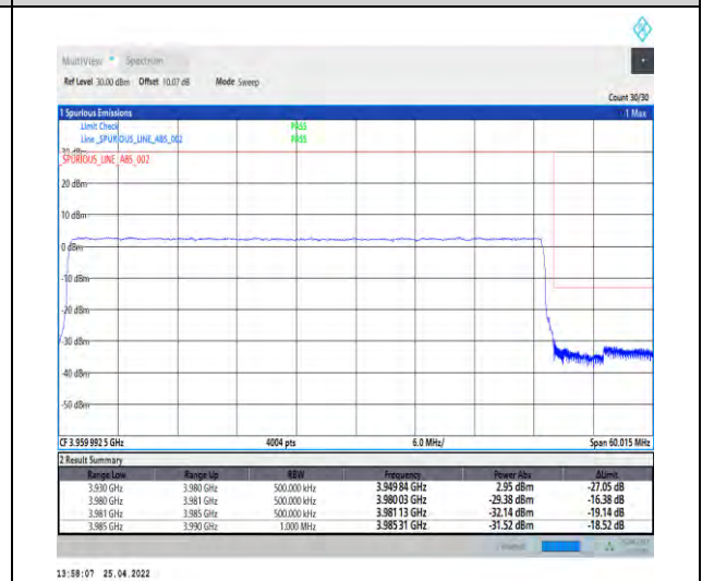
1-N77-3700-3980--30-50-H-6-CP-QPSK-Outer_Fu ll-133@0-Ant2-PASS-see graph
