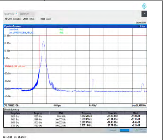
1-N77-3700-3980--30-30-L-4-CP-QPSK-Edge_1RB_Left-1@0-Ant1-PASS-see graph
