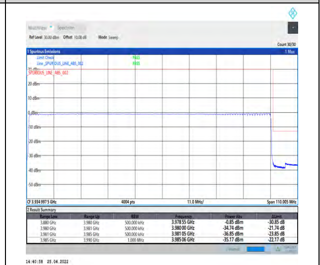
1-N77-3700-3980--30-100-H-6-CP-QPSK-Outer_Full-273@0-Ant2-PASS-see graph
