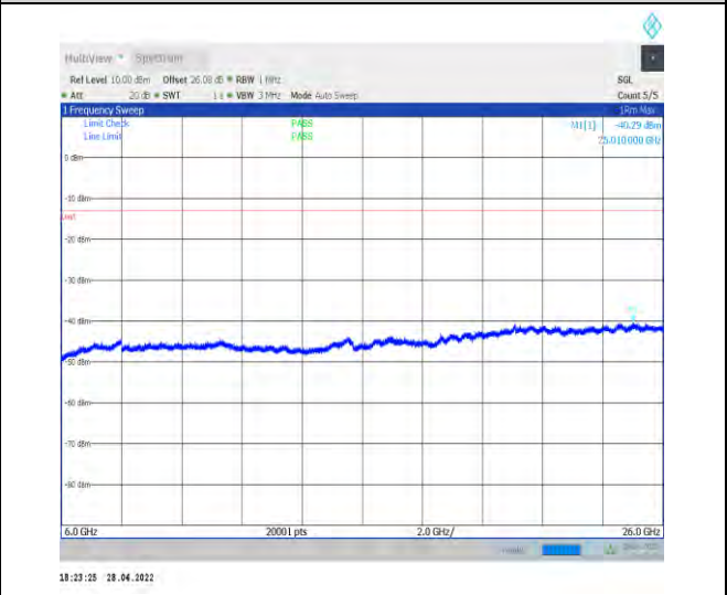
1-N77-3700-3980--30-100-H-1-DFT-QPSK-Edge_1R B_Left-1@0-6000-26000-Ant1--40.29--13-PASS
