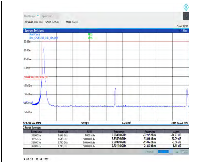
1-N77-3700-3980--30-80-L-4-CP-QPSK-Edge_1RB_Le ft-1@0-Ant2-PASS-see graph
