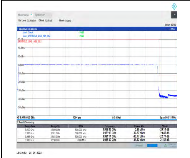
1-N77-3700-3980--30-80-H-6-CP-QPSK-Outer_Full-217@0-Ant1-PASS-see graph
