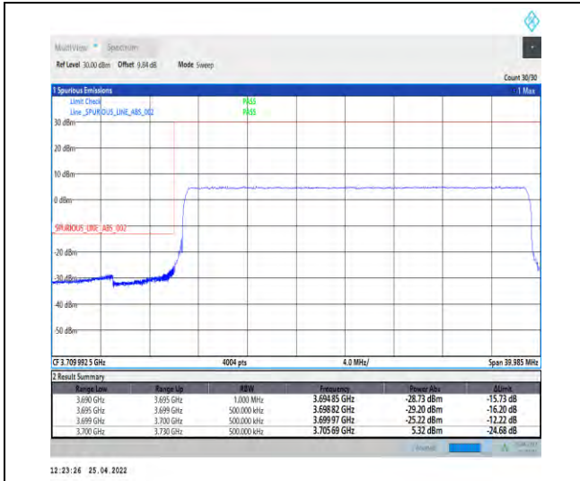
1-N77-3700-3980--30-30-L-6-CP-QPSK-Outer_Full-78@0-Ant1-PASS-see graph
