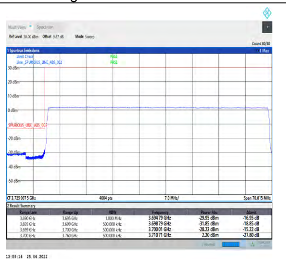
1-N77-3700-3980--30-60-L-6-CP-QPSK-Outer_Ful I-162@0-Ant2-PASS-see graph
