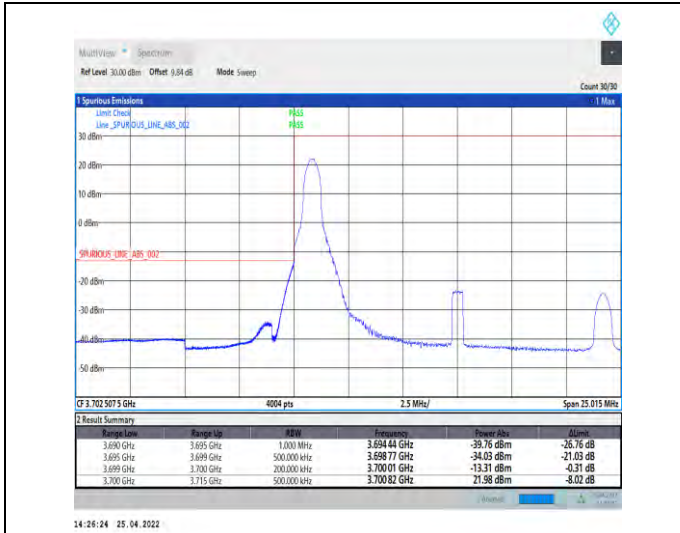
1-N77-3700-3980--30-15-L-4-CP-QPSK-Edge_1RB_Le ft-1@0-Ant2-PASS-see graph
