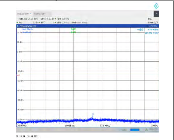
1-N77-3700-3980--30-100-M-1-DFT-QPSK-Edge_1R B_Left-1@0-30-1000-Ant2--67.69--23-PASS
