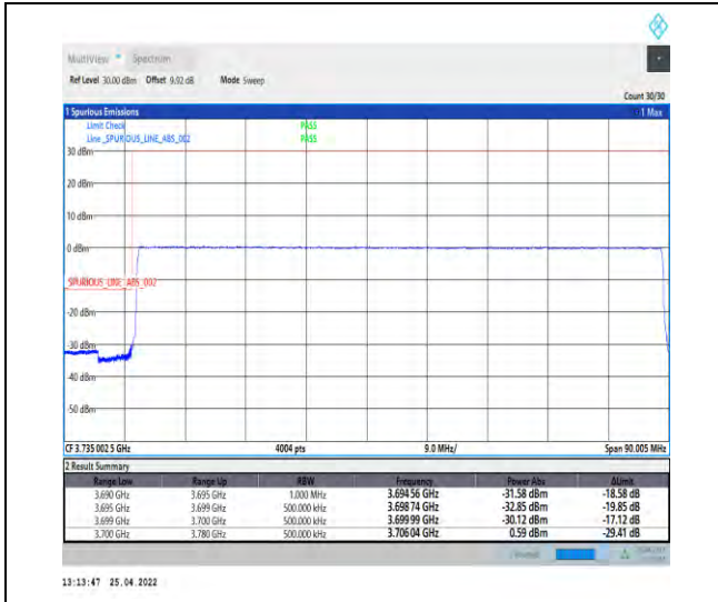
1-N77-3700-3980--30-80-L-6-CP-QPSK-Outer_Full-217@0-Ant1-PASS-see graph
