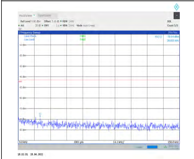
1-N77-3700-3980--30-100-H-1-DFT-QPSK-Edge_1R B_Left-1@0-0.009-0.15-Ant1--78.04--43-PASS
