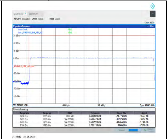
1-N77-3700-3980--30-80-L-6-CP-QPSK-Outer_Ful I-217@0-Ant2-PASS-see graph
