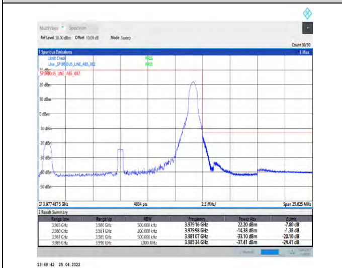
1-N77-3700-3980--30-15-H-5-CP-QPSK-Edge_1RB_Ri ght-1@37-Ant2-PASS-see graph
