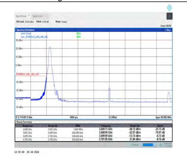
1-N77-3700-3980--30-40-L-4-CP-QPSK-Edge_1RB_Left-1@0-Ant1-PASS-see graph
