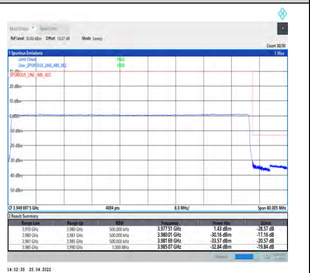
1-N77-3700-3980--30-70-H-6-CP-QPSK-Outer_Fu ll-189@0-Ant2-PASS-see graph
