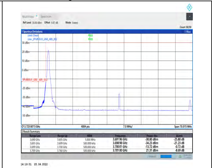
1-N77-3700-3980--30-60-L-4-CP-QPSK-Edge_1RB_Left-1@0-Ant1-PASS-see graph
