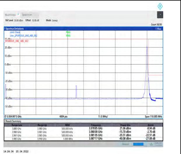
1-N77-3700-3980--30-100-H-5-CP-QPSK-Edge_1RB _Right-1@272-Ant1-PASS-see graph
