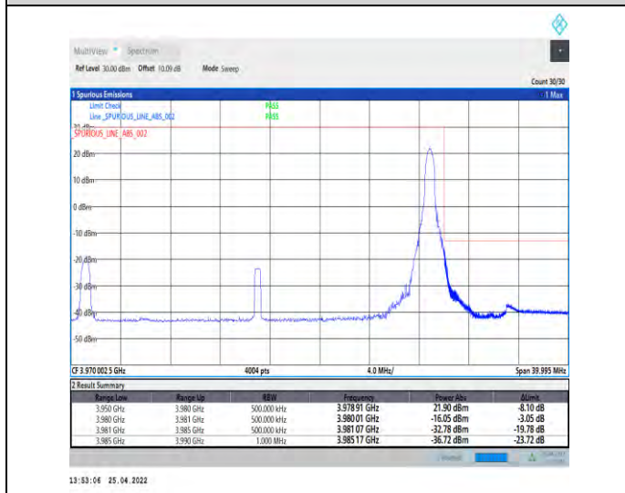
1-N77-3700-3980--30-30-H-5-CP-QPSK-Edge_1RB_Ri ght-1@77-Ant2-PASS-see graph
