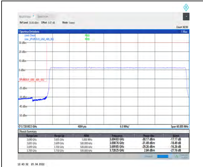
1-N77-3700-3980--30-50-L-6-CP-QPSK-Outer_Full-133@0-Ant1-PASS-see graph
