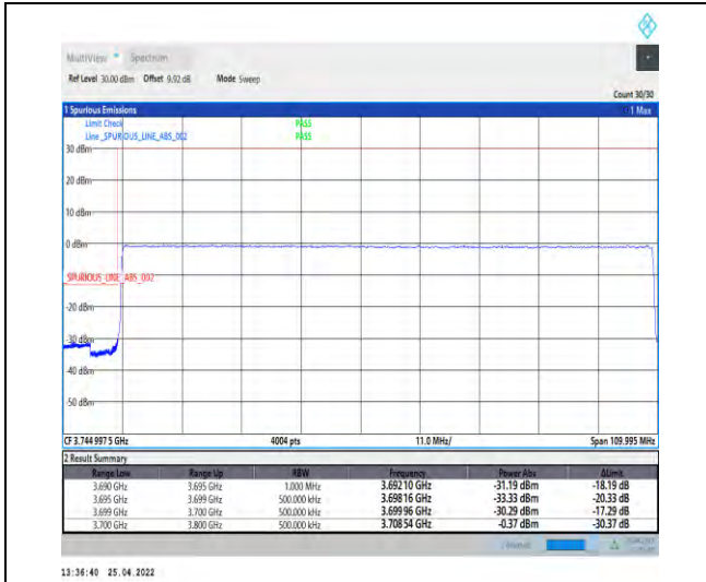
1-N77-3700-3980--30-100-L-6-CP-QPSK-Outer_Ful I-273@0-Ant1-PASS-see graph
