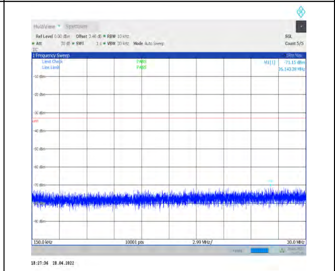
1-N77-3700-3980--30-100-H-1-DFT-QPSK-Edge_1R B_Left-1@0-0.15-30-Ant2--71.15--33-PASS
