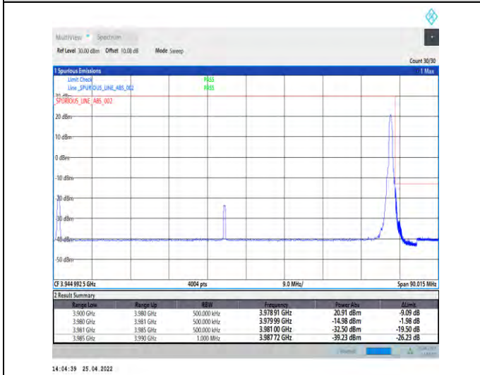
1-N77-3700-3980--30-80-H-5-CP-QPSK-Edge_1RB_Ri ght-1@216-Ant2-PASS-see graph
