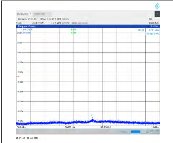
1-N77-3700-3980--30-100-H-1-DFT-QPSK-Edge_1R B_Left-1@0-30-1000-Ant2--67.61--23-PASS
