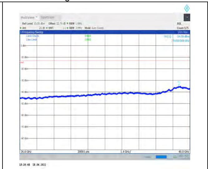
1-N77-3700-3980--30-100-M-1-DFT-QPSK-Edge_1R B_Left-1@0-26000-40000-Ant2--34.58--13-PASS
