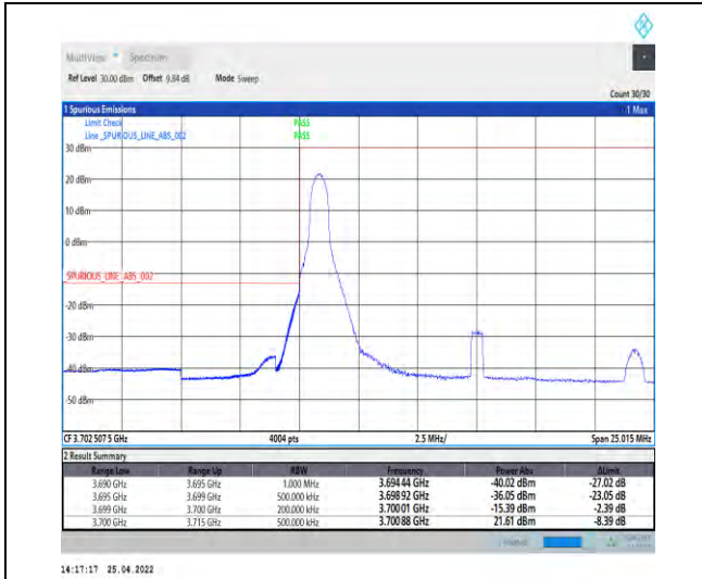
1-N77-3700-3980--30-15-L-4-CP-QPSK-Edge_1RB _Left-1@0-Ant1-PASS-see graph
