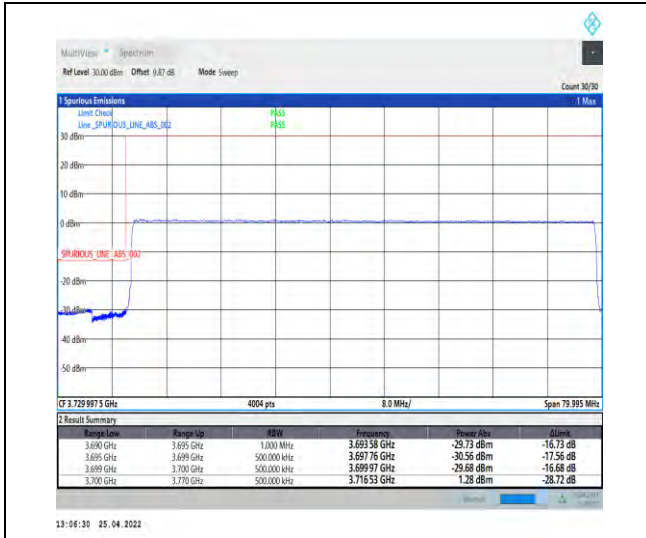
1-N77-3700-3980--30-70-L-6-CP-QPSK-Outer_Full-189@0-Ant1-PASS-see graph
