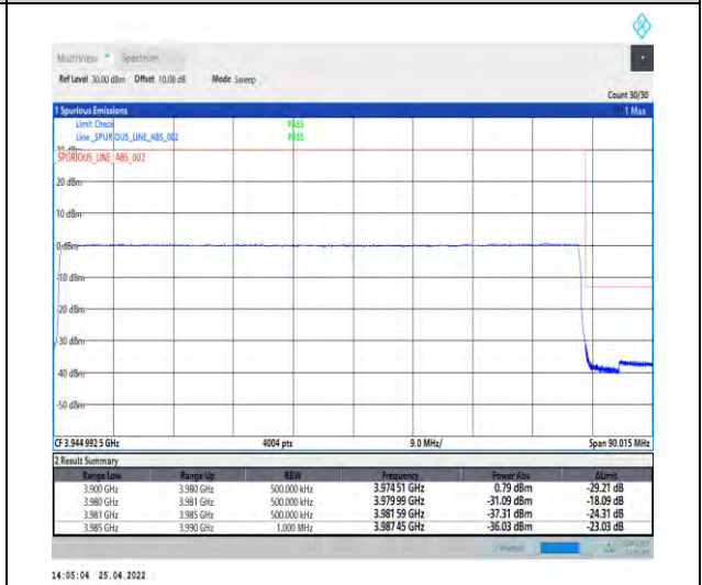
1-N77-3700-3980--30-80-H-6-CP-QPSK-Outer_Fu ll-217@0-Ant2-PASS-see graph
