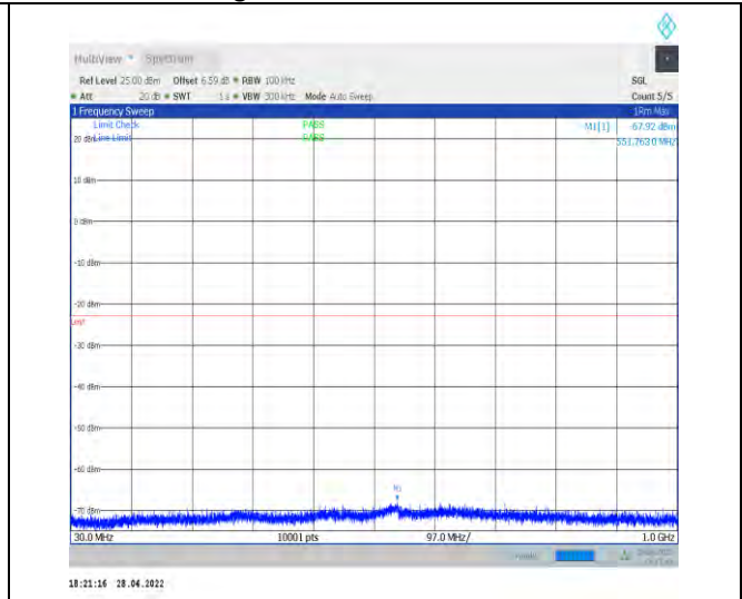
1-N77-3700-3980--30-100-M-1-DFT-QPSK-Edge_1R B_Left-1@0-30-1000-Ant1--67.92--23-PASS
