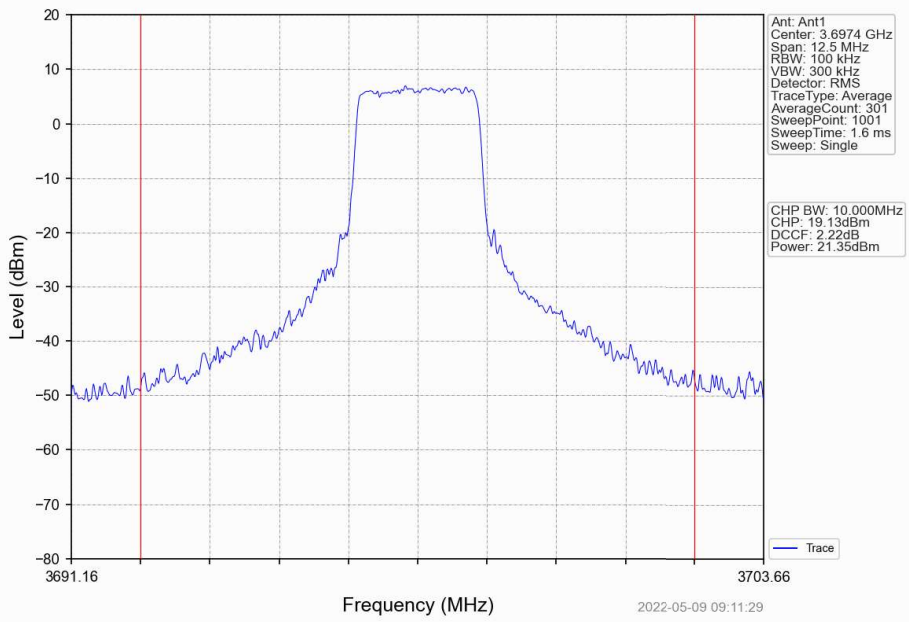
Band48_5MHz_QPSK_HCH_3697.5MHz_RB_12_13_NTNV
