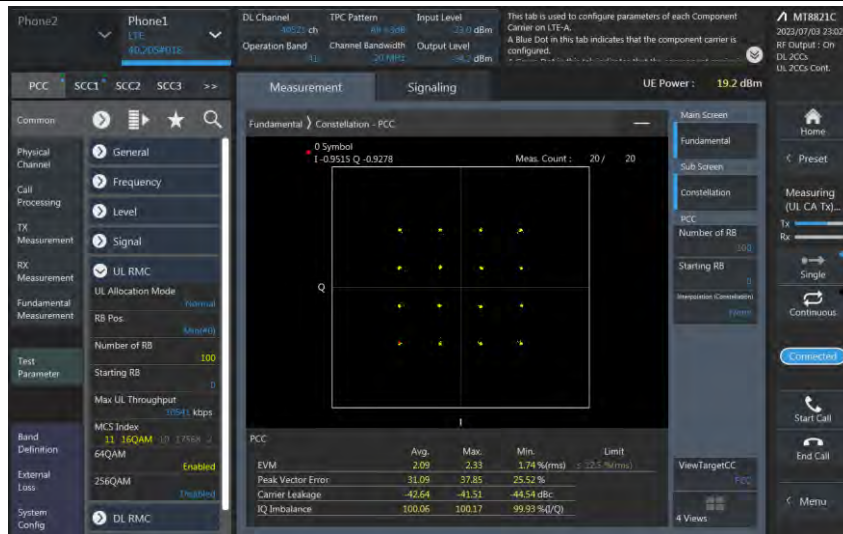
41-41-20MHz-20MHz-16QAM-16QAM-40521-40719-100RB#0-100RB#0
