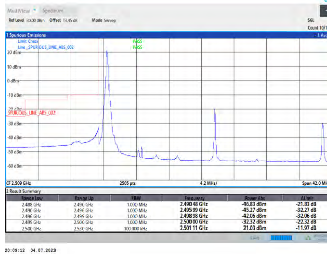
7-7-10MHz-20MHz-QPSK-QPSK-20805-20949-50RB#0-100RB#0
