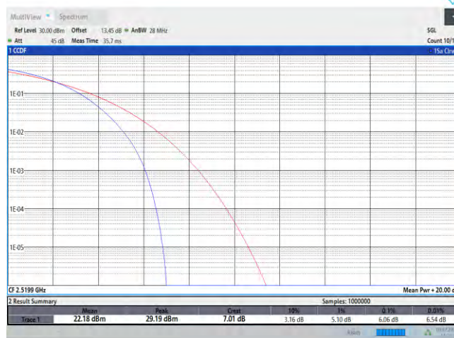
7-7-20MHz-20MHz-QPSK-QPSK-21001-21199-100RB#0-100RB#0
