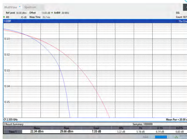
7-7-20MHz-20MHz-QPSK-QPSK-21001-21199-100RB#0-100RB#0
