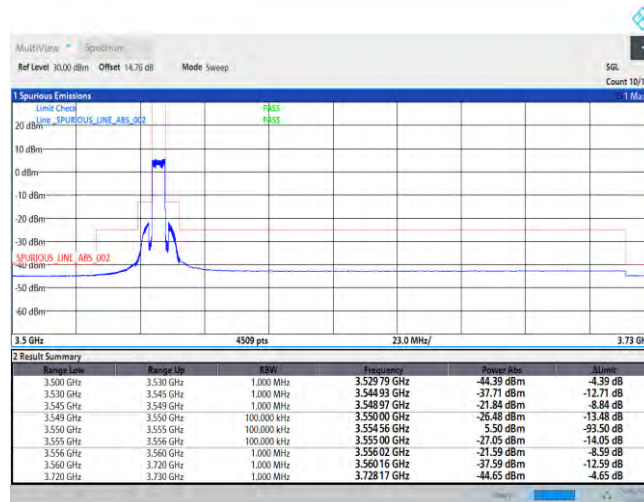
Band48-5MHz-QPSK-55265-25RB#0
