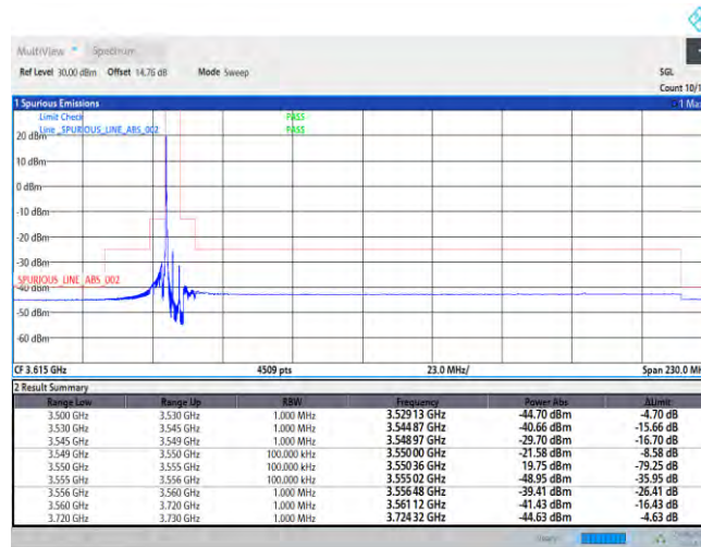
Band48-5MHz-QPSK-55265-1RB#0
