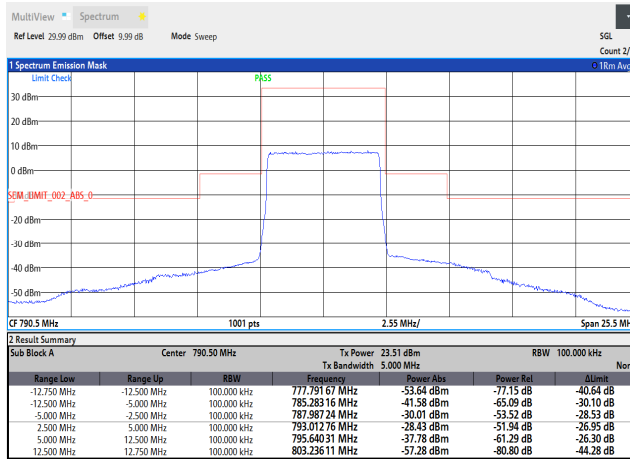
Band14-5MHz-QPSK-23305-25RB#0
