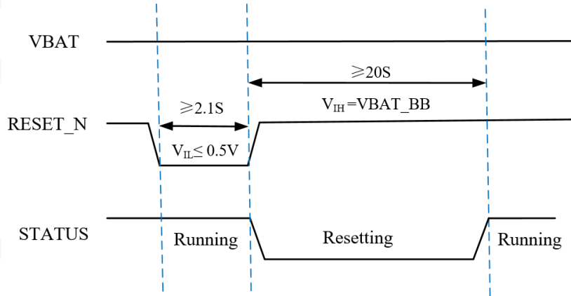
Figure 5-7 Reset timing
