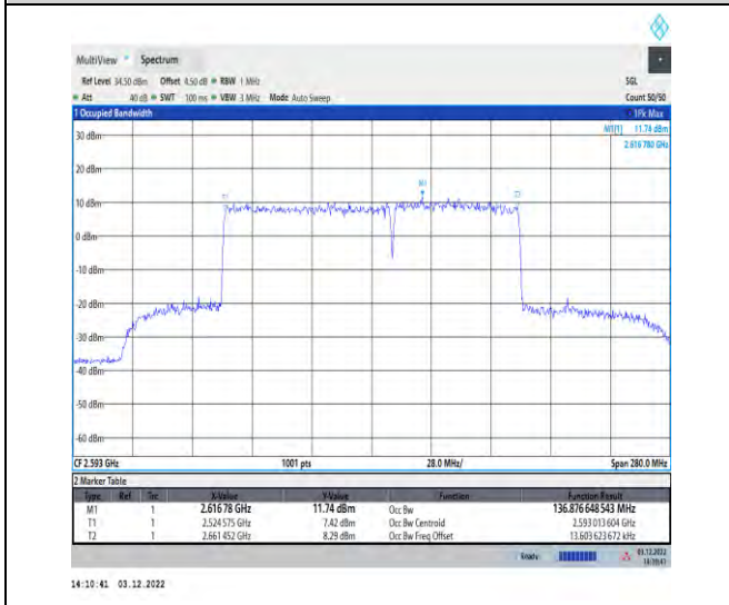
1-41-41-80+60-M-7-DFT-16QAM-Outer_Full
