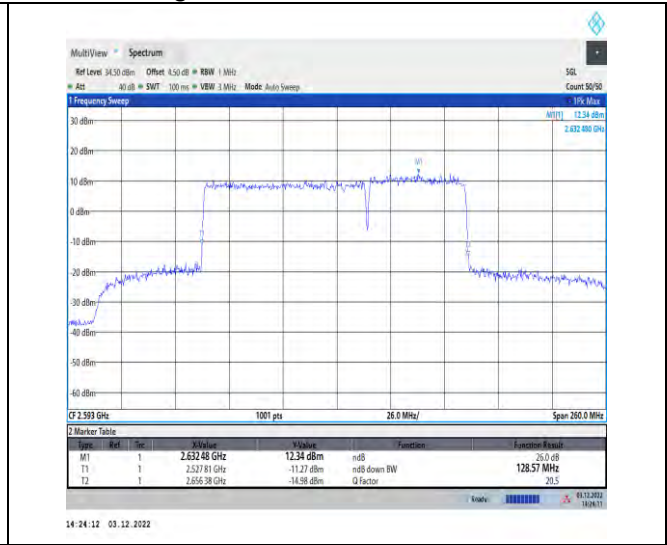
1-41-41-80+50-M-4-DFT-16QAM-Outer_Full
