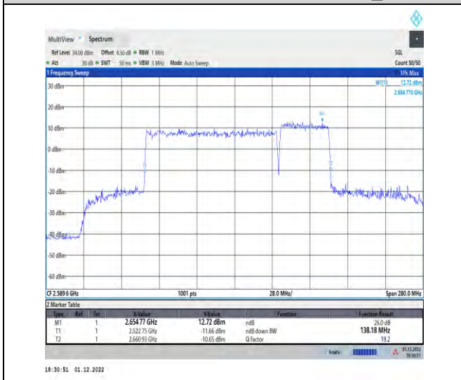
1-41-41-100+40-M-5-DFT-QPSK-Outer_Full
