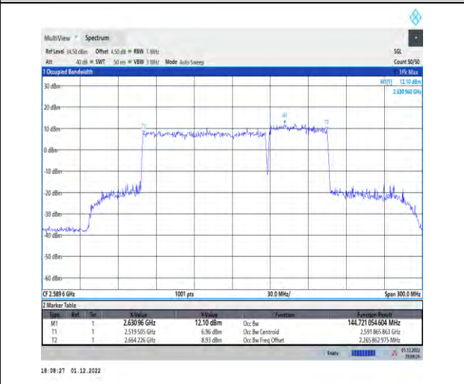
1-41-41-100+50-M-8-DFT-QPSK-Outer_Full
