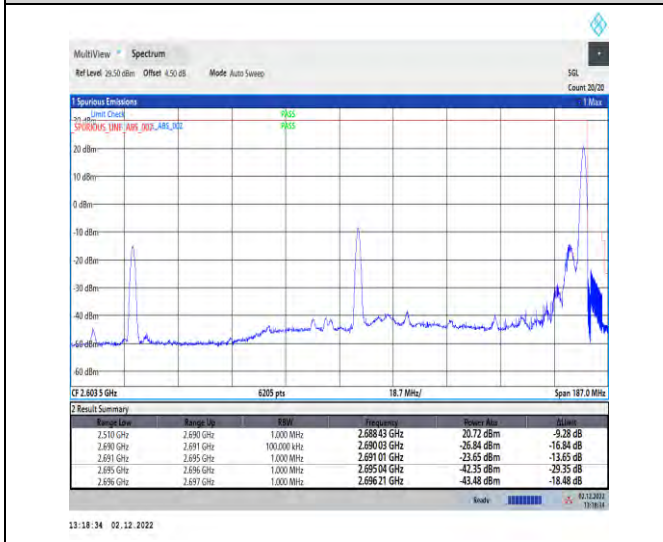
1-41-41-30-80+80-H-2-DFT-QPSK-Edge_1RB_Right
