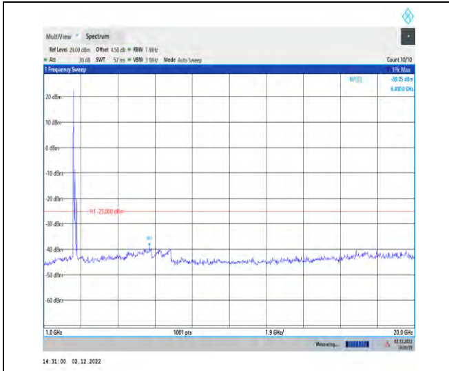
1-41-41-30-100-M-1-DFT-QPSK-Inner_1RB_Left-1 @1-1000-20000
