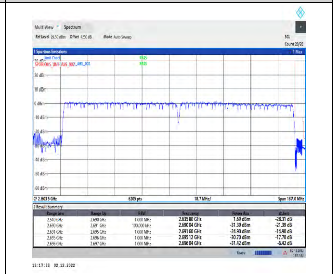
1-41-41-30-80+80-H-3-DFT-QPSK-Outer_Full
