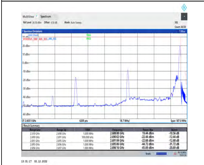
1-41-41-30-60+60-H-5-CP-QPSK-Edge_1RB_Right
