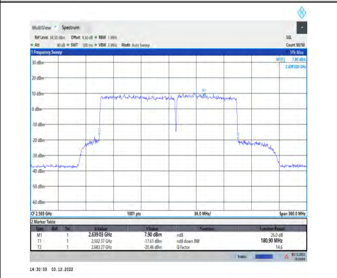
1-41-41-100+80-M-6-DFT-16QAM-Outer_Full
