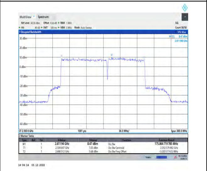
1-41-41-100+80-M-6-DFT-16QAM-Outer_Full
