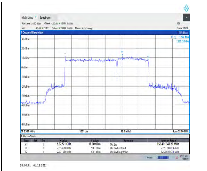
1-41-41-100+60-M-3-DFT-QPSK-Outer_Full
