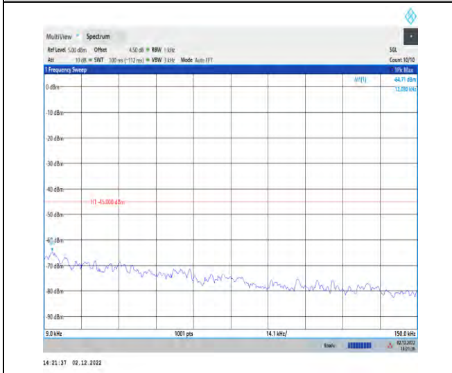
1-41-41-30-100-M-1-DFT-QPSK-Inner_1RB_Left-1 @1-0.009-0.15
