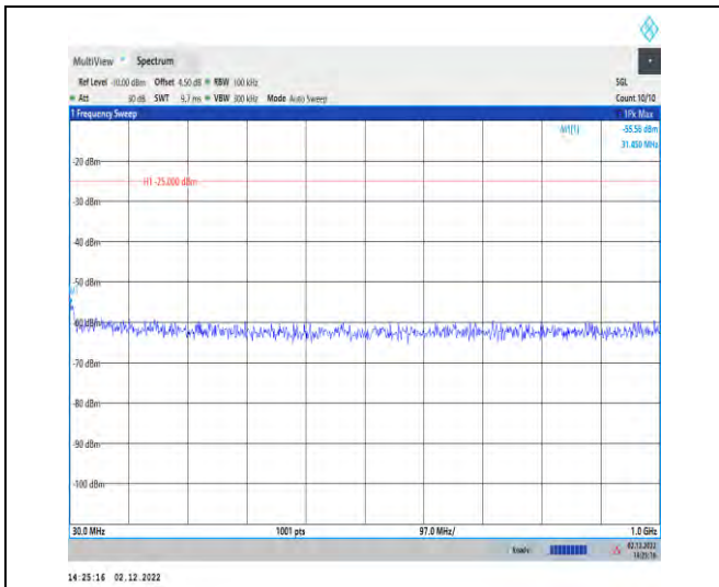
1-41-41-30-100-H-1-DFT-QPSK-Inner_1RB_Left-1@ 1-30-1000
