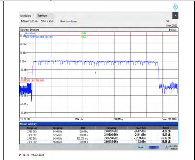
1-41-41-30-80+80-L-6-CP-QPSK-Outer_Full
