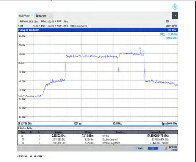
1-41-41-100+50-M-8-DFT-16QAM-Outer_Full
