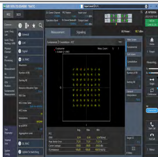
1-41-41-30-100-M-8-CP-64QAM-Outer_Full-273@0-Ant1-see graph-PASS
