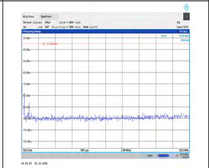
1-41-41-30-100-M-1-DFT-QPSK-Inner_1RB_Left-1@ 1-0.15-30
