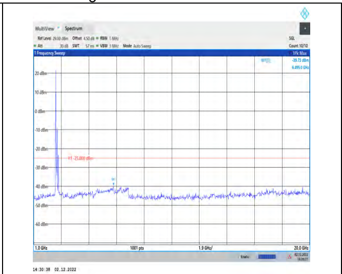
1-41-41-30-100-H-1-DFT-QPSK-Inner_1RB_Left-1@ 1-1000-20000
