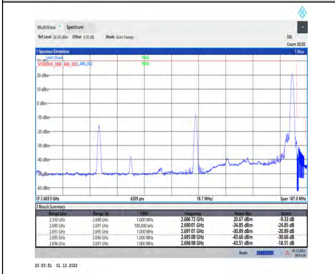
1-41-41-30-100+40-H-1-DFT-QPSK-Edge_1RB_Right
