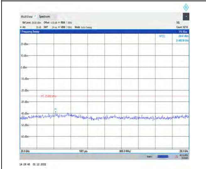
1-41-41-30-100-H-1-DFT-QPSK-Inner_1RB_Left-1@ 1-20000-28000
