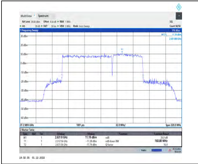
1-41-41-100+60-M-3-DFT-16QAM-Outer_Full
