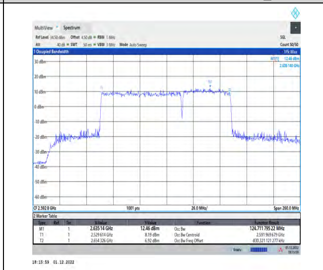
1-41-41-80+50-M-4-DFT-QPSK-Outer_Full
