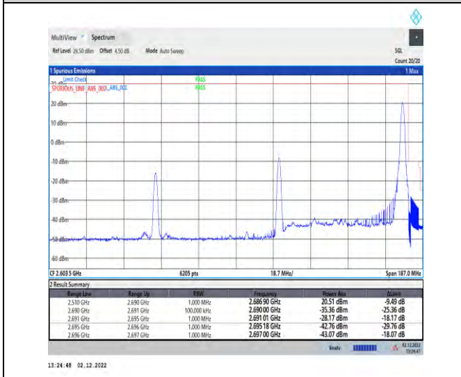
1-41-41-30-80+50-H-2-DFT-QPSK-Edge_1RB_Right
