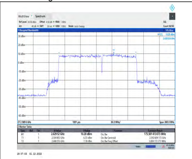
1-41-41-100+80-M-6-DFT-QPSK-Outer_Full
