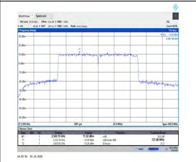
1-41-41-60+60-M-6-DFT-16QAM-Outer_Full
