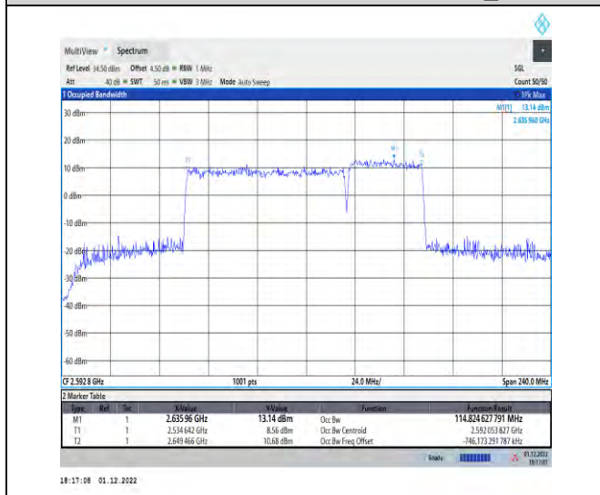
1-41-41-80+40-M-9-DFT-QPSK-Outer_Full
