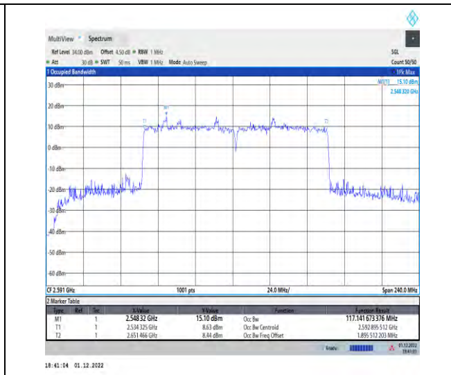
1-41-41-60+60-M-6-DFT-QPSK-Outer_Full
