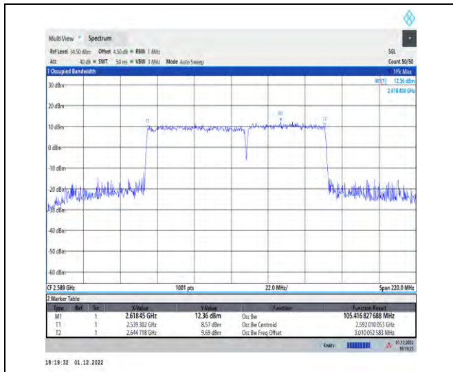
1-41-41-60+50-M-3-DFT-QPSK-Outer_Full
