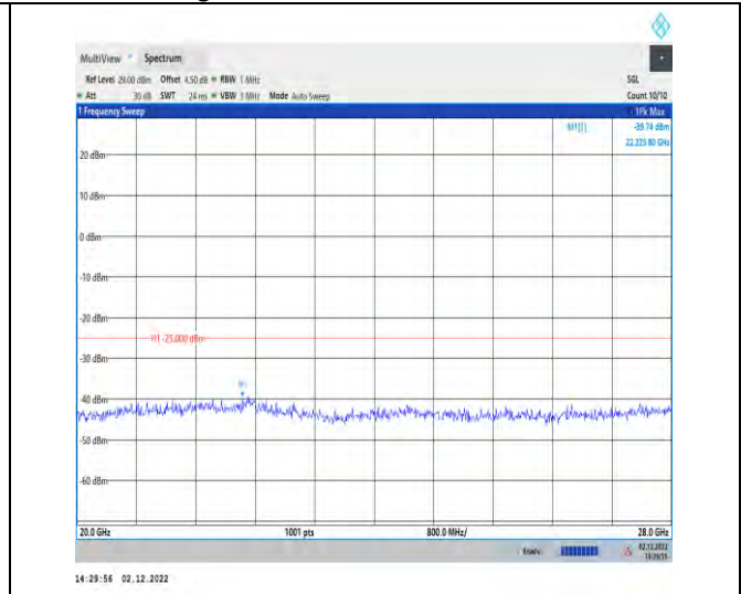
1-41-41-30-100-M-1-DFT-QPSK-Inner_1RB_Left-1@ 1-20000-28000
