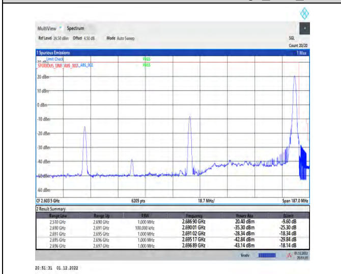
1-41-41-30-100+50-H-2-DFT-QPSK-Edge_1RB_Right
