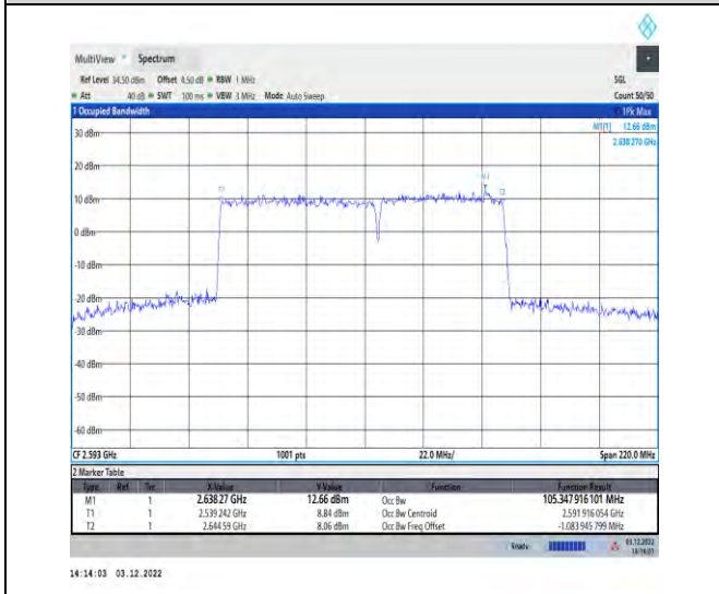
1-41-41-60+50-M-3-DFT-16QAM-Outer_Full
