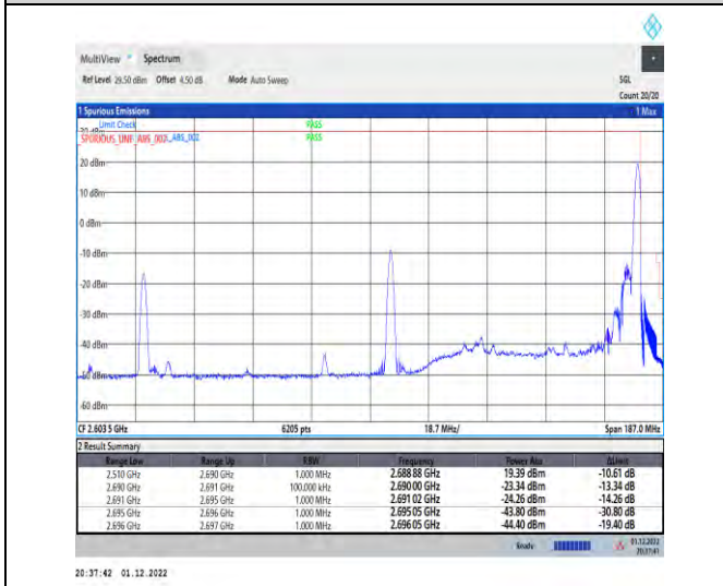
1-41-41-30-100+60-H-1-DFT-QPSK-Edge_1RB_Right
