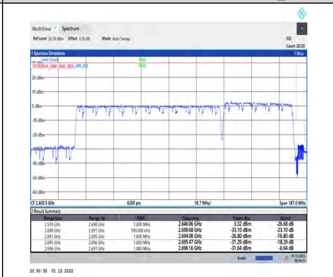
1-41-41-30-100+50-H-3-DFT-QPSK-Outer_Full
