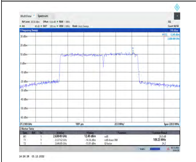
1-41-41-60+50-M-3-DFT-16QAM-Outer_Full
