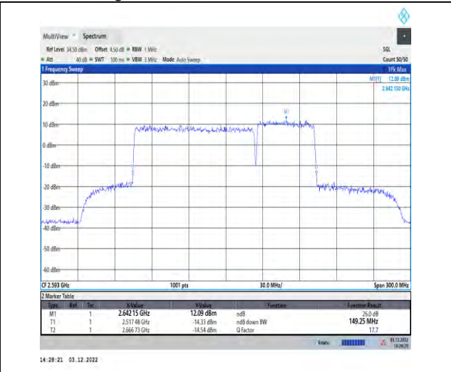
1-41-41-100+50-M-8-DFT-16QAM-Outer_Full
