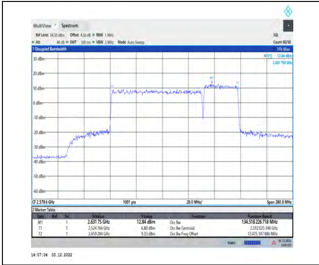
1-41-41-100+40-M-5-DFT-16QAM-Outer_Full
