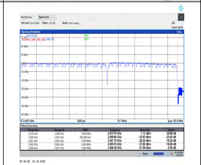
1-41-41-30-100+80-H-3-DFT-QPSK-Outer_Full
