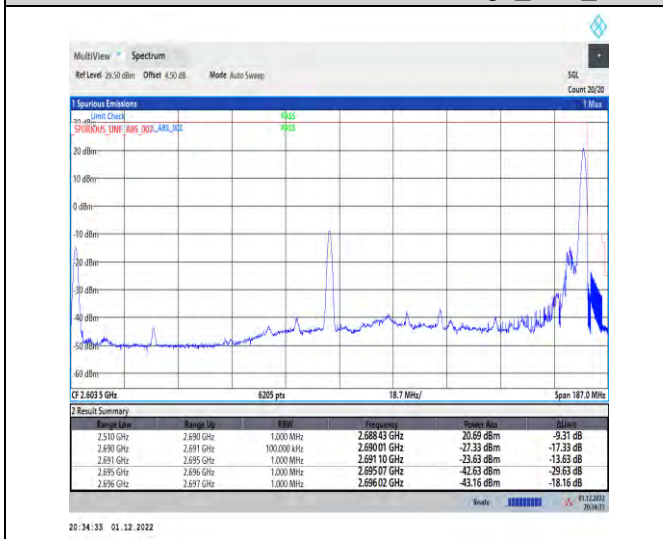
1-41-41-30-100+80-H-2-DFT-QPSK-Edge_1RB_Right
