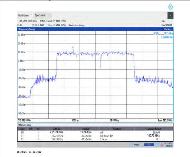
1-41-41-80+80-M-1-DFT-QPSK-Outer_Full
