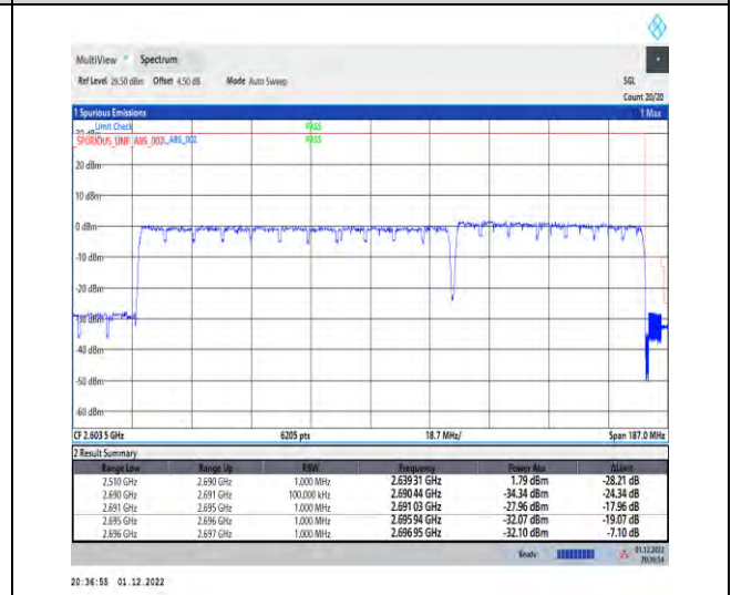
1-41-41-30-100+60-H-L-3-DFT-QPSK-Outer_Full
