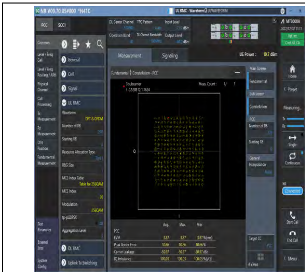
1-41-41-30-100-M-5-DFT-256QAM-Outer_Full-270@0-Ant1-see graph-PASS
