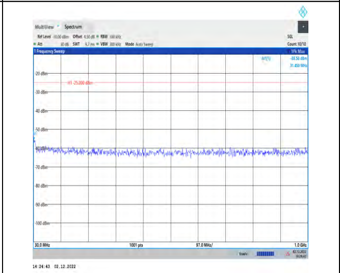
1-41-41-30-100-M-1-DFT-QPSK-Inner_1RB_Left-1@ 1-30-1000
