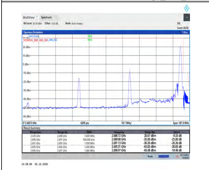
1-41-41-30-80+40-H-4-CP-QPSK-Edge_1RB_Right
