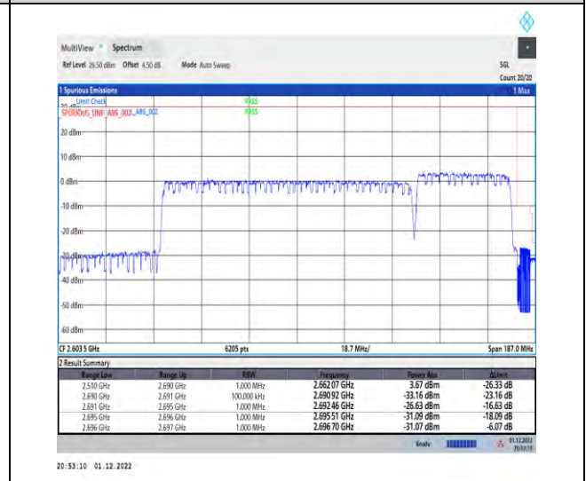
1-41-41-30-100+40-H-3-DFT-QPSK-Outer_Full
