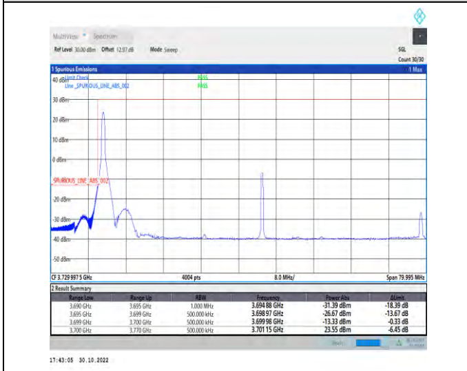
1-N77-3700-3980-PC2-30-70-L-4-CP-QPSK-Edge_1RB_Left-1@0-Ant1-1--PASS-see graph
