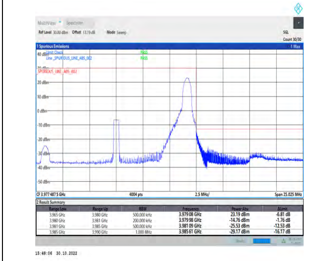
1-N77-3700-3980-PC2-30-15-H-5-CP-QPSK-Edge_1RB_Right-1@37-Ant1-1--PASS-see graph
