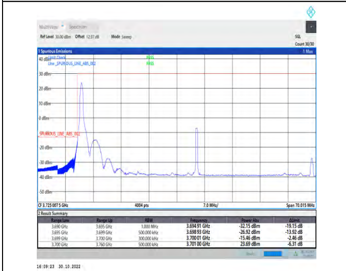
1-N77-3700-3980-PC2-30-60-L-4-CP-QPSK-Edge_1RB_Left-1@0-Ant1-1--PASS-see graph
