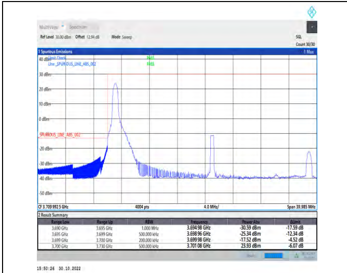
1-N77-3700-3980-PC2-30-30-L-1-DFT-PI2BPSK-Edge_1RB_Left-1@0-Ant1-1--PASS-see graph
