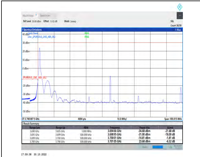
1-N77-3700-3980-PC2-30-90-L-1-DFT-PI2BPSK-Edge_1RB_Left-1@0-Ant1-1--PASS-see graph
