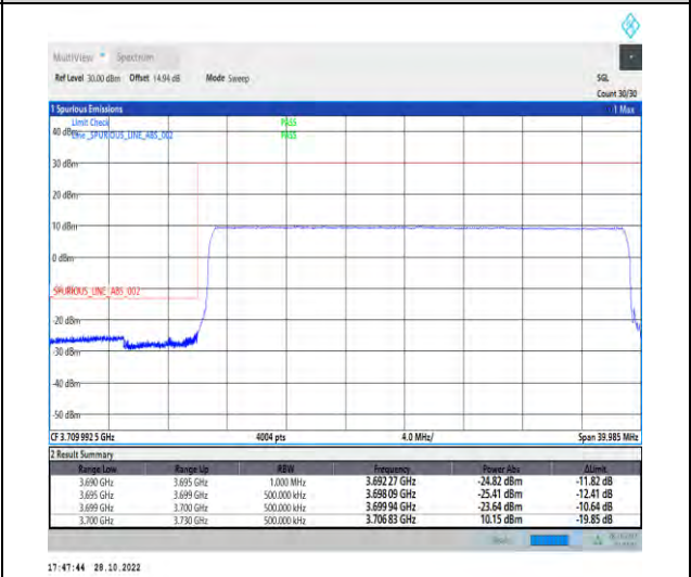
1-N77-3700-3980-PC2-30-30-L-6-CP-QPSK-Outer_Full-78@0-Ant1-1--PASS-see graph
