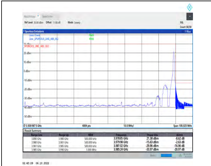
1-N77-3700-3980-PC2-30-90-H-2-DFT-QPSK-Edge_1 RB_Right-1@244-Ant1-1--PASS-see graph
