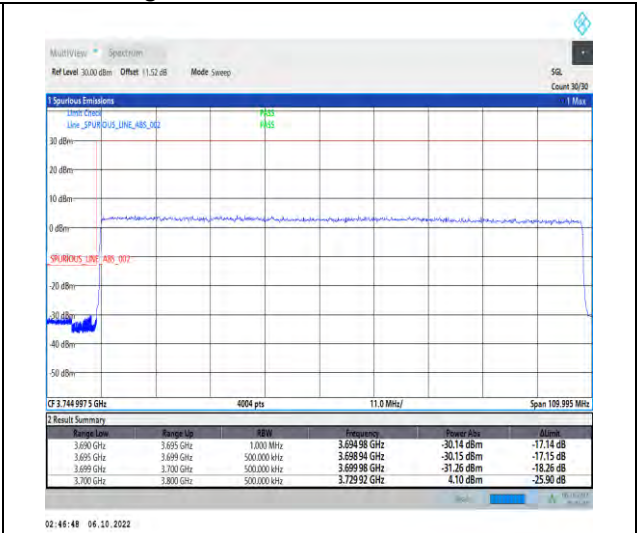
1-N77-3700-3980-PC2-30-100-L-3-DFT-QPSK-Out er_Full-270@0-Ant1-1--PASS-see graph
