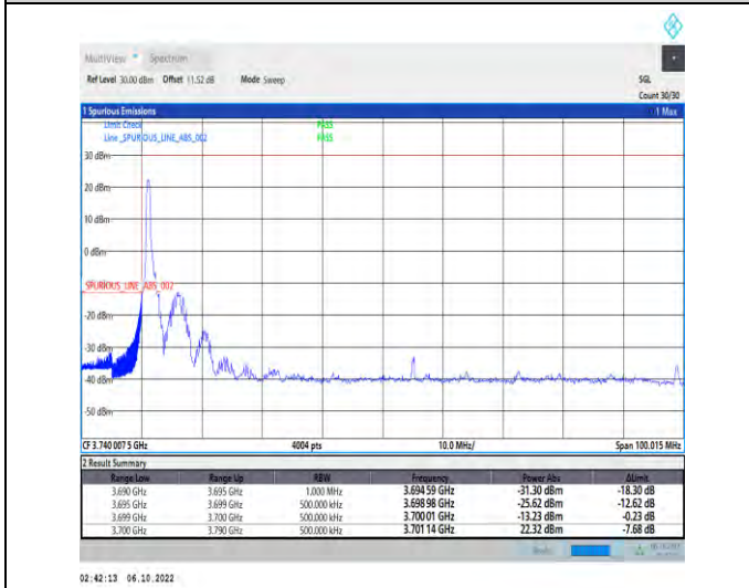
1-N77-3700-3980-PC2-30-90-L-4-CP-QPSK-Edge_1R B_Left-1@0-Ant1-1--PASS-see graph
