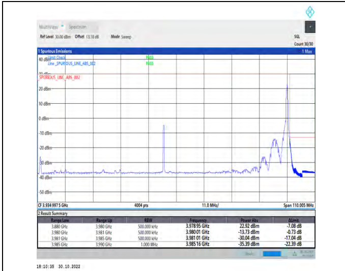
1-N77-3700-3980-PC2-30-100-H-2-DFT-PI2BPSK-Edge_1RB_Right-1@272-Ant1-1--PASS-see graph
