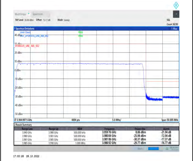
1-N77-3700-3980-PC2-30-40-H-6-CP-QPSK-Outer_Full-106@0-Ant1-1--PASS-see graph
