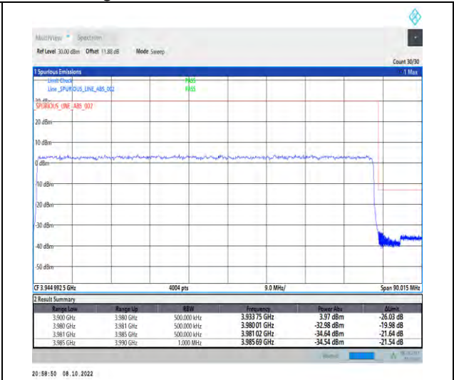
1-N77-3700-3980-PC2-30-80-H-3-DFT-QPSK-Out er_Full-216@0-Ant1-1--PASS-see graph
