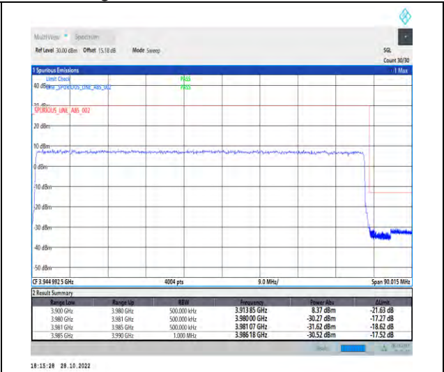
1-N77-3700-3980-PC2-30-80-H-3-DFT-PI2BPSK-Outer_Full-216@0-Ant1-1--PASS-see graph
