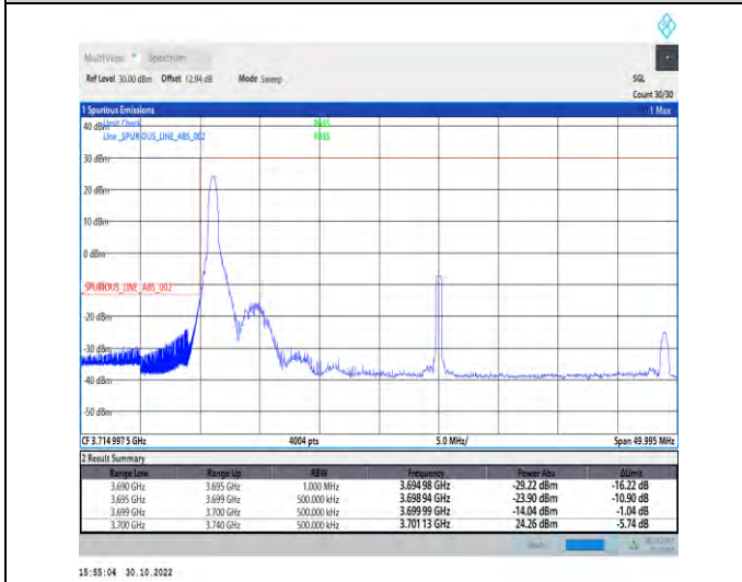
1-N77-3700-3980-PC2-30-40-L-4-CP-QPSK-Edge_1RB_Left-1@0-Ant1-1--PASS-see graph
