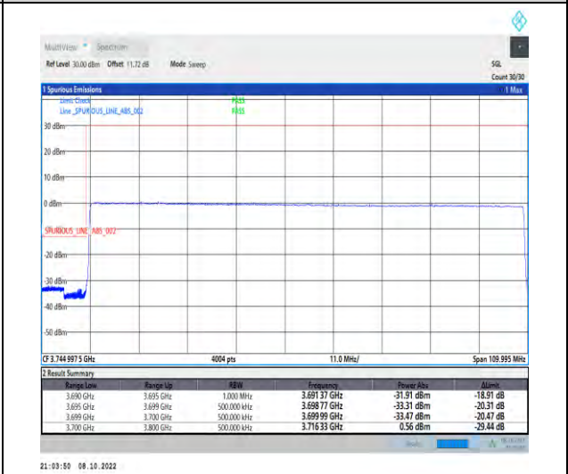
1-N77-3700-3980-PC2-30-100-L-6-CP-QPSK-Out er_Full-273@0-Ant1-1--PASS-see graph
