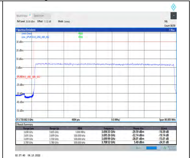
1-N77-3700-3980-PC2-30-80-L-3-DFT-QPSK-Outer_Full-216@0-Ant1-1--PASS-see graph
