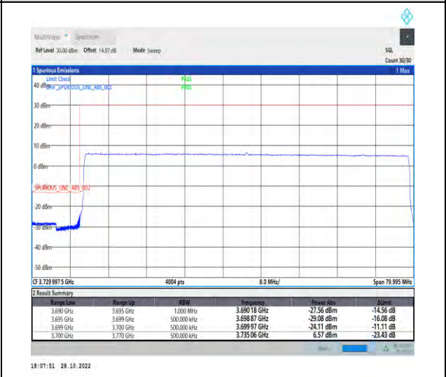
1-N77-3700-3980-PC2-30-70-L-6-CP-QPSK-Outer_Full-189@0-Ant1-1--PASS-see graph
