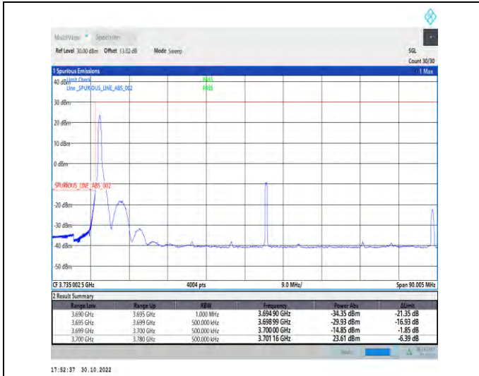
1-N77-3700-3980-PC2-30-80-L-1-DFT-PI2BPSK-Edge_1RB_Left-1@0-Ant1-1--PASS-see graph
