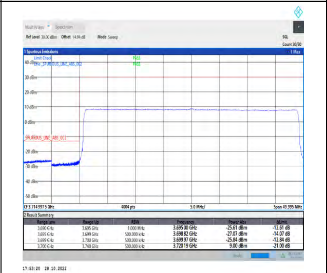
1-N77-3700-3980-PC2-30-40-L-6-CP-QPSK-Outer_Full-106@0-Ant1-1--PASS-see graph
