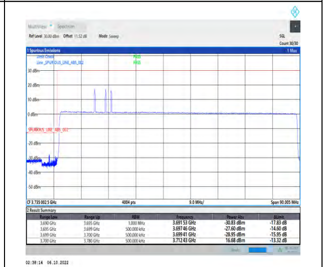
1-N77-3700-3980-PC2-30-80-L-6-CP-QPSK-Outer_Full-217@0-Ant1-1--PASS-see graph
