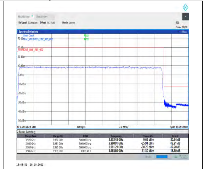
1-N77-3700-3980-PC2-30-60-H-3-DFT-PI2BPSK-Outer_Full-162@0-Ant1-1--PASS-see graph
