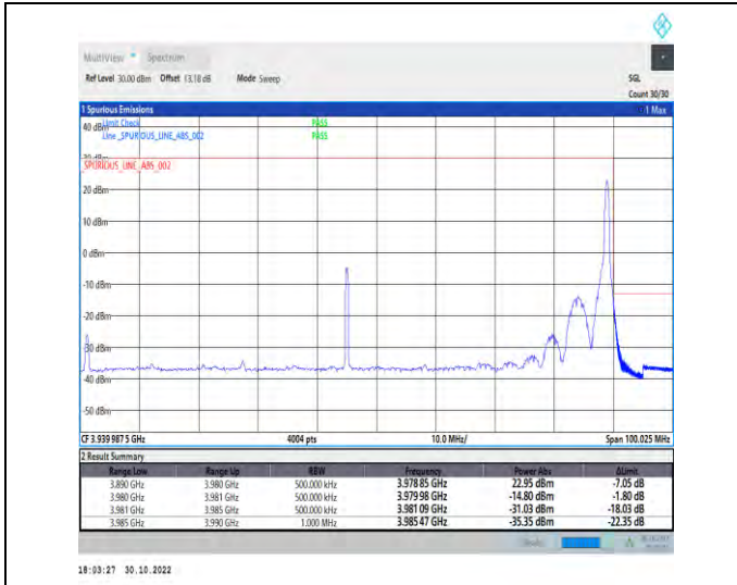
1-N77-3700-3980-PC2-30-90-H-2-DFT-PI2BPSK-Edge_1RB_Right-1@244-Ant1-1--PASS-see graph
