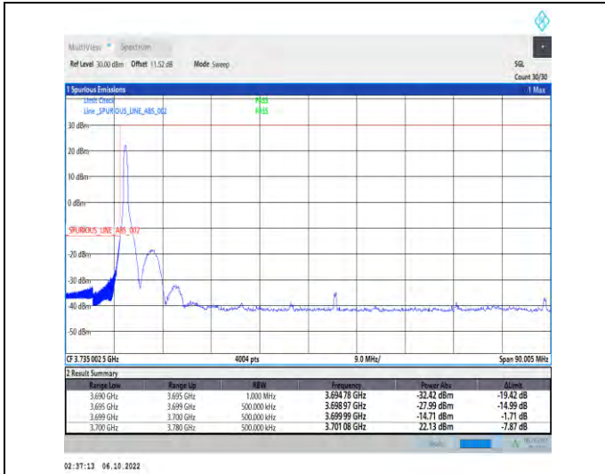
1-N77-3700-3980-PC2-30-80-L-1-DFT-QPSK-Edge_1 RB_Left-1@0-Ant1-1--PASS-see graph
