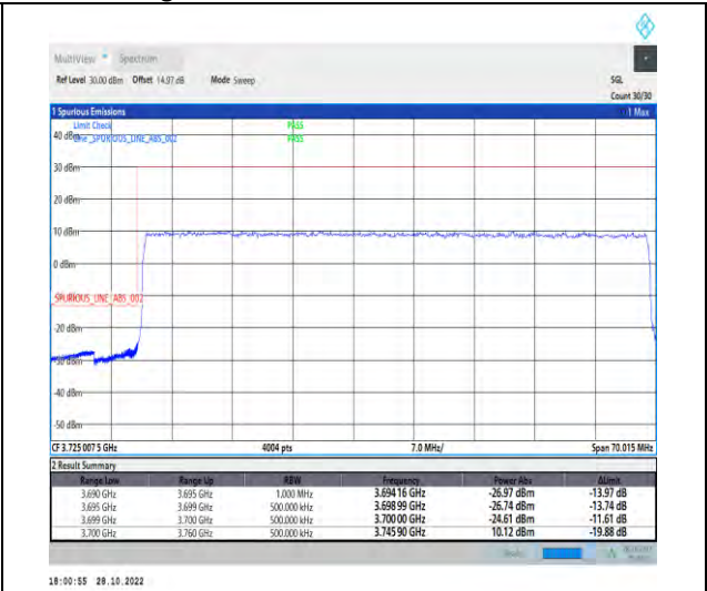
1-N77-3700-3980-PC2-30-60-L-3-DFT-PI2BPSK-Outer_Full-162@0-Ant1-1--PASS-see graph
