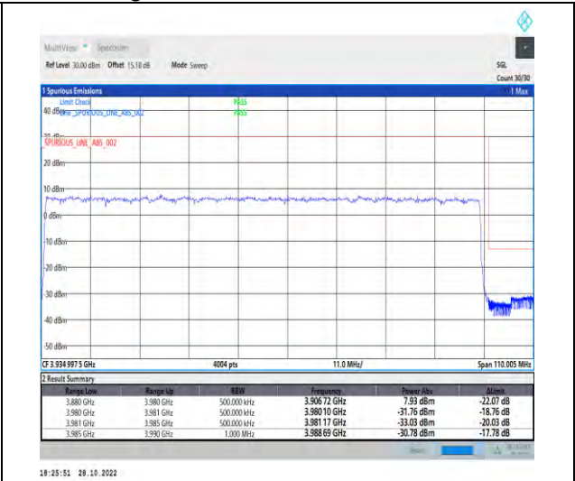
1-N77-3700-3980-PC2-30-100-H-3-DFT-PI2BPSK-Outer_Full-270@0-Ant1-1--PASS-see graph
