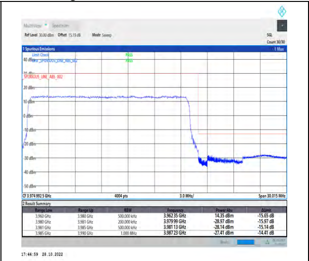
1-N77-3700-3980-PC2-30-20-H-3-DFT-PI2BPSK-Outer_Full-50@0-Ant1-1--PASS-see graph
