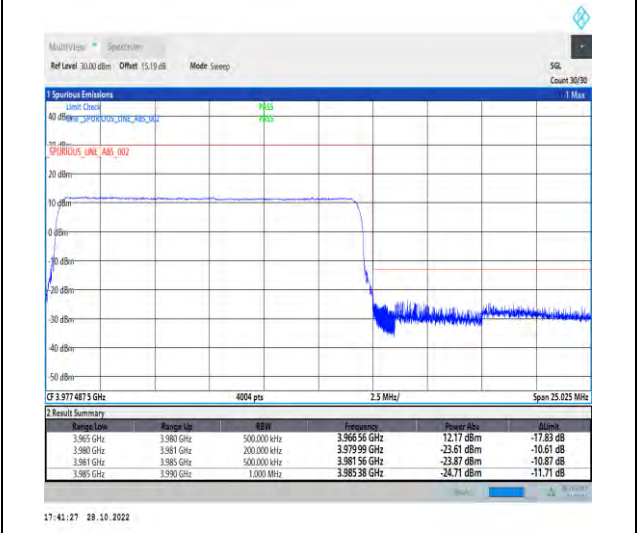
1-N77-3700-3980-PC2-30-15-H-6-CP-QPSK-Outer_Full-38@0-Ant1-1--PASS-see graph
