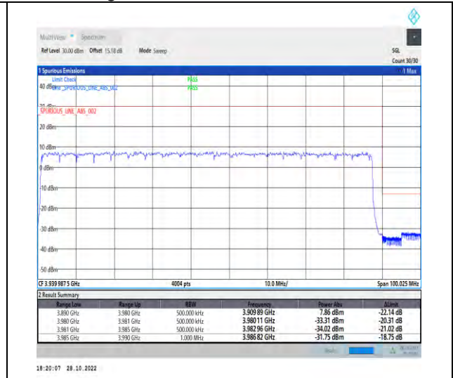
1-N77-3700-3980-PC2-30-90-H-3-DFT-PI2BPSK-Outer_Full-240@0-Ant1-1--PASS-see graph
