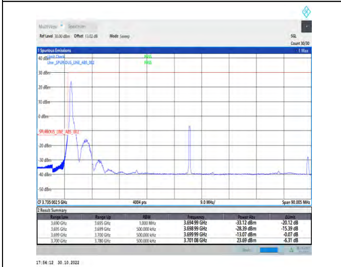
1-N77-3700-3980-PC2-30-80-L-4-CP-QPSK-Edge_1RB_Left-1@0-Ant1-1--PASS-see graph
