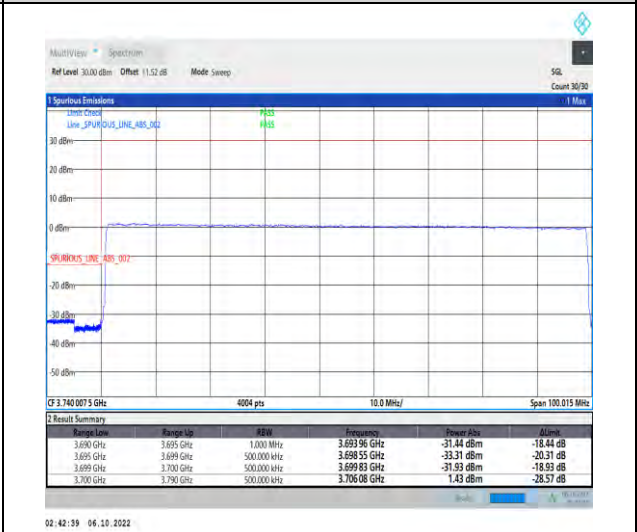
1-N77-3700-3980-PC2-30-90-L-6-CP-QPSK-Outer_Full-245@0-Ant1-1--PASS-see graph
