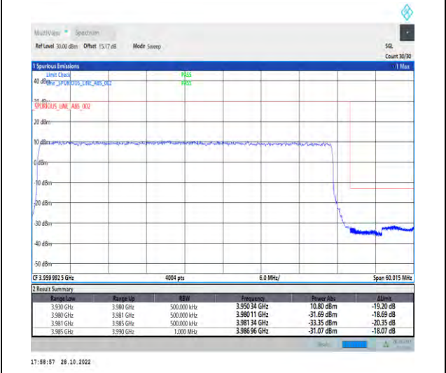
1-N77-3700-3980-PC2-30-50-H-6-CP-QPSK-Outer_Full-133@0-Ant1-1--PASS-see graph
