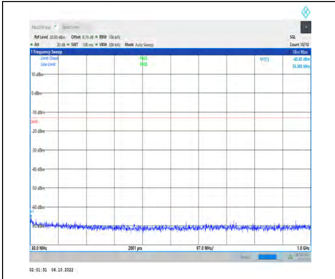
1-N77-3700-3980-PC2-30-100-M-1-DFT-PI2BPSK-Inner_1RB_Left-1@1-30-1000-Ant1-33.40--65.85--1 3-PASS
