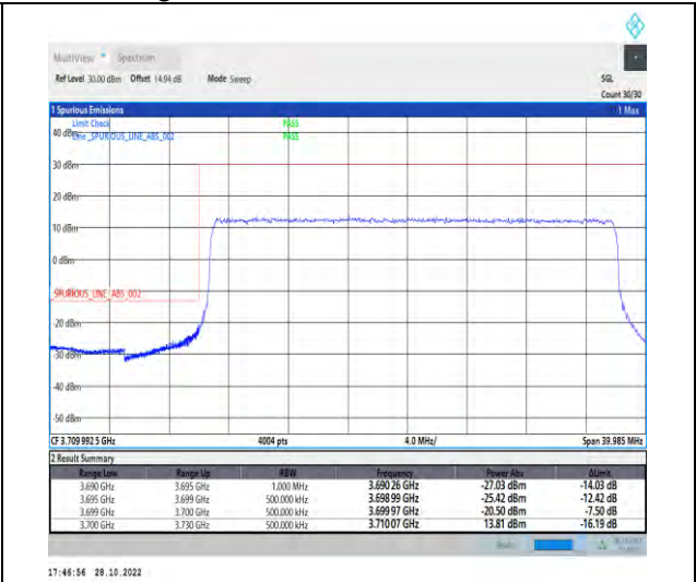
1-N77-3700-3980-PC2-30-30-L-3-DFT-PI2BPSK-Outer_Full-75@0-Ant1-1--PASS-see graph
