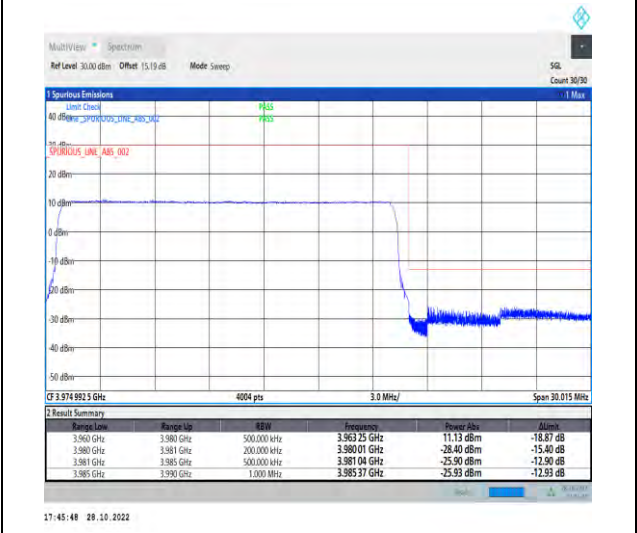
1-N77-3700-3980-PC2-30-20-H-6-CP-QPSK-Outer_Full-51@0-Ant1-1--PASS-see graph
