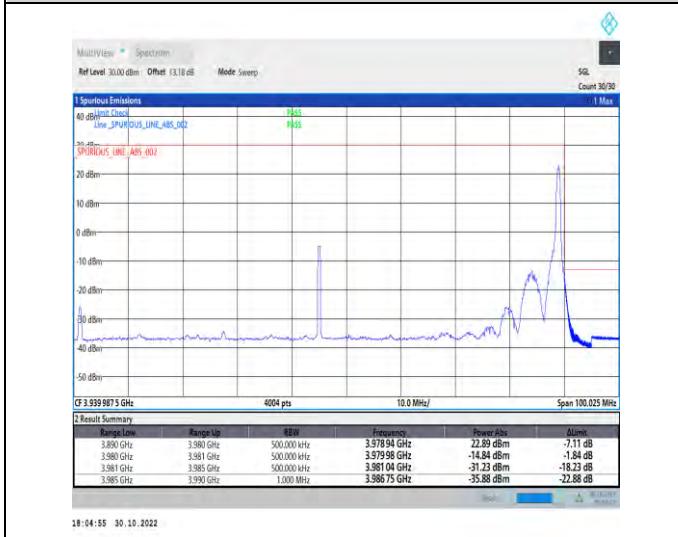
1-N77-3700-3980-PC2-30-90-H-5-CP-QPSK-Edge_1RB_Right-1@244-Ant1-1--PASS-see graph
