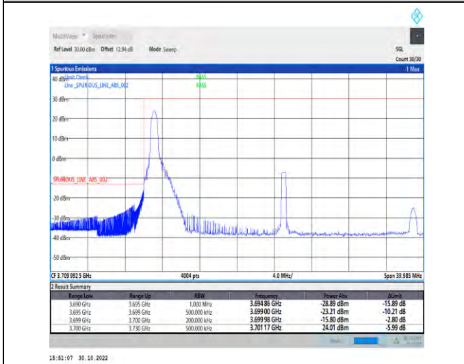
1-N77-3700-3980-PC2-30-30-L-4-CP-QPSK-Edge_1RB_Left-1@0-Ant1-1--PASS-see graph
