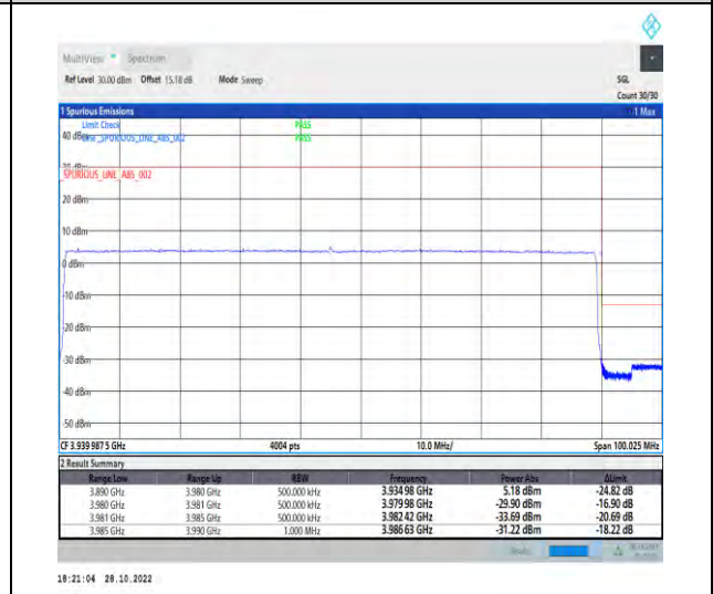
1-N77-3700-3980-PC2-30-90-H-6-CP-QPSK-Outer_Full-245@0-Ant1-1--PASS-see graph
