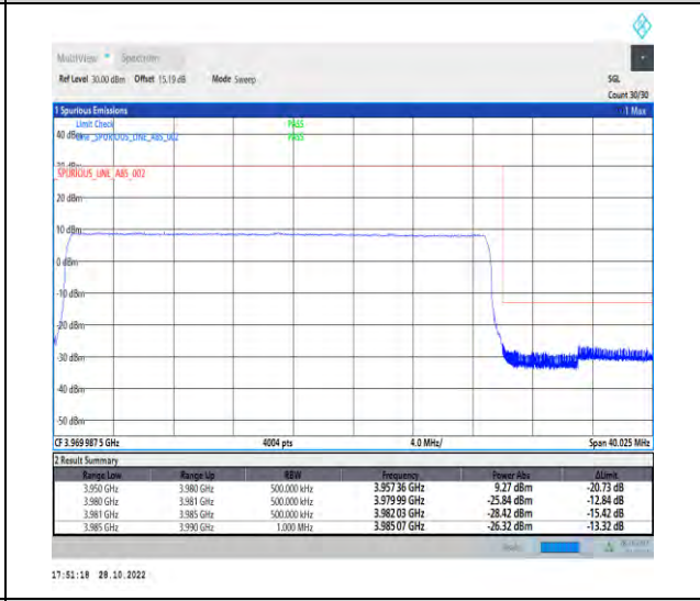
1-N77-3700-3980-PC2-30-30-H-6-CP-QPSK-Outer_Full-78@0-Ant1-1--PASS-see graph
