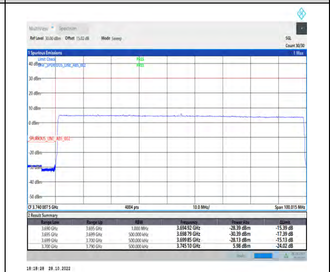
1-N77-3700-3980-PC2-30-90-L-6-CP-QPSK-Outer_Full-245@0-Ant1-1--PASS-see graph
