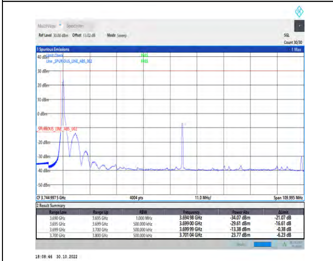
1-N77-3700-3980-PC2-30-100-L-4-CP-QPSK-Edge_1_RB_Left-1@0-Ant1-1--PASS-see graph
