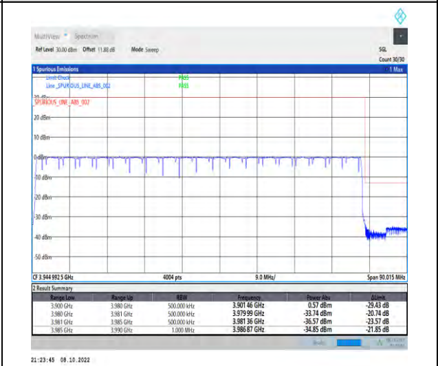
1-N77-3700-3980-PC2-30-80-H-6-CP-QPSK-Outer _Full-217@0-Ant1-1--PASS-see graph
