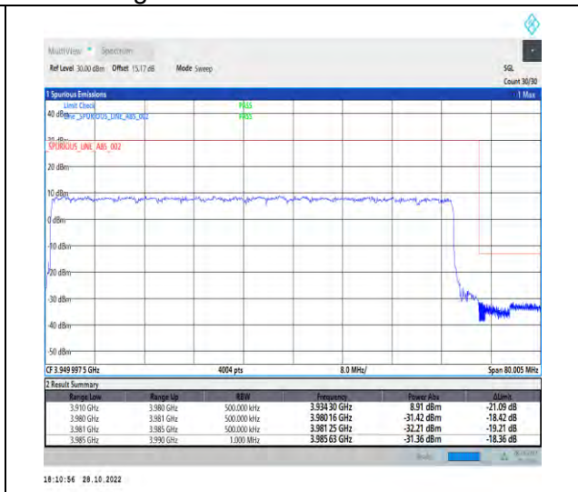
1-N77-3700-3980-PC2-30-70-H-3-DFT-PI2BPSK-Outer_Full-180@0-Ant1-1--PASS-see graph
