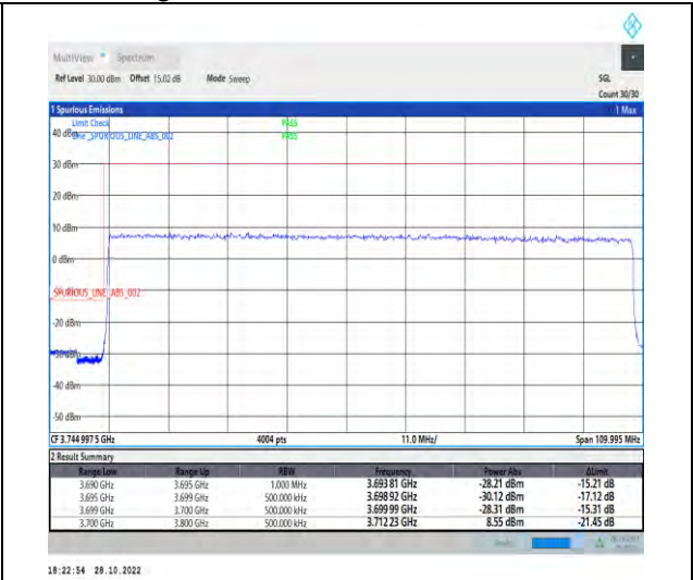
1-N77-3700-3980-PC2-30-100-L-3-DFT-PI2BPSK-Outer_Full-270@0-Ant1-1--PASS-see graph
