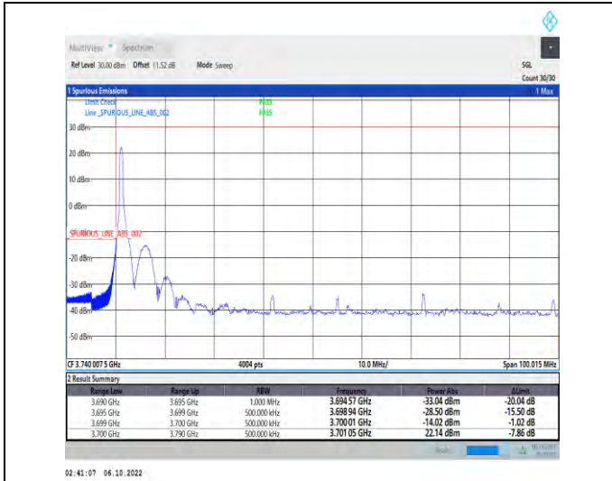
1-N77-3700-3980-PC2-30-90-L-1-DFT-QPSK-Edge_1 RB_Left-1@0-Ant1-1--PASS-see graph
