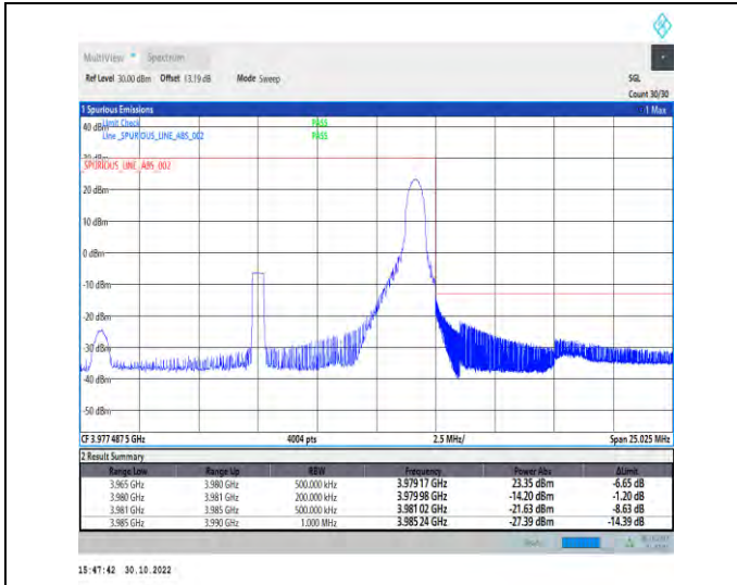
1-N77-3700-3980-PC2-30-15-H-2-DFT-PI2BPSK-Edge_1RB_Right-1@37-Ant1-1--PASS-see graph
