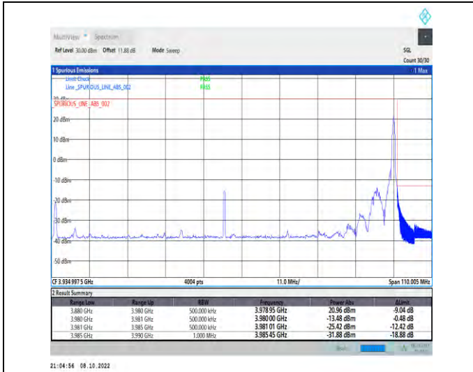
1-N77-3700-3980-PC2-30-100-H-2-DFT-QPSK-Edge_1RB_Right-1@272-Ant1-1--PASS-see graph
