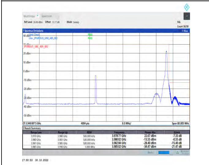
1-N77-3700-3980-PC2-30-70-H-5-CP-QPSK-Edge_1RB_Right-1@188-Ant1-1--PASS-see graph
