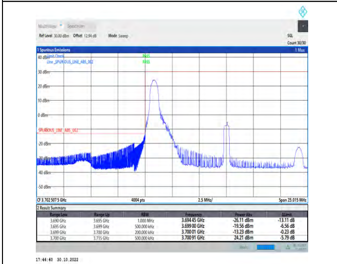
1-N77-3700-3980-PC2-30-15-L-4-CP-QPSK-Edge_1RB_Left-1@0-Ant1-1--PASS-see graph
