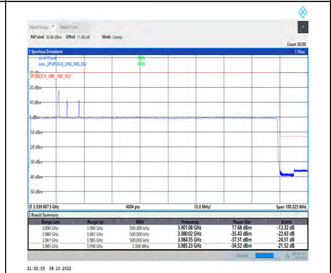
1-N77-3700-3980-PC2-30-90-H-6-CP-QPSK-Outer _Full-245@0-Ant1-1--PASS-see graph
