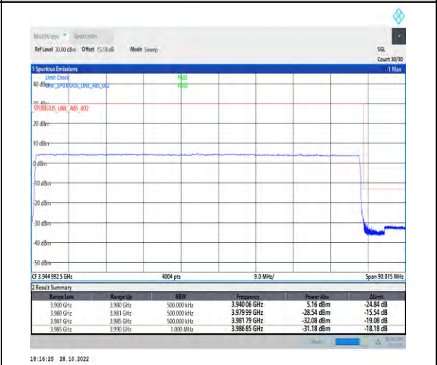
1-N77-3700-3980-PC2-30-80-H-6-CP-QPSK-Outer_Full-217@0-Ant1-1--PASS-see graph
