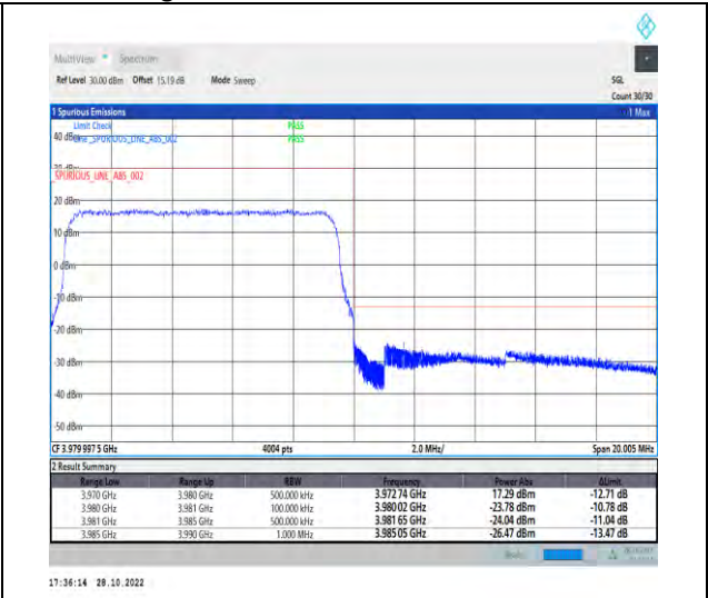
1-N77-3700-3980-PC2-30-10-H-3-DFT-PI2BPSK-Outer_Full-24@0-Ant1-1--PASS-see graph
