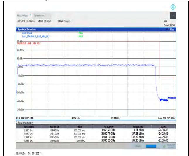
1-N77-3700-3980-PC2-30-90-H-3-DFT-QPSK-Out er_Full-240@0-Ant1-1--PASS-see graph
