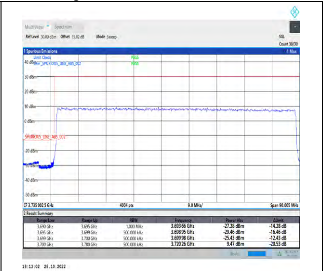
1-N77-3700-3980-PC2-30-80-L-3-DFT-PI2BPSK-Outer_Full-216@0-Ant1-1--PASS-see graph
