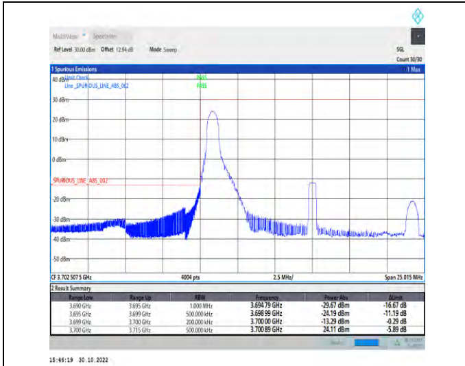
1-N77-3700-3980-PC2-30-15-L-1-DFT-PI2BPSK-Edge_1RB_Left-1@0-Ant1-1--PASS-see graph
