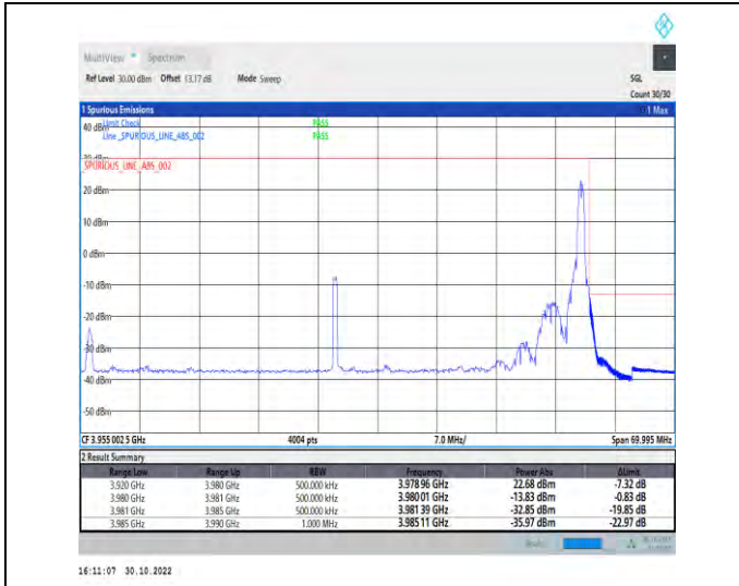
1-N77-3700-3980-PC2-30-60-H-2-DFT-PI2BPSK-Edge_1RB_Right-1@161-Ant1-1--PASS-see graph
