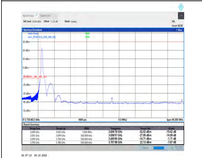
1-N77-3700-3980-PC2-30-80-L-6-CP-QPSK-Outer_Full-217@0-Ant1-1--PASS-see graph
