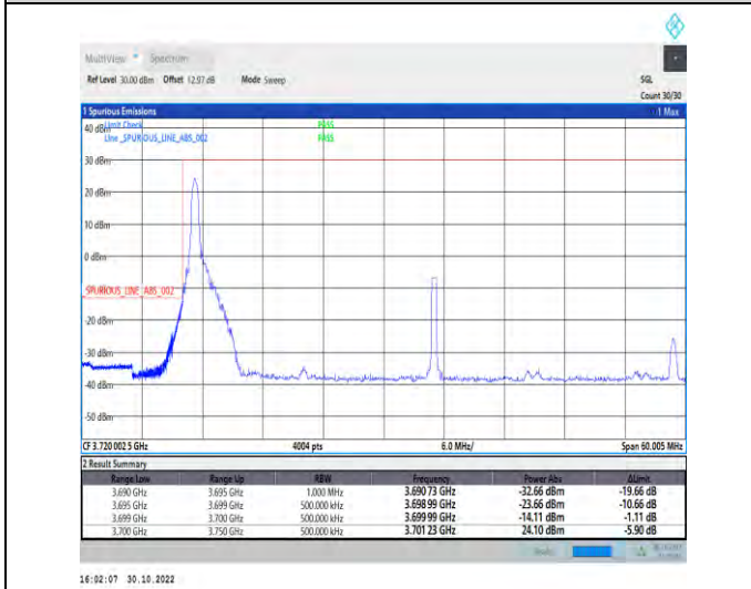
1-N77-3700-3980-PC2-30-50-L-4-CP-QPSK-Edge_1RB_Left-1@0-Ant1-1--PASS-see graph
