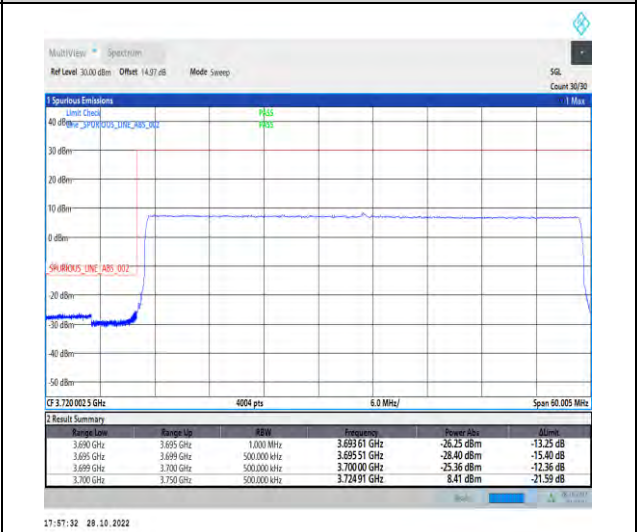
1-N77-3700-3980-PC2-30-50-L-6-CP-QPSK-Outer_Full-133@0-Ant1-1--PASS-see graph
