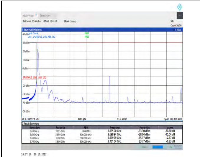
1-N77-3700-3980-PC2-30-100-L-1-DFT-PI2BPSK-Edge_1_RB_Left-1@0-Ant1-1--PASS-see graph
