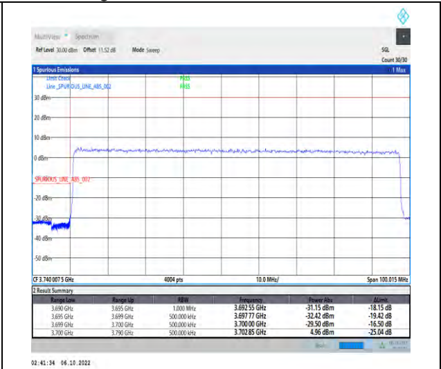
1-N77-3700-3980-PC2-30-90-L-3-DFT-QPSK-Outer_Full-240@0-Ant1-1--PASS-see graph
