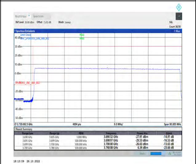
1-N77-3700-3980-PC2-30-80-L-6-CP-QPSK-Outer_Full-217@0-Ant1-1--PASS-see graph
