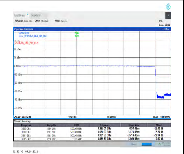
1-N77-3700-3980-PC2-30-100-H-6-CP-QPSK-Outer_Full-273@0-Ant1-1--PASS-see graph
