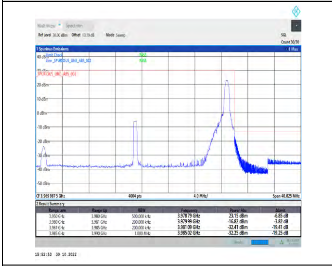
1-N77-3700-3980-PC2-30-30-H-5-CP-QPSK-Edge_1RB_Right-1@77-Ant1-1--PASS-see graph
