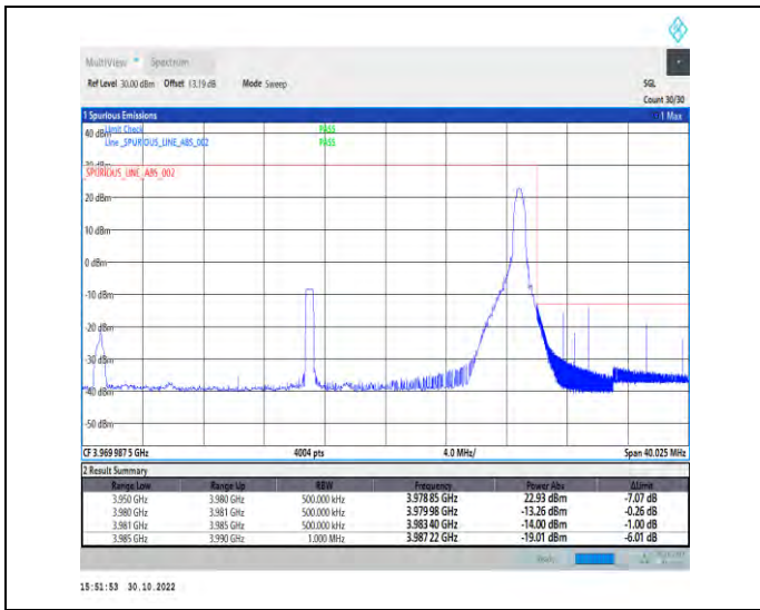
1-N77-3700-3980-PC2-30-30-H-2-DFT-PI2BPSK-Edge_1RB_Right-1@77-Ant1-1--PASS-see graph
