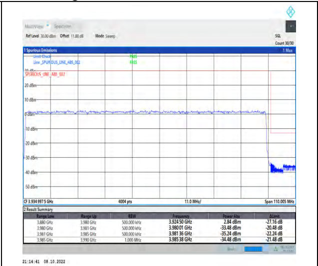
1-N77-3700-3980-PC2-30-100-H-3-DFT-QPSK-Outer_Full-270@0-Ant1-1--PASS-see graph
