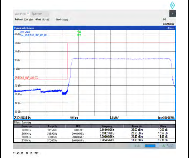
1-N77-3700-3980-PC2-30-20-L-6-CP-QPSK-Outer_Full-51@0-Ant1-1--PASS-see graph
