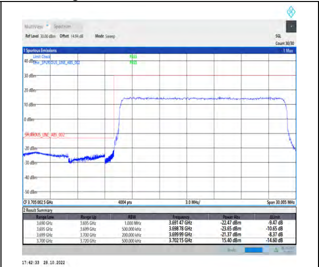
1-N77-3700-3980-PC2-30-20-L-3-DFT-PI2BPSK-Outer_Full-50@0-Ant1-1--PASS-see graph
