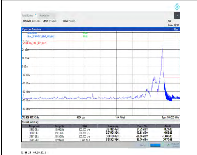
1-N77-3700-3980-PC2-30-90-H-5-CP-QPSK-Edge_1R B_Right-1@244-Ant1-1--PASS-see graph
