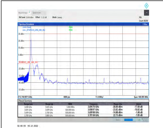
1-N77-3700-3980-PC2-30-100-L-1-DFT-QPSK-Edge_1 RB_Left-1@0-Ant1-1--PASS-see graph
