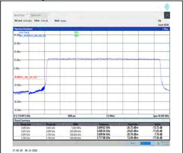
1-N77-3700-3980-PC2-30-40-L-3-DFT-PI2BPSK-Outer_Full-100@0-Ant1-1--PASS-see graph
