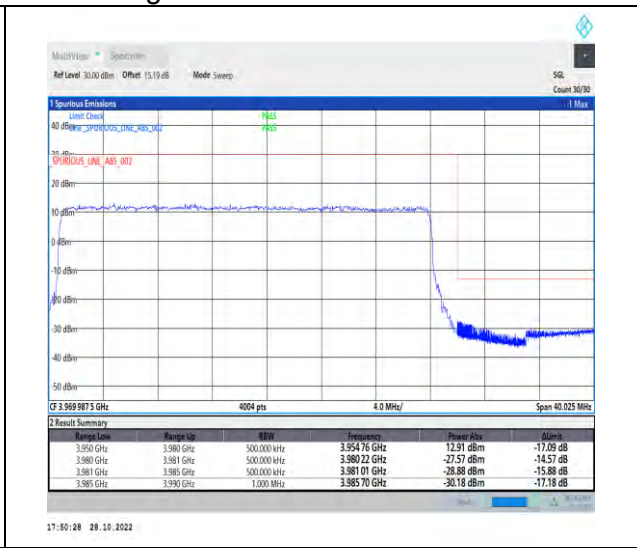
1-N77-3700-3980-PC2-30-30-H-3-DFT-PI2BPSK-Outer_Full-75@0-Ant1-1--PASS-see graph
