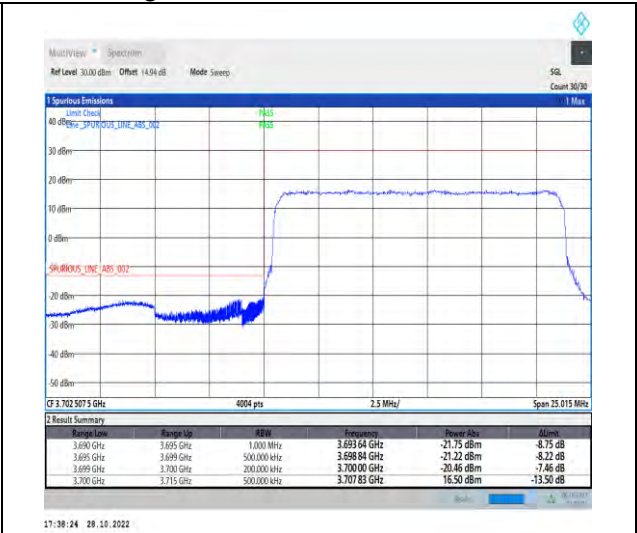
1-N77-3700-3980-PC2-30-15-L-3-DFT-PI2BPSK-Outer_Full-36@0-Ant1-1--PASS-see graph
