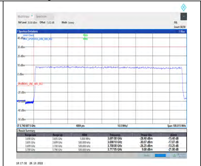
1-N77-3700-3980-PC2-30-90-L-3-DFT-PI2BPSK-Outer_Full-240@0-Ant1-1--PASS-see graph
