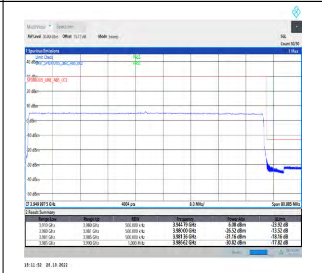
1-N77-3700-3980-PC2-30-70-H-6-CP-QPSK-Outer_Full-189@0-Ant1-1--PASS-see graph
