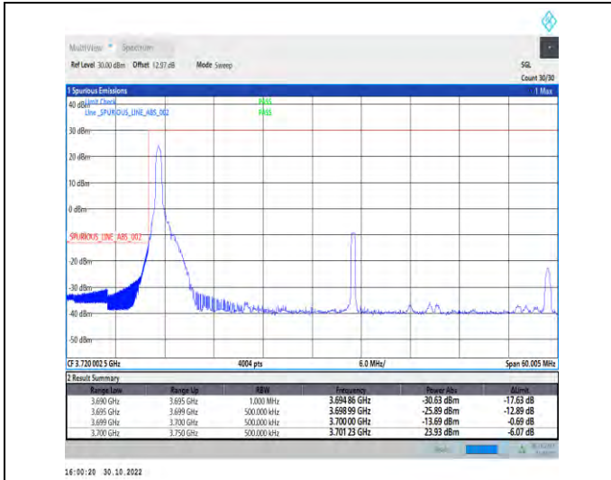
1-N77-3700-3980-PC2-30-50-L-1-DFT-PI2BPSK-Edge_1RB_Left-1@0-Ant1-1--PASS-see graph
