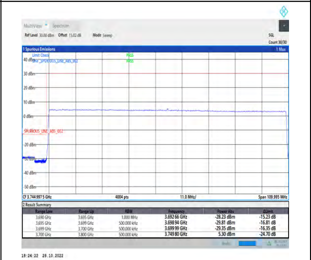
1-N77-3700-3980-PC2-30-100-L-6-CP-QPSK-Outer_Full-273@0-Ant1-1--PASS-see graph
