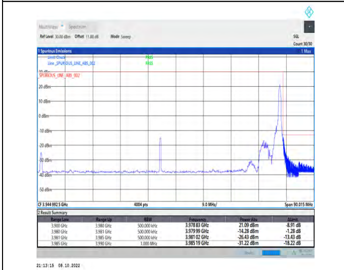
1-N77-3700-3980-PC2-30-80-H-5-CP-QPSK-Edge_1R B_Right-1@216-Ant1-1--PASS-see graph
