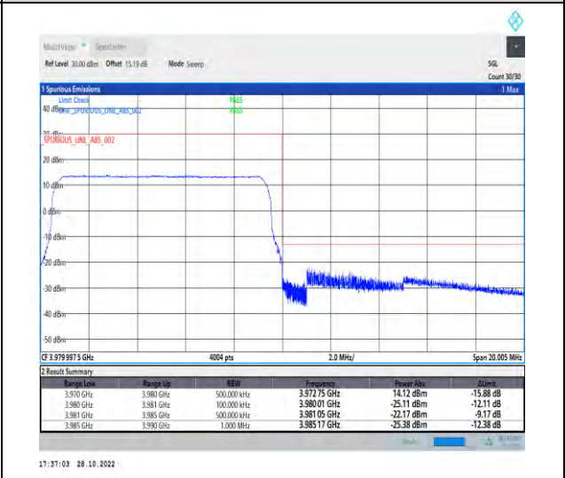
1-N77-3700-3980-PC2-30-10-H-6-CP-QPSK-Outer_Full-24@0-Ant1-1--PASS-see graph
