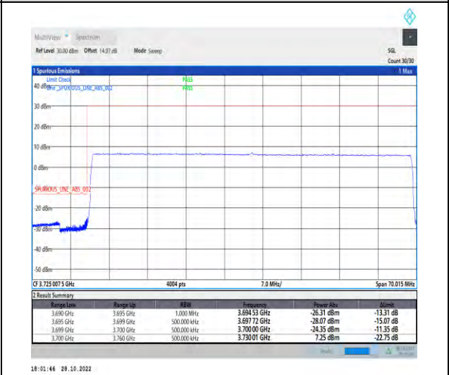
1-N77-3700-3980-PC2-30-60-L-6-CP-QPSK-Outer_Full-162@0-Ant1-1--PASS-see graph
