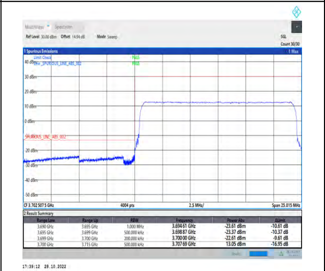
1-N77-3700-3980-PC2-30-15-L-6-CP-QPSK-Outer_Full-38@0-Ant1-1--PASS-see graph
