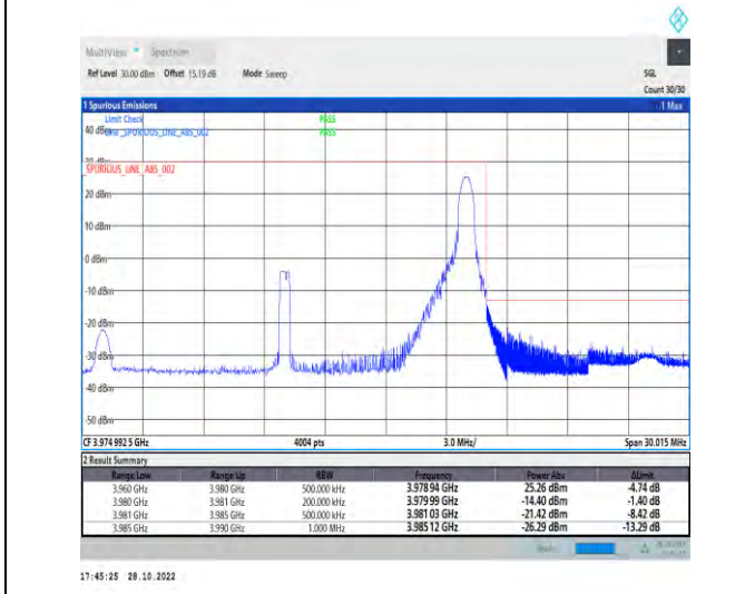
1-N77-3700-3980-PC2-30-20-H-5-CP-QPSK-Edge_1RB_Right-1@50-Ant1-1--PASS-see graph
