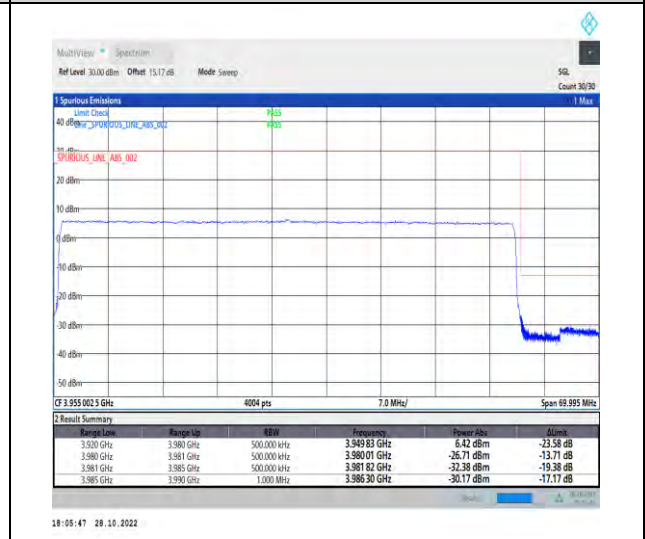
1-N77-3700-3980-PC2-30-60-H-6-CP-QPSK-Outer_Full-162@0-Ant1-1--PASS-see graph
