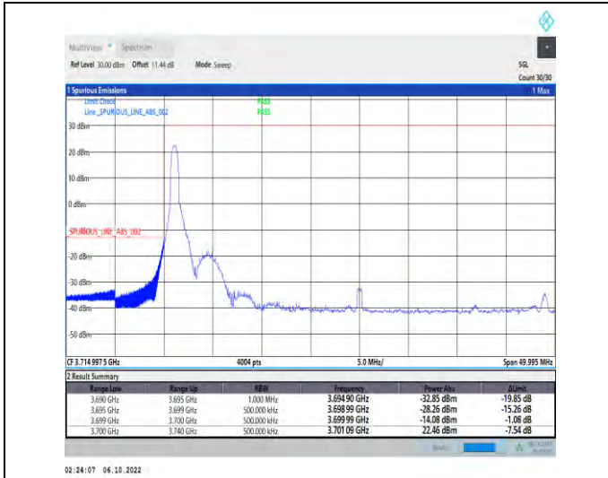
1-N77-3700-3980-PC2-30-40-L-1-DFT-QPSK-Edge_1 RB_Left-1@0-Ant1-1--PASS-see graph
