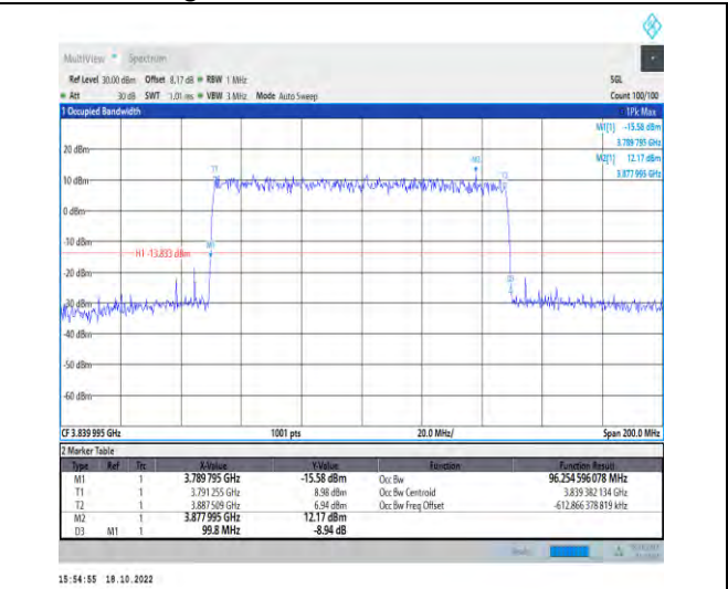
1-N77-3700-3980-PC2-30-100-M-3-DFT-16QAM-Out er_Full-270@0-Ant1-96.255-99.800-≤100-PASS
