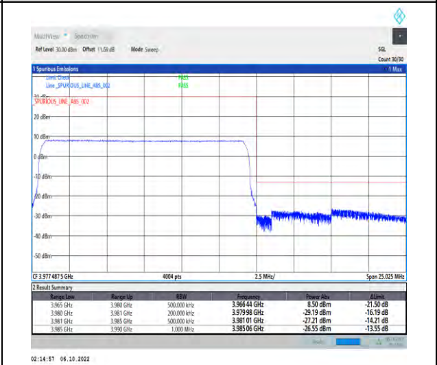
1-N77-3700-3980-PC2-30-15-H-6-CP-QPSK-Outer _Full-38@0-Ant1-1--PASS-see graph
