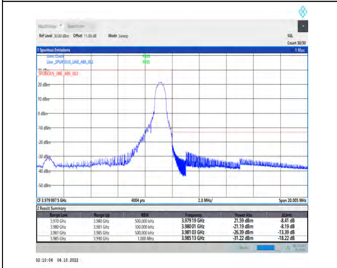
1-N77-3700-3980-PC2-30-10-H-5-CP-QPSK-Edge_1R B_Right-1@23-Ant1-1--PASS-see graph
