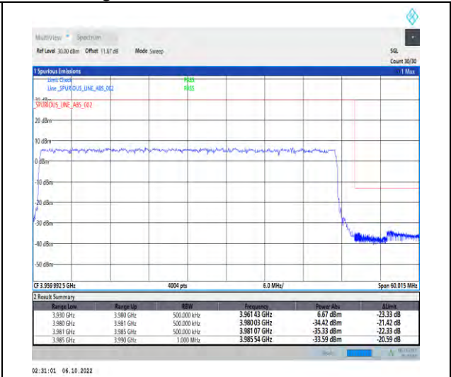
1-N77-3700-3980-PC2-30-50-H-3-DFT-QPSK-Out er_Full-128@0-Ant1-1--PASS-see graph
