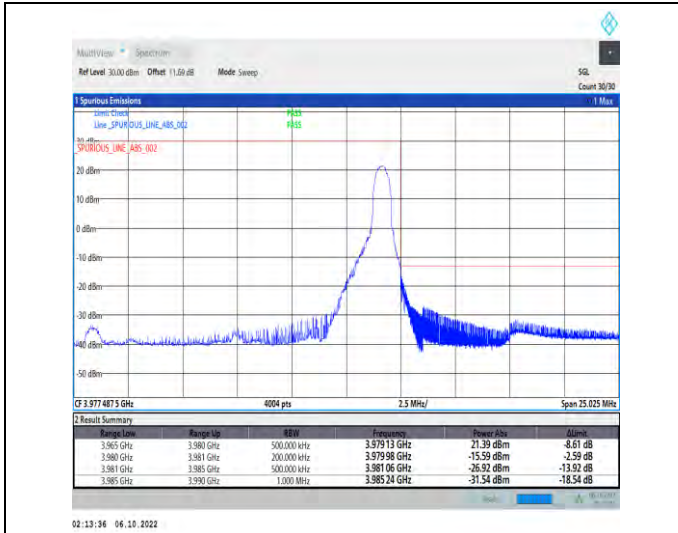
1-N77-3700-3980-PC2-30-15-H-2-DFT-QPSK-Edge_1 RB_Right-1@37-Ant1-1--PASS-see graph
