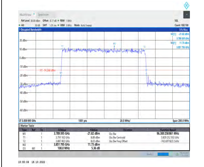
1-N77-3700-3980-PC2-30-100-M-4-DFT-64QAM-Out er_Full-270@0-Ant1-96.3-100.000-≤100-PASS
