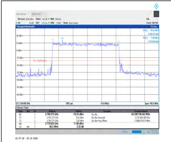
1-N77-3700-3980-PC2-30-70-L-1-DFT-QPSK-Outer_Full-180@0-Ant1-64.338-66.500-≤70-PASS
