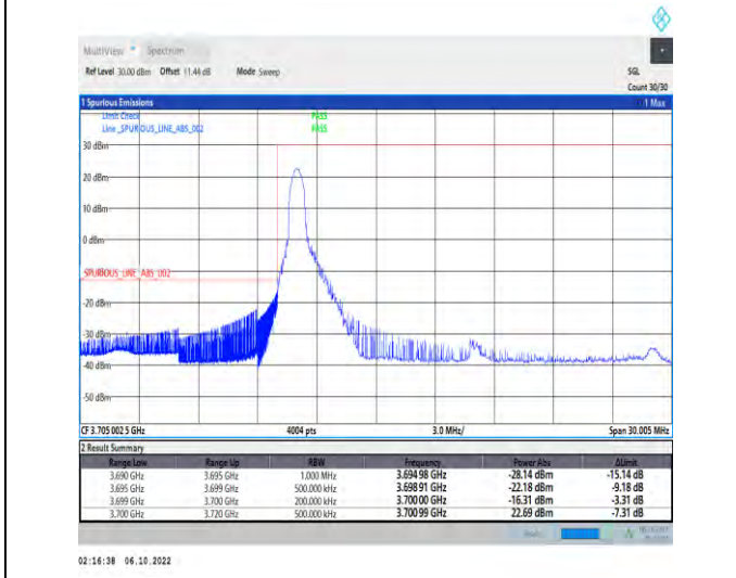
1-N77-3700-3980-PC2-30-20-L-4-CP-QPSK-Edge_1R B_Left-1@0-Ant1-1--PASS-see graph
