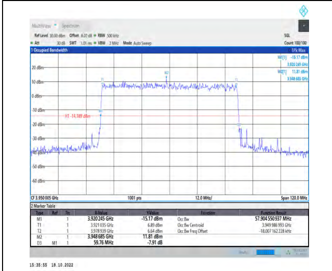
1-N77-3700-3980-PC2-30-60-H-4-DFT-64QAM-Outer_Full-162@0-Ant1-57.905-59.760-≤60-PASS
