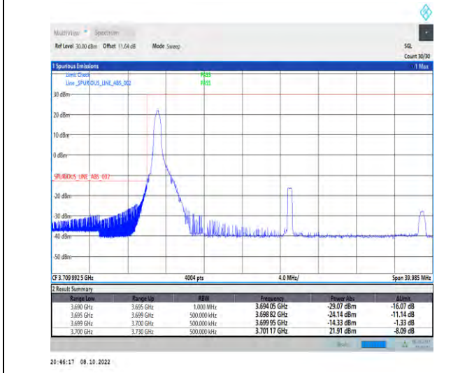
1-N77-3700-3980-PC2-30-30-L-4-CP-QPSK-Edge_1R B_Left-1@0-Ant1-1--PASS-see graph
