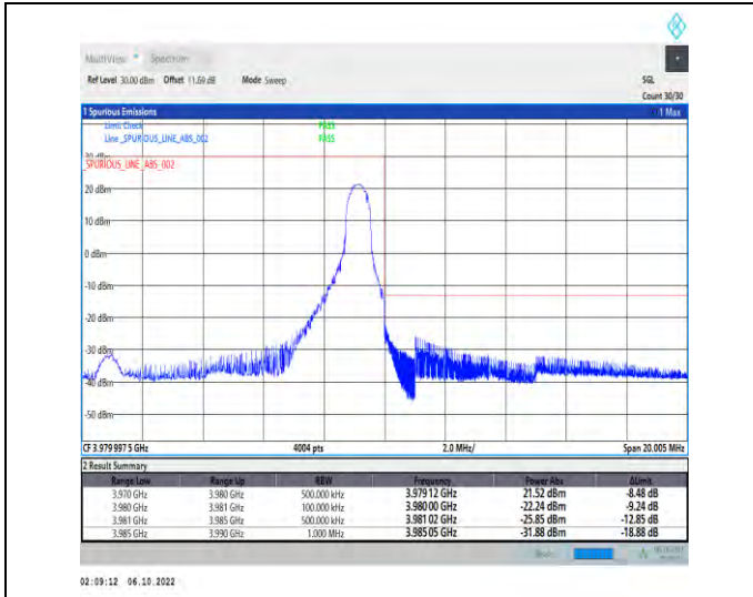
1-N77-3700-3980-PC2-30-10-H-2-DFT-QPSK-Edge_1 RB_Right-1@23-Ant1-1--PASS-see graph
