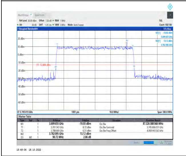
1-N77-3700-3980-PC2-30-90-L-8-CP-64QAM-Outer_Full-245@0-Ant1-87.326-90.720-<math>\leq 90</math>-PASS
