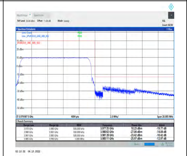
1-N77-3700-3980-PC2-30-10-H-6-CP-QPSK-Out er_Full-24@0-Ant1-1--PASS-see graph
