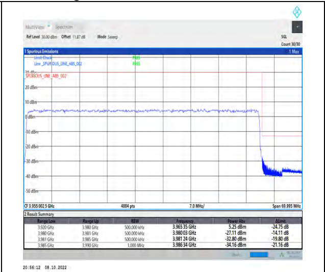
1-N77-3700-3980-PC2-30-60-H-3-DFT-QPSK-Out er_Full-162@0-Ant1-1--PASS-see graph
