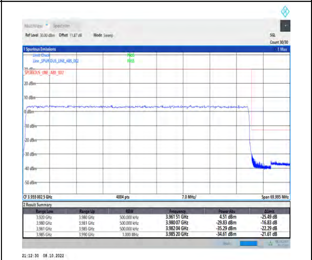
1-N77-3700-3980-PC2-30-60-H-6-CP-QPSK-Outer _Full-162@0-Ant1-1--PASS-see graph
