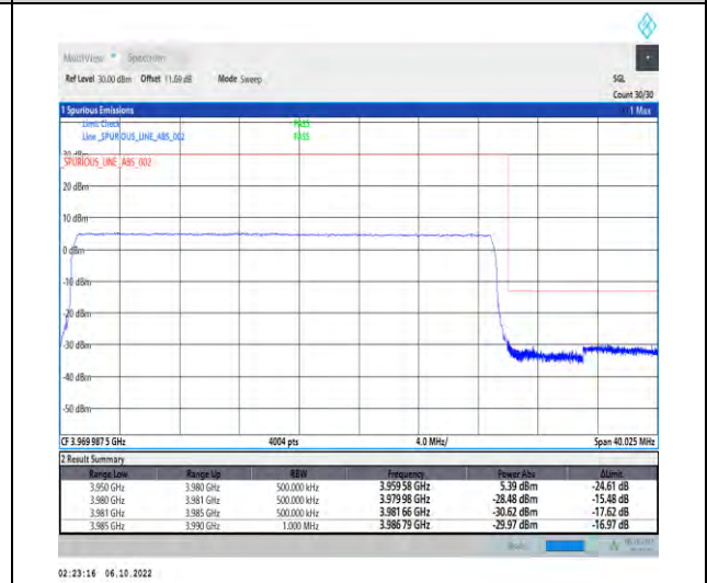
1-N77-3700-3980-PC2-30-30-H-6-CP-QPSK-Out er_Full-78@0-Ant1-1--PASS-see graph
