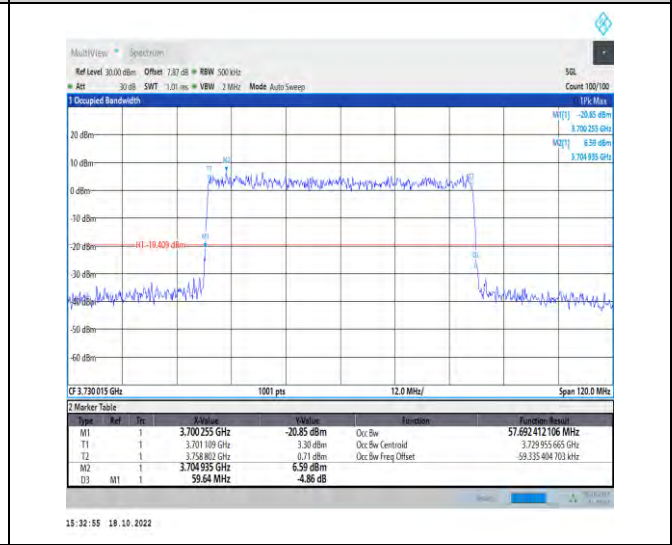
1-N77-3700-3980-PC2-30-60-L-9-CP-256QAM-Outer_Full-162@0-Ant1-57.692-59.640-≤60-PASS
