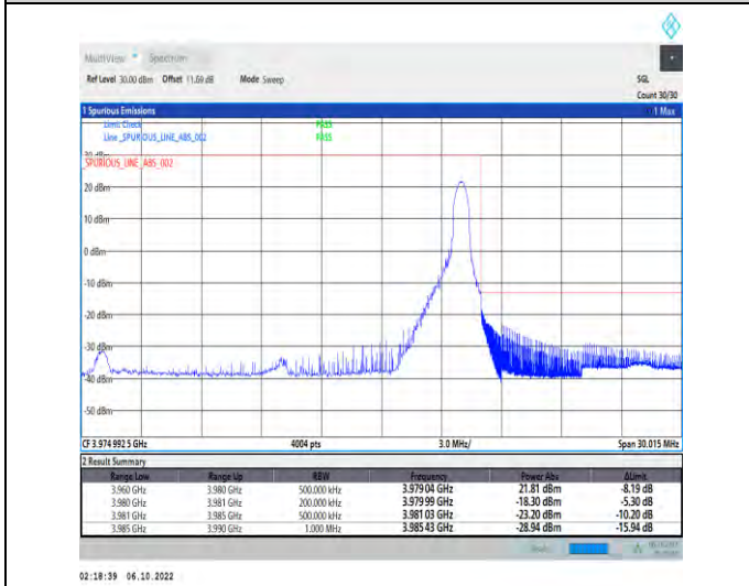
1-N77-3700-3980-PC2-30-20-H-5-CP-QPSK-Edge_1R B_Right-1@50-Ant1-1--PASS-see graph
