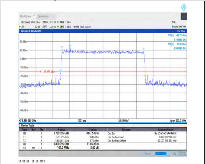
1-N77-3700-3980-PC2-30-100-M-7-CP-16QAM-Outer_Full-273@0-Ant1-97.356-101.000-≤100-PASS
