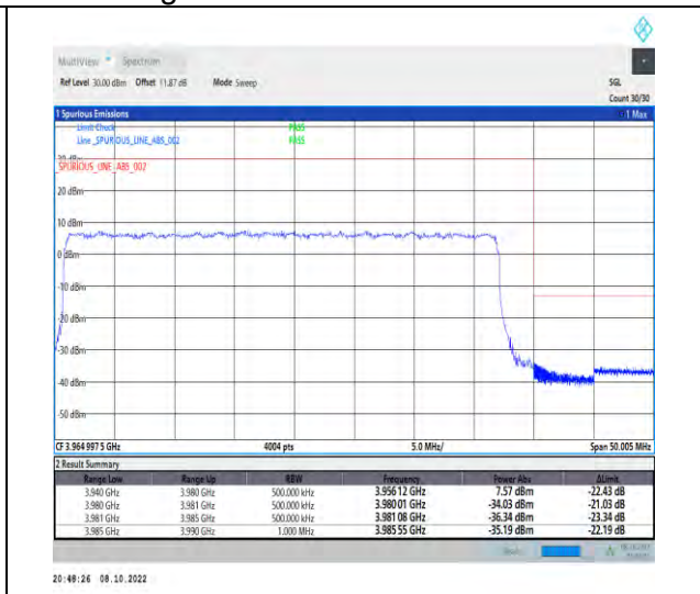
1-N77-3700-3980-PC2-30-40-H-3-DFT-QPSK-Out er_Full-100@0-Ant1-1--PASS-see graph
