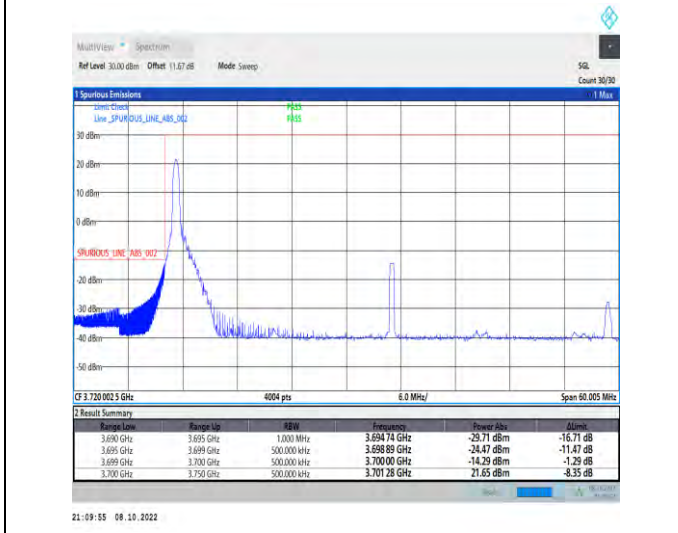
1-N77-3700-3980-PC2-30-50-L-4-CP-QPSK-Edge_1R B_Left-1@0-Ant1-1--PASS-see graph
