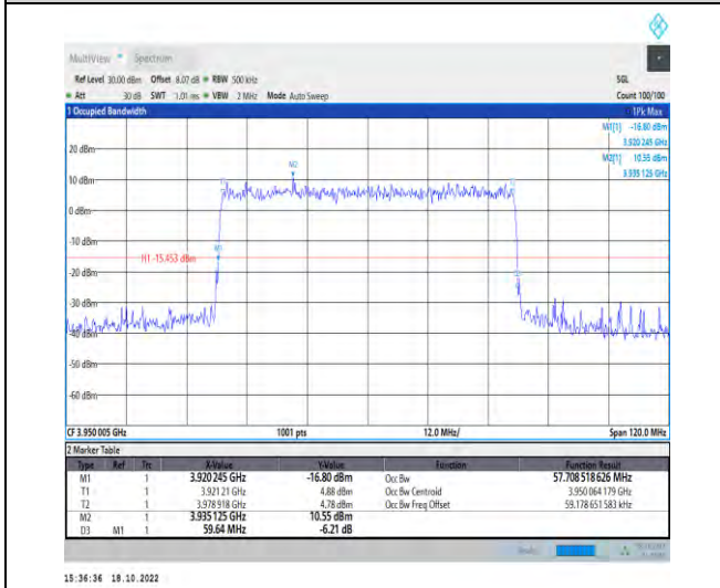
1-N77-3700-3980-PC2-30-60-H-8-CP-64QAM-Outer_Full-162@0-Ant1-57.709-59.640-≤60-PASS
