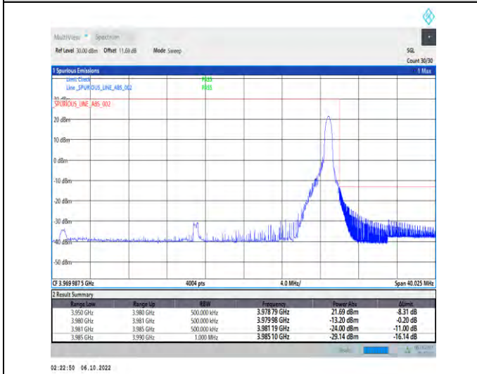
1-N77-3700-3980-PC2-30-30-H-5-CP-QPSK-Edge_1R B_Right-1@77-Ant1-1--PASS-see graph
