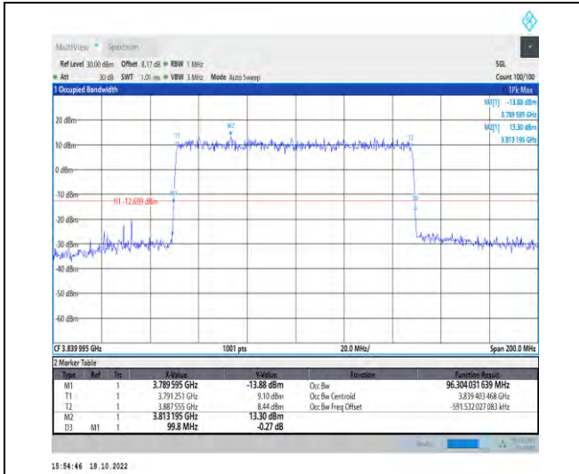
1-N77-3700-3980-PC2-30-100-M-1-DFT-QPSK-Out er_Full-270@0-Ant1-96.304-99.800-≤100-PASS
