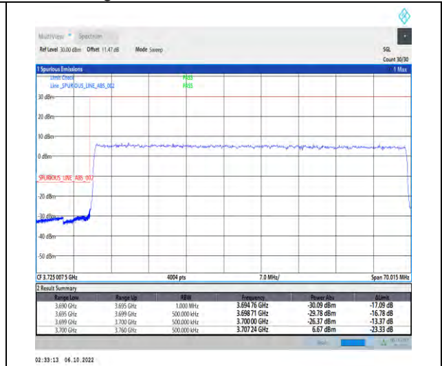
1-N77-3700-3980-PC2-30-60-L-3-DFT-QPSK-Outer_Full-162@0-Ant1-1--PASS-see graph
