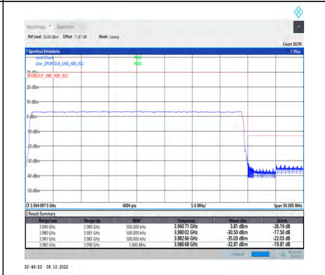
1-N77-3700-3980-PC2-30-40-H-6-CP-QPSK-Outer _Full-106@0-Ant1-1--PASS-see graph
