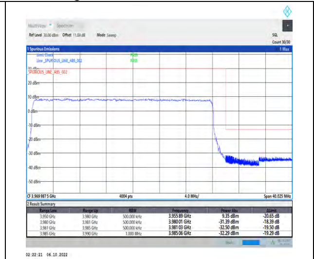
1-N77-3700-3980-PC2-30-30-H-3-DFT-QPSK-Out er_Full-75@0-Ant1-1--PASS-see graph
