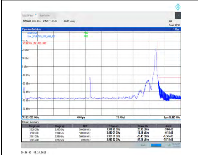
1-N77-3700-3980-PC2-30-60-H-5-CP-QPSK-Edge_1R B_Right-1@161-Ant1-1--PASS-see graph
