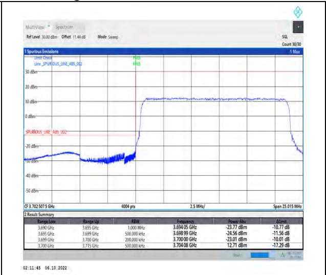
1-N77-3700-3980-PC2-30-15-L-3-DFT-QPSK-Outer_Full-36@0-Ant1-1--PASS-see graph
