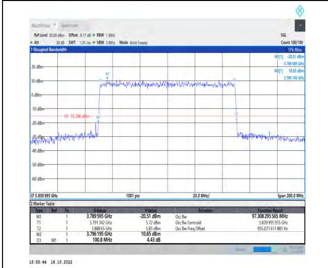
1-N77-3700-3980-PC2-30-100-M-8-CP-64QAM-Outer_Full-273@0-Ant1-97.308-100.800-≤100-PASS
