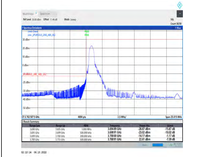
1-N77-3700-3980-PC2-30-15-L-4-CP-QPSK-Edge_1R B_Left-1@0-Ant1-1--PASS-see graph
