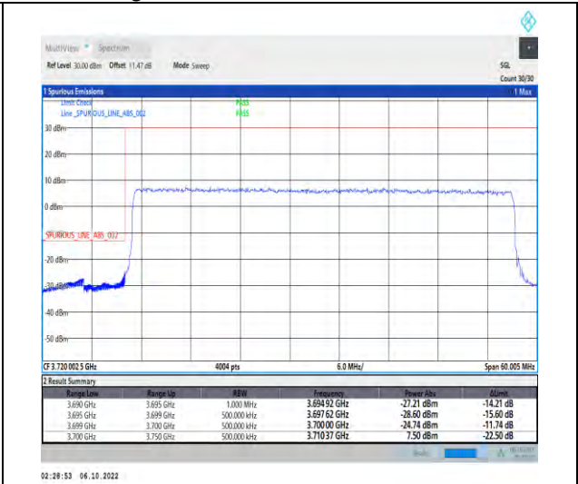
1-N77-3700-3980-PC2-30-50-L-3-DFT-QPSK-Outer_Full-128@0-Ant1-1--PASS-see graph
