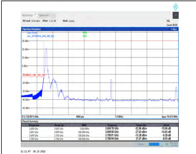
1-N77-3700-3980-PC2-30-60-L-1-DFT-QPSK-Edge_1 RB_Left-1@0-Ant1-1--PASS-see graph
