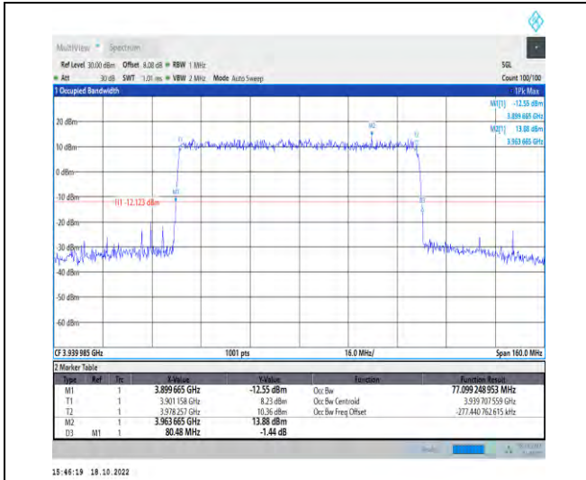
1-N77-3700-3980-PC2-30-80-H-1-DFT-QPSK-Outer_Full-216@0-Ant1-77.099-80.480-≤80-PASS
