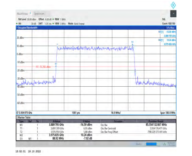
1-N77-3700-3980-PC2-30-90-H-5-DFT-256QAM-Outer_Full-240@0-Ant1-85.554-88.920-≤90-PASS
