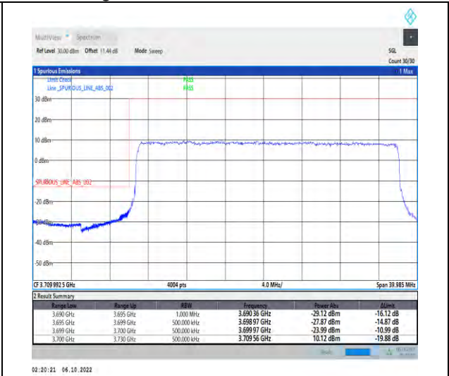
1-N77-3700-3980-PC2-30-30-L-3-DFT-QPSK-Outer_Full-75@0-Ant1-1--PASS-see graph
