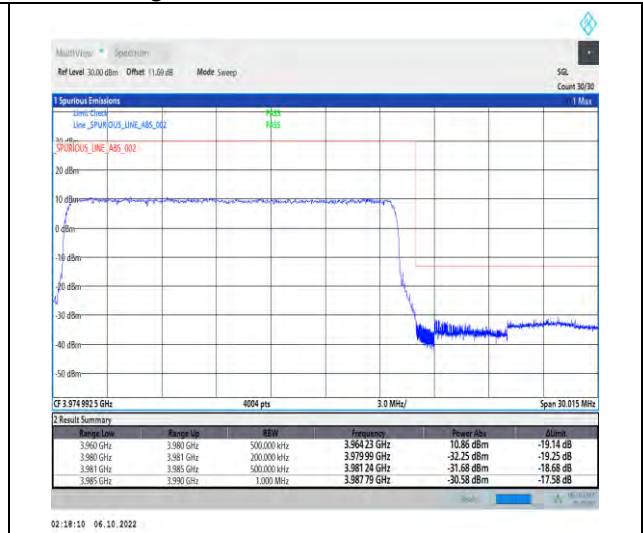
1-N77-3700-3980-PC2-30-20-H-3-DFT-QPSK-Out er_Full-50@0-Ant1-1--PASS-see graph
