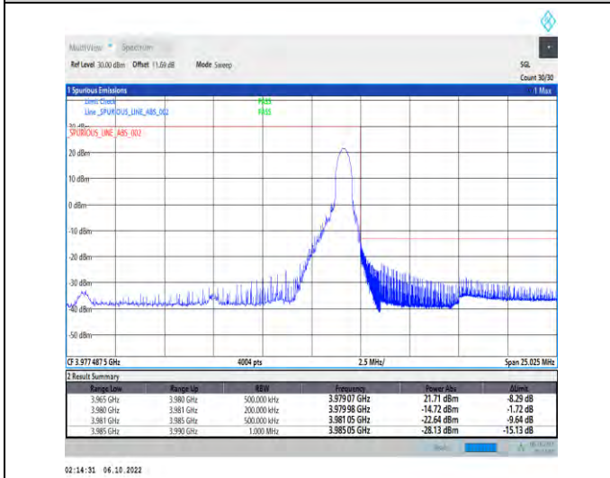
1-N77-3700-3980-PC2-30-15-H-5-CP-QPSK-Edge_1R B_Right-1@37-Ant1-1--PASS-see graph
