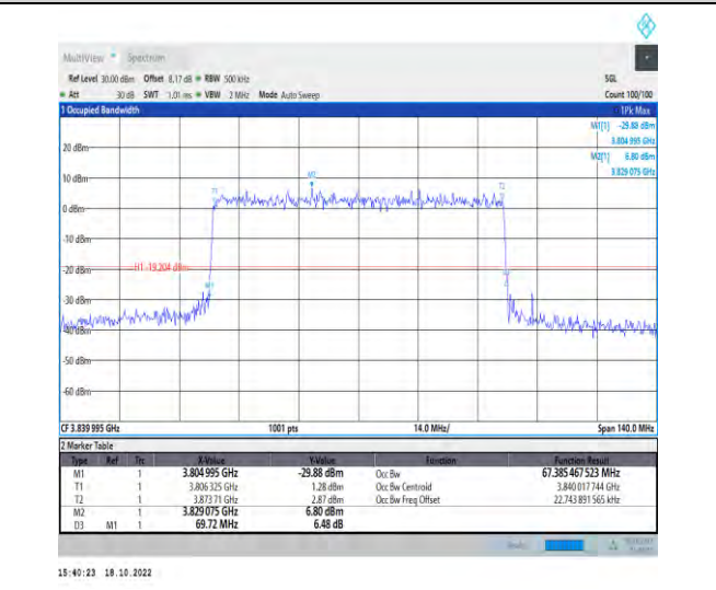
1-N77-3700-3980-PC2-30-70-M-9-CP-256QAM-Outer_Full-189@0-Ant1-67.385-69.720-≤70-PASS
