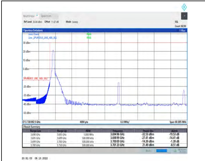
1-N77-3700-3980-PC2-30-50-L-1-DFT-QPSK-Edge_1 RB_Left-1@0-Ant1-1--PASS-see graph
