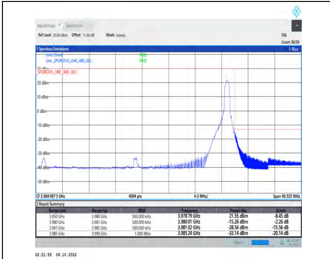
1-N77-3700-3980-PC2-30-30-H-2-DFT-QPSK-Edge_1 RB_Right-1@77-Ant1-1--PASS-see graph
