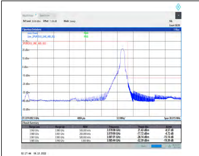
1-N77-3700-3980-PC2-30-20-H-2-DFT-QPSK-Edge_1 RB_Right-1@50-Ant1-1--PASS-see graph
