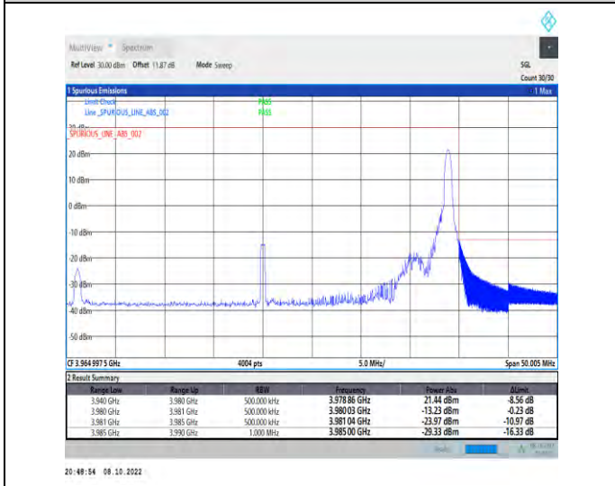
1-N77-3700-3980-PC2-30-40-H-5-CP-QPSK-Edge_1R B_Right-1@105-Ant1-1--PASS-see graph
