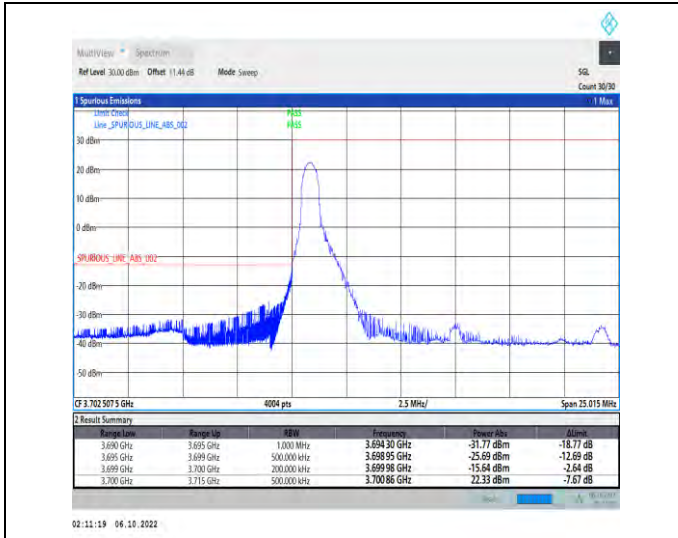
1-N77-3700-3980-PC2-30-15-L-1-DFT-QPSK-Edge_1 RB_Left-1@0-Ant1-1--PASS-see graph
