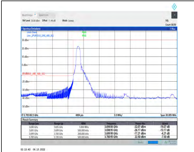
1-N77-3700-3980-PC2-30-20-L-1-DFT-QPSK-Edge_1 RB_Left-1@0-Ant1-1--PASS-see graph
