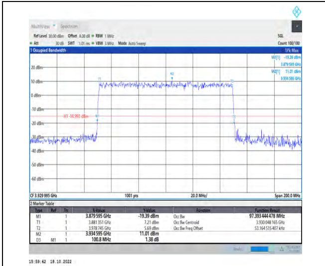
1-N77-3700-3980-PC2-30-100-H-6-CP-QPSK-Outer_Full-273@0-Ant1-97.393-100.800-≤100-PASS
