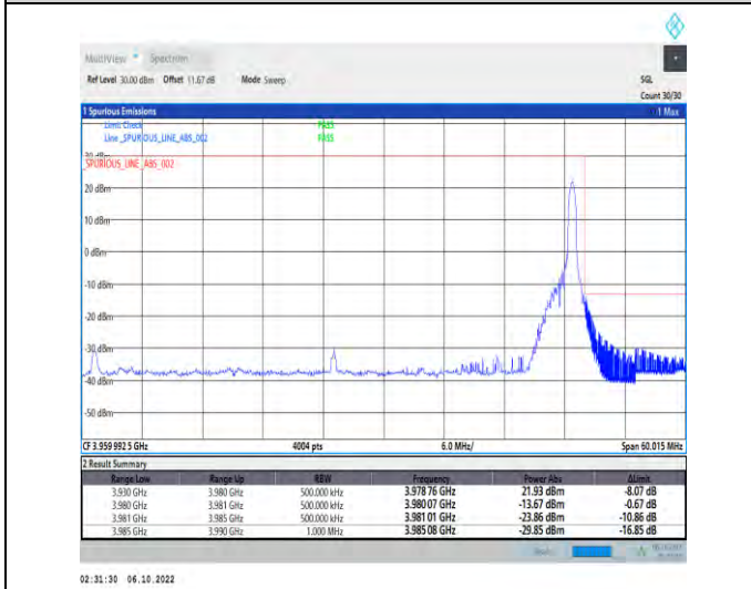
1-N77-3700-3980-PC2-30-50-H-5-CP-QPSK-Edge_1R B_Right-1@132-Ant1-1--PASS-see graph
