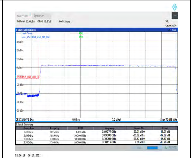
1-N77-3700-3980-PC2-30-60-L-6-CP-QPSK-Outer_Full-162@0-Ant1-1--PASS-see graph
