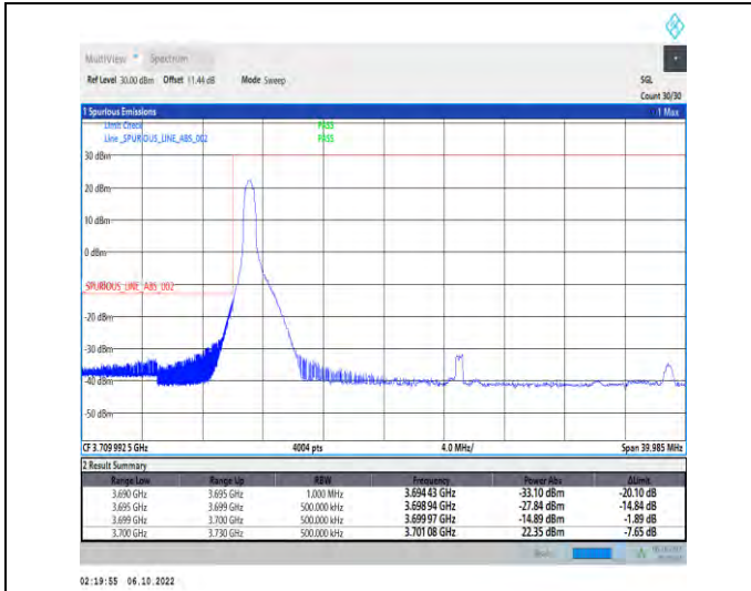
1-N77-3700-3980-PC2-30-30-L-1-DFT-QPSK-Edge_1 RB_Left-1@0-Ant1-1--PASS-see graph
