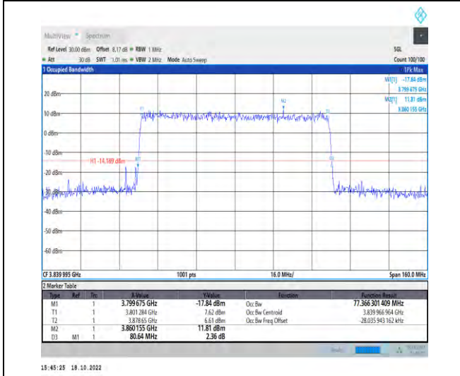
1-N77-3700-3980-PC2-30-80-M-8-CP-64QAM-Outer_Full-217@0-Ant1-77.366-80.640-≤80-PASS
