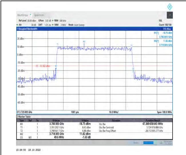
1-N77-3700-3980-PC2-30-50-L-6-CP-QPSK-Outer Full-133@0-Ant1-47.37-49.600-≤50-PASS
