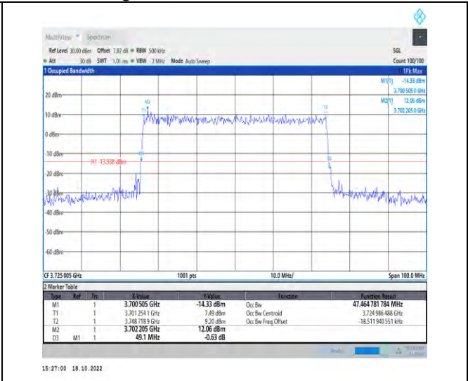
1-N77-3700-3980-PC2-30-50-L-7-CP-16QAM-Outer Full-133@0-Ant1-47.465-49.100-≤50-PASS
