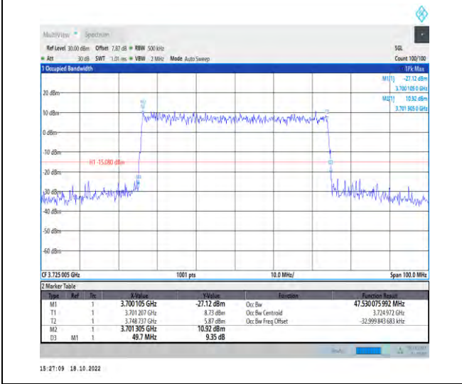
1-N77-3700-3980-PC2-30-50-L-8-CP-64QAM-Outer Full-133@0-Ant1-47.53-49.700-≤50-PASS
