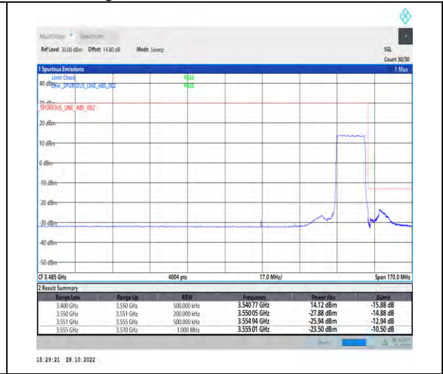
1-N77-3450-3550-PC2-30-15-H-3-DFT-PI2BPSK-Outer_Full-36@0-Ant1-1--PASS-see graph
