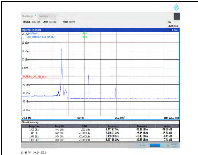
1-N77-3450-3550-PC2-30-70-L-1-DFT-PI2BPSK-Edge_1RB_Left-1@0-Ant1-1--PASS-see graph
