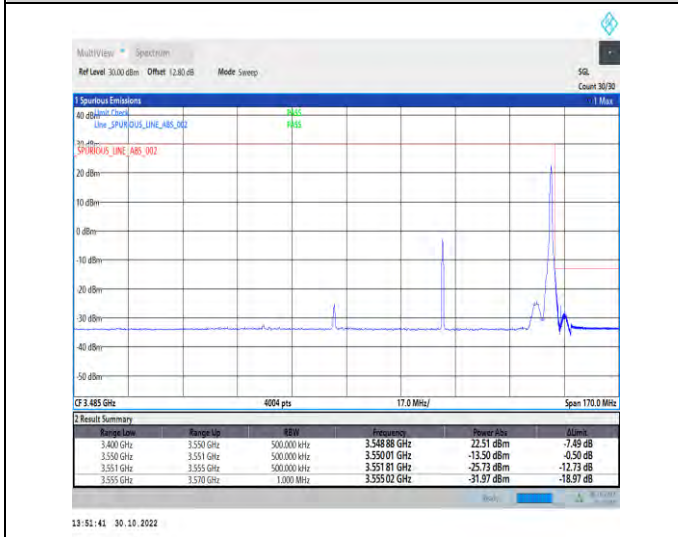
1-N77-3450-3550-PC2-30-70-H-5-CP-QPSK-Edge_1RB_Right-1@188-Ant1-1--PASS-see graph
