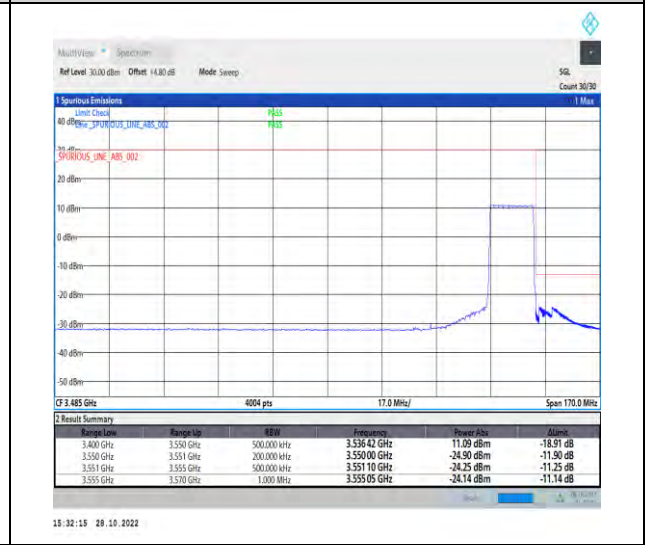
1-N77-3450-3550-PC2-30-15-H-6-CP-QPSK-Outer_Full-38@0-Ant1-1--PASS-see graph
