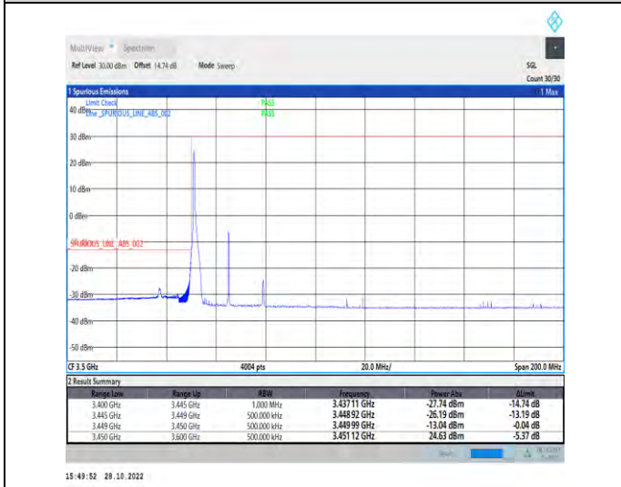
1-N77-3450-3550-PC2-30-30-L-4-CP-QPSK-Edge_1RB_Left-1@0-Ant1-1--PASS-see graph
