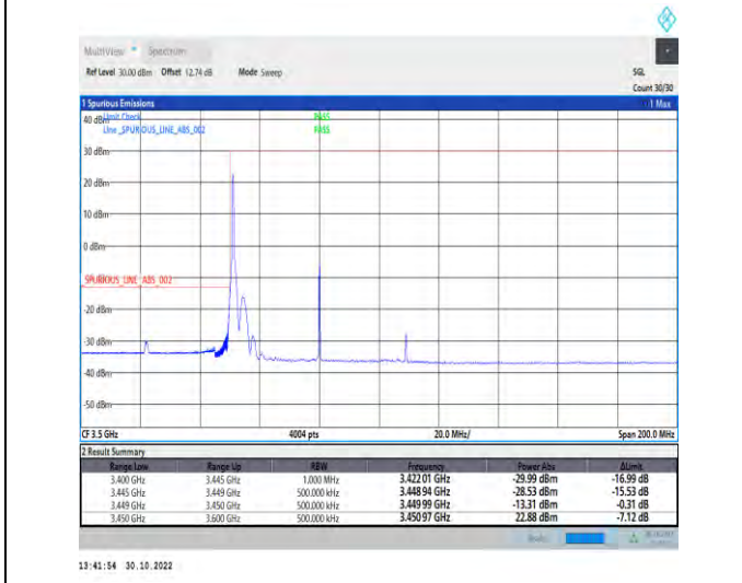
1-N77-3450-3550-PC2-30-60-L-4-CP-QPSK-Edge_1RB_Left-1@0-Ant1-1--PASS-see graph
