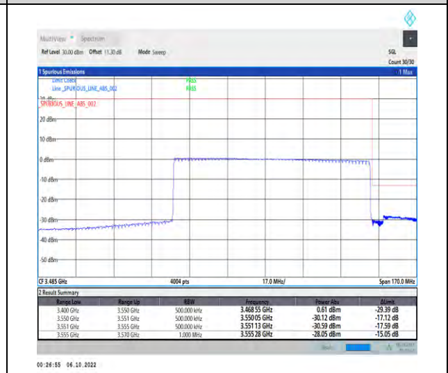
1-N77-3450-3550-PC2-30-90-H-6-DFT-PI2BPSK-Outer_Full-240@0-Ant1-1--PASS-see graph
