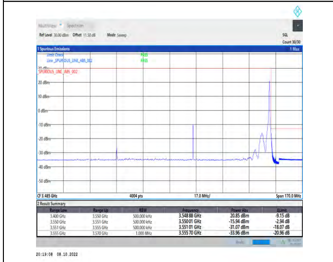
1-N77-3450-3550-PC2-30-100-H-5-CP-QPSK-Edge_1RB_Right-1@272-Ant1-1--PASS-see graph
