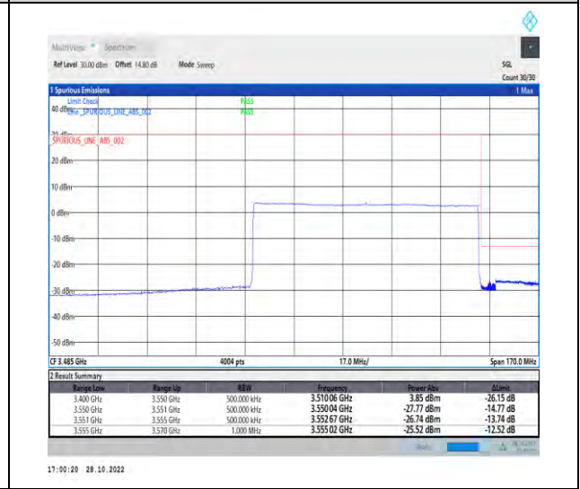
1-N77-3450-3550-PC2-30-80-H-6-CP-QPSK-Outer_Full-217@0-Ant1-1--PASS-see graph
