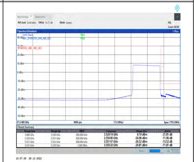
1-N77-3450-3550-PC2-30-30-H-6-CP-QPSK-Outer_Full-78@0-Ant1-1--PASS-see graph
