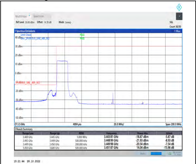
1-N77-3450-3550-PC2-30-15-L-3-DFT-PI2BPSK-Outer_Full-36@0-Ant1-1--PASS-see graph
