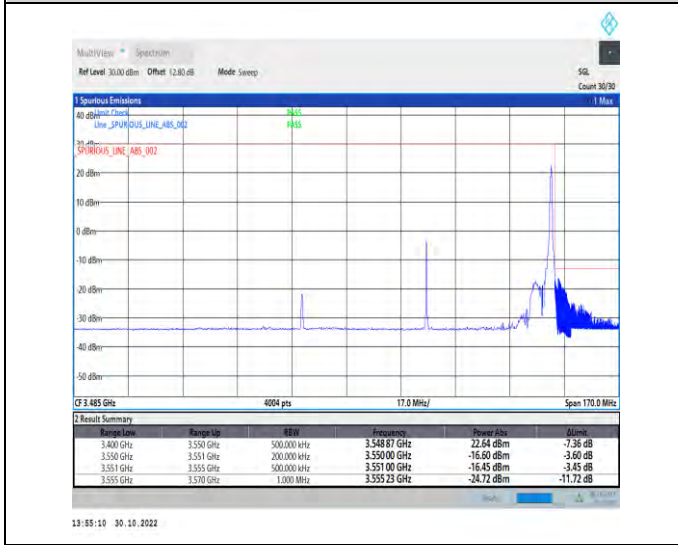
1-N77-3450-3550-PC2-30-80-H-5-CP-QPSK-Edge_1RB_Right-1@216-Ant1-1--PASS-see graph
