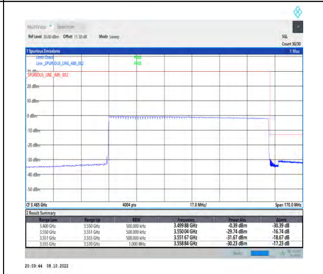
1-N77-3450-3550-PC2-30-100-H-6-CP-QPSK-Outer_Full-273@0-Ant1-1--PASS-see graph
