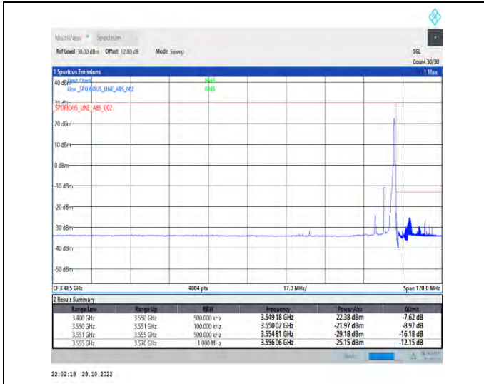
1-N77-3450-3550-PC2-30-10-H-2-DFT-PI2BPSK-Edge_1RB_Right-1@23-Ant1-1--PASS-see graph
