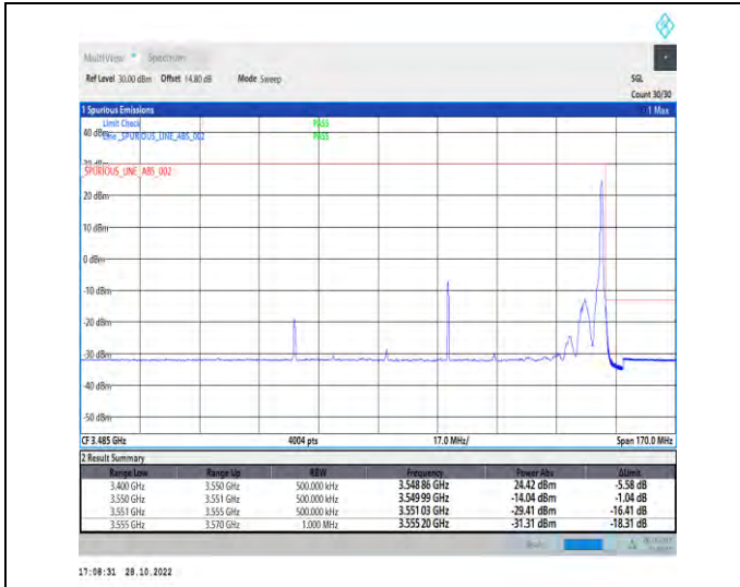
1-N77-3450-3550-PC2-30-90-H-2-DFT-PI2BPSK-Edge_1RB_Right-1@244-Ant1-1--PASS-see graph
