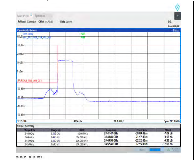
1-N77-3450-3550-PC2-30-20-L-3-DFT-PI2BPSK-Outer_Full-50@0-Ant1-1--PASS-see graph
