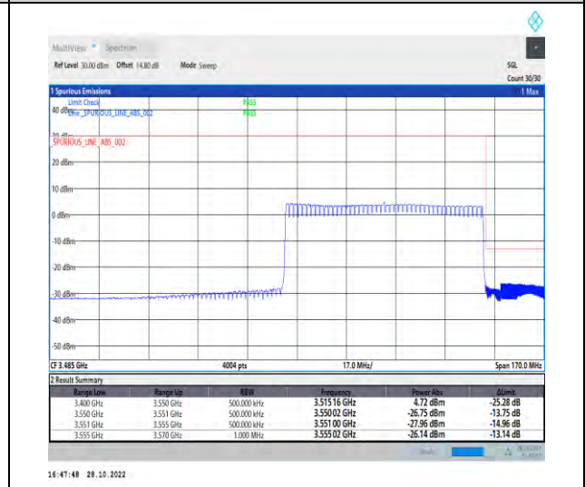
1-N77-3450-3550-PC2-30-70-H-6-CP-QPSK-Outer_Full-189@0-Ant1-1--PASS-see graph
