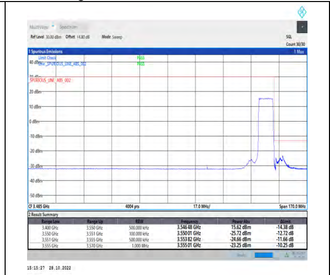
1-N77-3450-3550-PC2-30-10-H-3-DFT-PI2BPSK-Outer_Full-24@0-Ant1-1--PASS-see graph
