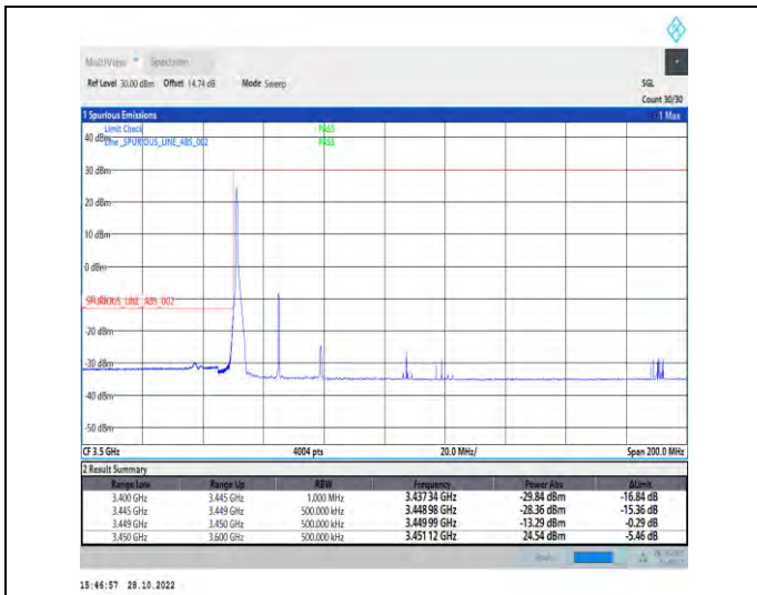
1-N77-3450-3550-PC2-30-30-L-1-DFT-PI2BPSK-Edge_1RB_Left-1@0-Ant1-1--PASS-see graph
