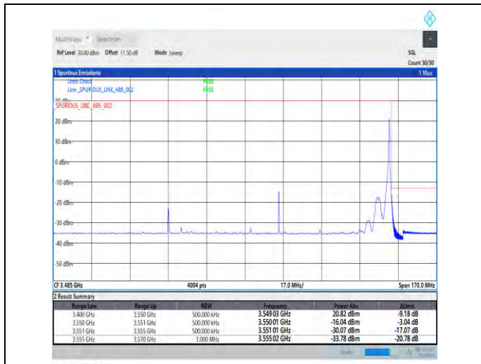
1-N77-3450-3550-PC2-30-100-H-2-DFT-QPSK-Edge_1RB_Right-1@272-Ant1-1--PASS-see graph
