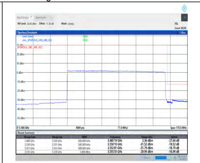
1-N77-3450-3550-PC2-30-100-H-3-DFT-QPSK-Outer_Full-270@0-Ant1-1--PASS-see graph
