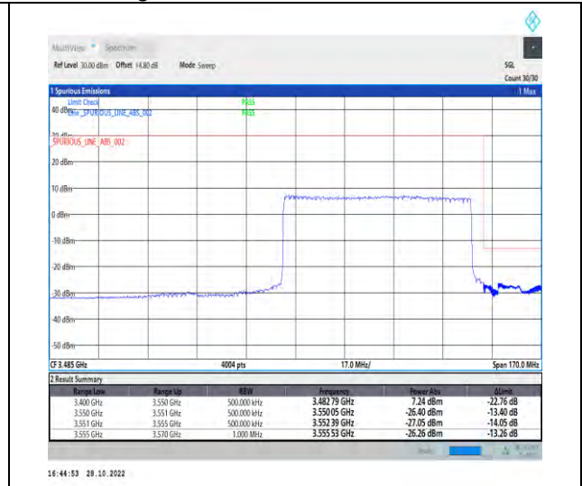
1-N77-3450-3550-PC2-30-70-H-3-DFT-PI2BPSK-Outer_Full-180@0-Ant1-1--PASS-see graph
