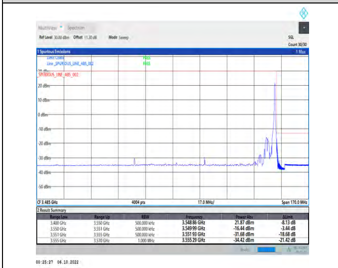
1-N77-3450-3550-PC2-30-90-H-5-DFT-PI2BPSK-Edge_1RB_Right-1@244-Ant1-1--PASS-see graph
