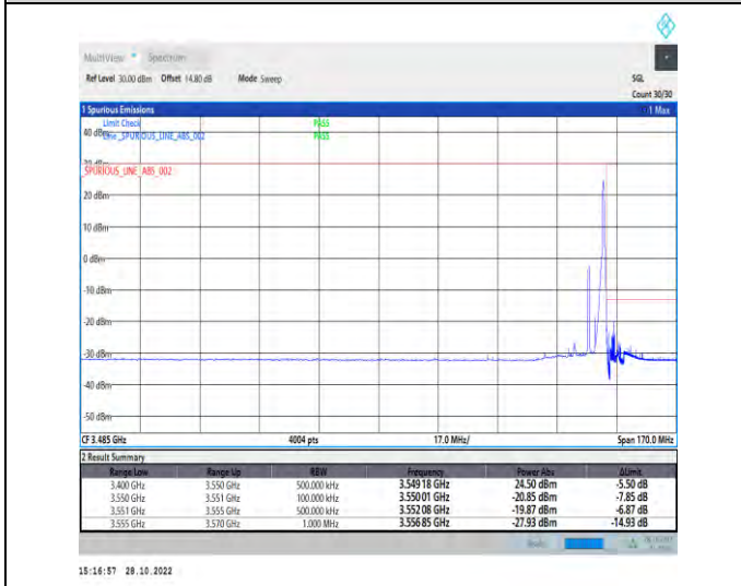
1-N77-3450-3550-PC2-30-10-H-5-CP-QPSK-Edge_1RB_Right-1@23-Ant1-1--PASS-see graph
