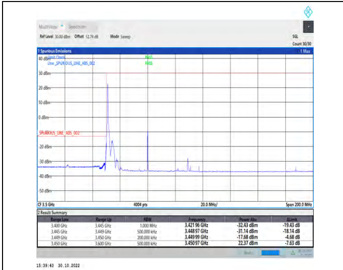
1-N77-3450-3550-PC2-30-60-L-1-DFT-PI2BPSK-Edge_1RB_Left-1@0-Ant1-1--PASS-see graph
