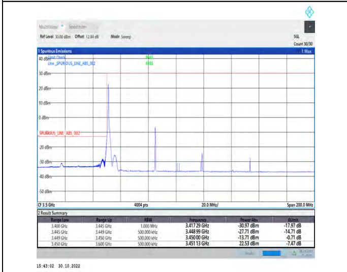
1-N77-3450-3550-PC2-30-70-L-4-CP-QPSK-Edge_1RB_Left-1@0-Ant1-1--PASS-see graph
