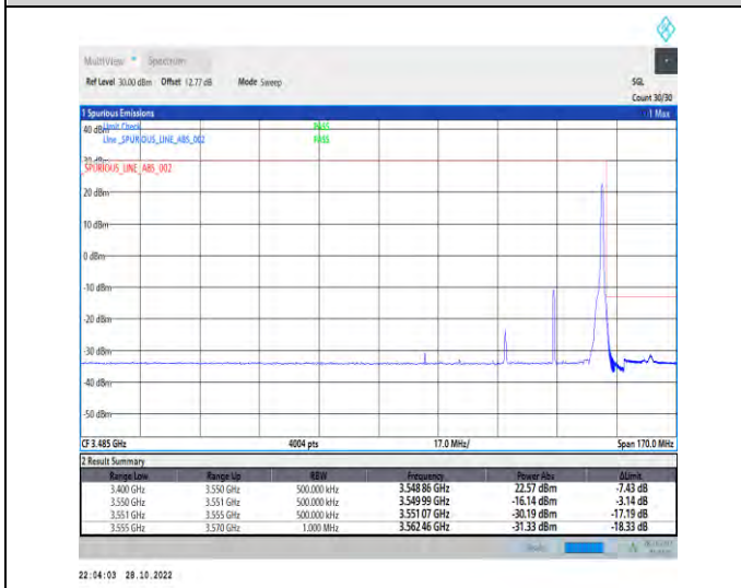
1-N77-3450-3550-PC2-30-30-H-5-CP-QPSK-Edge_1RB_Right-1@77-Ant1-1--PASS-see graph
