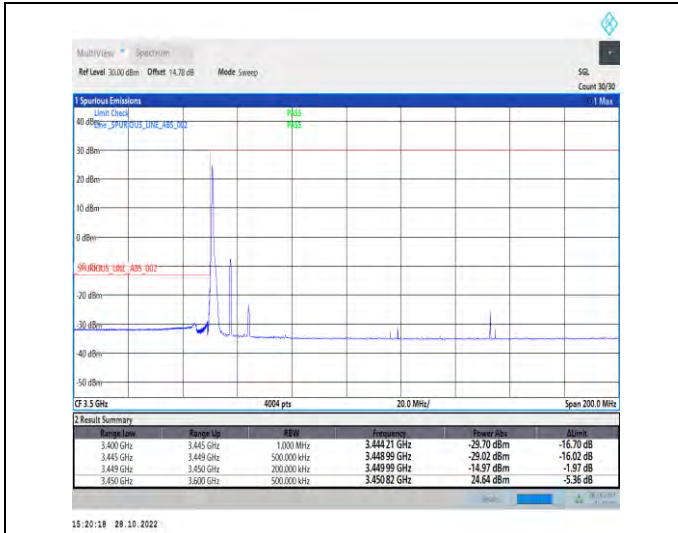
1-N77-3450-3550-PC2-30-15-L-1-DFT-PI2BPSK-Edge_1RB_Left-1@0-Ant1-1--PASS-see graph
