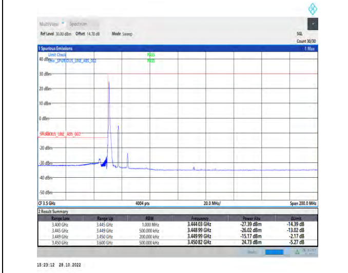
1-N77-3450-3550-PC2-30-15-L-4-CP-QPSK-Edge_1RB_Left-1@0-Ant1-1--PASS-see graph
