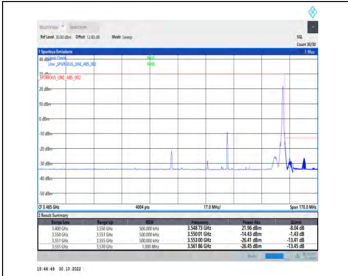
1-N77-3450-3550-PC2-30-70-H-2-DFT-PI2BPSK-Edge_1RB_Right-1@188-Ant1-1--PASS-see graph
