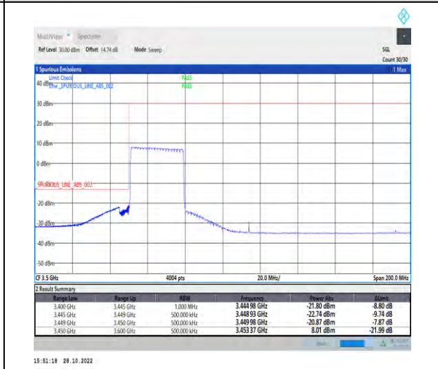
1-N77-3450-3550-PC2-30-30-L-6-CP-QPSK-Outer_Full-78@0-Ant1-1--PASS-see graph
