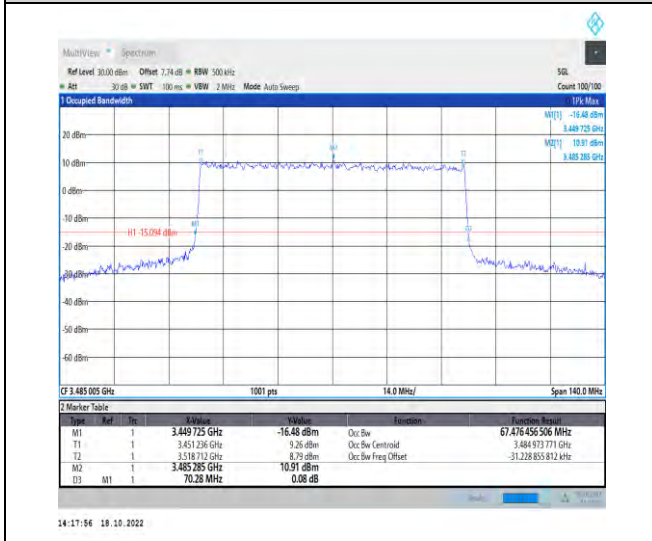
1-N77-3450-3550-PC2-30-70-L-8-CP-64QAM-Outer_Full-189@0-Ant1-67.476-70.280-≤70-PASS
