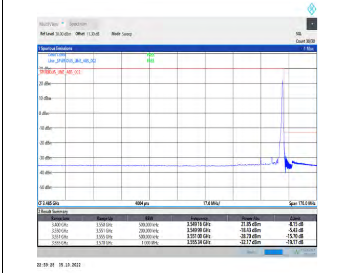
1-N77-3450-3550-PC2-30-15-H-5-CP-QPSK-Edge_1R B_Right-1@37-Ant1-1--PASS-see graph
