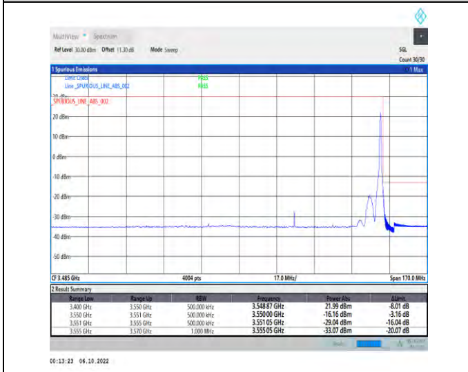
1-N77-3450-3550-PC2-30-80-H-5-CP-QPSK-Edge_1R B_Right-1@216-Ant1-1--PASS-see graph
