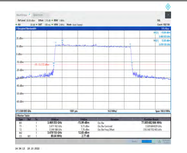
1-N77-3450-3550-PC2-30-80-H-5-DFT-256QAM-Outer_Full-216@0-Ant1-77.006-80.640-≤80-PASS
