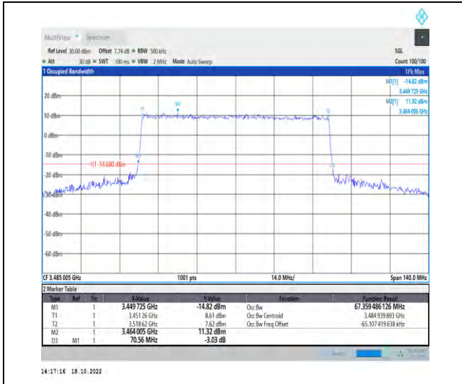
1-N77-3450-3550-PC2-30-70-L-6-CP-QPSK-Outer_Full-189@0-Ant1-67.359-70.560-≤70-PASS
