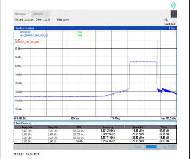
1-N77-3450-3550-PC2-30-30-H-6-CP-QPSK-Outer _Full-78@0-Ant1-1--PASS-see graph
