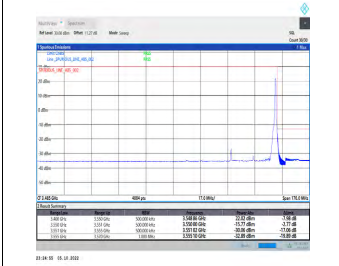
1-N77-3450-3550-PC2-30-30-H-5-CP-QPSK-Edge_1R B_Right-1@77-Ant1-1--PASS-see graph
