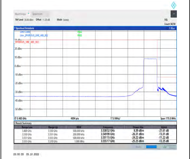
1-N77-3450-3550-PC2-30-15-H-6-CP-QPSK-Outer _Full-38@0-Ant1-1--PASS-see graph
