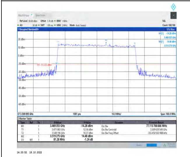
1-N77-3450-3550-PC2-30-80-H-4-DFT-64QAM-Outer_Full-216@0-Ant1-77.114-81.280-≤80-PASS
