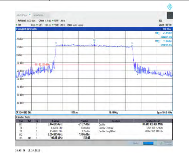
1-N77-3450-3550-PC2-30-90-H-7-CP-16QAM-Outer_Full-245@0-Ant1-87.447-109.980-<=90-PASS
