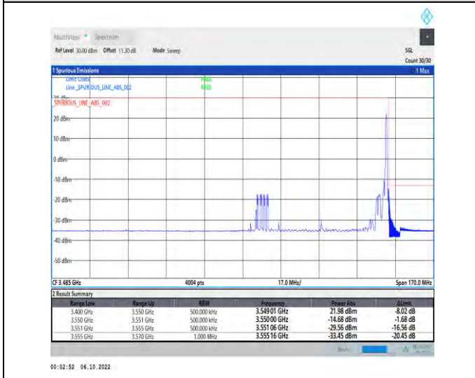
1-N77-3450-3550-PC2-30-60-H-5-CP-QPSK-Edge_1R B_Right-1@161-Ant1-1--PASS-see graph
