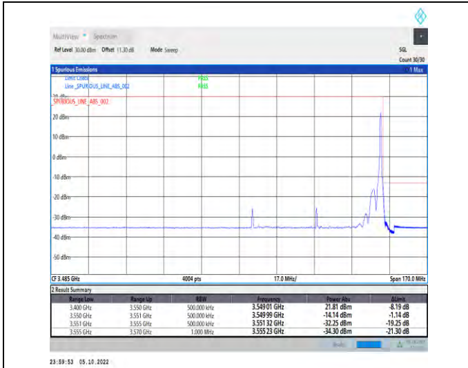
1-N77-3450-3550-PC2-30-60-H-2-DFT-QPSK-Edge_1 RB_Right-1@161-Ant1-1--PASS-see graph
