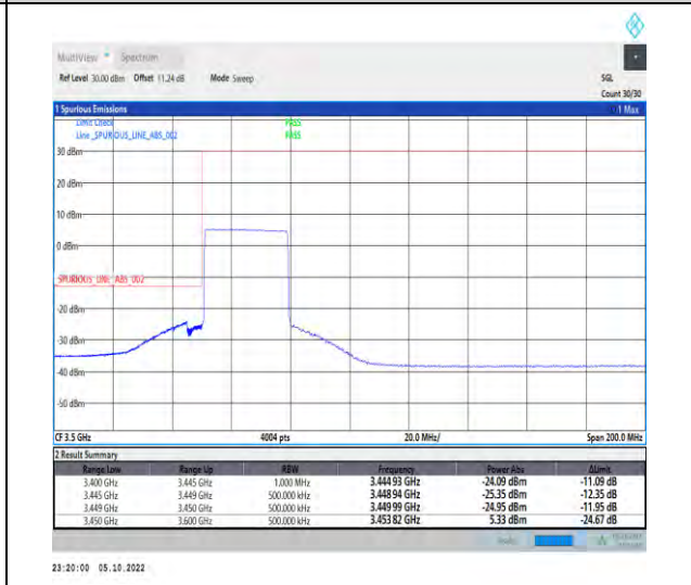
1-N77-3450-3550-PC2-30-30-L-6-CP-QPSK-Outer_Full-78@0-Ant1-1--PASS-see graph
