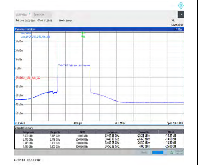
1-N77-3450-3550-PC2-30-40-L-6-CP-QPSK-Outer_Full-106@0-Ant1-1--PASS-see graph
