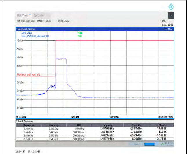
1-N77-3450-3550-PC2-30-15-L-6-CP-QPSK-Outer_Full-38@0-Ant1-1--PASS-see graph
