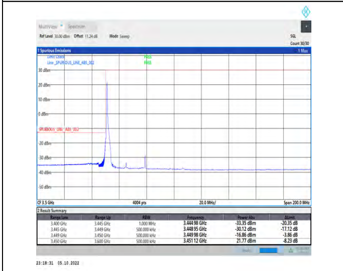
1-N77-3450-3550-PC2-30-30-L-4-CP-QPSK-Edge_1R B_Left-1@0-Ant1-1--PASS-see graph
