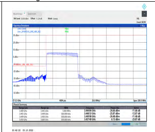
1-N77-3450-3550-PC2-30-50-L-3-DFT-QPSK-Outer_Full-128@0-Ant1-1--PASS-see graph
