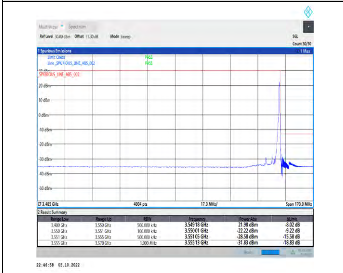
1-N77-3450-3550-PC2-30-10-H-5-CP-QPSK-Edge_1R B_Right-1@23-Ant1-1--PASS-see graph
