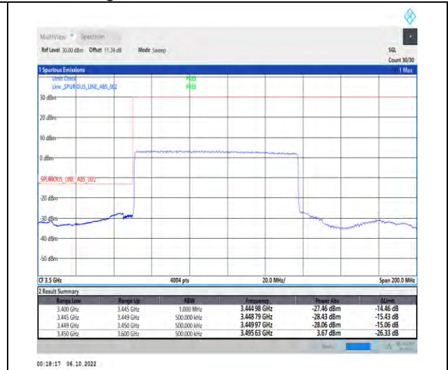
1-N77-3450-3550-PC2-30-90-L-3-DFT-QPSK-Outer_Full-240@0-Ant1-1--PASS-see graph
