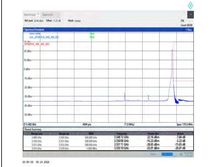
1-N77-3450-3550-PC2-30-50-H-5-CP-QPSK-Edge_1R B_Right-1@132-Ant1-1--PASS-see graph
