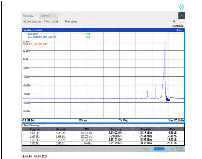
1-N77-3450-3550-PC2-30-20-H-2-DFT-QPSK-Edge_1 RB_Right-1@50-Ant1-1--PASS-see graph
