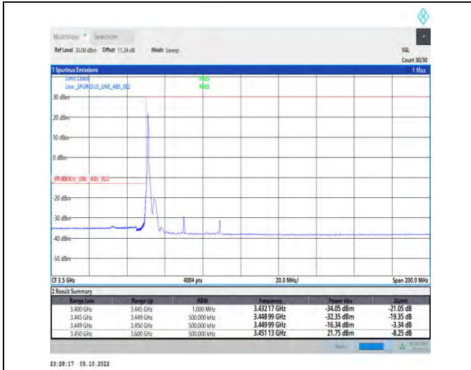
1-N77-3450-3550-PC2-30-40-L-1-DFT-QPSK-Edge_1 RB_Left-1@0-Ant1-1--PASS-see graph
