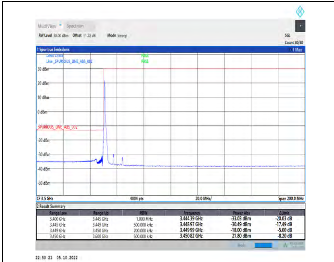
1-N77-3450-3550-PC2-30-15-L-1-DFT-QPSK-Edge_1 RB_Left-1@0-Ant1-1--PASS-see graph
