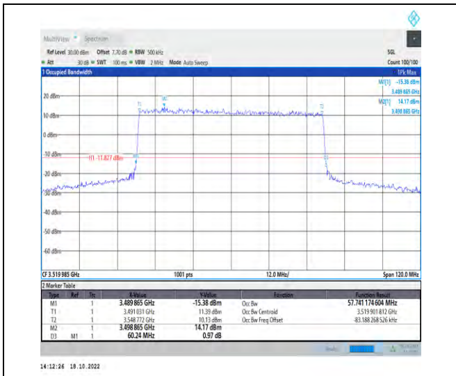
1-N77-3450-3550-PC2-30-60-H-1-DFT-QPSK-Outer_Full-162@0-Ant1-57.741-60.240-≤60-PASS
