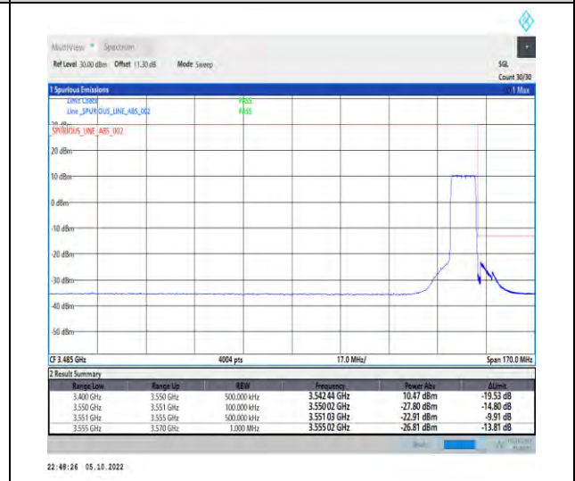
1-N77-3450-3550-PC2-30-10-H-6-CP-QPSK-Outer _Full-24@0-Ant1-1--PASS-see graph
