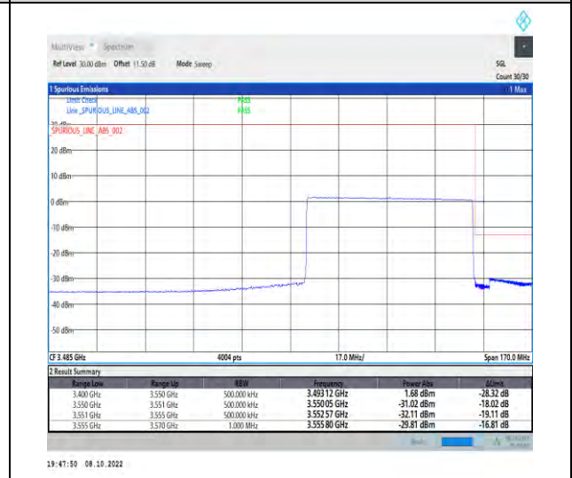
1-N77-3450-3550-PC2-30-60-H-6-CP-QPSK-Outer _Full-162@0-Ant1-1--PASS-see graph
