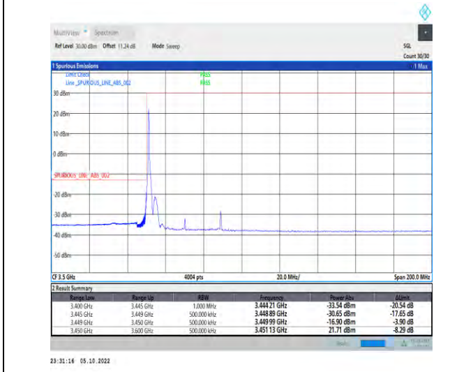
1-N77-3450-3550-PC2-30-40-L-4-CP-QPSK-Edge_1R B_Left-1@0-Ant1-1--PASS-see graph
