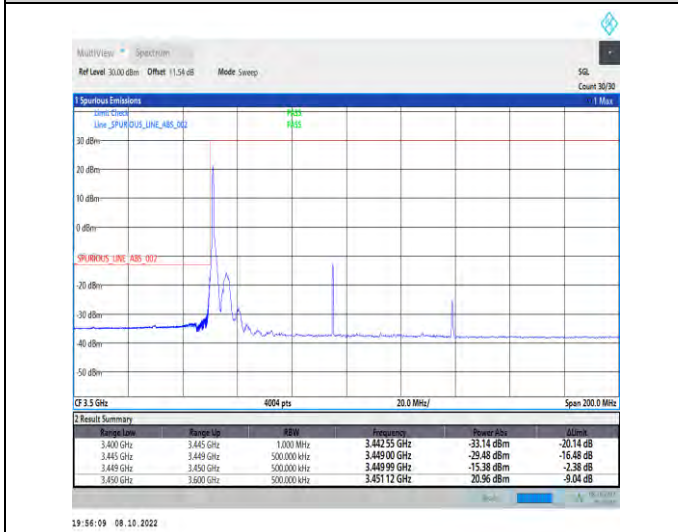
1-N77-3450-3550-PC2-30-90-L-4-CP-QPSK-Edge_1R B_Left-1@0-Ant1-1--PASS-see graph
