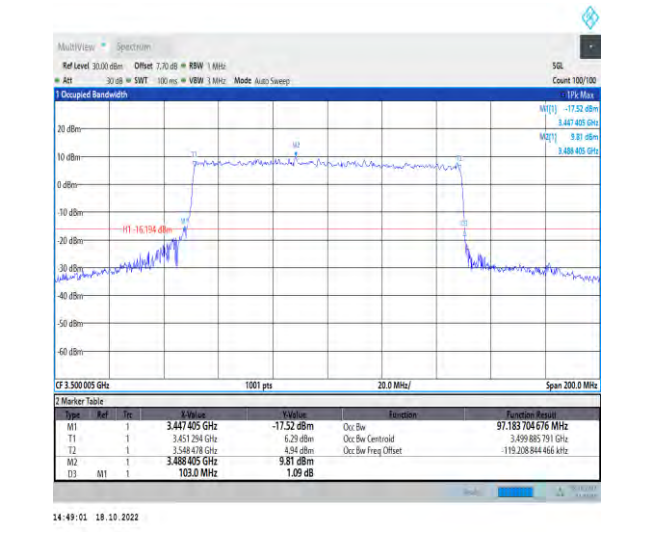
1-N77-3450-3550-PC2-30-100-L-9-CP-256QAM-Outer_Full-273@0-Ant1-97.184-103.000-≤100-PASS
