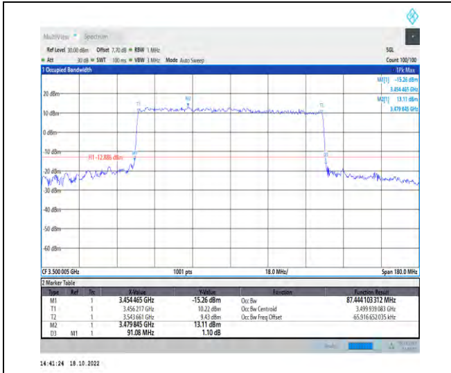
1-N77-3450-3550-PC2-30-90-M-6-CP-QPSK-Outer_Full-245@0-Ant1-87.444-91.080-≤90-PASS
