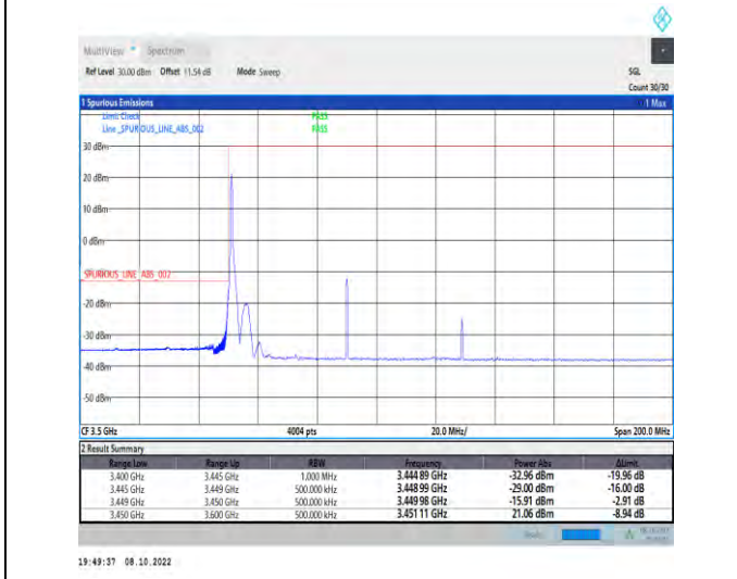
1-N77-3450-3550-PC2-30-80-L-4-CP-QPSK-Edge_1R B_Left-1@0-Ant1-1--PASS-see graph
