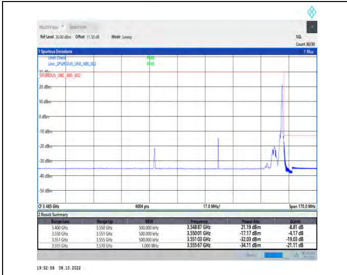
1-N77-3450-3550-PC2-30-80-H-2-DFT-QPSK-Edge_1 RB_Right-1@216-Ant1-1--PASS-see graph
