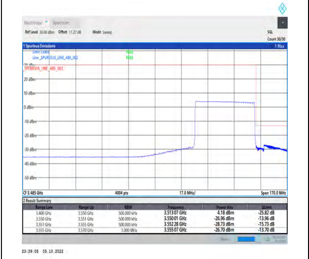
1-N77-3450-3550-PC2-30-40-H-6-CP-QPSK-Outer _Full-106@0-Ant1-1--PASS-see graph
