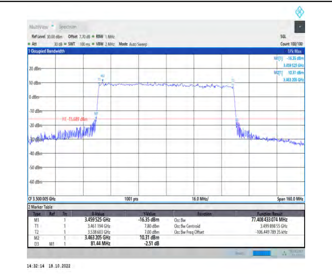
1-N77-3450-3550-PC2-30-80-M-9-CP-256QAM-Outer_Full-217@0-Ant1-77.408-81.440-≤80-PASS
