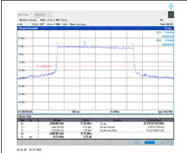
1-N77-3450-3550-PC2-30-70-M-8-CP-64QAM-Outer_Full-189@0-Ant1-67.377-70.140-≤70-PASS
