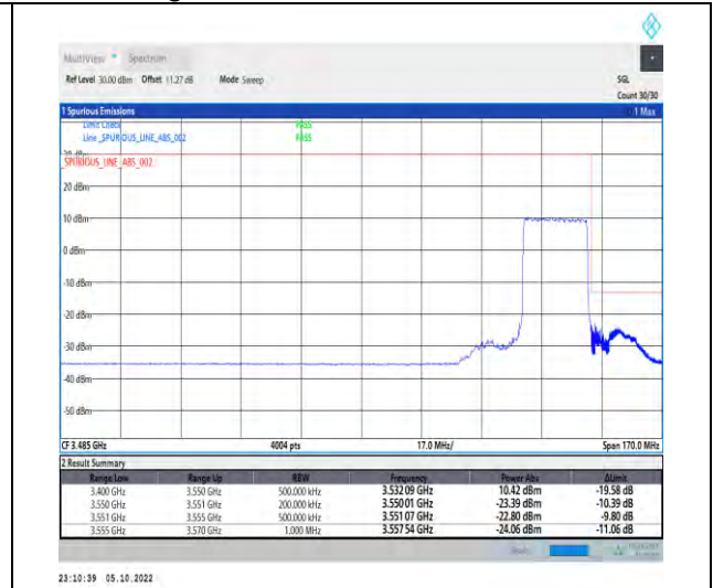
1-N77-3450-3550-PC2-30-20-H-3-DFT-QPSK-Out er_Full-50@0-Ant1-1--PASS-see graph
