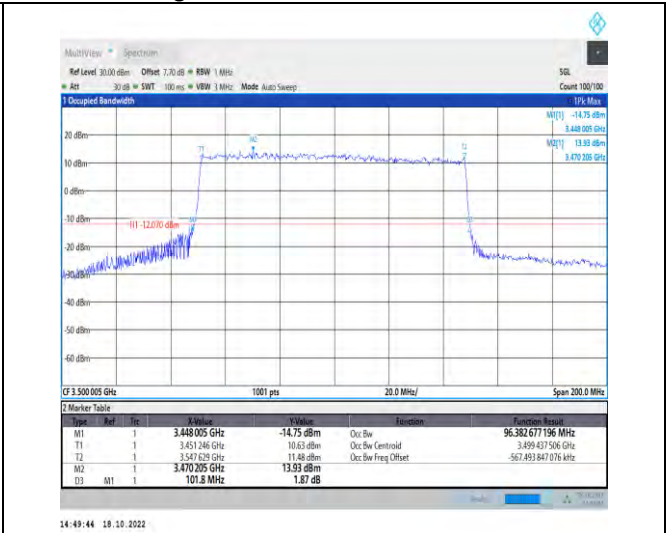
1-N77-3450-3550-PC2-30-100-M-3-DFT-16QAM-Out er_Full-270@0-Ant1-96.383-101.800-≤100-PASS
