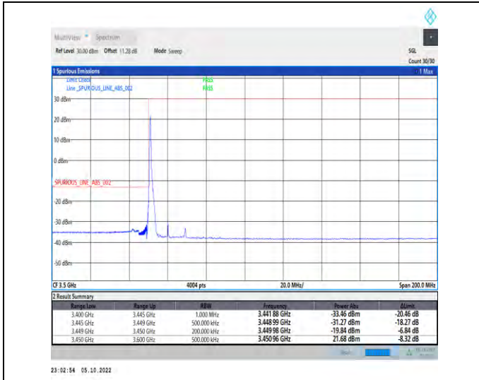
1-N77-3450-3550-PC2-30-20-L-1-DFT-QPSK-Edge_1 RB_Left-1@0-Ant1-1--PASS-see graph
