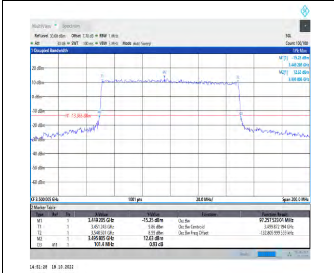
1-N77-3450-3550-PC2-30-100-M-8-CP-64QAM-Outer_Full-273@0-Ant1-97.258-101.400-≤100-PASS
