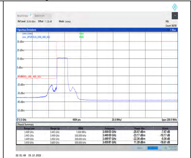
1-N77-3450-3550-PC2-30-15-L-3-DFT-QPSK-Outer_Full-36@0-Ant1-1--PASS-see graph
