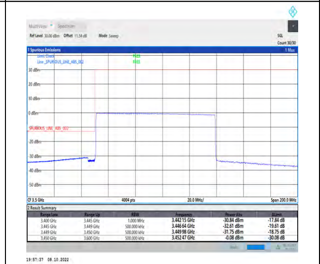
1-N77-3450-3550-PC2-30-90-L-6-CP-QPSK-Outer_Full-245@0-Ant1-1--PASS-see graph
