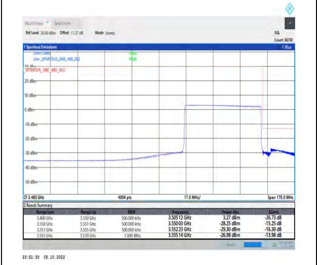
1-N77-3450-3550-PC2-30-50-H-6-CP-QPSK-Outer _Full-133@0-Ant1-1--PASS-see graph
