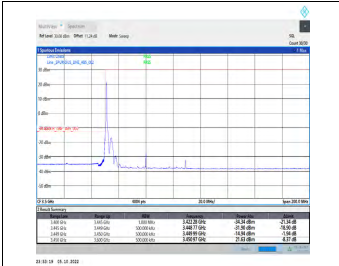
1-N77-3450-3550-PC2-30-60-L-1-DFT-QPSK-Edge_1 RB_Left-1@0-Ant1-1--PASS-see graph
