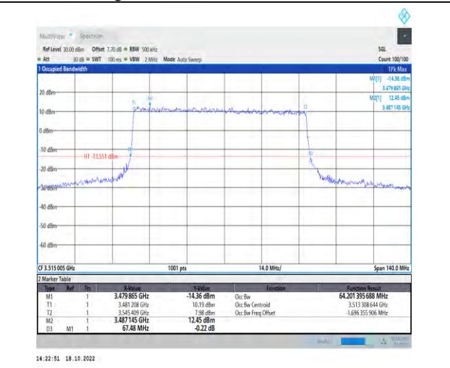
1-N77-3450-3550-PC2-30-70-H-3-DFT-16QAM-Outer_Full-180@0-Ant1-64.201-67.480-≤70-PASS
