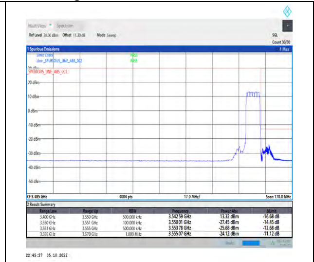
1-N77-3450-3550-PC2-30-10-H-3-DFT-QPSK-Out er_Full-24@0-Ant1-1--PASS-see graph
