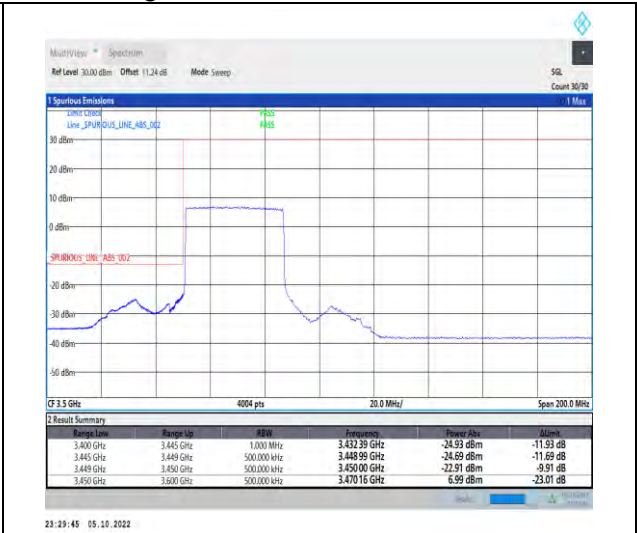
1-N77-3450-3550-PC2-30-40-L-3-DFT-QPSK-Outer_Full-100@0-Ant1-1--PASS-see graph
