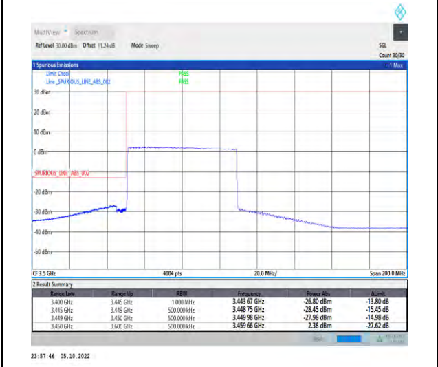
1-N77-3450-3550-PC2-30-60-L-6-CP-QPSK-Outer_Full-162@0-Ant1-1--PASS-see graph
