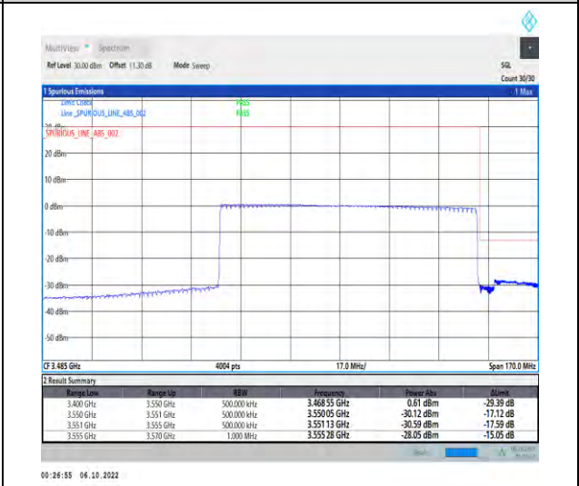
1-N77-3450-3550-PC2-30-90-H-6-CP-QPSK-Outer _Full-245@0-Ant1-1--PASS-see graph
