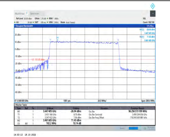
1-N77-3450-3550-PC2-30-100-H-5-DFT-256QAM-Outer_Full-270@0-Ant1-96.257-102.200-≤100-PASS
