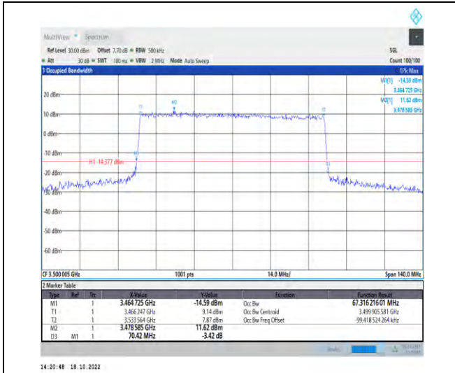
1-N77-3450-3550-PC2-30-70-M-6-CP-QPSK-Outer_Full-189@0-Ant1-67.316-70.420-≤70-PASS
