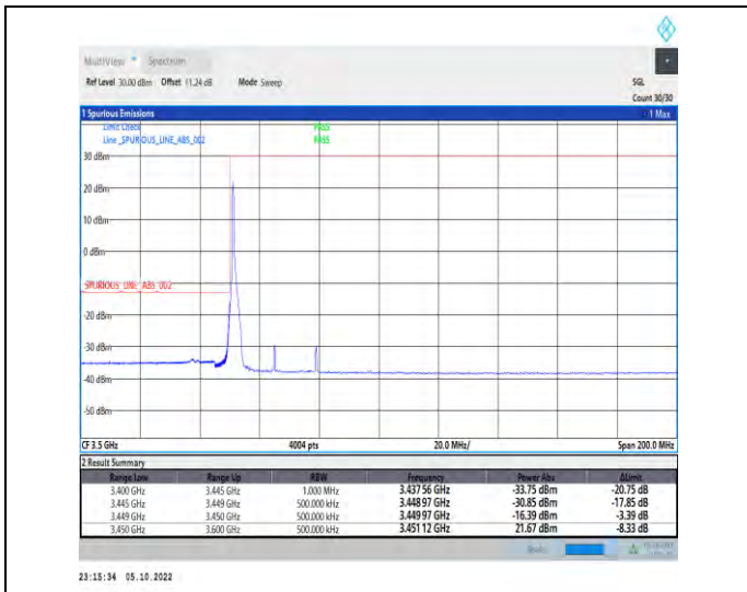
1-N77-3450-3550-PC2-30-30-L-1-DFT-QPSK-Edge_1 RB_Left-1@0-Ant1-1--PASS-see graph
