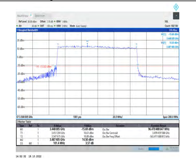
1-N77-3450-3550-PC2-30-100-H-3-DFT-16QAM-Outer_Full-270@0-Ant1-96.47-101.400-≤100-PASS
