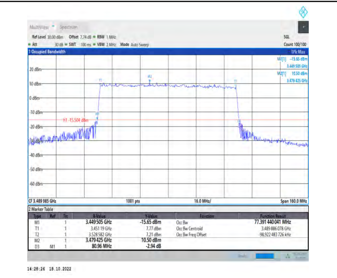
1-N77-3450-3550-PC2-30-80-L-9-CP-256QAM-Outer_Full-217@0-Ant1-77.391-80.960-≤80-PASS
