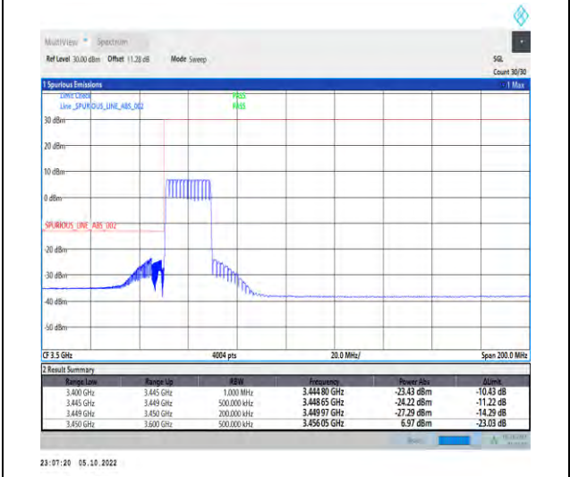
1-N77-3450-3550-PC2-30-20-L-6-CP-QPSK-Outer_Full-51@0-Ant1-1--PASS-see graph
