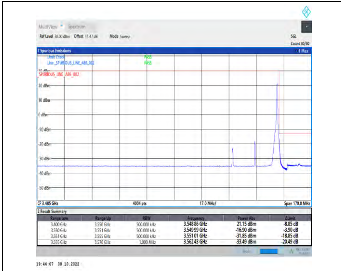
1-N77-3450-3550-PC2-30-30-H-2-DFT-QPSK-Edge_1 RB_Right-1@77-Ant1-1--PASS-see graph
