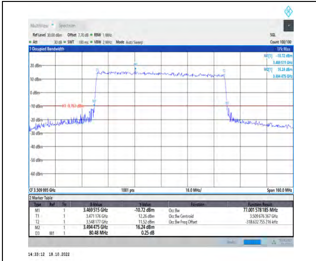
1-N77-3450-3550-PC2-30-80-H-1-DFT-QPSK-Outer_Full-216@0-Ant1-77.002-80.480-≤80-PASS
