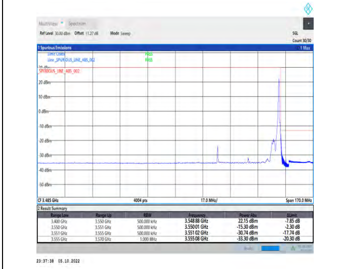
1-N77-3450-3550-PC2-30-40-H-5-CP-QPSK-Edge_1R B_Right-1@105-Ant1-1--PASS-see graph
