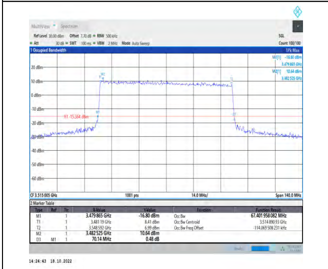
1-N77-3450-3550-PC2-30-70-H-8-CP-64QAM-Outer_Full-189@0-Ant1-67.402-70.140-≤70-PASS
