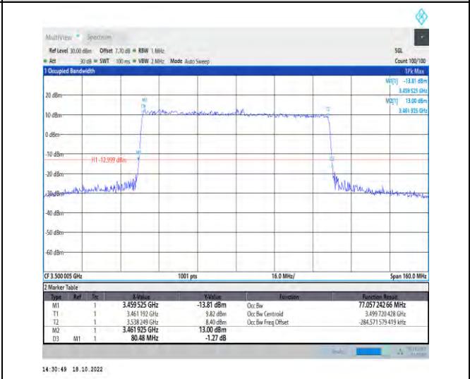
1-N77-3450-3550-PC2-30-80-M-5-DFT-256QAM-Outer_Full-216@0-Ant1-77.057-80.480-≤80-PASS
