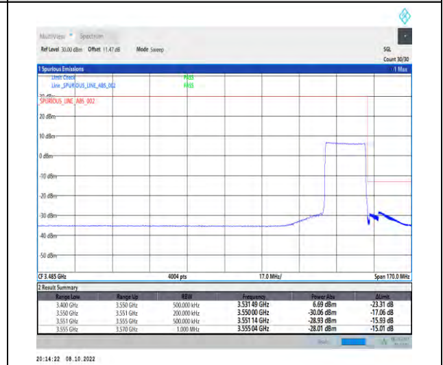
1-N77-3450-3550-PC2-30-20-H-6-CP-QPSK-Outer _Full-51@0-Ant1-1--PASS-see graph
