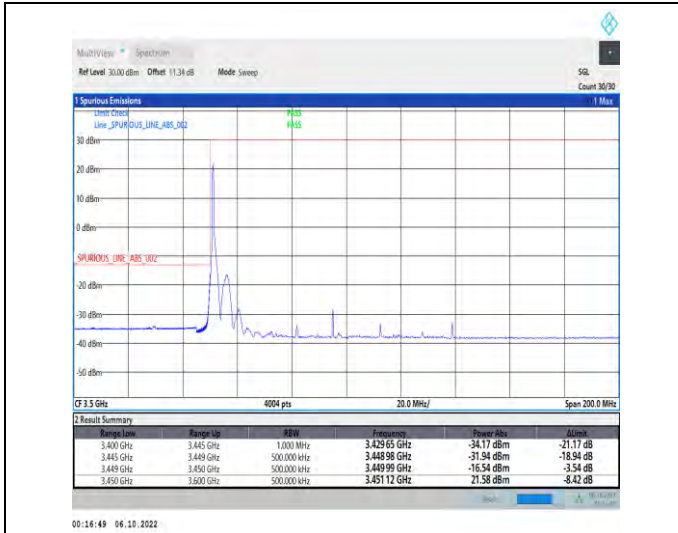
1-N77-3450-3550-PC2-30-90-L-1-DFT-QPSK-Edge_1 RB_Left-1@0-Ant1-1--PASS-see graph
