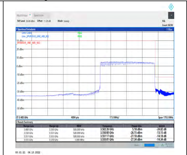
1-N77-3450-3550-PC2-30-60-H-3-DFT-QPSK-Out er_Full-162@0-Ant1-1--PASS-see graph
