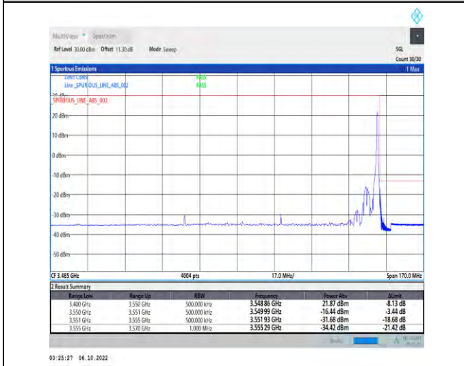
1-N77-3450-3550-PC2-30-90-H-5-CP-QPSK-Edge_1R B_Right-1@244-Ant1-1--PASS-see graph
