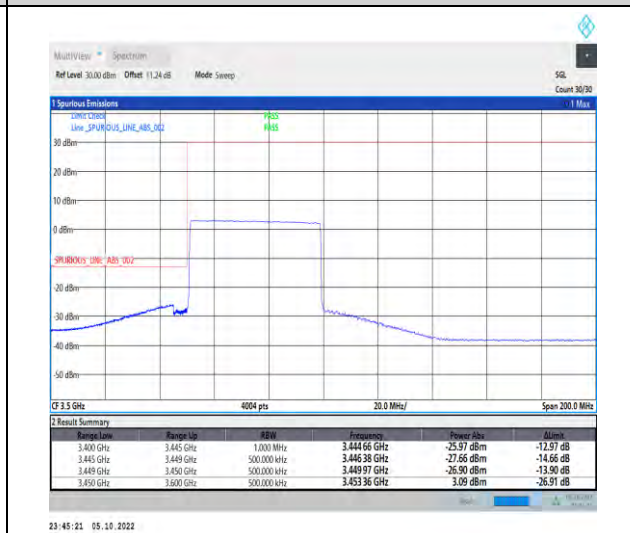
1-N77-3450-3550-PC2-30-50-L-6-CP-QPSK-Outer_Full-133@0-Ant1-1--PASS-see graph
