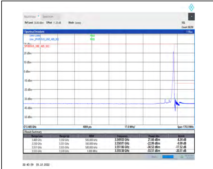
1-N77-3450-3550-PC2-30-10-H-2-DFT-QPSK-Edge_1 RB_Right-1@23-Ant1-1--PASS-see graph
