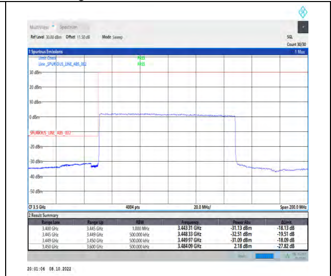
1-N77-3450-3550-PC2-30-100-L-3-DFT-QPSK-Out er_Full-270@0-Ant1-1--PASS-see graph
