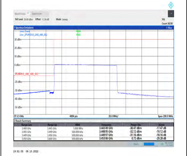
1-N77-3450-3550-PC2-30-80-L-6-CP-QPSK-Outer_Full-217@0-Ant1-1--PASS-see graph
