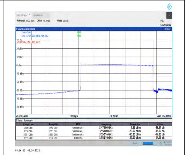
1-N77-3450-3550-PC2-30-80-H-6-CP-QPSK-Outer _Full-217@0-Ant1-1--PASS-see graph
