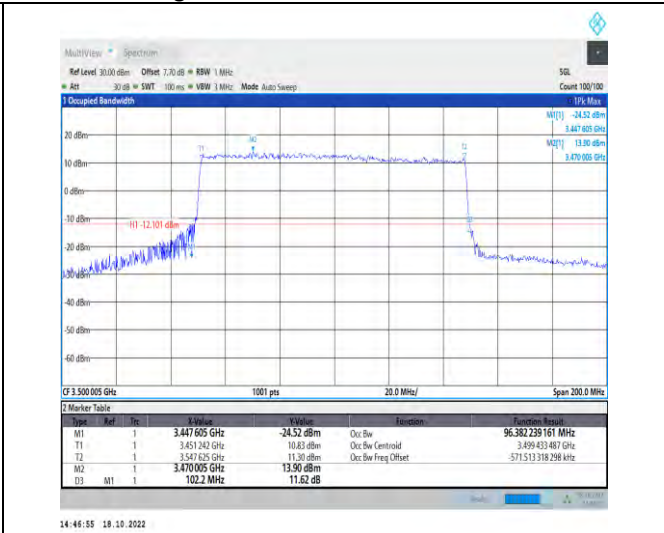
1-N77-3450-3550-PC2-30-100-L-3-DFT-16QAM-Outer_Full-270@0-Ant1-96.382-102.200-≤100-PASS
