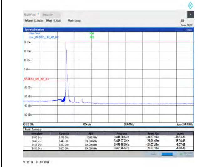
1-N77-3450-3550-PC2-30-20-L-4-CP-QPSK-Edge_1R B_Left-1@0-Ant1-1--PASS-see graph
