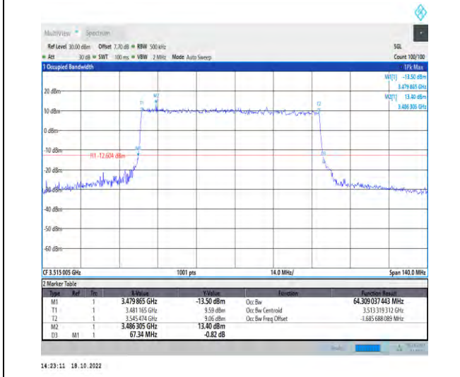
1-N77-3450-3550-PC2-30-70-H-4-DFT-64QAM-Outer_Full-180@0-Ant1-64.309-67.340-≤70-PASS
