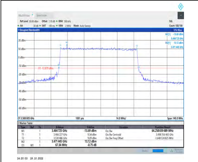
1-N77-3450-3550-PC2-30-70-M-4-DFT-64QAM-Outer_Full-180@0-Ant1-64.259-67.340-≤70-PASS
