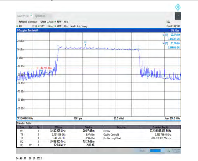
1-N77-3450-3550-PC2-30-100-L-7-CP-16QAM-Outer_Full-273@0-Ant1-97.44-129.400-≤100-PASS
