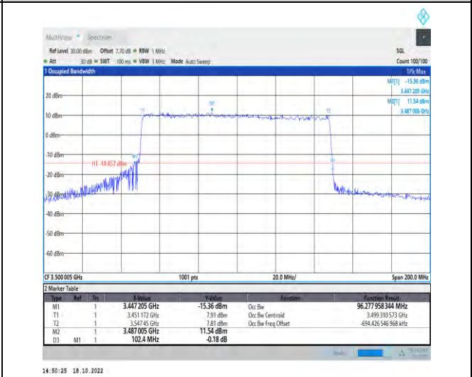
1-N77-3450-3550-PC2-30-100-M-5-DFT-256QAM-Out er_Full-270@0-Ant1-96.278-102.400-≤100-PASS
