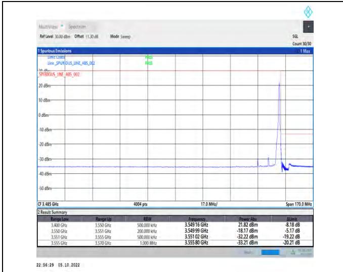
1-N77-3450-3550-PC2-30-15-H-2-DFT-QPSK-Edge_1 RB_Right-1@37-Ant1-1--PASS-see graph
