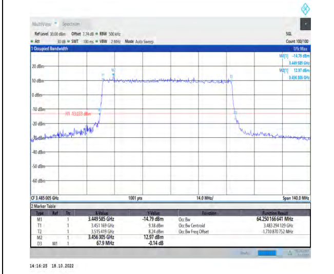
1-N77-3450-3550-PC2-30-70-L-4-DFT-64QAM-Outer_Full-180@0-Ant1-64.25-67.900-<=70-PASS
