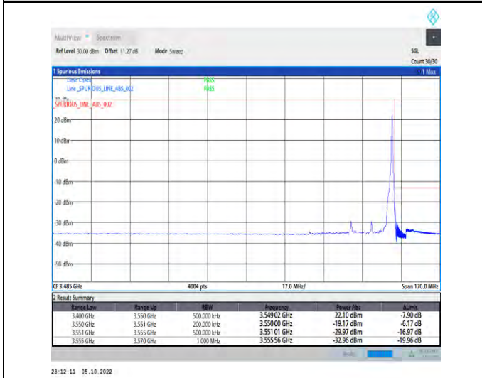
1-N77-3450-3550-PC2-30-20-H-5-CP-QPSK-Edge_1R B_Right-1@50-Ant1-1--PASS-see graph
