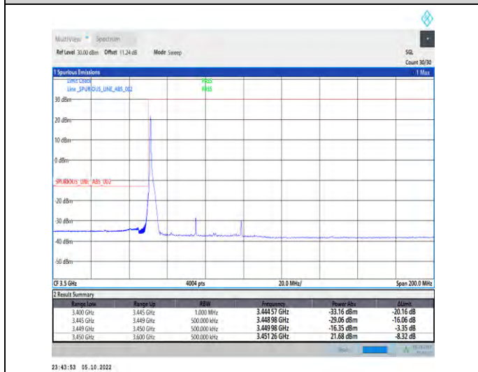
1-N77-3450-3550-PC2-30-50-L-4-CP-QPSK-Edge_1R B_Left-1@0-Ant1-1--PASS-see graph
