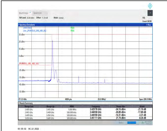
1-N77-3450-3550-PC2-30-80-L-1-DFT-QPSK-Edge_1 RB_Left-1@0-Ant1-1--PASS-see graph
