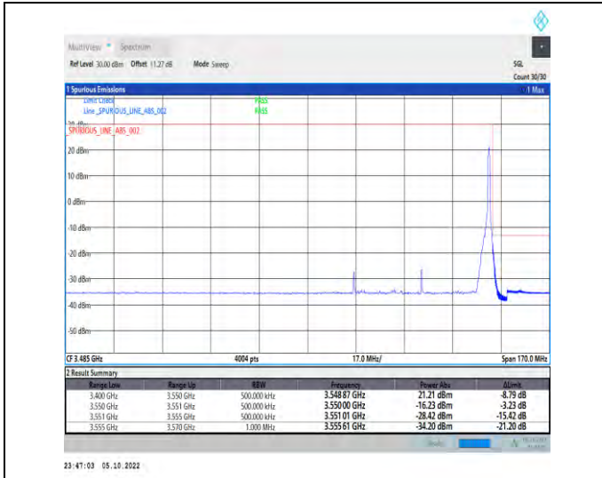
1-N77-3450-3550-PC2-30-50-H-2-DFT-QPSK-Edge_1 RB_Right-1@132-Ant1-1--PASS-see graph
