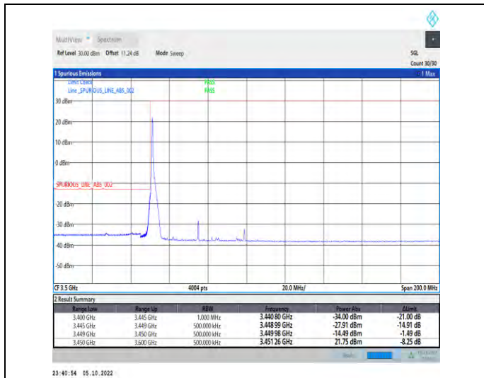
1-N77-3450-3550-PC2-30-50-L-1-DFT-QPSK-Edge_1 RB_Left-1@0-Ant1-1--PASS-see graph
