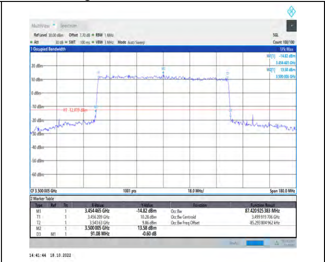
1-N77-3450-3550-PC2-30-90-M-7-CP-16QAM-Outer_Full-245@0-Ant1-87.421-91.080-≤90-PASS
