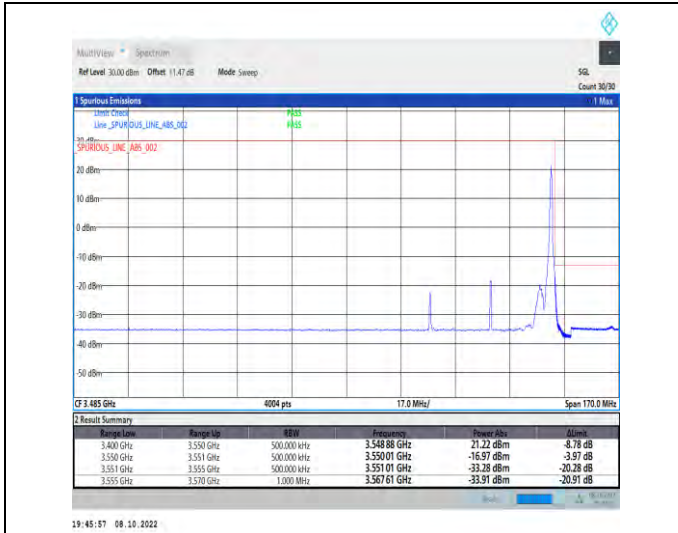
1-N77-3450-3550-PC2-30-40-H-2-DFT-QPSK-Edge_1 RB_Right-1@105-Ant1-1--PASS-see graph
