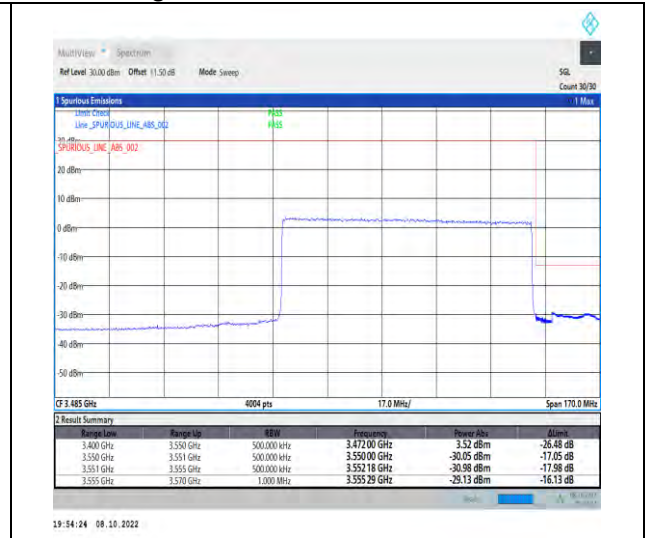
1-N77-3450-3550-PC2-30-80-H-3-DFT-QPSK-Out er_Full-216@0-Ant1-1--PASS-see graph
