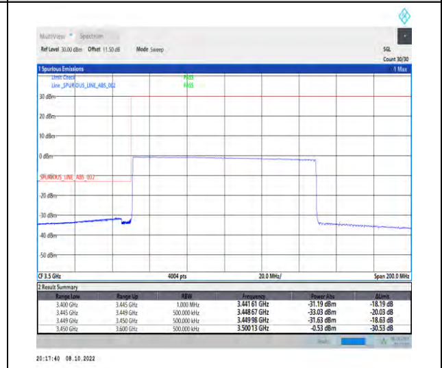
1-N77-3450-3550-PC2-30-100-L-6-CP-QPSK-Out er_Full-273@0-Ant1-1--PASS-see graph
