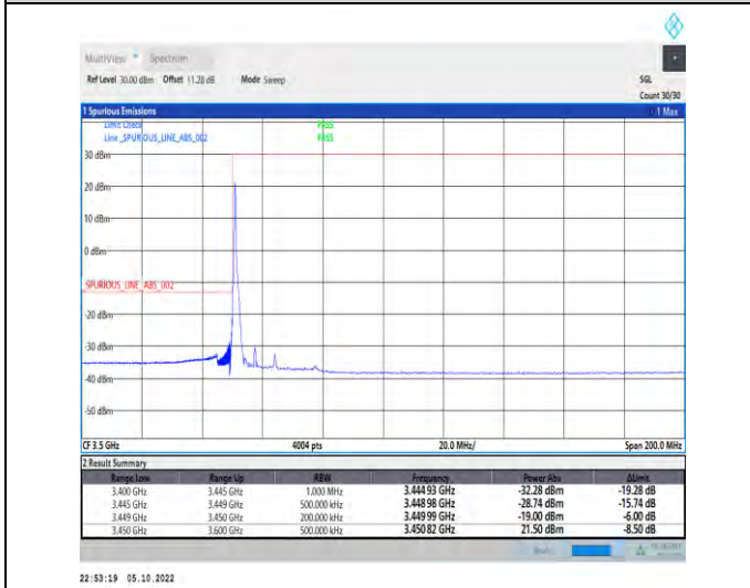
1-N77-3450-3550-PC2-30-15-L-4-CP-QPSK-Edge_1R B_Left-1@0-Ant1-1--PASS-see graph
