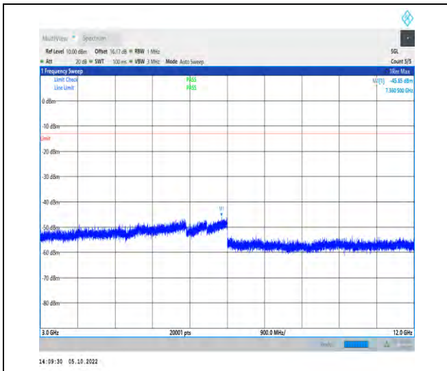
1-N71-PC3-15-20-L-1-DFT-QPSK-Inner_1RB_Left-1 @1-3000-12000-Ant1-7360.50--45.85--13-PASS
