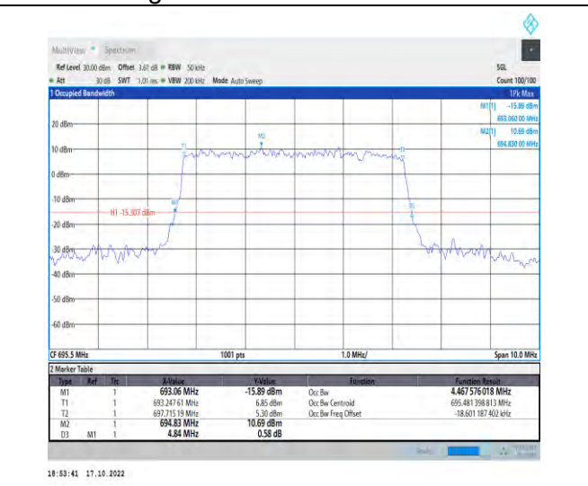
1-N71-PC3-15-5-H-7-CP-16QAM-Outer_Full-25@0- Ant1-4.468-4.840-≤5-PASS
