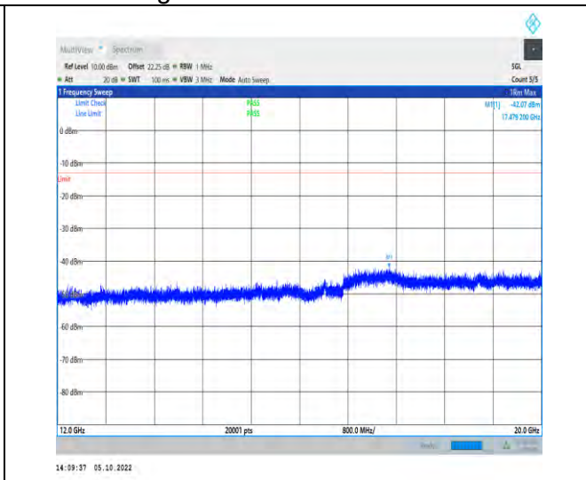
1-N71-PC3-15-20-L-1-DFT-QPSK-Inner_1RB_Left-1 @1-12000-20000-Ant1-17479.20--42.07--13-PASS
