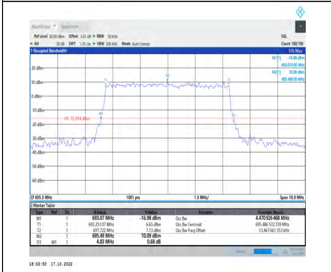
1-N71-PC3-15-5-H-8-CP-64QAM-Outer_Full-25@0- Ant1-4.471-4.830-≤5-PASS
