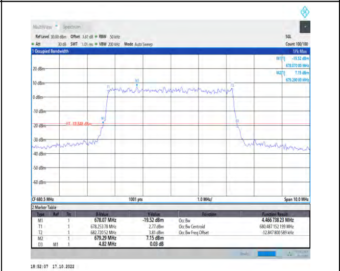
1-N71-PC3-15-5-M-9-CP-256QAM-Outer_Full-25@0-A nt1-4.467-4.820-<math>\leq</math>5-PASS
