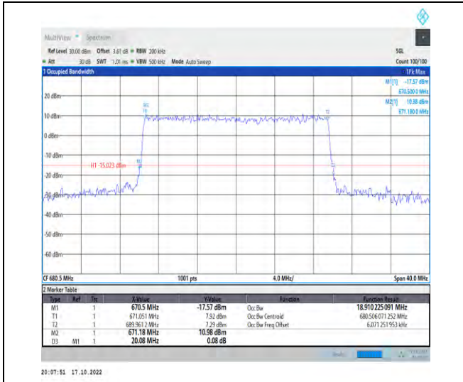
1-N71-PC3-15-20-M-6-CP-QPSK-Outer_Full-106@0 -Ant1-18.91-20.080-≤20-PASS
