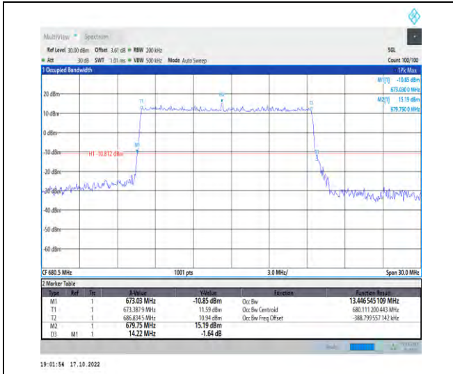
1-N71-PC3-15-15-M-1-DFT-QPSK-Outer_Full-75@0 -Ant1-13.447-14.220-≤15-PASS
