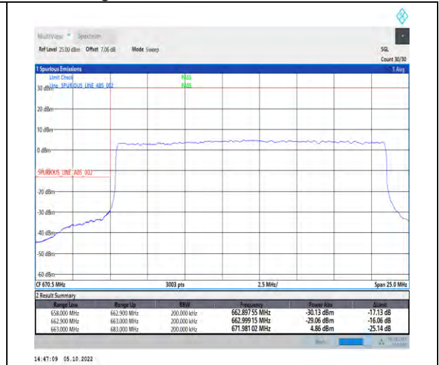
1-N71-PC3-15-20-L-3-DFT-QPSK-Outer_Full-100@0-Ant1-1--PASS-see graph
