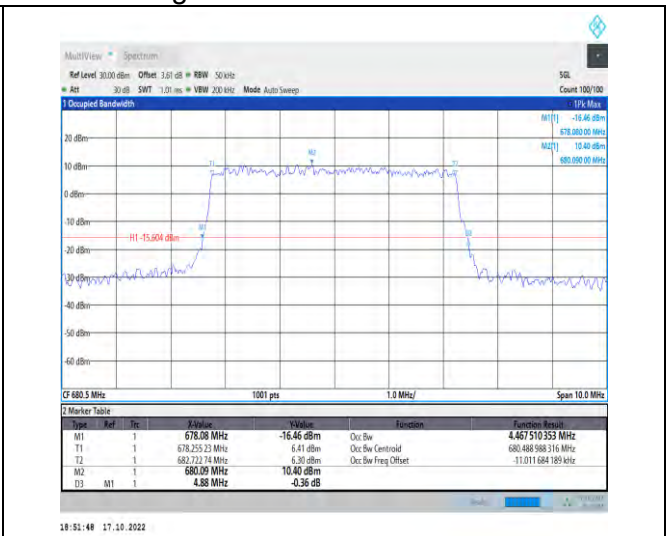
1-N71-PC3-15-5-M-7-CP-16QAM-Outer_Full-25@0-A nt1-4.468-4.880-<math>\leq</math>5-PASS
