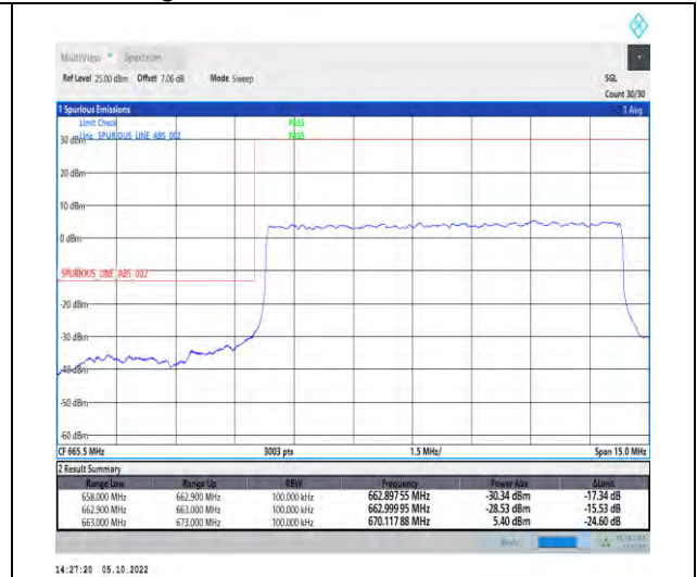
1-N71-PC3-15-10-L-3-DFT-QPSK-Outer_Full-50@0-Ant1-1--PASS-see graph
