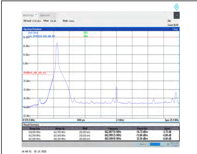
1-N71-PC3-15-20-L-1-DFT-QPSK-Edge_1RB_Left-1@0-Ant1-1--PASS-see graph
