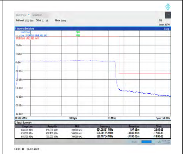
1-N71-PC3-15-10-H-6-CP-QPSK-Outer_Full-52@0-Ant1-1--PASS-see graph
