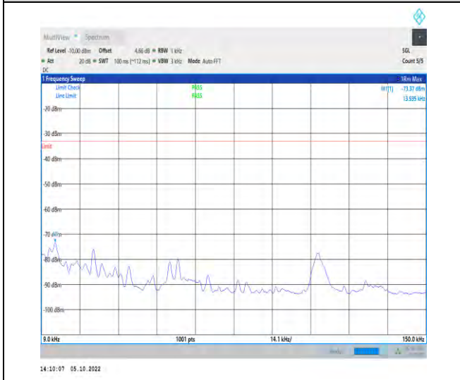
1-N71-PC3-15-20-M-1-DFT-QPSK-Inner_1RB_Left-1 @1-0.009-0.15-Ant1-0.01--73.37--33-PASS
