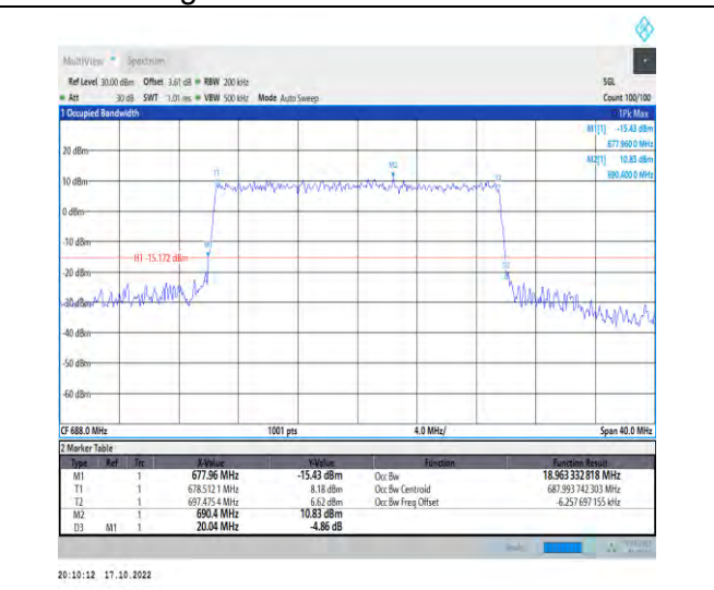
1-N71-PC3-15-20-H-7-CP-16QAM-Outer_Full-106@0 -Ant1-18.963-20.040-≤20-PASS
