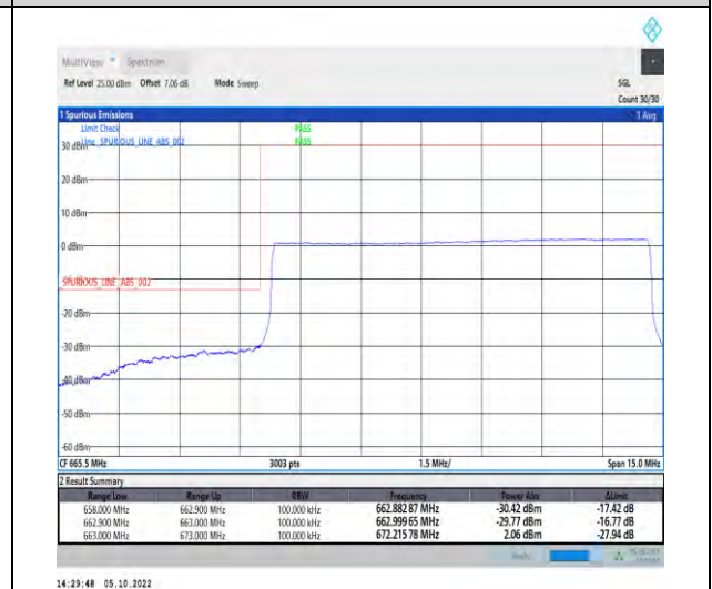
1-N71-PC3-15-10-L-6-CP-QPSK-Outer_Full-52@0-Ant1-1--PASS-see graph
