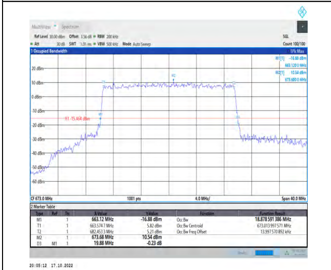
1-N71-PC3-15-20-L-8-CP-64QAM-Outer_Full-106@0 -Ant1-18.879-19.880-≤20-PASS
