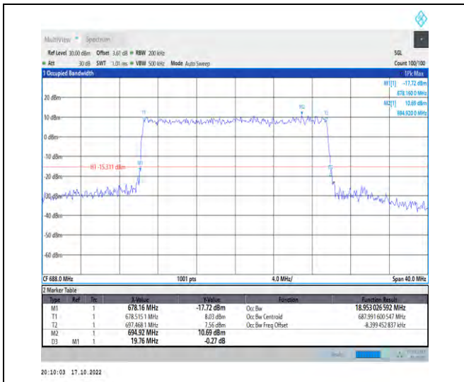
1-N71-PC3-15-20-H-6-CP-QPSK-Outer_Full-106@0 -Ant1-18.953-19.760-≤20-PASS
