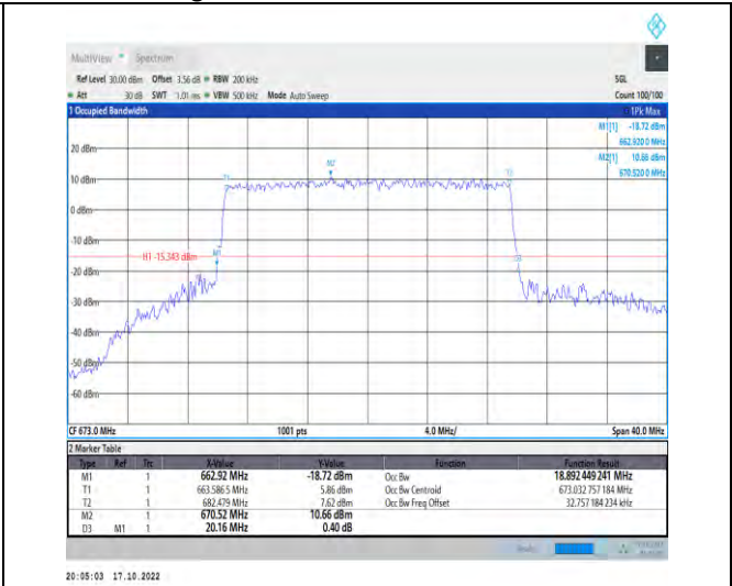
1-N71-PC3-15-20-L-7-CP-16QAM-Outer_Full-106@0 -Ant1-18.892-20.160-≤20-PASS
