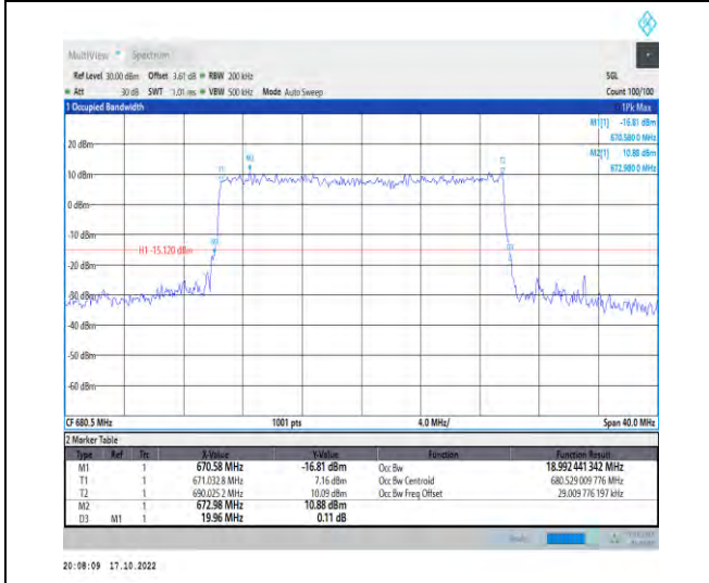
1-N71-PC3-15-20-M-8-CP-64QAM-Outer_Full-106 @0-Ant1-18.992-19.960-≤20-PASS
