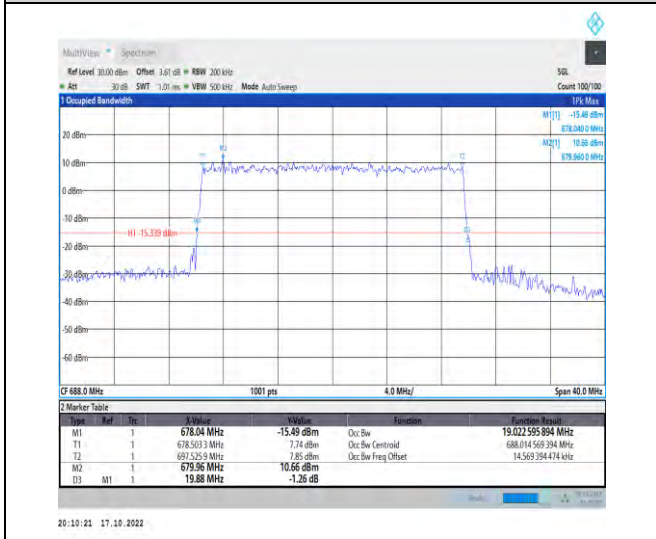
1-N71-PC3-15-20-H-8-CP-64QAM-Outer_Full-106@0 -Ant1-19.023-19.880-≤20-PASS
