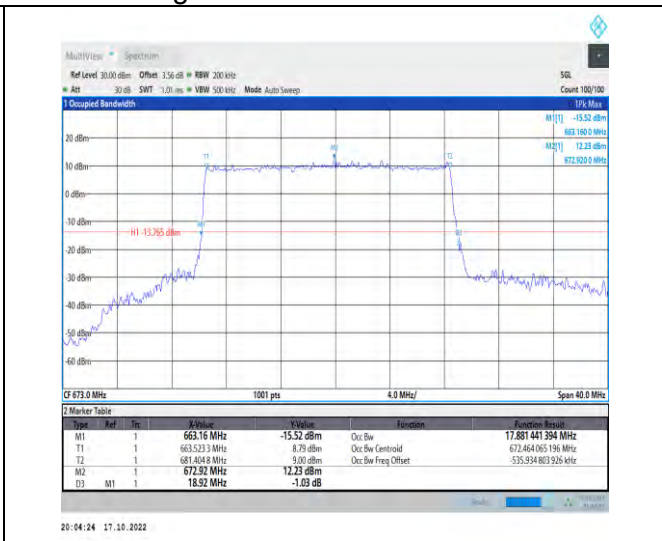
1-N71-PC3-15-20-L-3-DFT-16QAM-Outer_Full-100@ 0-Ant1-17.881-18.920-≤20-PASS
