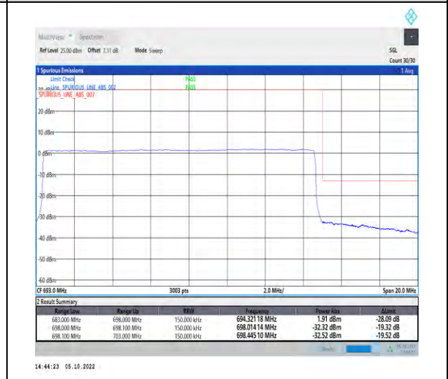
1-N71-PC3-15-15-H-6-CP-QPSK-Outer_Full-79@0-Ant1-1--PASS-see graph
