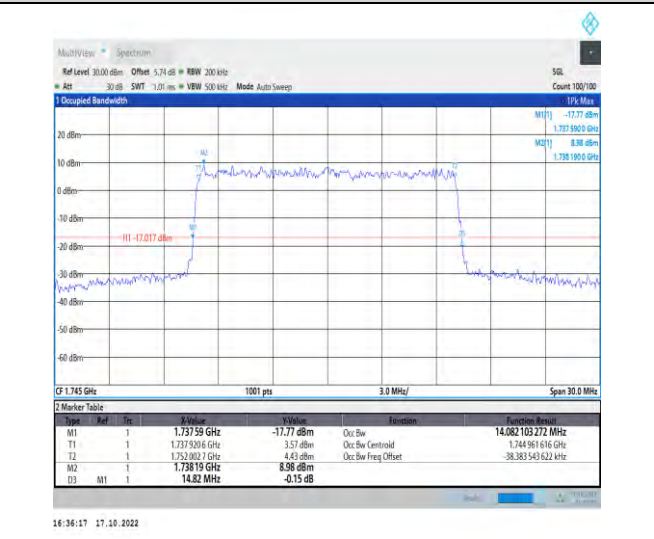
1-N66-PC3-15-15-M-9-CP-256QAM-Outer_Full-79@0-Ant1-14.082-14.820-≤15-PASS
