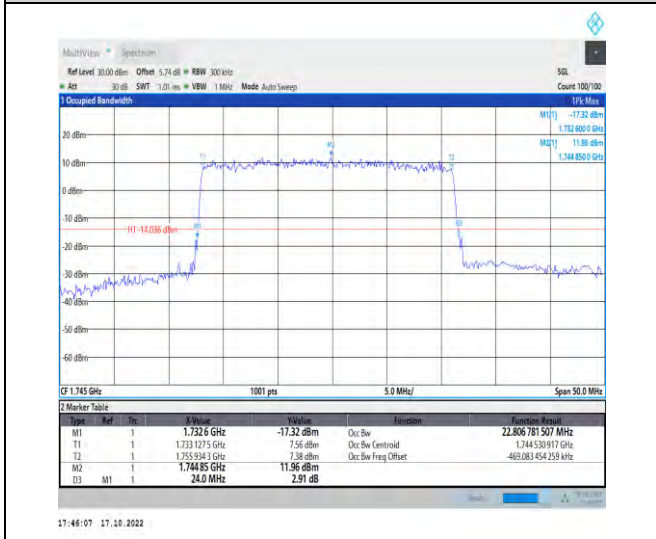
1-N66-PC3-15-25-M-4-DFT-64QAM-Outer_Full-128 @0-Ant1-22.807-24.000-≤25-PASS
