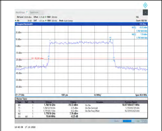
1-N66-PC3-15-20-H-9-CP-256QAM-Outer_Full-106@0 -Ant1-18.978-19.640-≤20-PASS
