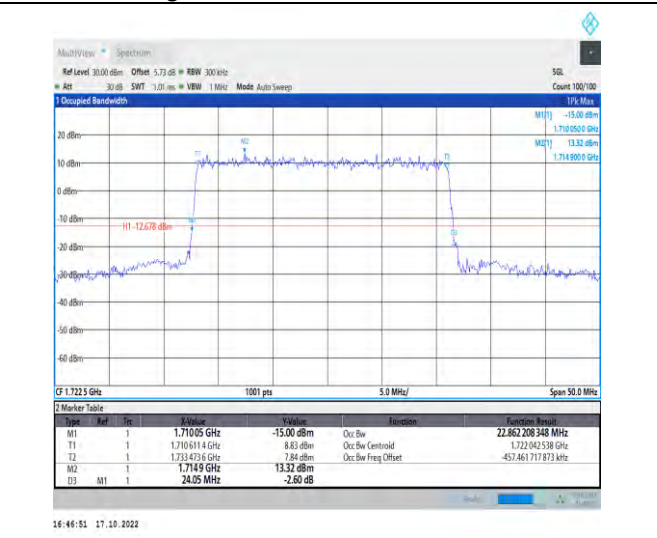
1-N66-PC3-15-25-L-3-DFT-16QAM-Outer_Full-128@ 0-Ant1-22.862-24.050-≤25-PASS
