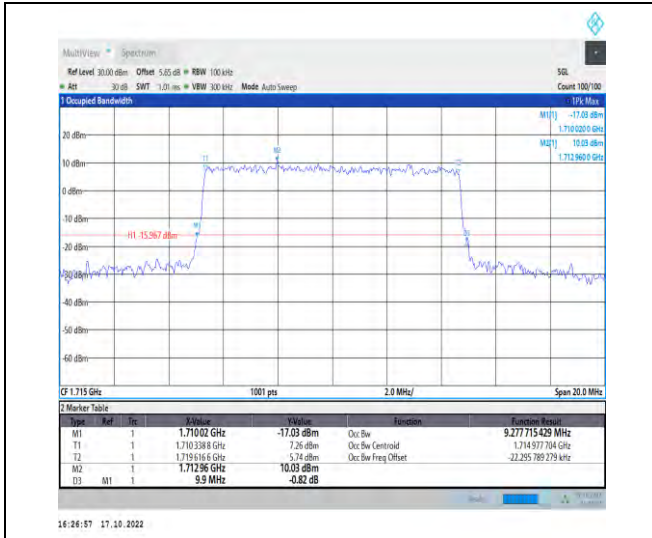
1-N66-PC3-15-10-L-6-CP-QPSK-Outer_Full-52@0-Ant1-9.278-9.900-≤10-PASS
