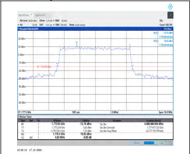
1-N66-PC3-15-5-H-7-CP-16QAM-Outer_Full-25@0- Ant1-4.486-4.830-≤5-PASS
