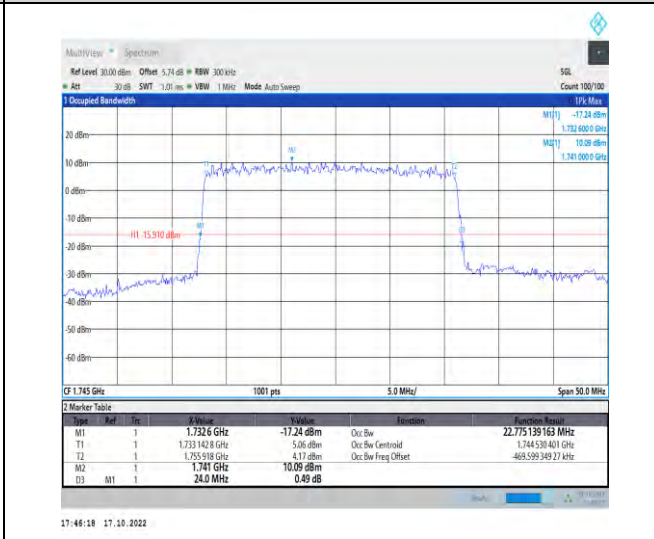
1-N66-PC3-15-25-M-5-DFT-256QAM-Outer_Full-128 @0-Ant1-22.775-24.000-≤25-PASS
