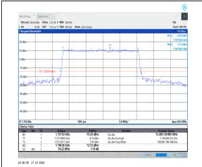
1-N66-PC3-15-15-M-1-DFT-QPSK-Outer_Full-75@0 -Ant1-13.383-14.220-≤15-PASS
