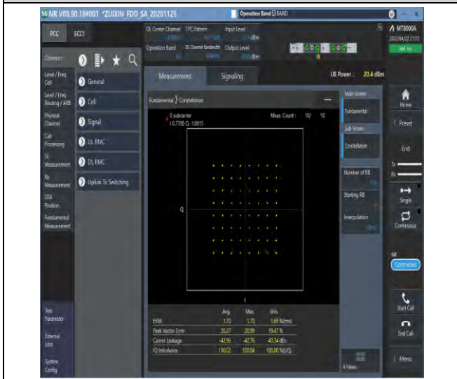
1-N66-PC3-15-40-M-4-DFT-64QAM-Outer_Full-216 @0-Ant1-see graph-PASS
