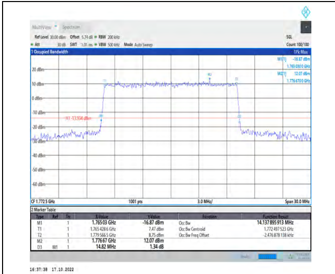
1-N66-PC3-15-15-H-6-CP-QPSK-Outer_Full-79@0-Ant1-14.138-14.820-≤15-PASS
