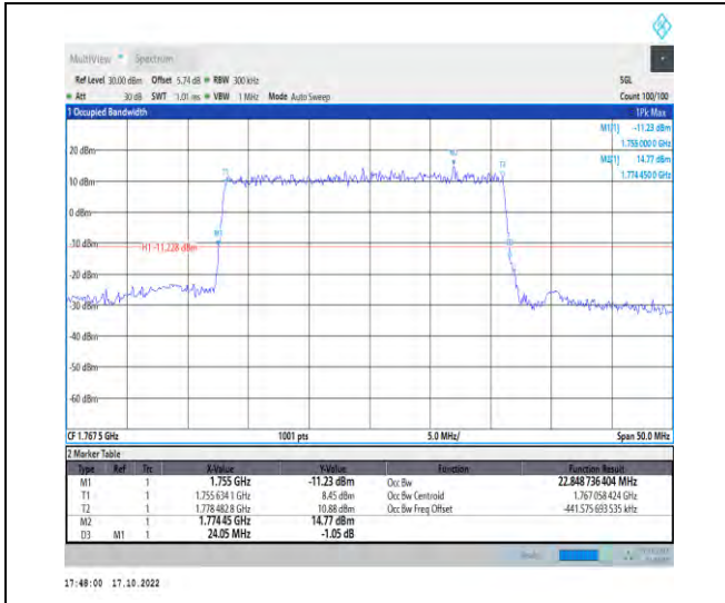
1-N66-PC3-15-25-H-1-DFT-QPSK-Outer_Full-128@ 0-Ant1-22.849-24.050-≤25-PASS
