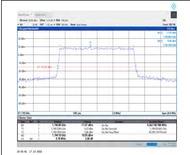
1-N66-PC3-15-10-M-8-CP-64QAM-Outer_Full-52@0-Ant1-9.262-9.780-≤10-PASS
