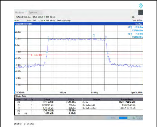
1-N66-PC3-15-15-M-5-DFT-256QAM-Outer_Full-75@0 -Ant1-13.433-14.220-≤15-PASS
