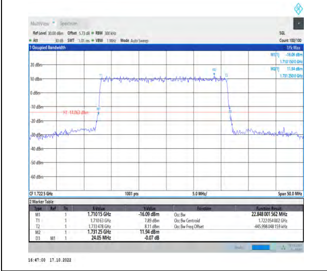
1-N66-PC3-15-25-L-4-DFT-64QAM-Outer_Full-128 @0-Ant1-22.848-24.050-≤25-PASS
