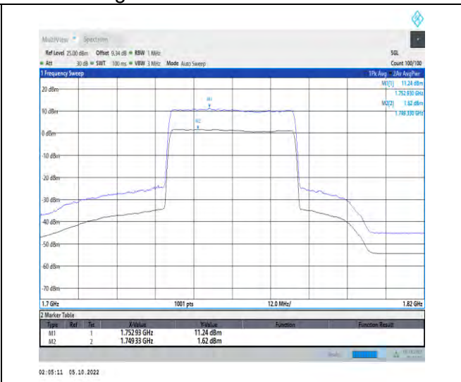
1-N66-PC3-15-40-H-2-CP-256QAM-Outer_Full-216 @0-Ant1-9.62-100%-0.00-9.62-PASS-≤13
