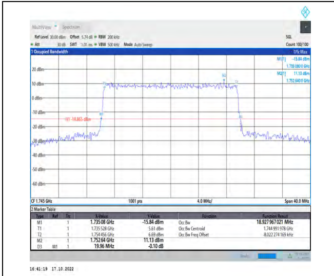
1-N66-PC3-15-20-M-6-CP-QPSK-Outer_Full-106@0 -Ant1-18.928-19.960-≤20-PASS
