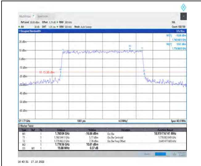
1-N66-PC3-15-20-H-6-CP-QPSK-Outer_Full-106@0 -Ant1-18.919-19.880-≤20-PASS
