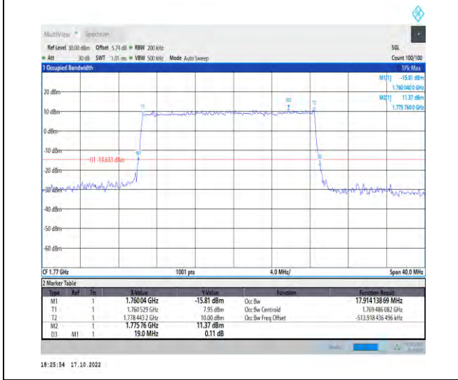
1-N66-PC3-15-20-H-4-DFT-64QAM-Outer_Full-100 @0-Ant1-17.914-19.000-≤20-PASS
