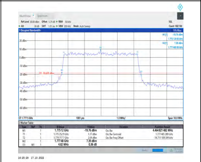
1-N66-PC3-15-5-H-9-CP-256QAM-Outer_Full-25@0- Ant1-4.465-4.820-≤5-PASS
