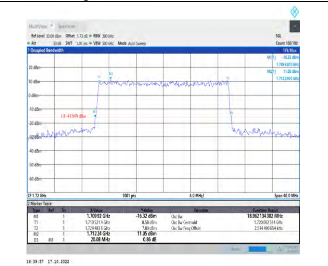
1-N66-PC3-15-20-L-7-CP-16QAM-Outer_Full-106@0 -Ant1-18.962-20.080-≤20-PASS
