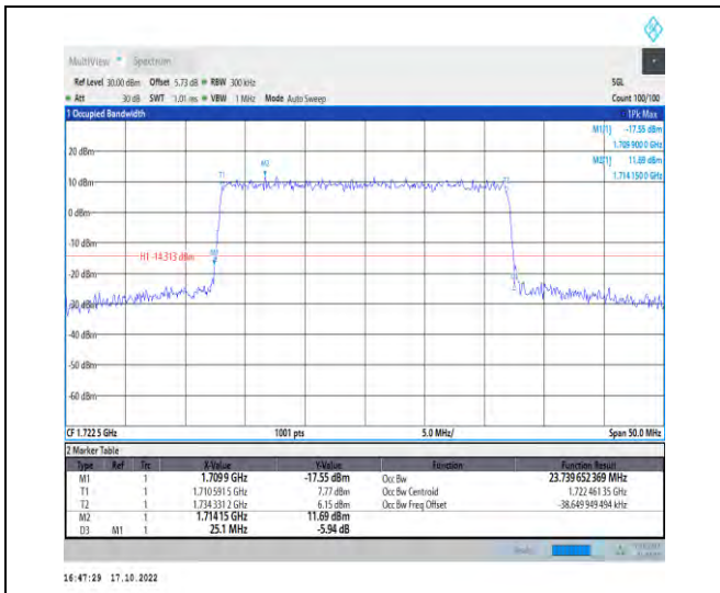
1-N66-PC3-15-25-L-6-CP-QPSK-Outer_Full-133@0 -Ant1-23.74-25.100-≤25-PASS
