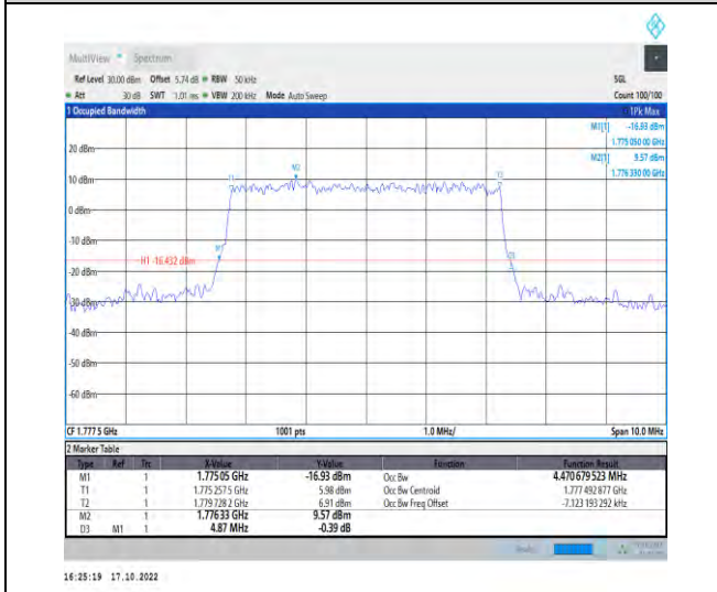
1-N66-PC3-15-5-H-8-CP-64QAM-Outer_Full-25@0- Ant1-4.471-4.870-≤5-PASS
