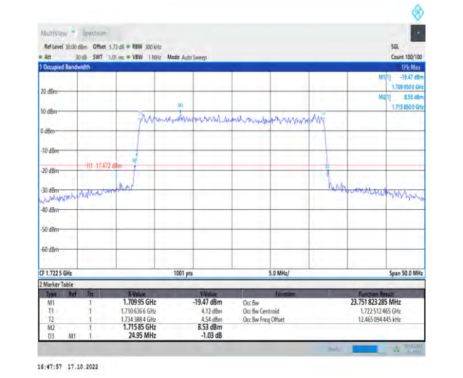
1-N66-PC3-15-25-L-9-CP-256QAM-Outer_Full-133@0 -Ant1-23.752-24.950-≤25-PASS
