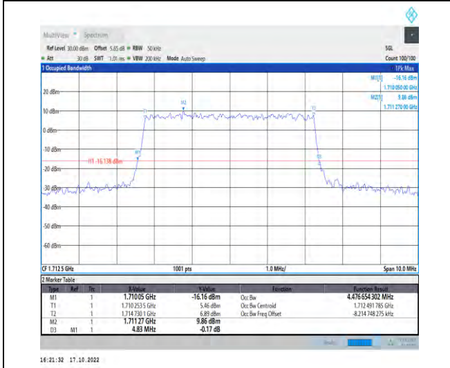
1-N66-PC3-15-5-L-8-CP-64QAM-Outer_Full-25@0-A Ant1-4.477-4.830-≤5-PASS
