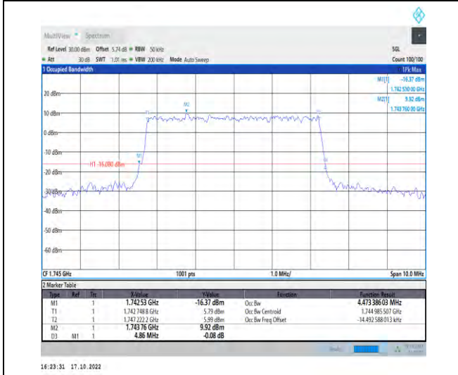
1-N66-PC3-15-5-M-8-CP-64QAM-Outer_Full-25@0-A Ant1-4.473-4.860-<math>\leq</math>5-PASS
