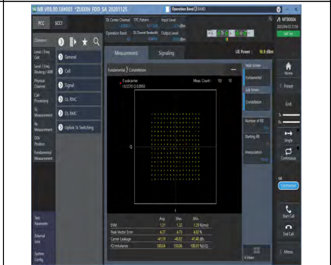
1-N66-PC3-15-40-M-9-CP-256QAM-Outer_Full-216@0-Ant1-see graph-PASS
