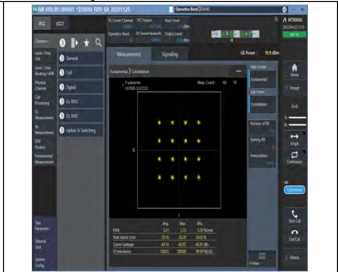
1-N66-PC3-15-40-M-7-CP-16QAM-Outer_Full-216@0-Ant1-see graph-PASS
