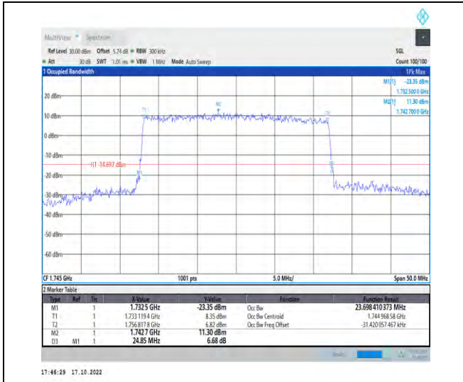
1-N66-PC3-15-25-M-6-CP-QPSK-Outer_Full-133@0 -Ant1-23.698-24.850-≤25-PASS
