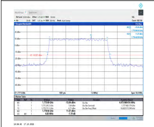
1-N66-PC3-15-5-H-4-DFT-64QAM-Outer_Full-25@0-Ant1-4.476-4.830-≤5-PASS
