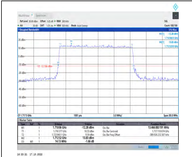
1-N66-PC3-15-15-L-1-DFT-QPSK-Outer_Full-75@0-Ant1-13.466-14.130-≤15-PASS
