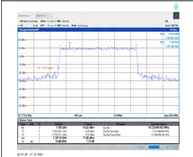
1-N66-PC3-15-15-H-8-CP-64QAM-Outer_Full-79@0-Ant1-14.125-14.880-≤15-PASS
