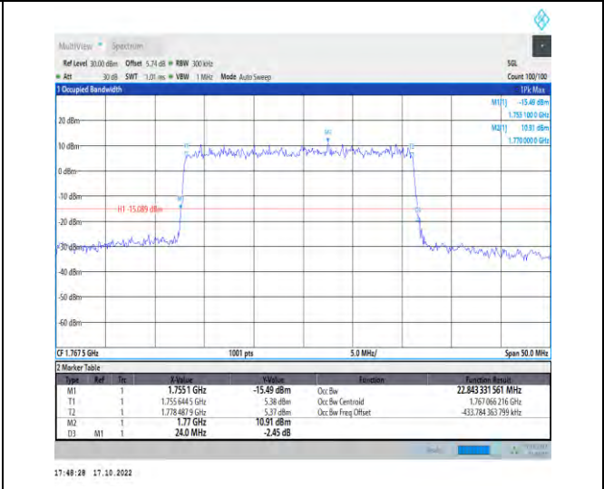
1-N66-PC3-15-25-H-5-DFT-256QAM-Outer_Full-128 @0-Ant1-22.843-24.000-≤25-PASS
