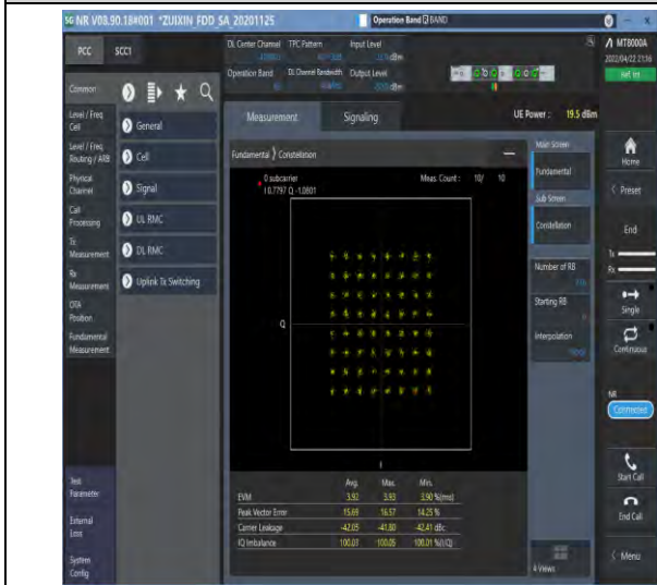
1-N66-PC3-15-40-M-8-CP-64QAM-Outer_Full-216@0-Ant1-see graph-PASS
