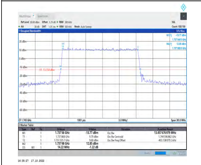
1-N66-PC3-15-15-M-4-DFT-64QAM-Outer_Full-75@0 -Ant1-13.458-14.220-≤15-PASS
