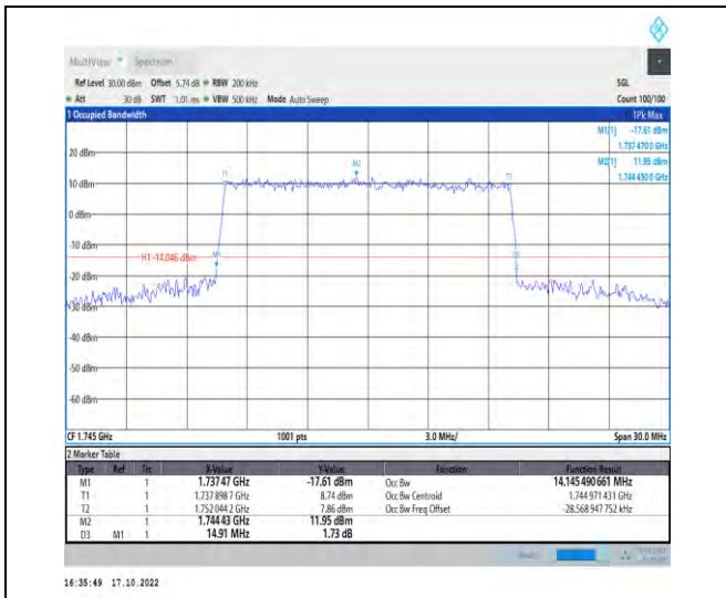
1-N66-PC3-15-15-M-6-CP-QPSK-Outer_Full-79@0-Ant1-14.145-14.910-≤15-PASS
