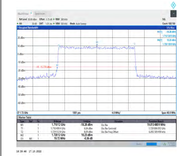
1-N66-PC3-15-20-L-8-CP-64QAM-Outer_Full-106@0 0-Ant1-19.013-19.720-≤20-PASS
