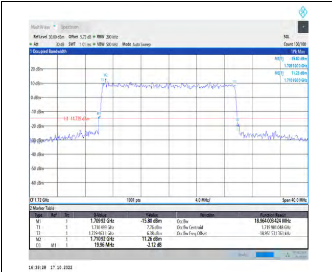
1-N66-PC3-15-20-L-6-CP-QPSK-Outer_Full-106@0 -Ant1-18.964-19.960-≤20-PASS
