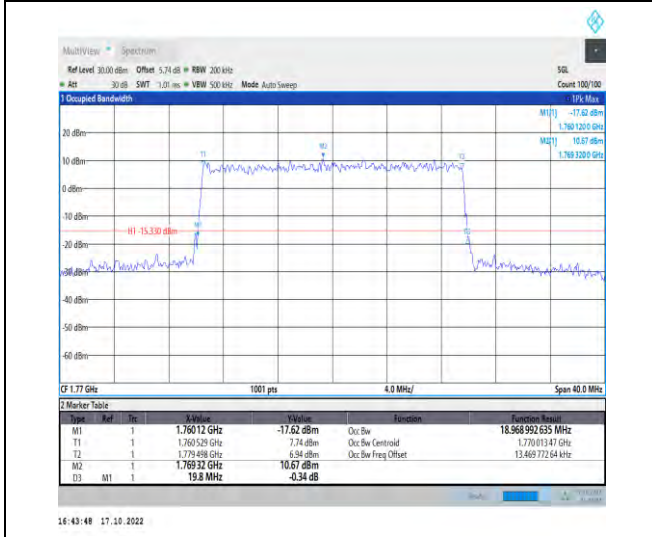
1-N66-PC3-15-20-H-8-CP-64QAM-Outer_Full-106@0 -Ant1-18.969-19.800-≤20-PASS
