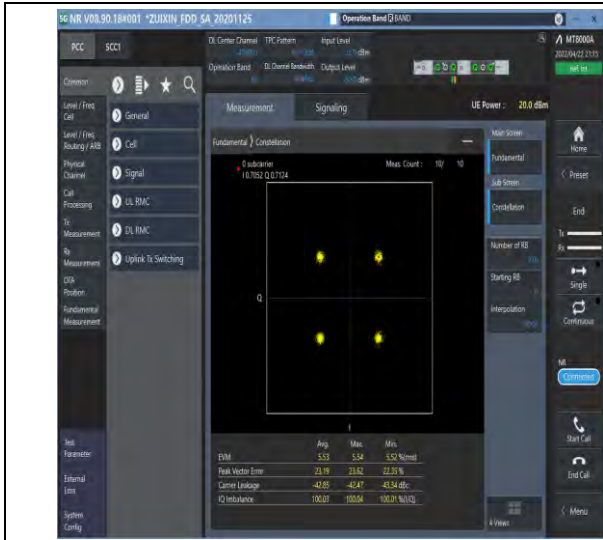
1-N66-PC3-15-40-M-6-CP-QPSK-Outer_Full-216@0-Ant1-see graph-PASS
