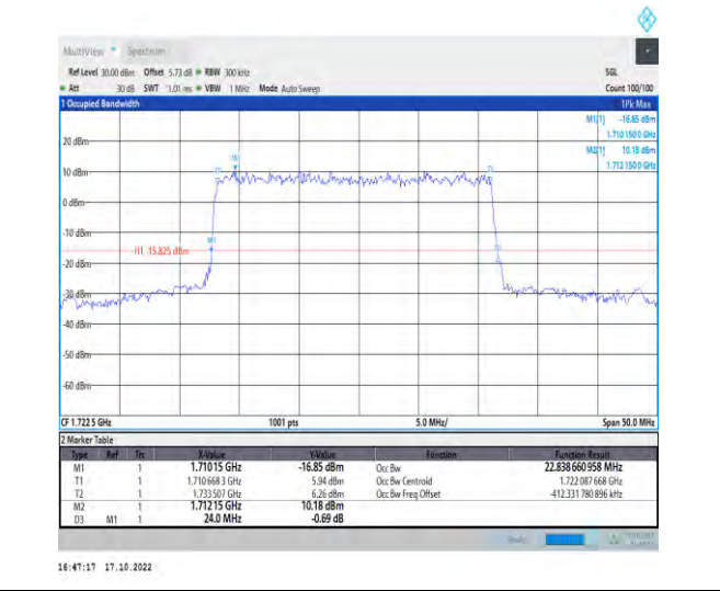
1-N66-PC3-15-25-L-5-DFT-256QAM-Outer_Full-128 @0-Ant1-22.839-24.000-≤25-PASS
