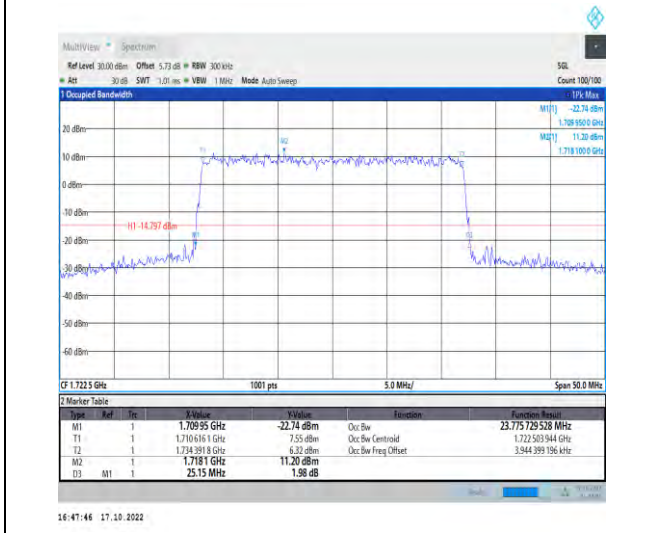
1-N66-PC3-15-25-L-8-CP-64QAM-Outer_Full-133@0 -Ant1-23.776-25.150-≤25-PASS
