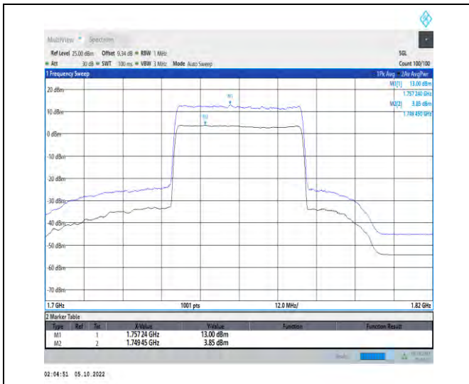
1-N66-PC3-15-40-H-1-DFT-256QAM-Outer_Full-216 @0-Ant1-9.15-100%-0.00-9.15-PASS-≤13
