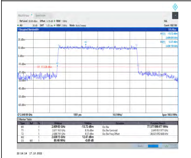
1-N41-PC2-30-80-H-8-CP-64QAM-Outer_Full-217@0 -Ant1-77.577-80.480-≤80-PASS
