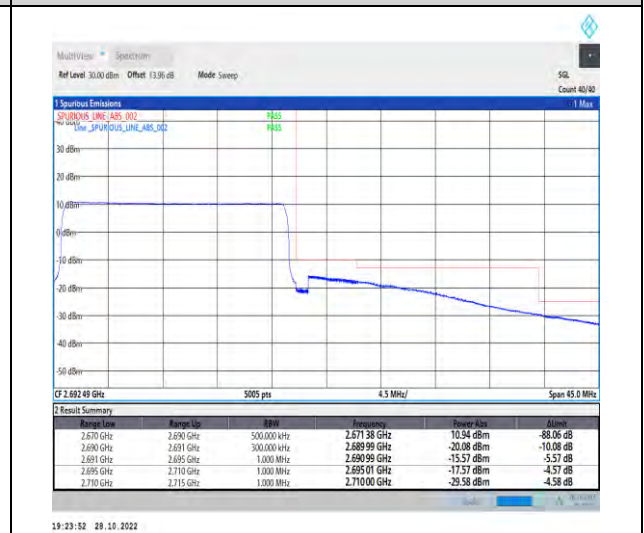
1-N41-PC2-30-20-H-6-CP-QPSK-Outer_Full-51 @0-Ant1-1--PASS-see graph
