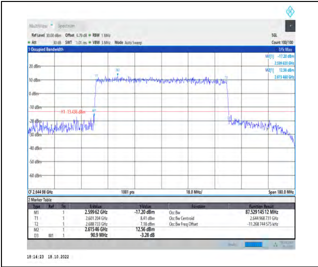
1-N41-PC2-30-90-H-6-CP-QPSK-Outer_Full-245@0 -Ant1-87.529-90.900-<math>\leq 90</math>-PASS
