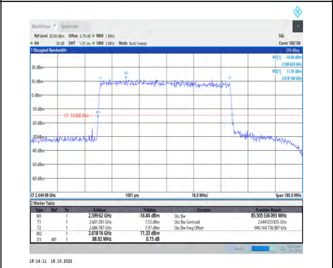
1-N41-PC2-30-90-H-5-DFT-256QAM-Outer_Full-240 @0-Ant1-85.506-88.920-≤90-PASS
