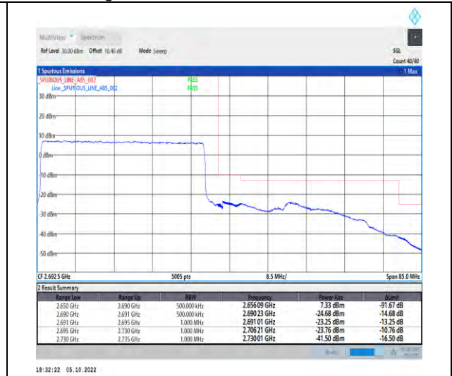
1-N41-PC2-30-40-H-3-DFT-QPSK-Outer_Full-100 @0-Ant1-1--PASS-see graph
