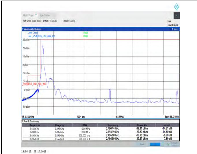
1-N41-PC2-30-60-L-1-DFT-QPSK-Edge_1RB_Left-1@ 0-Ant1-1--PASS-see graph
