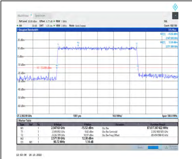
1-N41-PC2-30-90-M-6-CP-QPSK-Outer_Full-245@ 0-Ant1-87.617-90.720-≤90-PASS
