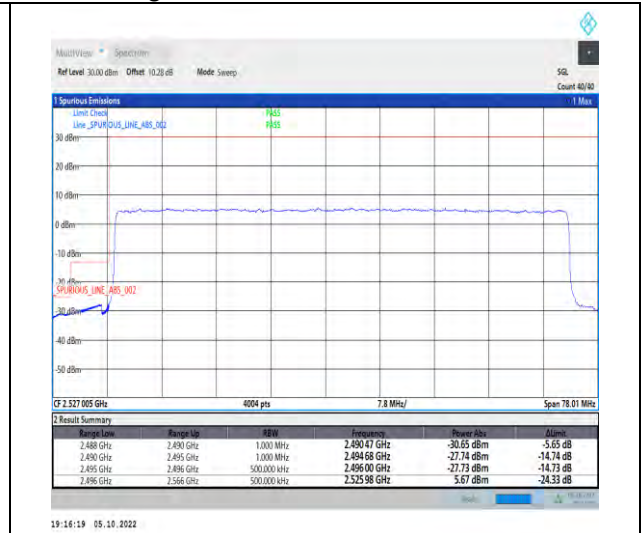
1-N41-PC2-30-70-L-3-DFT-QPSK-Outer_Full-180@0-Ant1-1--PASS-see graph
