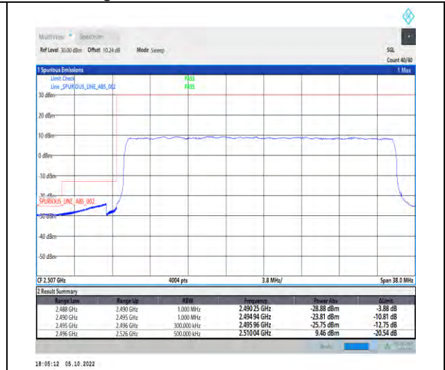
1-N41-PC2-30-30-L-3-DFT-QPSK-Outer_Full-75@ 0-Ant1-1--PASS-see graph
