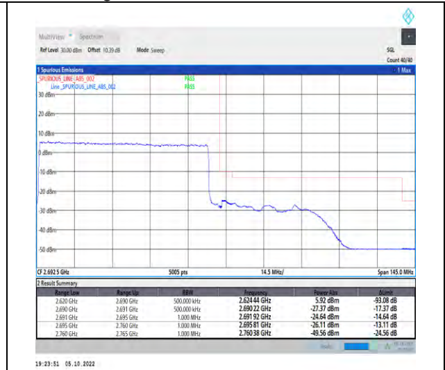
1-N41-PC2-30-70-H-3-DFT-QPSK-Outer_Full-180 @0-Ant1-1--PASS-see graph
