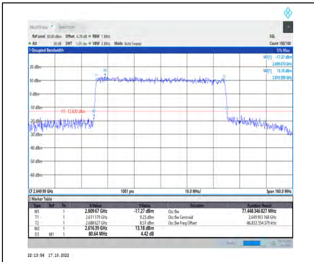
1-N41-PC2-30-80-H-6-CP-QPSK-Outer_Full-217@0 -Ant1-77.448-80.640-≤80-PASS
