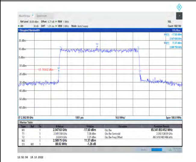
1-N41-PC2-30-90-M-5-DFT-256QAM-Outer_Full-240 @0-Ant1-85.542-88.920-≤90-PASS
