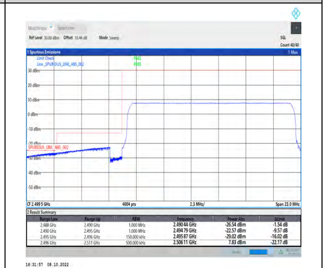
1-N41-PC2-30-15-L-6-CP-QPSK-Outer_Full-38@0-Ant1-1--PASS-see graph
