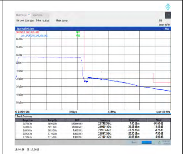
1-N41-PC2-30-20-H-6-CP-QPSK-Outer_Full-51@ 0-Ant1-1--PASS-see graph
