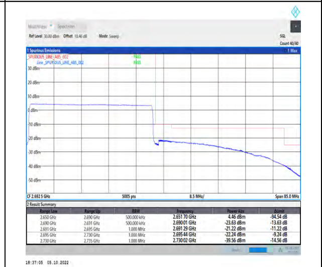
1-N41-PC2-30-40-H-6-CP-QPSK-Outer_Full-106 @0-Ant1-1--PASS-see graph
