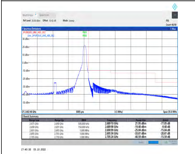
1-N41-PC2-30-15-H-5-CP-QPSK-Edge_1RB_Right-1 @37-Ant1-1--PASS-see graph
