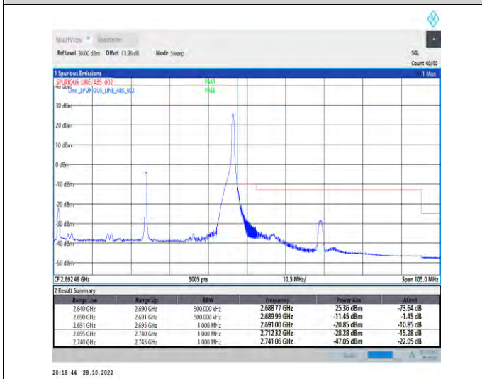
1-N41-PC2-30-50-H-5-CP-QPSK-Edge_1RB_Right-1 @132-Ant1-1--PASS-see graph
