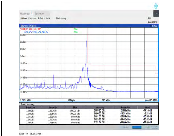
1-N41-PC2-30-100-H-2-DFT-QPSK-Edge_1RB_Right-1@272-Ant1-1--PASS-see graph
