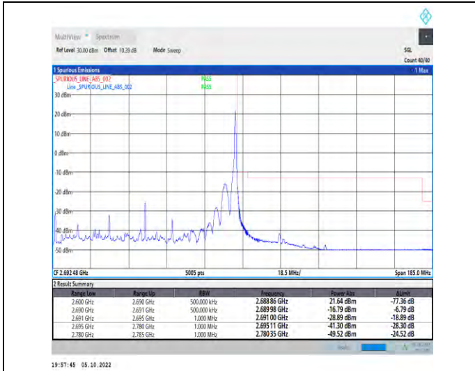
1-N41-PC2-30-90-H-2-DFT-QPSK-Edge_1RB_Right-1 @244-Ant1-1--PASS-see graph
