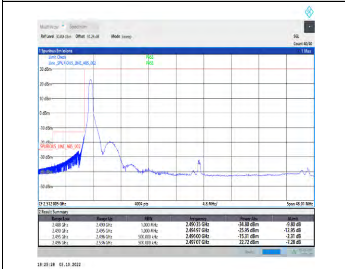
1-N41-PC2-30-40-L-4-CP-QPSK-Edge_1RB_Left-1@0-Ant1-1--PASS-see graph
