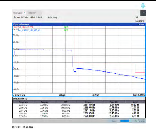
1-N41-PC2-30-30-H-6-CP-QPSK-Outer_Full-78@ 0-Ant1-1--PASS-see graph
