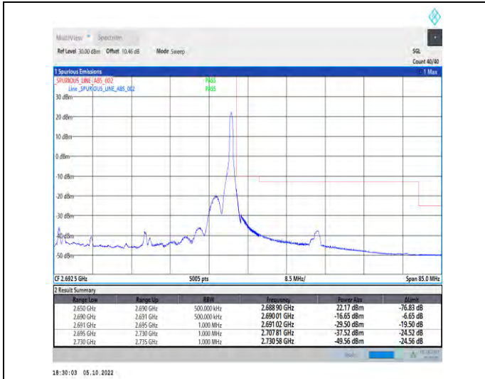
1-N41-PC2-30-40-H-2-DFT-QPSK-Edge_1RB_Right-1 @105-Ant1-1--PASS-see graph
