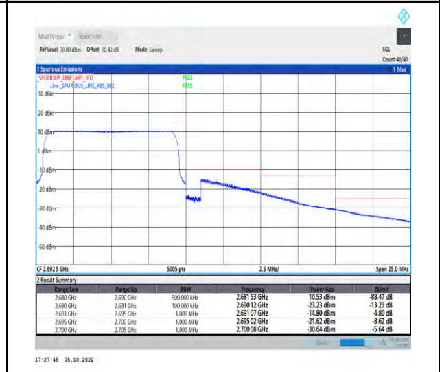
1-N41-PC2-30-10-H-6-CP-QPSK-Outer_Full-24@ 0-Ant1-1--PASS-see graph
