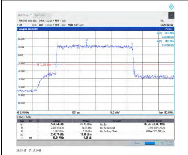
1-N41-PC2-30-90-L-4-DFT-64QAM-Outer_Full-240 @0-Ant1-85.598-89.640-≤90-PASS
