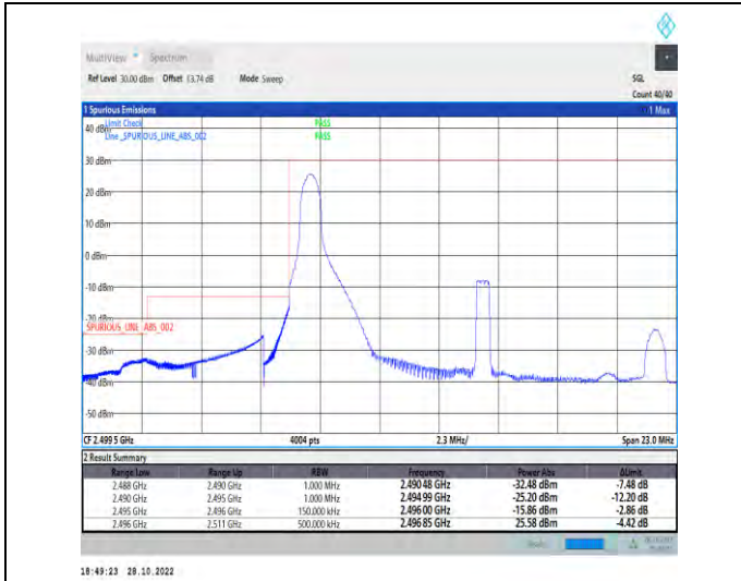
1-N41-PC2-30-15-L-1-DFT-PI2BPSK-Edge_1RB_Left-1@0-Ant1-1--PASS-see graph
