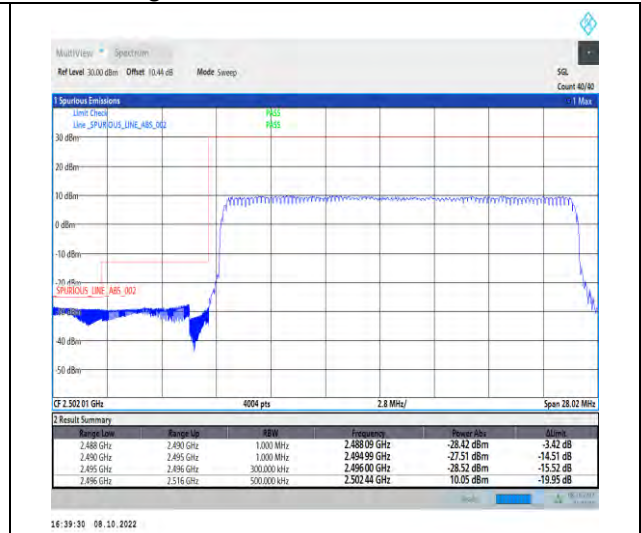
1-N41-PC2-30-20-L-3-DFT-QPSK-Outer_Full-50@ 0-Ant1-1--PASS-see graph
