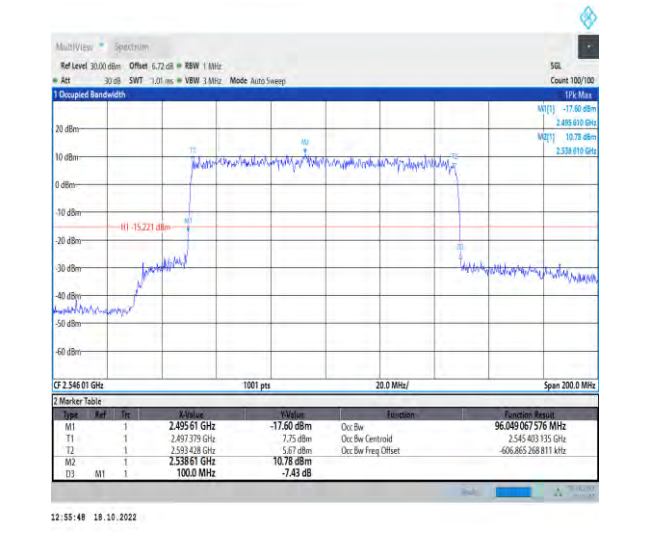
1-N41-PC2-30-100-L-5-DFT-256QAM-Outer_Full-270 @0-Ant1-96.049-100.000-≤100-PASS
