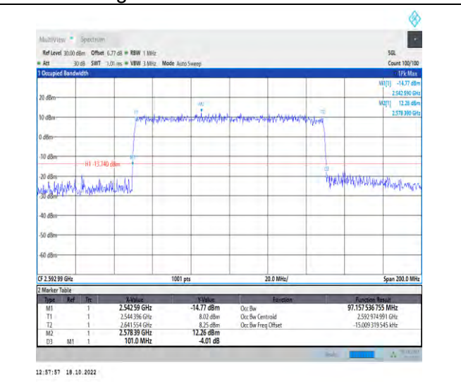
1-N41-PC2-30-100-M-7-CP-16QAM-Outer_Full-273 @0-Ant1-97.158-101.000-≤100-PASS
