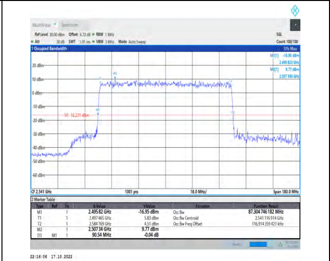
1-N41-PC2-30-90-L-9-CP-256QAM-Outer_Full-245@0 -Ant1-87.305-90.540-≤90-PASS
