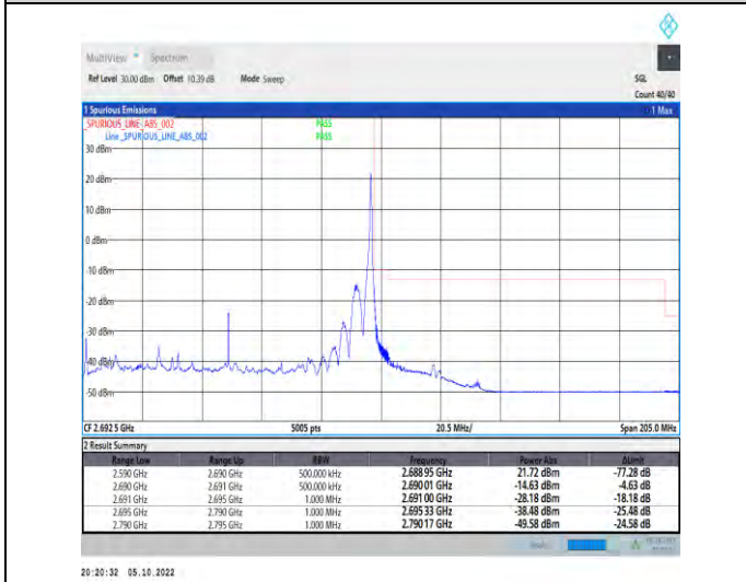
1-N41-PC2-30-100-H-5-CP-QPSK-Edge_1RB_Right-1@272-Ant1-1--PASS-see graph
