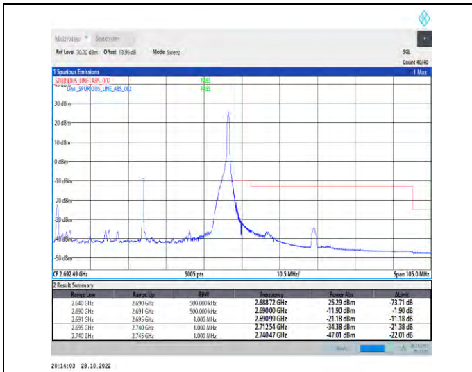
1-N41-PC2-30-50-H-2-DFT-PI2BPSK-Edge_1RB_Righ t-1@132-Ant1-1--PASS-see graph
