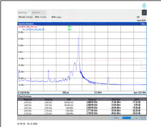
1-N41-PC2-30-60-H-2-DFT-QPSK-Edge_1RB_Right-1 @161-Ant1-1--PASS-see graph
