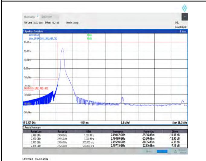
1-N41-PC2-30-30-L-4-CP-QPSK-Edge_1RB_Left-1@0 -Ant1-1--PASS-see graph
