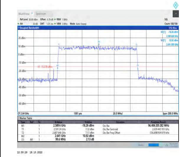
1-N41-PC2-30-100-H-5-DFT-256QAM-Outer_Full-270 @0-Ant1-96.406-99.600-≤100-PASS
