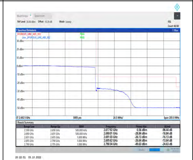
1-N41-PC2-30-100-H-6-CP-QPSK-Outer_Full-273@0-Ant1-1--PASS-see graph
