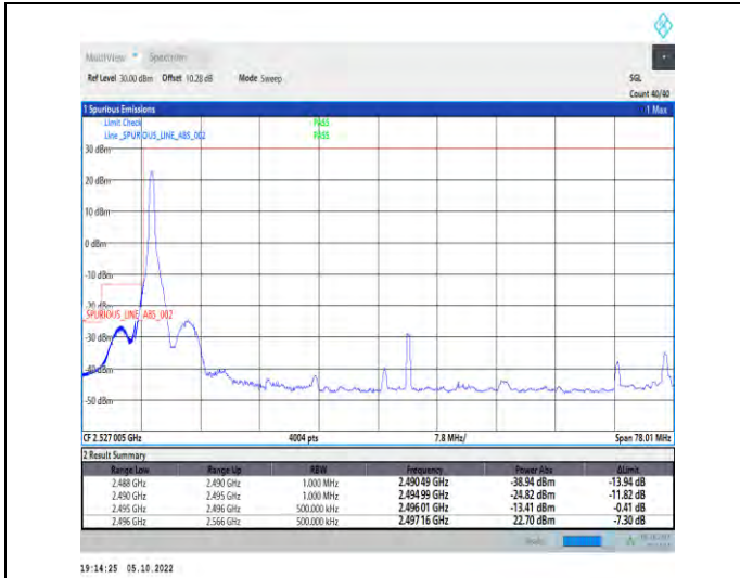
1-N41-PC2-30-70-L-1-DFT-QPSK-Edge_1RB_Left-1@0-Ant1-1--PASS-see graph
