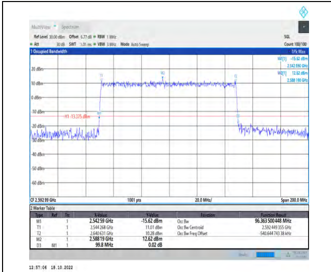
1-N41-PC2-30-100-M-1-DFT-QPSK-Outer_Full-270 @0-Ant1-96.364-99.800-≤100-PASS
