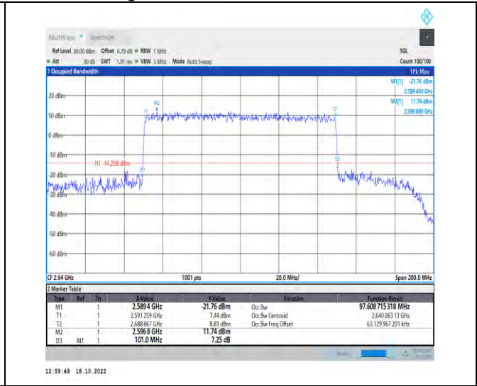
1-N41-PC2-30-100-H-7-CP-16QAM-Outer_Full-273 @0-Ant1-97.609-101.000-≤100-PASS
