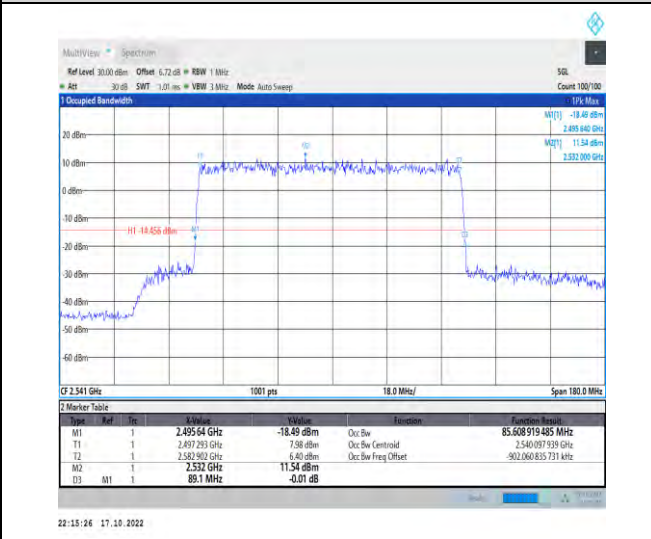
1-N41-PC2-30-90-L-5-DFT-256QAM-Outer_Full-240 @0-Ant1-85.609-89.100-≤90-PASS
