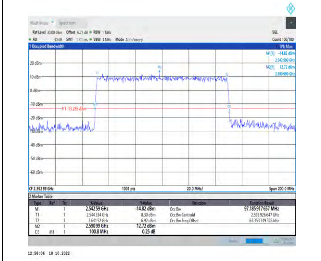
1-N41-PC2-30-100-M-8-CP-64QAM-Outer_Full-273 @0-Ant1-97.186-100.800-≤100-PASS
