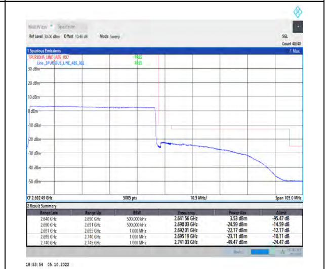
1-N41-PC2-30-50-H-6-CP-QPSK-Outer_Full-133 @0-Ant1-1--PASS-see graph
