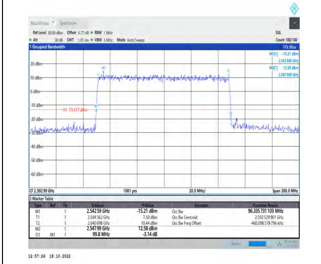
1-N41-PC2-30-100-M-4-DFT-64QAM-Outer_Full-270 @0-Ant1-96.336-99.800-≤100-PASS
