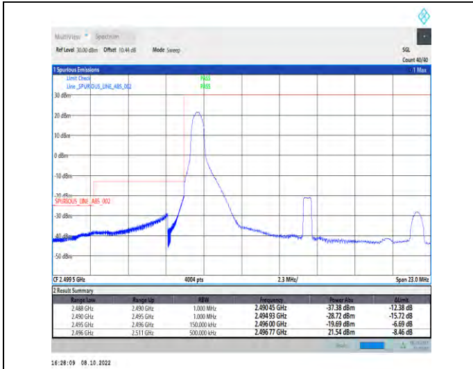
1-N41-PC2-30-15-L-1-DFT-QPSK-Edge_1RB_Left-1@0-Ant1-1--PASS-see graph
