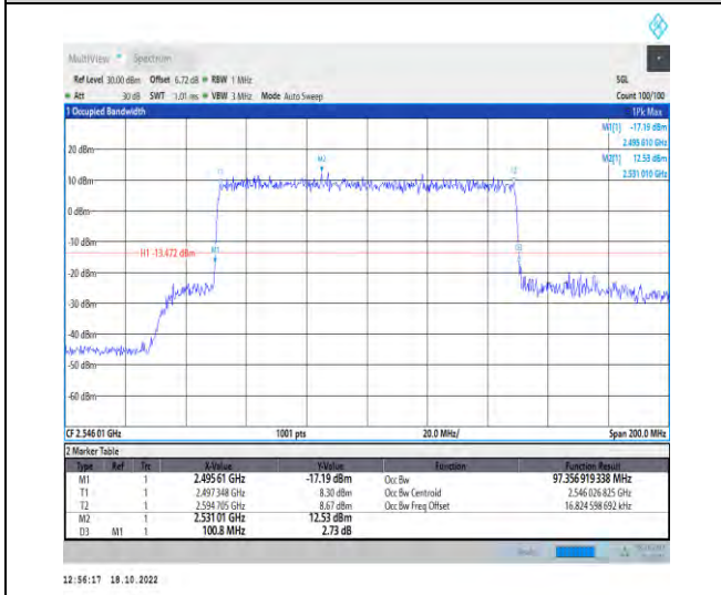
1-N41-PC2-30-100-L-8-CP-64QAM-Outer_Full-273 @0-Ant1-97.357-100.800-≤100-PASS
