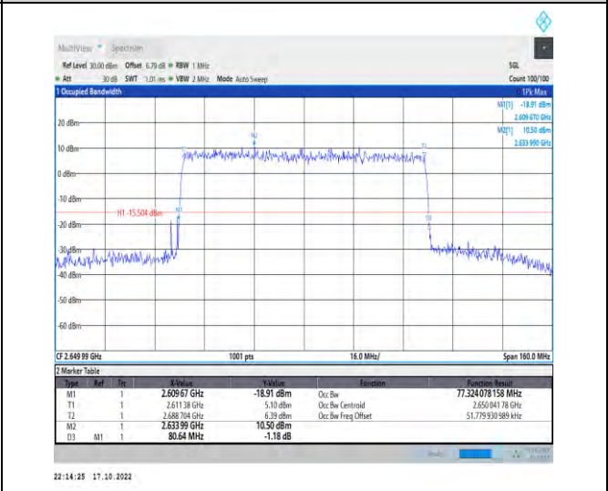
1-N41-PC2-30-80-H-9-CP-256QAM-Outer_Full-217@0 -Ant1-77.324-80.640-≤80-PASS
