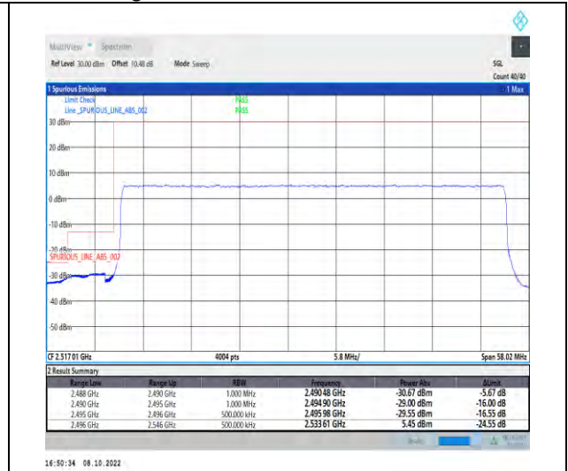
1-N41-PC2-30-50-L-3-DFT-QPSK-Outer_Full-128@0-Ant1-1--PASS-see graph
