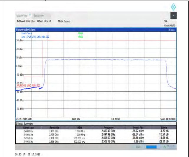
1-N41-PC2-30-40-L-3-DFT-QPSK-Outer_Full-100@0-Ant1-1--PASS-see graph
