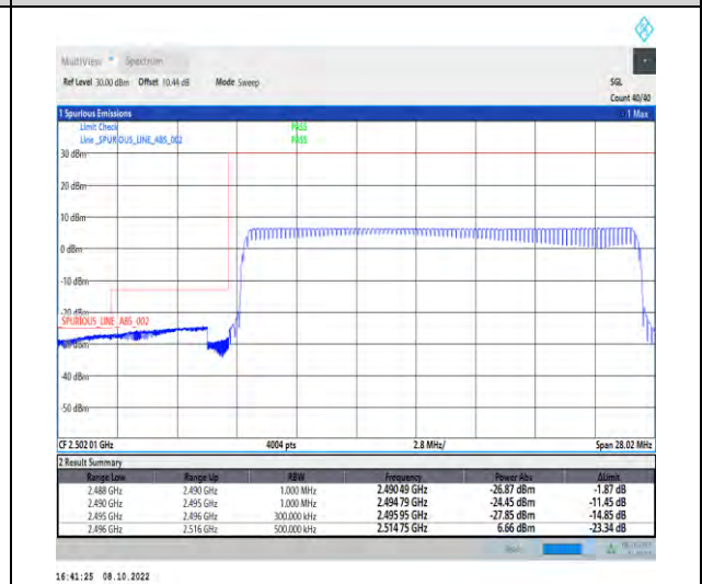
1-N41-PC2-30-20-L-6-CP-QPSK-Outer_Full-51@ 0-Ant1-1--PASS-see graph
