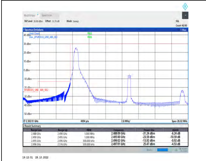
1-N41-PC2-30-20-L-4-CP-QPSK-Edge_1RB_Left-1@0-Ant1-1--PASS-see graph
