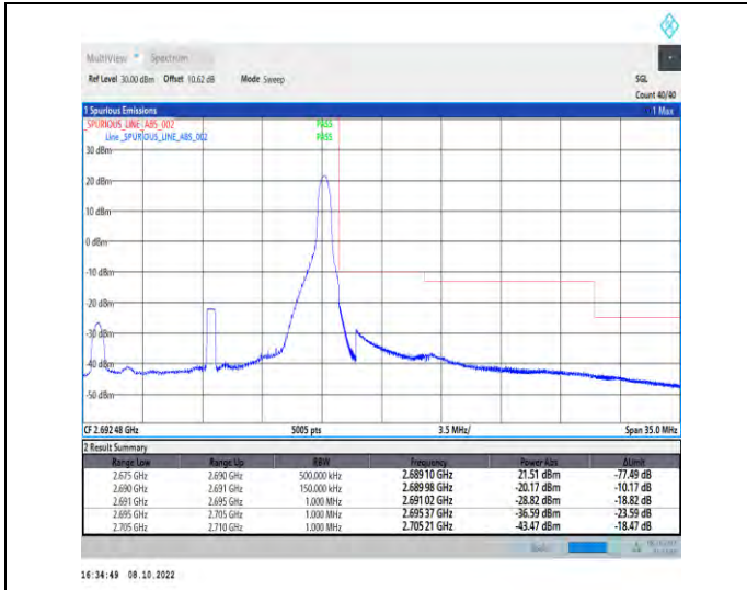
1-N41-PC2-30-15-H-2-DFT-QPSK-Edge_1RB_Right-1 @37-Ant1-1--PASS-see graph
