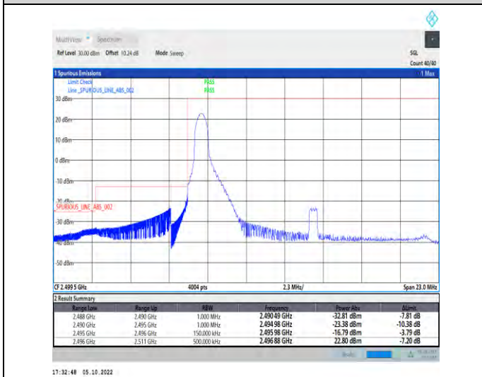
1-N41-PC2-30-15-L-4-CP-QPSK-Edge_1RB_Left-1@0-Ant1-1--PASS-see graph
