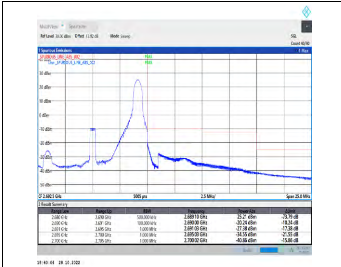
1-N41-PC2-30-10-H-2-DFT-PI2BPSK-Edge_1RB_Right-t-1@23-Ant1-1--PASS-see graph
