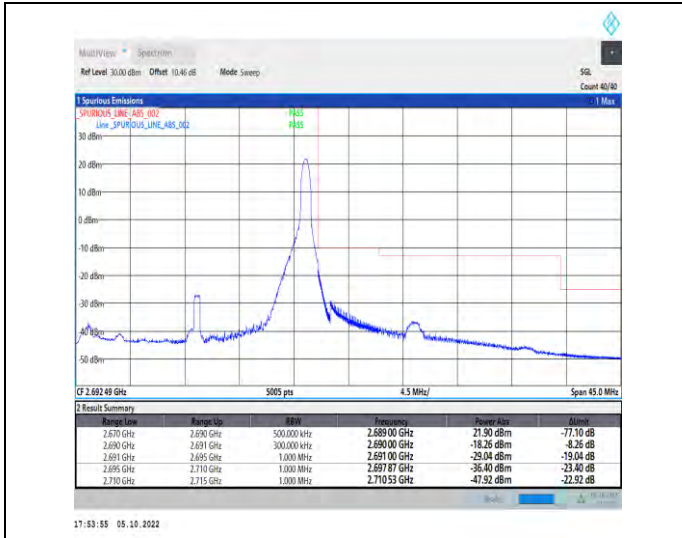
1-N41-PC2-30-20-H-2-DFT-QPSK-Edge_1RB_Right-1 @50-Ant1-1--PASS-see graph
