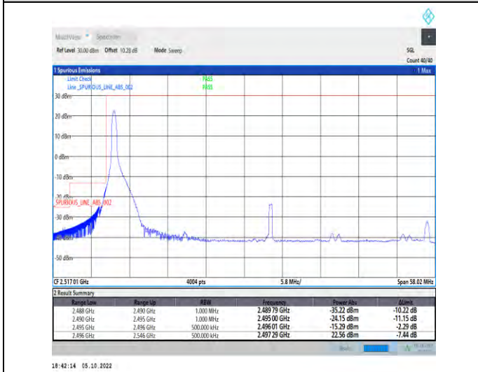
1-N41-PC2-30-50-L-4-CP-QPSK-Edge_1RB_Left-1@0-Ant1-1--PASS-see graph
