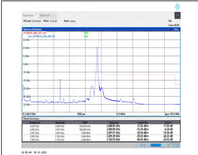
1-N41-PC2-30-70-H-2-DFT-QPSK-Edge_1RB_Right-1 @188-Ant1-1--PASS-see graph
