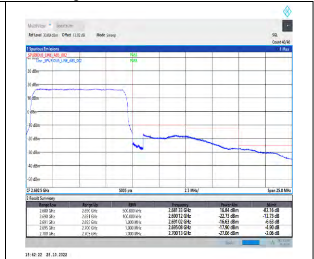
1-N41-PC2-30-10-H-3-DFT-PI2BPSK-Outer_Full-24@0-Ant1-1--PASS-see graph
