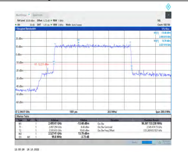
1-N41-PC2-30-100-L-3-DFT-16QAM-Outer_Full-270 @0-Ant1-96.361-99.800-≤100-PASS
