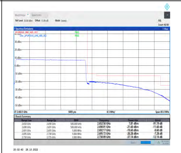
1-N41-PC2-30-40-H-6-CP-QPSK-Outer_Full-106 @0-Ant1-1--PASS-see graph
