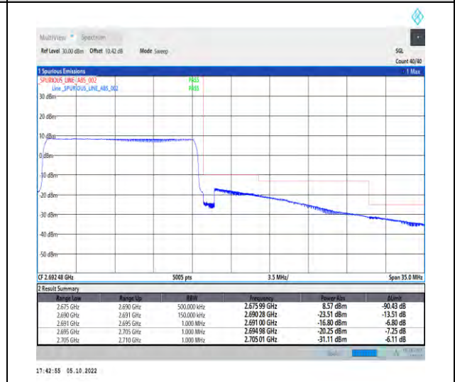
1-N41-PC2-30-15-H-6-CP-QPSK-Outer_Full-38@ 0-Ant1-1--PASS-see graph
