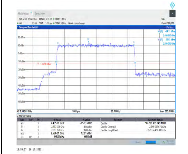
1-N41-PC2-30-100-L-4-DFT-64QAM-Outer_Full-270 @0-Ant1-96.206-99.800-≤100-PASS
