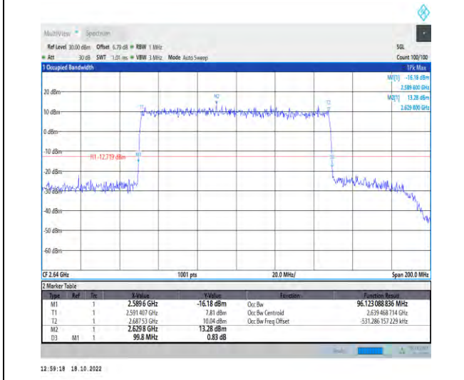
1-N41-PC2-30-100-H-4-DFT-64QAM-Outer_Full-270 @0-Ant1-96.123-99.800-≤100-PASS
