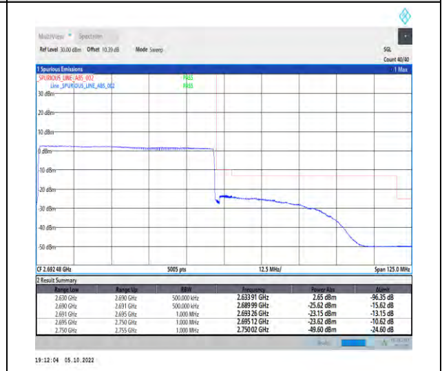
1-N41-PC2-30-60-H-6-CP-QPSK-Outer_Full-162 @0-Ant1-1--PASS-see graph
