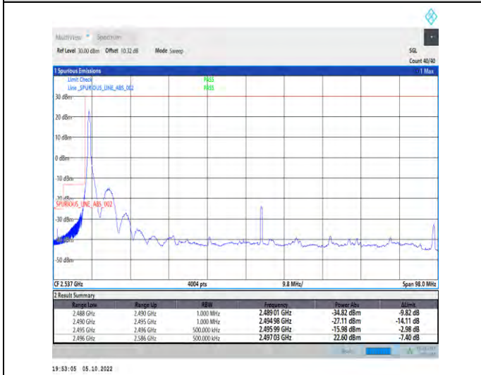
1-N41-PC2-30-90-L-4-CP-QPSK-Edge_1RB_Left-1@0-Ant1-1--PASS-see graph
