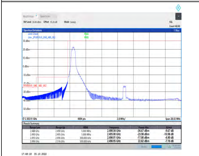
1-N41-PC2-30-20-L-4-CP-QPSK-Edge_1RB_Left-1@0 -Ant1-1--PASS-see graph
