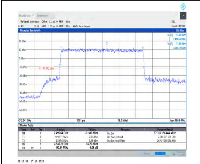
1-N41-PC2-30-90-L-8-CP-64QAM-Outer_Full-245@0 -Ant1-87.312-90.540-≤90-PASS
