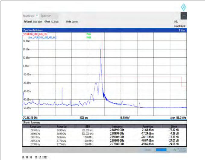
1-N41-PC2-30-80-H-2-DFT-QPSK-Edge_1RB_Right-1 @216-Ant1-1--PASS-see graph
