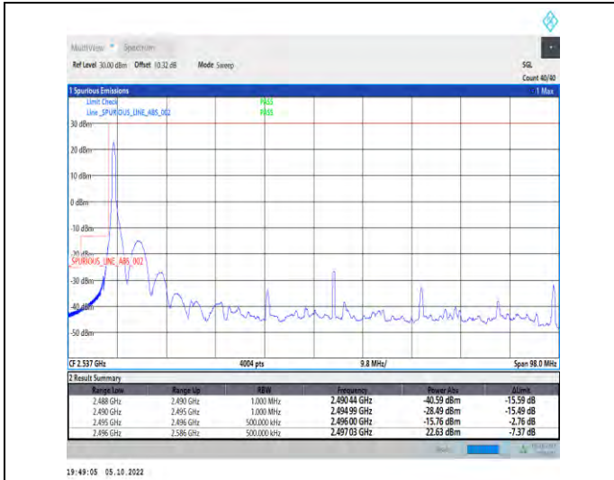
1-N41-PC2-30-90-L-1-DFT-QPSK-Edge_1RB_Left-1@0-Ant1-1--PASS-see graph
