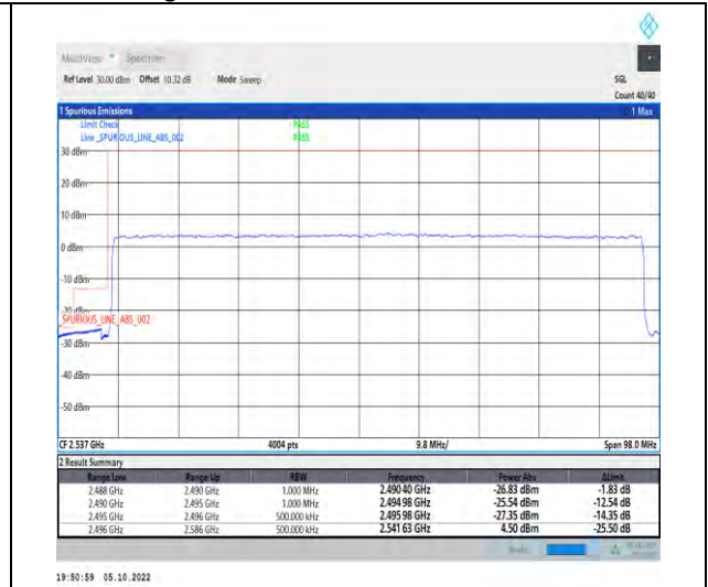
1-N41-PC2-30-90-L-3-DFT-QPSK-Outer_Full-240@0-Ant1-1--PASS-see graph
