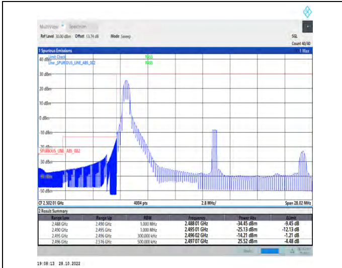
1-N41-PC2-30-20-L-1-DFT-PI2BPSK-Edge_1RB_Left-1@0-Ant1-1--PASS-see graph
