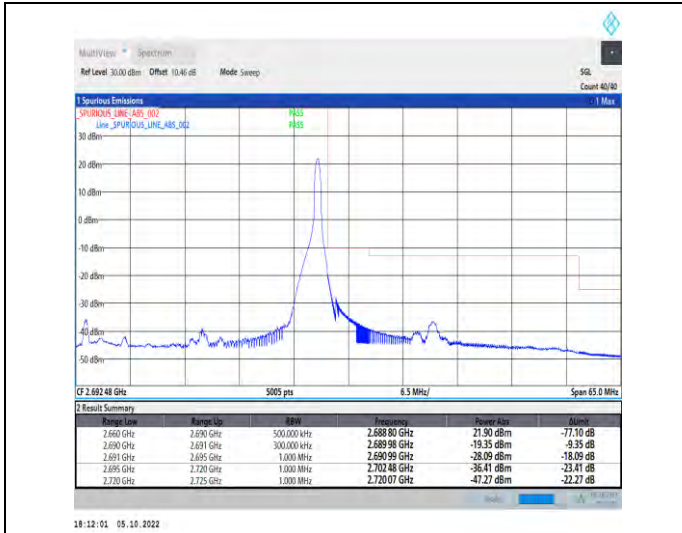
1-N41-PC2-30-30-H-2-DFT-QPSK-Edge_1RB_Right-1 @77-Ant1-1--PASS-see graph
