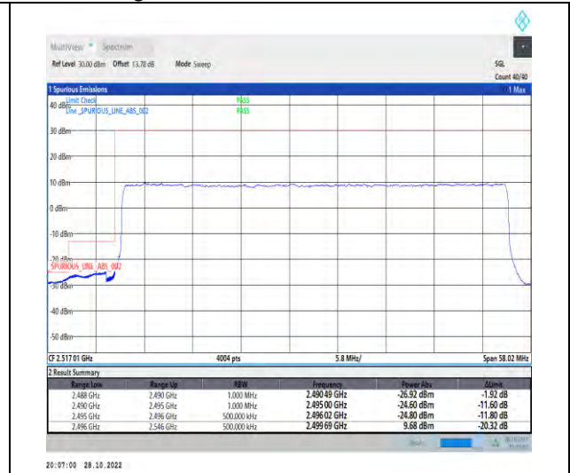
1-N41-PC2-30-50-L-3-DFT-PI2BPSK-Outer_Full-128@0-Ant1-1--PASS-see graph
