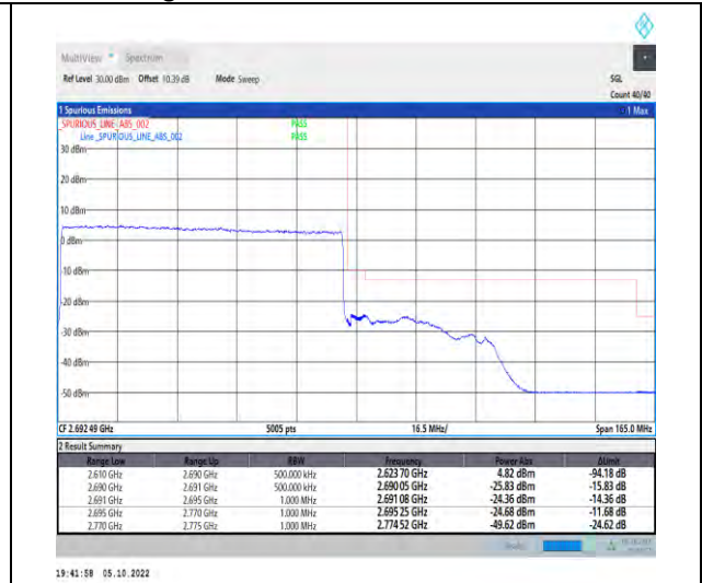
1-N41-PC2-30-80-H-3-DFT-QPSK-Outer_Full-216 @0-Ant1-1--PASS-see graph
