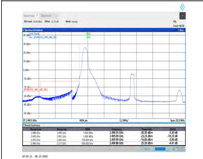
1-N41-PC2-30-15-L-4-CP-QPSK-Edge_1RB_Left-1@0-Ant1-1--PASS-see graph
