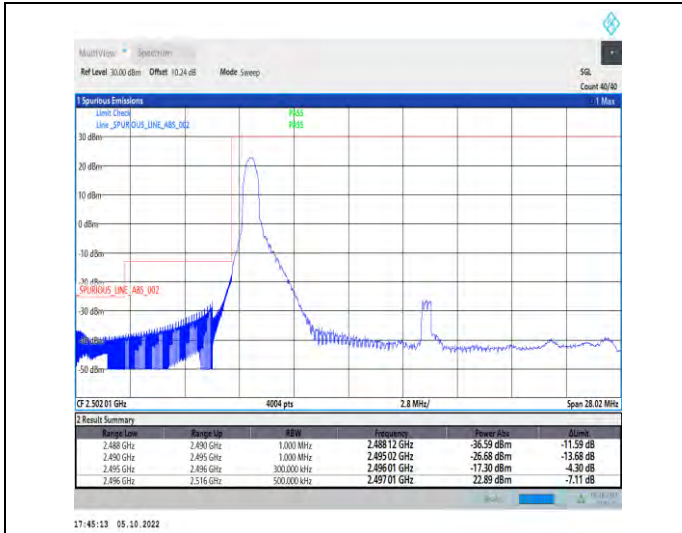
1-N41-PC2-30-20-L-1-DFT-QPSK-Edge_1RB_Left-1@ 0-Ant1-1--PASS-see graph
