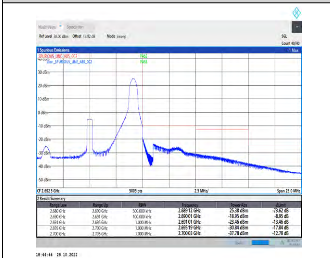
1-N41-PC2-30-10-H-5-CP-QPSK-Edge_1RB_Right-1@23-Ant1-1--PASS-see graph
