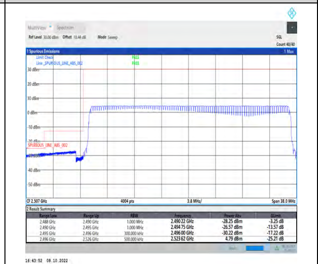
1-N41-PC2-30-30-L-6-CP-QPSK-Outer_Full-78@ 0-Ant1-1--PASS-see graph
