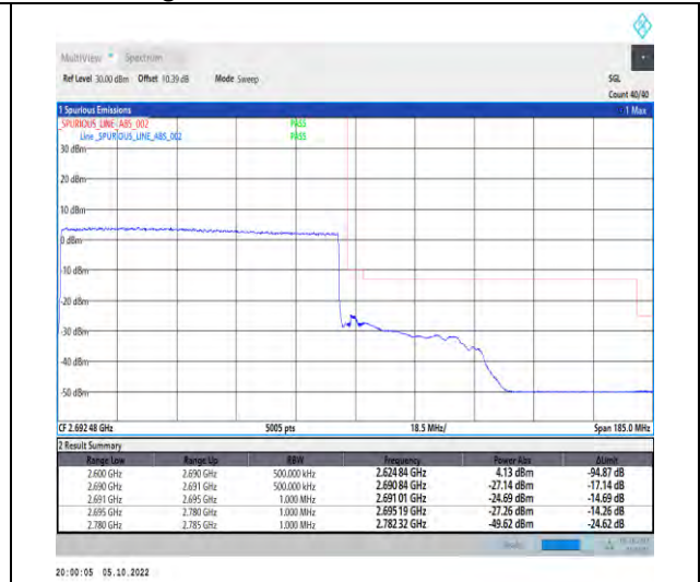
1-N41-PC2-30-90-H-3-DFT-QPSK-Outer_Full-240 @0-Ant1-1--PASS-see graph
