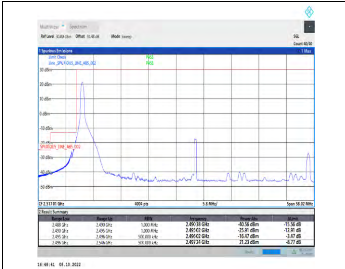
1-N41-PC2-30-50-L-1-DFT-QPSK-Edge_1RB_Left-1@0-Ant1-1--PASS-see graph
