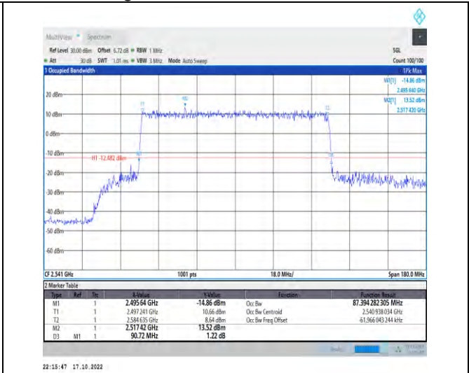
1-N41-PC2-30-90-L-7-CP-16QAM-Outer_Full-245@0 -Ant1-87.394-90.720-≤90-PASS
