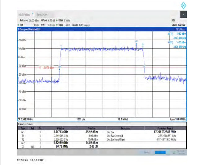
1-N41-PC2-30-90-M-8-CP-64QAM-Outer_Full-245 @0-Ant1-87.247-90.720-≤90-PASS
