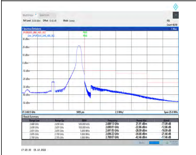
1-N41-PC2-30-10-H-5-CP-QPSK-Edge_1RB_Right-1 @23-Ant1-1--PASS-see graph
