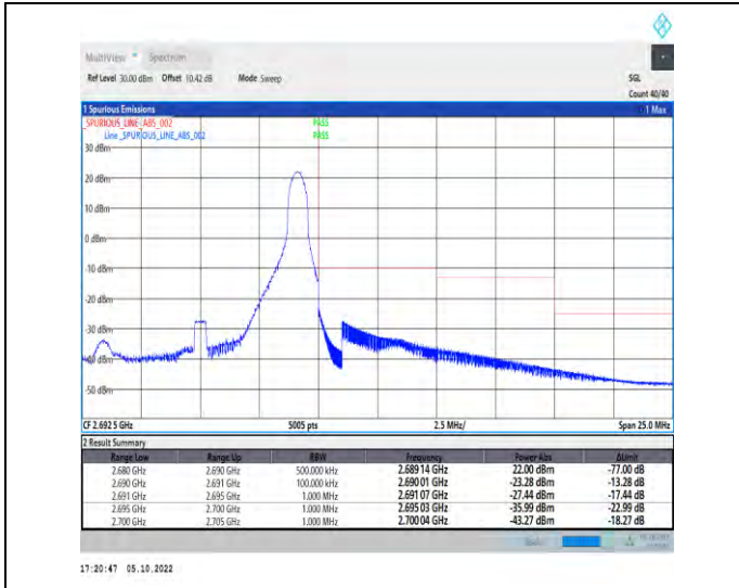
1-N41-PC2-30-10-H-2-DFT-QPSK-Edge_1RB_Right-1 @23-Ant1-1--PASS-see graph
