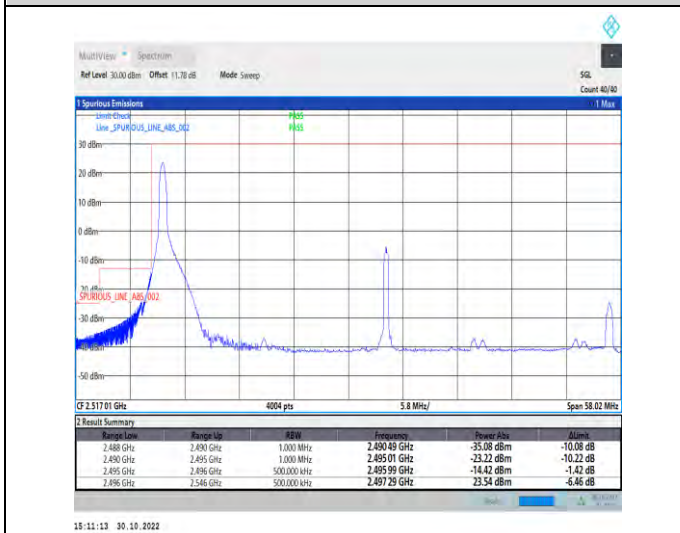
1-N41-PC2-30-50-L-4-CP-QPSK-Edge_1RB_Left-1@0-Ant1-1--PASS-see graph
