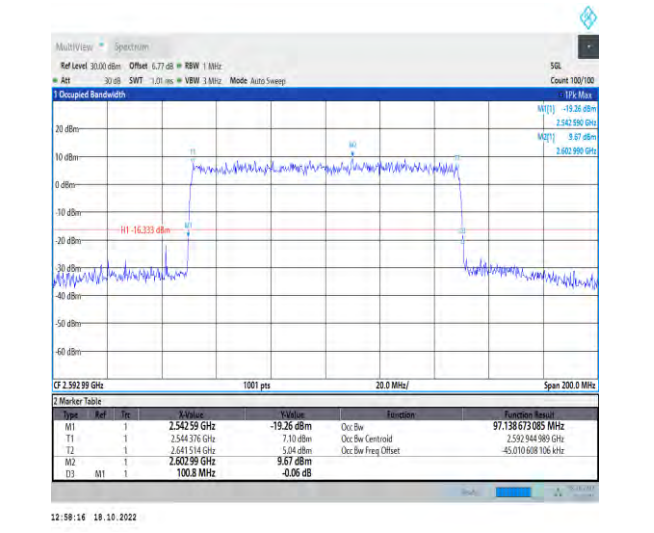
1-N41-PC2-30-100-M-9-CP-256QAM-Outer_Full-273 @0-Ant1-97.139-100.800-≤100-PASS
