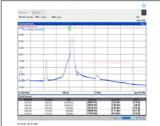
1-N41-PC2-30-20-H-2-DFT-PI2BPSK-Edge_1RB_Righ t-1@50-Ant1-1--PASS-see graph
