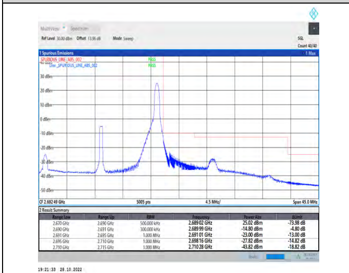
1-N41-PC2-30-20-H-5-CP-QPSK-Edge_1RB_Righ t1 @50-Ant1-1--PASS-see graph
