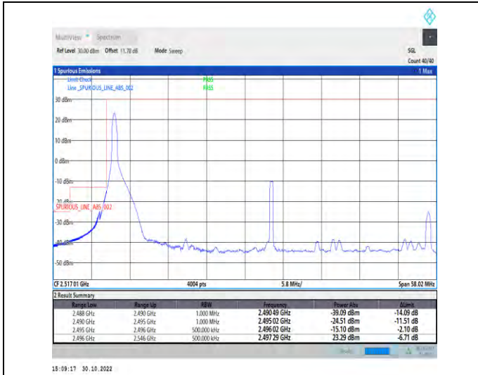
1-N41-PC2-30-50-L-1-DFT-PI2BPSK-Edge_1RB_Left-1@0-Ant1-1--PASS-see graph
