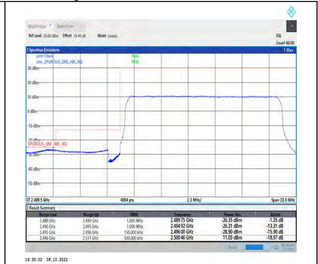
1-N41-PC2-30-15-L-3-DFT-QPSK-Outer_Full-36@0-Ant1-1--PASS-see graph
