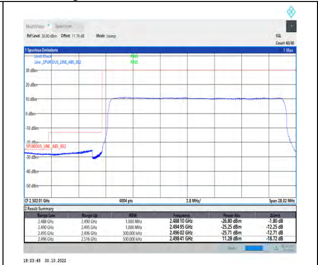
1-N41-PC2-30-20-L-3-DFT-PI2BPSK-Outer_Full-50@0-Ant1-1--PASS-see graph
