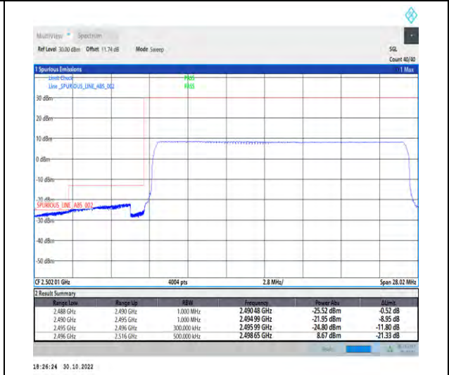
1-N41-PC2-30-20-L-6-CP-QPSK-Outer_Full-51@0-Ant1-1--PASS-see graph
