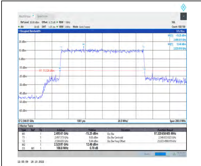
1-N41-PC2-30-100-L-6-CP-QPSK-Outer_Full-273@ 0-Ant1-97.321-100.800-≤100-PASS
