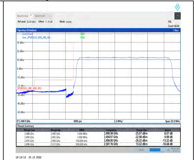
1-N41-PC2-30-15-L-3-DFT-PI2BPSK-Outer_Full-36@0-Ant1-1--PASS-see graph
