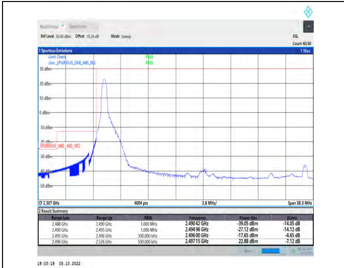
1-N41-PC2-30-30-L-1-DFT-QPSK-Edge_1RB_Left-1@ 0-Ant1-1--PASS-see graph
