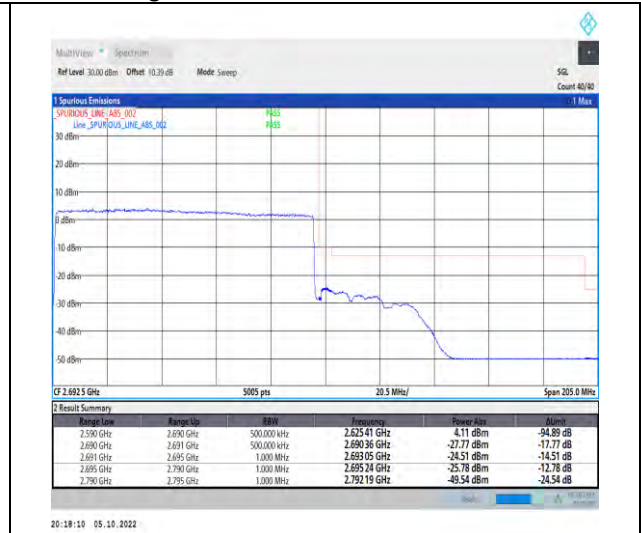
1-N41-PC2-30-100-H-3-DFT-QPSK-Outer_Full-270@0-Ant1-1--PASS-see graph
