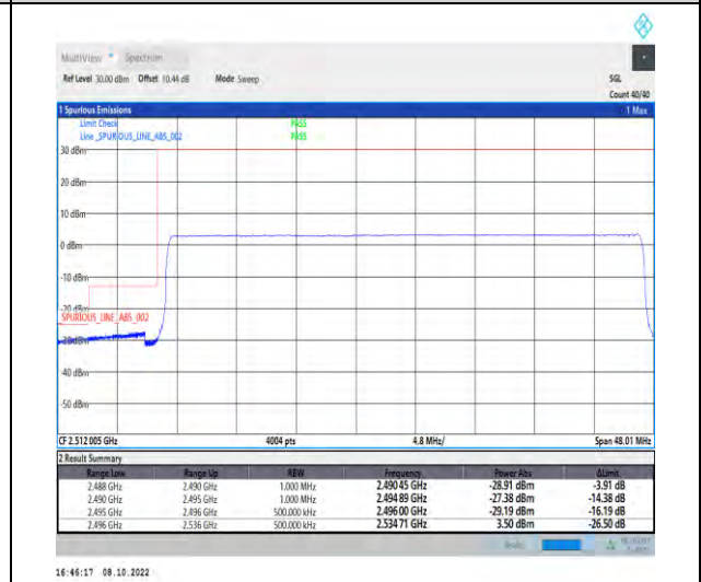
1-N41-PC2-30-40-L-6-CP-QPSK-Outer_Full-106@0-Ant1-1--PASS-see graph
