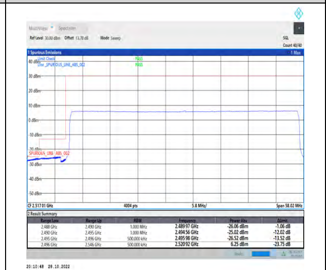
1-N41-PC2-30-50-L-6-CP-QPSK-Outer_Full-133@0-Ant1-1--PASS-see graph
