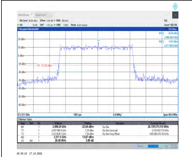
1-N41-PC2-30-30-L-4-DFT-64QAM-Outer_Full-75@0 -Ant1-26.74-28.380-≤30-PASS
