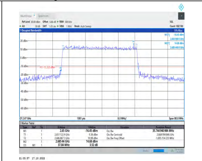
1-N41-PC2-30-40-H-3-DFT-16QAM-Outer_Full-100 @0-Ant1-35.745-37.840-≤40-PASS
