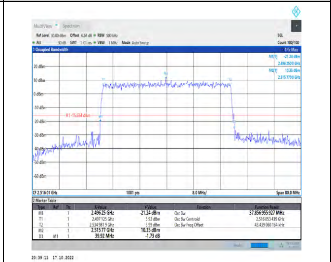
1-N41-PC2-30-40-L-9-CP-256QAM-Outer_Full-106@0 -Ant1-37.857-39.920-≤40-PASS
