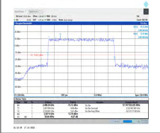
1-N41-PC2-30-60-L-4-DFT-64QAM-Outer_Full-162 @0-Ant1-57.748-59.640-≤60-PASS
