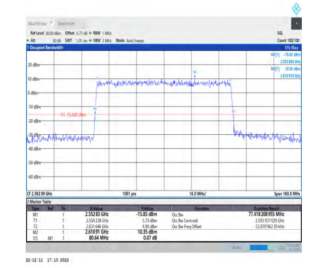
1-N41-PC2-30-80-M-9-CP-256QAM-Outer_Full-217@0-Ant1-77.418-80.640-≤80-PASS
