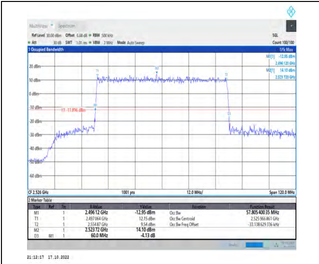
1-N41-PC2-30-60-L-1-DFT-QPSK-Outer_Full-162@ 0-Ant1-57.805-60.000-≤60-PASS
