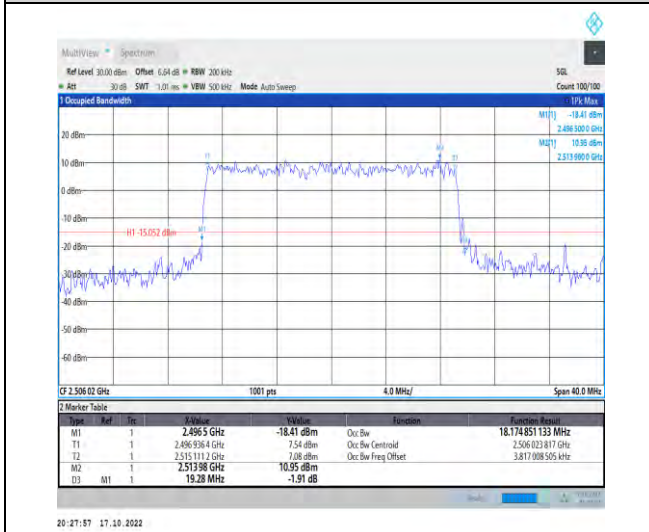
1-N41-PC2-30-20-L-8-CP-64QAM-Outer_Full-51@0-Ant1-18.175-19.280-≤20-PASS
