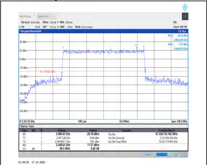
1-N41-PC2-30-50-L-7-CP-16QAM-Outer_Full-133@0 -Ant1-47.537-49.500-≤50-PASS
