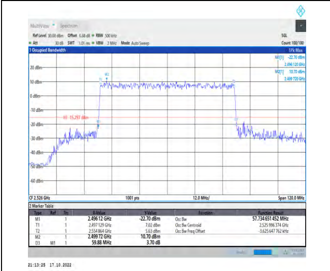
1-N41-PC2-30-60-L-8-CP-64QAM-Outer_Full-162@0 -Ant1-57.735-59.880-≤60-PASS
