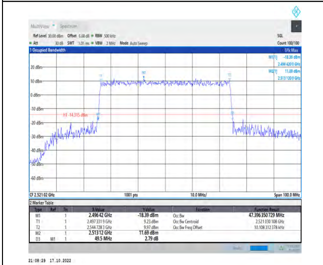
1-N41-PC2-30-50-L-8-CP-64QAM-Outer_Full-133@0 -Ant1-47.396-49.500-≤50-PASS
