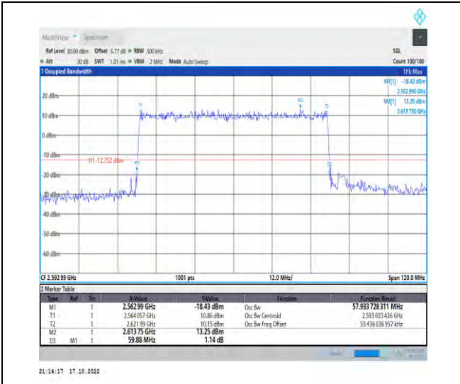
1-N41-PC2-30-60-M-1-DFT-QPSK-Outer_Full-162@ 0-Ant1-57.934-59.880-≤60-PASS
