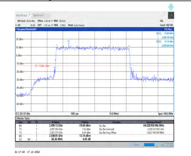
1-N41-PC2-30-70-L-3-DFT-16QAM-Outer_Full-180@0-Ant1-64.029-66.360-≤70-PASS
