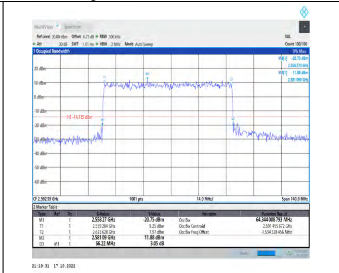
1-N41-PC2-30-70-M-3-DFT-16QAM-Outer_Full-180 @0-Ant1-64.344-66.220-≤70-PASS
