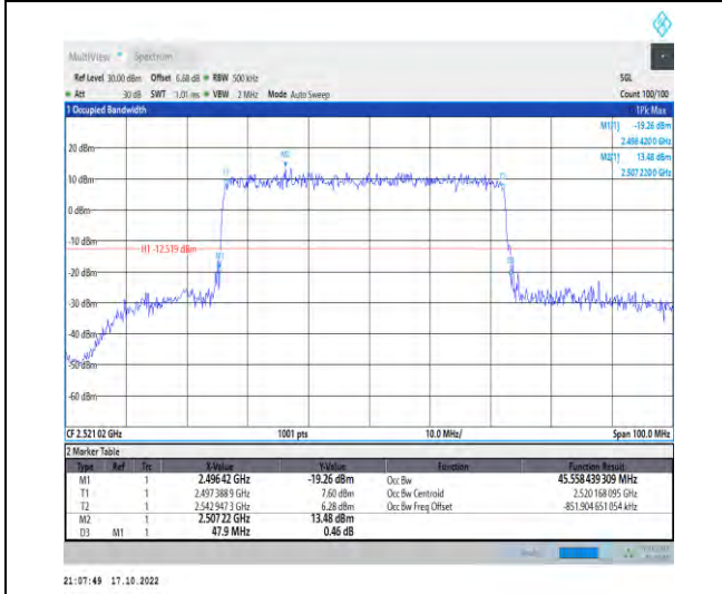
1-N41-PC2-30-50-L-4-DFT-64QAM-Outer_Full-128 @0-Ant1-45.558-47.900-≤50-PASS
