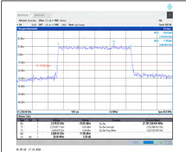
1-N41-PC2-30-30-M-6-CP-QPSK-Outer_Full-78@0-Ant1-27.781-29.040-≤30-PASS
