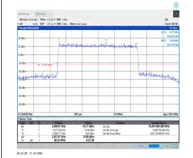
1-N41-PC2-30-80-H-4-DFT-64QAM-Outer_Full-216 @0-Ant1-76.941-80.320-≤80-PASS
