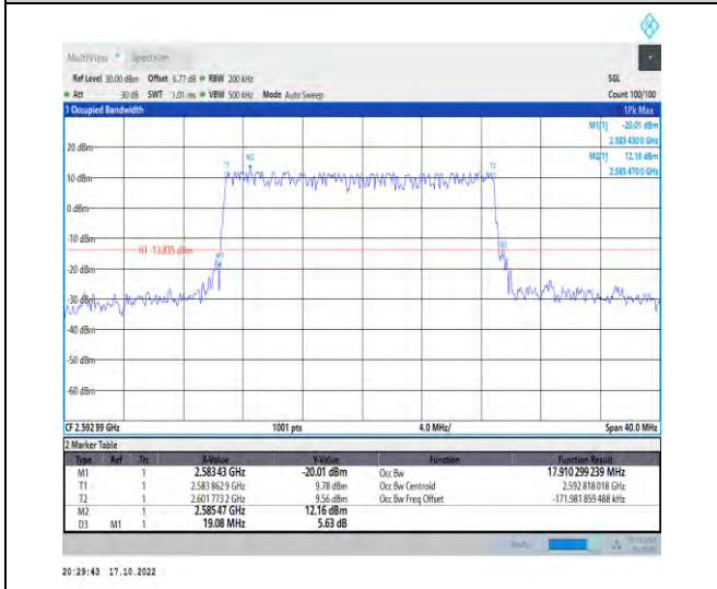
1-N41-PC2-30-20-M-4-DFT-64QAM-Outer_Full-50 @0-Ant1-17.91-19.080-<=20-PASS
