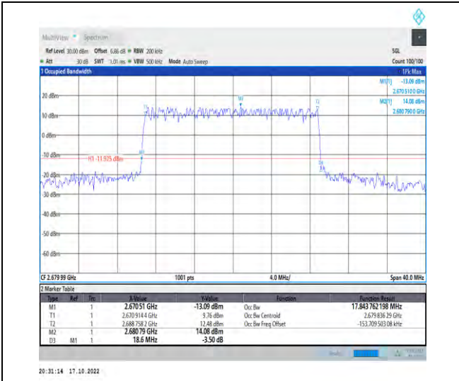
1-N41-PC2-30-20-H-1-DFT-QPSK-Outer_Full-50@0 -Ant1-17.844-18.600-≤20-PASS
