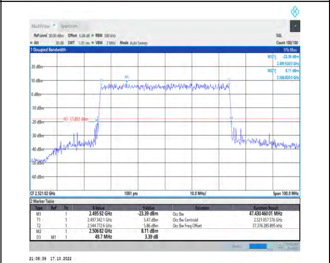
1-N41-PC2-30-50-L-9-CP-256QAM-Outer_Full-133@0 -Ant1-47.43-49.700-≤50-PASS
