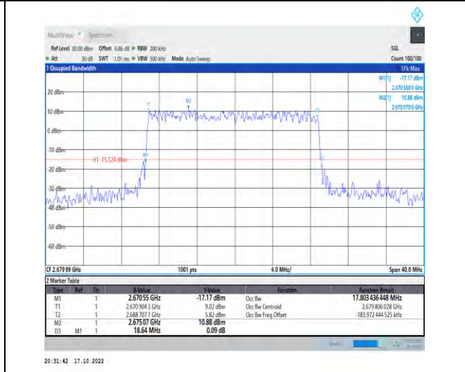
1-N41-PC2-30-20-H-5-DFT-256QAM-Outer_Full-50@0 -Ant1-17.803-18.640-≤20-PASS
