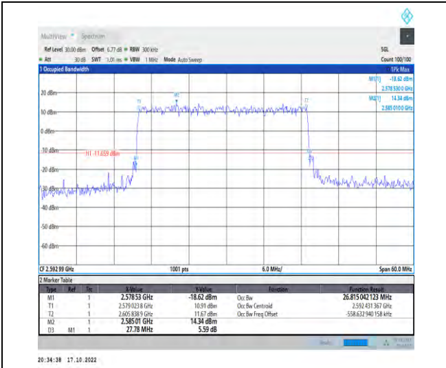
1-N41-PC2-30-30-M-1-DFT-QPSK-Outer_Full-75@0-Ant1-26.815-27.780-≤30-PASS
