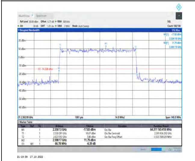
1-N41-PC2-30-70-M-4-DFT-64QAM-Outer_Full-180 @0-Ant1-64.311-66.780-≤70-PASS
