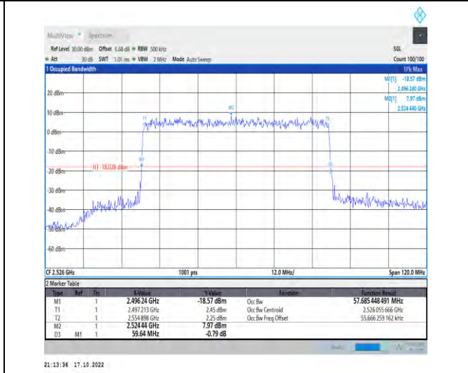
1-N41-PC2-30-60-L-9-CP-256QAM-Outer_Full-162@0 -Ant1-57.685-59.640-≤60-PASS
