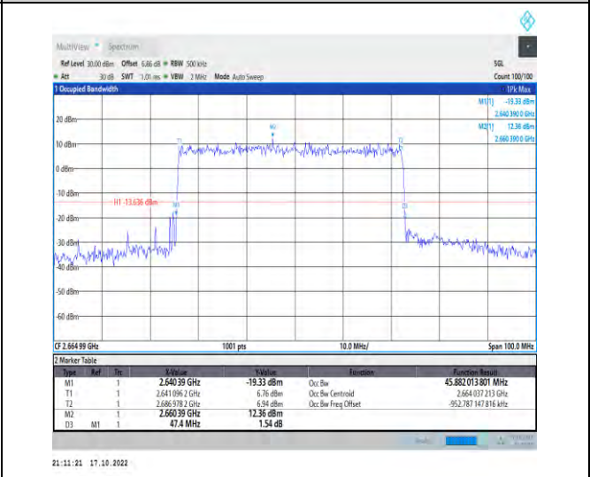
1-N41-PC2-30-50-H-5-DFT-256QAM-Outer_Full-128 @0-Ant1-45.882-47.400-≤50-PASS
