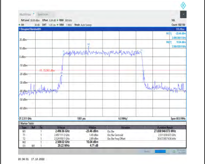
1-N41-PC2-30-30-L-9-CP-256QAM-Outer_Full-78@0-Ant1-27.839-29.220-≤30-PASS
