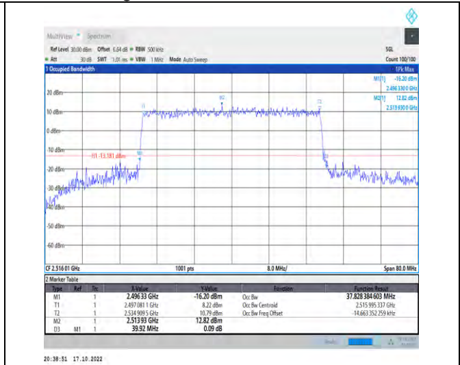
1-N41-PC2-30-40-L-7-CP-16QAM-Outer_Full-106@0 -Ant1-37.828-39.920-≤40-PASS
