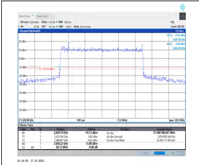
1-N41-PC2-30-60-H-1-DFT-QPSK-Outer_Full-162@ 0-Ant1-57.941-60.120-≤60-PASS
