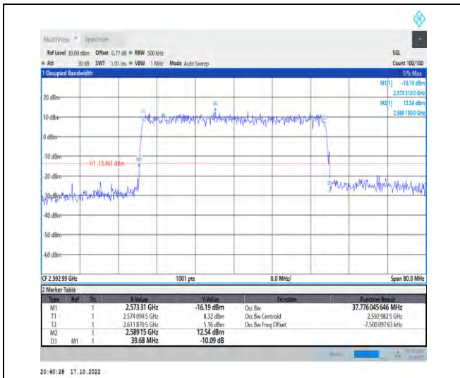
1-N41-PC2-30-40-M-6-CP-QPSK-Outer_Full-106@ 0-Ant1-37.776-39.680-≤40-PASS
