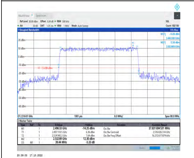
1-N41-PC2-30-40-L-8-CP-64QAM-Outer_Full-106@0 -Ant1-37.832-39.440-≤40-PASS
