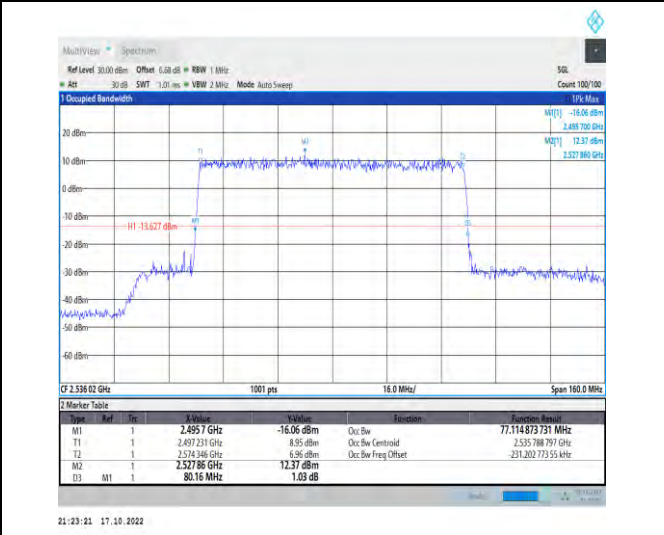
1-N41-PC2-30-80-L-5-DFT-256QAM-Outer_Full-216 @0-Ant1-77.115-80.160-≤80-PASS
