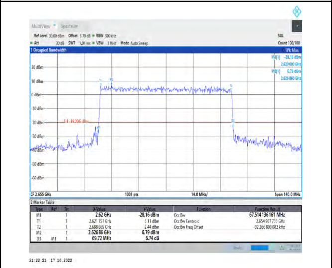
1-N41-PC2-30-70-H-9-CP-256QAM-Outer_Full-189@0 -Ant1-67.514-69.720-≤70-PASS
