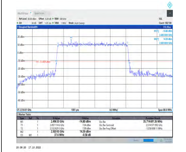
1-N41-PC2-30-40-L-4-DFT-64QAM-Outer_Full-100 @0-Ant1-35.715-37.600-≤40-PASS
