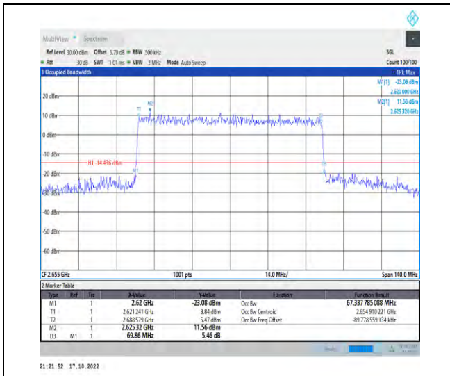
1-N41-PC2-30-70-H-6-CP-QPSK-Outer_Full-189@0 -Ant1-67.338-69.860-≤70-PASS
