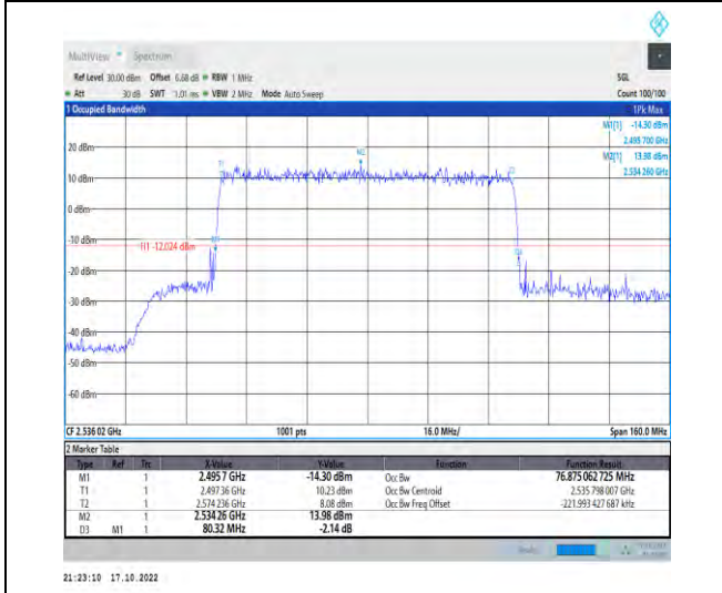
1-N41-PC2-30-80-L-4-DFT-64QAM-Outer_Full-216 @0-Ant1-76.875-80.320-≤80-PASS
