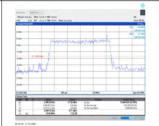
1-N41-PC2-30-15-L-9-CP-256QAM-Outer_Full-38@0-Ant1-13.644-14.460-≤15-PASS
