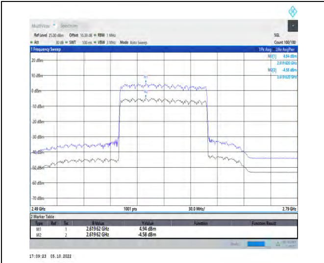
1-N41-PC2-30-100-H-1-DFT-256QAM-Outer_Full-27 0@0-Ant1-9.52-100%-0.00-9.52-PASS-≤13
