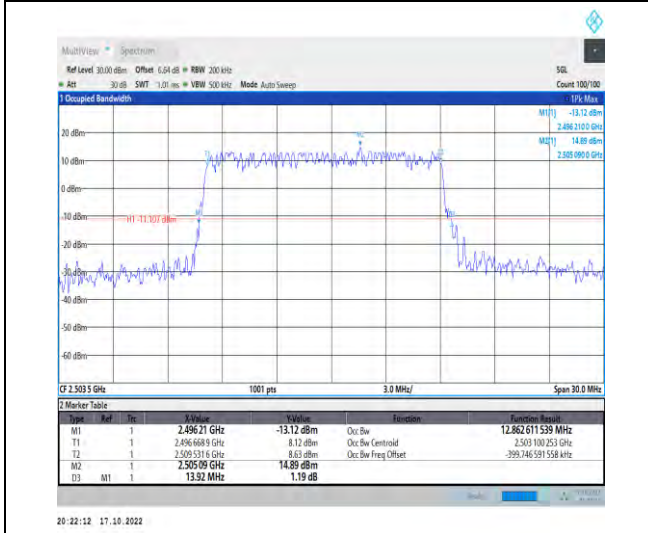
1-N41-PC2-30-15-L-4-DFT-64QAM-Outer_Full-36@0 -Ant1-12.863-13.920-≤15-PASS
