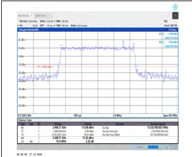
1-N41-PC2-30-15-L-6-CP-QPSK-Outer_Full-38@0-Ant1-13.532-14.400-≤15-PASS
