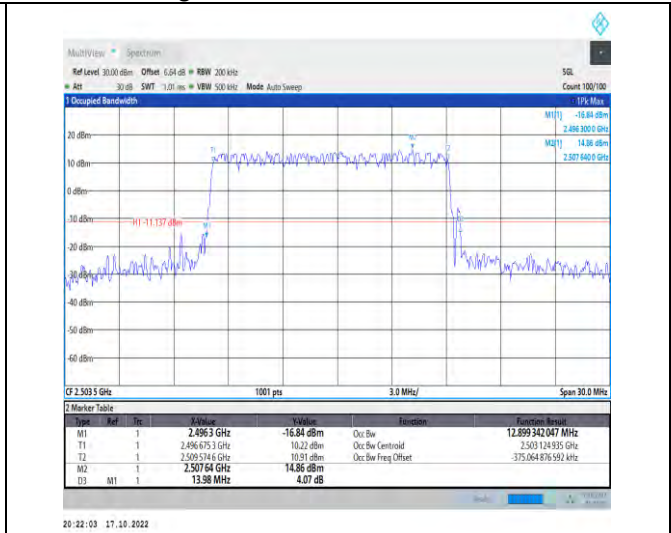
1-N41-PC2-30-15-L-3-DFT-16QAM-Outer_Full-36@0 -Ant1-12.899-13.980-≤15-PASS
