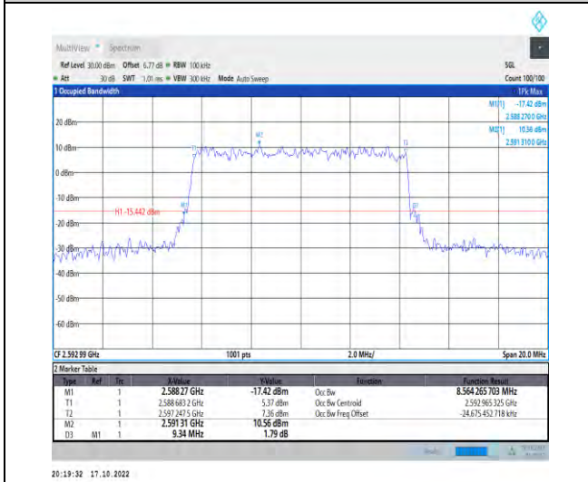
1-N41-PC2-30-10-M-8-CP-64QAM-Outer_Full-24@0-Ant1-8.564-9.340-≤10-PASS
