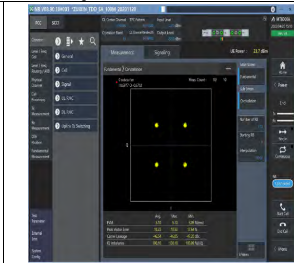
1-N41--30-100-M-6-CP-QPSK-Outer_Full-273@0-Ant1-see graph-PASS
