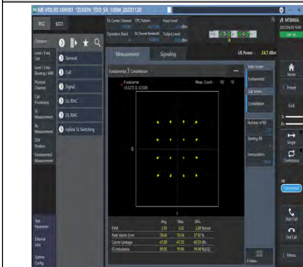
1-N41--30-100-M-3-DFT-16QAM-Outer_Full-270@0-Ant1-see graph-PASS
