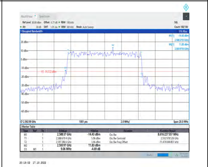
1-N41-PC2-30-10-M-5-DFT-256QAM-Outer_Full-24 @0-Ant1-8.616-9.060-≤10-PASS
