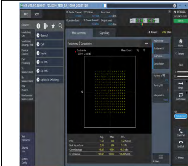
1-N41--30-100-M-9-CP-256QAM-Outer_Full-273@0-Ant1-see graph-PASS
