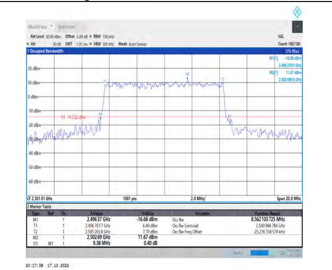
1-N41-PC2-30-10-L-7-CP-16QAM-Outer_Full-24@0-Ant1-8.562-9.380-≤10-PASS
