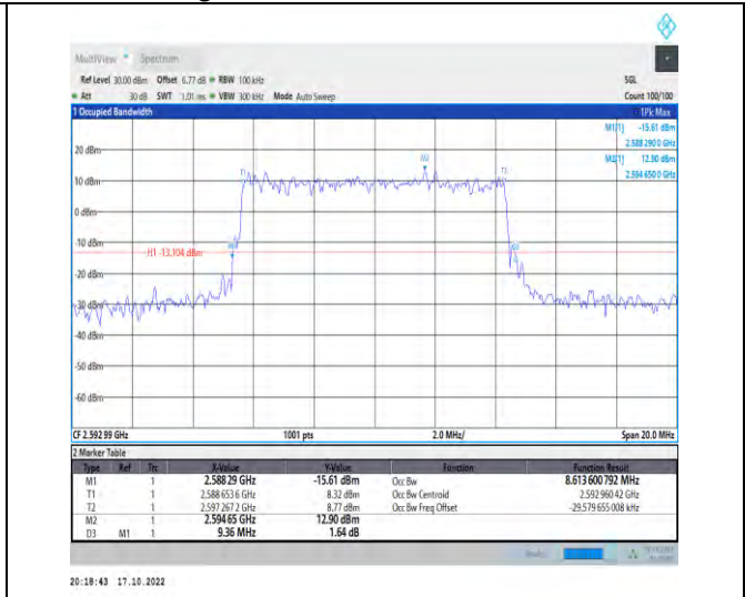
1-N41-PC2-30-10-M-3-DFT-16QAM-Outer_Full-24@ 0-Ant1-8.614-9.360-≤10-PASS
