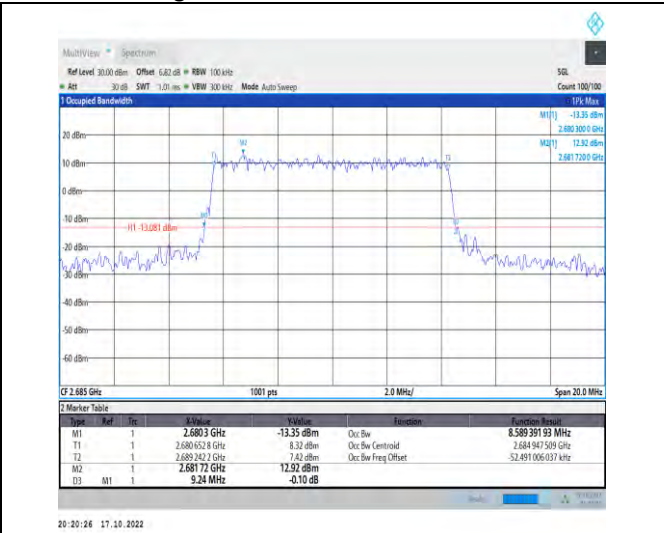
1-N41-PC2-30-10-H-3-DFT-16QAM-Outer_Full-24@ 0-Ant1-8.589-9.240-≤10-PASS
