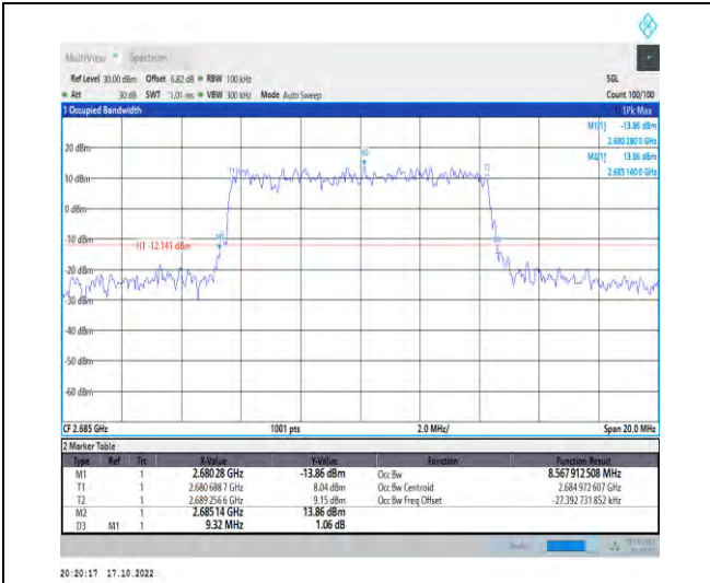
1-N41-PC2-30-10-H-1-DFT-QPSK-Outer_Full-24@0 -Ant1-8.568-9.320-≤10-PASS
