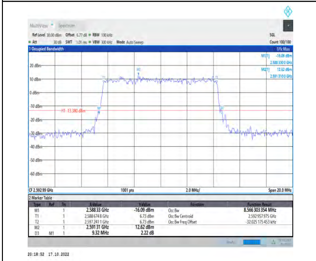
1-N41-PC2-30-10-M-4-DFT-64QAM-Outer_Full-24 @0-Ant1-8.566-9.320-≤10-PASS
