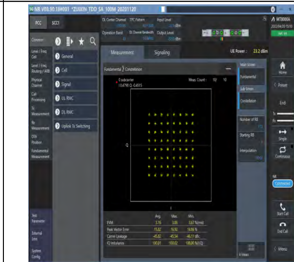
1-N41--30-100-M-8-CP-64QAM-Outer_Full-273@0-Ant1-see graph-PASS
