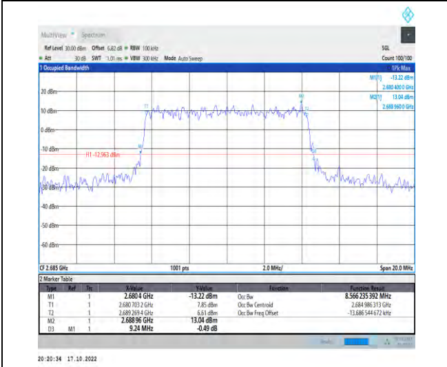
1-N41-PC2-30-10-H-4-DFT-64QAM-Outer_Full-24@ 0-Ant1-8.566-9.240-≤10-PASS
