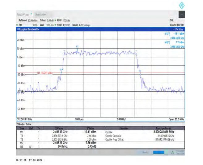
1-N41-PC2-30-10-L-9-CP-256QAM-Outer_Full-24@0-Ant1-8.57-9.400-≤10-PASS
