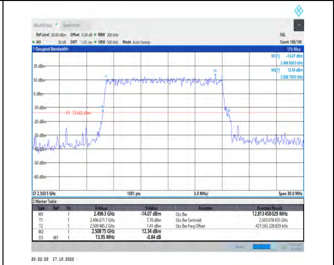
1-N41-PC2-30-15-L-5-DFT-256QAM-Outer_Full-36@0 -Ant1-12.813-13.950-≤15-PASS
