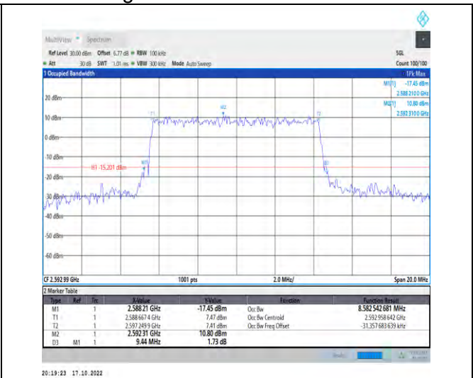
1-N41-PC2-30-10-M-7-CP-16QAM-Outer_Full-24@0-Ant1-8.583-9.440-≤10-PASS
