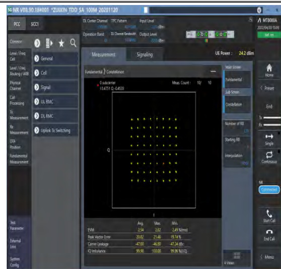
1-N41--30-100-M-4-DFT-64QAM-Outer_Full-270@0-Ant1-see graph-PASS
