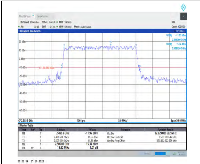
1-N41-PC2-30-15-L-1-DFT-QPSK-Outer_Full-36@0 -Ant1-12.83-13.920-≤15-PASS
