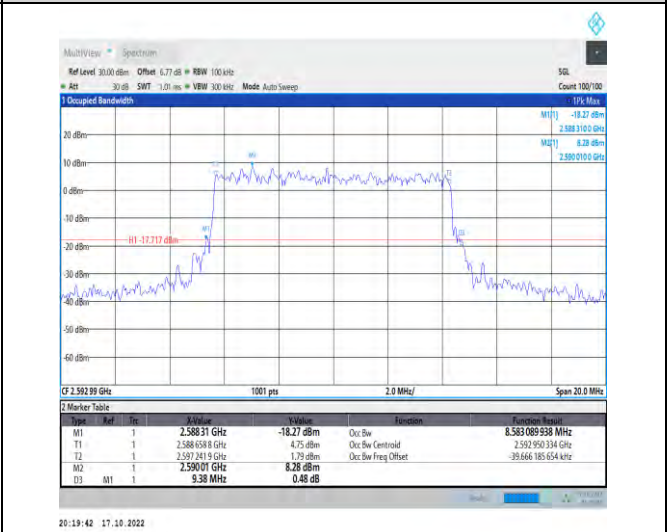
1-N41-PC2-30-10-M-9-CP-256QAM-Outer_Full-24@0-Ant1-8.583-9.380-≤10-PASS
