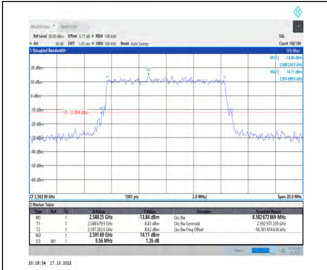
1-N41-PC2-30-10-M-1-DFT-QPSK-Outer_Full-24@0 -Ant1-8.583-9.560-≤10-PASS
