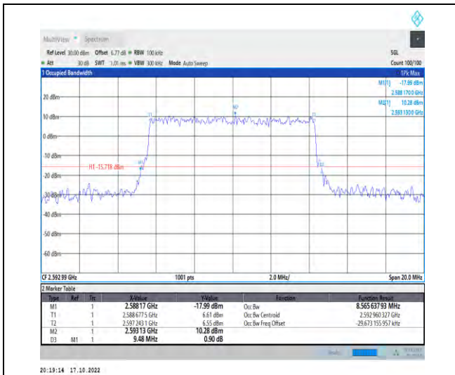
1-N41-PC2-30-10-M-6-CP-QPSK-Outer_Full-24@0-Ant1-8.566-9.480-≤10-PASS
