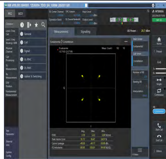
1-N41--30-100-M-2-DFT-QPSK-Outer_Full-270@0-Ant1-see graph-PASS
