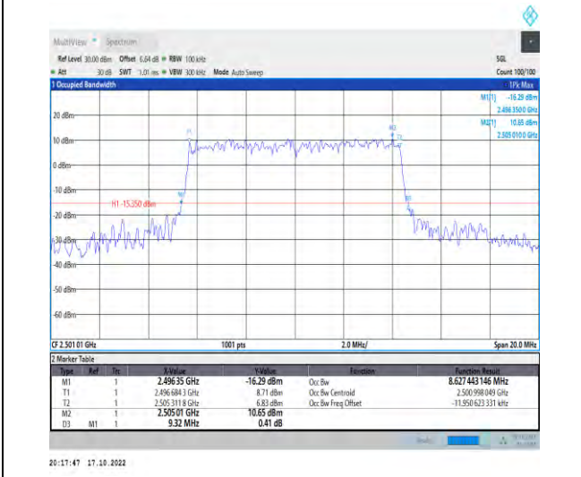
1-N41-PC2-30-10-L-8-CP-64QAM-Outer_Full-24@0-Ant1-8.627-9.320-≤10-PASS
