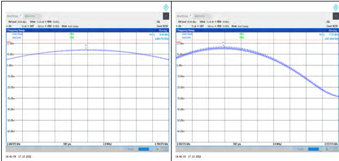
1-N48-PC3-30-10-H-3-CP-QPSK-Outer_Full-24@0-3684 .975-3704.975-Ant2-3695.10-14.59-23-PASS
