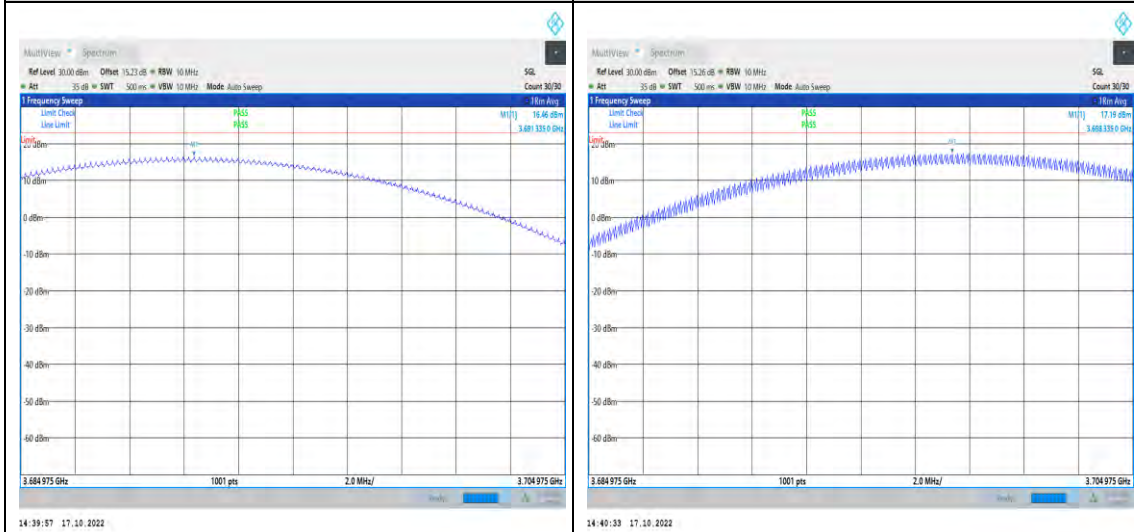
1-N48-PC3-30-10-H-1-CP-QPSK-Inner_1RB_Left-1@1- 3684.975-3704.975-Ant2-3691.22-16.46-23-PASS
