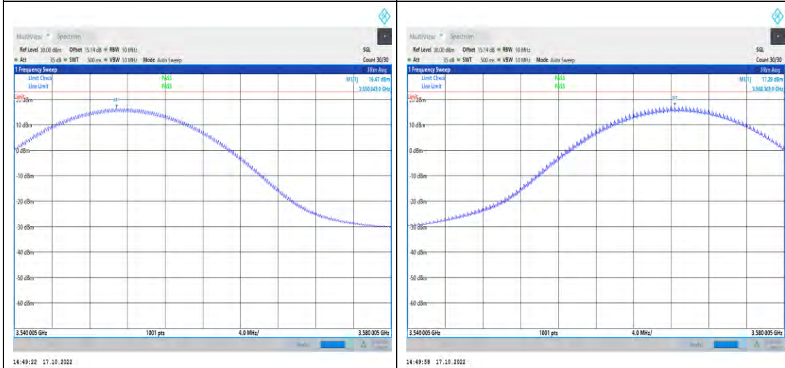
1-N48-PC3-30-20-L-1-CP-QPSK-Inner_1RB_Left-1@1-3 540.005-3580.005-Ant2-3551.53-16.47-23-PASS
