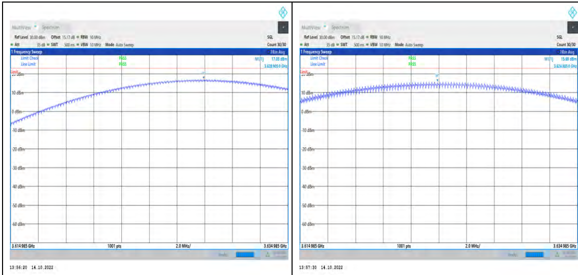
1-N48-PC3-30-10-M-2-CP-QPSK-Inner_1RB_Right-1@2 2-3614.985-3634.985-Ant1-3633.63-17.03-23-PASS
