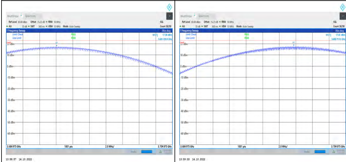
1-N48-PC3-30-10-H-1-CP-QPSK-Inner_1RB_Left-1@1- 3684.975-3704.975-Ant1-3691.70-17.39-23-PASS
