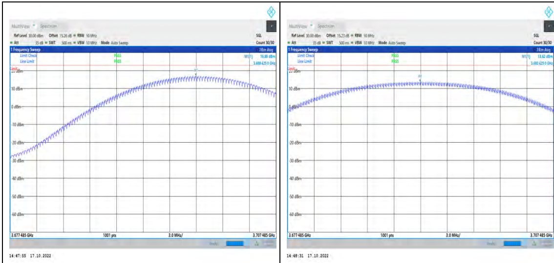
1-N48-PC3-30-15-H-2-CP-QPSK-Inner_1RB_Right-1@3 6-3677.485-3707.485-Ant2-3698.97-16.89-23-PASS
