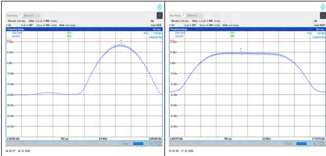
1-N48-PC3-30-40-L-2-CP-QPSK-Inner_1RB_Right-1@1 04-3529.995-3609.995-Ant1-3588.16-17.69-23-PASS
