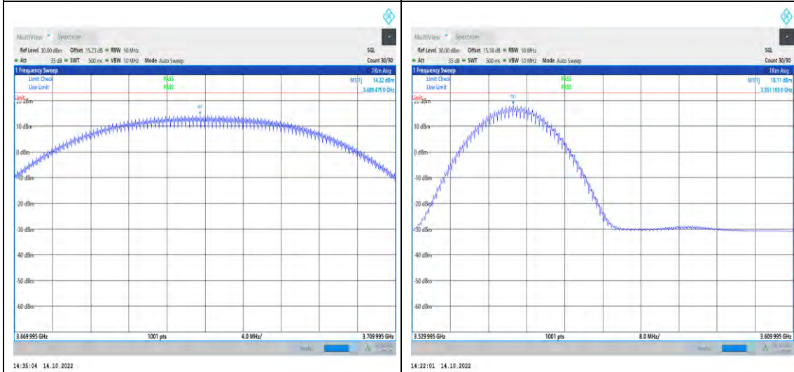
1-N48-PC3-30-20-H-3-CP-QPSK-Outer_Full-51@0-3669 .995-3709.995-Ant1-3691.32-14.22-23-PASS
