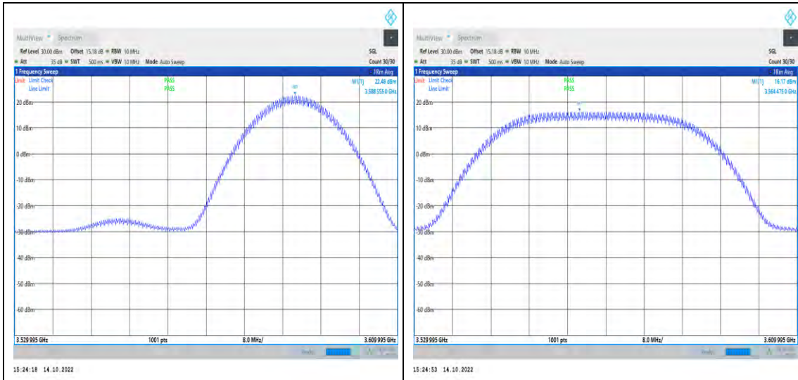
1-N48-PC3-30-40-L-5-DFT-QPSK-Inner_1RB_Right-1@ 104-3529.995-3609.995-Ant1-3588.72-22.48-99-PASS
