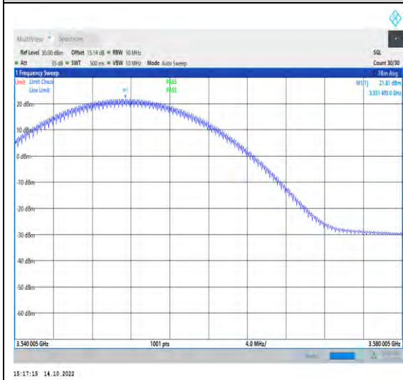
1-N48-PC3-30-20-L-4-DFT-QPSK-Inner_1RB_Left-1@1- 3540.005-3580.005-Ant1-3551.81-21.81-99-PASS
