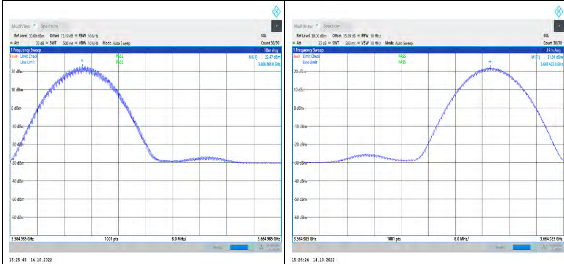
1-N48-PC3-30-40-M-4-DFT-QPSK-Inner_1RB_Left-1@1 -3584.985-3664.985-Ant1-3606.51-22.47-99-PASS
