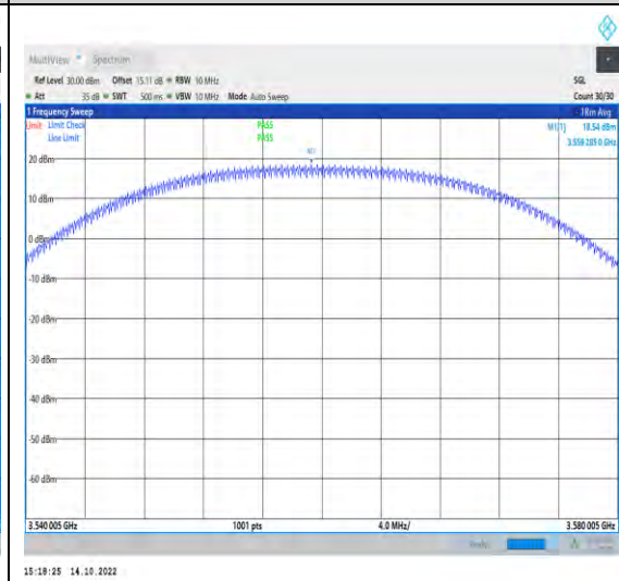
1-N48-PC3-30-20-L-6-DFT-QPSK-Outer_Full-50@0-354 0.005-3580.005-Ant1-3567.93-18.54-99-PASS
