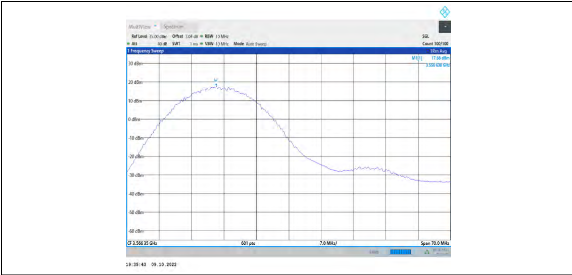
48-48-15MHz-20MHz-16QAM-16QAM-55318-55489-75RB#0-100RB#0
