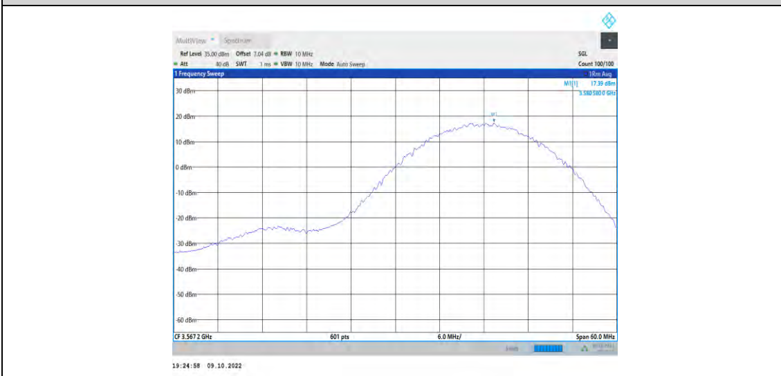
48-48-20MHz-10MHz-16QAM-16QAM-55340-55484-100RB#0-50RB#0
