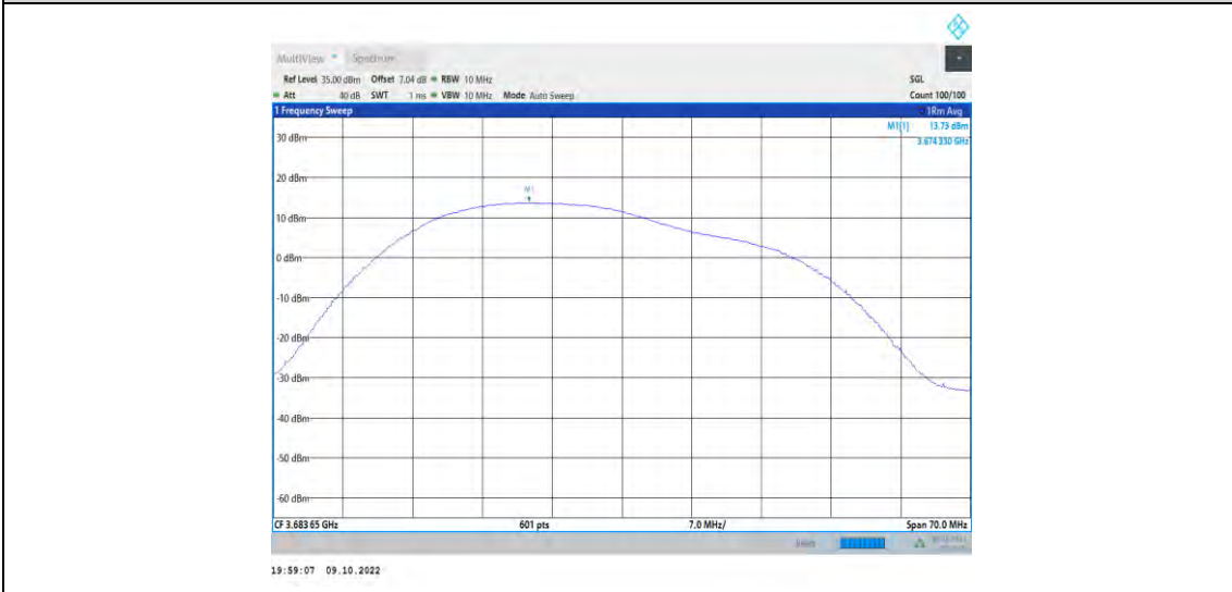
48-48-20MHz-15MHz-QPSK-QPSK-56491-56662-1RB#0-0RB#0
