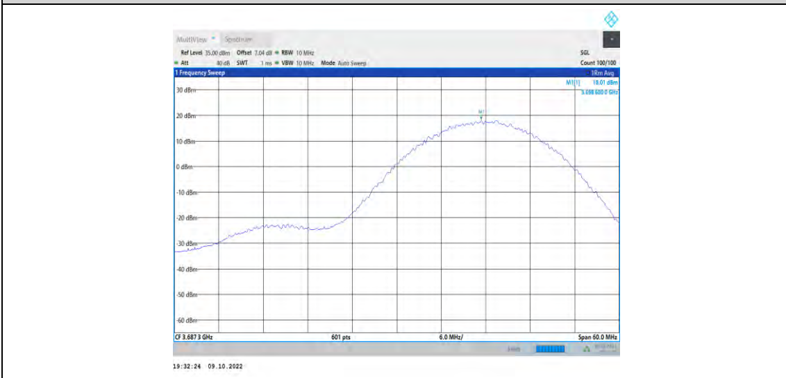
48-48-20MHz-10MHz-16QAM-16QAM-56541-56685-100RB#0-50RB#0
