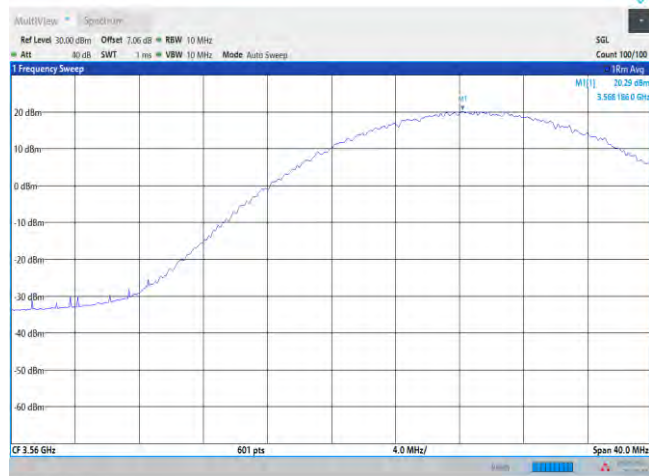
Band48-20MHz-16QAM-55340-1RB#99
