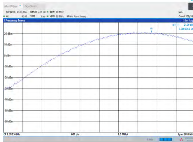
Band48-15MHz-16QAM-56665-1RB#74
