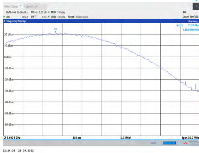
Band48-15MHz-16QAM-56665-1RB#0
