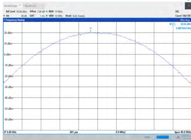
Band48-20MHz-16QAM-56640-1RB#99
