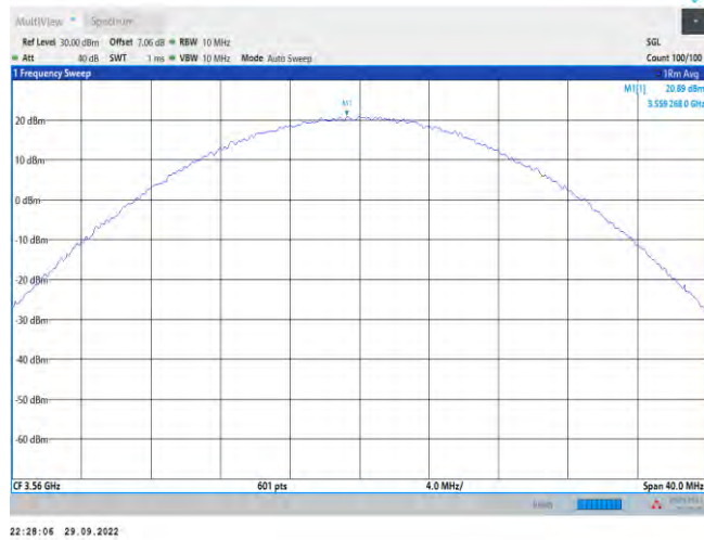
Band48-20MHz-16QAM-55340-1RB#99
