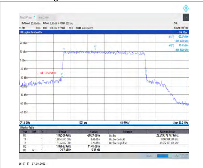
1-N25-PC3-15-30-H-7-CP-16QAM-Outer_Full-160@0 -Ant1-28.52-29.700-≤30-PASS
