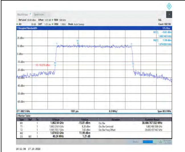
1-N25-PC3-15-40-M-8-CP-64QAM-Outer_Full-216 @0-Ant1-38.487-40.240-≤40-PASS
