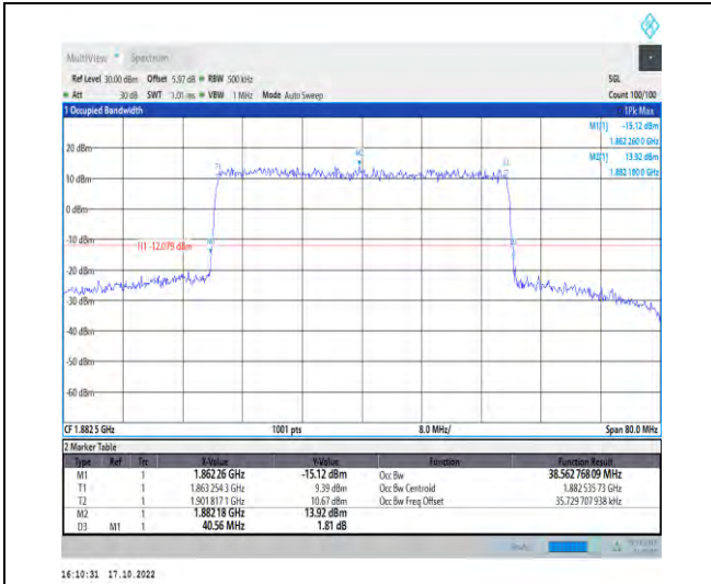
1-N25-PC3-15-40-M-1-DFT-QPSK-Outer_Full-216@ 0-Ant1-38.563-40.560-≤40-PASS
