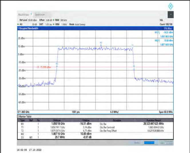
1-N25-PC3-15-30-L-5-DFT-256QAM-Outer_Full-160 @0-Ant1-28.526-29.700-≤30-PASS
