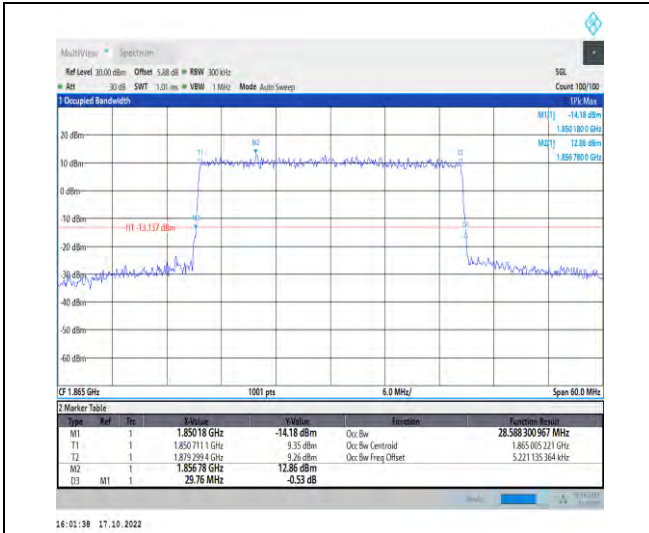
1-N25-PC3-15-30-L-1-DFT-QPSK-Outer_Full-160@ 0-Ant1-28.588-29.760-≤30-PASS
