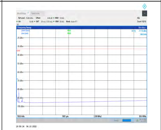
1-N25-PC3-15-40-M-1-DFT-QPSK-Inner_1RB_Left-1 @1-0.15-30-Ant1-0.15--71.73--33-PASS
