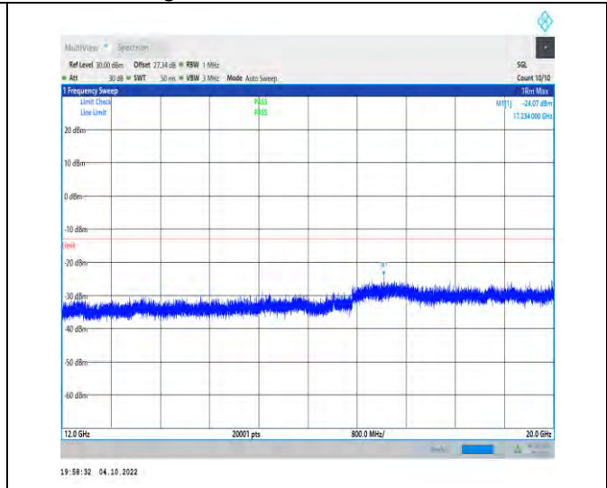
1-N25-PC3-15-40-L-1-DFT-QPSK-Inner_1RB_Left-1 @1-12000-20000-Ant1-17234.00--24.07--13-PASS
