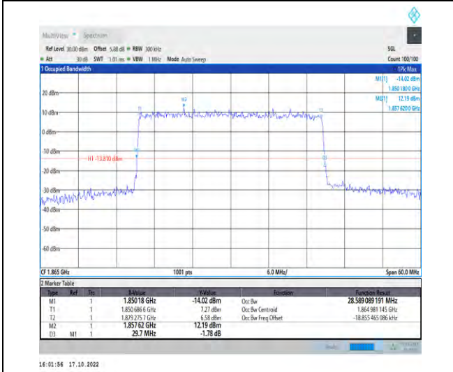
1-N25-PC3-15-30-L-4-DFT-64QAM-Outer_Full-160 @0-Ant1-28.589-29.700-≤30-PASS
