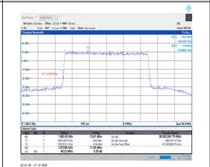
1-N25-PC3-15-40-M-5-DFT-256QAM-Outer_Full-216 @0-Ant1-38.583-40.320-≤40-PASS
