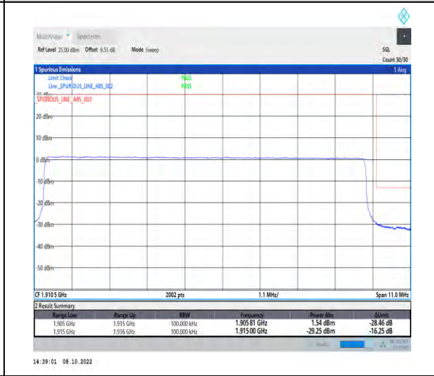
1-N25-PC3-15-10-H-6-CP-QPSK-Outer_Full-52@0-Ant1-1-seegraph-PASS-see graph
