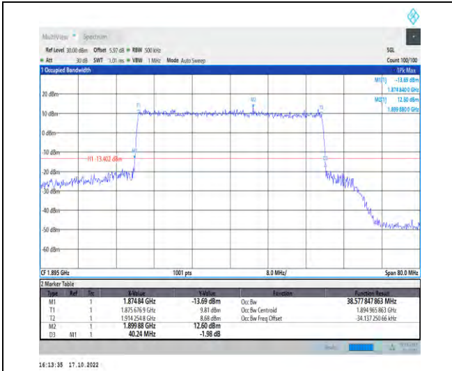
1-N25-PC3-15-40-H-6-CP-QPSK-Outer_Full-216@0 -Ant1-38.578-40.240-≤40-PASS
