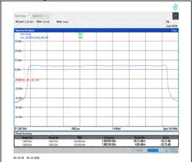
1-N25-PC3-15-15-L-3-DFT-QPSK-Outer_Full-75@0-Ant1-1-seegraph-PASS-see graph
