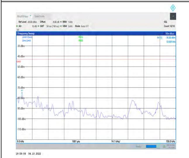
1-N25-PC3-15-40-M-1-DFT-QPSK-Inner_1RB_Left-1 @1-0.009-0.15-Ant1-0.01--76.36--43-PASS
