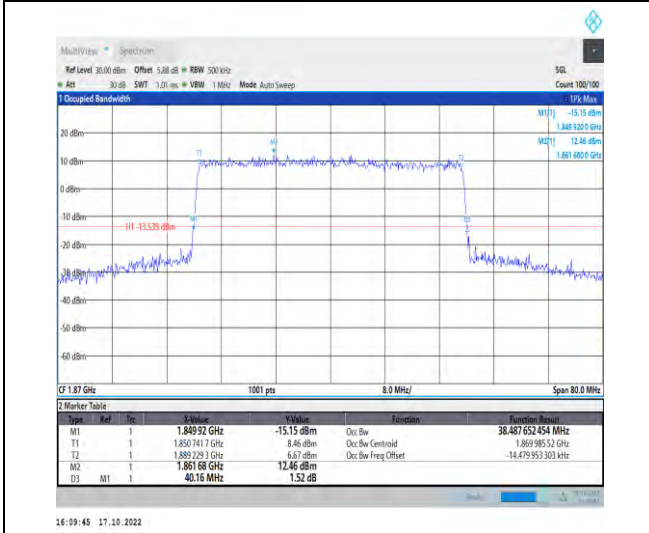
1-N25-PC3-15-40-L-8-CP-64QAM-Outer_Full-216@0 0-Ant1-38.488-40.160-≤40-PASS
