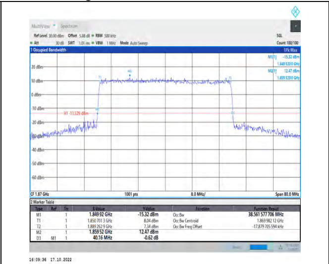
1-N25-PC3-15-40-L-7-CP-16QAM-Outer_Full-216@0 -Ant1-38.562-40.160-≤40-PASS
