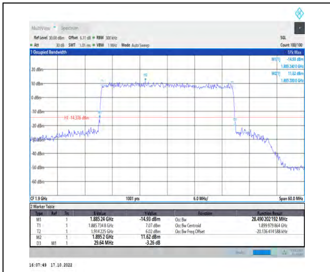
1-N25-PC3-15-30-H-6-CP-QPSK-Outer_Full-160@0 -Ant1-28.49-29.640-≤30-PASS
