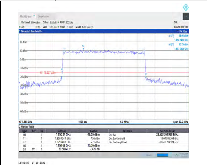
1-N25-PC3-15-30-L-7-CP-16QAM-Outer_Full-160@0 -Ant1-28.524-29.580-≤30-PASS
