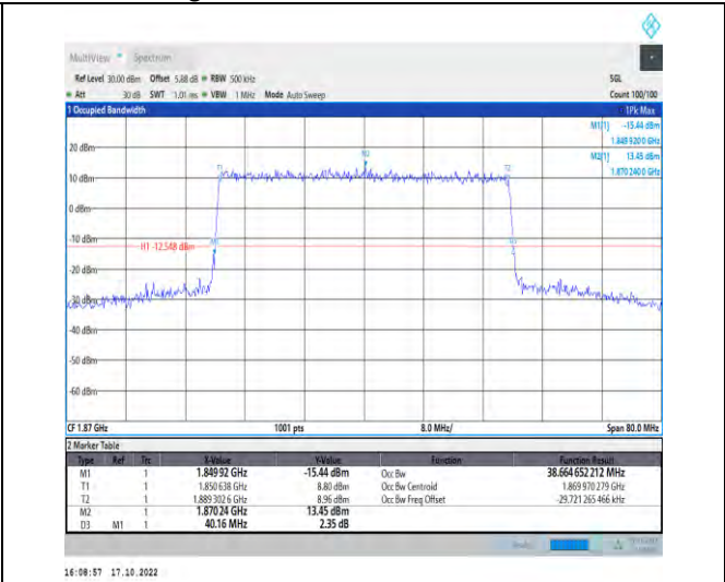
1-N25-PC3-15-40-L-3-DFT-16QAM-Outer_Full-216@ 0-Ant1-38.665-40.160-≤40-PASS
