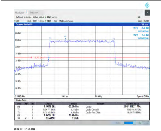
1-N25-PC3-15-30-L-8-CP-64QAM-Outer_Full-160@0 0-Ant1-28.491-29.640-≤30-PASS
