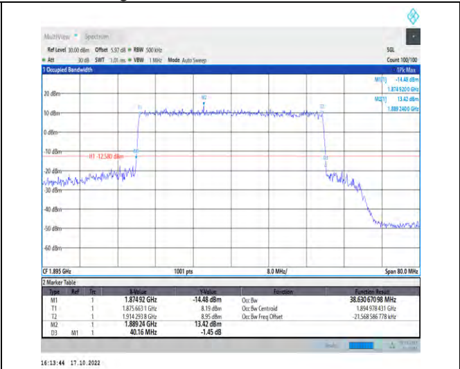
1-N25-PC3-15-40-H-7-CP-16QAM-Outer_Full-216@ 0-Ant1-38.631-40.160-≤40-PASS
