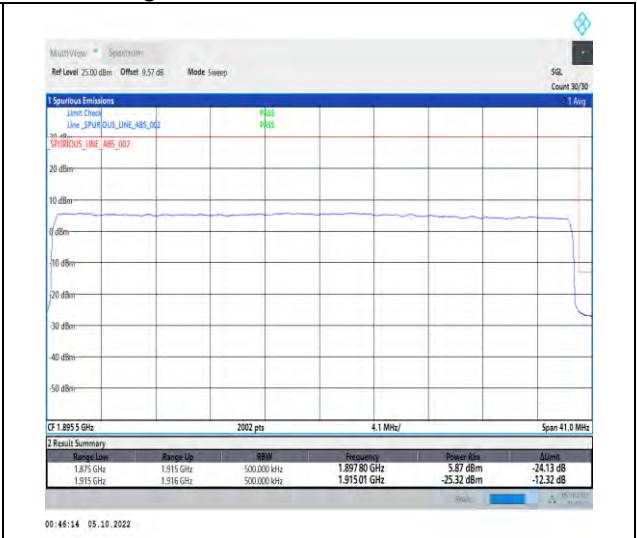
1-N25-PC3-15-40-H-3-DFT-QPSK-Outer_Full-216 @0-Ant1-1-seegraph-PASS-see graph
