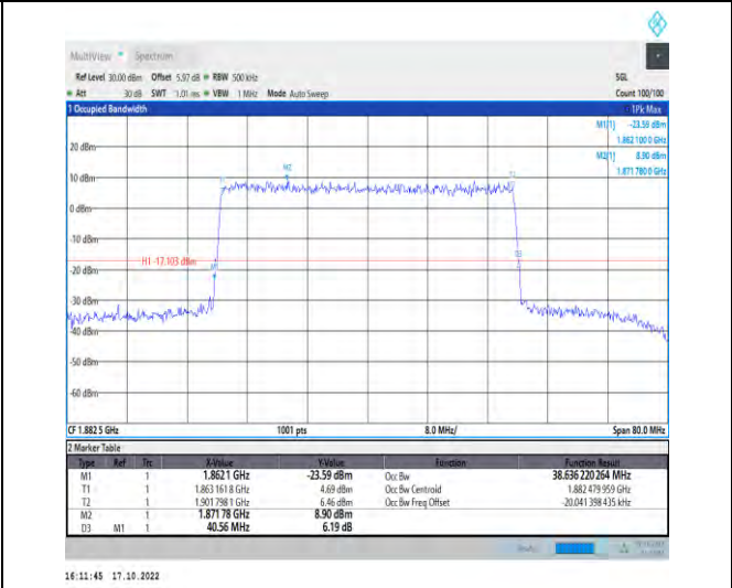
1-N25-PC3-15-40-M-9-CP-256QAM-Outer_Full-216 @0-Ant1-38.636-40.560-≤40-PASS
