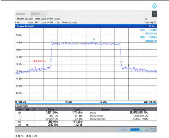
1-N25-PC3-15-30-L-6-CP-QPSK-Outer_Full-160@0 -Ant1-28.548-29.820-≤30-PASS
