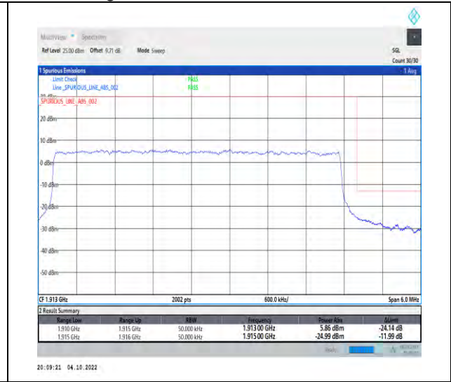
1-N25-PC3-15-5-H-3-DFT-QPSK-Outer_Full-25@0-Ant1-1-seegraph-PASS-see graph
