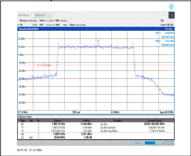
1-N25-PC3-15-30-H-3-DFT-16QAM-Outer_Full-160 @0-Ant1-28.601-29.640-≤30-PASS
