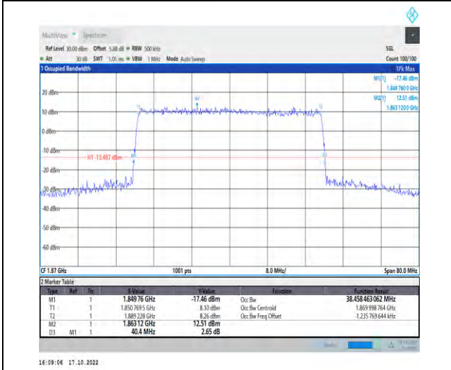
1-N25-PC3-15-40-L-4-DFT-64QAM-Outer_Full-216 @0-Ant1-38.458-40.400-≤40-PASS
