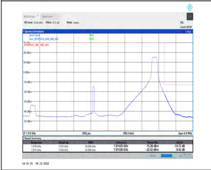
1-N25-PC3-15-5-H-5-CP-QPSK-Edge_1RB_Right-1@24-Ant1-1-seegraph-PASS-see graph
