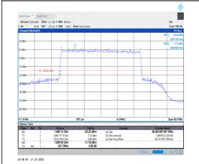
1-N25-PC3-15-30-H-8-CP-64QAM-Outer_Full-160@0 -Ant1-28.483-29.700-≤30-PASS
