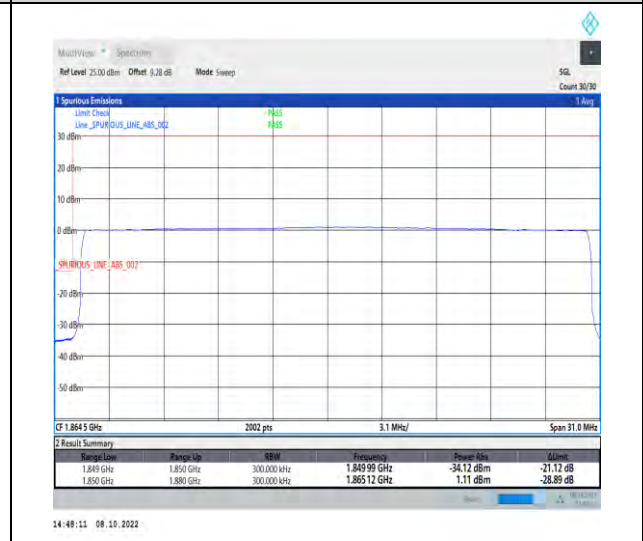
1-N25-PC3-15-30-L-6-CP-QPSK-Outer_Full-160@0-Ant1-1-seegraph-PASS-see graph
