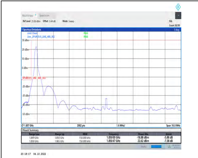
1-N25-PC3-15-15-L-1-DFT-QPSK-Edge_1RB_Left-1@0-Ant1-1-seegraph-PASS-see graph
