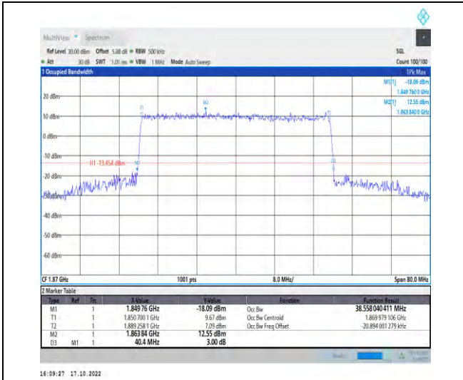
1-N25-PC3-15-40-L-6-CP-QPSK-Outer_Full-216@0 -Ant1-38.558-40.400-≤40-PASS
