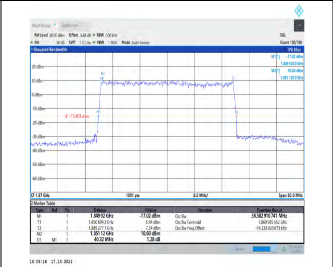
1-N25-PC3-15-40-L-5-DFT-256QAM-Outer_Full-216 @0-Ant1-38.583-40.320-≤40-PASS
