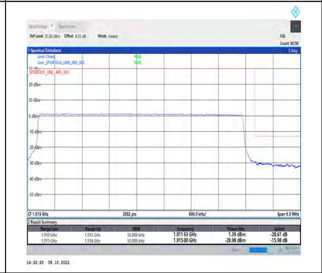
1-N25-PC3-15-5-H-6-CP-QPSK-Outer_Full-25@0-Ant1-1-seegraph-PASS-see graph
