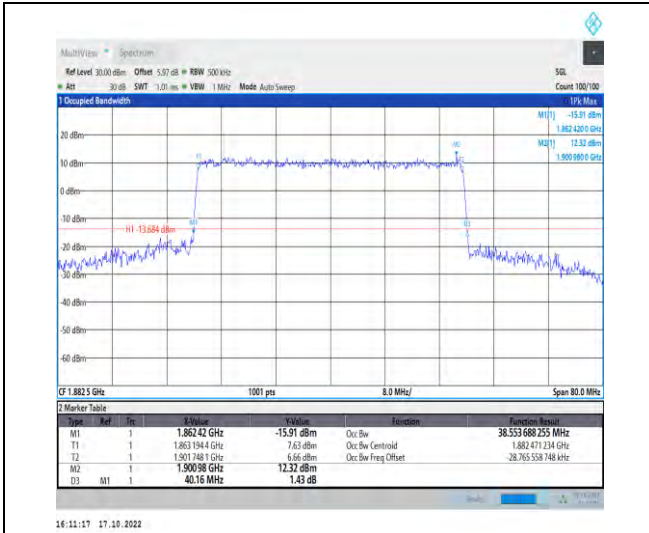
1-N25-PC3-15-40-M-6-CP-QPSK-Outer_Full-216@0 -Ant1-38.554-40.160-≤40-PASS
