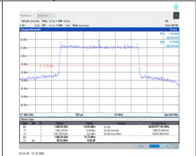
1-N25-PC3-15-40-M-3-DFT-16QAM-Outer_Full-216 @0-Ant1-38.656-40.320-≤40-PASS
