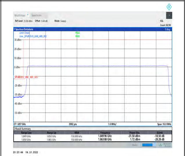
1-N25-PC3-15-15-L-6-CP-QPSK-Outer_Full-79@0-Ant1-1-seegraph-PASS-see graph
