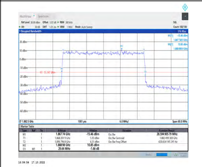
1-N25-PC3-15-30-M-5-DFT-256QAM-Outer_Full-160 @0-Ant1-28.595-29.640-≤30-PASS
