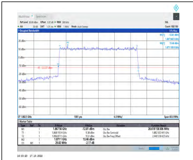
1-N25-PC3-15-30-M-1-DFT-QPSK-Outer_Full-160@ 0-Ant1-28.618-29.820-≤30-PASS
