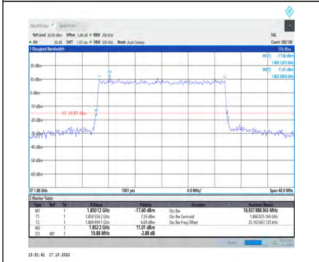
1-N25-PC3-15-20-L-8-CP-64QAM-Outer_Full-106@0 -Ant1-18.938-19.880-≤20-PASS
