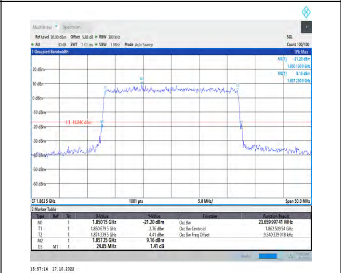
1-N25-PC3-15-25-L-9-CP-256QAM-Outer_Full-133@0 -Ant1-23.66-24.850-≤25-PASS
