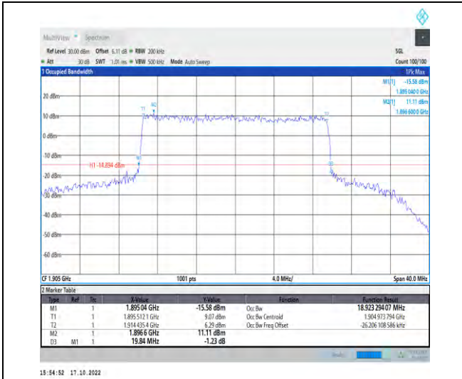
1-N25-PC3-15-20-H-6-CP-QPSK-Outer_Full-106@0 -Ant1-18.923-19.840-≤20-PASS
