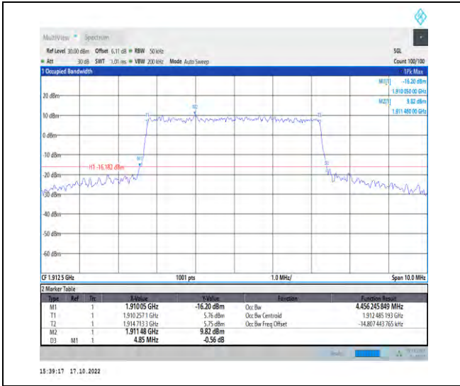
1-N25-PC3-15-5-H-6-CP-QPSK-Outer_Full-25@0-A nt1-4.456-4.850- \leq 5-PASS
