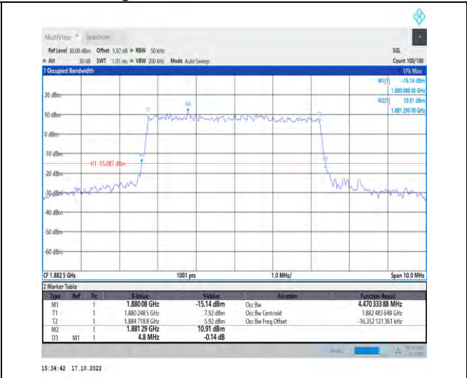
1-N25-PC3-15-5-M-7-CP-16QAM-Outer_Full-25@0- Ant1-4.47-4.800-≤5-PASS
