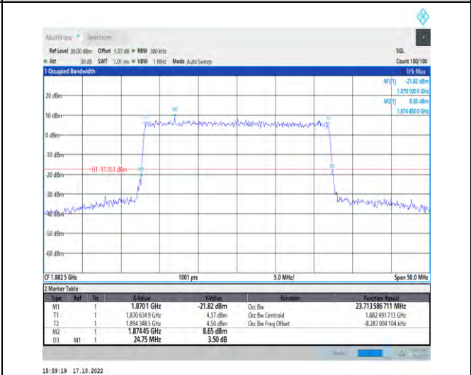
1-N25-PC3-15-25-M-9-CP-256QAM-Outer_Full-133 @0-Ant1-23.714-24.750-≤25-PASS
