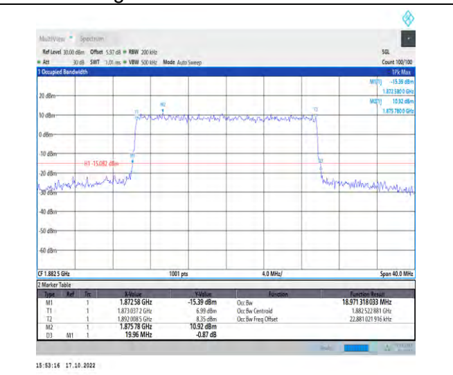
1-N25-PC3-15-20-M-7-CP-16QAM-Outer_Full-106@0 -Ant1-18.971-19.960-≤20-PASS
