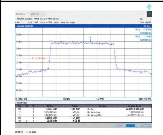
1-N25-PC3-15-25-M-5-DFT-256QAM-Outer_Full-128 @0-Ant1-22.883-23.950-≤25-PASS
