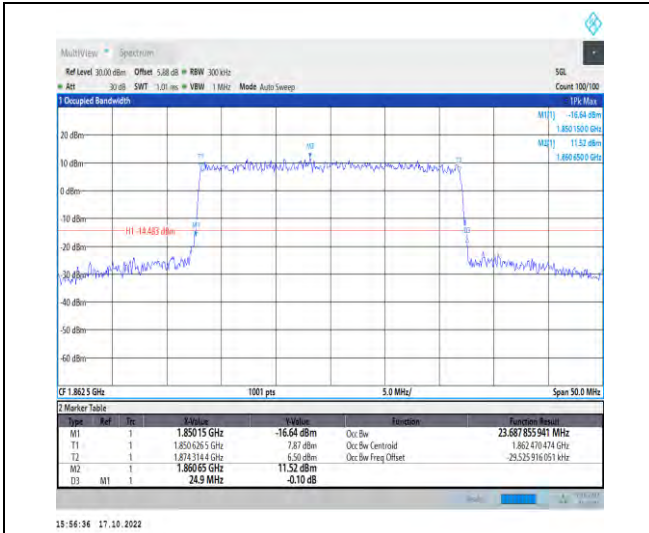
1-N25-PC3-15-25-L-6-CP-QPSK-Outer_Full-133@0 -Ant1-23.688-24.900-≤25-PASS
