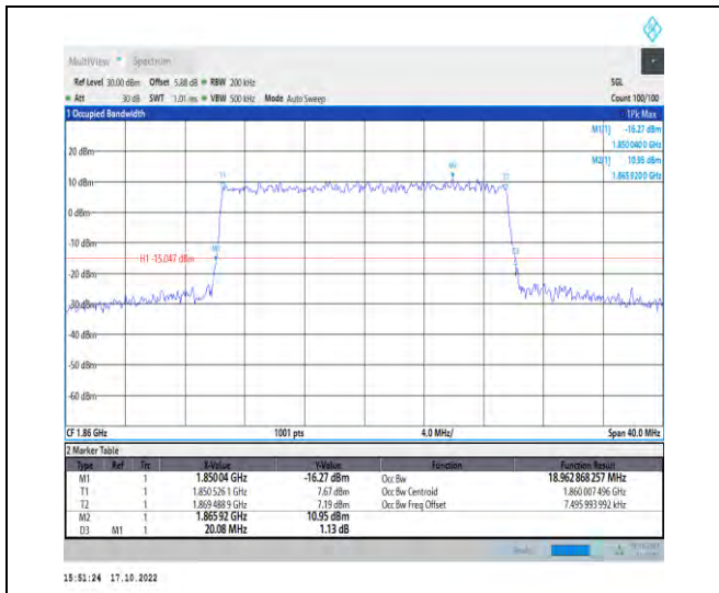
1-N25-PC3-15-20-L-6-CP-QPSK-Outer_Full-106@0 -Ant1-18.963-20.080-≤20-PASS
