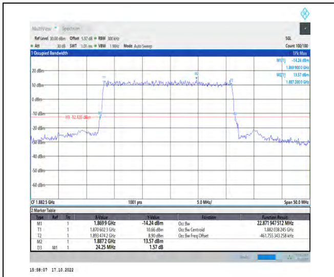
1-N25-PC3-15-25-M-1-DFT-QPSK-Outer_Full-128@ 0-Ant1-22.872-24.250-≤25-PASS
