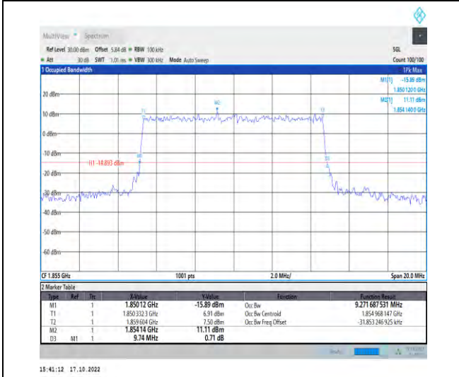
1-N25-PC3-15-10-L-8-CP-64QAM-Outer_Full-52@0-Ant1-9.272-9.740-≤10-PASS
