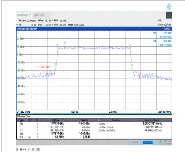
1-N25-PC3-15-10-M-6-CP-QPSK-Outer_Full-52@0-Ant1-9.285-9.800-≤10-PASS
