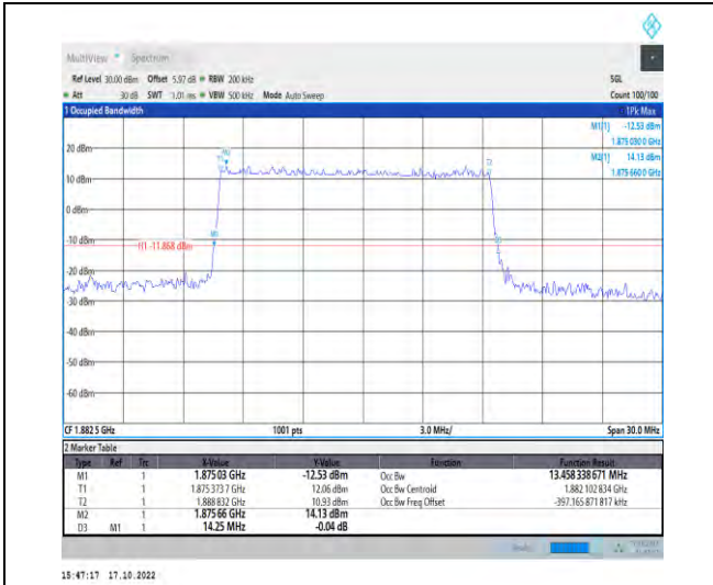
1-N25-PC3-15-15-M-1-DFT-QPSK-Outer_Full-75@0 -Ant1-13.458-14.250-≤15-PASS
