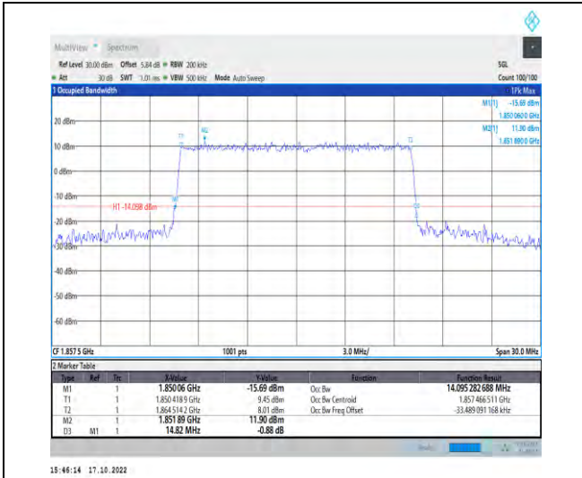
1-N25-PC3-15-15-L-6-CP-QPSK-Outer_Full-79@0-Ant1-14.095-14.820-≤15-PASS
