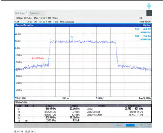
1-N25-PC3-15-25-M-8-CP-64QAM-Outer_Full-133 @0-Ant1-23.735-25.050-≤25-PASS
