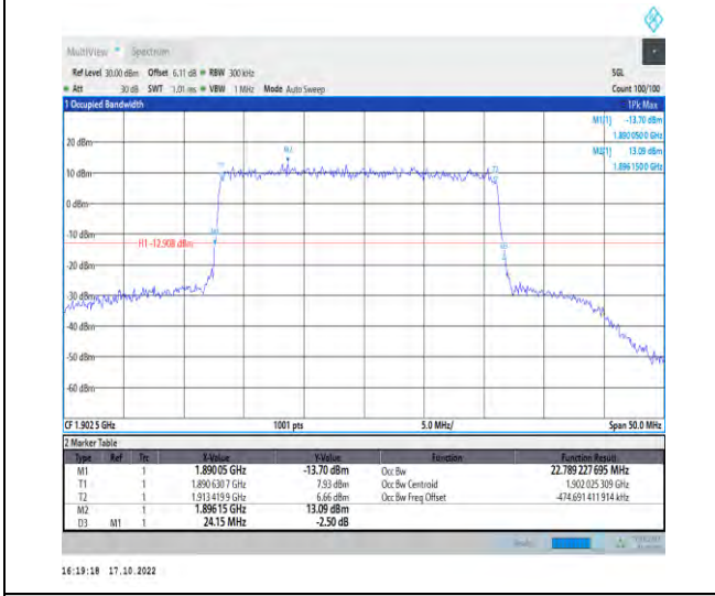
1-N25-PC3-15-25-H-4-DFT-64QAM-Outer_Full-128 @0-Ant1-22.789-24.150-≤25-PASS
