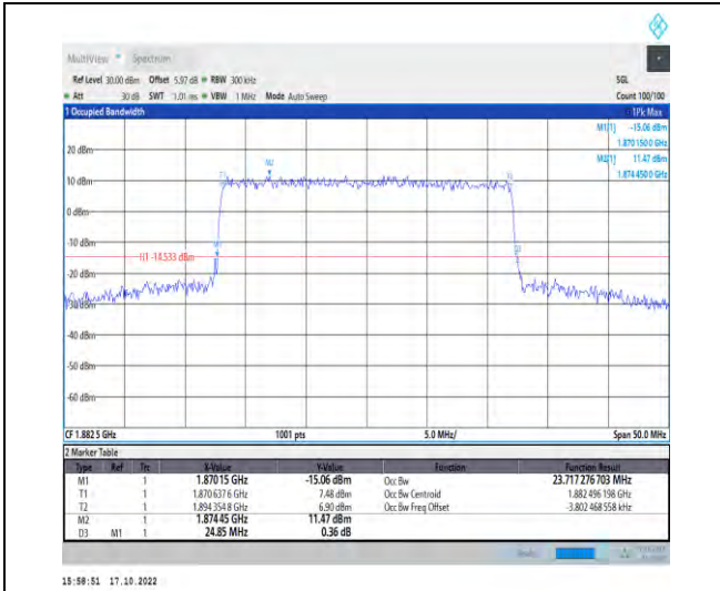
1-N25-PC3-15-25-M-6-CP-QPSK-Outer_Full-133@0 -Ant1-23.717-24.850-≤25-PASS
