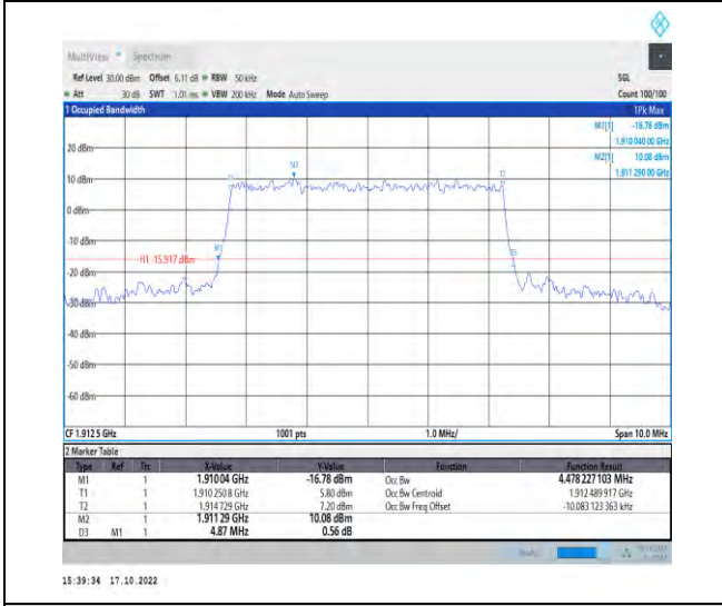
1-N25-PC3-15-5-H-8-CP-64QAM-Outer_Full-25@0-A Ant1-4.478-4.870- \leq 5-PASS
