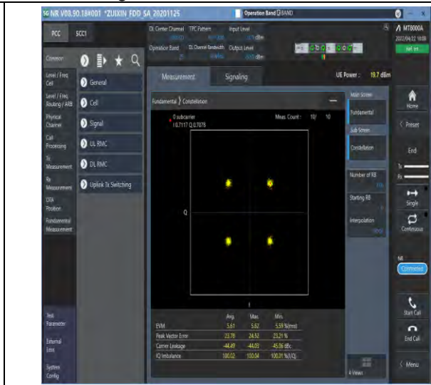
1-N25--15-40-M-6-CP-QPSK-Outer_Full-216@0-Ant1-see graph-PASS
