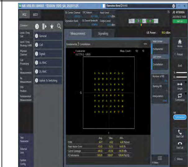
1-N25--15-40-M-8-CP-64QAM-Outer_Full-216@0-Ant1-see graph-PASS
