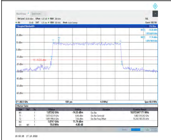
1-N25-PC3-15-20-M-8-CP-64QAM-Outer_Full-106 @0-Ant1-18.973-19.800-≤20-PASS
