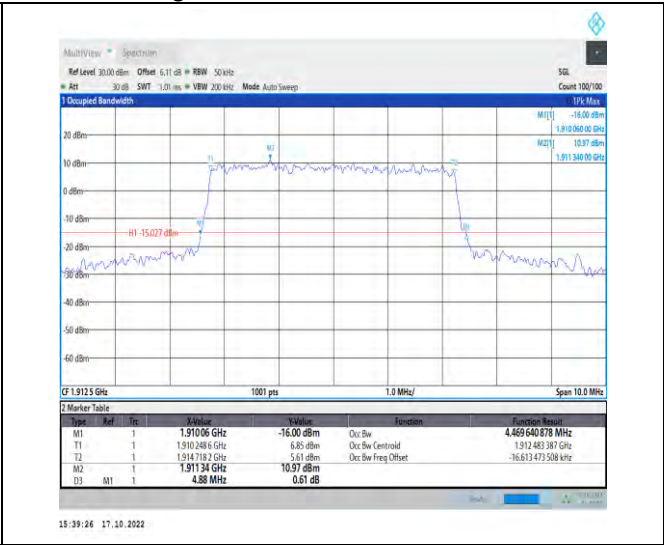
1-N25-PC3-15-5-H-7-CP-16QAM-Outer_Full-25@0-A Ant1-4.47-4.880- \leq 5-PASS
