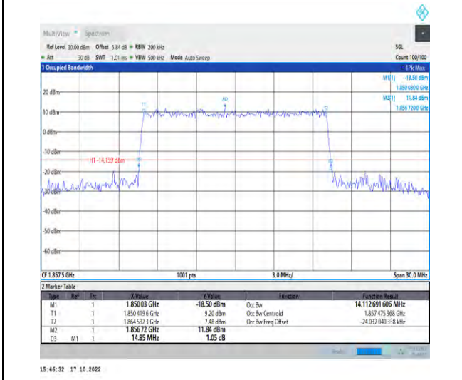
1-N25-PC3-15-15-L-8-CP-64QAM-Outer_Full-79@0-Ant1-14.113-14.850-≤15-PASS
