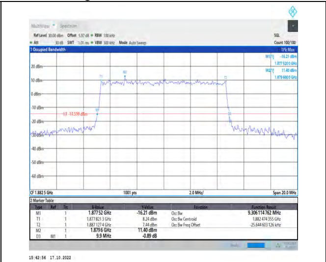
1-N25-PC3-15-10-M-7-CP-16QAM-Outer_Full-52@0-Ant1-9.306-9.900-≤10-PASS
