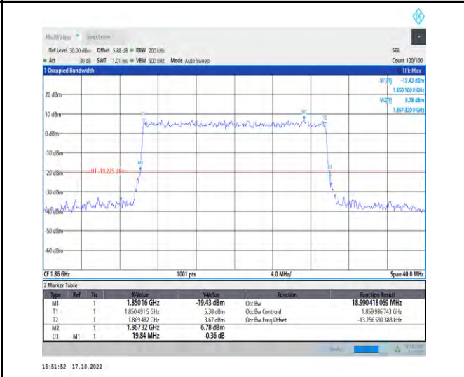
1-N25-PC3-15-20-L-9-CP-256QAM-Outer_Full-106@0 -Ant1-18.99-19.840-≤20-PASS
