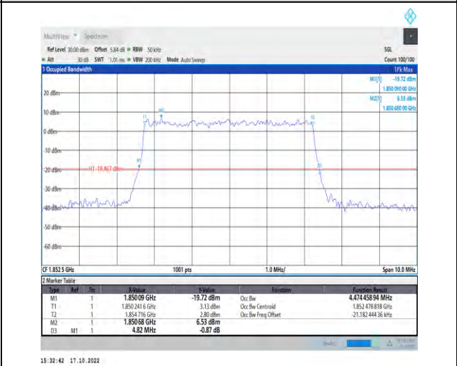
1-N25-PC3-15-5-L-9-CP-256QAM-Outer_Full-25@0-A Ant1-4.474-4.820-≤5-PASS
