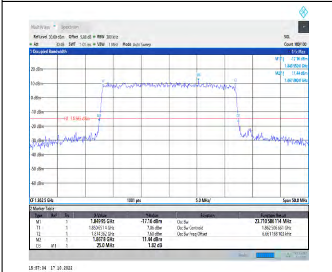
1-N25-PC3-15-25-L-8-CP-64QAM-Outer_Full-133@0 -Ant1-23.711-25.000-≤25-PASS
