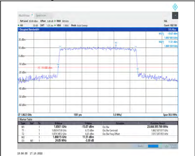
1-N25-PC3-15-25-L-7-CP-16QAM-Outer_Full-133@0 -Ant1-23.666-24.850-≤25-PASS
