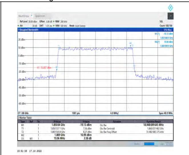
1-N25-PC3-15-20-L-7-CP-16QAM-Outer_Full-106@0 -Ant1-18.949-19.960-≤20-PASS
