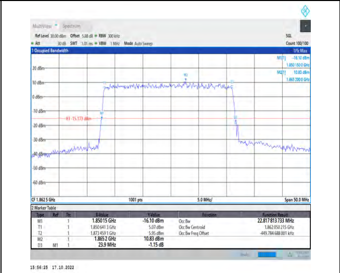
1-N25-PC3-15-25-L-5-DFT-256QAM-Outer_Full-128 @0-Ant1-22.818-23.900-≤25-PASS
