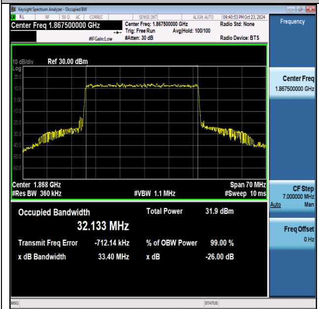
NTNV-n25-PC3-15-35-L-DFT-QPSK-Outer_Full-Ant1-PASS
