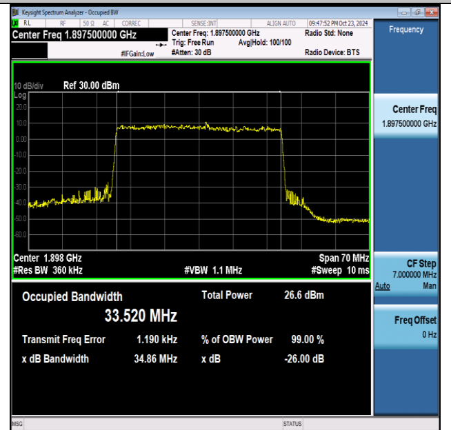
NTNV-n25-PC3-15-35-H-CP-256QAM-Outer_Full-Ant1-PASS
