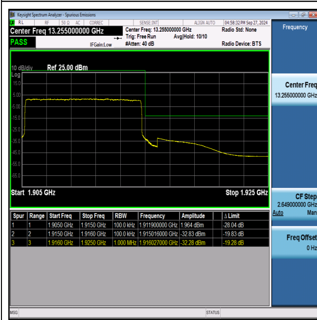
NTNV_N25_PC3_15_10_H_TID16_#1
