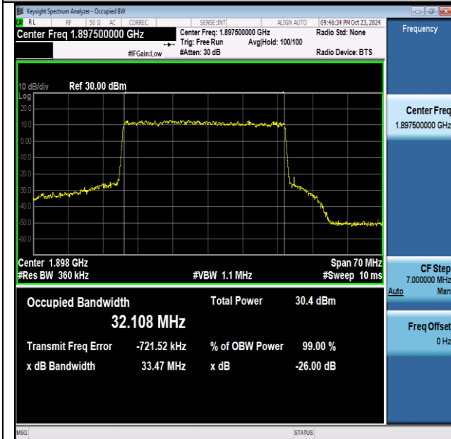
NTNV-n25-PC3-15-35-H-DFT-64QAM-Outer_Full-Ant1- PASS
