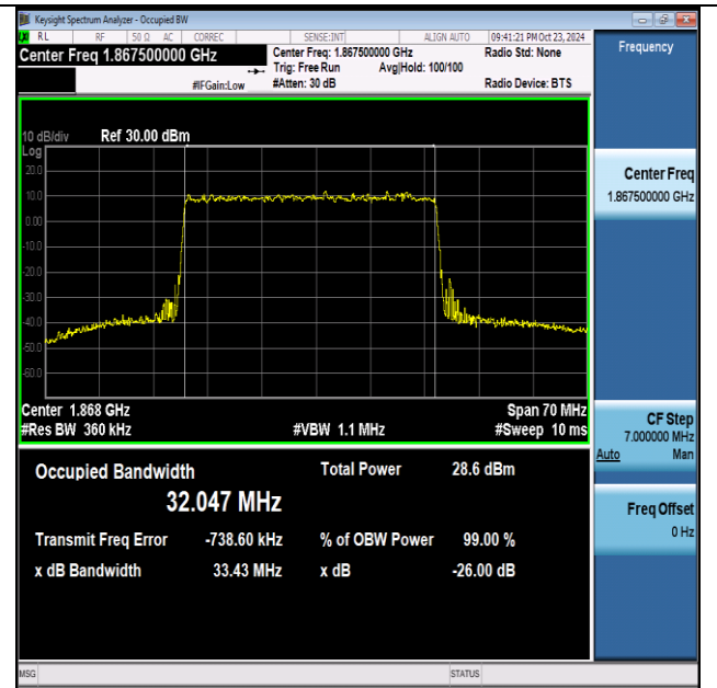
NTNV-n25-PC3-15-35-L-DFT-256QAM-Outer_Full-Ant1- PASS
