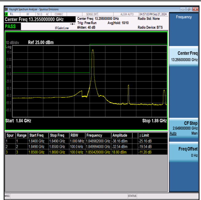
NTNV_N25_PC3_15_10_L_TID17_#1
