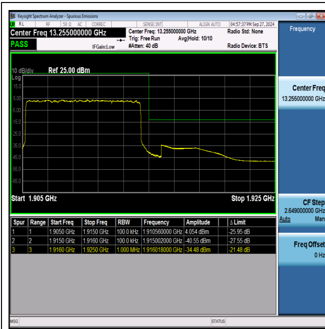
NTNV_N25_PC3_15_10_H_TID1_#1
