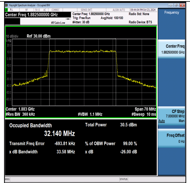
NTNV-n25-PC3-15-35-M-DFT-64QAM-Outer_Full-Ant1- PASS
