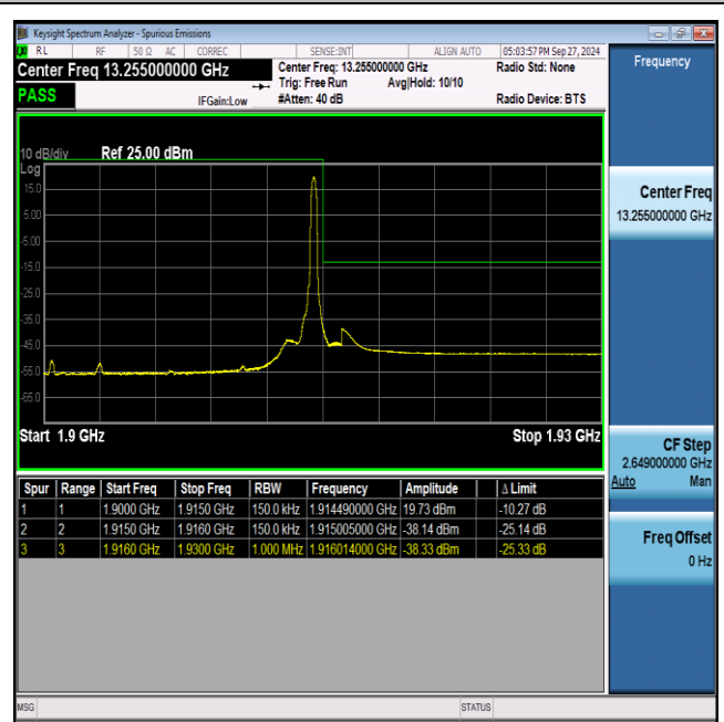
NTNV_N25_PC3_15_15_H_TID18_#1
