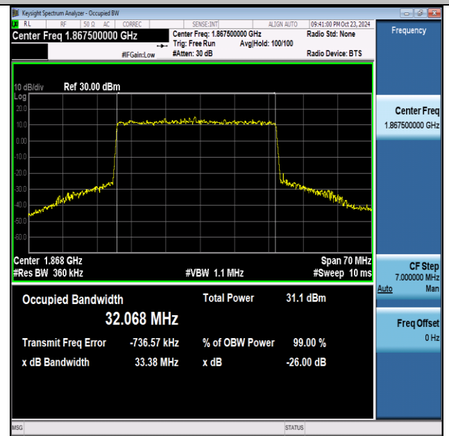
NTNV-n25-PC3-15-35-L-DFT-16QAM-Outer_Full-Ant1-PASS
