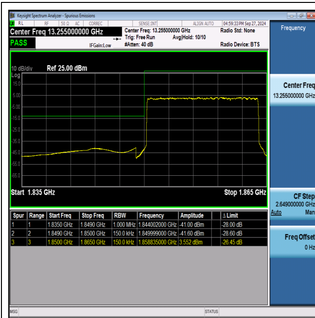
NTNV_N25_PC3_15_15_L_TID1_#1
