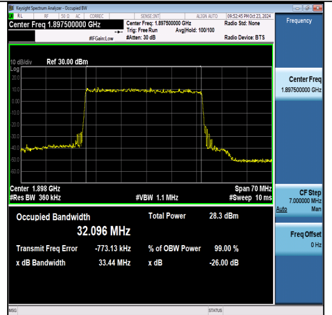
NTNV-n25-PC3-15-35-H-DFT-256QAM-Outer_Full-Ant1- PASS
