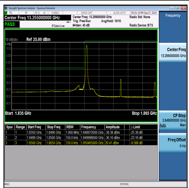
NTNV_N25_PC3_15_15_L_TID17_#1
