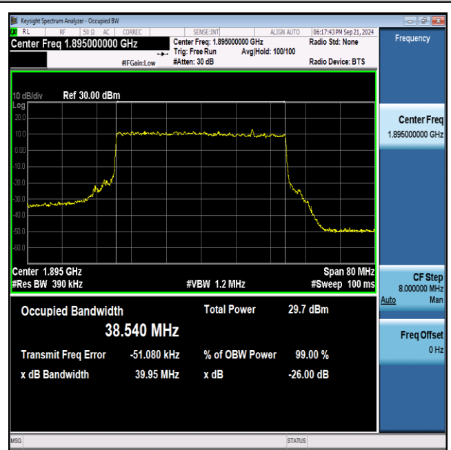
NTNV_N25_PC3_15_40_H_TID8_Ant1#1
