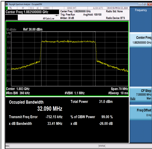
NTNV-n25-PC3-15-35-M-DFT-16QAM-Outer_Full-Ant1- PASS
