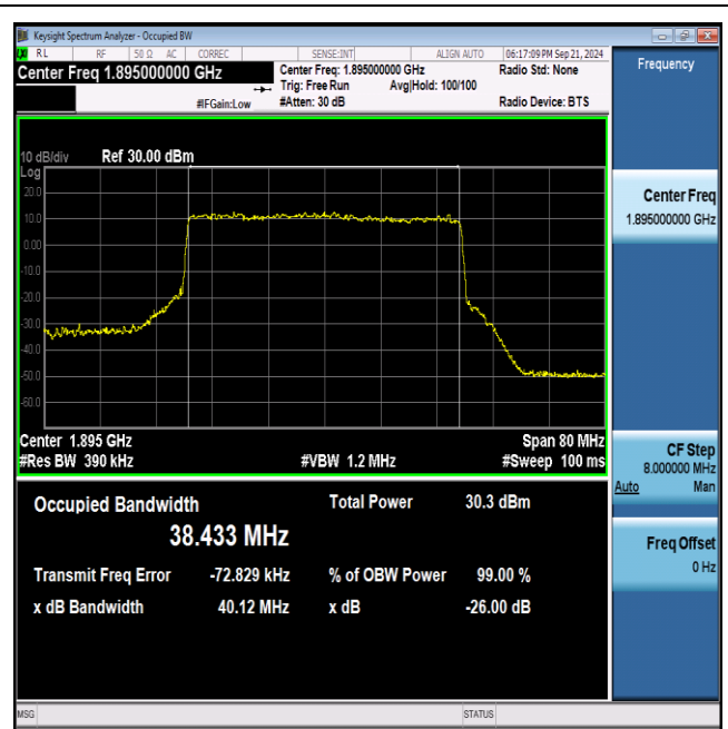
NTNV_N25_PC3_15_40_H_TID6_Ant1#1
