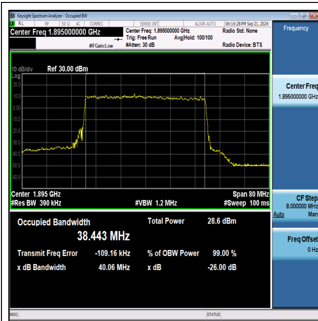
NTNV_N25_PC3_15_40_H_TID5_Ant1#1
