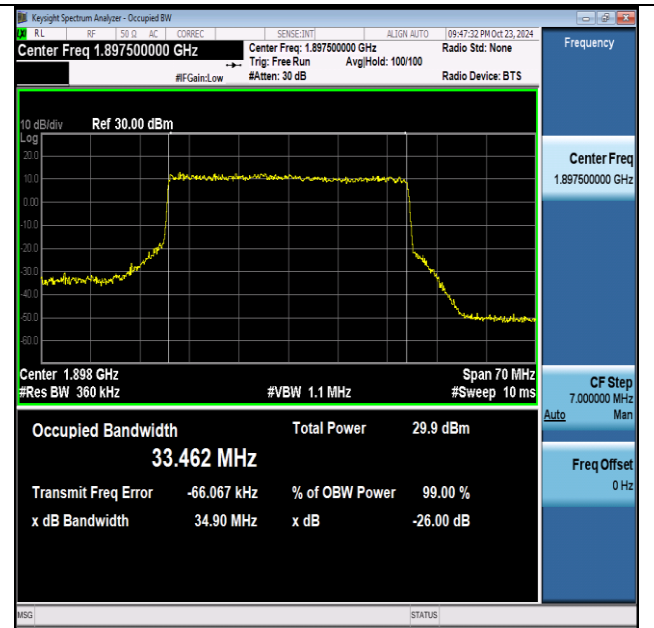
NTNV-n25-PC3-15-35-H-CP-16QAM-Outer_Full-Ant1-PASS
