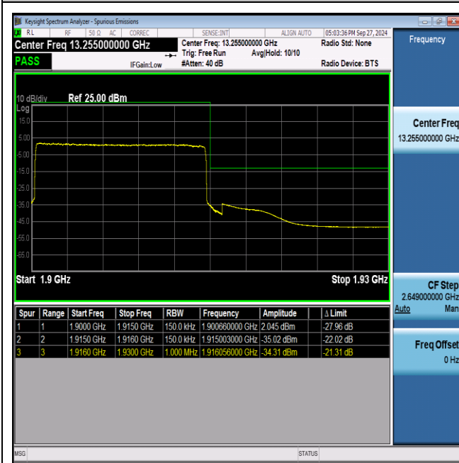
NTNV_N25_PC3_15_15_H_TID16_#1
