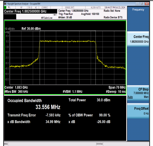
NTNV-n25-PC3-15-35-M-DFT-64QAM-Outer_Full-Ant1- PASS
