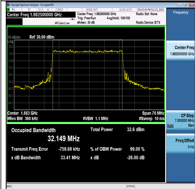
NTNV-n25-PC3-15-35-M-DFT-BPSK-Outer_Full-Ant1- PASS
