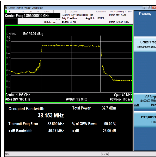
NTVN_N25_PC3_15_40_H_TID1_Ant1#1
