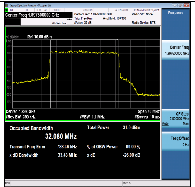
NTNV-n25-PC3-15-35-H-DFT-16QAM-Outer_Full-Ant1- PASS
