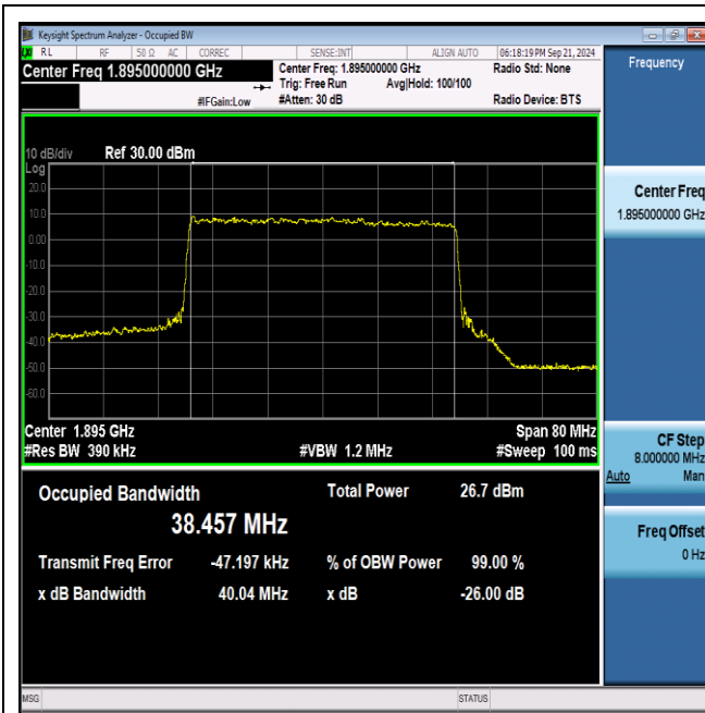
NTNV_N25_PC3_15_40_H_TID9_Ant1#1
