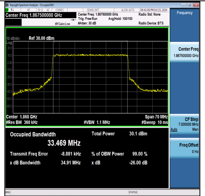
NTNV-n25-PC3-15-35-L-CP-16QAM-Outer_Full-Ant1- PASS
