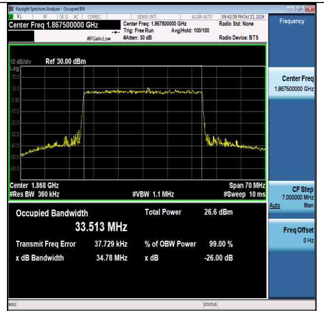
NTNV-n25-PC3-15-35-L-CP-256QAM-Outer_Full-Ant1- PASS
