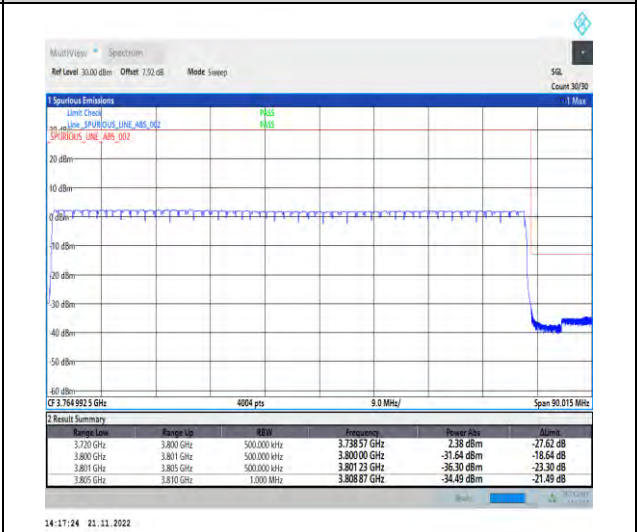
1-N78-3700-3800-PC2-30-80-H-6-CP-QPSK-Outer _Full-217@0-Ant1-1--PASS-see graph
