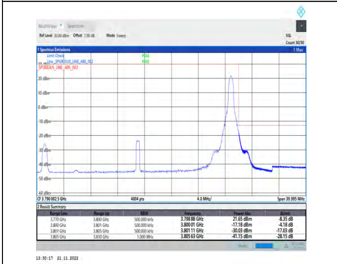
1-N78-3700-3800-PC2-30-30-H-5-CP-QPSK-Edge_1R_B_Right-1@77-Ant1-1--PASS-see graph
