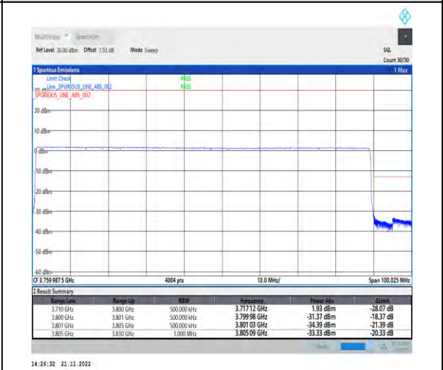
1-N78-3700-3800-PC2-30-90-H-6-CP-QPSK-Outer _Full-245@0-Ant1-1--PASS-see graph
