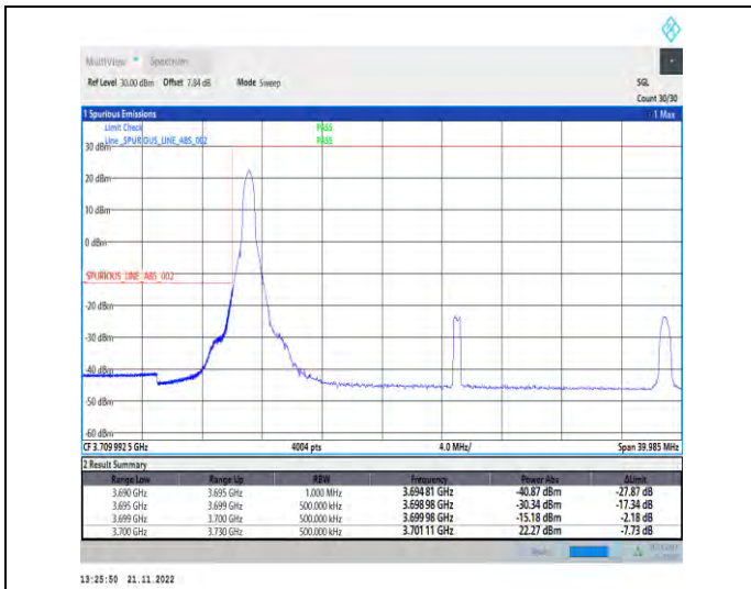
1-N78-3700-3800-PC2-30-30-L-4-CP-QPSK-Edge_1R_B_Left-1@0-Ant1-1--PASS-see graph
