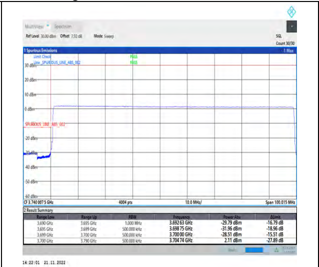
1-N78-3700-3800-PC2-30-90-L-6-CP-QPSK-Outer _Full-245@0-Ant1-1--PASS-see graph
