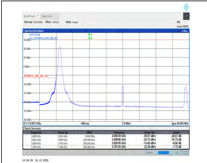
1-N78-3700-3800-PC2-30-40-L-4-CP-QPSK-Edge_1R B_Left-1@0-Ant1-1--PASS-see graph
