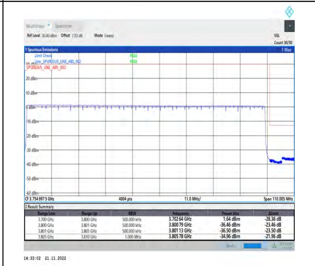
1-N78-3700-3800-PC2-30-100-H-6-CP-QPSK-Out er_Full-273@0-Ant1-1--PASS-see graph
