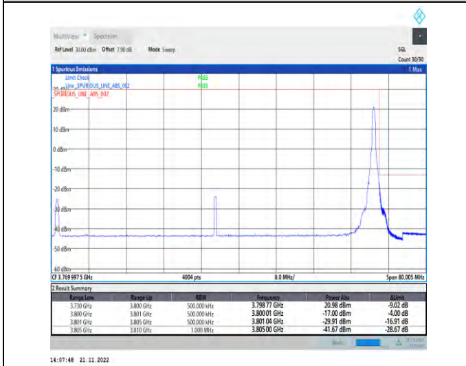
1-N78-3700-3800-PC2-30-70-H-5-CP-QPSK-Edge_1R B_Right-1@188-Ant1-1--PASS-see graph
