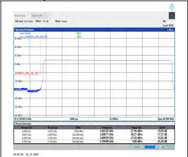
1-N78-3700-3800-PC2-30-50-L-6-CP-QPSK-Outer _Full-133@0-Ant1-1--PASS-see graph
