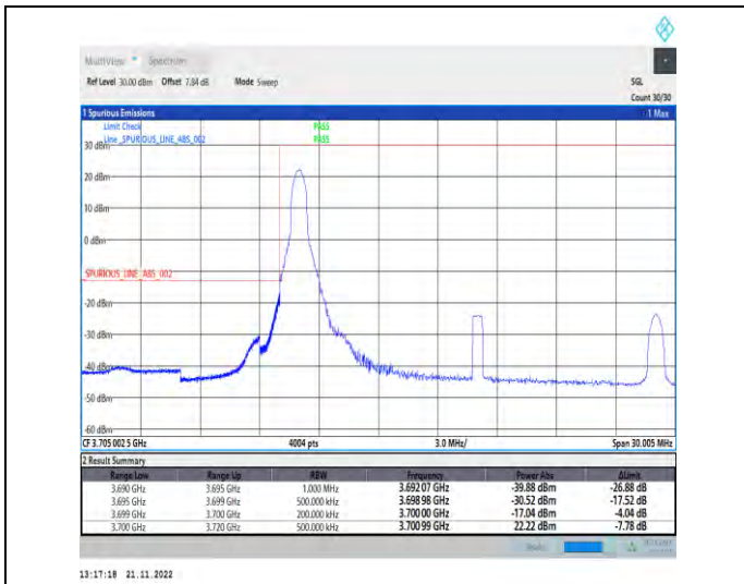
1-N78-3700-3800-PC2-30-20-L-4-CP-QPSK-Edge_1R_B_Left-1@0-Ant1-1--PASS-see graph
