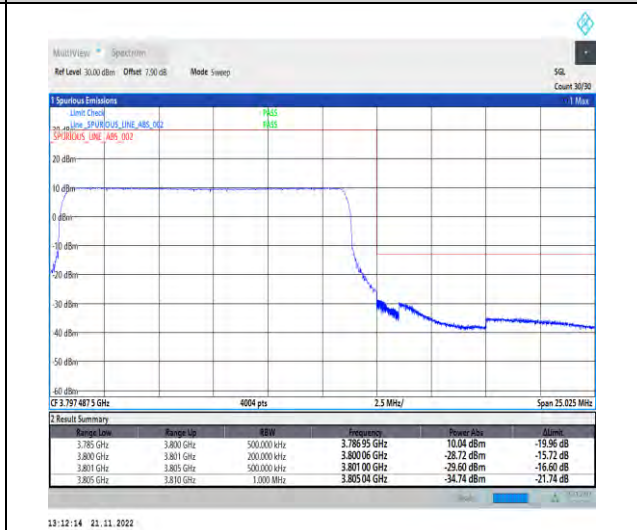
1-N78-3700-3800-PC2-30-15-H-6-CP-QPSK-Outer_Full-38@0-Ant1-1--PASS-see graph
