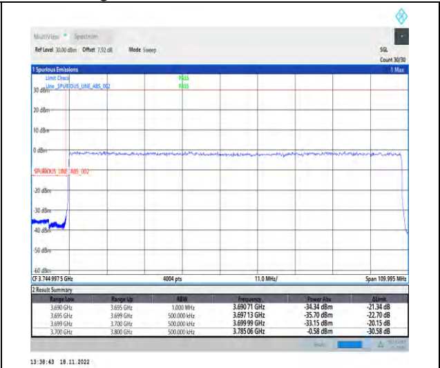
1-N78-3700-3800-PC2-30-100-L-3-DFT-PI2BPSK-Outer_Full-270@0-Ant1-1--PASS-see graph
