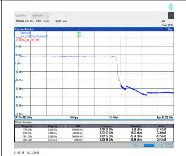
1-N78-3700-3800-PC2-30-20-H-6-CP-QPSK-Outer_Full-51@0-Ant1-1--PASS-see graph
