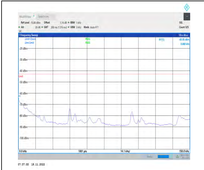
1-N78-3700-3800-PC2-30-100-H-1-DFT-PI2BPSK- Inner_1RB_Left-1@1-0.009-0.15-Ant1-0.01--65.95-- 43-PASS
