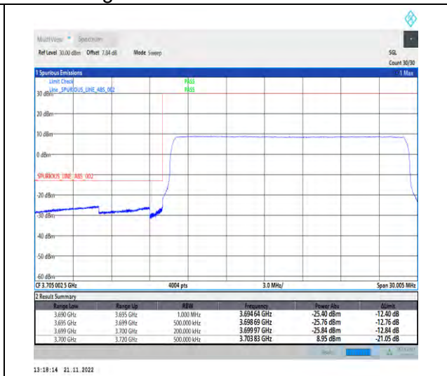
1-N78-3700-3800-PC2-30-20-L-6-CP-QPSK-Outer_Full-51@0-Ant1-1--PASS-see graph
