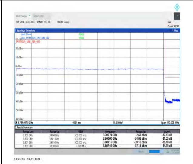
1-N78-3700-3800-PC2-30-100-H-6-CP-QPSK-Outer_Full-273@0-Ant1-1--PASS-see graph
