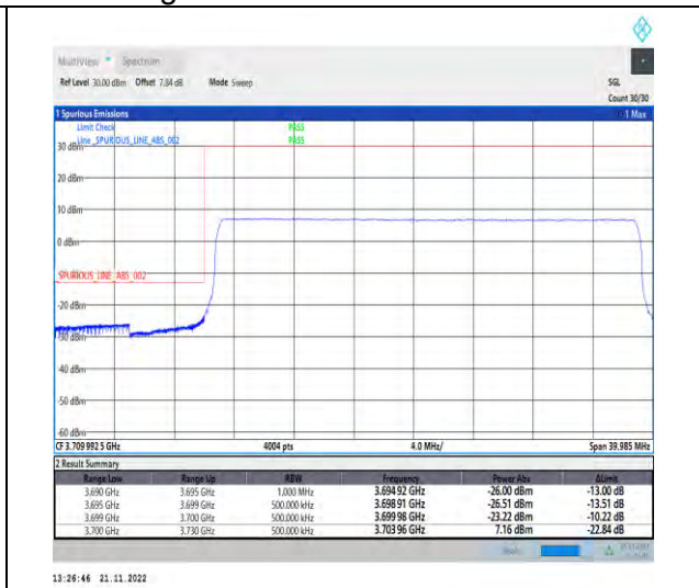
1-N78-3700-3800-PC2-30-30-L-6-CP-QPSK-Outer_Full-78@0-Ant1-1--PASS-see graph
