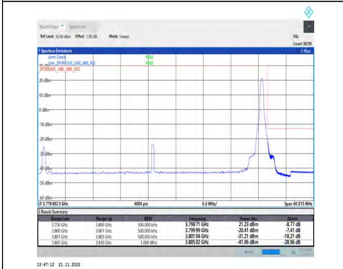
1-N78-3700-3800-PC2-30-50-H-5-CP-QPSK-Edge_1R B_Right-1@132-Ant1-1--PASS-see graph
