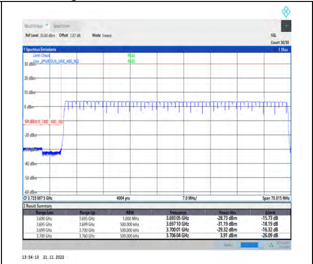
1-N78-3700-3800-PC2-30-60-L-6-CP-QPSK-Outer _Full-162@0-Ant1-1--PASS-see graph
