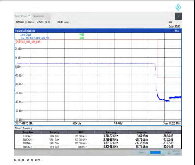
1-N78-3700-3800-PC2-30-60-H-6-CP-QPSK-Outer _Full-162@0-Ant1-1--PASS-see graph
