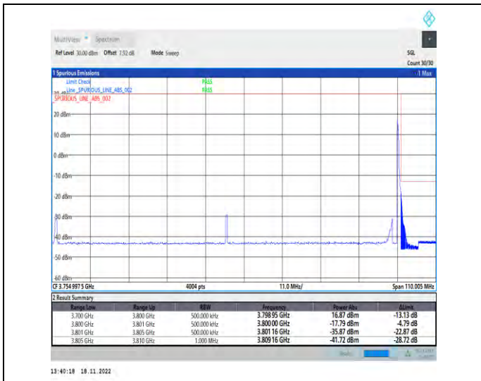
1-N78-3700-3800-PC2-30-100-H-2-DFT-PI2BPSK-Edge_1_RB_Right-1@272-Ant1-1--PASS-see graph
