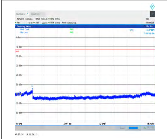
1-N78-3700-3800-PC2-30-100-M-1-DFT-PI2BPSK- Inner_1RB_Left-1@1-6000-18000-Ant1-7480.80--55. 37--13-PASS
