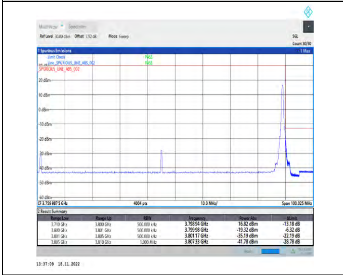
1-N78-3700-3800-PC2-30-90-H-5-CP-QPSK-Edge_1RB_Right-1@244-Ant1-1--PASS-see graph
