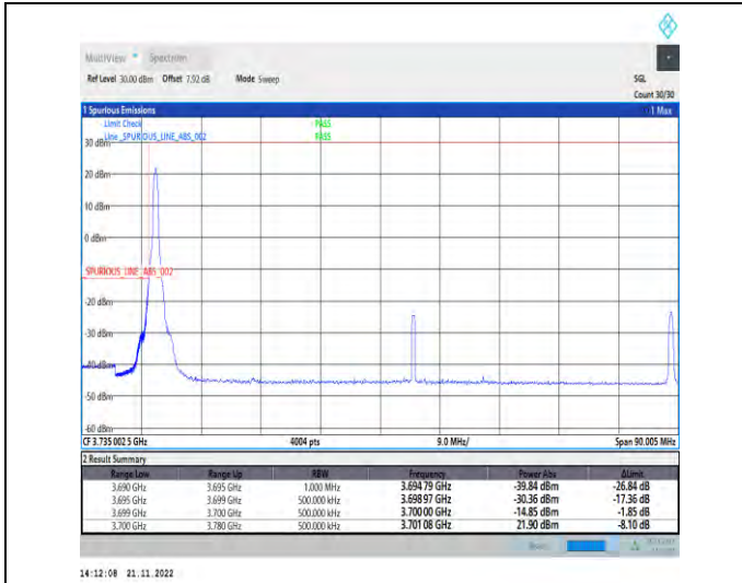
1-N78-3700-3800-PC2-30-80-L-4-CP-QPSK-Edge_1R B_Left-1@0-Ant1-1--PASS-see graph
