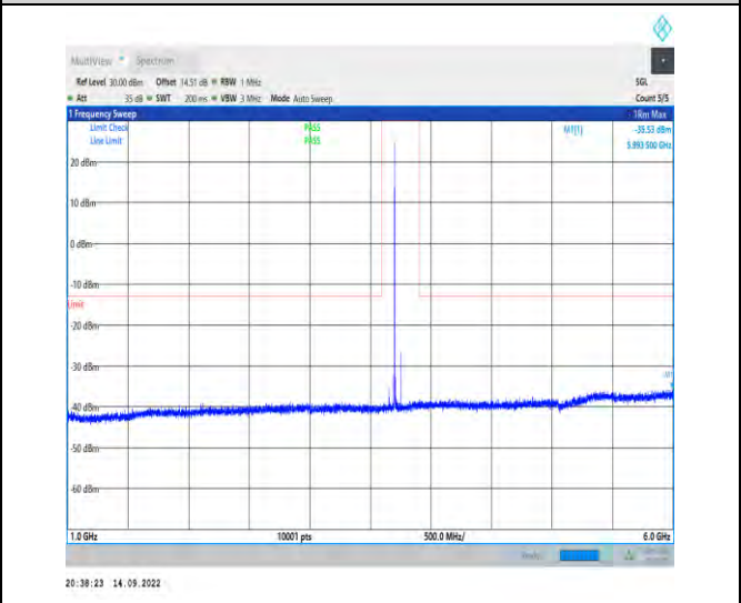
1-N78-3700-3800-PC2-30-100-H-1-DFT-QPSK-Edge _1RB_Left-1@0-1000-6000-Ant1-5928.50--47.44--13 -PASS
