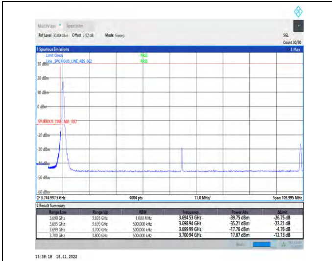
1-N78-3700-3800-PC2-30-100-L-1-DFT-PI2BPSK-Edge_1RB_Left-1@0-Ant1-1--PASS-see graph
