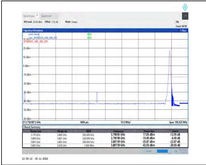
1-N78-3700-3800-PC2-30-90-H-2-DFT-PI2BPSK-Edge_1RB_Right-1@244-Ant1-1--PASS-see graph
