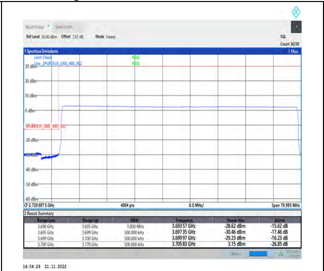
1-N78-3700-3800-PC2-30-70-L-6-CP-QPSK-Outer _Full-189@0-Ant1-1--PASS-see graph
