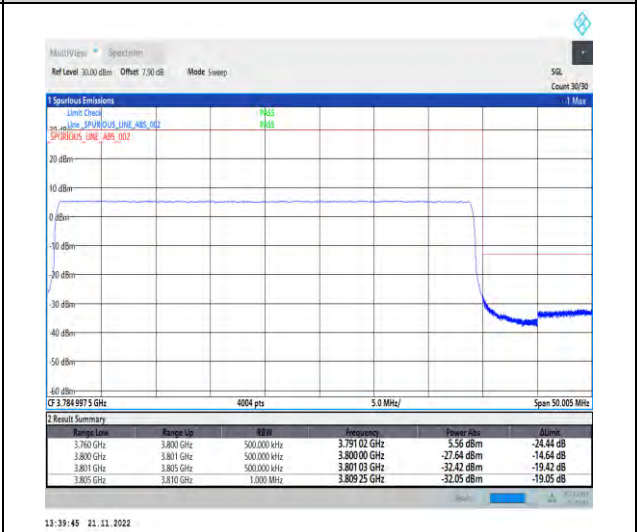
1-N78-3700-3800-PC2-30-40-H-6-CP-QPSK-Outer _Full-106@0-Ant1-1--PASS-see graph
