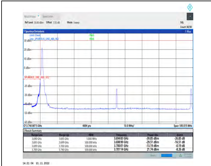
1-N78-3700-3800-PC2-30-90-L-4-CP-QPSK-Edge_1R B_Left-1@0-Ant1-1--PASS-see graph
