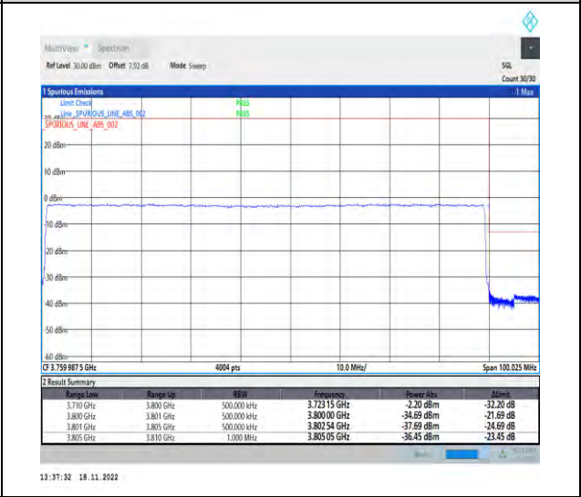
1-N78-3700-3800-PC2-30-90-H-6-CP-QPSK-Outer_Full-245@0-Ant1-1--PASS-see graph
