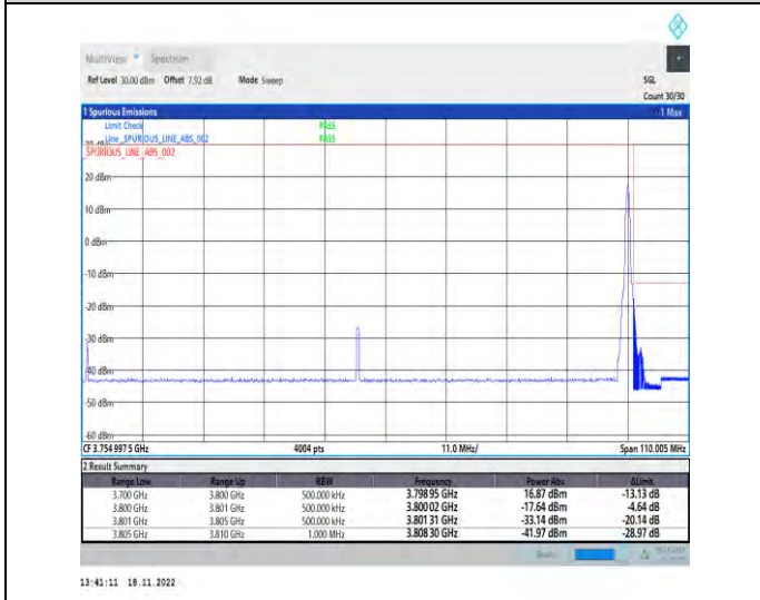
1-N78-3700-3800-PC2-30-100-H-5-CP-QPSK-Edge_1_RB_Right-1@272-Ant1-1--PASS-see graph
