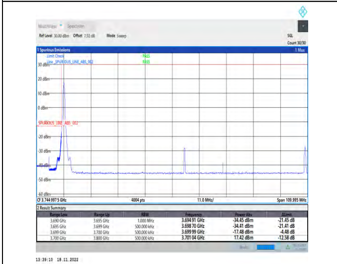
1-N78-3700-3800-PC2-30-100-L-4-CP-QPSK-Edge_1RB_Left-1@0-Ant1-1--PASS-see graph
