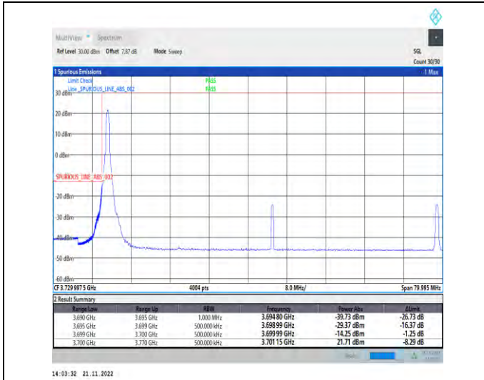
1-N78-3700-3800-PC2-30-70-L-4-CP-QPSK-Edge_1R B_Left-1@0-Ant1-1--PASS-see graph
