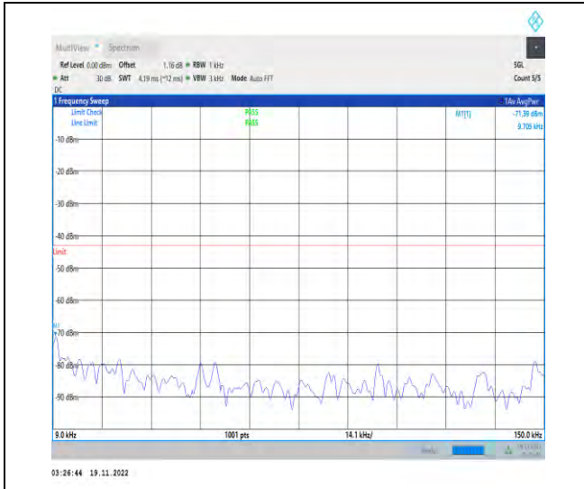
1-N78-3700-3800-PC2-30-100-H-1-DFT-QPSK-Edge e_1RB_Left-1@0-0.009-0.15-Ant1-0.01--71.39--43- PASS
