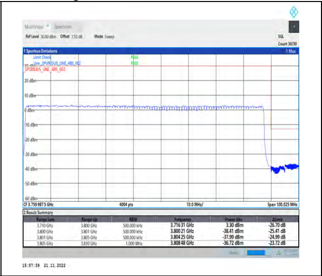
1-N78-3700-3800-PC2-30-90-H-3-DFT-PI2BPSK-Outer_Full-240@0-Ant1-1--PASS-see graph
