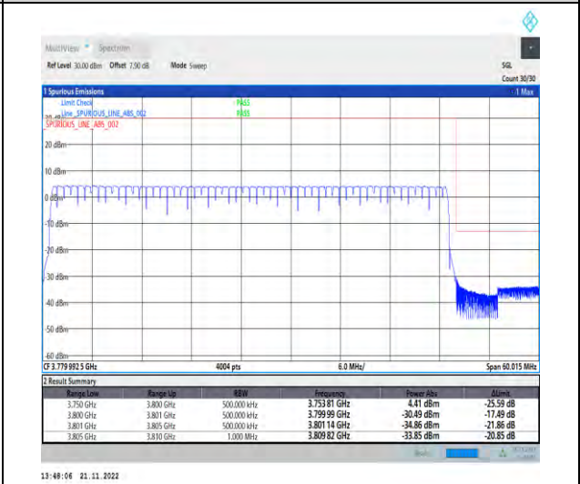
1-N78-3700-3800-PC2-30-50-H-6-CP-QPSK-Outer _Full-133@0-Ant1-1--PASS-see graph
