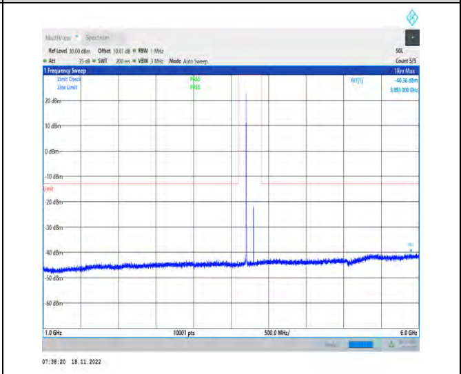
1-N78-3700-3800-PC2-30-100-H-1-DFT-PI2BPSK- Inner_1RB_Left-1@1-1000-6000-Ant1-5893.00--40.36- -13-PASS
