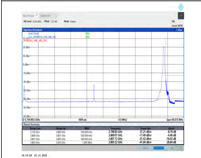
1-N78-3700-3800-PC2-30-80-H-5-CP-QPSK-Edge_1R B_Right-1@216-Ant1-1--PASS-see graph
