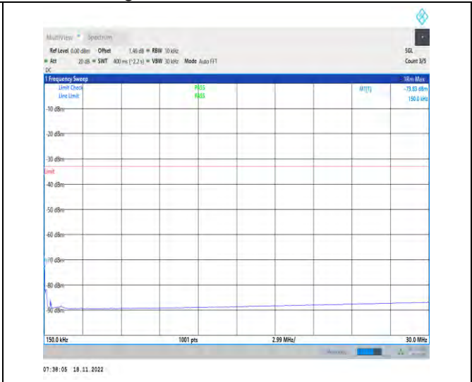
1-N78-3700-3800-PC2-30-100-H-1-DFT-PI2BPSK- Inner_1RB_Left-1@1-0.15-30-Ant1-0.15--73.83--33-PA SS
