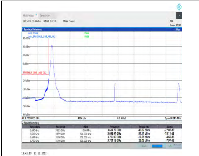
1-N78-3700-3800-PC2-30-50-L-4-CP-QPSK-Edge_1R B_Left-1@0-Ant1-1--PASS-see graph
