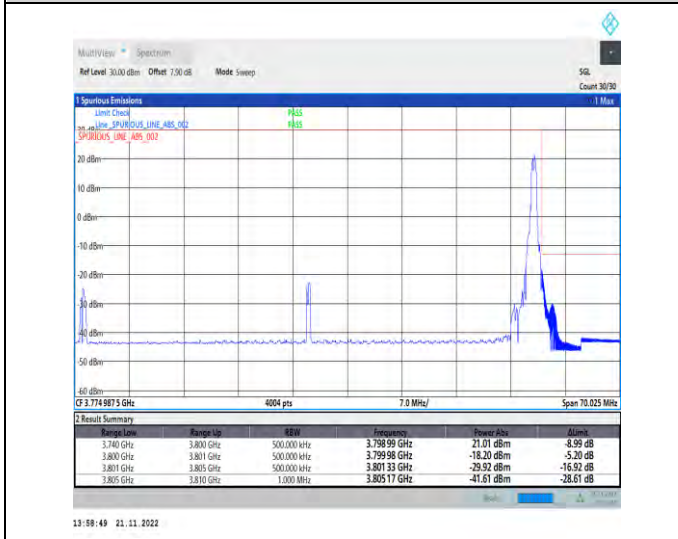
1-N78-3700-3800-PC2-30-60-H-5-CP-QPSK-Edge_1R B_Right-1@161-Ant1-1--PASS-see graph
