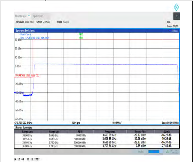
1-N78-3700-3800-PC2-30-80-L-6-CP-QPSK-Outer _Full-217@0-Ant1-1--PASS-see graph
