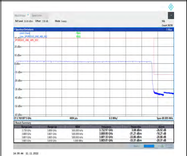
1-N78-3700-3800-PC2-30-70-H-6-CP-QPSK-Outer _Full-189@0-Ant1-1--PASS-see graph
