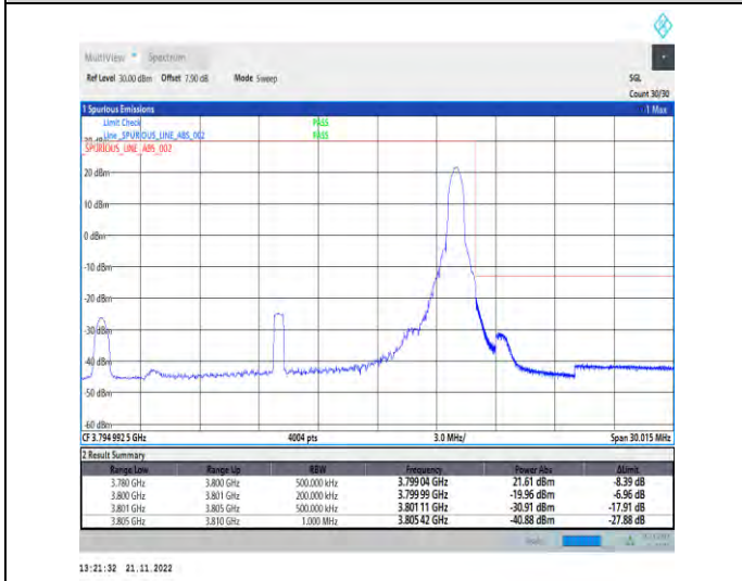
1-N78-3700-3800-PC2-30-20-H-5-CP-QPSK-Edge_1R_B_Right-1@50-Ant1-1--PASS-see graph
