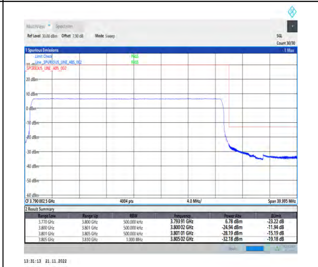
1-N78-3700-3800-PC2-30-30-H-6-CP-QPSK-Outer_Full-78@0-Ant1-1--PASS-see graph
