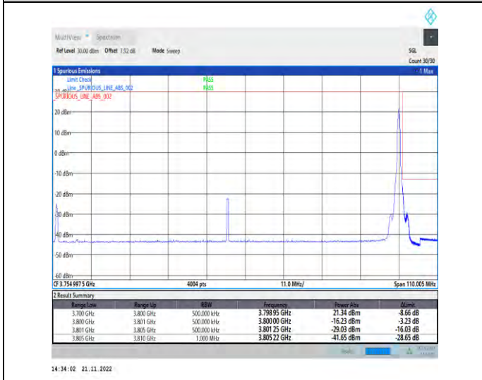
1-N78-3700-3800-PC2-30-100-H-5-CP-QPSK-Edge_1 RB_Right-1@272-Ant1-1--PASS-see graph
