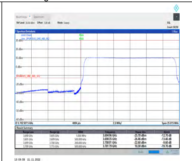
1-N78-3700-3800-PC2-30-15-L-6-CP-QPSK-Outer_Full-38@0-Ant1-1--PASS-see graph
