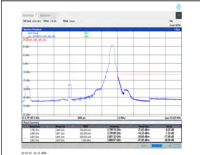
1-N78-3700-3800-PC2-30-15-H-5-CP-QPSK-Edge_1R_B_Right-1@37-Ant1-1--PASS-see graph
