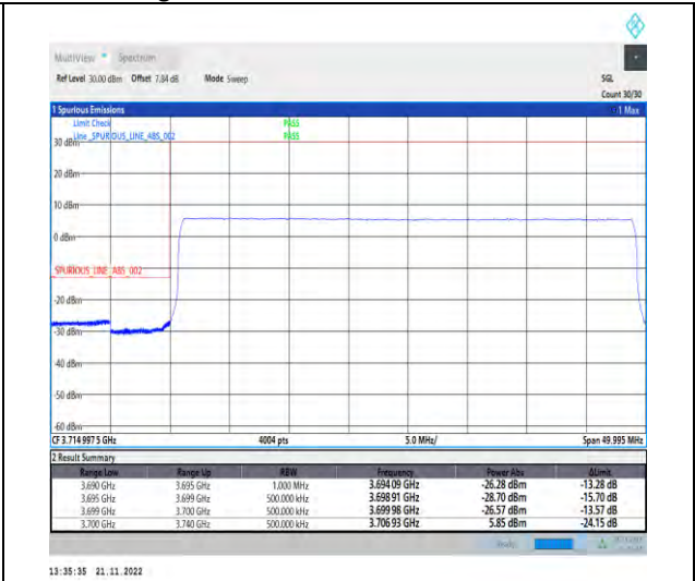
1-N78-3700-3800-PC2-30-40-L-6-CP-QPSK-Outer _Full-106@0-Ant1-1--PASS-see graph
