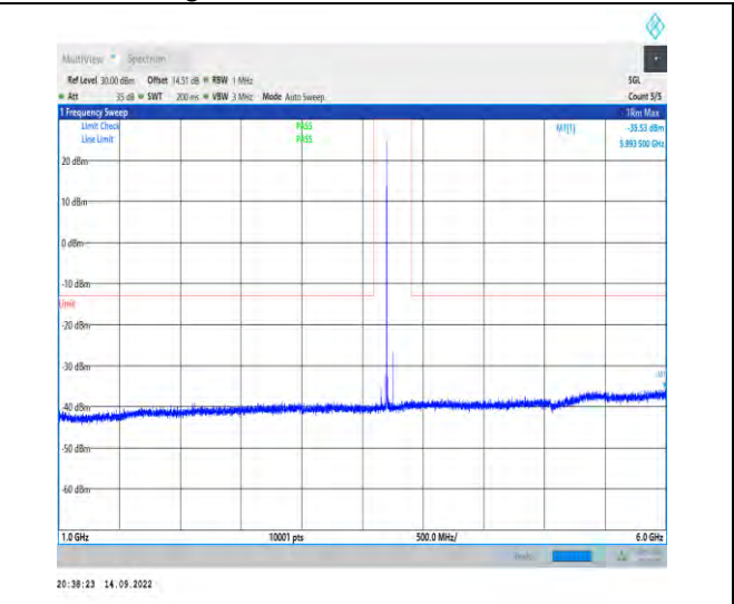
1-N78-3700-3800-PC2-30-100-M-1-DFT-PI2BPSK- Inner_1RB_Left-1@1-1000-6000-Ant1-5893.50--39.75-- 13-PASS
