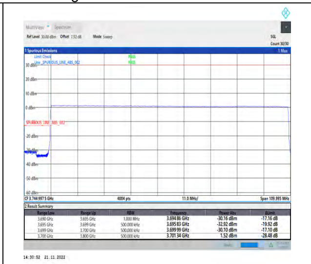
1-N78-3700-3800-PC2-30-100-L-6-CP-QPSK-Out er_Full-273@0-Ant1-1--PASS-see graph
