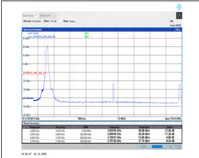
1-N78-3700-3800-PC2-30-60-L-4-CP-QPSK-Edge_1R B_Left-1@0-Ant1-1--PASS-see graph
