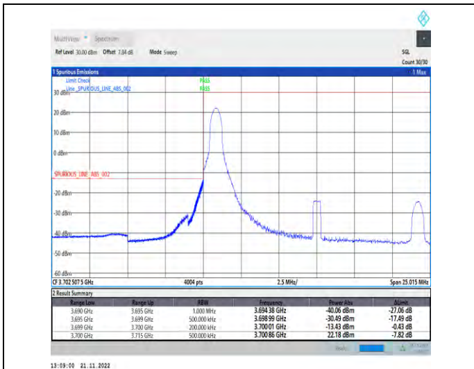
1-N78-3700-3800-PC2-30-15-L-4-CP-QPSK-Edge_1R_B_Left-1@0-Ant1-1--PASS-see graph
