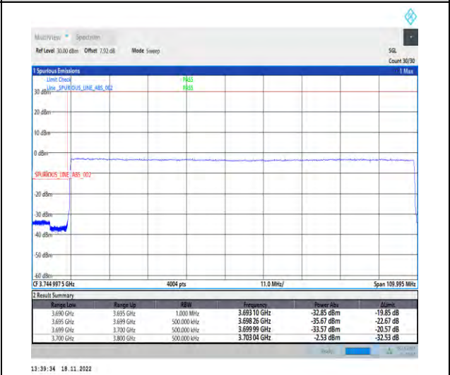
1-N78-3700-3800-PC2-30-100-L-6-CP-QPSK-Outer_Full-273@0-Ant1-1--PASS-see graph
