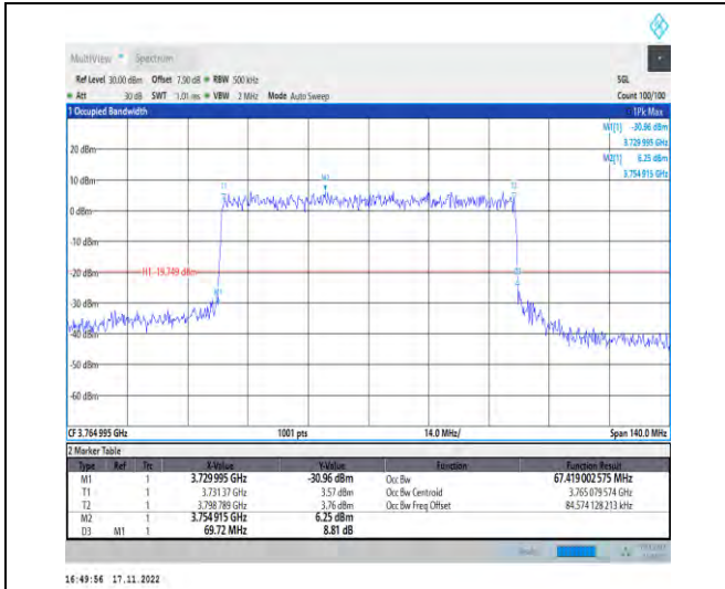
1-N78-3700-3800-PC2-30-70-H-6-CP-QPSK-Outer_Full-189@0-Ant1-67.419-69.720-≤70-PASS
