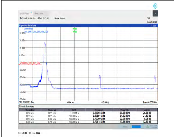
1-N78-3700-3800-PC2-30-50-L-4-CP-QPSK-Edge_1RB_Left-1@0-Ant1-1--PASS-see graph
