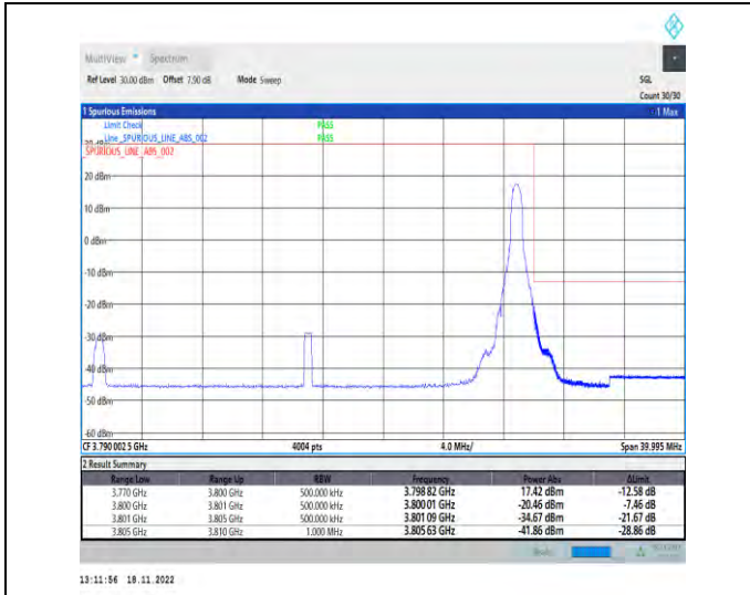
1-N78-3700-3800-PC2-30-30-H-2-DFT-PI2BPSK-Edge_1RB_Right-1@77-Ant1-1--PASS-see graph
