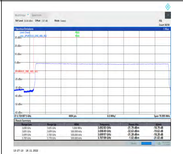
1-N78-3700-3800-PC2-30-70-L-6-CP-QPSK-Outer_Full-189@0-Ant1-1--PASS-see graph
