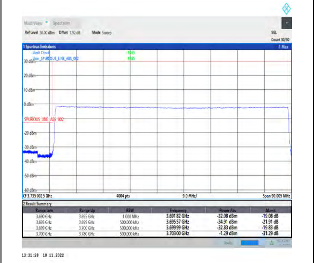
1-N78-3700-3800-PC2-30-80-L-6-CP-QPSK-Outer_Full-217@0-Ant1-1--PASS-see graph
