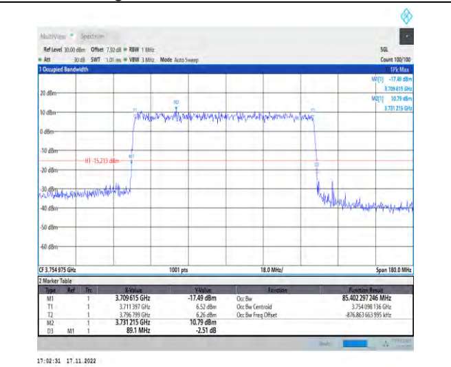
1-N78-3700-3800-PC2-30-90-H-1-DFT-QPSK-Outer_Full-240@0-Ant1-85.402-89.100-<=90-PASS
