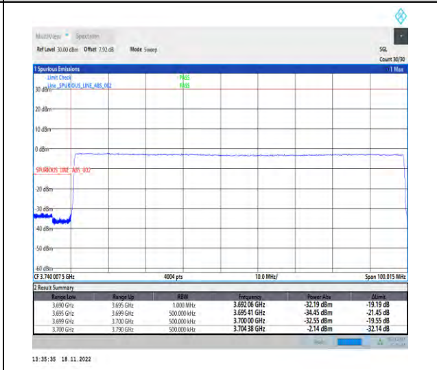
1-N78-3700-3800-PC2-30-90-L-6-CP-QPSK-Outer_Full-245@0-Ant1-1--PASS-see graph
