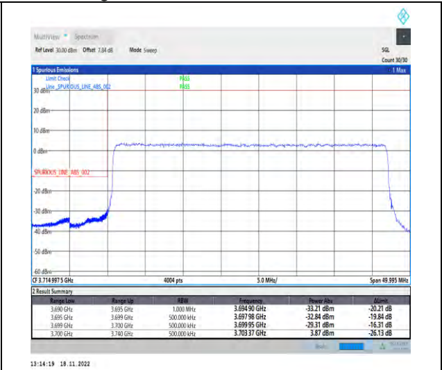
1-N78-3700-3800-PC2-30-40-L-3-DFT-PI2BPSK-Outer_Full-100@0-Ant1-1--PASS-see graph
