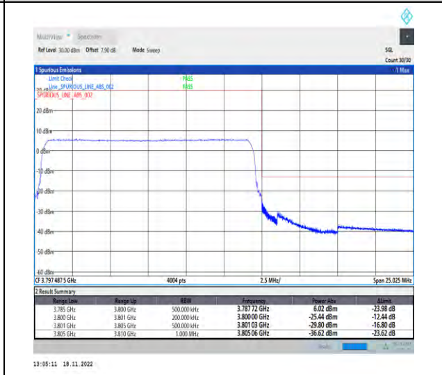
1-N78-3700-3800-PC2-30-15-H-6-CP-QPSK-Outer_Full-38@0-Ant1-1--PASS-see graph
