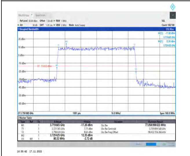
1-N78-3700-3800-PC2-30-80-H-1-DFT-QPSK-Outer_Full-216@0-Ant1-77.059-80.320-≤80-PASS
