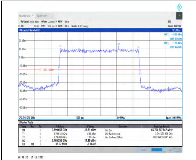
1-N78-3700-3800-PC2-30-90-L-2-DFT-PI2BPSK-Out er_Full-240@0-Ant1-85.704-88.920-≤90-PASS
