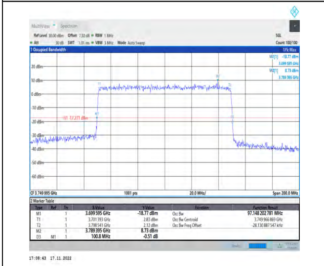
1-N78-3700-3800-PC2-30-100-M-8-CP-64QAM-Outer_Full-273@0-Ant1-97.148-100.800-≤100-PASS
