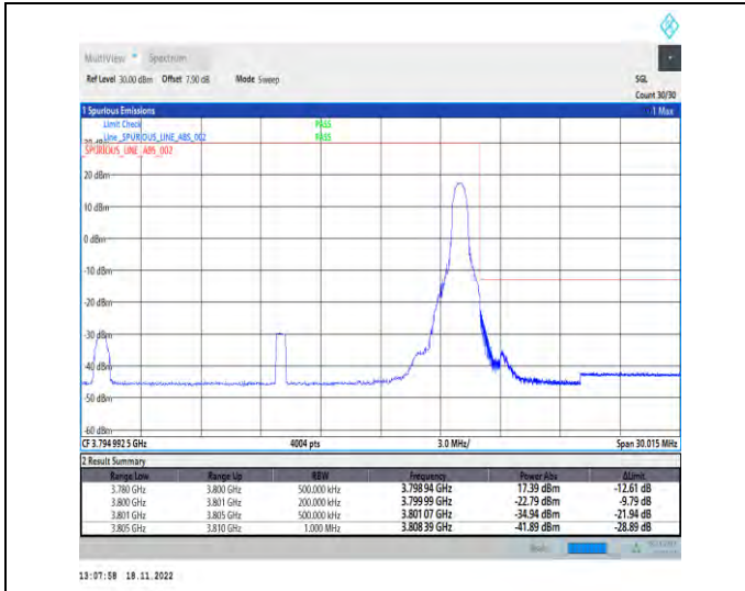
1-N78-3700-3800-PC2-30-20-H-2-DFT-PI2BPSK-Edge_1RB_Right-1@50-Ant1-1--PASS-see graph
