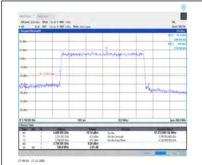
1-N78-3700-3800-PC2-30-100-M-6-CP-QPSK-Outer_Full-273@0-Ant1-97.372-100.800-≤100-PASS
