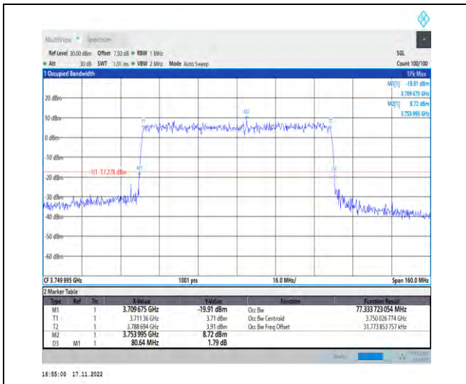
1-N78-3700-3800-PC2-30-80-M-8-CP-64QAM-Outer_Full-217@0-Ant1-77.334-80.640-≤80-PASS
