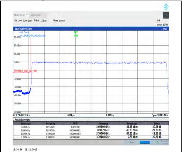
1-N78-3700-3800-PC2-30-80-L-3-DFT-PI2BPSK-Outer_Full-216@0-Ant1-1--PASS-see graph
