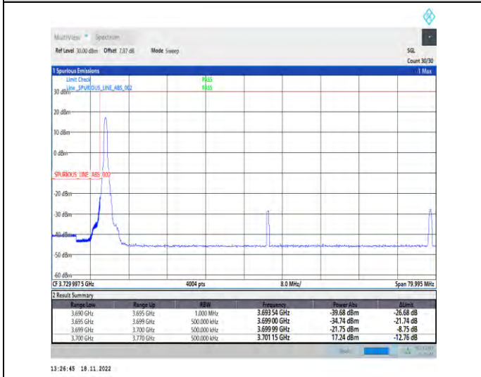
1-N78-3700-3800-PC2-30-70-L-4-CP-QPSK-Edge_1RB_Left-1@0-Ant1-1--PASS-see graph
