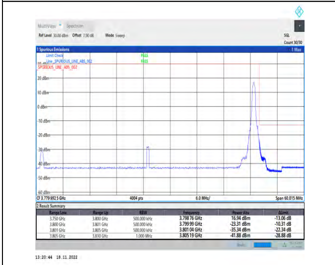
1-N78-3700-3800-PC2-30-50-H-5-CP-QPSK-Edge_1RB_Right-1@132-Ant1-1--PASS-see graph
