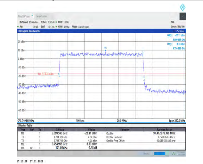
1-N78-3700-3800-PC2-30-100-H-6-CP-QPSK-Outer_Full-273@0-Ant1-97.413-101.000-≤100-PASS
