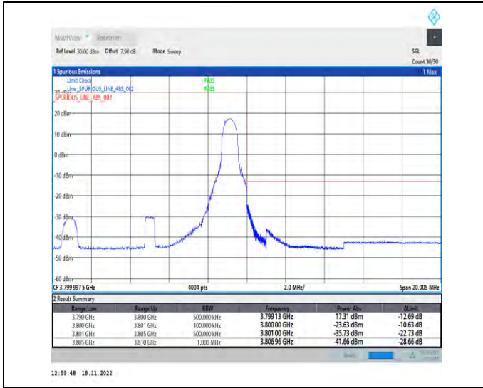
1-N78-3700-3800-PC2-30-10-H-2-DFT-PI2BPSK-Edge_1RB_Right-1@23-Ant1-1--PASS-see graph
