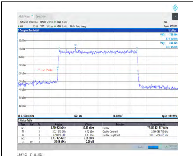
1-N78-3700-3800-PC2-30-80-H-7-CP-16QAM-Outer_Full-217@0-Ant1-77.543-80.480-≤80-PASS
