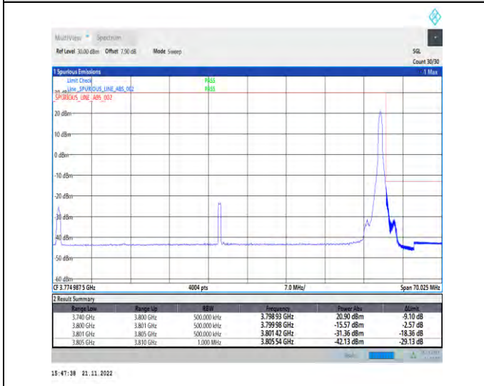
1-N78-3700-3800-PC2-30-60-H-5-CP-QPSK-Edge_1RB_Right-1@161-Ant1-1--PASS-see graph
