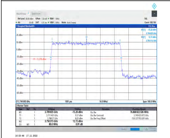
1-N78-3700-3800-PC2-30-80-M-2-DFT-PI2BPSK-Outer_Full-216@0-Ant1-76.869-80.000-≤80-PASS
