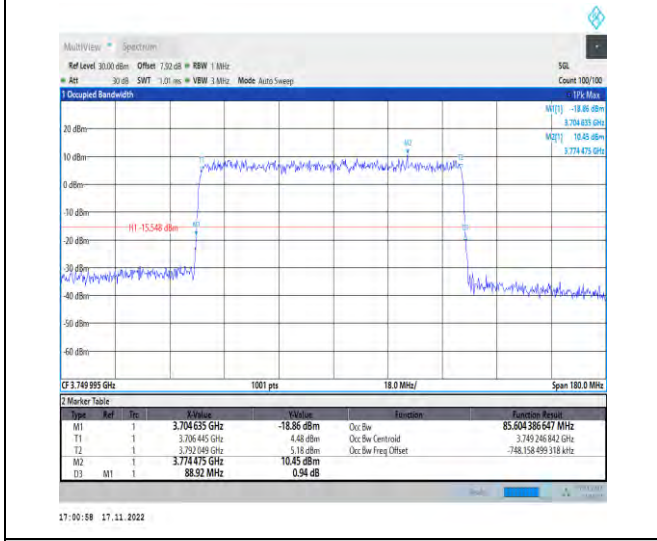
1-N78-3700-3800-PC2-30-90-M-3-DFT-16QAM-Outer_Full-240@0-Ant1-85.604-88.920-≤90-PASS
