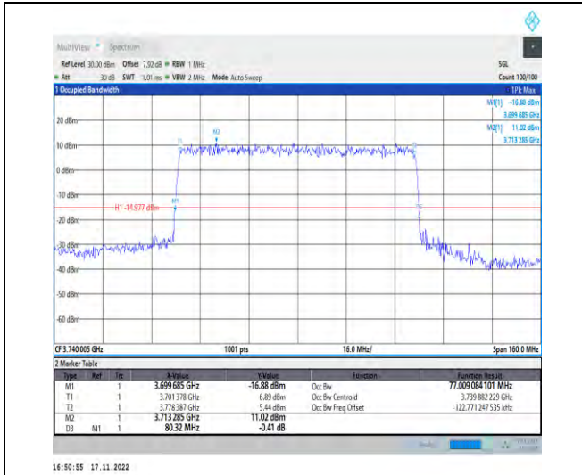
1-N78-3700-3800-PC2-30-80-L-1-DFT-QPSK-Outer_Full-216@0-Ant1-77.009-80.320-≤80-PASS
