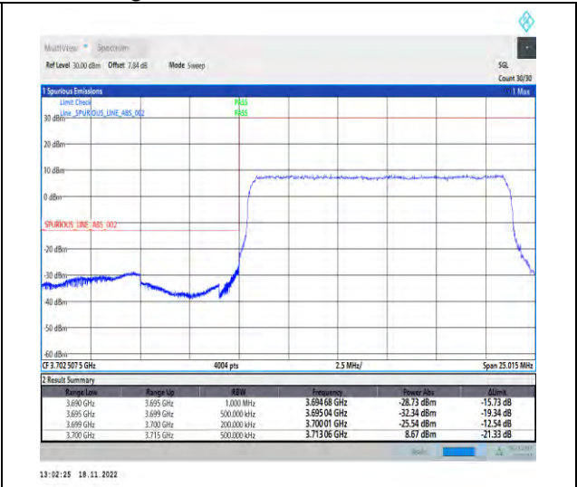
1-N78-3700-3800-PC2-30-15-L-3-DFT-PI2BPSK-Outer_Full-36@0-Ant1-1--PASS-see graph
