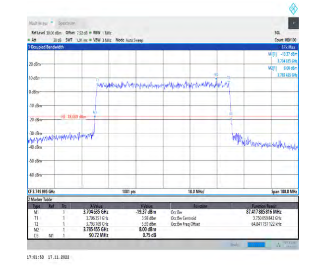
1-N78-3700-3800-PC2-30-90-M-8-CP-64QAM-Outer_Full-245@0-Ant1-87.418-90.720-≤90-PASS
