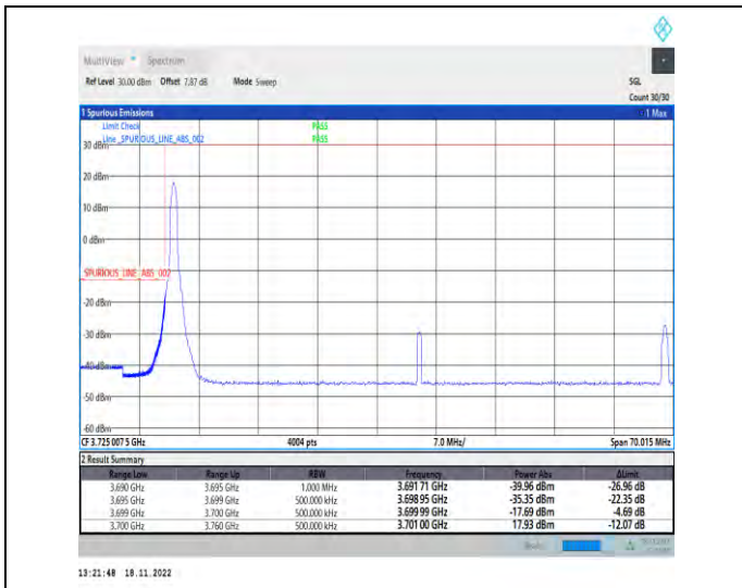
1-N78-3700-3800-PC2-30-60-L-1-DFT-PI2BPSK-Edge_1RB_Left-1@0-Ant1-1--PASS-see graph
