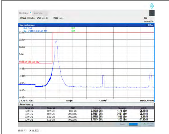
1-N78-3700-3800-PC2-30-30-L-1-DFT-PI2BPSK-Edge_1RB_Left-1@0-Ant1-1--PASS-see graph
