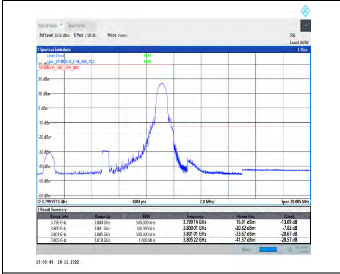
1-N78-3700-3800-PC2-30-10-H-5-CP-QPSK-Edge_1RB_Right-1@23-Ant1-1--PASS-see graph
