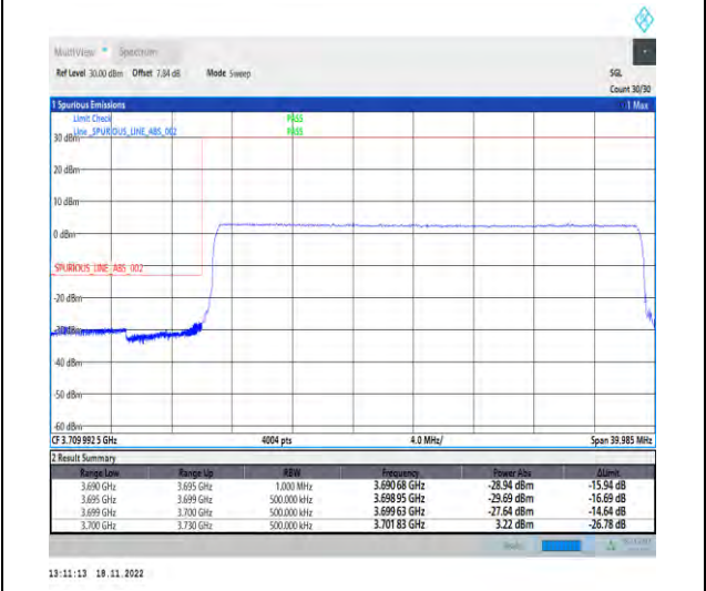
1-N78-3700-3800-PC2-30-30-L-6-CP-QPSK-Outer_Full-78@0-Ant1-1--PASS-see graph
