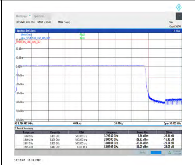
1-N78-3700-3800-PC2-30-40-H-6-CP-QPSK-Outer_Full-106@0-Ant1-1--PASS-see graph
