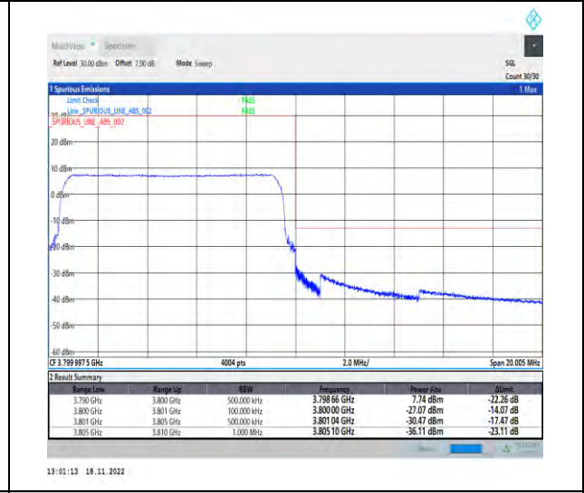
1-N78-3700-3800-PC2-30-10-H-6-CP-QPSK-Outer_Full-24@0-Ant1-1--PASS-see graph
