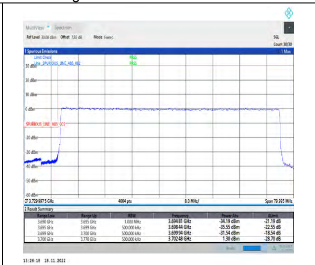
1-N78-3700-3800-PC2-30-70-L-3-DFT-PI2BPSK-Outer_Full-180@0-Ant1-1--PASS-see graph
