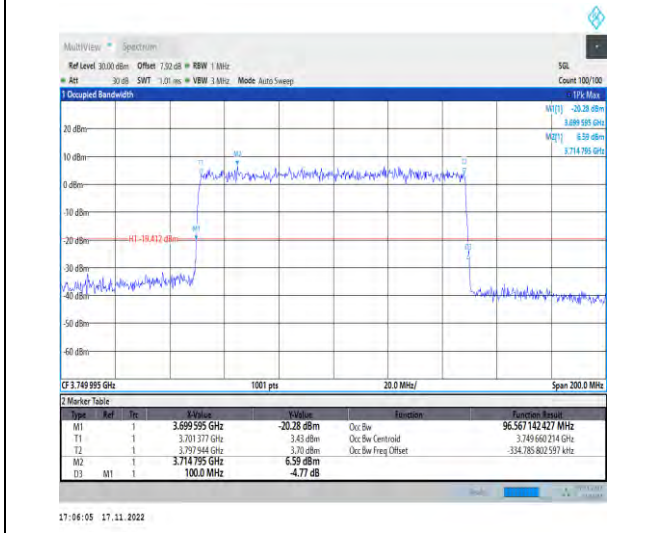
1-N78-3700-3800-PC2-30-100-L-5-DFT-256QAM-Outer_Full-270@0-Ant1-96.567-100.000-≤100-PASS
