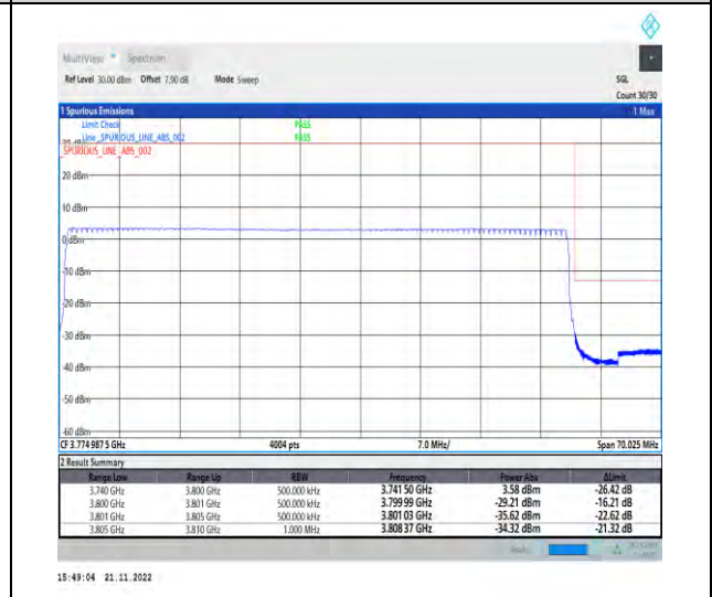
1-N78-3700-3800-PC2-30-60-H-6-CP-QPSK-Outer_Full-162@0-Ant1-1--PASS-see graph
