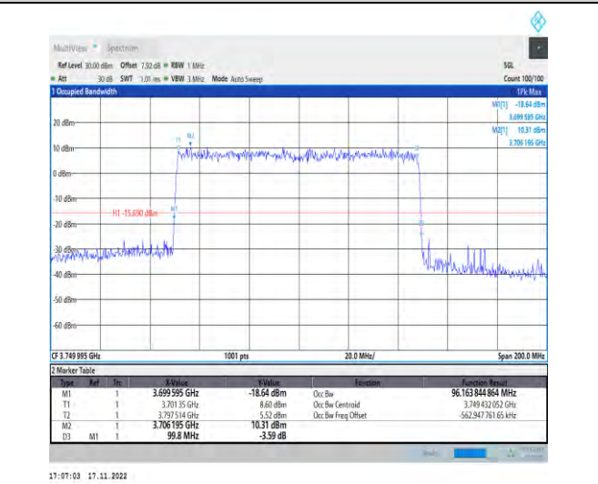
1-N78-3700-3800-PC2-30-100-M-1-DFT-QPSK-Outer_Full-270@0-Ant1-96.164-99.800-≤100-PASS
