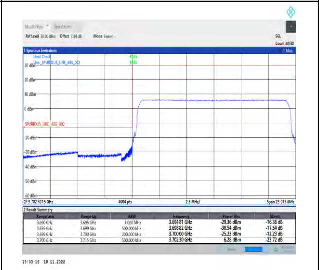
1-N78-3700-3800-PC2-30-15-L-6-CP-QPSK-Outer_Full-38@0-Ant1-1--PASS-see graph
