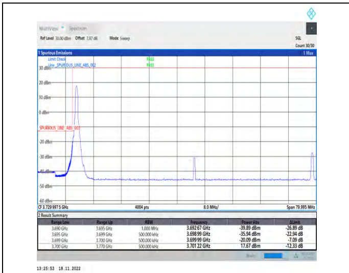
1-N78-3700-3800-PC2-30-70-L-1-DFT-PI2BPSK-Edge_1RB_Left-1@0-Ant1-1--PASS-see graph
