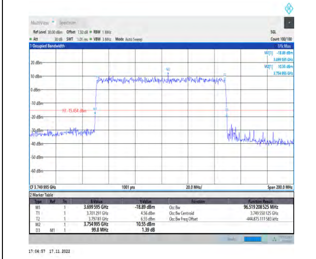
1-N78-3700-3800-PC2-30-100-L-1-DFT-QPSK-Outer_Full-270@0-Ant1-96.519-99.800-≤100-PASS
