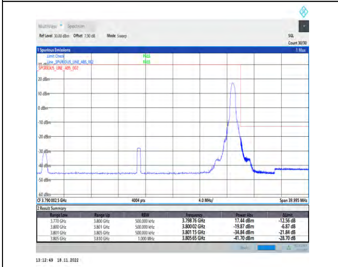
1-N78-3700-3800-PC2-30-30-H-5-CP-QPSK-Edge_1RB_Right-1@77-Ant1-1--PASS-see graph
