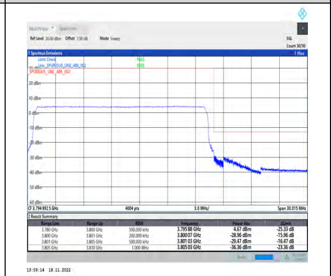
1-N78-3700-3800-PC2-30-20-H-6-CP-QPSK-Outer_Full-51@0-Ant1-1--PASS-see graph
