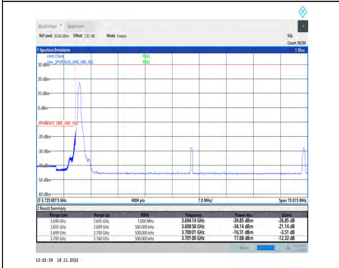
1-N78-3700-3800-PC2-30-60-L-4-CP-QPSK-Edge_1RB_Left-1@0-Ant1-1--PASS-see graph
