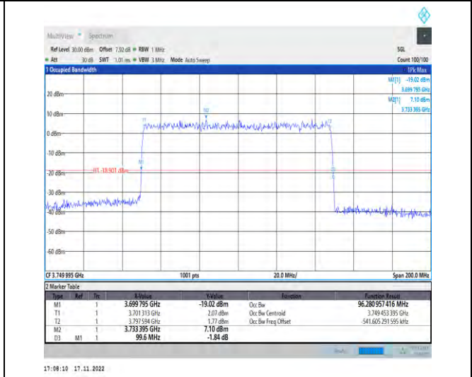
1-N78-3700-3800-PC2-30-100-M-5-DFT-256QAM-Out_Full-270@0-Ant1-96.281-99.600-≤100-PASS
