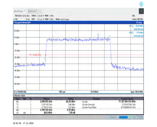
1-N78-3700-3800-PC2-30-80-L-4-DFT-64QAM-Outer_Full-216@0-Ant1-77.187-80.800-≤80-PASS
