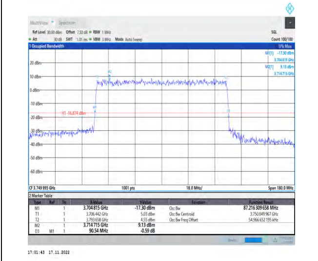
1-N78-3700-3800-PC2-30-90-M-7-CP-16QAM-Outer_Full-245@0-Ant1-87.216-90.540-≤90-PASS
