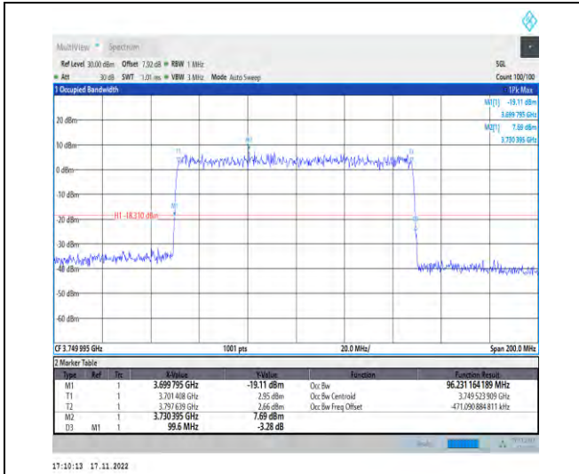
1-N78-3700-3800-PC2-30-100-H-5-DFT-256QAM-Outer_Full-270@0-Ant1-96.231-99.600-≤100-PASS
