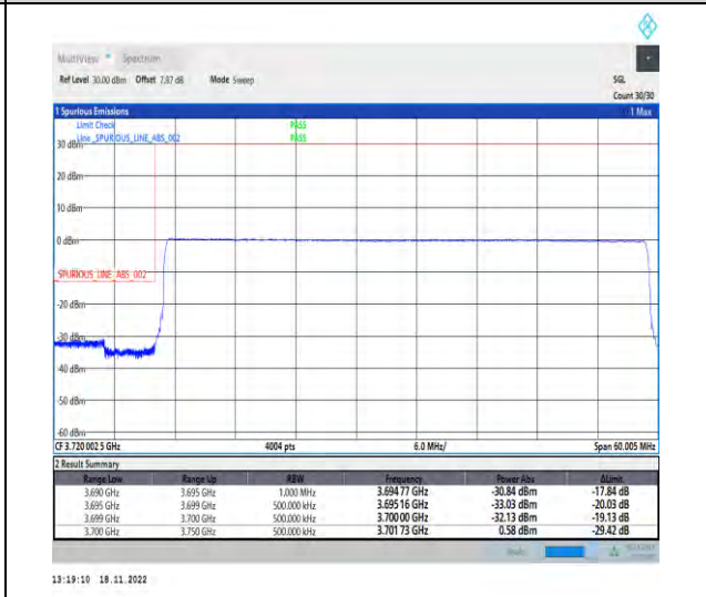
1-N78-3700-3800-PC2-30-50-L-6-CP-QPSK-Outer_Full-133@0-Ant1-1--PASS-see graph
