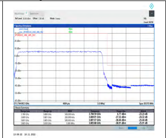
1-N78-3700-3800-PC2-30-20-H-3-DFT-PI2BPSK-Outer_Full-50@0-Ant1-1--PASS-see graph
