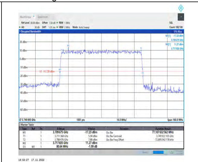
1-N78-3700-3800-PC2-30-80-M-1-DFT-QPSK-Outer_Full-216@0-Ant1-77.108-80.640-≤80-PASS
