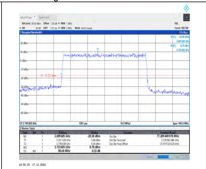
1-N78-3700-3800-PC2-30-80-L-6-CP-QPSK-Outer_Full-217@0-Ant1-77.309-80.640-≤80-PASS
