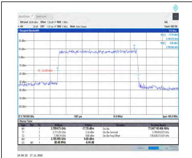
1-N78-3700-3800-PC2-30-80-M-4-DFT-64QAM-Out_er_Full-216@0-Ant1-77.047-80.480-≤80-PASS
