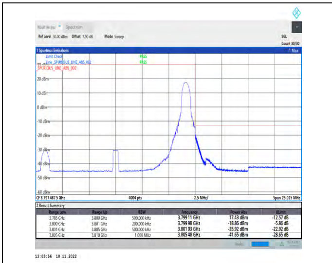
1-N78-3700-3800-PC2-30-15-H-2-DFT-PI2BPSK-Edge_1RB_Right-1@37-Ant1-1--PASS-see graph
