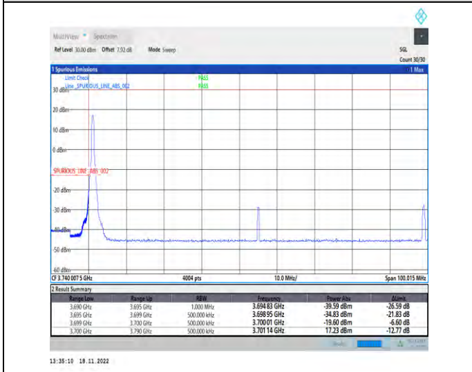
1-N78-3700-3800-PC2-30-90-L-4-CP-QPSK-Edge_1RB_Left-1@0-Ant1-1--PASS-see graph
