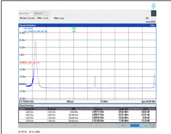
1-N78-3700-3800-PC2-30-80-L-1-DFT-PI2BPSK-Edge_1RB_Left-1@0-Ant1-1--PASS-see graph
