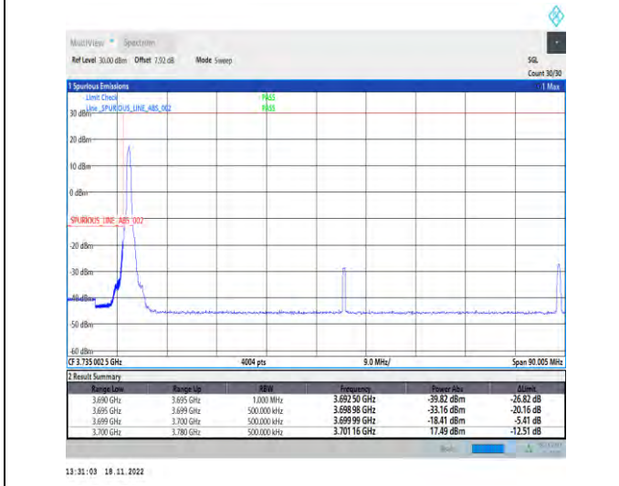
1-N78-3700-3800-PC2-30-80-L-4-CP-QPSK-Edge_1RB_Left-1@0-Ant1-1--PASS-see graph
