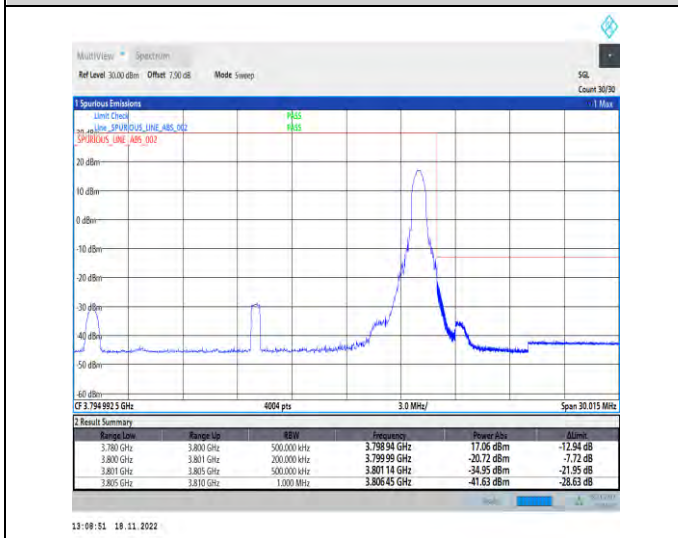
1-N78-3700-3800-PC2-30-20-H-5-CP-QPSK-Edge_1RB_Right-1@50-Ant1-1--PASS-see graph
