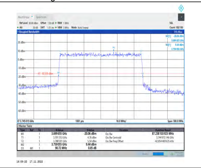
1-N78-3700-3800-PC2-30-90-L-7-CP-16QAM-Outer_Full-245@0-Ant1-87.238-90.720-≤90-PASS
