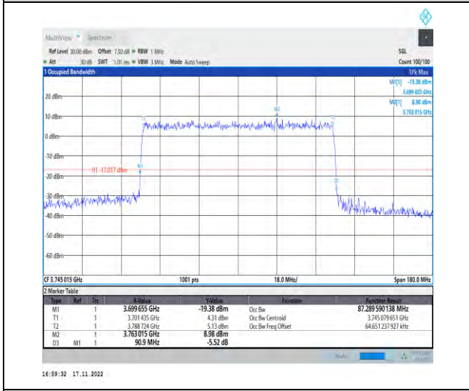
1-N78-3700-3800-PC2-30-90-L-8-CP-64QAM-Outer_Full-245@0-Ant1-87.29-90.900-≤90-PASS
