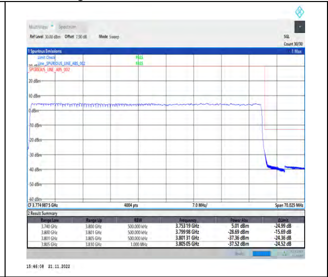
1-N78-3700-3800-PC2-30-60-H-3-DFT-PI2BPSK-Outer_Full-162@0-Ant1-1--PASS-see graph
