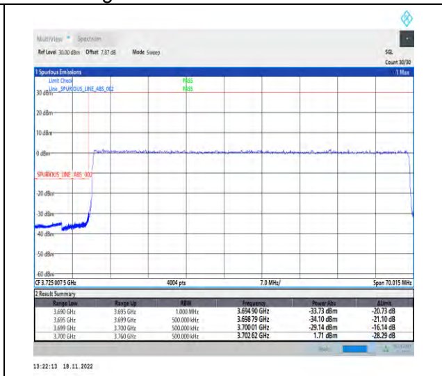
1-N78-3700-3800-PC2-30-60-L-3-DFT-PI2BPSK-Outer_Full-162@0-Ant1-1--PASS-see graph
