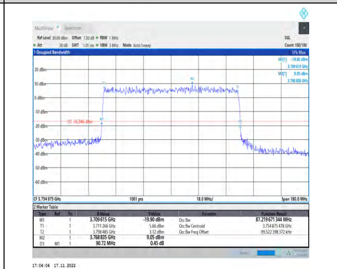
1-N78-3700-3800-PC2-30-90-H-7-CP-16QAM-Outer_Full-245@0-Ant1-87.22-90.720-≤90-PASS
