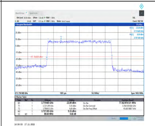
1-N78-3700-3800-PC2-30-80-H-6-CP-QPSK-Outer_Full-217@0-Ant1-77.563-80.640-≤80-PASS
