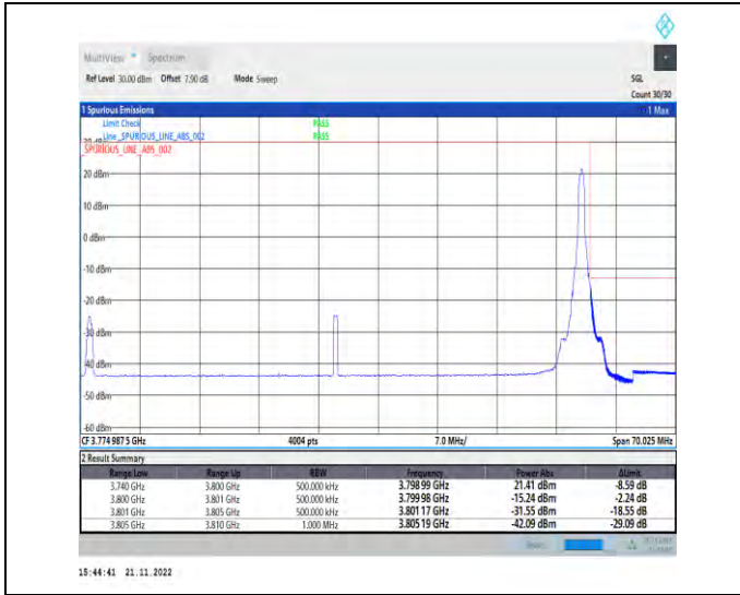
1-N78-3700-3800-PC2-30-60-H-2-DFT-PI2BPSK-Edge_1RB_Right-1@161-Ant1-1--PASS-see graph
