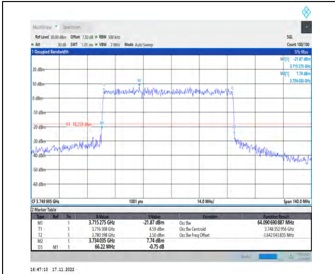
1-N78-3700-3800-PC2-30-70-M-3-DFT-16QAM-Out er_Full-180@0-Ant1-64.091-66.220-≤70-PASS
