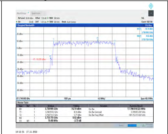
1-N78-3700-3800-PC2-30-20-M-3-DFT-16QAM-Outer_Full-50@0-Ant1-17.798-19.480-≤20-PASS
