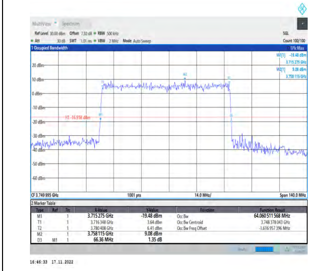
1-N78-3700-3800-PC2-30-70-M-1-DFT-QPSK-Outer_Full-180@0-Ant1-64.061-66.360-≤70-PASS
