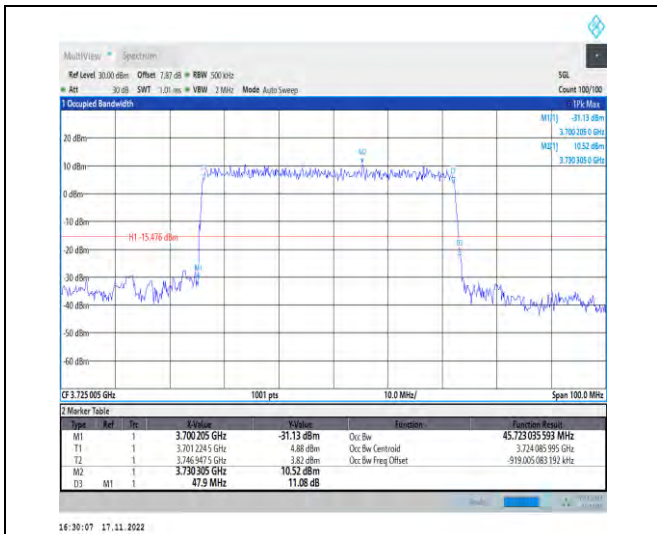
1-N78-3700-3800-PC2-30-50-L-2-DFT-PI2BPSK-Out er_Full-128@0-Ant1-45.723-47.900-≤50-PASS
