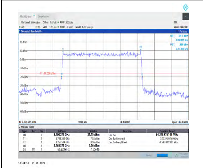
1-N78-3700-3800-PC2-30-70-L-2-DFT-PI2BPSK-Outer_Full-180@0-Ant1-64.249-66.220-≤70-PASS
