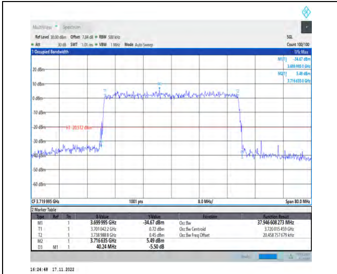
1-N78-3700-3800-PC2-30-40-L-9-CP-256QAM-Outer_Full-106@0-Ant1-37.947-40.240-≤40-PASS
