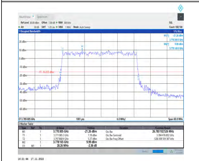
1-N78-3700-3800-PC2-30-30-H-4-DFT-64QAM-Outer_Full-75@0-Ant1-26.783-28.260-≤30-PASS
