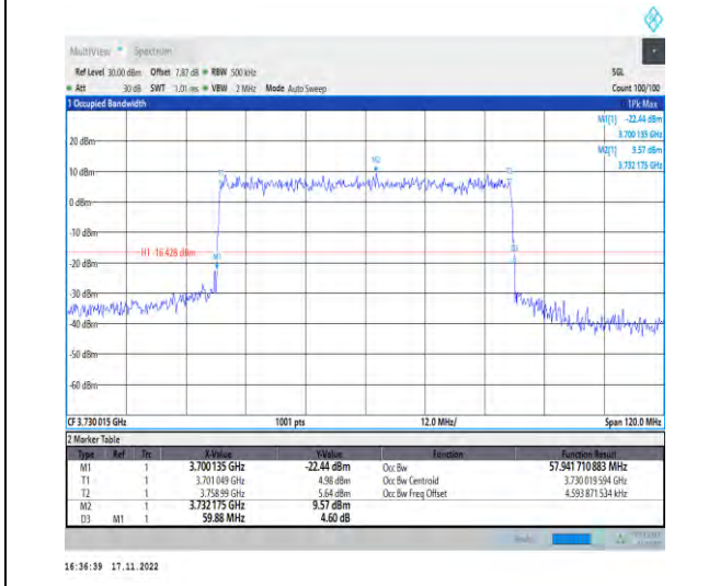
1-N78-3700-3800-PC2-30-60-L-1-DFT-QPSK-Outer_Full-162@0-Ant1-57.942-59.880-≤60-PASS
