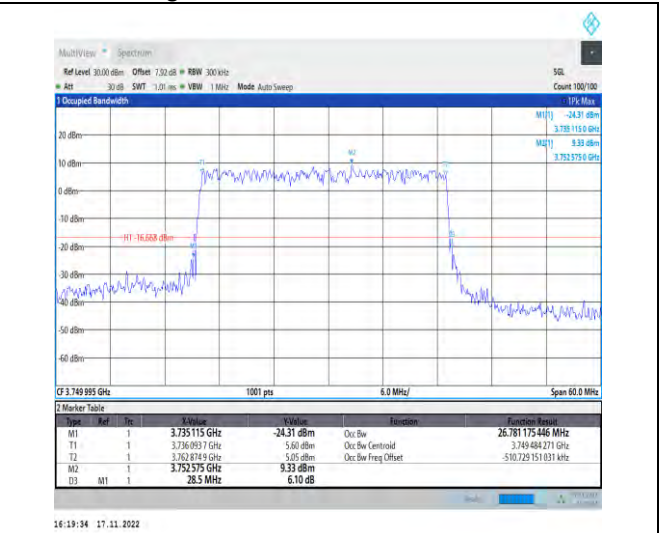
1-N78-3700-3800-PC2-30-30-M-4-DFT-64QAM-Out r_Full-75@0-Ant1-26.781-28.500-≤30-PASS
