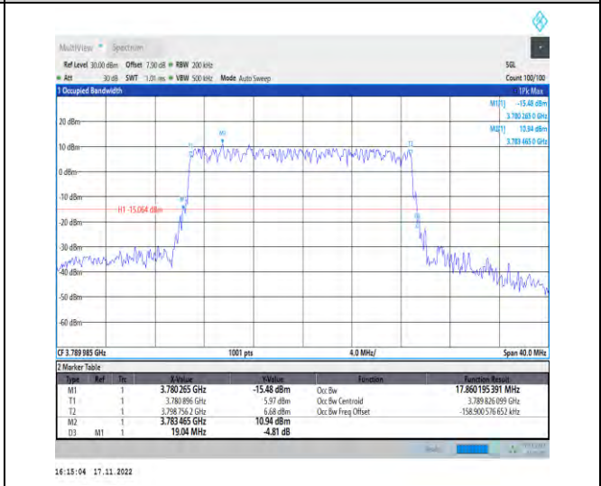
1-N78-3700-3800-PC2-30-20-H-4-DFT-64QAM-Outer_Full-50@0-Ant1-17.86-19.040-<=20-PASS
