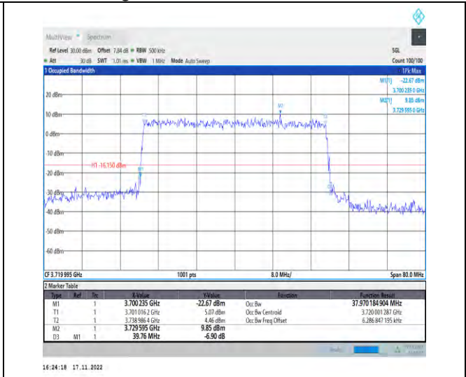
1-N78-3700-3800-PC2-30-40-L-6-CP-QPSK-Outer_Full-106@0-Ant1-37.97-39.760-≤40-PASS
