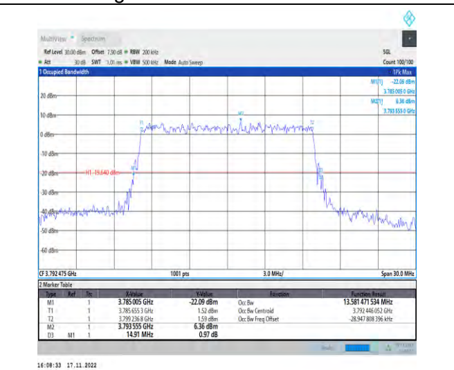
1-N78-3700-3800-PC2-30-15-H-9-CP-256QAM-Outer_Full-38@0-Ant1-13.581-14.910-≤15-PASS
