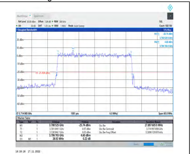
1-N78-3700-3800-PC2-30-30-L-9-CP-256QAM-Outer_Full-78@0-Ant1-27.898-28.920-≤30-PASS
