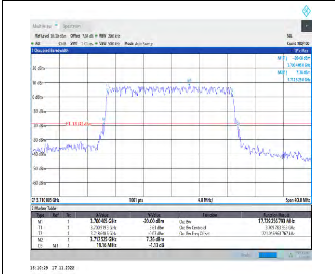
1-N78-3700-3800-PC2-30-20-L-5-DFT-256QAM-Outer_Full-50@0-Ant1-17.729-19.160-<=20-PASS
