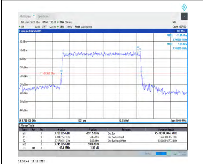
1-N78-3700-3800-PC2-30-50-L-4-DFT-64QAM-Outer_Full-128@0-Ant1-45.786-47.500-≤50-PASS
