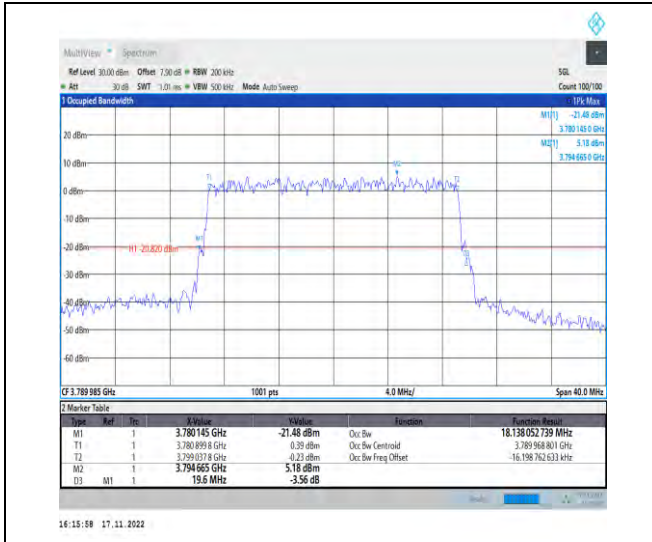
1-N78-3700-3800-PC2-30-20-H-9-CP-256QAM-Outer_Full-51@0-Ant1-18.138-19.600-≤20-PASS
