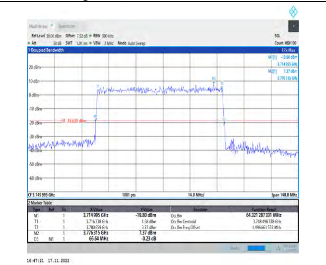
1-N78-3700-3800-PC2-30-70-M-4-DFT-64QAM-Out er_Full-180@0-Ant1-64.321-66.640-≤70-PASS
