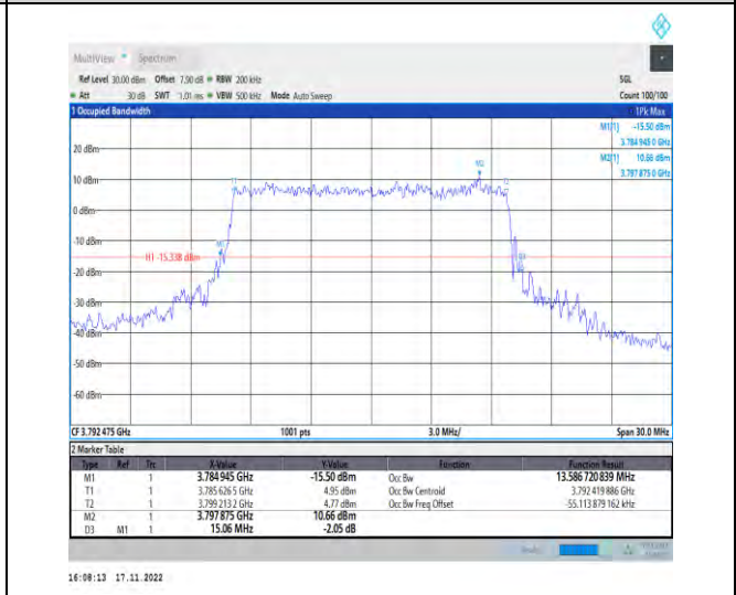
1-N78-3700-3800-PC2-30-15-H-7-CP-16QAM-Outer_Full-38@0-Ant1-13.587-15.060-≤15-PASS
