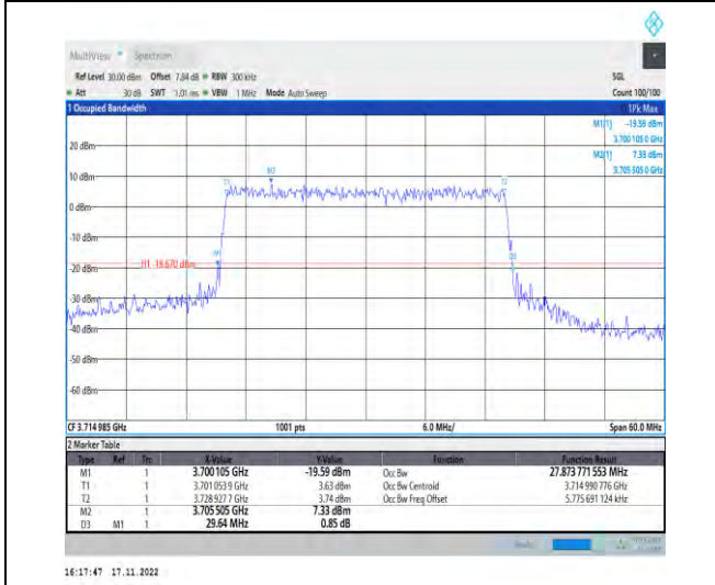
1-N78-3700-3800-PC2-30-30-L-6-CP-QPSK-Outer_Full-78@0-Ant1-27.874-29.640-≤30-PASS
