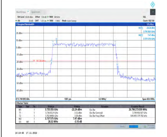
1-N78-3700-3800-PC2-30-30-M-5-DFT-256QAM-Out ter_Full-75@0-Ant1-26.796-28.320-≤30-PASS
