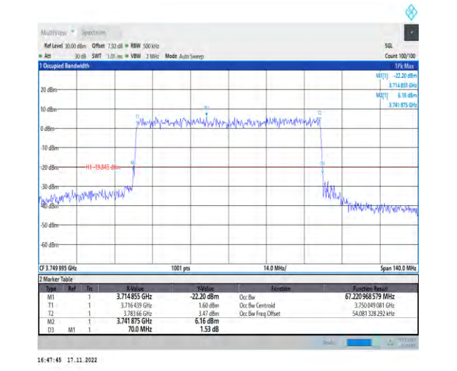
1-N78-3700-3800-PC2-30-70-M-6-CP-QPSK-Out er_Full-189@0-Ant1-67.221-70.000-≤70-PASS
