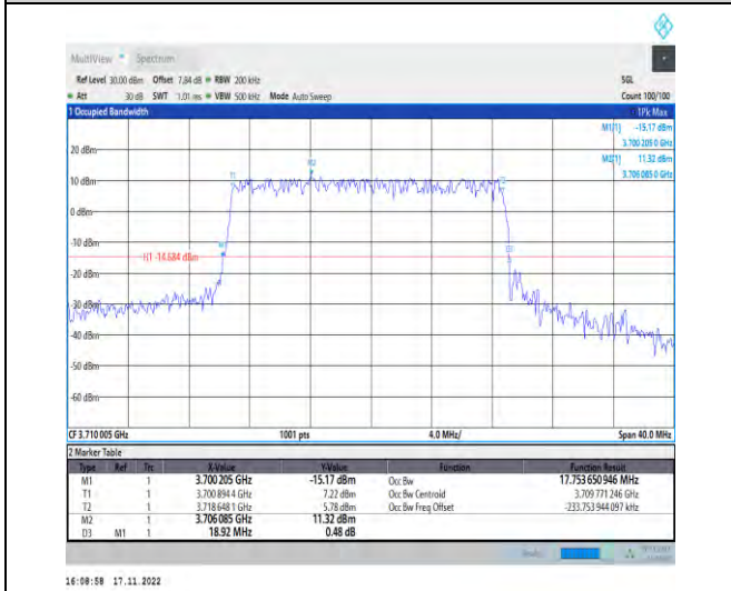
1-N78-3700-3800-PC2-30-20-L-1-DFT-QPSK-Outer_Full-50@0-Ant1-17.754-18.920-≤20-PASS
