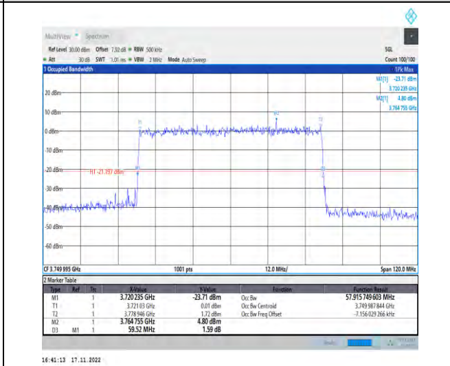
1-N78-3700-3800-PC2-30-60-M-9-CP-256QAM-Outer_Full-162@0-Ant1-57.916-59.520-≤60-PASS
