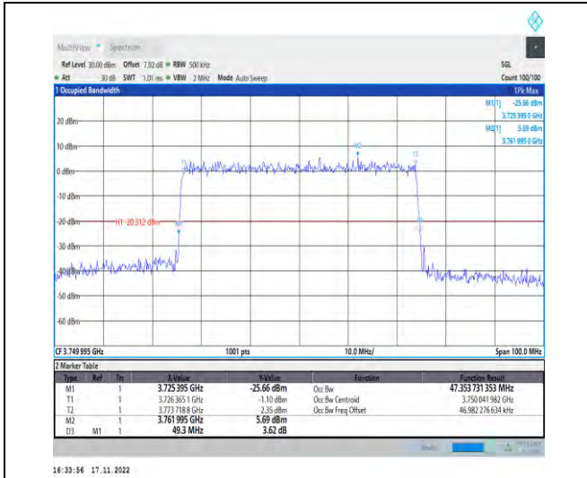
1-N78-3700-3800-PC2-30-50-M-9-CP-256QAM-Outer_Full-133@0-Ant1-47.354-49.300-≤50-PASS
