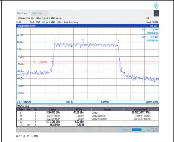
1-N78-3700-3800-PC2-30-30-L-3-DFT-16QAM-Outer_Full-75@0-Ant1-26.755-28.380-≤30-PASS
