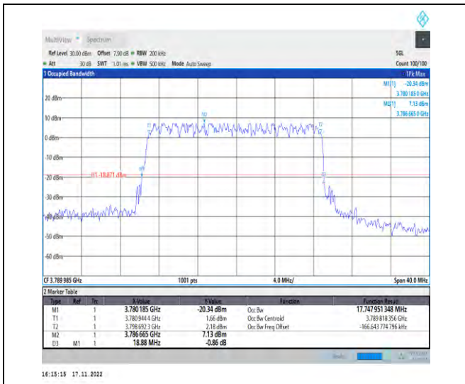
1-N78-3700-3800-PC2-30-20-H-5-DFT-256QAM-Out_Full-50@0-Ant1-17.748-18.880-≤20-PASS
