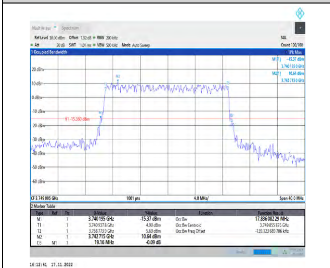
1-N78-3700-3800-PC2-30-20-M-4-DFT-64QAM-Outer_Full-50@0-Ant1-17.836-19.160-≤20-PASS
