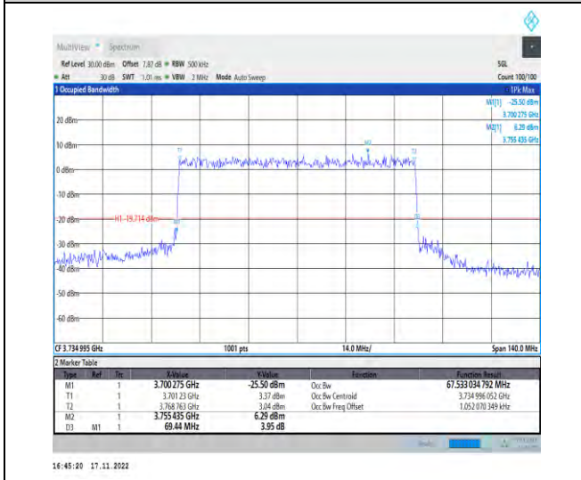
1-N78-3700-3800-PC2-30-70-L-6-CP-QPSK-Outer_Full-189@0-Ant1-67.533-69.440-≤70-PASS
