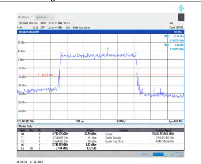
1-N78-3700-3800-PC2-30-40-M-5-DFT-256QAM-Out er_Full-100@0-Ant1-35.815-37.440-≤40-PASS
