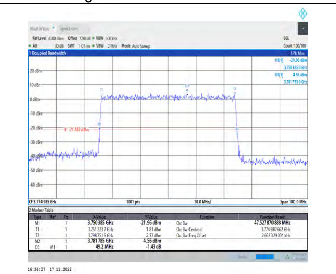
1-N78-3700-3800-PC2-30-50-H-9-CP-256QAM-Outer_Full-133@0-Ant1-47.528-49.200-≤50-PASS
