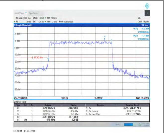
1-N78-3700-3800-PC2-30-50-H-1-DFT-QPSK-Outer_Full-128@0-Ant1-45.558-47.500-≤50-PASS
