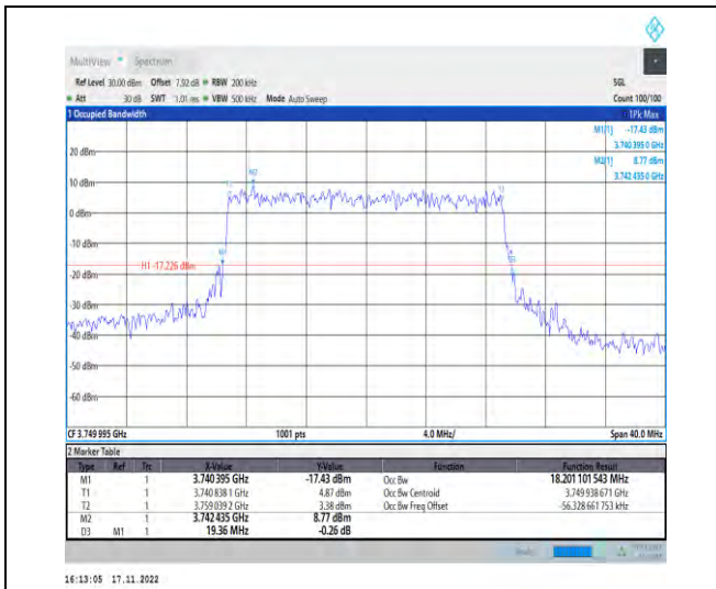
1-N78-3700-3800-PC2-30-20-M-6-CP-QPSK-Outer_Full-51@0-Ant1-18.201-19.360-≤20-PASS
