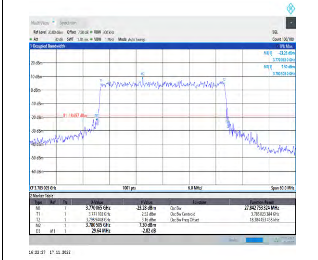
1-N78-3700-3800-PC2-30-30-H-8-CP-64QAM-Outer_Full-78@0-Ant1-27.843-29.640-≤30-PASS
