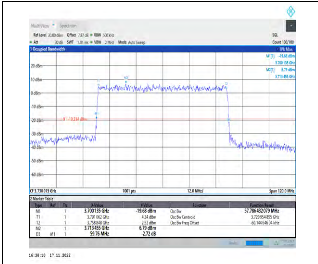
1-N78-3700-3800-PC2-30-60-L-7-CP-16QAM-Outer_Full-162@0-Ant1-57.786-59.760-≤60-PASS
