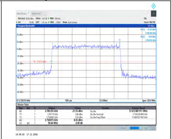
1-N78-3700-3800-PC2-30-60-L-8-CP-64QAM-Outer_Full-162@0-Ant1-57.673-59.640-≤60-PASS
