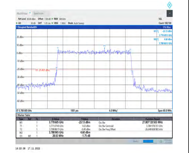
1-N78-3700-3800-PC2-30-30-H-9-CP-256QAM-Outer_Full-78@0-Ant1-27.807-28.920-≤30-PASS
