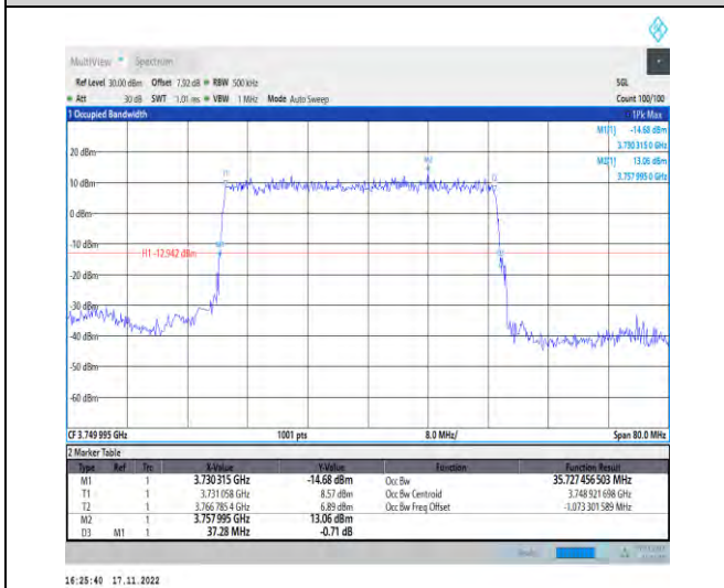
1-N78-3700-3800-PC2-30-40-M-2-DFT-PI2BPSK-Outer_Full-100@0-Ant1-35.727-37.280-≤40-PASS
