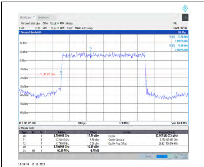
1-N78-3700-3800-PC2-30-60-M-2-DFT-PI2BPSK-Outer_Full-162@0-Ant1-57.957-60.360-≤60-PASS
