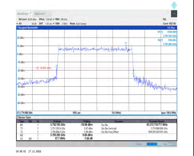
1-N78-3700-3800-PC2-30-50-H-3-DFT-16QAM-Outer_Full-128@0-Ant1-45.573-47.700-≤50-PASS
