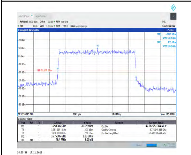
1-N78-3700-3800-PC2-30-50-H-6-CP-QPSK-Outer_Full-133@0-Ant1-47.383-49.400-≤50-PASS
