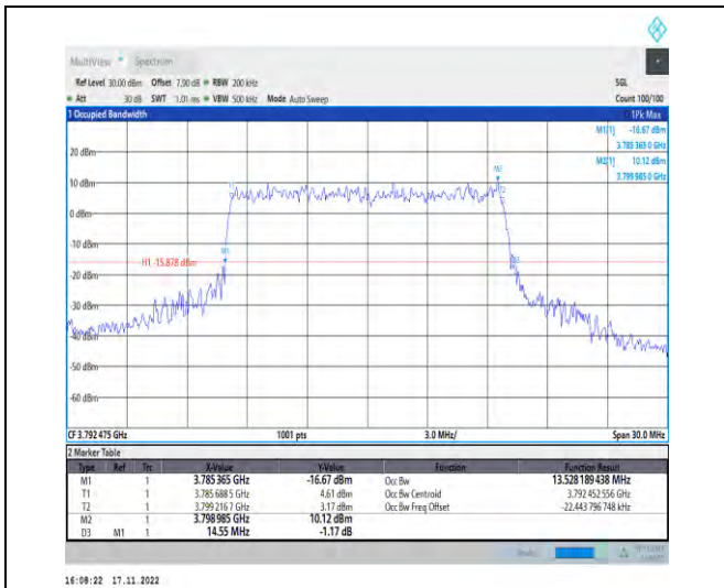
1-N78-3700-3800-PC2-30-15-H-8-CP-64QAM-Outer_Full-38@0-Ant1-13.528-14.550-≤15-PASS
