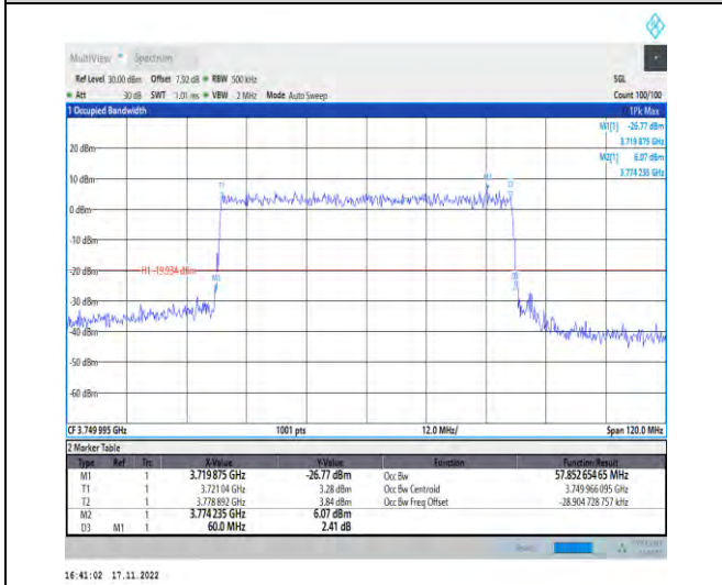
1-N78-3700-3800-PC2-30-60-M-8-CP-64QAM-Outer_Full-162@0-Ant1-57.853-60.000-≤60-PASS
