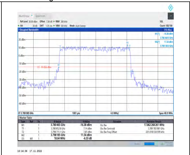
1-N78-3700-3800-PC2-30-20-H-2-DFT-PI2BPSK-Outer_Full-50@0-Ant1-17.862-18.640-<=20-PASS
