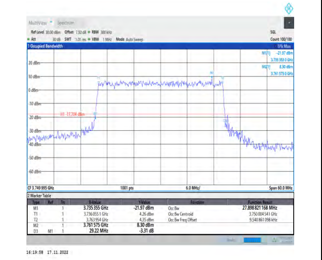
1-N78-3700-3800-PC2-30-30-M-6-CP-QPSK-Outer Full-78@0-Ant1-27.899-29.220-≤30-PASS
