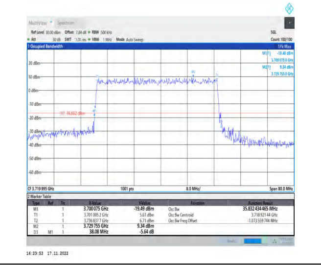
1-N78-3700-3800-PC2-30-40-L-4-DFT-64QAM-Outer_Full-100@0-Ant1-35.832-38.080-≤40-PASS
