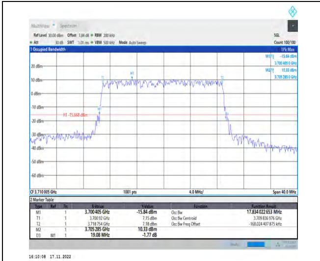
1-N78-3700-3800-PC2-30-20-L-3-DFT-16QAM-Outer_Full-50@0-Ant1-17.834-19.080-<=20-PASS
