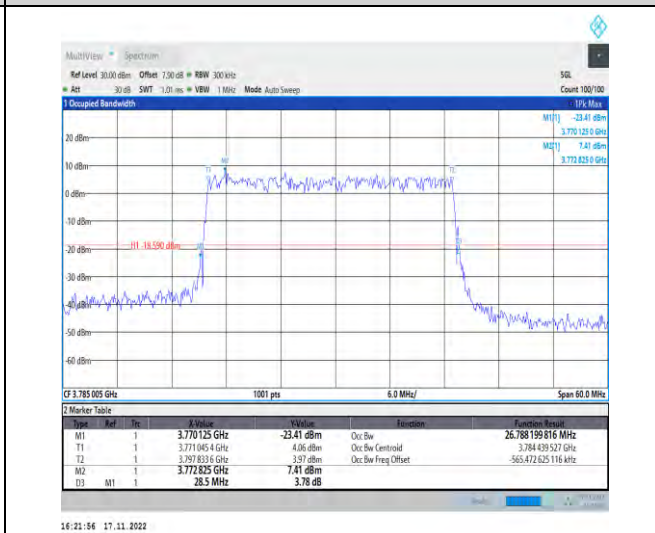
1-N78-3700-3800-PC2-30-30-H-5-DFT-256QAM-Outer_Full-75@0-Ant1-26.788-28.500-≤30-PASS
