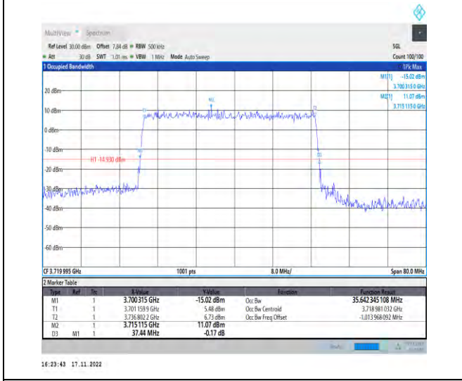
1-N78-3700-3800-PC2-30-40-L-3-DFT-16QAM-Outer_Full-100@0-Ant1-35.642-37.440-≤40-PASS
