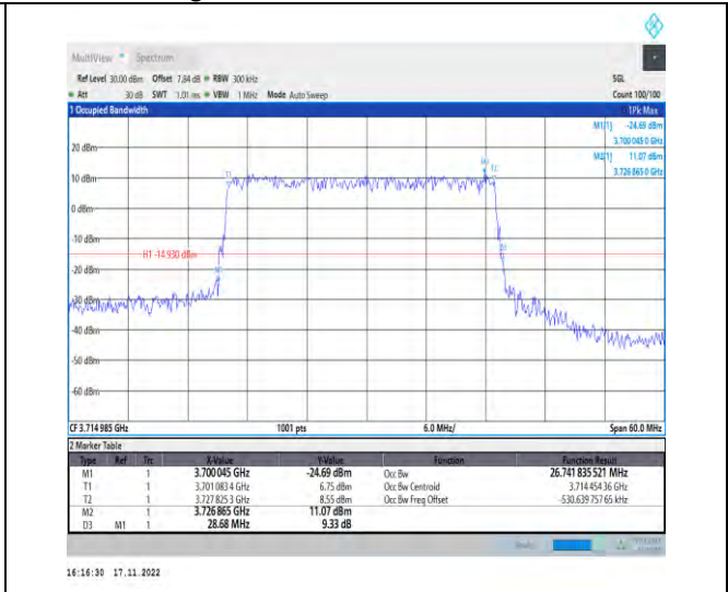
1-N78-3700-3800-PC2-30-30-L-1-DFT-QPSK-Outer_Full-75@0-Ant1-26.742-28.680-≤30-PASS
