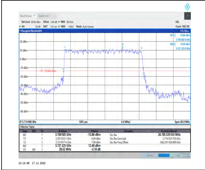
1-N78-3700-3800-PC2-30-30-L-2-DFT-PI2BPSK-Outer_Full-75@0-Ant1-26.785-28.020-≤30-PASS
