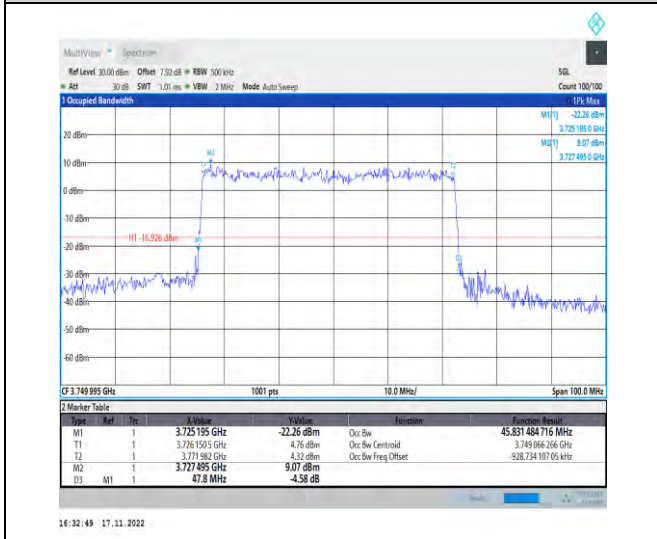
1-N78-3700-3800-PC2-30-50-M-3-DFT-16QAM-Outer_Full-128@0-Ant1-45.831-47.800-≤50-PASS
