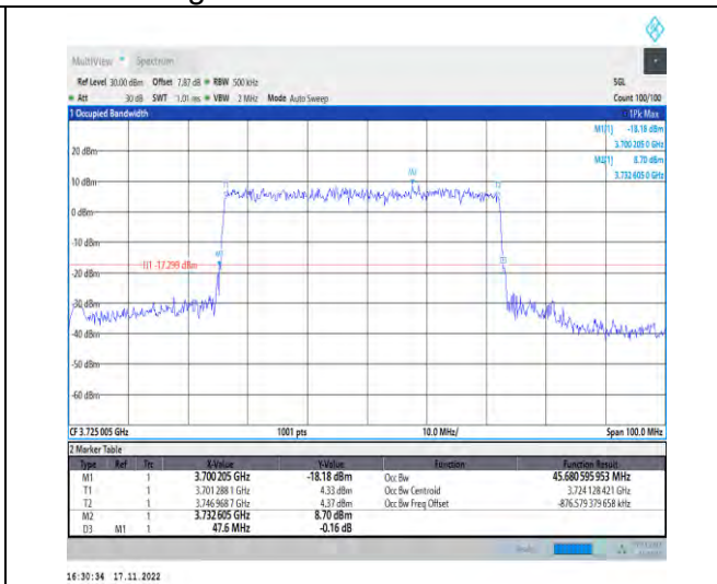
1-N78-3700-3800-PC2-30-50-L-3-DFT-16QAM-Outer_Full-128@0-Ant1-45.681-47.600-≤50-PASS
