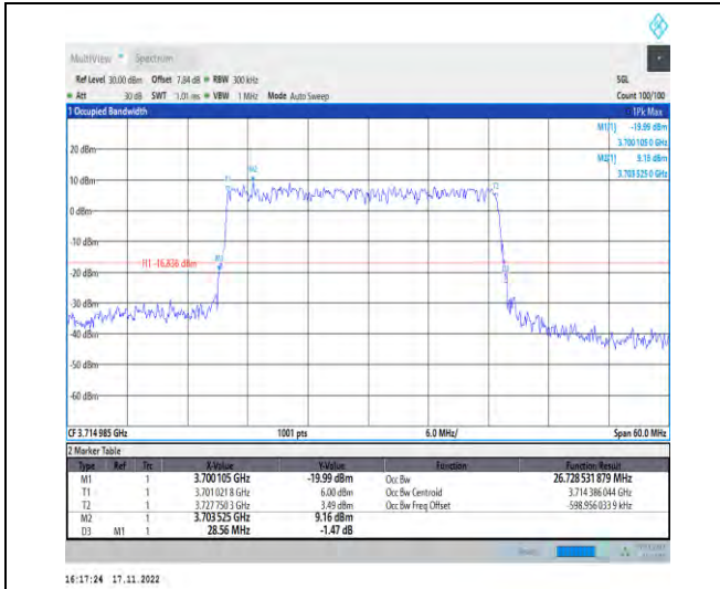
1-N78-3700-3800-PC2-30-30-L-4-DFT-64QAM-Outer_Full-75@0-Ant1-26.729-28.560-≤30-PASS
