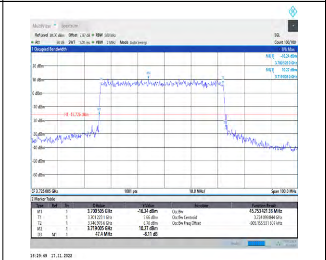
1-N78-3700-3800-PC2-30-50-L-1-DFT-QPSK-Outer_Full-128@0-Ant1-45.753-47.400-≤50-PASS
