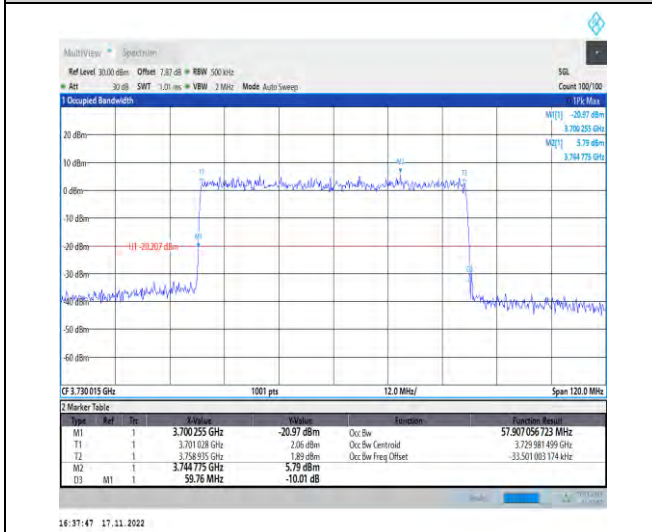
1-N78-3700-3800-PC2-30-60-L-5-DFT-256QAM-Outer_Full-162@0-Ant1-57.907-59.760-≤60-PASS
