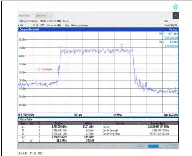
1-N78-3700-3800-PC2-30-30-M-3-DFT-16QAM-Out er_Full-75@0-Ant1-26.825-28.500-≤30-PASS
