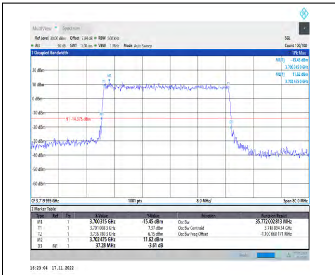
1-N78-3700-3800-PC2-30-40-L-1-DFT-QPSK-Outer_Full-100@0-Ant1-35.772-37.280-≤40-PASS
