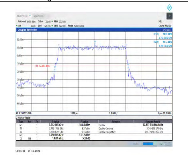
1-N78-3700-3800-PC2-30-15-M-2-DFT-PI2BPSK-Outer_Full-36@0-Ant1-12.897-14.070-≤15-PASS
