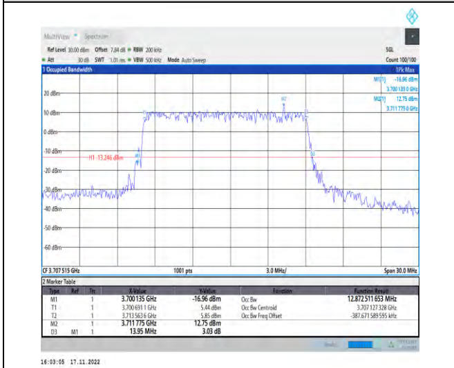
1-N78-3700-3800-PC2-30-15-L-4-DFT-64QAM-Outer_Full-36@0-Ant1-12.873-13.950-≤15-PASS
