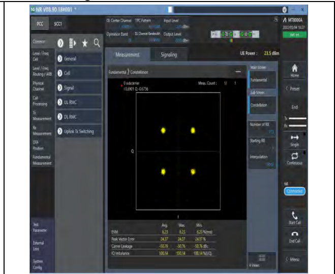
1-N78-3700-3800--30-100-M-6-CP-QPSK-Outer_Fu II-273@0-Ant1-see graph-PASS
