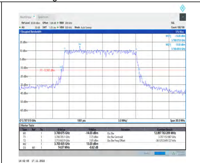
1-N78-3700-3800-PC2-30-15-L-3-DFT-16QAM-Outer_Full-36@0-Ant1-12.898-14.070-≤15-PASS
