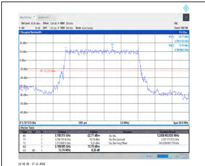
1-N78-3700-3800-PC2-30-15-L-2-DFT-PI2BPSK-Out er_Full-36@0-Ant1-12.858-13.740-≤15-PASS
