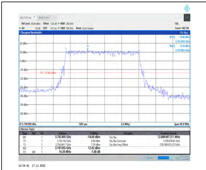
1-N78-3700-3800-PC2-30-15-M-1-DFT-QPSK-Outer_Full-36@0-Ant1-12.85-14.340-≤15-PASS
