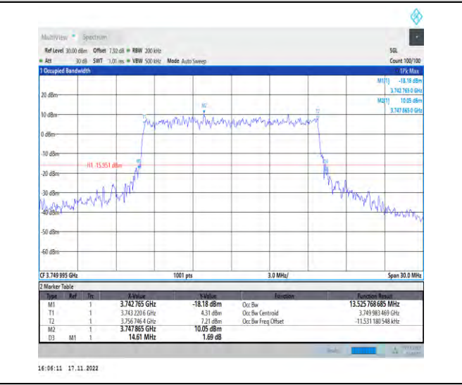
1-N78-3700-3800-PC2-30-15-M-8-CP-64QAM-Outer_Full-38@0-Ant1-13.526-14.610-≤15-PASS
