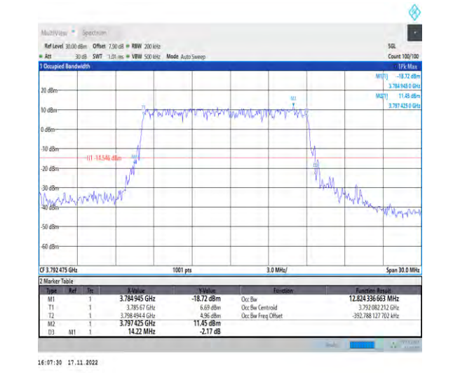
1-N78-3700-3800-PC2-30-15-H-3-DFT-16QAM-Outer_Full-36@0-Ant1-12.824-14.220-≤15-PASS
