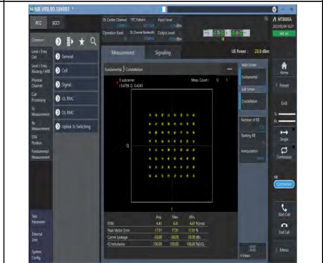
1-N78-3700-3800--30-100-M-8-CP-64QAM-Outer_Fu ull-273@0-Ant1-see graph-PASS
