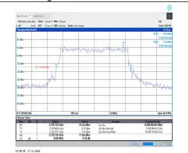
1-N78-3700-3800-PC2-30-10-M-1-DFT-QPSK-Outer_Full-24@0-Ant1-8.59-9.640-≤10-PASS
