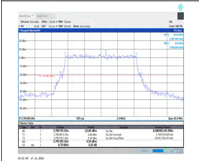
1-N78-3700-3800-PC2-30-10-H-9-CP-256QAM-Outer_Full-24@0-Ant1-8.589-9.740-≤10-PASS
