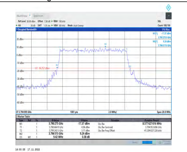
1-N78-3700-3800-PC2-30-10-H-4-DFT-64QAM-Outer_Full-24@0-Ant1-8.578-9.420-≤10-PASS
