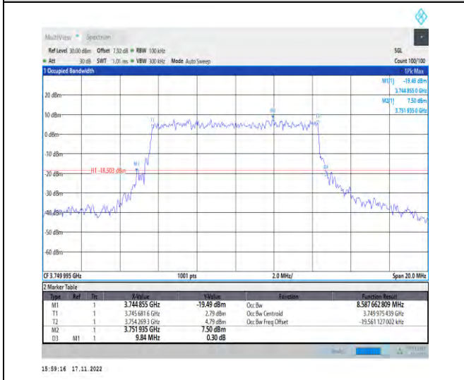
1-N78-3700-3800-PC2-30-10-M-6-CP-QPSK-Outer Full-24@0-Ant1-8.588-9.840-≤10-PASS
