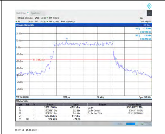
1-N78-3700-3800-PC2-30-10-L-8-CP-64QAM-Outer_Full-24@0-Ant1-8.565-9.540-≤10-PASS
