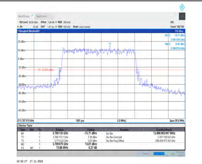
1-N78-3700-3800-PC2-30-15-L-1-DFT-QPSK-Outer_Full-36@0-Ant1-12.807-13.860-≤15-PASS
