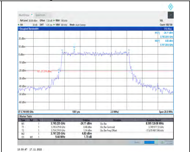
1-N78-3700-3800-PC2-30-10-M-9-CP-256QAM-Outer_Full-24@0-Ant1-8.595-9.440-≤10-PASS
