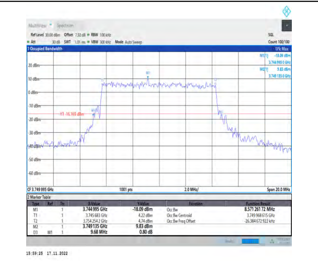
1-N78-3700-3800-PC2-30-10-M-7-CP-16QAM-Outer Full-24@0-Ant1-8.571-9.680-≤10-PASS
