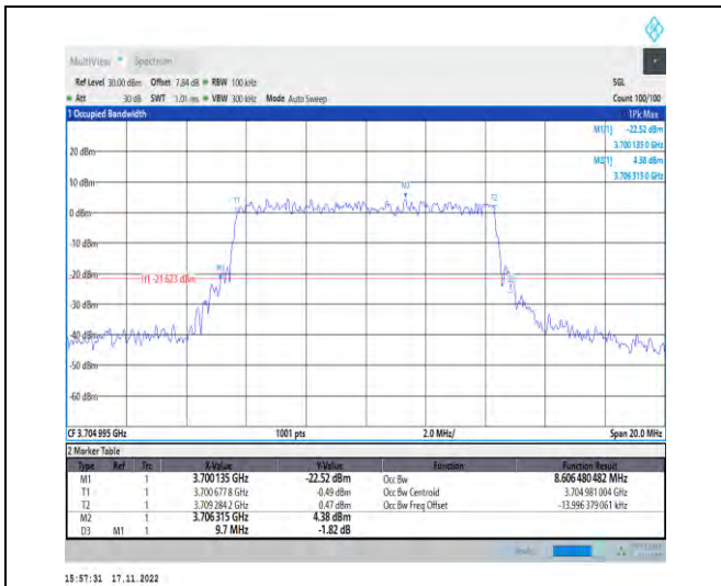
1-N78-3700-3800-PC2-30-10-L-9-CP-256QAM-Outer_Full-24@0-Ant1-8.606-9.700-≤10-PASS
