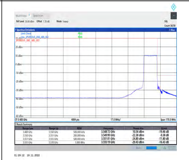
1-N78-3450-3550-PC2-30-15-H-6-CP-QPSK-Outer_Full-38@0-Ant1-1--PASS-see graph
