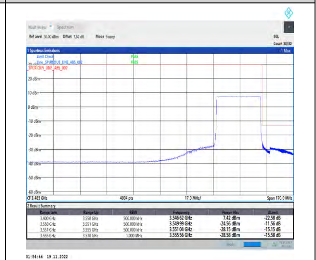
1-N78-3450-3550-PC2-30-30-H-6-CP-QPSK-Outer_Full-78@0-Ant1-1--PASS-see graph
