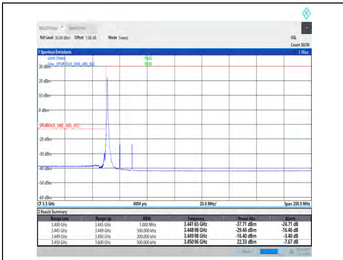
1-N78-3450-3550-PC2-30-20-L-4-CP-QPSK-Edge_1R_B_Left-1@0-Ant1-1--PASS-see graph
