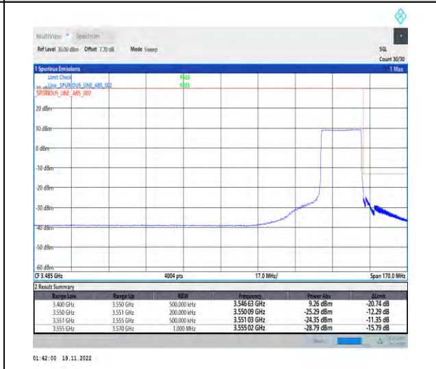
1-N78-3450-3550-PC2-30-20-H-6-CP-QPSK-Outer_Full-51@0-Ant1-1--PASS-see graph
