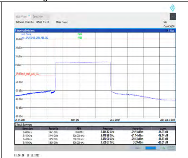
1-N78-3450-3550-PC2-30-70-L-6-CP-QPSK-Outer_Full-189@0-Ant1-1--PASS-see graph
