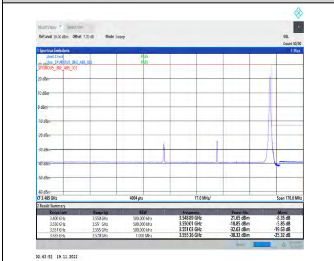
1-N78-3450-3550-PC2-30-70-H-5-CP-QPSK-Edge_1R_B_Right-1@188-Ant1-1--PASS-see graph
