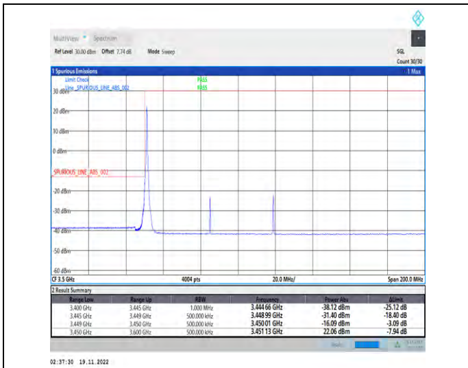
1-N78-3450-3550-PC2-30-70-L-4-CP-QPSK-Edge_1R_B_Left-1@0-Ant1-1--PASS-see graph
