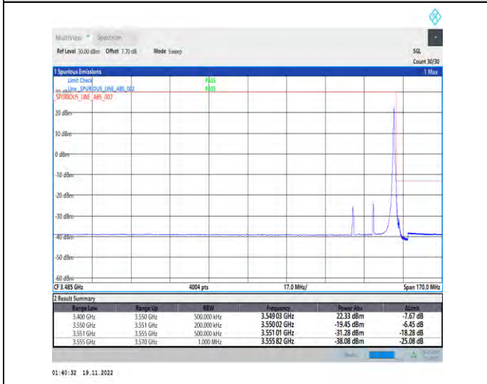
1-N78-3450-3550-PC2-30-20-H-5-CP-QPSK-Edge_1R_B_Right-1@50-Ant1-1--PASS-see graph
