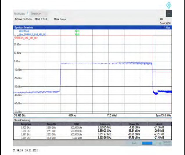
1-N78-3450-3550-PC2-30-100-H-6-CP-QPSK-Outer_Full-273@0-Ant1-1--PASS-see graph
