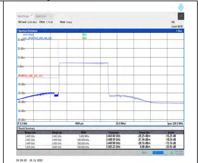
1-N78-3450-3550-PC2-30-60-L-6-CP-QPSK-Outer_Full-162@0-Ant1-1--PASS-see graph
