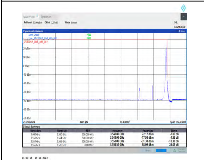
1-N78-3450-3550-PC2-30-30-H-5-CP-QPSK-Edge_1R_B_Right-1@77-Ant1-1--PASS-see graph
