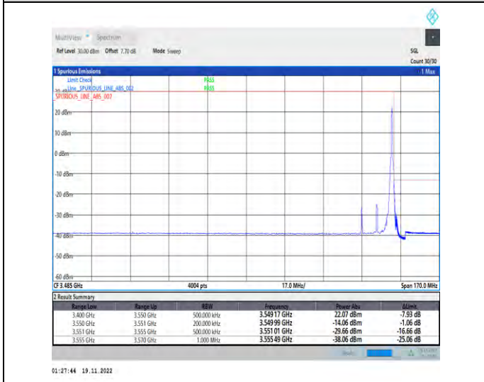
1-N78-3450-3550-PC2-30-15-H-5-CP-QPSK-Edge_1R_B_Right-1@37-Ant1-1--PASS-see graph
