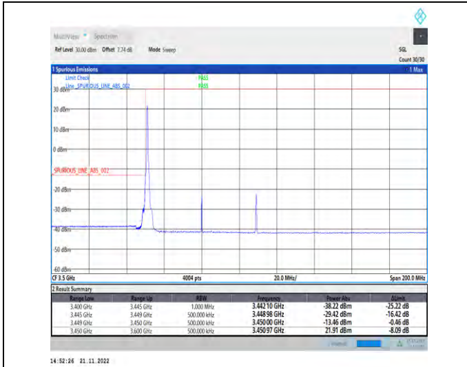
1-N78-3450-3550-PC2-30-60-L-4-CP-QPSK-Edge_1R_B_Left-1@0-Ant1-1--PASS-see graph
