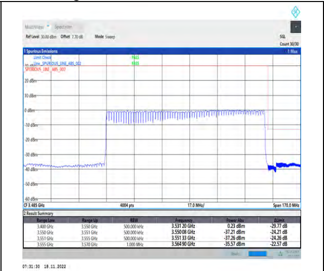
1-N78-3450-3550-PC2-30-100-H-3-DFT-PI2BPSK-Outer_Full-270@0-Ant1-1--PASS-see graph
