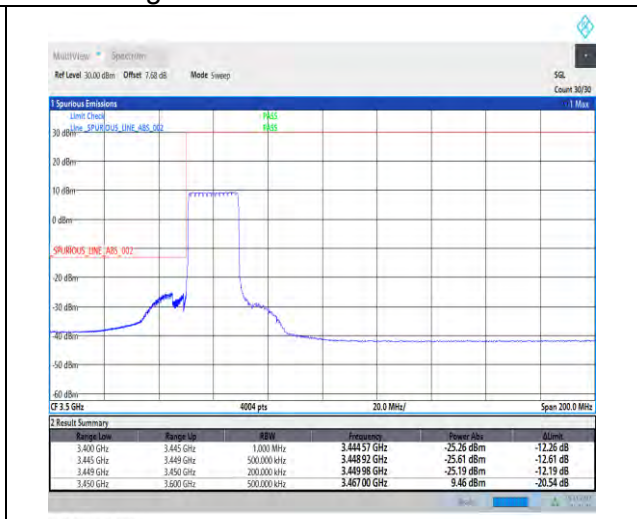
1-N78-3450-3550-PC2-30-20-L-6-CP-QPSK-Outer_Full-51@0-Ant1-1--PASS-see graph
