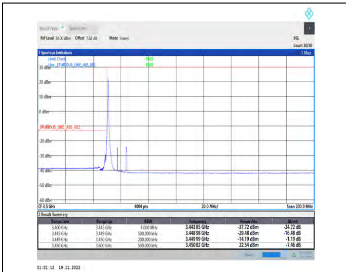
1-N78-3450-3550-PC2-30-15-L-4-CP-QPSK-Edge_1R_B_Left-1@0-Ant1-1--PASS-see graph
