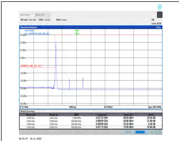
1-N78-3450-3550-PC2-30-40-L-1-DFT-PI2BPSK-Edge_1RB_Left-1@0-Ant1-1--PASS-see graph
