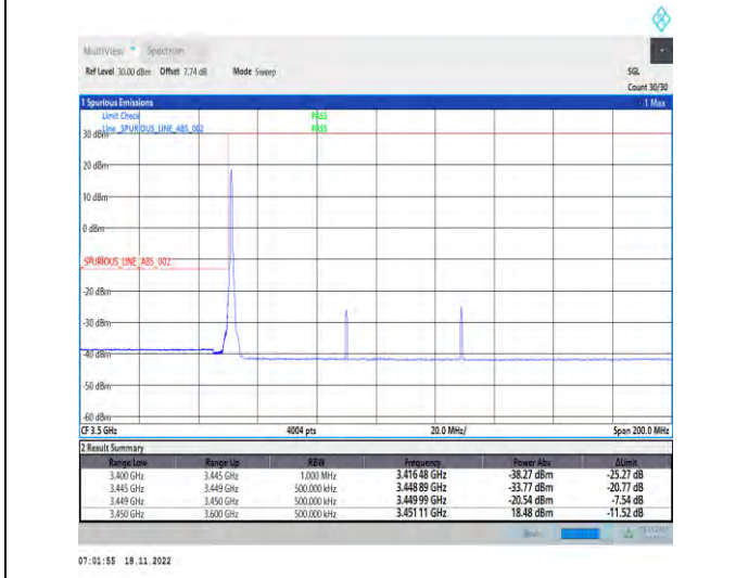
1-N78-3450-3550-PC2-30-80-L-4-CP-QPSK-Edge_1RB_Left-1@0-Ant1-1--PASS-see graph
