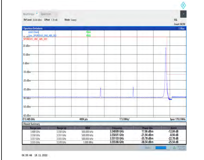
1-N78-3450-3550-PC2-30-70-H-5-CP-QPSK-Edge_1RB_Right-1@188-Ant1-1--PASS-see graph
