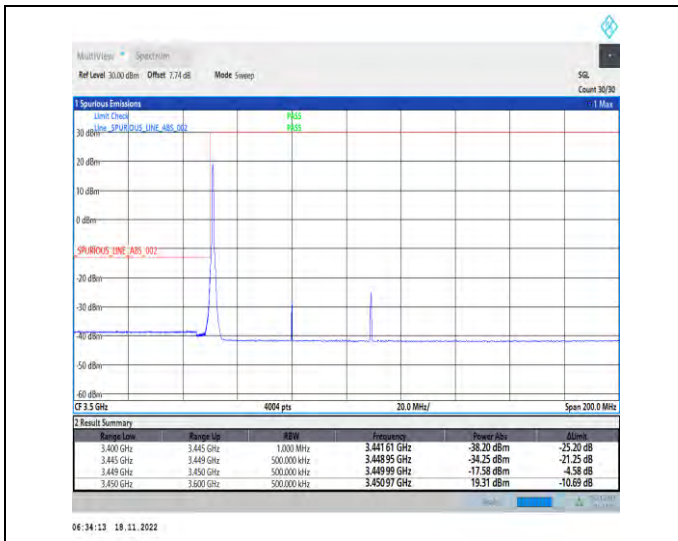
1-N78-3450-3550-PC2-30-60-L-1-DFT-PI2BPSK-Edge_1RB_Left-1@0-Ant1-1--PASS-see graph
