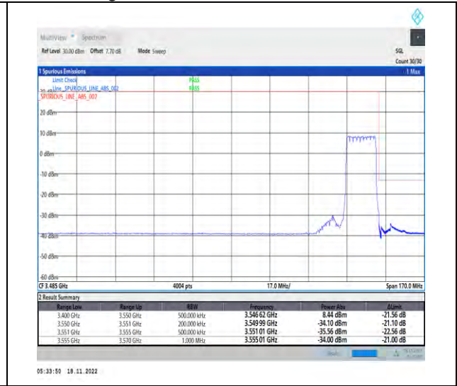
1-N78-3450-3550-PC2-30-15-H-3-DFT-PI2BPSK-Outer_Full-36@0-Ant1-1--PASS-see graph
