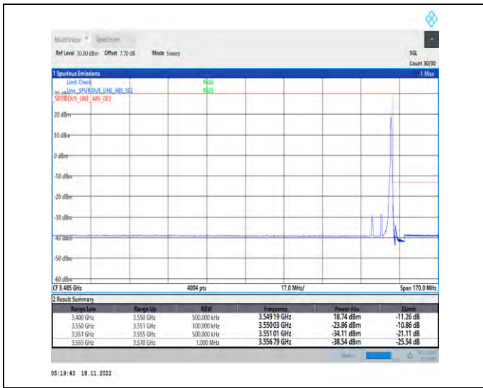
1-N78-3450-3550-PC2-30-10-H-2-DFT-PI2BPSK-Edge_1RB_Right-1@23-Ant1-1--PASS-see graph
