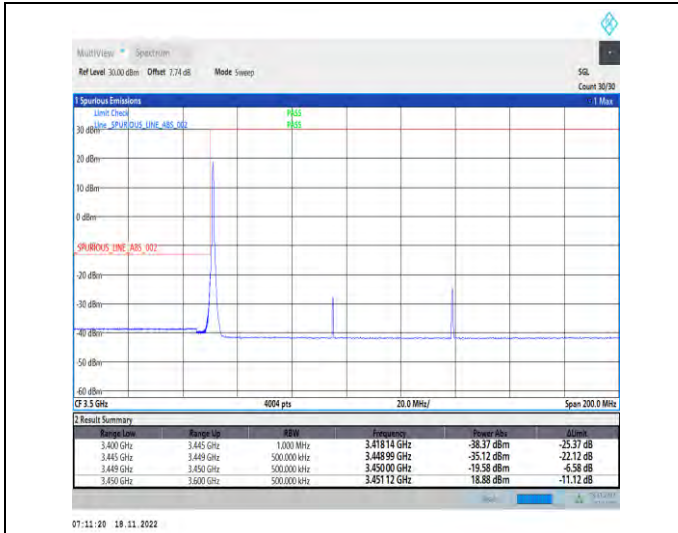
1-N78-3450-3550-PC2-30-90-L-1-DFT-PI2BPSK-Edge_1RB_Left-1@0-Ant1-1--PASS-see graph
