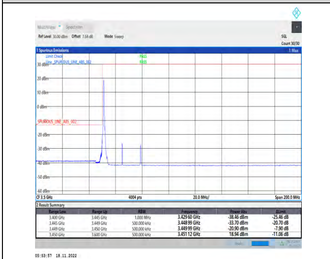
1-N78-3450-3550-PC2-30-30-L-4-CP-QPSK-Edge_1RB_Left-1@0-Ant1-1--PASS-see graph
