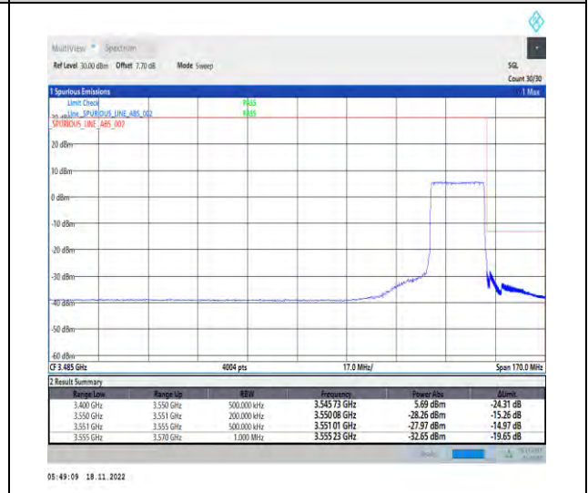
1-N78-3450-3550-PC2-30-20-H-6-CP-QPSK-Outer_Full-51@0-Ant1-1--PASS-see graph
