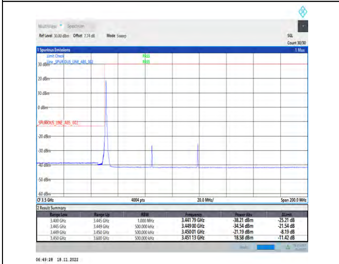
1-N78-3450-3550-PC2-30-70-L-4-CP-QPSK-Edge_1RB_Left-1@0-Ant1-1--PASS-see graph
