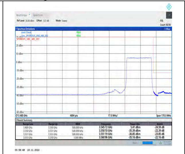
1-N78-3450-3550-PC2-30-30-H-3-DFT-PI2BPSK-Outer_Full-75@0-Ant1-1--PASS-see graph
