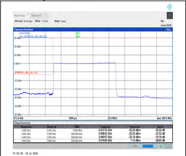
1-N78-3450-3550-PC2-30-80-L-3-DFT-PI2BPSK-Outer_Full-216@0-Ant1-1--PASS-see graph
