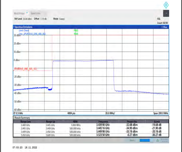
1-N78-3450-3550-PC2-30-80-L-6-CP-QPSK-Outer_Full-217@0-Ant1-1--PASS-see graph
