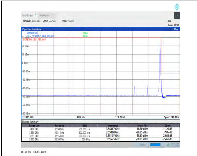
1-N78-3450-3550-PC2-30-30-H-2-DFT-PI2BPSK-Edge_1RB_Right-1@77-Ant1-1--PASS-see graph
