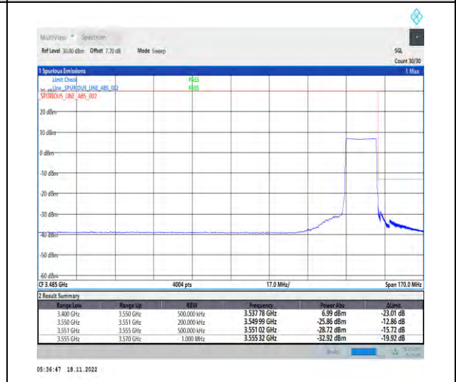
1-N78-3450-3550-PC2-30-15-H-6-CP-QPSK-Outer_Full-38@0-Ant1-1--PASS-see graph
