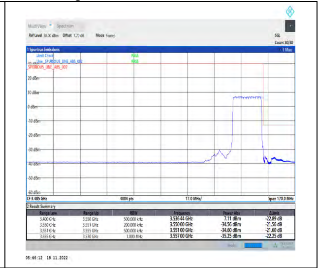
1-N78-3450-3550-PC2-30-20-H-3-DFT-PI2BPSK-Outer_Full-50@0-Ant1-1--PASS-see graph
