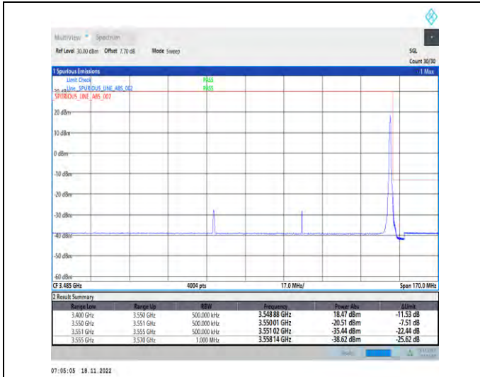
1-N78-3450-3550-PC2-30-80-H-2-DFT-PI2BPSK-Edge_1RB_Right-1@216-Ant1-1--PASS-see graph
