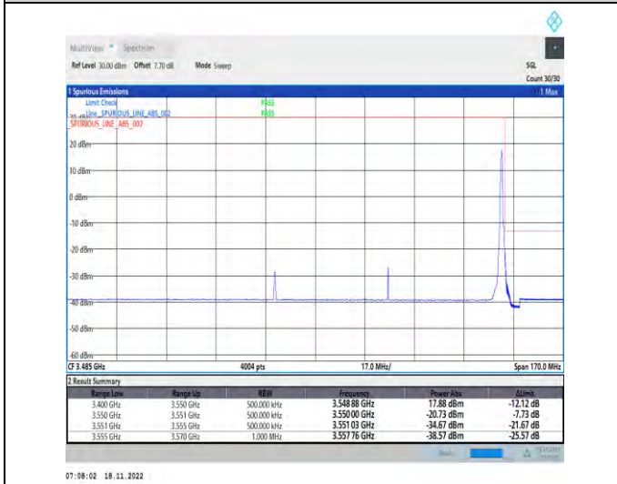
1-N78-3450-3550-PC2-30-80-H-5-CP-QPSK-Edge_1RB_Right-1@216-Ant1-1--PASS-see graph
