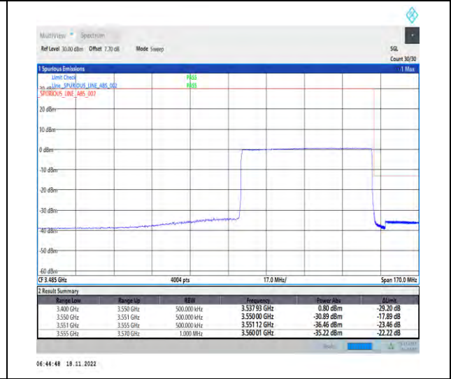
1-N78-3450-3550-PC2-30-60-H-6-CP-QPSK-Outer_Full-162@0-Ant1-1--PASS-see graph
