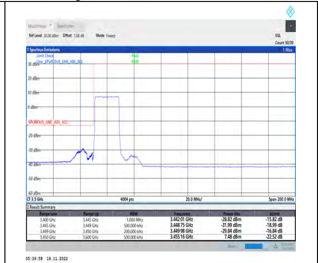
1-N78-3450-3550-PC2-30-20-L-3-DFT-PI2BPSK-Outer_Full-50@0-Ant1-1--PASS-see graph
