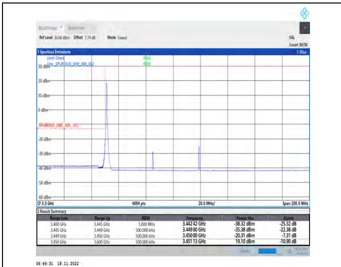
1-N78-3450-3550-PC2-30-70-L-1-DFT-PI2BPSK-Edge_1RB_Left-1@0-Ant1-1--PASS-see graph
