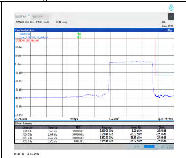
1-N78-3450-3550-PC2-30-50-H-3-DFT-PI2BPSK-Outer_Full-128@0-Ant1-1--PASS-see graph
