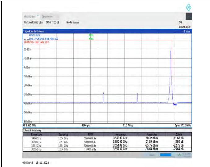
1-N78-3450-3550-PC2-30-70-H-2-DFT-PI2BPSK-Edge_1RB_Right-1@188-Ant1-1--PASS-see graph
