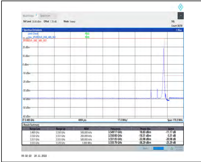
1-N78-3450-3550-PC2-30-15-H-2-DFT-PI2BPSK-Edge_1RB_Right-1@37-Ant1-1--PASS-see graph
