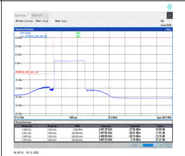
1-N78-3450-3550-PC2-30-40-L-6-CP-QPSK-Outer_Full-106@0-Ant1-1--PASS-see graph
