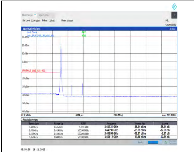
1-N78-3450-3550-PC2-30-30-L-1-DFT-PI2BPSK-Edge_1RB_Left-1@0-Ant1-1--PASS-see graph
