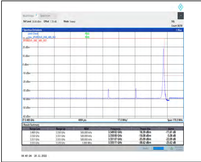
1-N78-3450-3550-PC2-30-60-H-2-DFT-PI2BPSK-Edge_1RB_Right-1@161-Ant1-1--PASS-see graph
