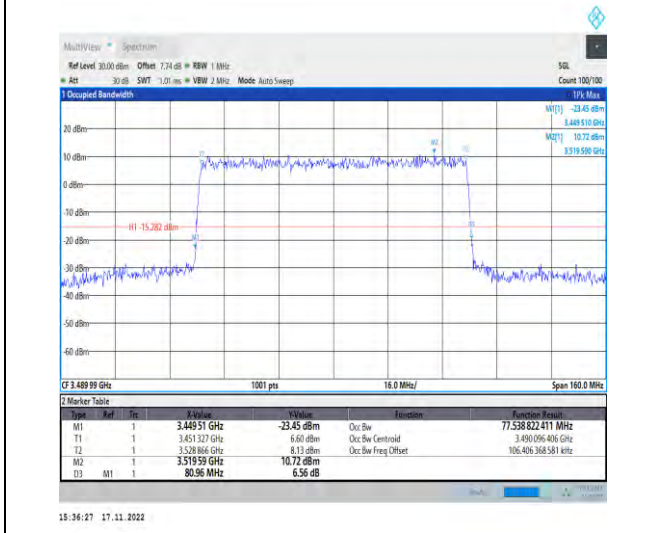
1-N78-3450-3550-PC2-30-80-L-7-CP-16QAM-Outer_Full-217@0-Ant1-77.539-80.960-<=80-PASS
