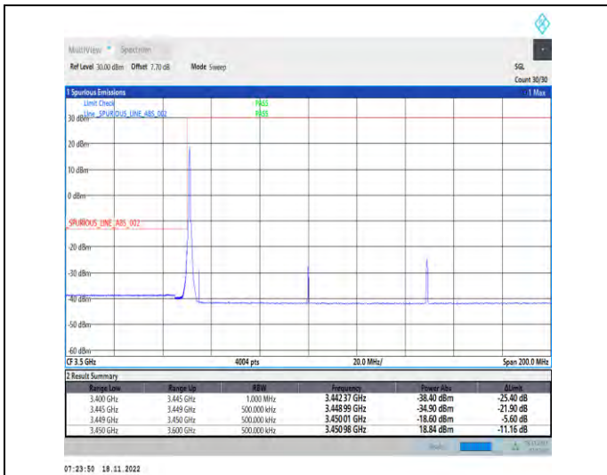
1-N78-3450-3550-PC2-30-100-L-1-DFT-PI2BPSK-Edge_1_RB_Left-1@0-Ant1-1--PASS-see graph
