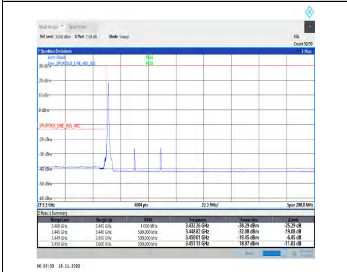
1-N78-3450-3550-PC2-30-40-L-4-CP-QPSK-Edge_1RB_Left-1@0-Ant1-1--PASS-see graph
