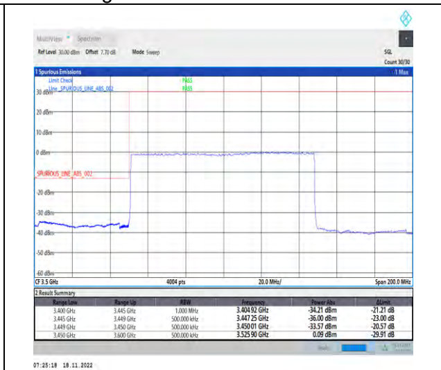
1-N78-3450-3550-PC2-30-100-L-3-DFT-PI2BPSK-Outer_Full-270@0-Ant1-1--PASS-see graph
