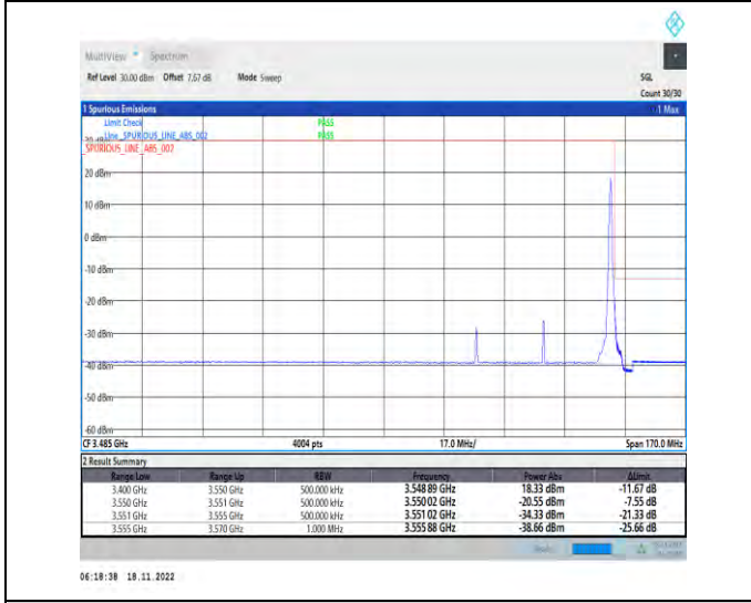
1-N78-3450-3550-PC2-30-40-H-5-CP-QPSK-Edge_1RB_Right-1@105-Ant1-1--PASS-see graph
