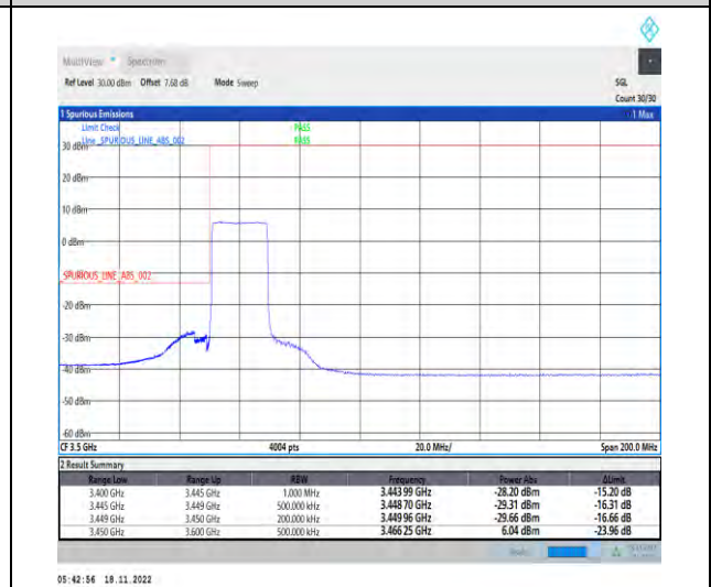
1-N78-3450-3550-PC2-30-20-L-6-CP-QPSK-Outer_Full-51@0-Ant1-1--PASS-see graph
