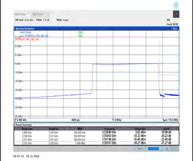
1-N78-3450-3550-PC2-30-70-H-6-CP-QPSK-Outer_Full-189@0-Ant1-1--PASS-see graph
