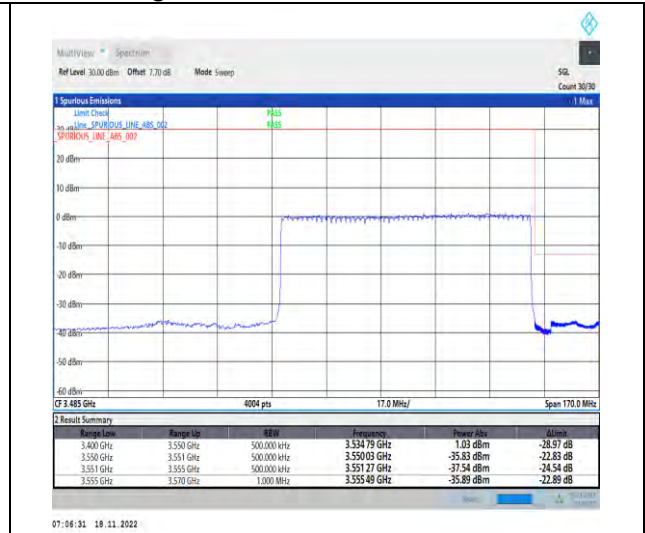
1-N78-3450-3550-PC2-30-80-H-3-DFT-PI2BPSK-Outer_Full-216@0-Ant1-1--PASS-see graph
