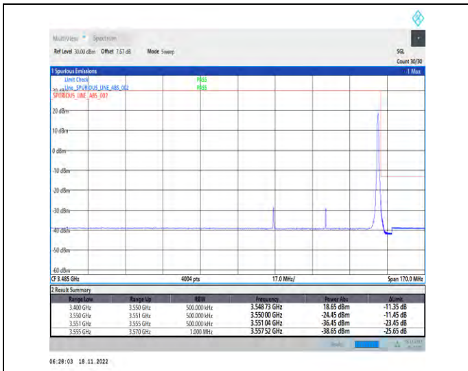
1-N78-3450-3550-PC2-30-50-H-2-DFT-PI2BPSK-Edge_1RB_Right-1@132-Ant1-1--PASS-see graph
