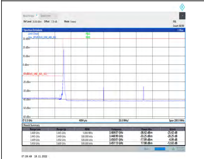
1-N78-3450-3550-PC2-30-100-L-4-CP-QPSK-Edge_1_RB_Left-1@0-Ant1-1--PASS-see graph
