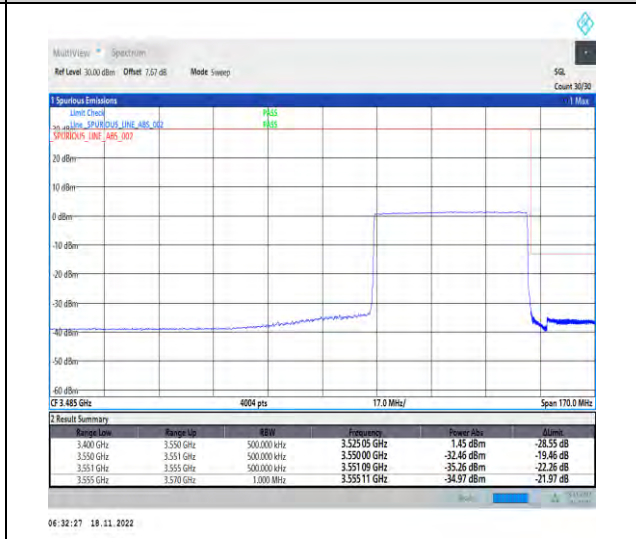
1-N78-3450-3550-PC2-30-50-H-6-CP-QPSK-Outer_Full-133@0-Ant1-1--PASS-see graph
