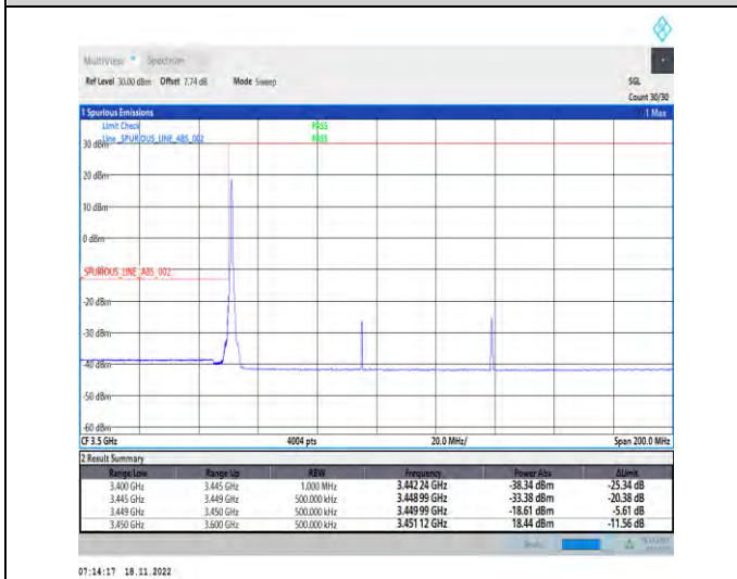
1-N78-3450-3550-PC2-30-90-L-4-CP-QPSK-Edge_1RB_Left-1@0-Ant1-1--PASS-see graph
