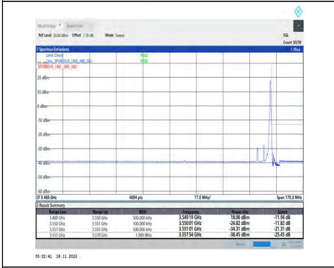
1-N78-3450-3550-PC2-30-10-H-5-CP-QPSK-Edge_1RB_Right-1@23-Ant1-1--PASS-see graph
