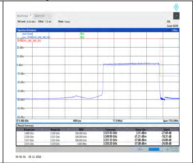
1-N78-3450-3550-PC2-30-60-H-3-DFT-PI2BPSK-Outer_Full-162@0-Ant1-1--PASS-see graph
