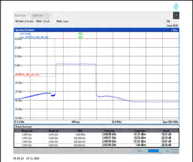
1-N78-3450-3550-PC2-30-50-L-6-CP-QPSK-Outer_Full-133@0-Ant1-1--PASS-see graph
