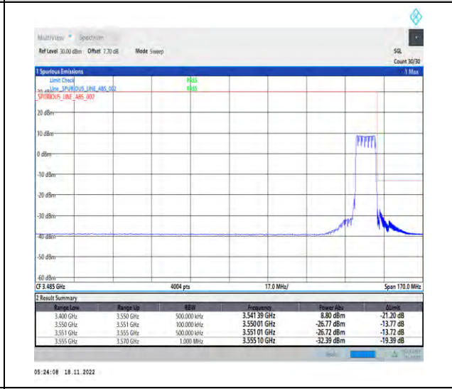
1-N78-3450-3550-PC2-30-10-H-6-CP-QPSK-Outer_Full-24@0-Ant1-1--PASS-see graph
