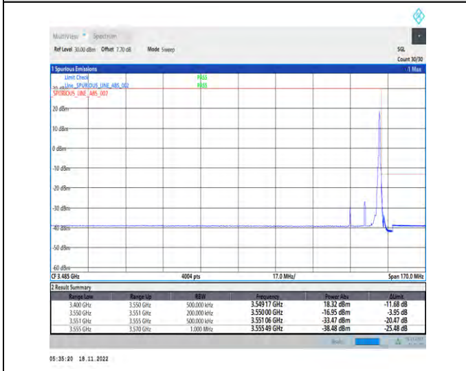
1-N78-3450-3550-PC2-30-15-H-5-CP-QPSK-Edge_1RB_Right-1@37-Ant1-1--PASS-see graph
