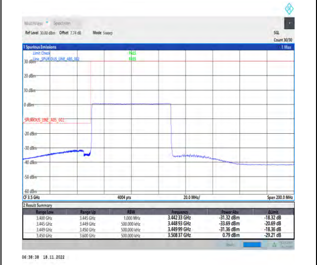
1-N78-3450-3550-PC2-30-60-L-6-CP-QPSK-Outer_Full-162@0-Ant1-1--PASS-see graph
