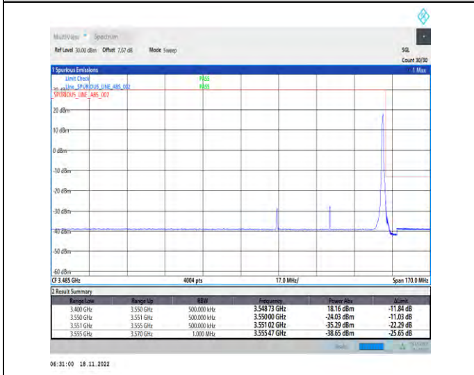
1-N78-3450-3550-PC2-30-50-H-5-CP-QPSK-Edge_1RB_Right-1@132-Ant1-1--PASS-see graph
