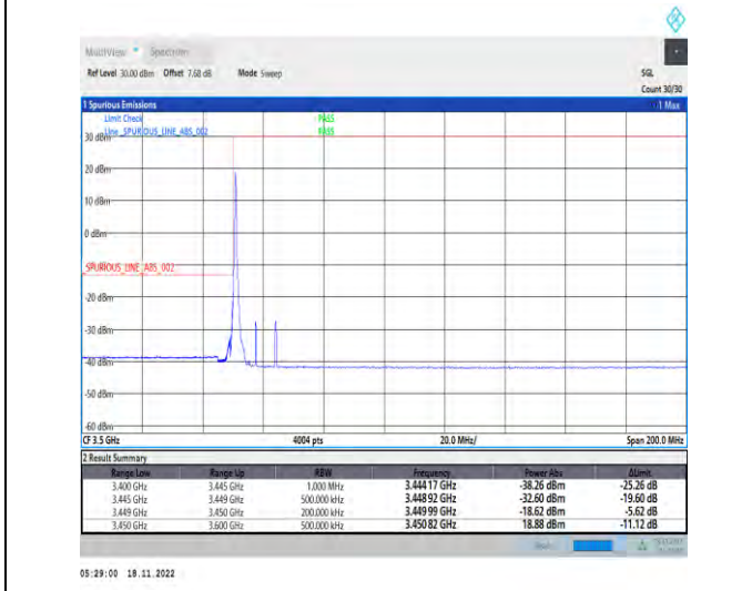
1-N78-3450-3550-PC2-30-15-L-4-CP-QPSK-Edge_1RB_Left-1@0-Ant1-1--PASS-see graph
