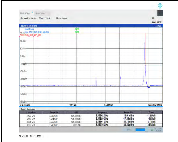
1-N78-3450-3550-PC2-30-60-H-5-CP-QPSK-Edge_1RB_Right-1@161-Ant1-1--PASS-see graph
