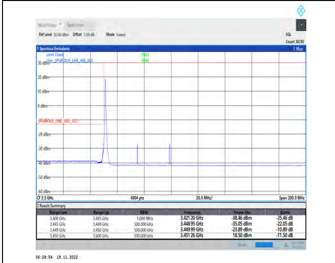
1-N78-3450-3550-PC2-30-50-L-4-CP-QPSK-Edge_1RB_Left-1@0-Ant1-1--PASS-see graph
