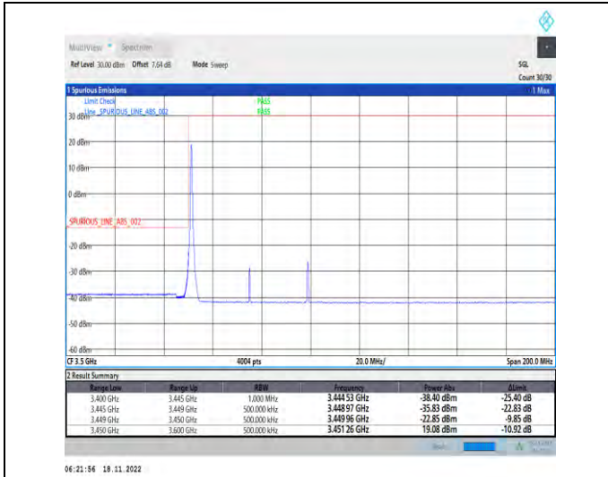
1-N78-3450-3550-PC2-30-50-L-1-DFT-PI2BPSK-Edge_1RB_Left-1@0-Ant1-1--PASS-see graph
