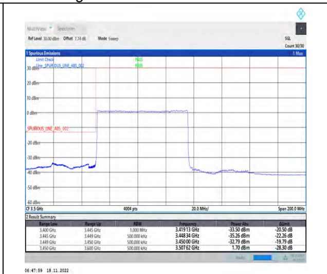
1-N78-3450-3550-PC2-30-70-L-3-DFT-PI2BPSK-Outer_Full-180@0-Ant1-1--PASS-see graph
