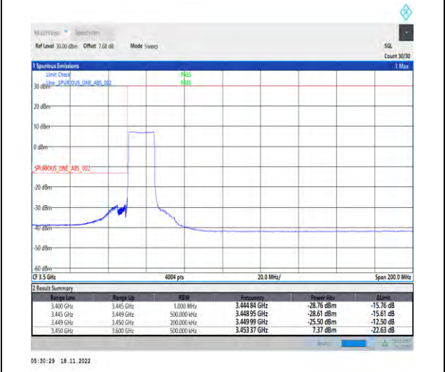
1-N78-3450-3550-PC2-30-15-L-6-CP-QPSK-Outer_Full-38@0-Ant1-1--PASS-see graph
