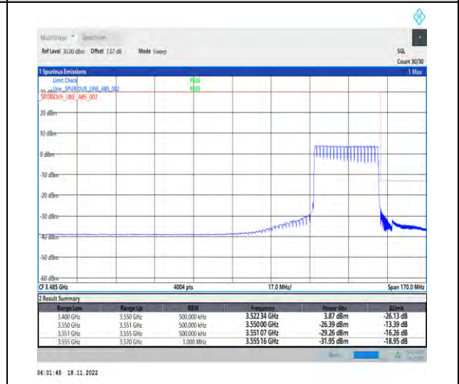
1-N78-3450-3550-PC2-30-30-H-6-CP-QPSK-Outer_Full-78@0-Ant1-1--PASS-see graph
