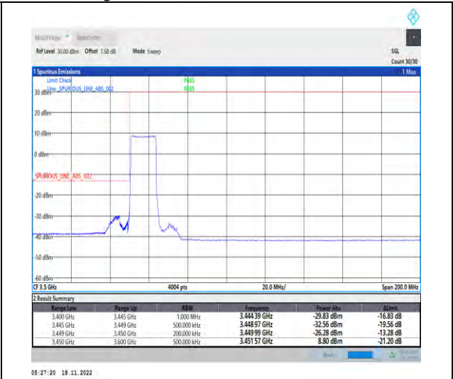
1-N78-3450-3550-PC2-30-15-L-3-DFT-PI2BPSK-Outer_Full-36@0-Ant1-1--PASS-see graph
