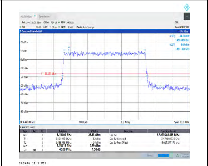
1-N78-3450-3550-PC2-30-40-L-8-CP-64QAM-Outer_Full-106@0-Ant1-37.975-40.080-≤40-PASS
