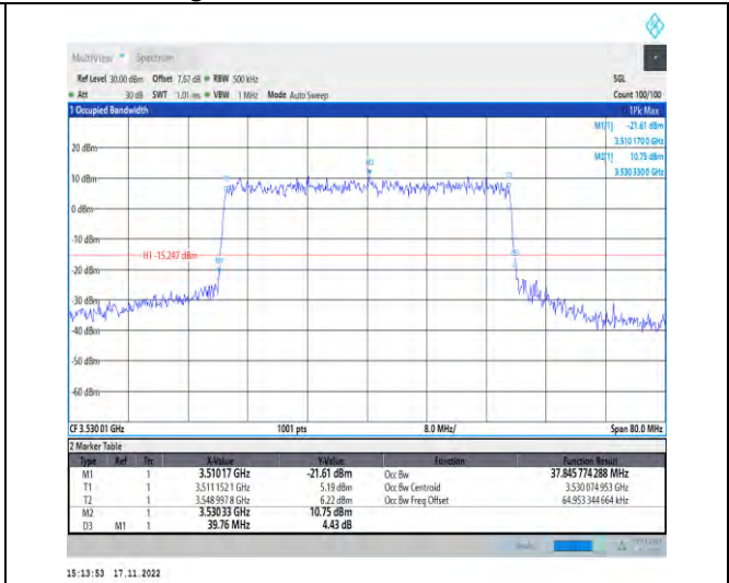
1-N78-3450-3550-PC2-30-40-H-8-CP-64QAM-Outer _Full-106@0-Ant1-37.846-39.760-≤40-PASS
