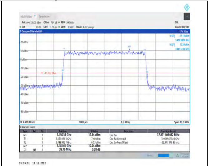
1-N78-3450-3550-PC2-30-40-L-6-CP-QPSK-Outer_Full-106@0-Ant1-37.891-39.760-≤40-PASS
