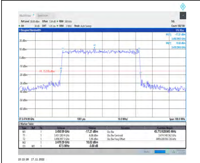
1-N78-3450-3550-PC2-30-50-L-4-DFT-64QAM-Outer _Full-128@0-Ant1-45.714-47.500-≤50-PASS
