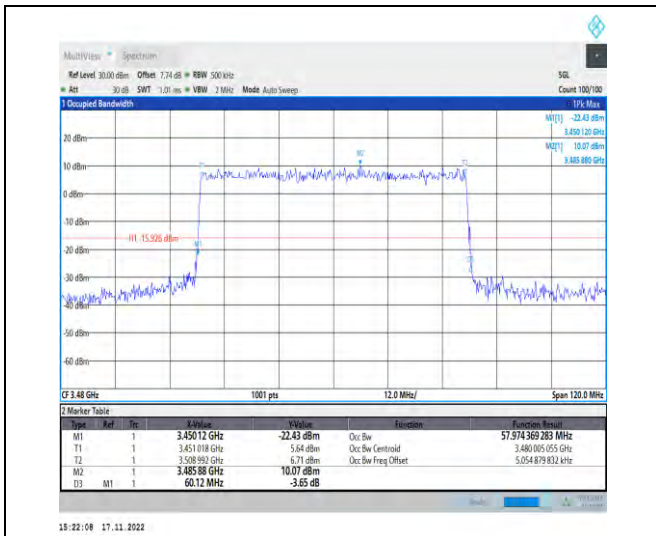
1-N78-3450-3550-PC2-30-60-L-3-DFT-16QAM-Outer_Full-162@0-Ant1-57.974-60.120-≤60-PASS
