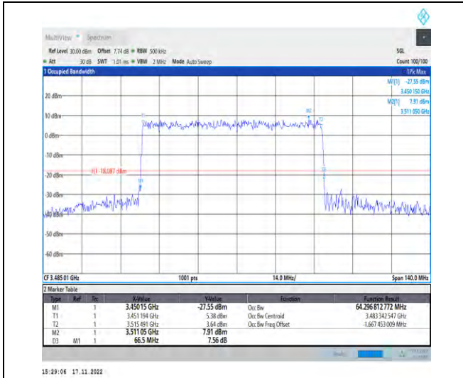
1-N78-3450-3550-PC2-30-70-L-4-DFT-64QAM-Outer_Full-180@0-Ant1-64.297-66.500-≤70-PASS
