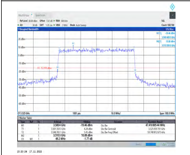
1-N78-3450-3550-PC2-30-50-H-6-CP-QPSK-Outer_Full-133@0-Ant1-47.411-49.200-≤50-PASS
