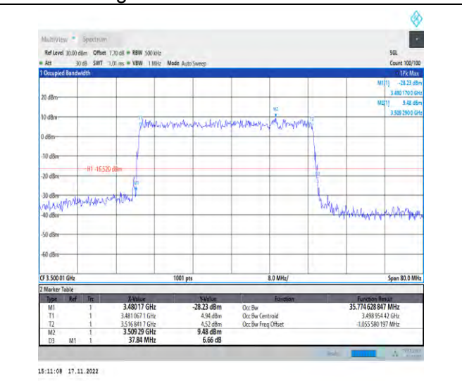
1-N78-3450-3550-PC2-30-40-M-5-DFT-256QAM-Out er_Full-100@0-Ant1-35.775-37.840-≤40-PASS
