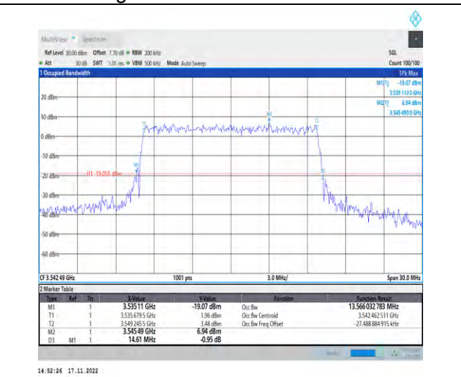
1-N78-3450-3550-PC2-30-15-H-9-CP-256QAM-Outer_Full-38@0-Ant1-13.566-14.610-≤15-PASS
