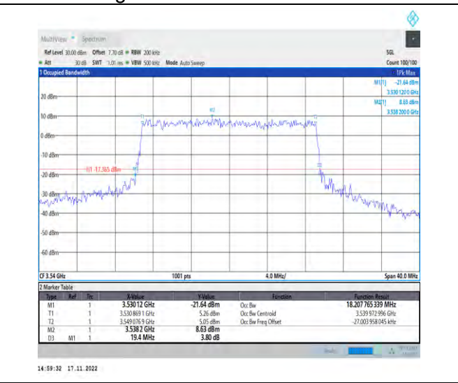
1-N78-3450-3550-PC2-30-20-H-6-CP-QPSK-Outer_Full-51@0-Ant1-18.208-19.400-≤20-PASS
