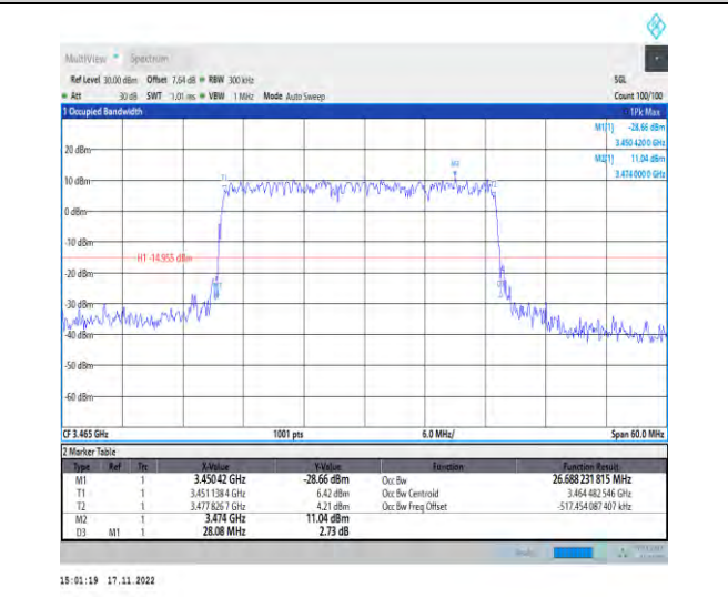
1-N78-3450-3550-PC2-30-30-L-3-DFT-16QAM-Outer_Full-75@0-Ant1-26.688-28.080-≤30-PASS
