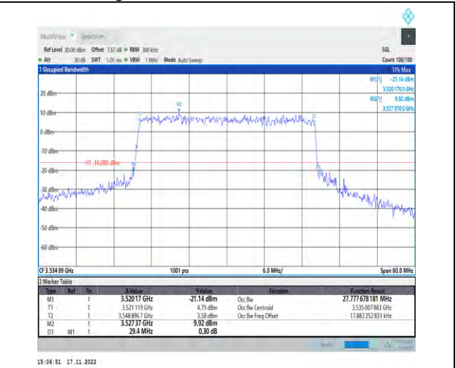
1-N78-3450-3550-PC2-30-30-H-7-CP-16QAM-Outer_Full-78@0-Ant1-27.778-29.400-≤30-PASS
