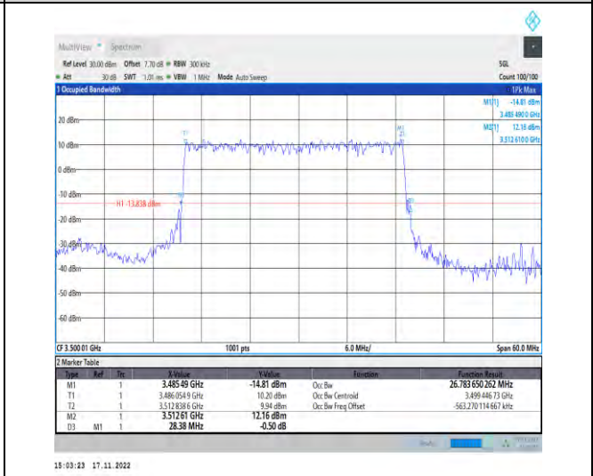
1-N78-3450-3550-PC2-30-30-M-2-DFT-PI2BPSK-Outer _Full-75@0-Ant1-26.784-28.380-≤30-PASS
