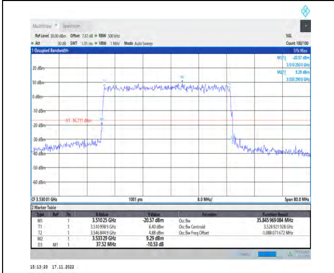
1-N78-3450-3550-PC2-30-40-H-5-DFT-256QAM-Outer_Full-100@0-Ant1-35.846-37.520-≤40-PASS
