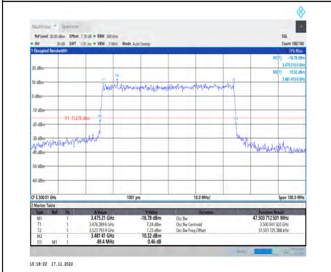
1-N78-3450-3550-PC2-30-50-M-7-CP-16QAM-Outer_Full-133@0-Ant1-47.504-49.400-≤50-PASS
