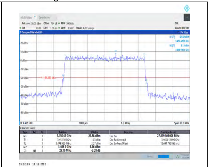
1-N78-3450-3550-PC2-30-30-L-9-CP-256QAM-Outer _Full-78@0-Ant1-27.819-29.160-≤30-PASS
