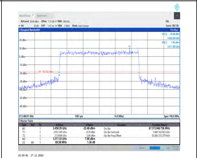
1-N78-3450-3550-PC2-30-70-L-7-CP-16QAM-Outer_Full-189@0-Ant1-67.515-69.580-≤70-PASS
