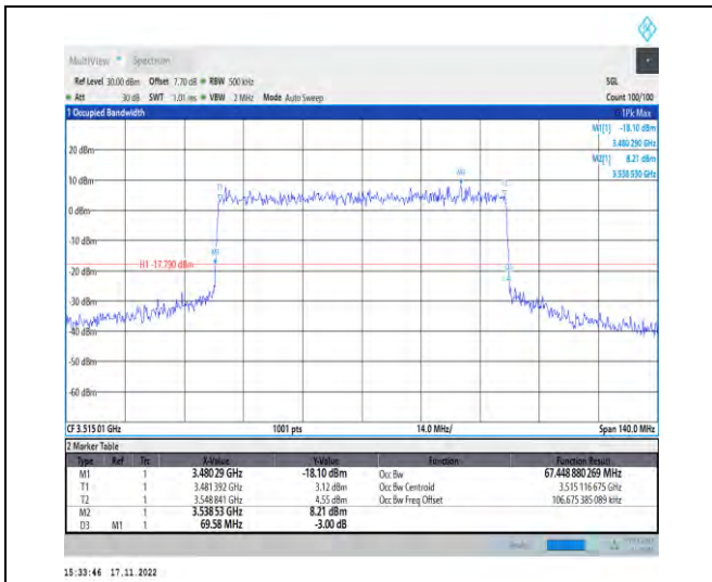
1-N78-3450-3550-PC2-30-70-H-6-CP-QPSK-Outer_Full-189@0-Ant1-67.449-69.580-≤70-PASS
