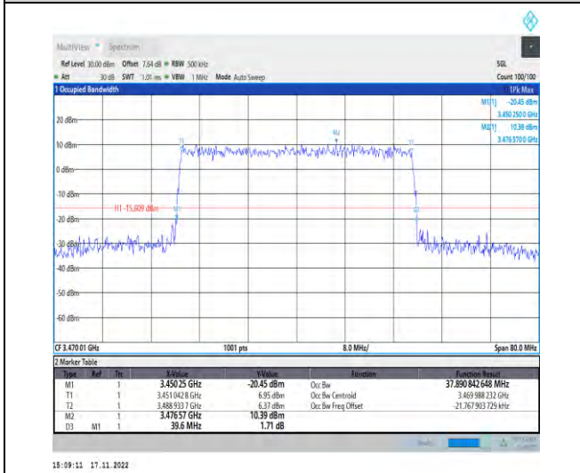
1-N78-3450-3550-PC2-30-40-L-7-CP-16QAM-Outer_Full-106@0-Ant1-37.891-39.600-≤40-PASS
