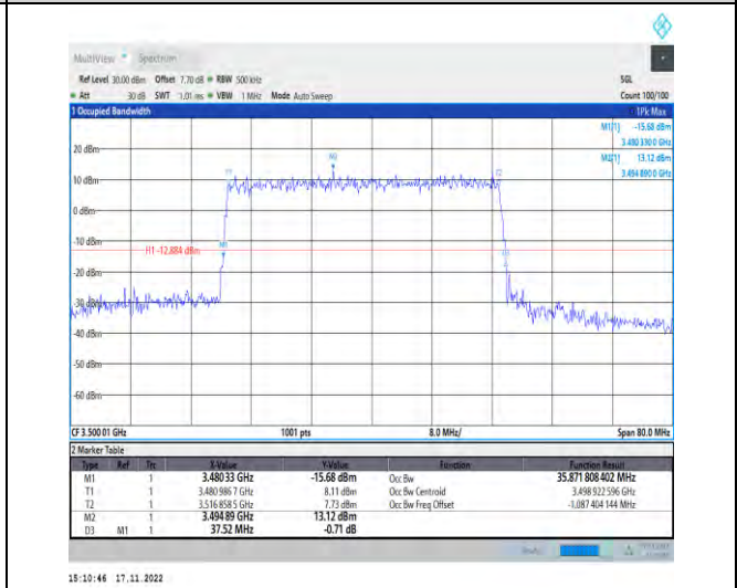
1-N78-3450-3550-PC2-30-40-M-3-DFT-16QAM-Outer_Full-100@0-Ant1-35.872-37.520-≤40-PASS
