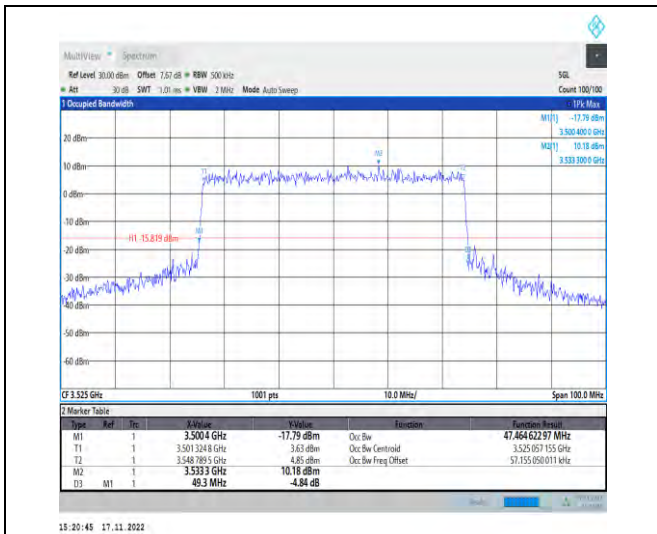
1-N78-3450-3550-PC2-30-50-H-8-CP-64QAM-Outer_Full-133@0-Ant1-47.465-49.300-≤50-PASS
