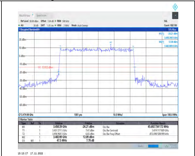
1-N78-3450-3550-PC2-30-50-L-3-DFT-16QAM-Outer _Full-128@0-Ant1-45.693-47.500-≤50-PASS
