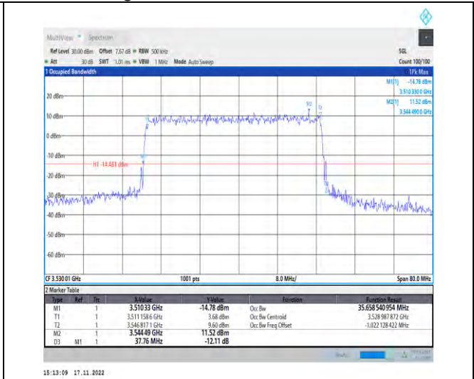
1-N78-3450-3550-PC2-30-40-H-4-DFT-64QAM-Outer_Full-100@0-Ant1-35.659-37.760-≤40-PASS
