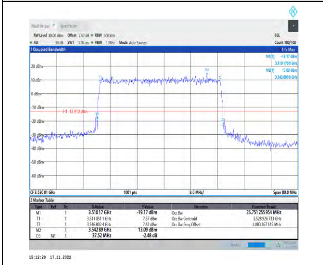
1-N78-3450-3550-PC2-30-40-H-1-DFT-QPSK-Outer_Full-100@0-Ant1-35.751-37.520-≤40-PASS
