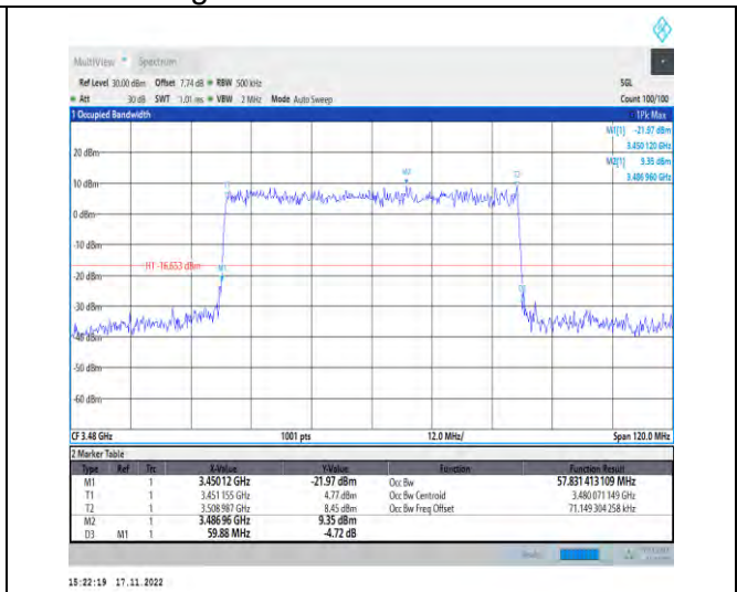
1-N78-3450-3550-PC2-30-60-L-4-DFT-64QAM-Outer_Full-162@0-Ant1-57.831-59.880-≤60-PASS
