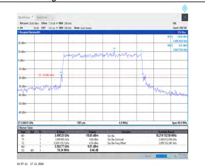
1-N78-3450-3550-PC2-30-20-M-7-CP-16QAM-Outer_Full-51@0-Ant1-18.214-19.240-≤20-PASS
