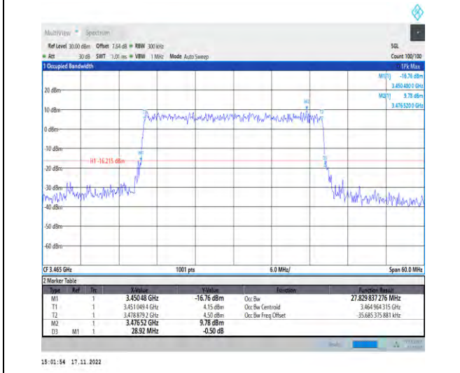
1-N78-3450-3550-PC2-30-30-L-6-CP-QPSK-Outer_Full-78@0-Ant1-27.83-28.920-≤30-PASS
