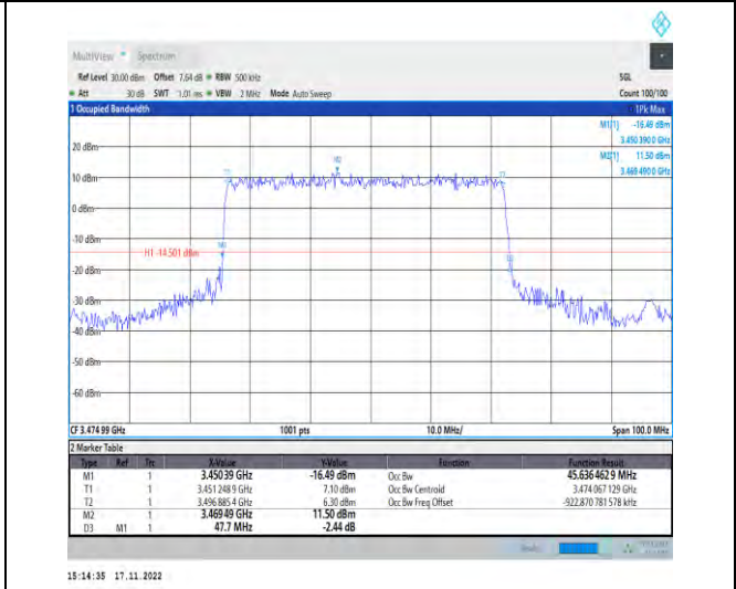
1-N78-3450-3550-PC2-30-50-L-1-DFT-QPSK-Outer _Full-128@0-Ant1-45.636-47.700-≤50-PASS
