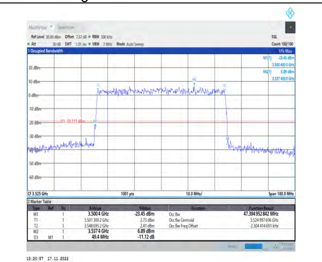
1-N78-3450-3550-PC2-30-50-H-9-CP-256QAM-Outer_Full-133@0-Ant1-47.395-49.400-≤50-PASS
