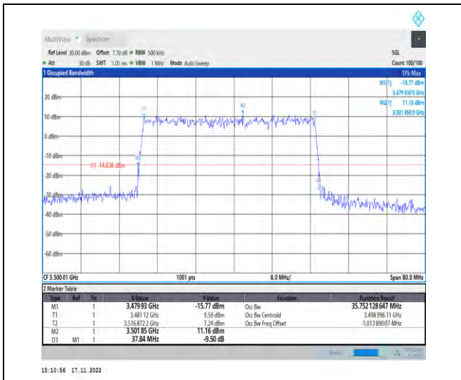
1-N78-3450-3550-PC2-30-40-M-4-DFT-64QAM-Out er_Full-100@0-Ant1-35.752-37.840-≤40-PASS
