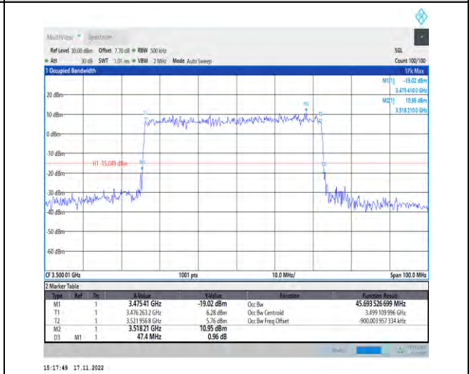
1-N78-3450-3550-PC2-30-50-M-4-DFT-64QAM-Outer_Full-128@0-Ant1-45.694-47.400-≤50-PASS
