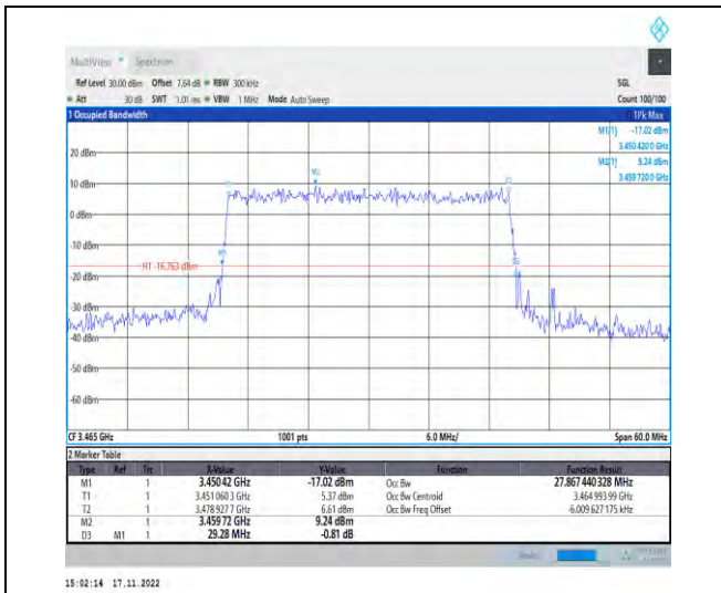
1-N78-3450-3550-PC2-30-30-L-8-CP-64QAM-Outer _Full-78@0-Ant1-27.867-29.280-≤30-PASS
