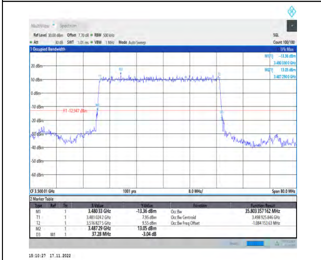
1-N78-3450-3550-PC2-30-40-M-2-DFT-PI2BPSK-Outer_Full-100@0-Ant1-35.803-37.280-≤40-PASS
