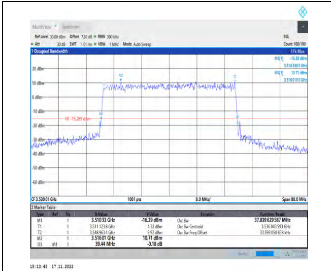
1-N78-3450-3550-PC2-30-40-H-7-CP-16QAM-Outer _Full-106@0-Ant1-37.84-39.440-≤40-PASS
