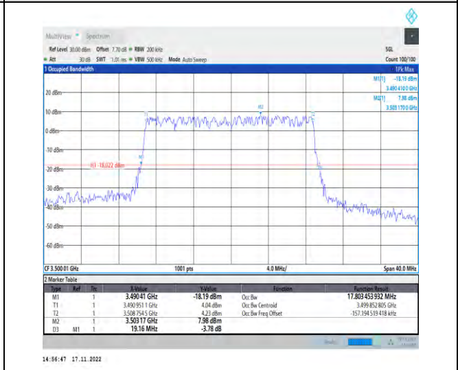
1-N78-3450-3550-PC2-30-20-M-5-DFT-256QAM-Outer_Full-50@0-Ant1-17.803-19.160-≤20-PASS
