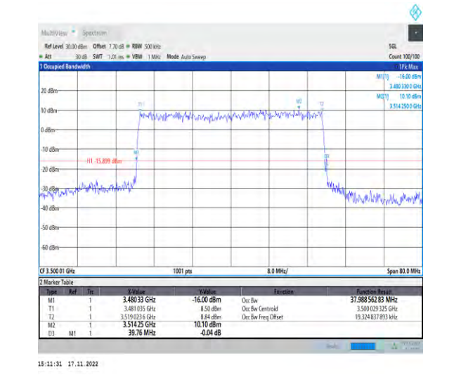
1-N78-3450-3550-PC2-30-40-M-7-CP-16QAM-Outer_Full-106@0-Ant1-37.989-39.760-≤40-PASS
