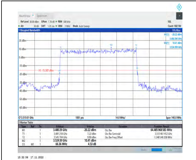
1-N78-3450-3550-PC2-30-70-H-2-DFT-PI2BPSK-Outer_Full-180@0-Ant1-64.486-66.360-≤70-PASS
