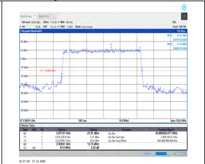
1-N78-3450-3550-PC2-30-50-M-2-DFT-PI2BPSK-Outer_Full-128@0-Ant1-45.81-47.900-≤50-PASS
