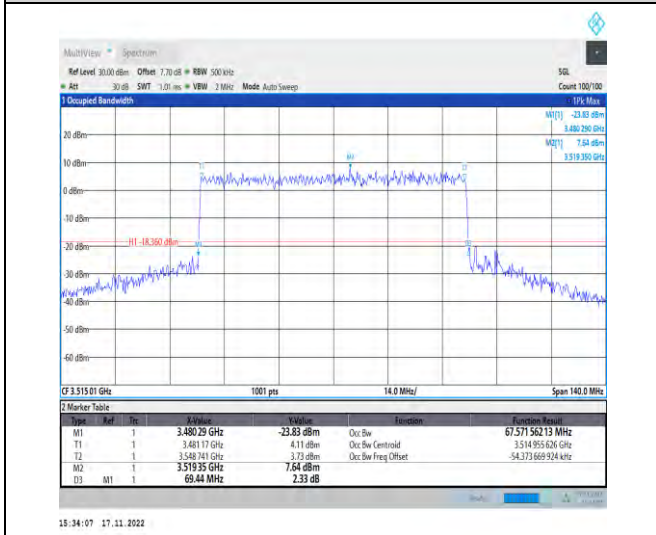
1-N78-3450-3550-PC2-30-70-H-8-CP-64QAM-Outer_Full-189@0-Ant1-67.572-69.440-≤70-PASS
