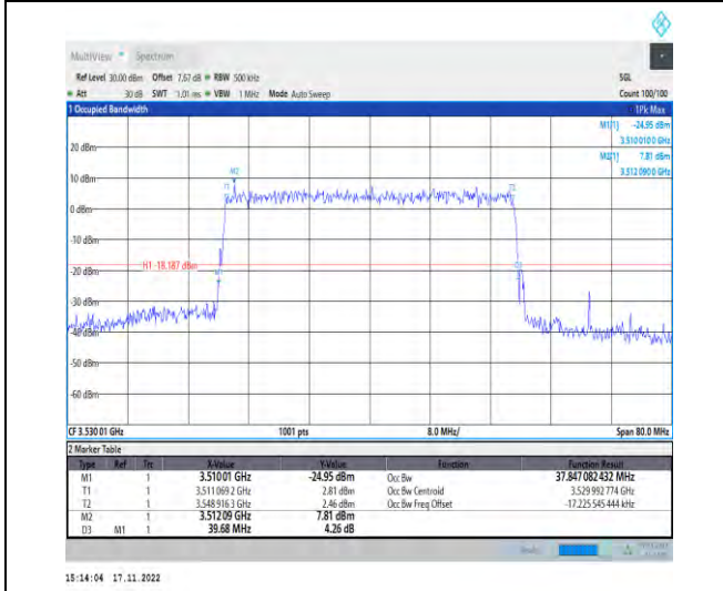
1-N78-3450-3550-PC2-30-40-H-9-CP-256QAM-Outer _Full-106@0-Ant1-37.847-39.680-≤40-PASS
