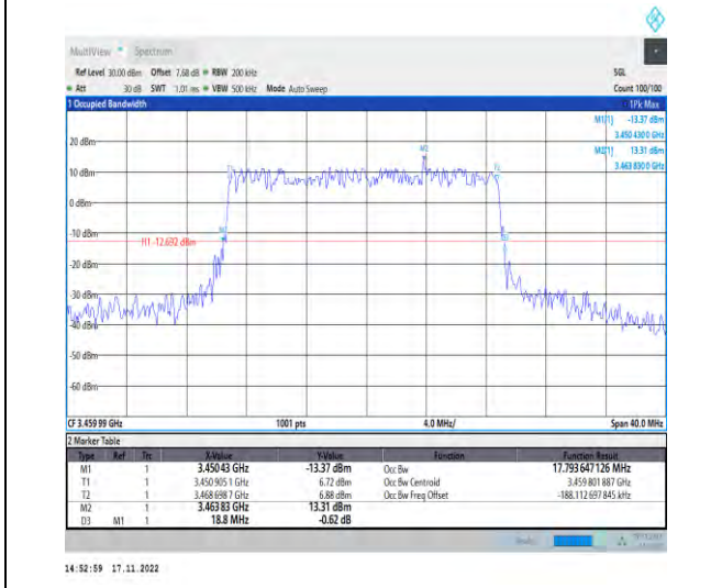
1-N78-3450-3550-PC2-30-20-L-1-DFT-QPSK-Outer_Full-50@0-Ant1-17.794-18.800-≤20-PASS
