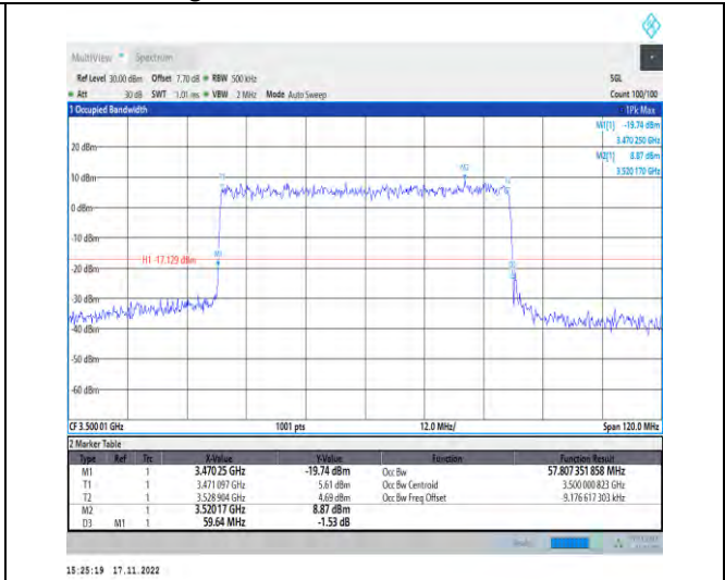
1-N78-3450-3550-PC2-30-60-M-7-CP-16QAM-Outer_Full-162@0-Ant1-57.807-59.640-≤60-PASS
