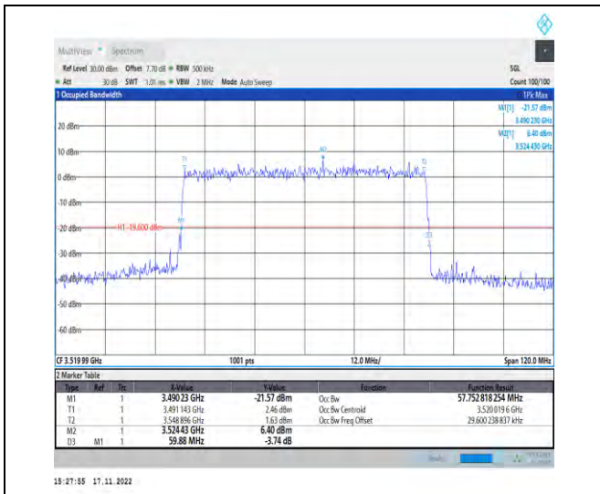
1-N78-3450-3550-PC2-30-60-H-9-CP-256QAM-Outer_Full-162@0-Ant1-57.753-59.880-≤60-PASS
