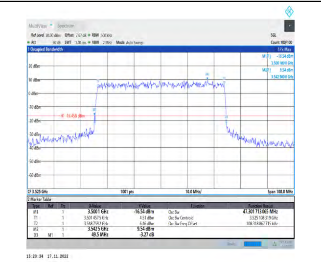
1-N78-3450-3550-PC2-30-50-H-7-CP-16QAM-Outer_Full-133@0-Ant1-47.302-49.500-≤50-PASS
