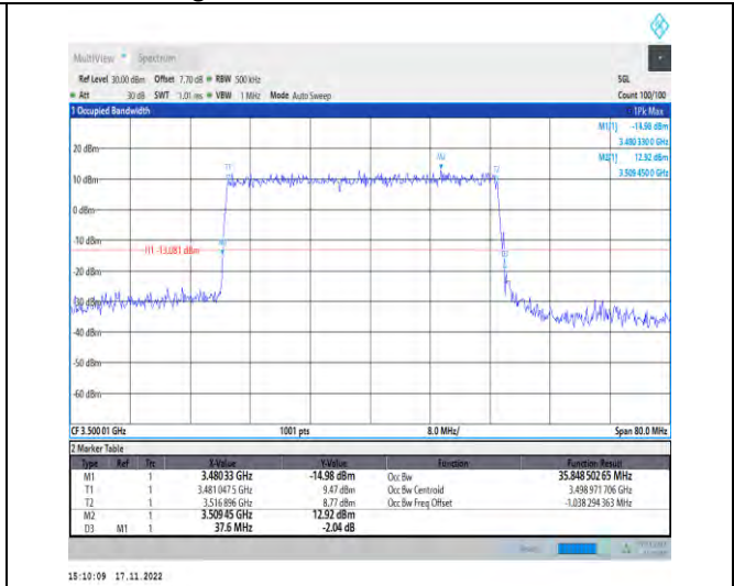
1-N78-3450-3550-PC2-30-40-M-1-DFT-QPSK-Outer_Full-100@0-Ant1-35.849-37.600-≤40-PASS
