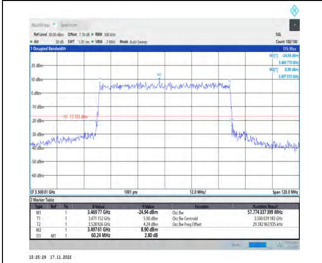
1-N78-3450-3550-PC2-30-60-M-8-CP-64QAM-Outer_Full-162@0-Ant1-57.774-60.240-≤60-PASS
