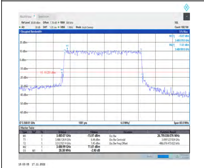
1-N78-3450-3550-PC2-30-30-M-1-DFT-QPSK-Outer _Full-75@0-Ant1-26.795-28.380-≤30-PASS
