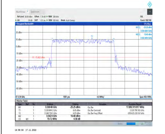
1-N78-3450-3550-PC2-30-20-H-3-DFT-16QAM-Outer_Full-50@0-Ant1-17.892-19.120-≤20-PASS
