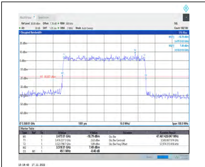
1-N78-3450-3550-PC2-30-50-M-9-CP-256QAM-Out er_Full-133@0-Ant1-47.461-49.100-<=50-PASS
