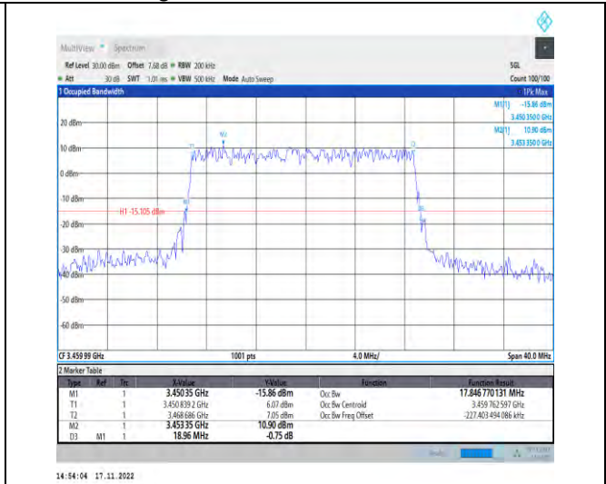
1-N78-3450-3550-PC2-30-20-L-4-DFT-64QAM-Outer_Full-50@0-Ant1-17.847-18.960-<=20-PASS
