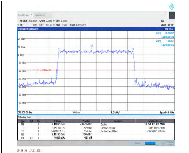
1-N78-3450-3550-PC2-30-40-L-9-CP-256QAM-Outer_Full-106@0-Ant1-37.791-40.080-≤40-PASS
