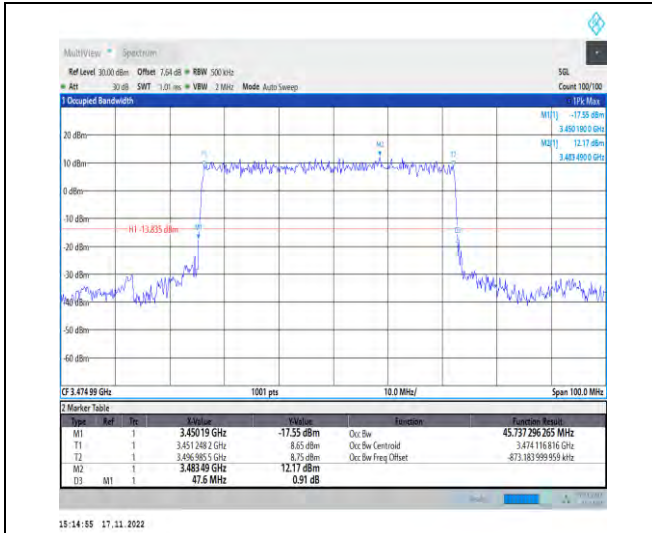
1-N78-3450-3550-PC2-30-50-L-2-DFT-PI2BPSK-Out er_Full-128@0-Ant1-45.737-47.600-≤50-PASS
