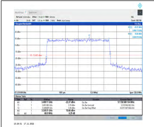
1-N78-3450-3550-PC2-30-60-H-1-DFT-QPSK-Outer_Full-162@0-Ant1-57.727-60.000-≤60-PASS
