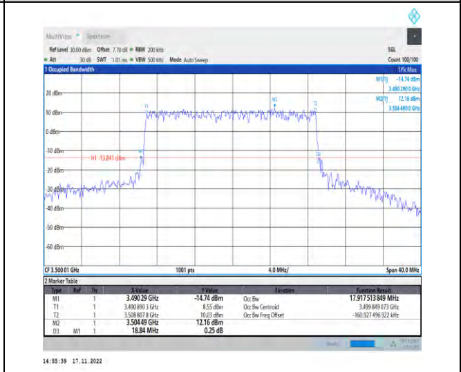
1-N78-3450-3550-PC2-30-20-M-1-DFT-QPSK-Outer_Full-50@0-Ant1-17.918-18.840-≤20-PASS
