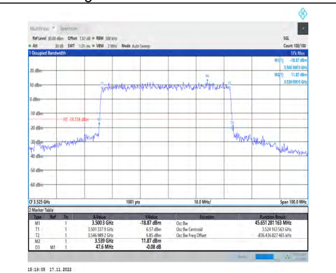
1-N78-3450-3550-PC2-30-50-H-1-DFT-QPSK-Outer_Full-128@0-Ant1-45.651-47.600-<=50-PASS
