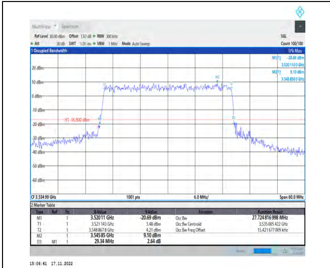
1-N78-3450-3550-PC2-30-30-H-6-CP-QPSK-Outer_Full-78@0-Ant1-27.725-29.340-≤30-PASS
