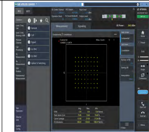
1-N78-3450-3550--30-100-M-4-DFT-64QAM-Outer_Full-270@0-Ant1-see graph-PASS
