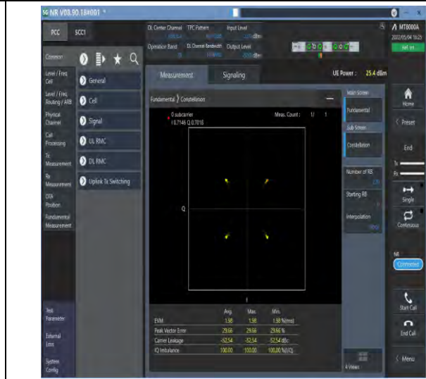
1-N78-3450-3550--30-100-M-2-DFT-QPSK-Outer_Full-270@0-Ant1-see graph-PASS
