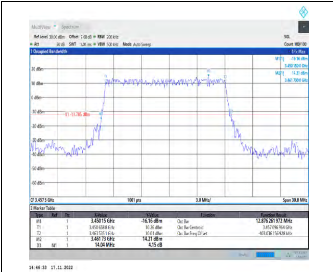
1-N78-3450-3550-PC2-30-15-L-2-DFT-PI2BPSK-Out er_Full-36@0-Ant1-12.876-14.040-≤15-PASS
