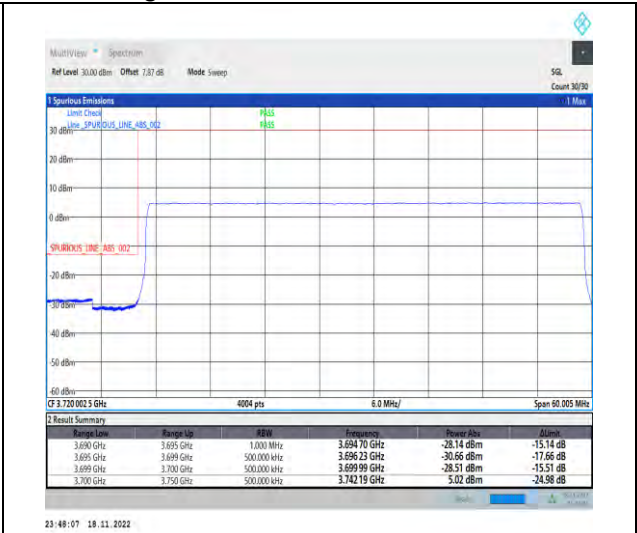
1-N77-3700-3980-PC2-30-50-L-6-CP-QPSK-Outer _Full-133@0-Ant1-1--PASS-see graph
