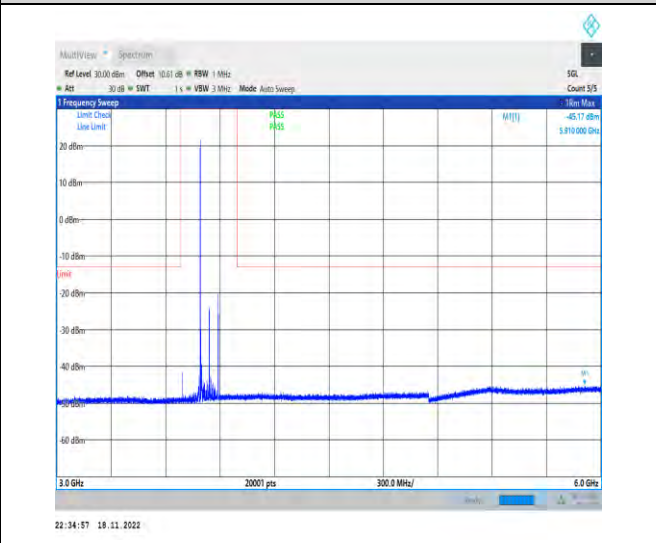
1-N77-3700-3980-PC2-30-100-M-1-CP-QPSK-Edge _1RB_Left-1@0-3000-6000-Ant1-5910.00--45.17--1 3-PASS
