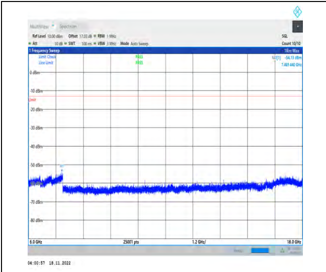
1-N77-3700-3980-PC2-30-100-L-1-DFT-PI2BPSK-Inner_1RB_Left-1@1-6000-18000-Ant1-7465.44--54.1 3--13-PASS
