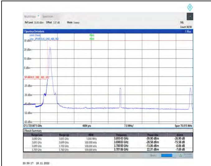
1-N77-3700-3980-PC2-30-60-L-4-CP-QPSK-Edge_1R B_Left-1@0-Ant1-1--PASS-see graph
