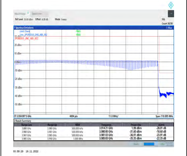
1-N77-3700-3980-PC2-30-100-H-6-CP-QPSK-Out er_Full-273@0-Ant1-1--PASS-see graph
