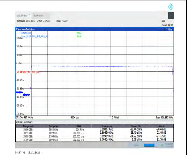
1-N77-3700-3980-PC2-30-100-L-6-CP-QPSK-Outer_Full-273@0-Ant1-1--PASS-see graph
