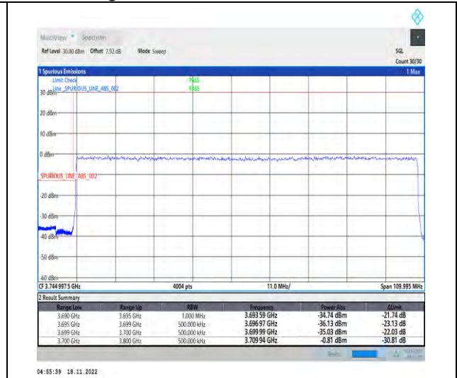
1-N77-3700-3980-PC2-30-100-L-3-DFT-PI2BPSK-Outer_Full-270@0-Ant1-1--PASS-see graph
