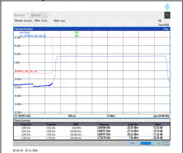
1-N77-3700-3980-PC2-30-30-L-6-CP-QPSK-Outer _Full-78@0-Ant1-1--PASS-see graph
