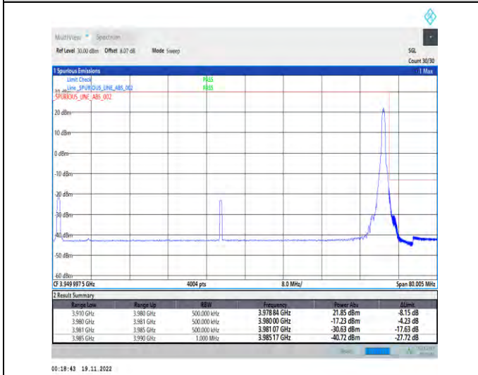
1-N77-3700-3980-PC2-30-70-H-5-CP-QPSK-Edge_1R B_Right-1@188-Ant1-1--PASS-see graph
