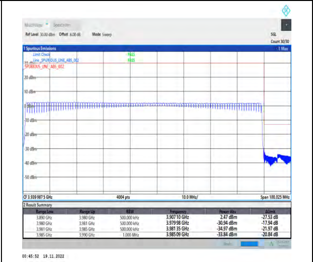
1-N77-3700-3980-PC2-30-90-H-6-CP-QPSK-Outer _Full-245@0-Ant1-1--PASS-see graph
