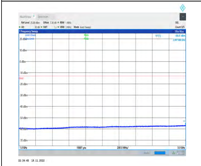
1-N77-3700-3980-PC2-30-100-M-1-CP-QPSK-Edge _1RB_Left-1@0-1000-3000-Ant1-2997.00--56.41--1 3-PASS
