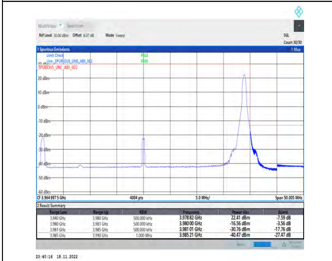
1-N77-3700-3980-PC2-30-40-H-5-CP-QPSK-Edge_1R B_Right-1@105-Ant1-1--PASS-see graph
