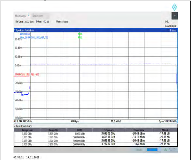
1-N77-3700-3980-PC2-30-100-L-6-CP-QPSK-Out er_Full-273@0-Ant1-1--PASS-see graph
