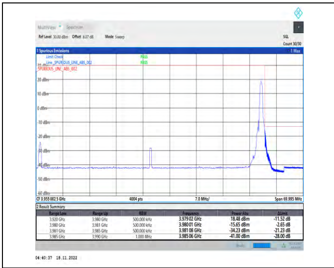
1-N77-3700-3980-PC2-30-60-H-2-DFT-PI2BPSK-Edge_1RB_Right-1@161-Ant1-1--PASS-see graph
