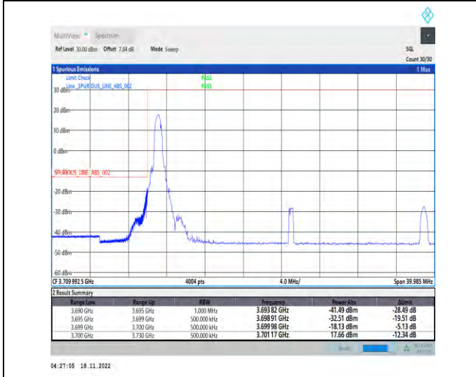
1-N77-3700-3980-PC2-30-30-L-4-CP-QPSK-Edge_1RB_Left-1@0-Ant1-1--PASS-see graph
