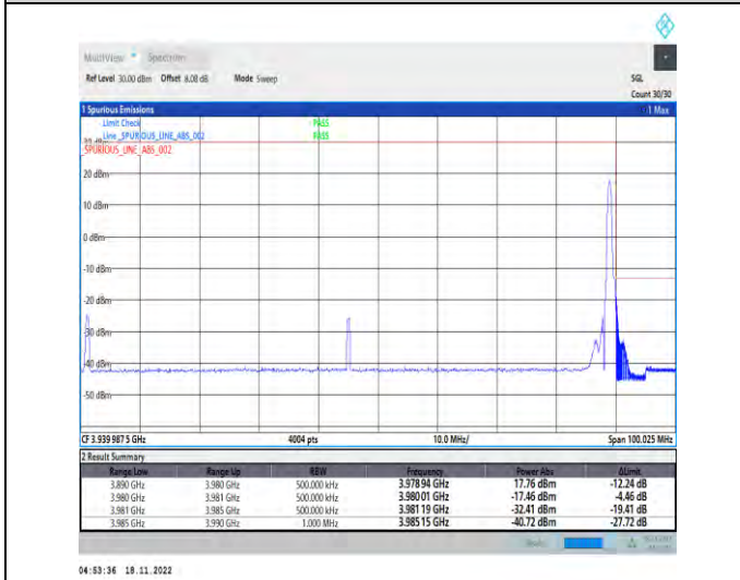
1-N77-3700-3980-PC2-30-90-H-5-CP-QPSK-Edge_1RB_Right-1@244-Ant1-1--PASS-see graph
