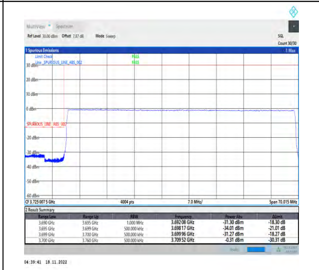
1-N77-3700-3980-PC2-30-60-L-6-CP-QPSK-Outer_Full-162@0-Ant1-1--PASS-see graph
