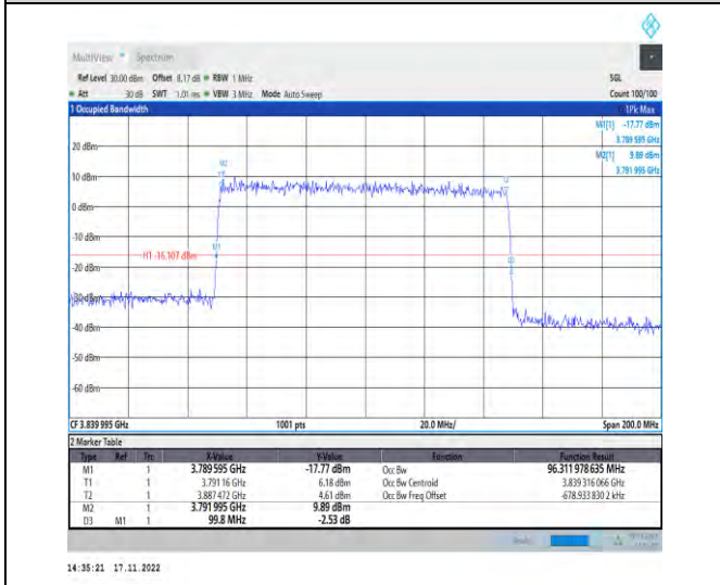
1-N77-3700-3980-PC2-30-100-M-4-DFT-64QAM-Out er_Full-270@0-Ant1-96.312-99.800-≤100-PASS
