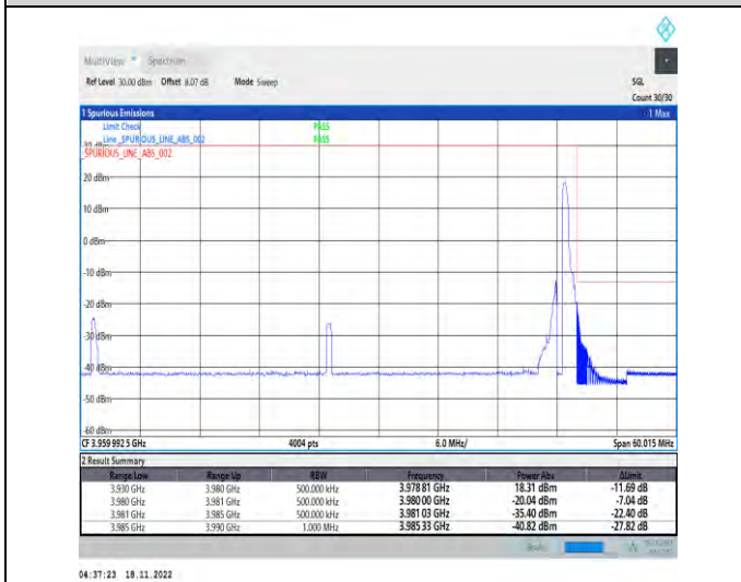
1-N77-3700-3980-PC2-30-50-H-5-CP-QPSK-Edge_1RB_Right-1@132-Ant1-1--PASS-see graph
