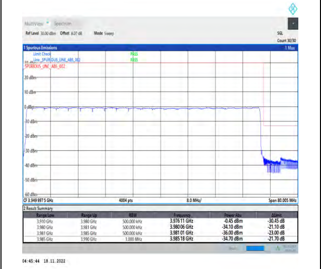
1-N77-3700-3980-PC2-30-70-H-6-CP-QPSK-Outer_Full-189@0-Ant1-1--PASS-see graph
