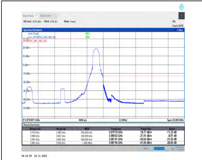
1-N77-3700-3980-PC2-30-10-H-2-DFT-PI2BPSK-Edge_1RB_Right-1@23-Ant1-1--PASS-see graph
