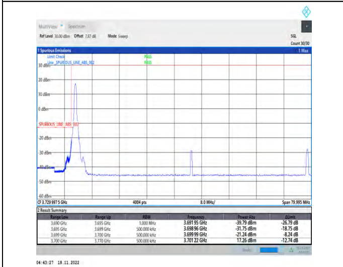
1-N77-3700-3980-PC2-30-70-L-4-CP-QPSK-Edge_1RB_Left-1@0-Ant1-1--PASS-see graph
