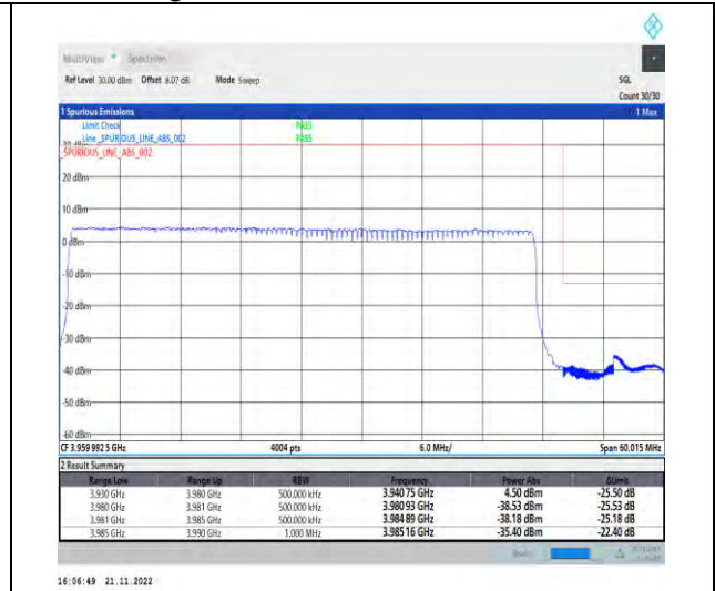
1-N77-3700-3980-PC2-30-50-H-3-DFT-PI2BPSK-Outer_Full-128@0-Ant1-1--PASS-see graph
