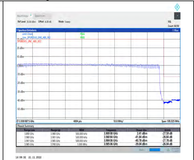
1-N77-3700-3980-PC2-30-90-H-3-DFT-PI2BPSK-Outer_Full-240@0-Ant1-1--PASS-see graph
