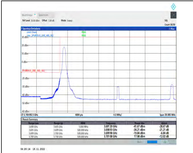
1-N77-3700-3980-PC2-30-30-L-1-DFT-PI2BPSK-Edge_1RB_Left-1@0-Ant1-1--PASS-see graph
