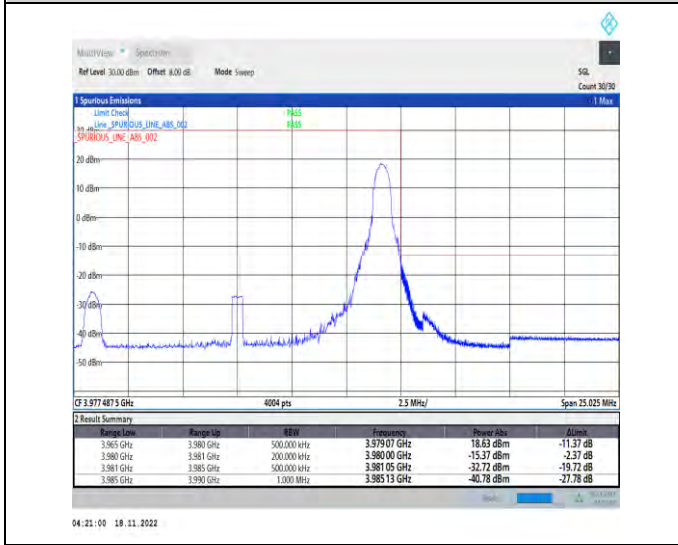
1-N77-3700-3980-PC2-30-15-H-5-CP-QPSK-Edge_1RB_Right-1@37-Ant1-1--PASS-see graph
