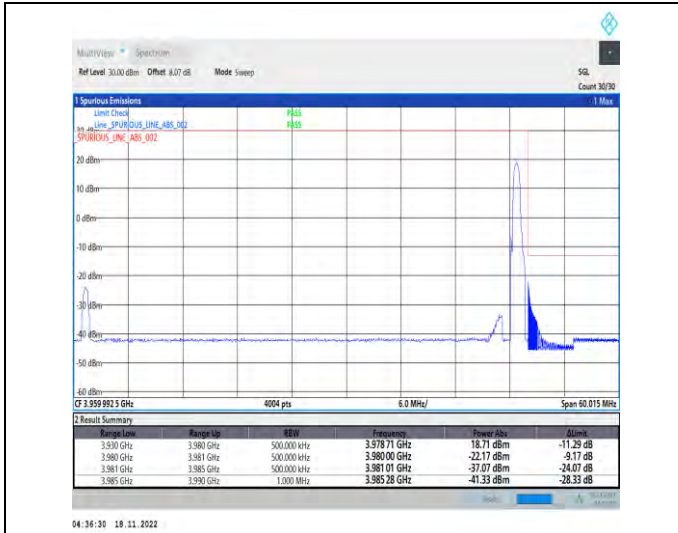
1-N77-3700-3980-PC2-30-50-H-2-DFT-PI2BPSK-Edge_1RB_Right-1@132-Ant1-1--PASS-see graph
