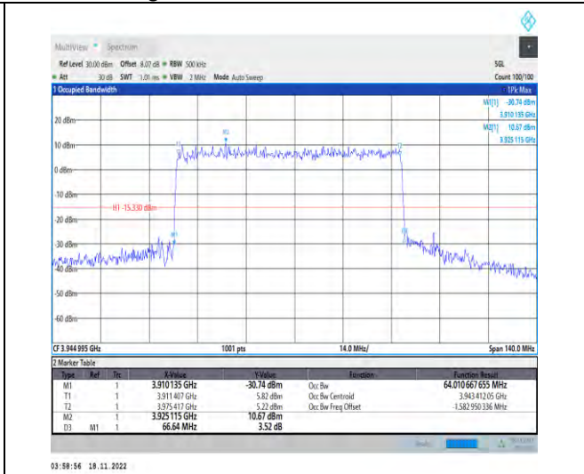
1-N77-3700-3980-PC2-30-70-H-3-DFT-16QAM-Out er_Full-180@0-Ant1-64.011-66.640-≤70-PASS
