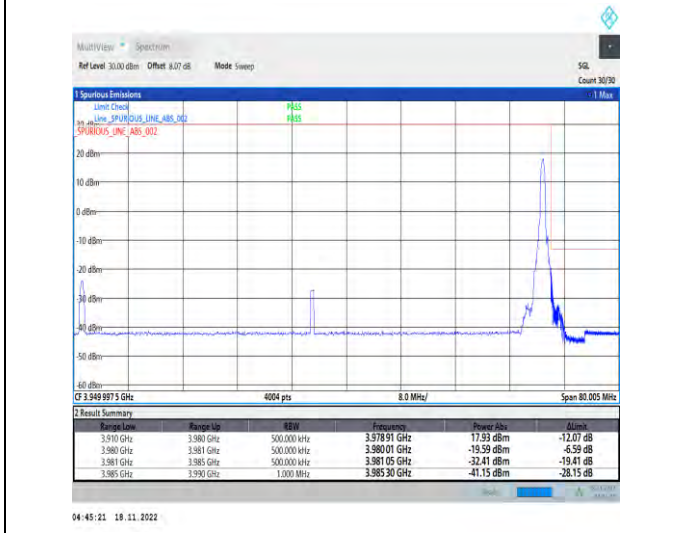
1-N77-3700-3980-PC2-30-70-H-5-CP-QPSK-Edge_1RB_Right-1@188-Ant1-1--PASS-see graph
