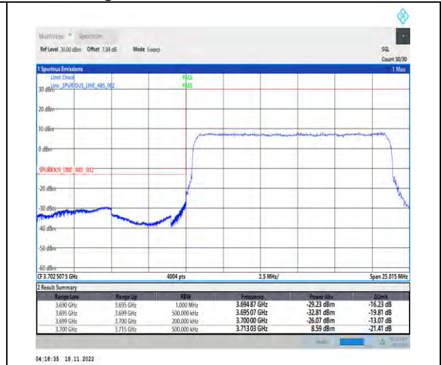
1-N77-3700-3980-PC2-30-15-L-3-DFT-PI2BPSK-Outer_Full-36@0-Ant1-1--PASS-see graph
