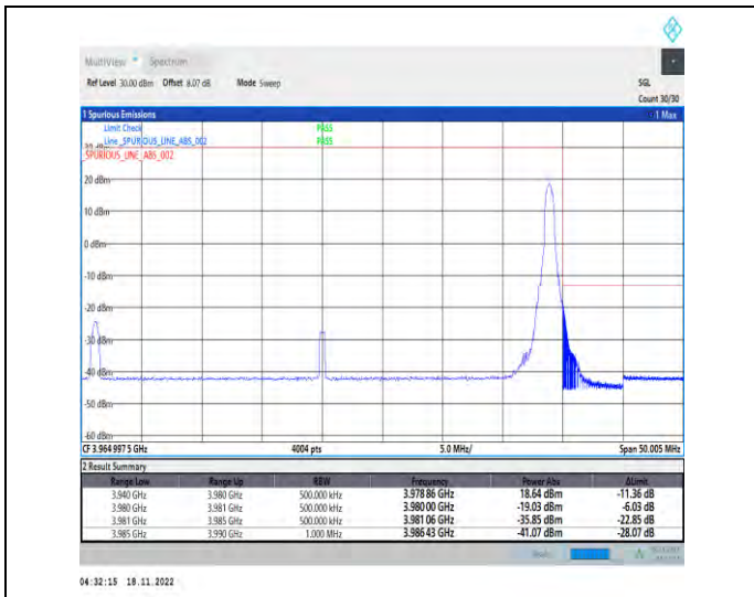
1-N77-3700-3980-PC2-30-40-H-2-DFT-PI2BPSK-Edge_1RB_Right-1@105-Ant1-1--PASS-see graph
