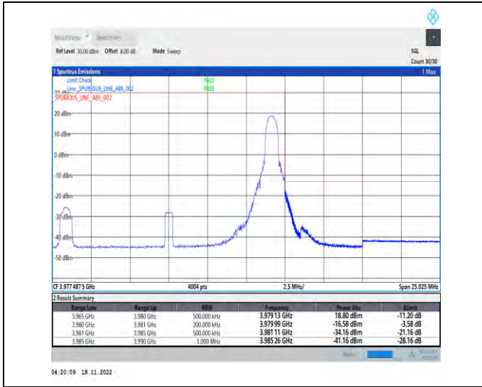
1-N77-3700-3980-PC2-30-15-H-2-DFT-PI2BPSK-Edge_1RB_Right-1@37-Ant1-1--PASS-see graph
