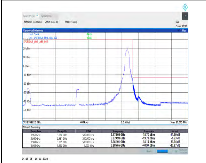
1-N77-3700-3980-PC2-30-20-H-5-CP-QPSK-Edge_1RB_Right-1@50-Ant1-1--PASS-see graph
