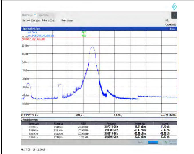
1-N77-3700-3980-PC2-30-10-H-5-CP-QPSK-Edge_1RB_Right-1@23-Ant1-1--PASS-see graph
