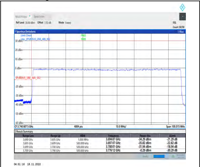
1-N77-3700-3980-PC2-30-90-L-3-DFT-PI2BPSK-Outer_Full-240@0-Ant1-1--PASS-see graph
