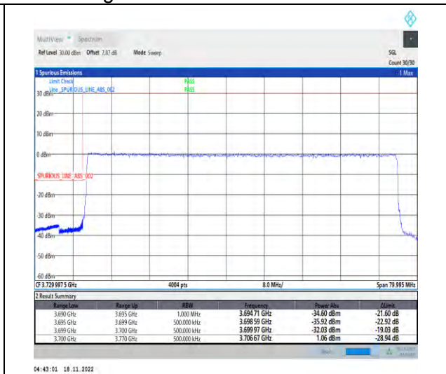
1-N77-3700-3980-PC2-30-70-L-3-DFT-PI2BPSK-Outer_Full-180@0-Ant1-1--PASS-see graph
