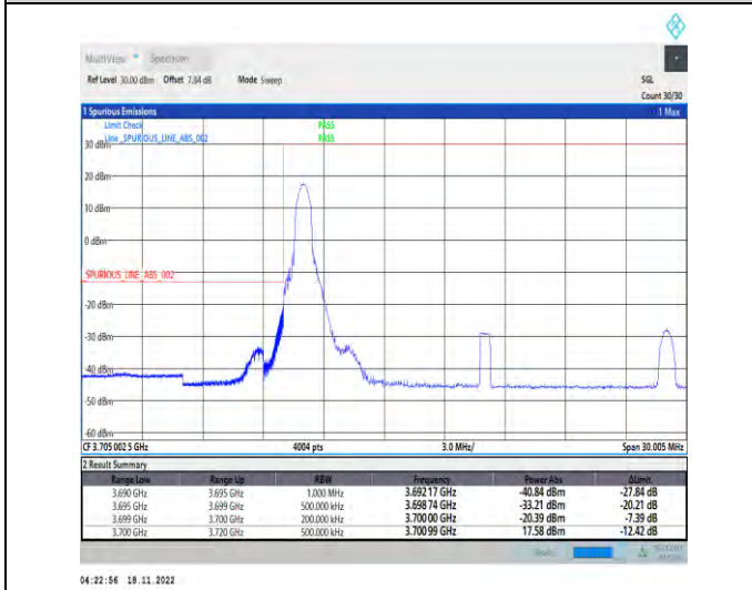
1-N77-3700-3980-PC2-30-20-L-4-CP-QPSK-Edge_1RB_Left-1@0-Ant1-1--PASS-see graph
