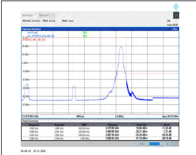
1-N77-3700-3980-PC2-30-20-H-2-DFT-PI2BPSK-Edge_1RB_Right-1@50-Ant1-1--PASS-see graph
