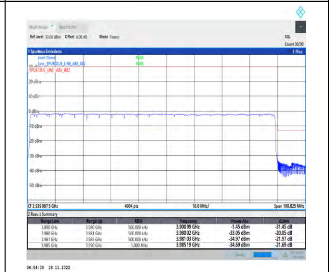
1-N77-3700-3980-PC2-30-90-H-6-CP-QPSK-Outer_Full-245@0-Ant1-1--PASS-see graph
