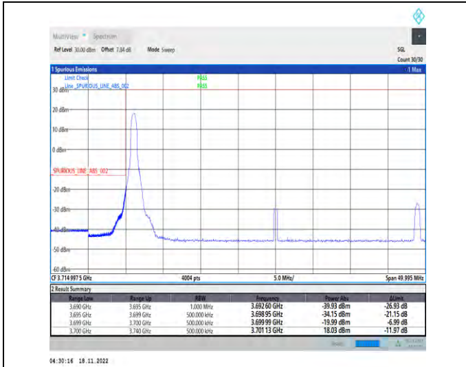
1-N77-3700-3980-PC2-30-40-L-1-DFT-PI2BPSK-Edge_1RB_Left-1@0-Ant1-1--PASS-see graph
