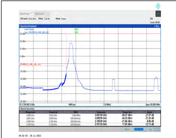
1-N77-3700-3980-PC2-30-20-L-1-DFT-PI2BPSK-Edge_1RB_Left-1@0-Ant1-1--PASS-see graph
