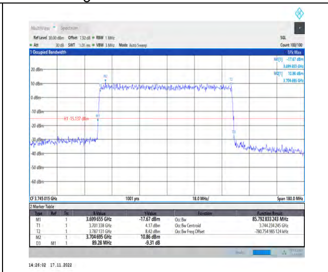
1-N77-3700-3980-PC2-30-90-L-3-DFT-16QAM-Out er_Full-240@0-Ant1-85.793-89.280-<math>\leq 90</math>-PASS
