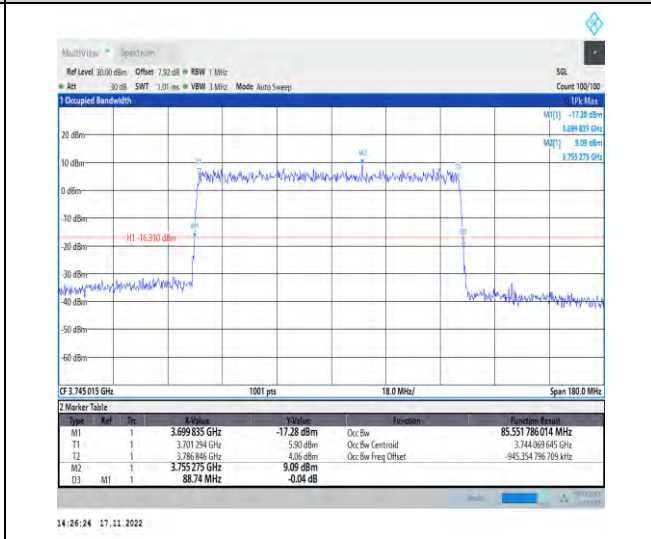
1-N77-3700-3980-PC2-30-90-L-5-DFT-256QAM-Out er_Full-240@0-Ant1-85.552-88.740-<math>\leq 90</math>-PASS
