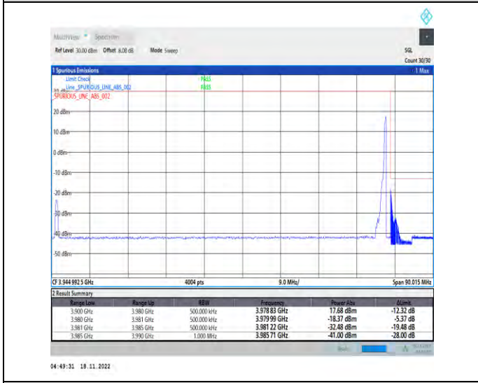
1-N77-3700-3980-PC2-30-80-H-5-CP-QPSK-Edge_1RB_Right-1@216-Ant1-1--PASS-see graph
