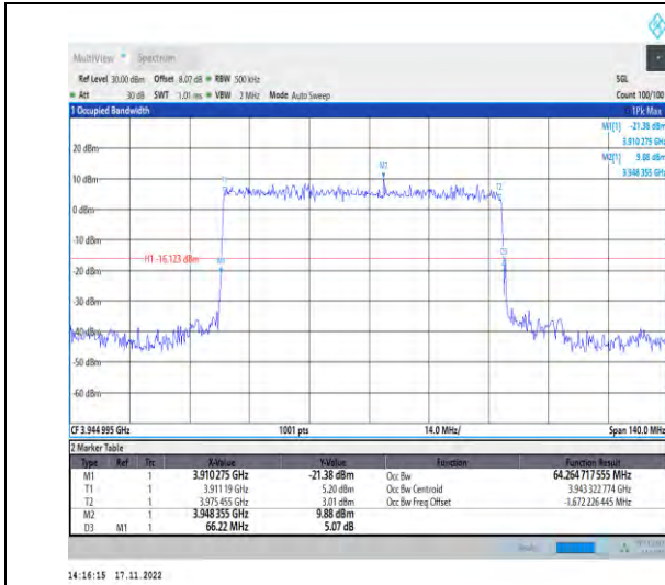
1-N77-3700-3980-PC2-30-70-H-2-DFT-PI2BPSK-Out er_Full-180@0-Ant1-64.265-66.220-≤70-PASS
