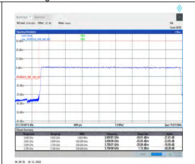
1-N77-3700-3980-PC2-30-60-L-3-DFT-PI2BPSK-Outer_Full-162@0-Ant1-1--PASS-see graph
