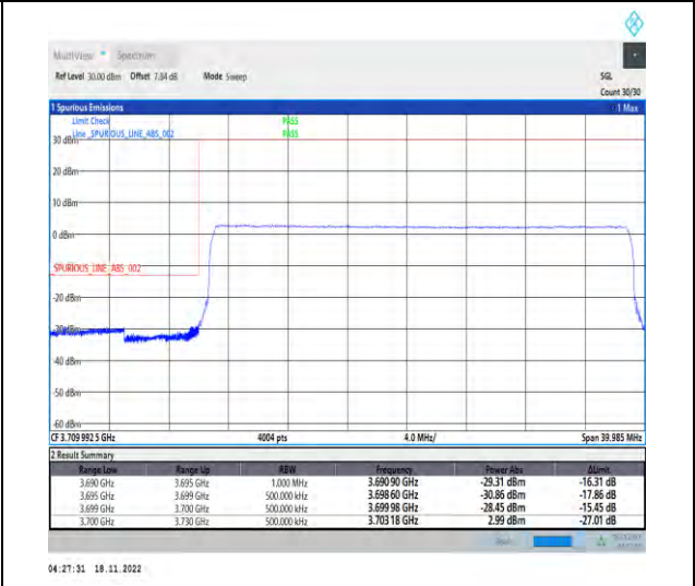
1-N77-3700-3980-PC2-30-30-L-6-CP-QPSK-Outer_Full-78@0-Ant1-1--PASS-see graph
