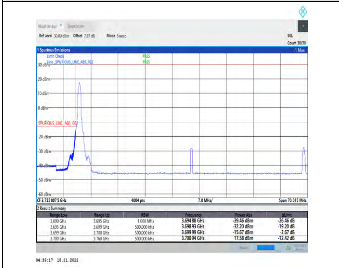
1-N77-3700-3980-PC2-30-60-L-4-CP-QPSK-Edge_1RB_Left-1@0-Ant1-1--PASS-see graph
