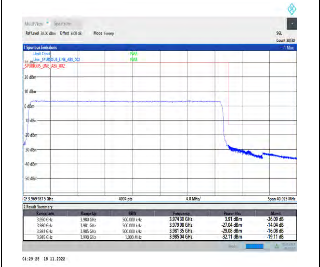
1-N77-3700-3980-PC2-30-30-H-6-CP-QPSK-Outer_Full-78@0-Ant1-1--PASS-see graph
