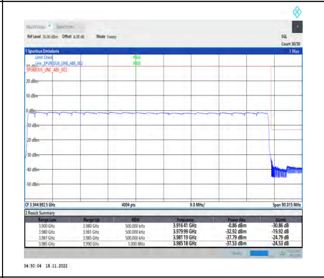
1-N77-3700-3980-PC2-30-80-H-6-CP-QPSK-Outer_Full-217@0-Ant1-1--PASS-see graph
