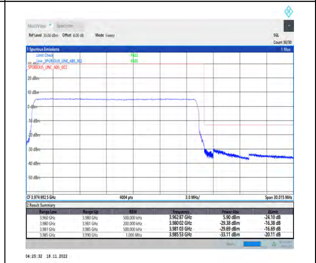
1-N77-3700-3980-PC2-30-20-H-6-CP-QPSK-Outer_Full-51@0-Ant1-1--PASS-see graph
