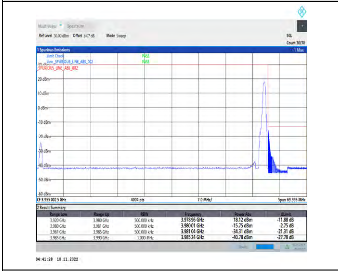
1-N77-3700-3980-PC2-30-60-H-5-CP-QPSK-Edge_1RB_Right-1@161-Ant1-1--PASS-see graph
