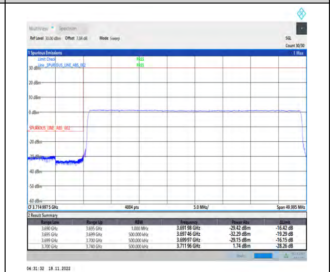
1-N77-3700-3980-PC2-30-40-L-6-CP-QPSK-Outer_Full-106@0-Ant1-1--PASS-see graph
