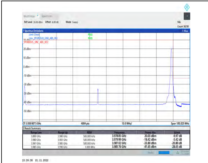
1-N77-3700-3980-PC2-30-90-H-2-DFT-PI2BPSK-Edge_1RB_Right-1@244-Ant1-1--PASS-see graph
