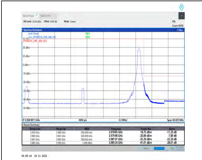
1-N77-3700-3980-PC2-30-30-H-2-DFT-PI2BPSK-Edge_1RB_Right-1@77-Ant1-1--PASS-see graph
