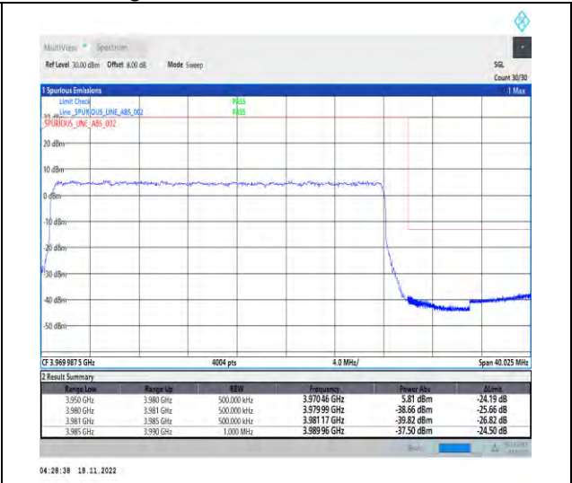
1-N77-3700-3980-PC2-30-30-H-3-DFT-PI2BPSK-Outer_Full-75@0-Ant1-1--PASS-see graph
