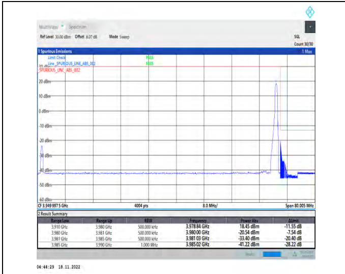
1-N77-3700-3980-PC2-30-70-H-2-DFT-PI2BPSK-Edge_1RB_Right-1@188-Ant1-1--PASS-see graph
