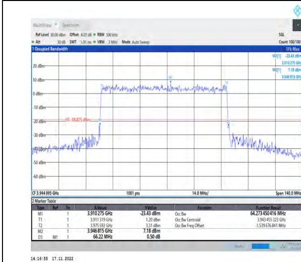
1-N77-3700-3980-PC2-30-70-H-4-DFT-64QAM-Out er_Full-180@0-Ant1-64.273-66.220-≤70-PASS
