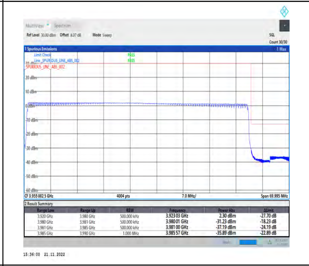
1-N77-3700-3980-PC2-30-60-H-6-CP-QPSK-Outer_Full-162@0-Ant1-1--PASS-see graph
