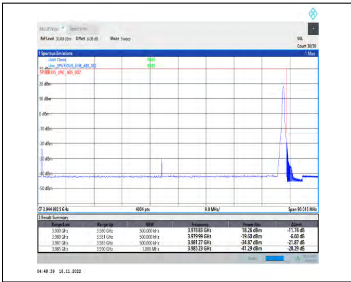
1-N77-3700-3980-PC2-30-80-H-2-DFT-PI2BPSK-Edge_1RB_Right-1@216-Ant1-1--PASS-see graph
