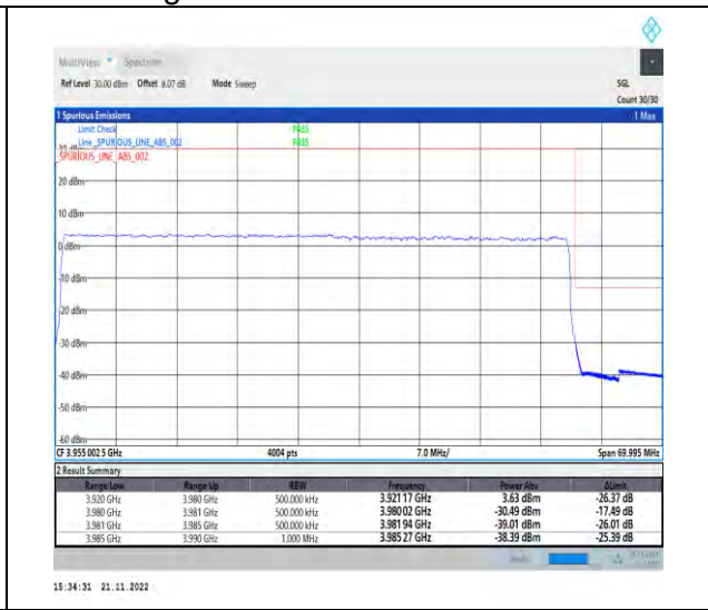
1-N77-3700-3980-PC2-30-60-H-3-DFT-PI2BPSK-Outer_Full-162@0-Ant1-1--PASS-see graph
