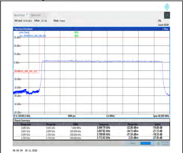
1-N77-3700-3980-PC2-30-50-L-3-DFT-PI2BPSK-Outer_Full-128@0-Ant1-1--PASS-see graph
