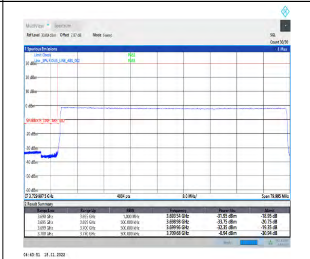
1-N77-3700-3980-PC2-30-70-L-6-CP-QPSK-Outer_Full-189@0-Ant1-1--PASS-see graph
