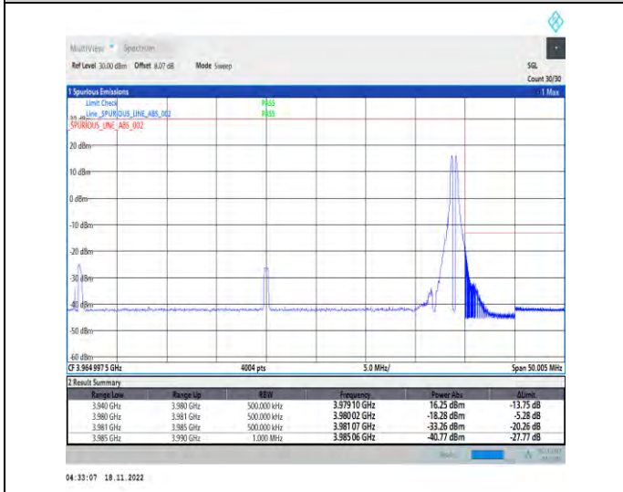
1-N77-3700-3980-PC2-30-40-H-5-CP-QPSK-Edge_1RB_Right-1@105-Ant1-1--PASS-see graph
