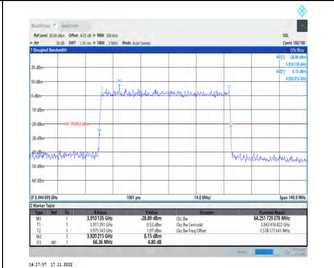
1-N77-3700-3980-PC2-30-70-H-5-DFT-256QAM-Out er_Full-180@0-Ant1-64.252-66.360-≤70-PASS
