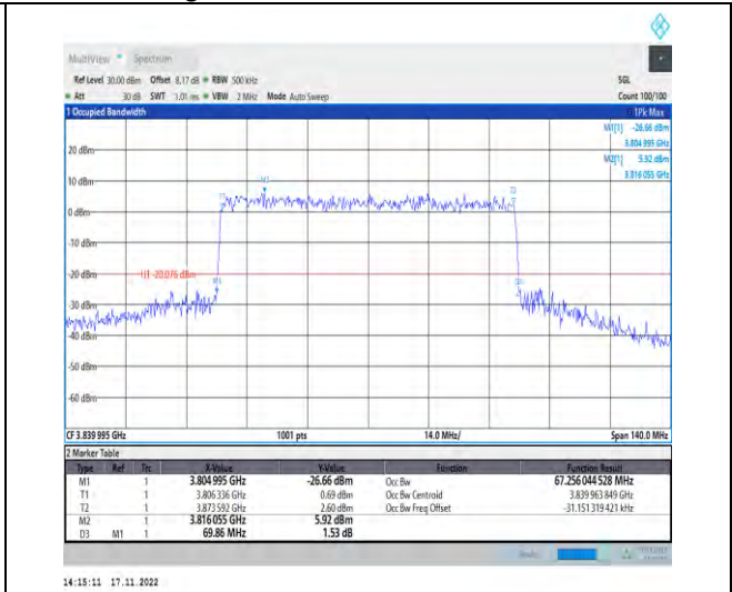
1-N77-3700-3980-PC2-30-70-M-8-CP-64QAM-Outer _Full-189@0-Ant1-67.256-69.860-≤70-PASS
