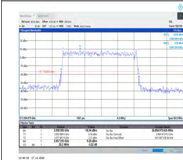
1-N77-3700-3980-PC2-30-30-H-4-DFT-64QAM-Out er_Full-75@0-Ant1-26.857-28.200-≤30-PASS
