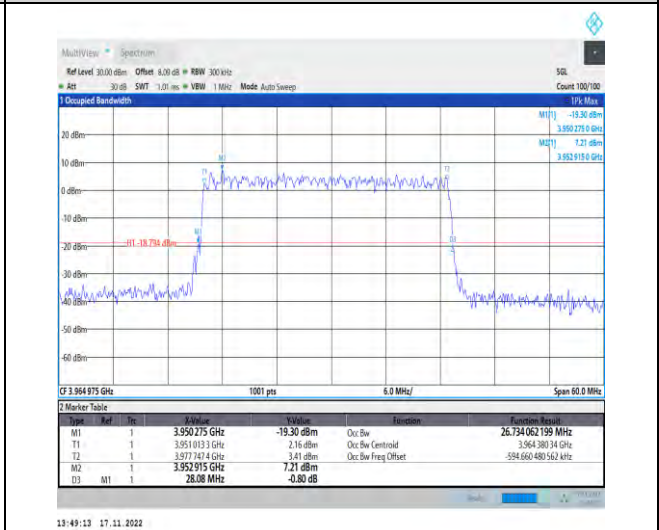
1-N77-3700-3980-PC2-30-30-H-5-DFT-256QAM-Out er_Full-75@0-Ant1-26.734-28.080-≤30-PASS
