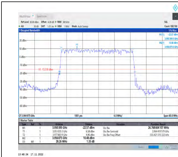
1-N77-3700-3980-PC2-30-30-H-2-DFT-PI2BPSK-Out er_Full-75@0-Ant1-26.769-28.260-≤30-PASS
