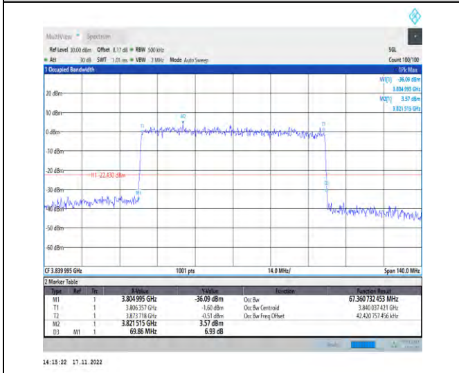
1-N77-3700-3980-PC2-30-70-M-9-CP-256QAM-Outer _Full-189@0-Ant1-67.361-69.860-≤70-PASS
