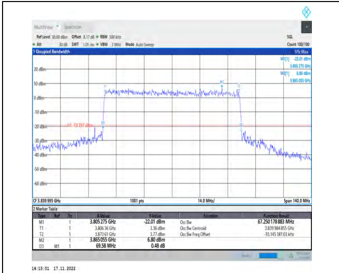
1-N77-3700-3980-PC2-30-70-M-7-CP-16QAM-Outer _Full-189@0-Ant1-67.25-69.580-≤70-PASS
