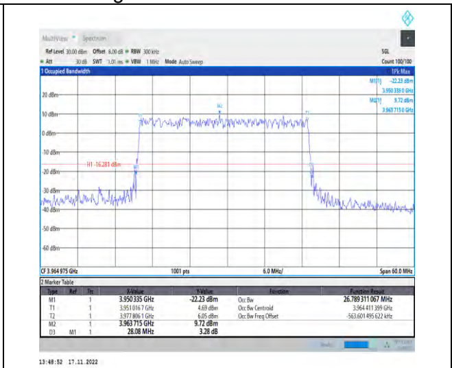
1-N77-3700-3980-PC2-30-30-H-3-DFT-16QAM-Out er_Full-75@0-Ant1-26.789-28.080-≤30-PASS
