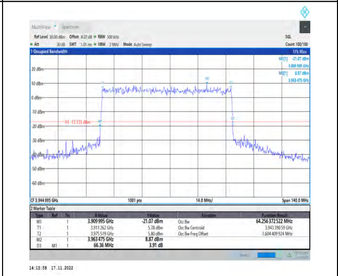
1-N77-3700-3980-PC2-30-70-H-1-DFT-QPSK-Outer _Full-180@0-Ant1-64.256-66.360-≤70-PASS
