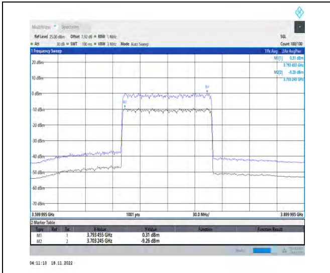
1-N77-3700-3980-PC2-30-100-L-1-DFT-256QAM-Outer_Full-270@0-Ant1-9.57-100%-0.00-9.57-PASS<=13
