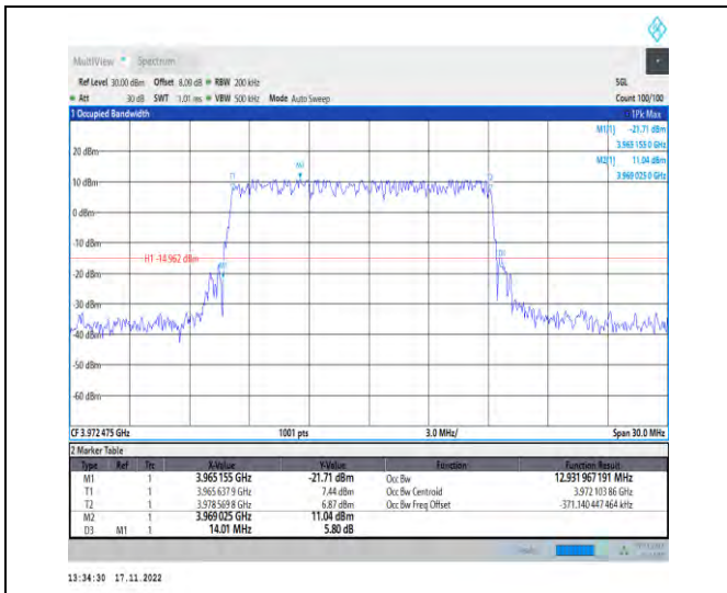
1-N77-3700-3980-PC2-30-15-H-4-DFT-64QAM-Outer_Full-36@0-Ant1-12.932-14.010-≤15-PASS
