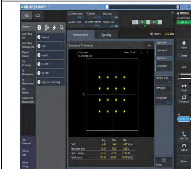
1-N77-3700-3980-PC2-30-100-M-7-CP-16QAM-Outer_Full-273@0-Ant1-see graph-PASS
