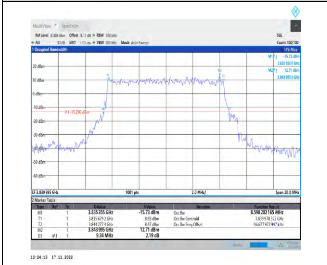
1-N77-3700-3980-PC2-30-10-M-2-DFT-PI2BPSK-Outer_Full-24@0-Ant1-8.598-9.340-≤10-PASS
