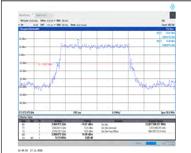
1-N77-3700-3980-PC2-30-15-H-2-DFT-PI2BPSK-Outer_Full-36@0-Ant1-12.858-14.190-≤15-PASS
