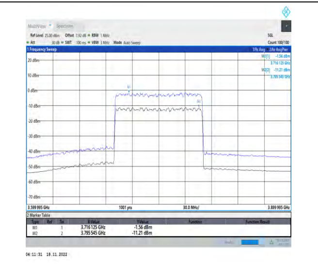
1-N77-3700-3980-PC2-30-100-L-2-CP-256QAM-Outer_Full-273@0-Ant1-9.65-100%-0.00-9.65-PASS<=13
