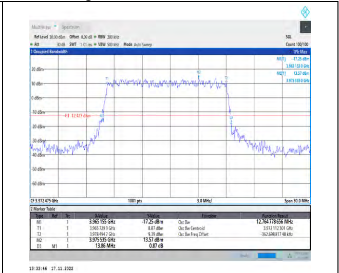
1-N77-3700-3980-PC2-30-15-H-1-DFT-QPSK-Outer_Full-36@0-Ant1-12.765-13.860-≤15-PASS
