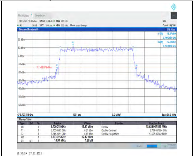
1-N77-3700-3980-PC2-30-15-L-7-CP-16QAM-Outer_Full-38@0-Ant1-13.629-14.970-≤15-PASS
