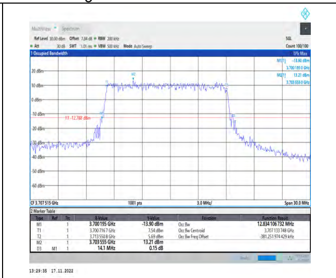
1-N77-3700-3980-PC2-30-15-L-3-DFT-16QAM-Out er_Full-36@0-Ant1-12.834-14.100-≤15-PASS
