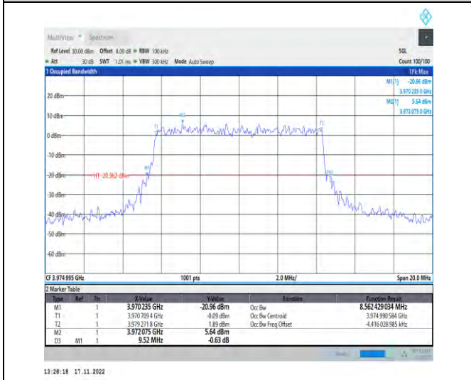
1-N77-3700-3980-PC2-30-10-H-9-CP-256QAM-Outer_Full-24@0-Ant1-8.562-9.520-≤10-PASS
