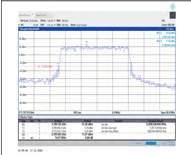
1-N77-3700-3980-PC2-30-15-L-4-DFT-64QAM-Out er_Full-36@0-Ant1-12.857-14.070-≤15-PASS
