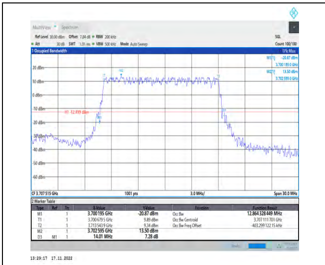
1-N77-3700-3980-PC2-30-15-L-2-DFT-PI2BPSK-Out er_Full-36@0-Ant1-12.864-14.010-≤15-PASS
