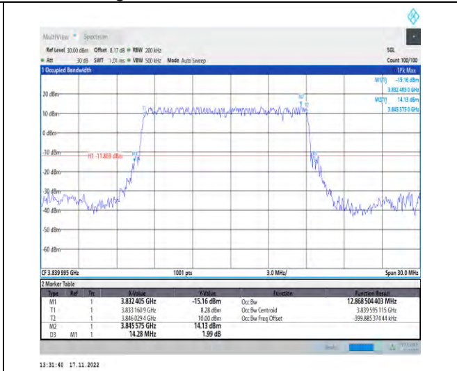
1-N77-3700-3980-PC2-30-15-M-2-DFT-PI2BPSK-Outer_Full-36@0-Ant1-12.869-14.280-≤15-PASS
