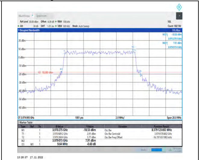
1-N77-3700-3980-PC2-30-10-H-8-CP-64QAM-Outer_Full-24@0-Ant1-8.579-9.640-≤10-PASS
