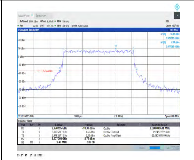
1-N77-3700-3980-PC2-30-10-H-6-CP-QPSK-Outer_Full-24@0-Ant1-8.588-9.460-≤10-PASS
