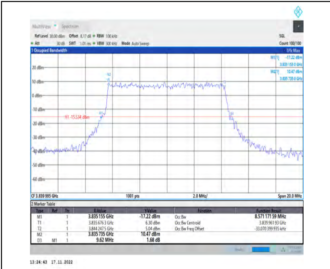
1-N77-3700-3980-PC2-30-10-M-4-DFT-64QAM-Outer_Full-24@0-Ant1-8.571-9.620-≤10-PASS
