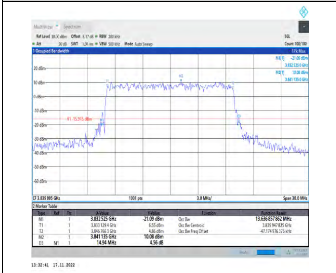
1-N77-3700-3980-PC2-30-15-M-7-CP-16QAM-Outer_Full-38@0-Ant1-13.637-14.940-≤15-PASS
