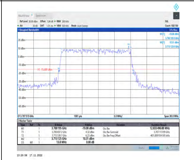
1-N77-3700-3980-PC2-30-15-L-5-DFT-256QAM-Out er_Full-36@0-Ant1-12.833-13.800-≤15-PASS
