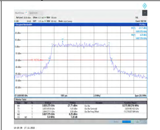
1-N77-3700-3980-PC2-30-10-M-9-CP-256QAM-Outer_Full-24@0-Ant1-8.575-9.400-≤10-PASS
