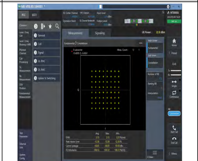
1-N77-3700-3980-PC2-30-100-M-8-CP-64QAM-Outer_Full-273@0-Ant1-see graph-PASS
