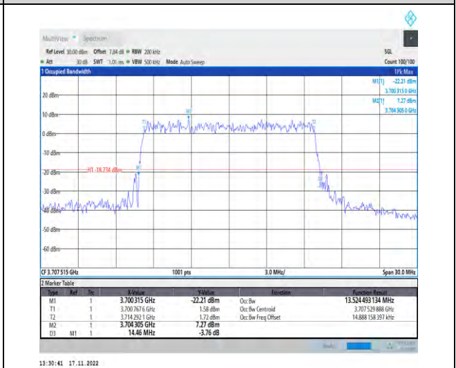
1-N77-3700-3980-PC2-30-15-L-9-CP-256QAM-Outer_Full-38@0-Ant1-13.524-14.460-≤15-PASS
