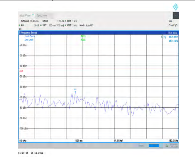
1-N70-PC3-15-15-M-1-DFT-PI2BPSK-Inner_1RB_Le ft-1@1-0.009-0.15-Ant1-0.06--66.01--43-PASS
