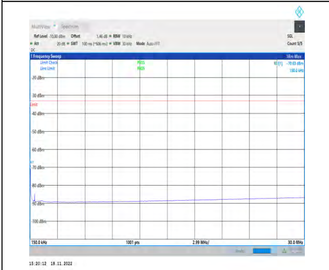
1-N70-PC3-15-15-M-1-DFT-PI2BPSK-Inner_1RB_Le ft-1@1-0.15-30-Ant1-0.15--70.63--33-PASS
