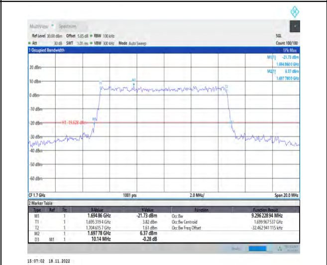
1-N70-PC3-15-10-L-9-CP-256QAM-Outer_Full-52@0- Ant1-9.296-10.140-≤10-PASS
