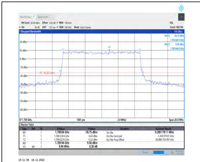
1-N70-PC3-15-10-H-8-CP-64QAM-Outer_Full-52@0 -Ant1-9.289-9.940-≤10-PASS
