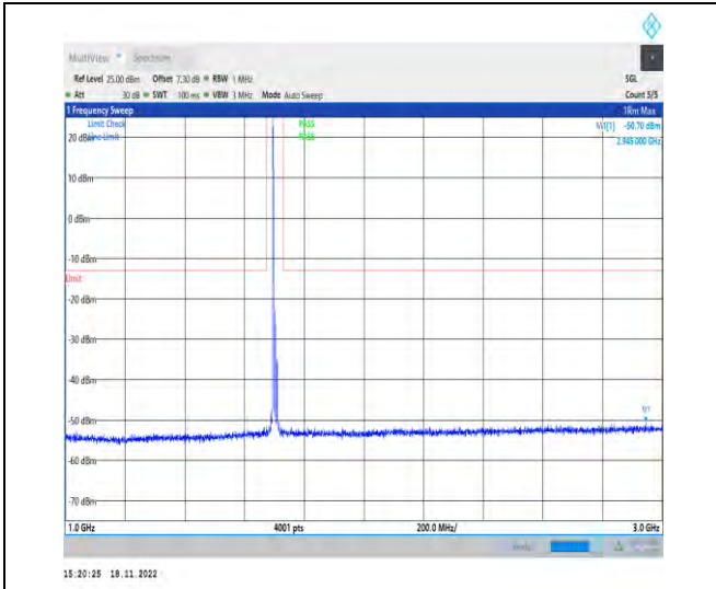
1-N70-PC3-15-15-M-1-DFT-PI2BPSK-Inner_1RB_Le ft-1@1-1000-3000-Ant1-2945.00--50.70--13-PASS
