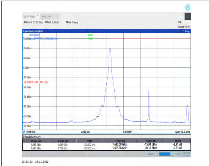
1-N70-PC3-15-10-L-1-DFT-PI2BPSK-Edge_1RB_Left-1@0-Ant1-1-seegraph-PASS-see graph
