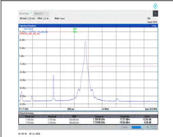
1-N70-PC3-15-10-H-5-CP-QPSK-Edge_1RB_Right-1@51-Ant1-1-seegraph-PASS-see graph
