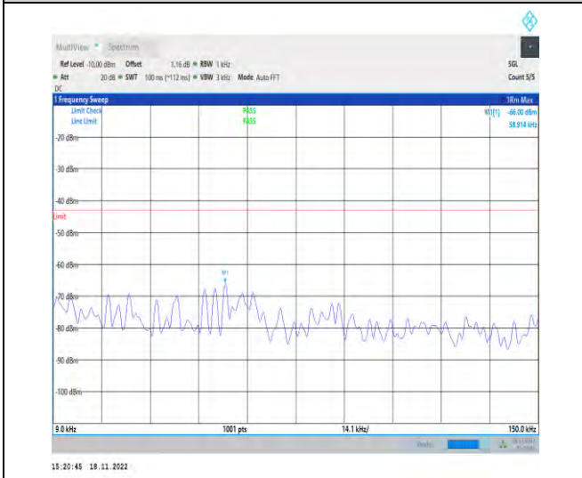
1-N70-PC3-15-15-H-1-DFT-PI2BPSK-Inner_1RB_Le ft-1@1-0.009-0.15-Ant1-0.06--66.00--43-PASS
