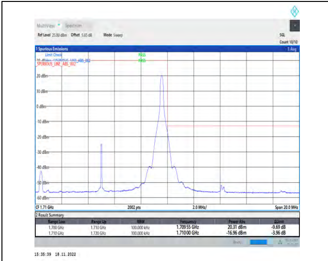
1-N70-PC3-15-10-H-2-DFT-PI2BPSK-Edge_1RB_Right-t@51-Ant1-1-seegraph-PASS-see graph
