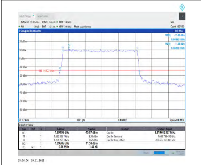
1-N70-PC3-15-10-L-4-DFT-64QAM-Outer_Full-50 @0-Ant1-8.92-9.560-≤10-PASS
