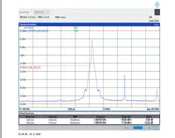
1-N70-PC3-15-10-L-4-CP-QPSK-Edge_1RB_Left-1@0-Ant1-1-seegraph-PASS-see graph
