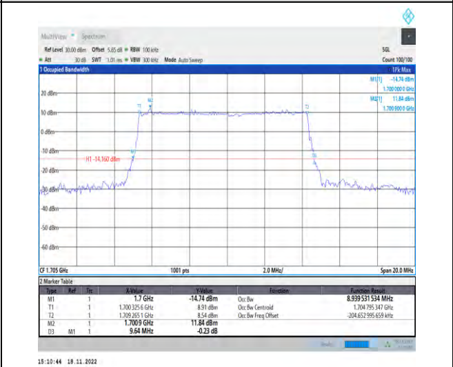
1-N70-PC3-15-10-H-3-DFT-16QAM-Outer_Full-50@ 0-Ant1-8.94-9.640-≤10-PASS
