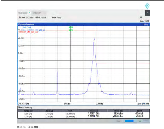
1-N70-PC3-15-15-H-5-CP-QPSK-Edge_1RB_Right1@78-Ant1-1-seegraph-PASS-see graph
