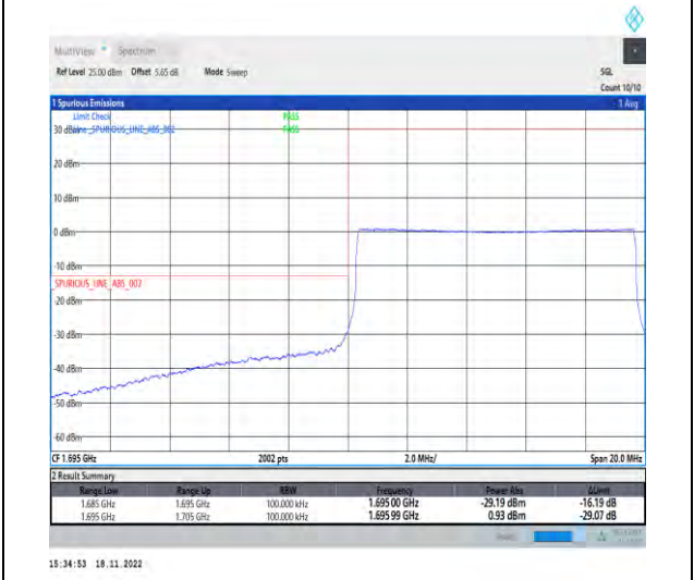
1-N70-PC3-15-10-L-6-CP-QPSK-Outer_Full-52@0-Ant1-1-seegraph-PASS-see graph
