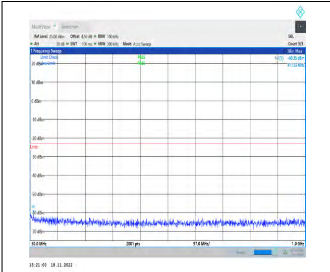
1-N70-PC3-15-15-H-1-DFT-PI2BPSK-Inner_1RB_Le ft-1@1-30-1000-Ant1-41.16--60.35--23-PASS
