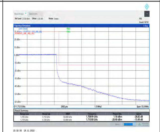
1-N70-PC3-15-5-H-6-CP-QPSK-Outer_Full-25@0-Ant1-1-seegraph-PASS-see graph
