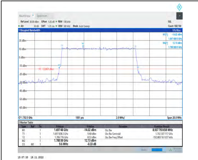
1-N70-PC3-15-10-M-1-DFT-QPSK-Outer_Full-50@0 -Ant1-8.938-9.600-≤10-PASS
