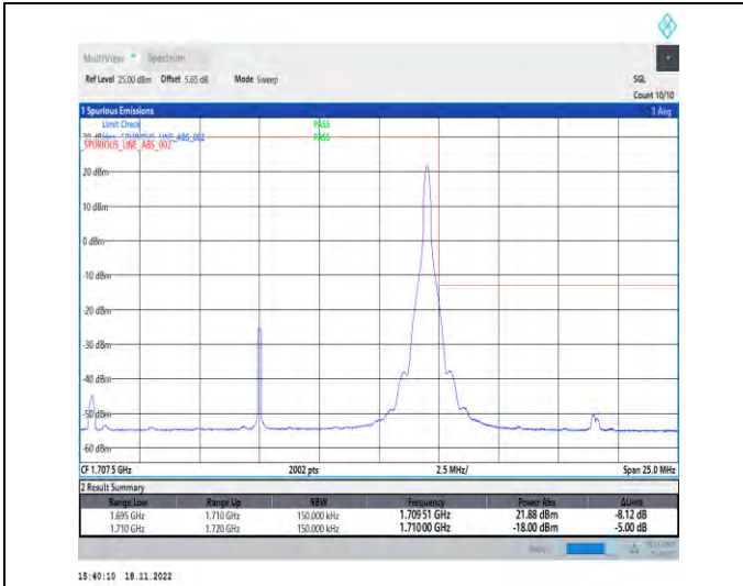
1-N70-PC3-15-15-H-2-DFT-PI2BPSK-Edge_1RB_Right-t1@78-Ant1-1-seegraph-PASS-see graph
