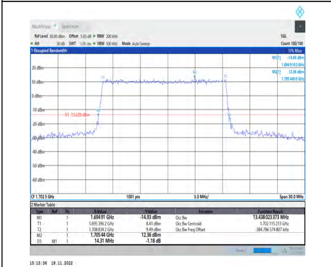
1-N70-PC3-15-15-M-4-DFT-64QAM-Outer_Full-75 @0-Ant1-13.438-14.310-≤15-PASS
