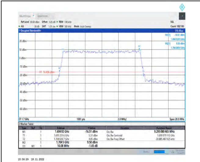
1-N70-PC3-15-10-L-6-CP-QPSK-Outer_Full-52@0-A Ant1-9.295-10.080-≤10-PASS
