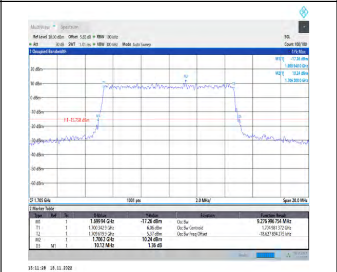
1-N70-PC3-15-10-H-7-CP-16QAM-Outer_Full-52@0 -Ant1-9.277-10.120-≤10-PASS
