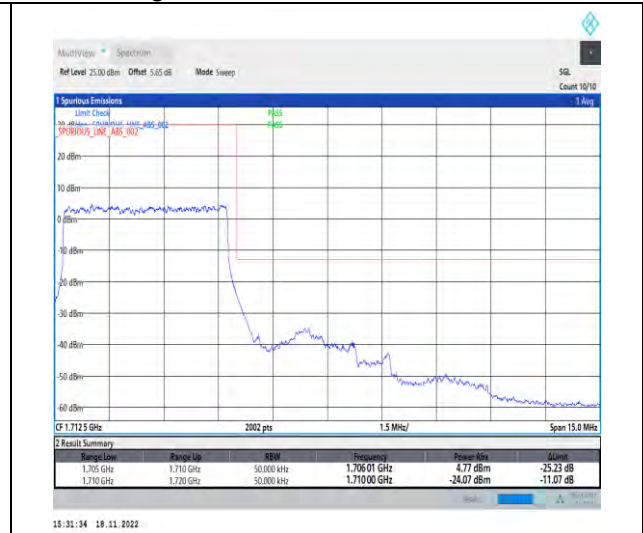
1-N70-PC3-15-5-H-3-DFT-PI2BPSK-Outer_Full-25@0-Ant1-1-seegraph-PASS-see graph
