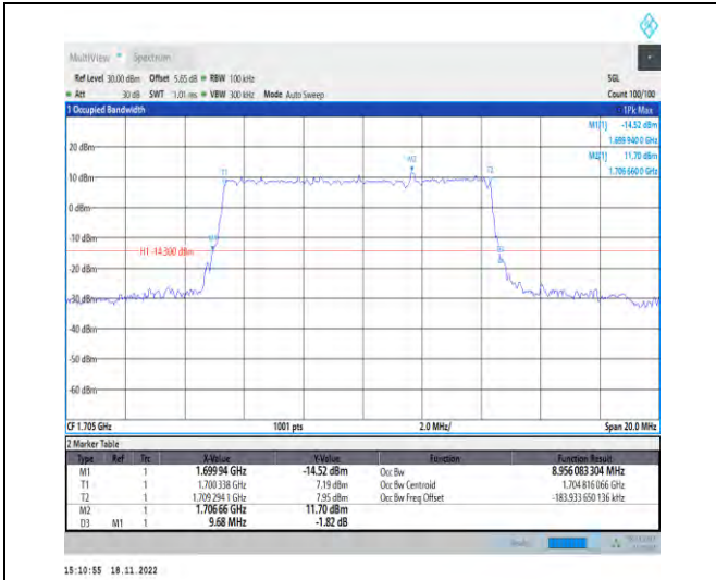
1-N70-PC3-15-10-H-4-DFT-64QAM-Outer_Full-50@ 0-Ant1-8.956-9.680-≤10-PASS
