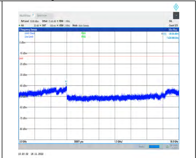
1-N70-PC3-15-15-M-1-DFT-PI2BPSK-Inner_1RB_Le ft-1@1-3000-18000-Ant1-7428.00--39.56--13-PASS
