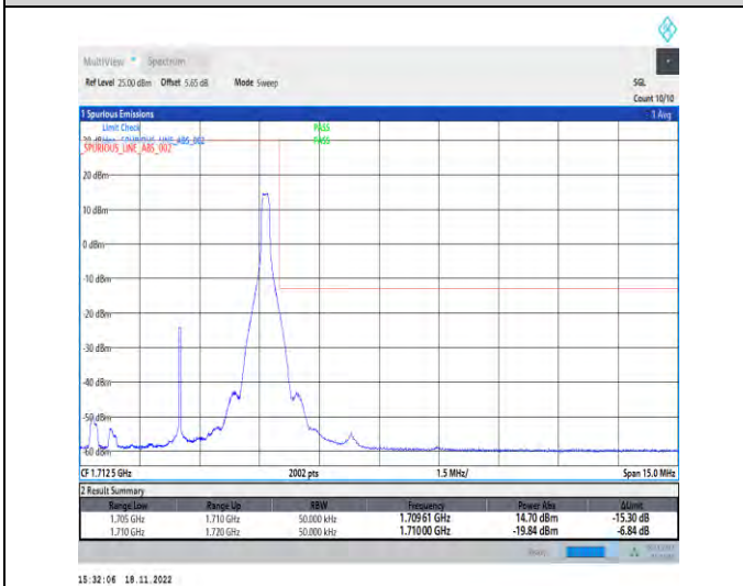
1-N70-PC3-15-5-H-5-CP-QPSK-Edge_1RB_Right-1@24-Ant1-1-seegraph-PASS-see graph
