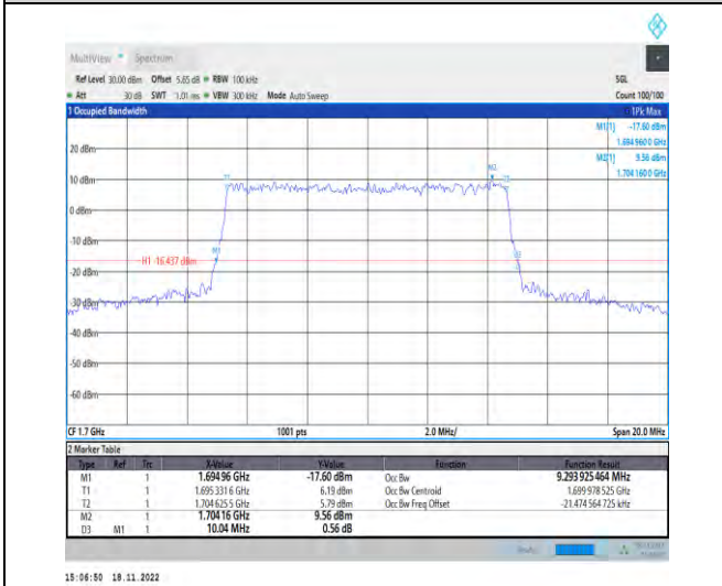
1-N70-PC3-15-10-L-8-CP-64QAM-Outer_Full-52@0- Ant1-9.294-10.040-≤10-PASS
