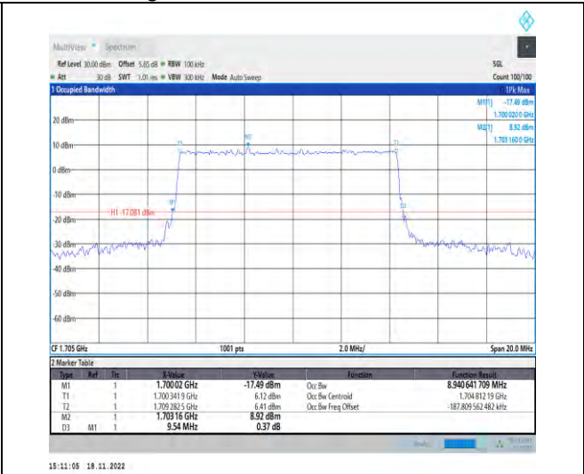
1-N70-PC3-15-10-H-5-DFT-256QAM-Outer_Full-50 @0-Ant1-8.941-9.540-≤10-PASS
