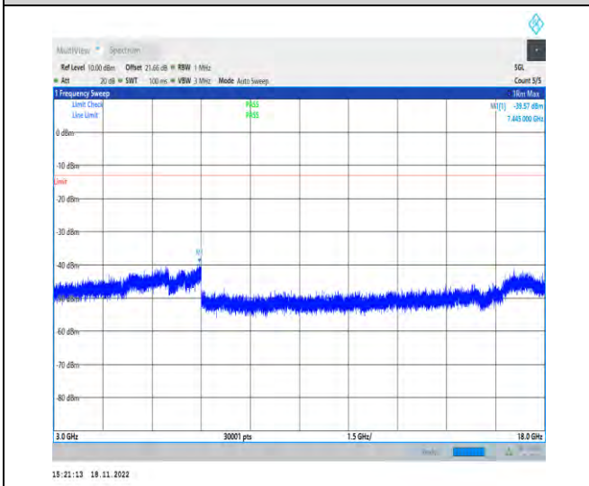
1-N70-PC3-15-15-H-1-DFT-PI2BPSK-Inner_1RB_Le ft-1@1-3000-18000-Ant1-7445.00--39.57--13-PASS
