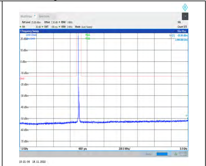
1-N70-PC3-15-15-H-1-DFT-PI2BPSK-Inner_1RB_Le ft-1@1-1000-3000-Ant1-2996.00--50.89--13-PASS
