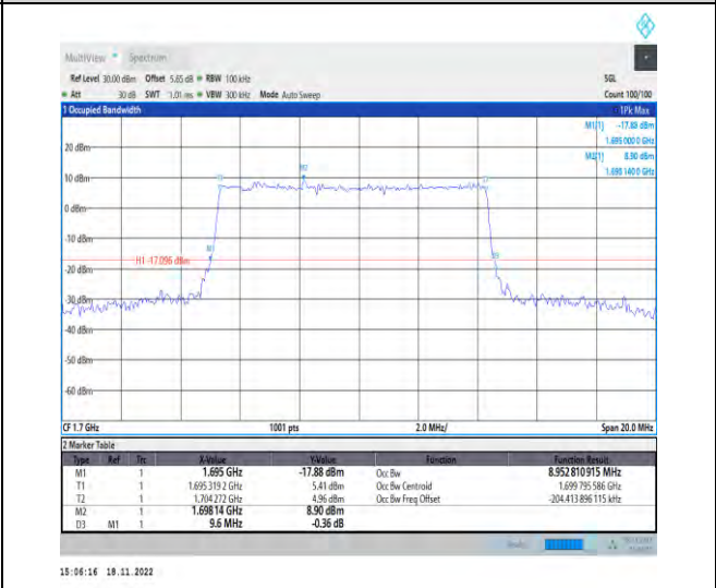
1-N70-PC3-15-10-L-5-DFT-256QAM-Outer_Full-50 @0-Ant1-8.953-9.600-≤10-PASS
