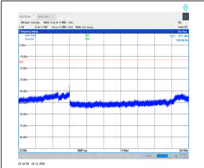
1-N70-PC3-15-15-L-1-DFT-PI2BPSK-Inner_1RB_Lef t-1@1-3000-18000-Ant1-7489.50--39.71--13-PASS
