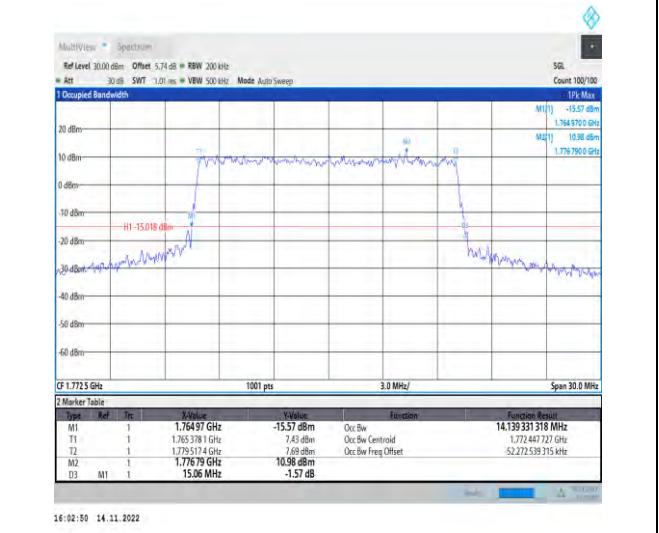
1-N66-PC3-15-15-H-8-CP-64QAM-Outer_Full-79@0 -Ant1-14.139-15.060-≤15-PASS
