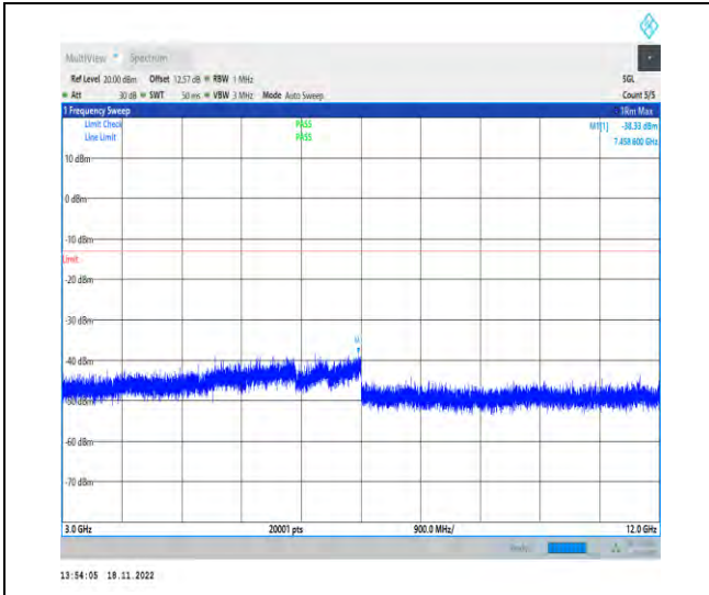
1-N66-PC3-15-40-H-1-DFT-PI2BPSK-Inner_1RB_L eft-1@1-3000-12000-Ant1-7458.60--38.33--13-PAS S
