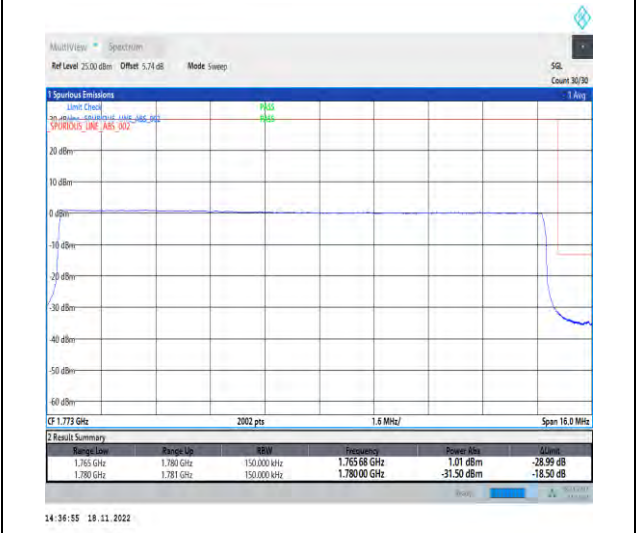
1-N66-PC3-15-15-H-6-CP-QPSK-Outer_Full-79@ 0-Ant1-1-seegraph-PASS-see graph
