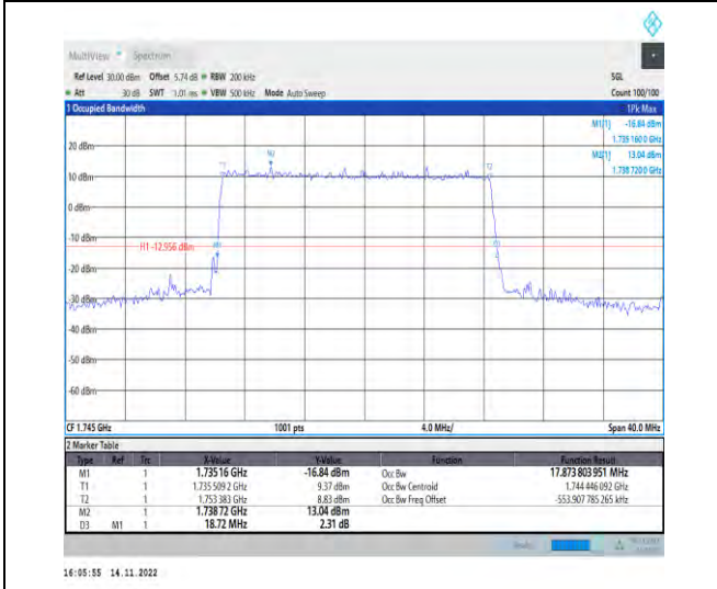
1-N66-PC3-15-20-M-1-DFT-QPSK-Outer_Full-100@ 0-Ant1-17.874-18.720-<20-PASS
