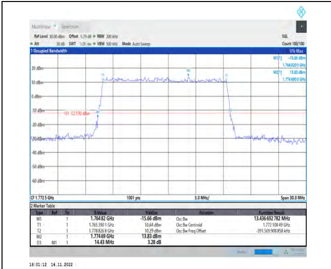
1-N66-PC3-15-15-H-1-DFT-QPSK-Outer_Full-75@0-Ant1-13.437-14.430-≤15-PASS
