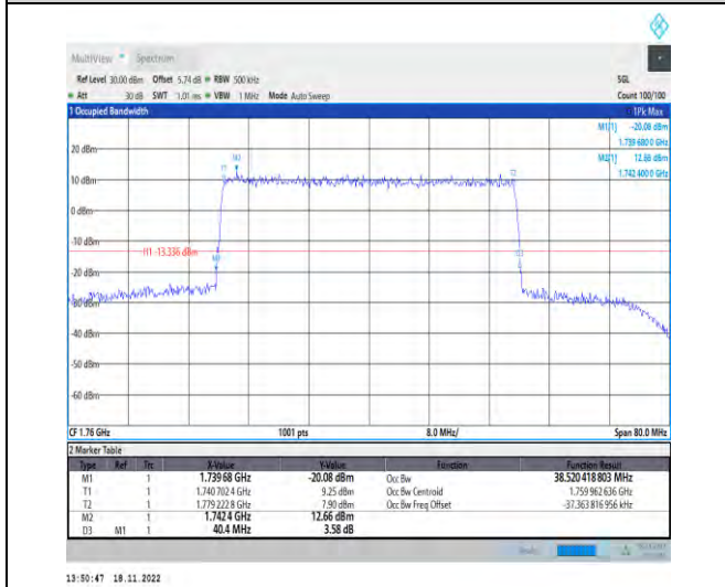
1-N66-PC3-15-40-H-6-CP-QPSK-Outer_Full-216@0 -Ant1-38.52-40.400-≤40-PASS
