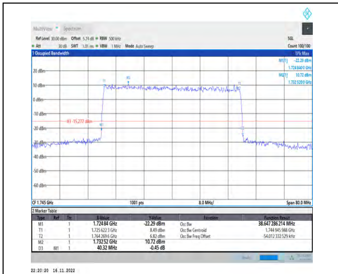
1-N66-PC3-15-40-M-5-DFT-256QAM-Outer_Full-216 @0-Ant1-38.647-40.320-≤40-PASS
