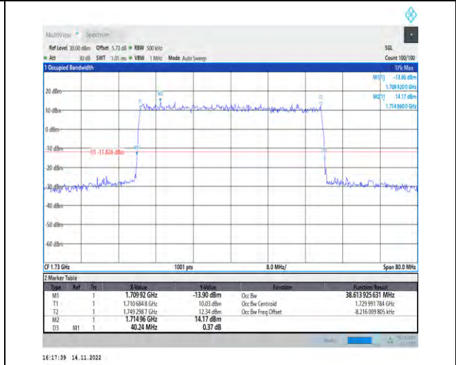
1-N66-PC3-15-40-L-1-DFT-QPSK-Outer_Full-216@ 0-Ant1-38.614-40.240-≤40-PASS
