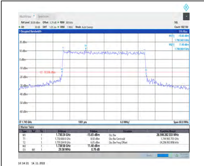
1-N66-PC3-15-30-M-8-CP-64QAM-Outer_Full-160@ 0-Ant1-28.598-29.580-≤30-PASS
