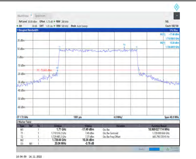
1-N66-PC3-15-20-L-7-CP-16QAM-Outer_Full-106@0-Ant1-18.969-20.040-≤20-PASS
