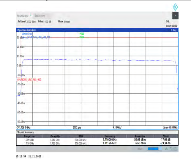
1-N66-PC3-15-40-L-3-DFT-PI2BPSK-Outer_Full-216@0-Ant1-1-seegraph-PASS-see graph
