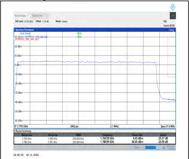
1-N66-PC3-15-20-H-3-DFT-PI2BPSK-Outer_Full-100@0-Ant1-1-seegraph-PASS-see graph
