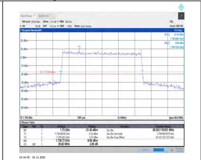
1-N66-PC3-15-30-M-9-CP-256QAM-Outer_Full-160 @0-Ant1-28.592-29.820-≤30-PASS
