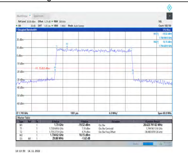
1-N66-PC3-15-30-M-5-DFT-256QAM-Outer_Full-160 @0-Ant1-28.624-29.880-≤30-PASS
