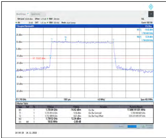
1-N66-PC3-15-20-M-3-DFT-16QAM-Outer_Full-100 @0-Ant1-17.898-18.920-≤20-PASS
