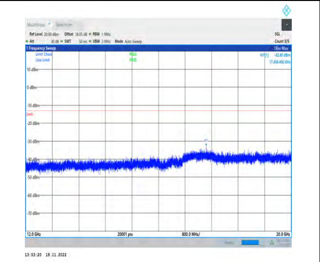
1-N66-PC3-15-40-M-1-DFT-PI2BPSK-Inner_1RB_Lef t-1@1-12000-20000-Ant1-17436.40--32.80--13-PASS
