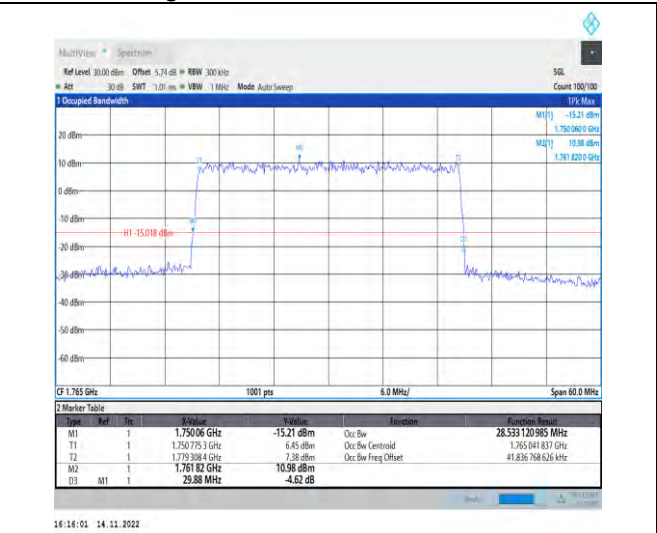
1-N66-PC3-15-30-H-4-DFT-64QAM-Outer_Full-160 @0-Ant1-28.533-29.880-≤30-PASS
