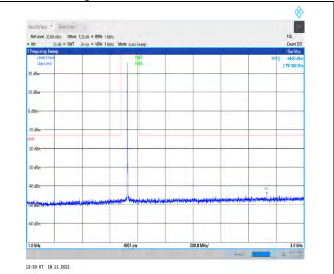
1-N66-PC3-15-40-M-1-DFT-PI2BPSK-Inner_1RB_Lef t-1@1-1000-3000-Ant1-2731.50--44.80--13-PASS
