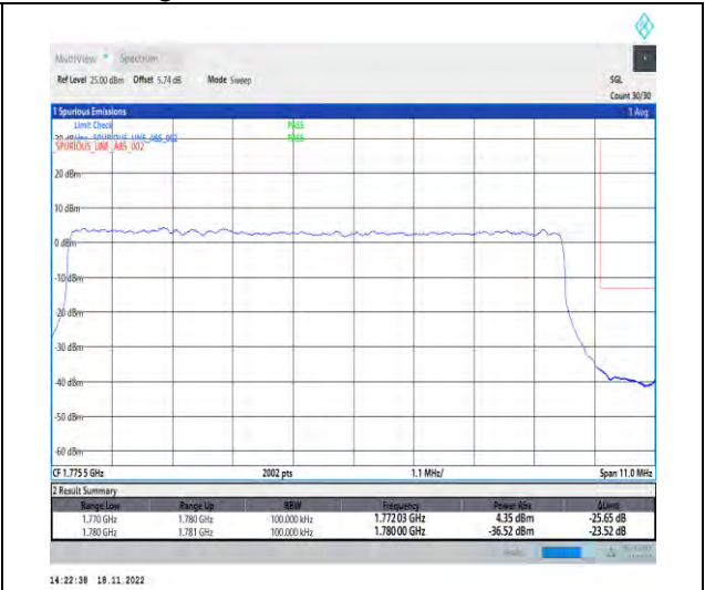
1-N66-PC3-15-10-H-3-DFT-PI2BPSK-Outer_Full-50@0-Ant1-1-seegraph-PASS-see graph
