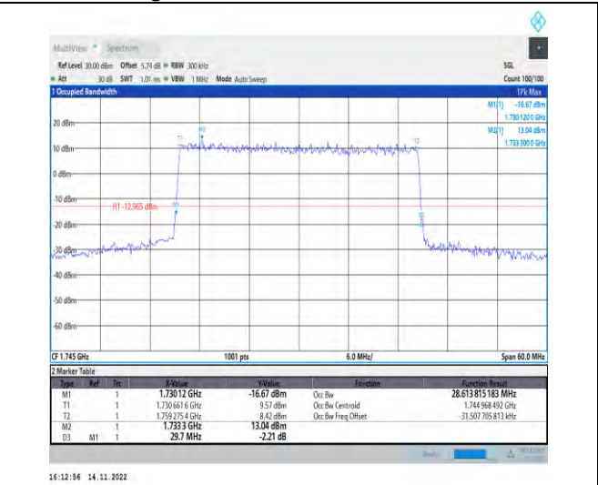
1-N66-PC3-15-30-M-1-DFT-QPSK-Outer_Full-160 @0-Ant1-28.614-29.700-≤30-PASS
