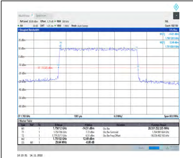
1-N66-PC3-15-30-H-3-DFT-16QAM-Outer_Full-160 @0-Ant1-28.551-29.640-≤30-PASS
