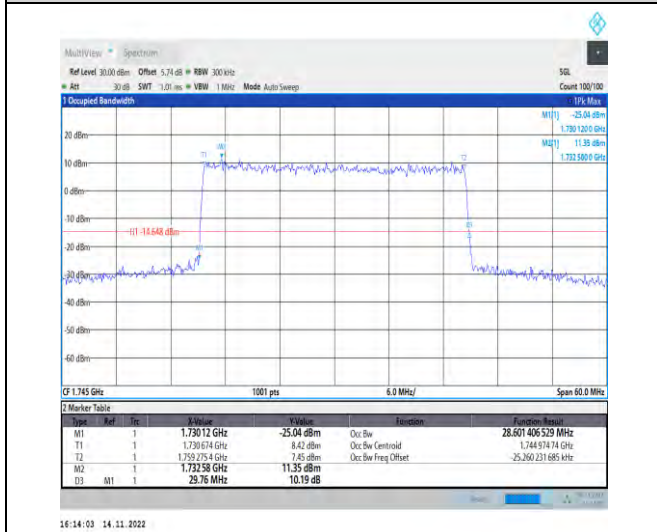
1-N66-PC3-15-30-M-6-CP-QPSK-Outer_Full-160@0 -Ant1-28.601-29.760-≤30-PASS
