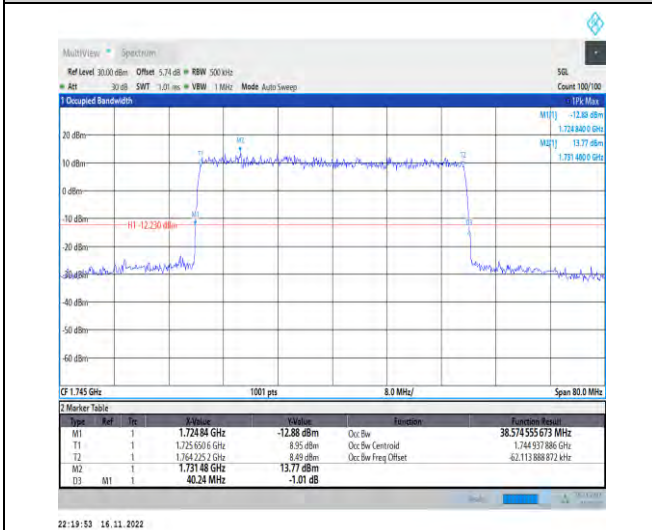
1-N66-PC3-15-40-M-3-DFT-16QAM-Outer_Full-216 @0-Ant1-38.575-40.240-≤40-PASS
