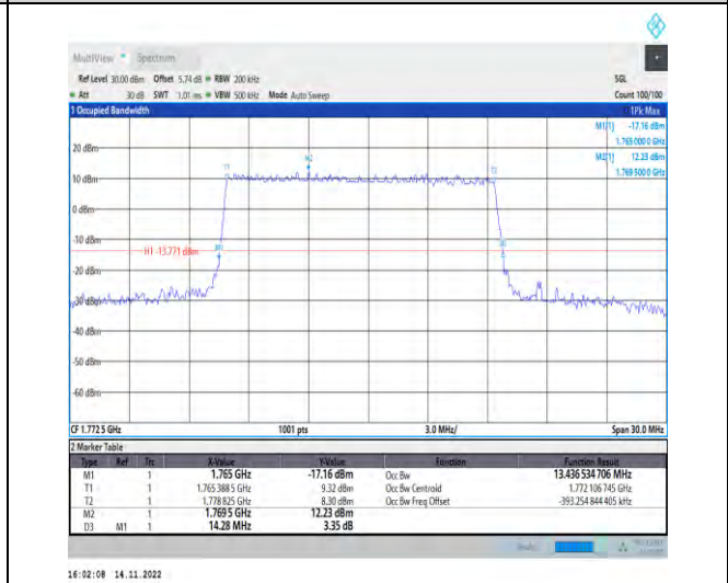
1-N66-PC3-15-15-H-4-DFT-64QAM-Outer_Full-75@0-Ant1-13.437-14.280-≤15-PASS
