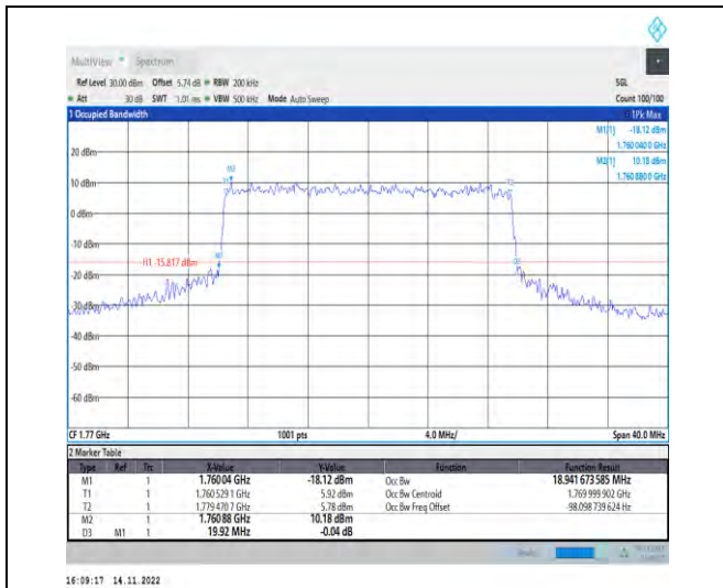
1-N66-PC3-15-20-H-6-CP-QPSK-Outer_Full-106@0 -Ant1-18.942-19.920-≤20-PASS
