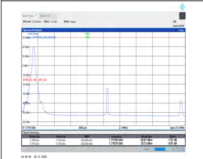
1-N66-PC3-15-20-L-4-CP-QPSK-Edge_1RB_Left-1@0-Ant1-1-seegraph-PASS-see graph
