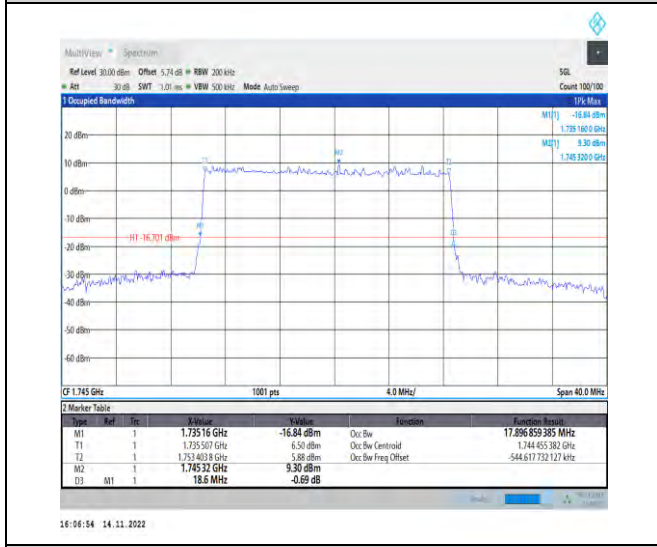
1-N66-PC3-15-20-M-5-DFT-256QAM-Outer_Full-100 @0-Ant1-17.897-18.600-≤20-PASS
