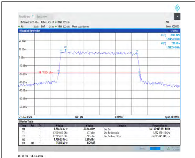
1-N66-PC3-15-15-H-9-CP-256QAM-Outer_Full-79@ 0-Ant1-14.133-15.030-≤15-PASS
