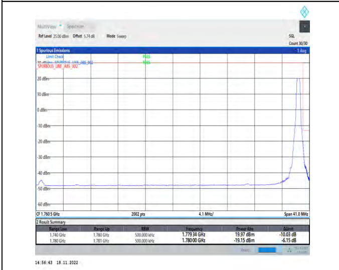
1-N66-PC3-15-40-H-5-CP-QPSK-Edge_1RB_Right-1@215-Ant1-1-seegraph-PASS-see graph
