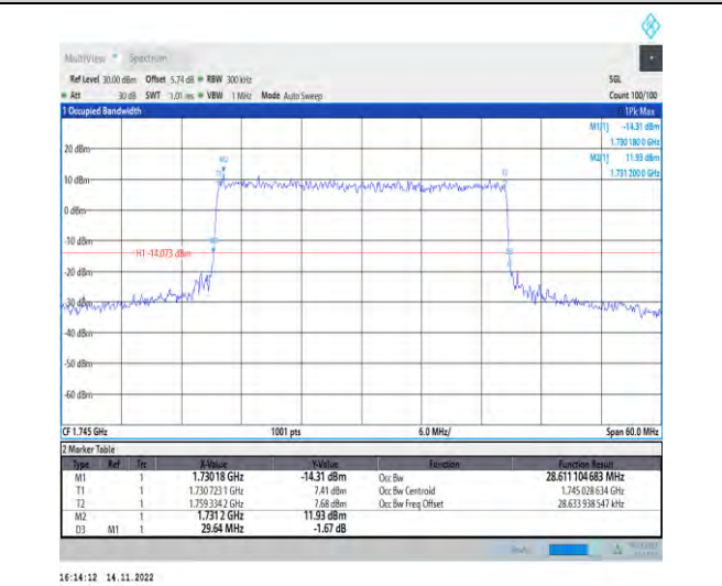
1-N66-PC3-15-30-M-7-CP-16QAM-Outer_Full-160@0 -Ant1-28.611-29.640-≤30-PASS
