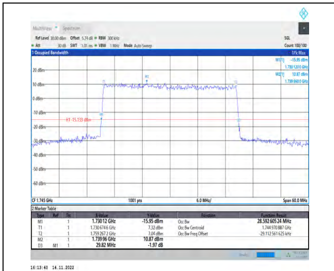
1-N66-PC3-15-30-M-4-DFT-64QAM-Outer_Full-160 @0-Ant1-28.593-29.820-≤30-PASS
