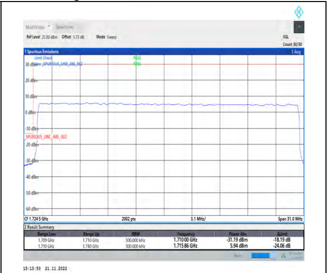
1-N66-PC3-15-30-L-3-DFT-PI2BPSK-Outer_Full-160@0-Ant1-1-seegraph-PASS-see graph
