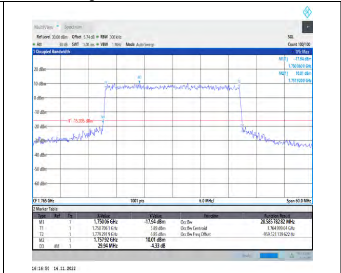
1-N66-PC3-15-30-H-8-CP-64QAM-Outer_Full-160@ 0-Ant1-28.586-29.940-≤30-PASS
