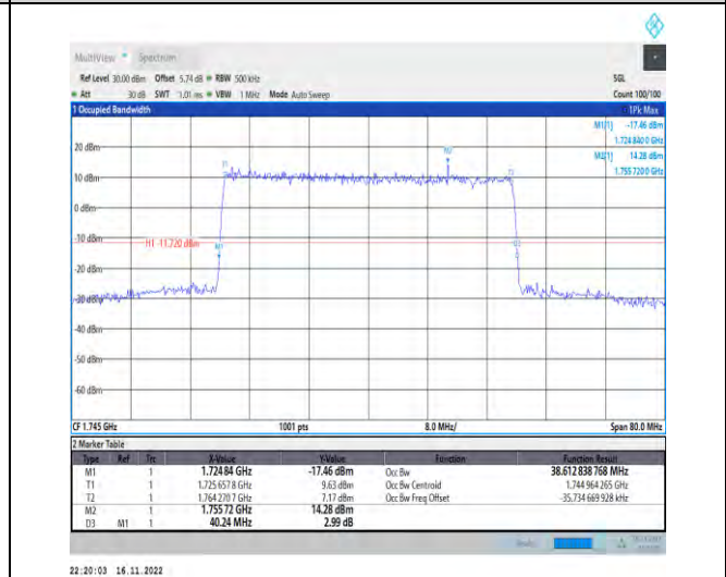
1-N66-PC3-15-40-M-4-DFT-64QAM-Outer_Full-216 @0-Ant1-38.613-40.240-≤40-PASS
