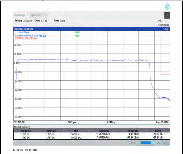
1-N66-PC3-15-15-H-3-DFT-PI2BPSK-Outer_Full-7 5@0-Ant1-1-seegraph-PASS-see graph
