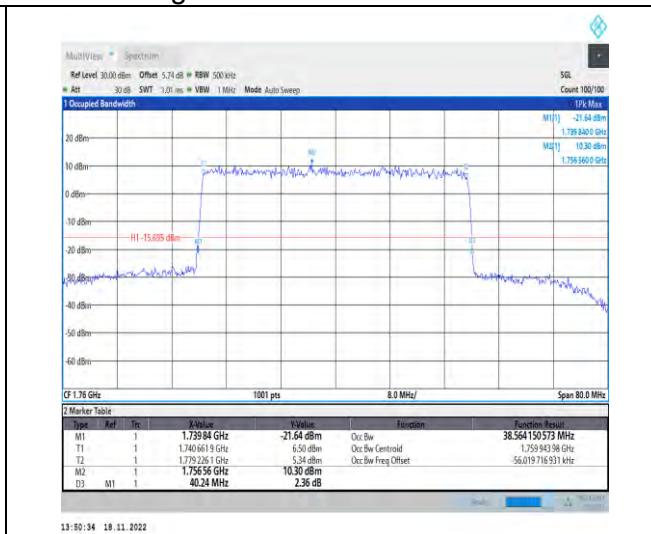
1-N66-PC3-15-40-H-5-DFT-256QAM-Outer_Full-216 @0-Ant1-38.564-40.240-≤40-PASS
