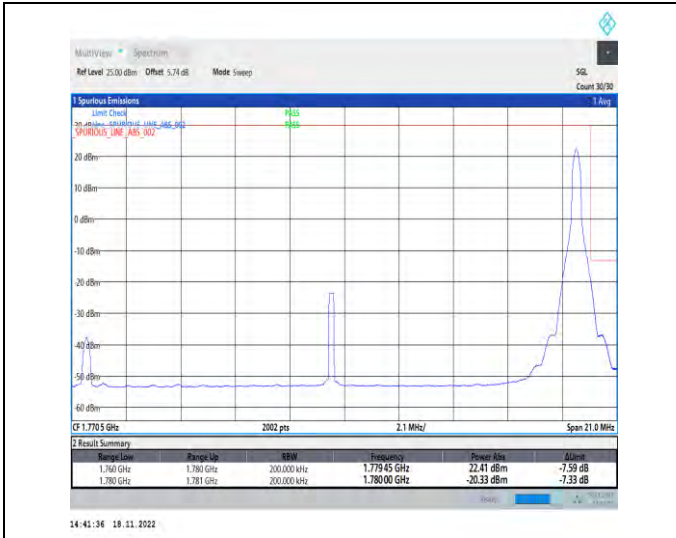
1-N66-PC3-15-20-H-2-DFT-PI2BPSK-Edge_1RB_Right-t-1@105-Ant1-1-seegraph-PASS-see graph
