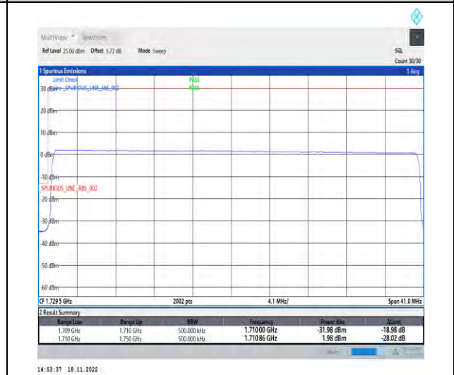
1-N66-PC3-15-40-L-6-CP-QPSK-Outer_Full-216@0-Ant1-1-seegraph-PASS-see graph
