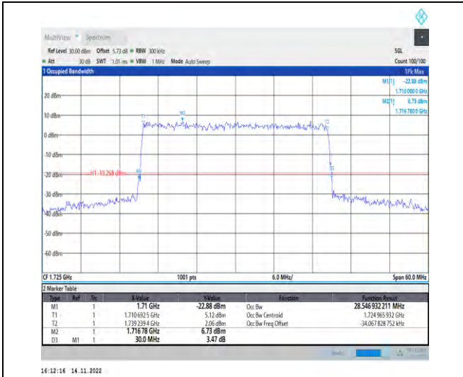
1-N66-PC3-15-30-L-9-CP-256QAM-Outer_Full-160 @0-Ant1-28.547-30.000-≤30-PASS
