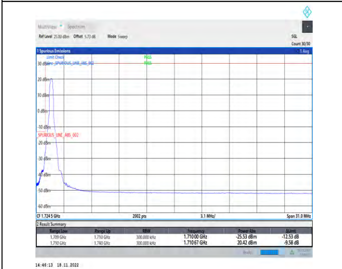
1-N66-PC3-15-30-L-4-CP-QPSK-Edge_1RB_Left-1@0-Ant1-1-seegraph-PASS-see graph
