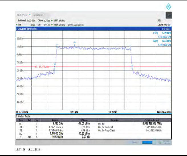
1-N66-PC3-15-20-M-6-CP-QPSK-Outer_Full-106@0 -Ant1-18.934-19.920-≤20-PASS
