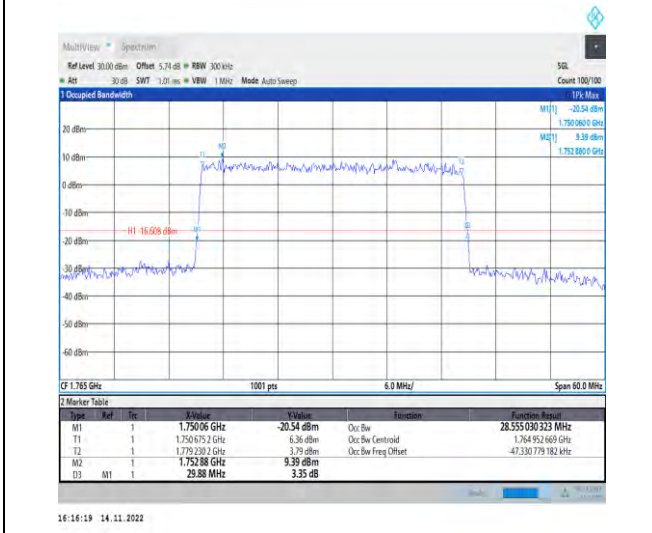
1-N66-PC3-15-30-H-5-DFT-256QAM-Outer_Full-160 @0-Ant1-28.555-29.880-≤30-PASS
