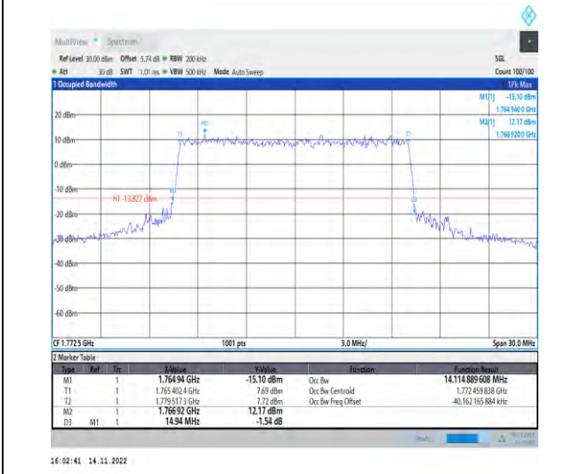
1-N66-PC3-15-15-H-7-CP-16QAM-Outer_Full-79@0 -Ant1-14.115-14.940-≤15-PASS
