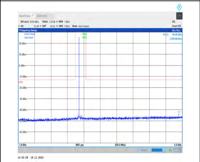
1-N66-PC3-15-40-H-1-DFT-PI2BPSK-Inner_1RB_L ef t-1@1-1000-3000-Ant1-2959.00--45.48--13-PASS
