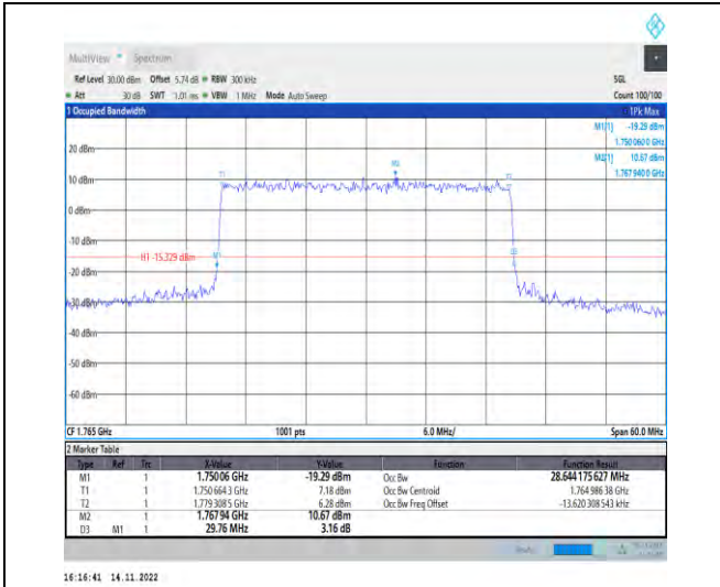
1-N66-PC3-15-30-H-7-CP-16QAM-Outer_Full-160@ 0-Ant1-28.644-29.760-≤30-PASS
