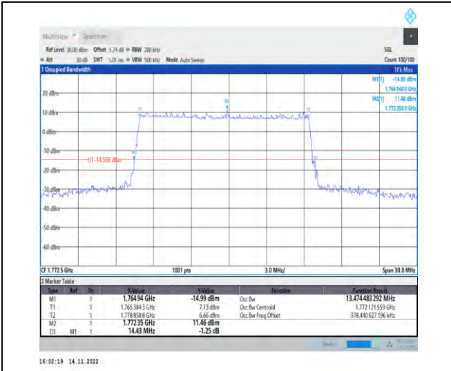
1-N66-PC3-15-15-H-5-DFT-256QAM-Outer_Full-75 @0-Ant1-13.474-14.430-≤15-PASS
