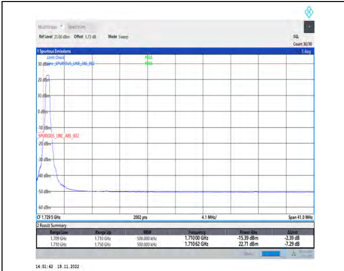
1-N66-PC3-15-40-L-1-DFT-PI2BPSK-Edge_1RB_Left-1@0-Ant1-1-seegraph-PASS-see graph
