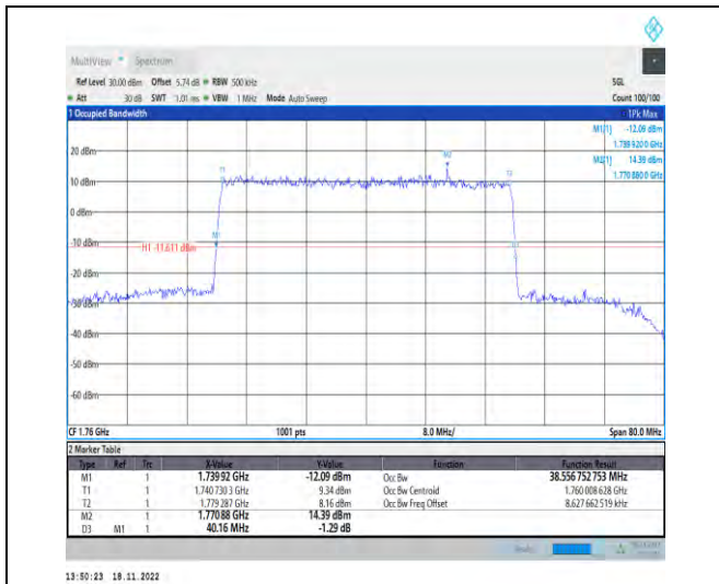
1-N66-PC3-15-40-H-4-DFT-64QAM-Outer_Full-216 @0-Ant1-38.557-40.160-≤40-PASS
