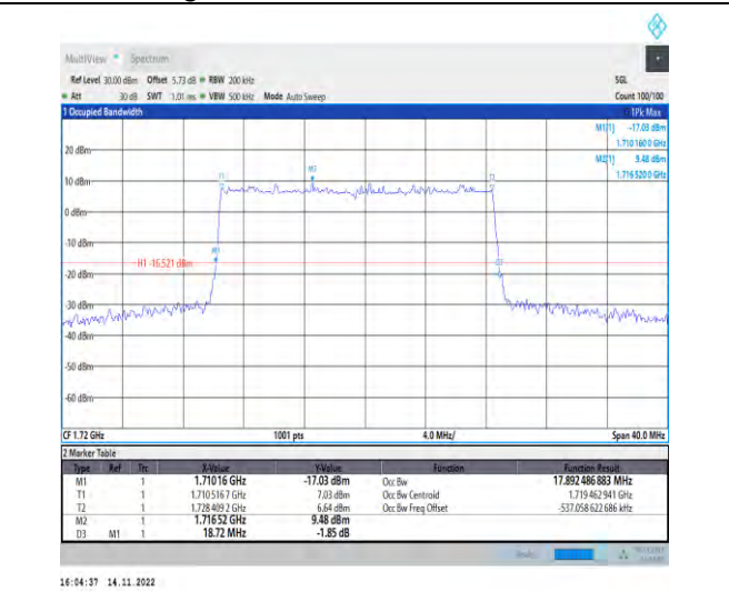
1-N66-PC3-15-20-L-5-DFT-256QAM-Outer_Full-100 @0-Ant1-17.892-18.720-≤20-PASS
