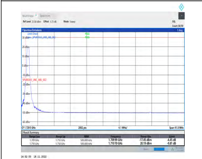
1-N66-PC3-15-40-L-4-CP-QPSK-Edge_1RB_Left-1@0-Ant1-1-seegraph-PASS-see graph
