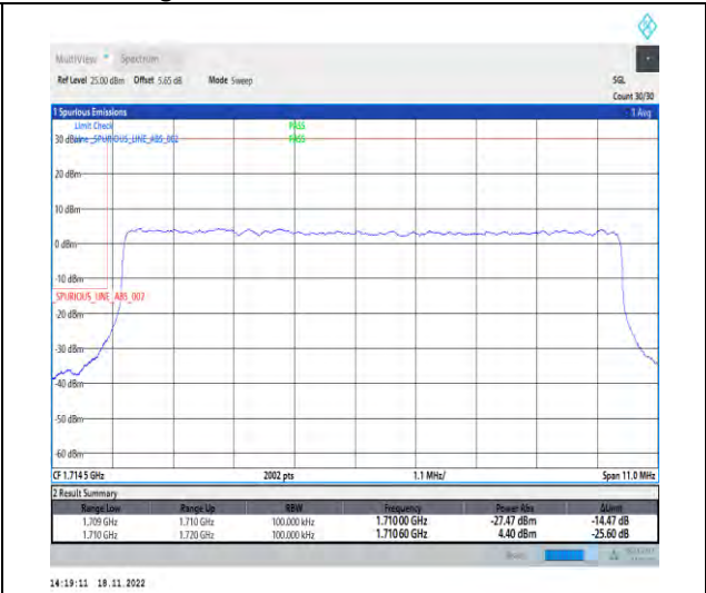
1-N66-PC3-15-10-L-3-DFT-PI2BPSK-Outer_Full-50@0-Ant1-1-seegraph-PASS-see graph
