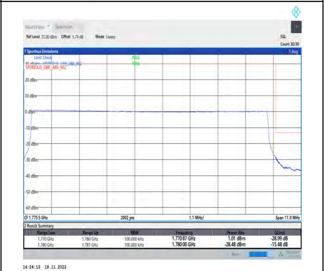
1-N66-PC3-15-10-H-6-CP-QPSK-Outer_Full-52@0-Ant1-1-seegraph-PASS-see graph
