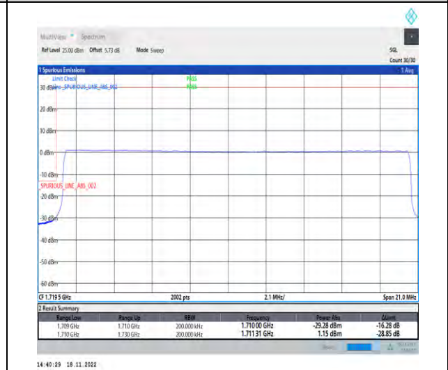
1-N66-PC3-15-20-L-6-CP-QPSK-Outer_Full-106@0-Ant1-1-seegraph-PASS-see graph
