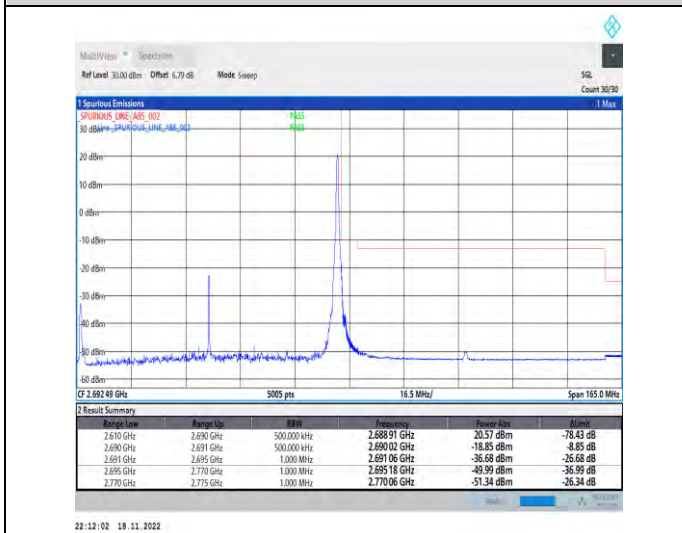
1-N41-PC2-30-80-H-5-CP-QPSK-Edge_1RB_Right-1 @216-Ant1-1--PASS-see graph
