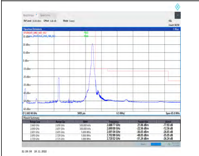
1-N41-PC2-30-30-H-5-CP-QPSK-Edge_1RB_Right-1 @77-Ant1-1--PASS-see graph
