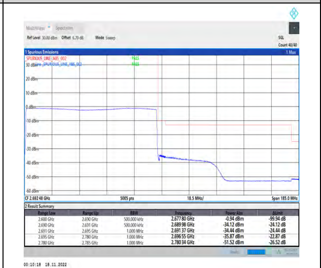
1-N41-PC2-30-90-H-6-CP-QPSK-Outer_Full-245 @0-Ant1-1--PASS-see graph
