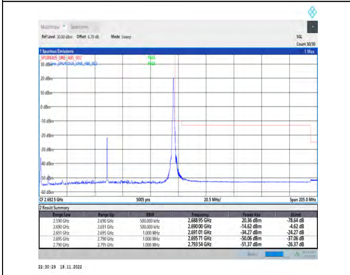
1-N41-PC2-30-100-H-5-CP-QPSK-Edge_1RB_Right-1 @272-Ant1-1--PASS-see graph
