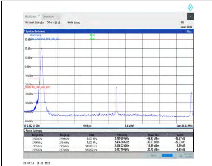
1-N41-PC2-30-80-L-4-CP-QPSK-Edge_1RB_Left-1@0 -Ant1-1--PASS-see graph
