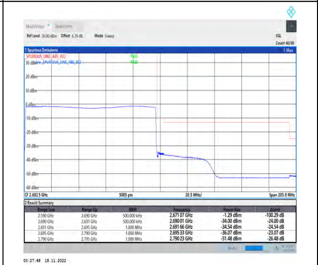
1-N41-PC2-30-100-H-6-CP-QPSK-Outer_Full-273 @0-Ant1-1--PASS-see graph
