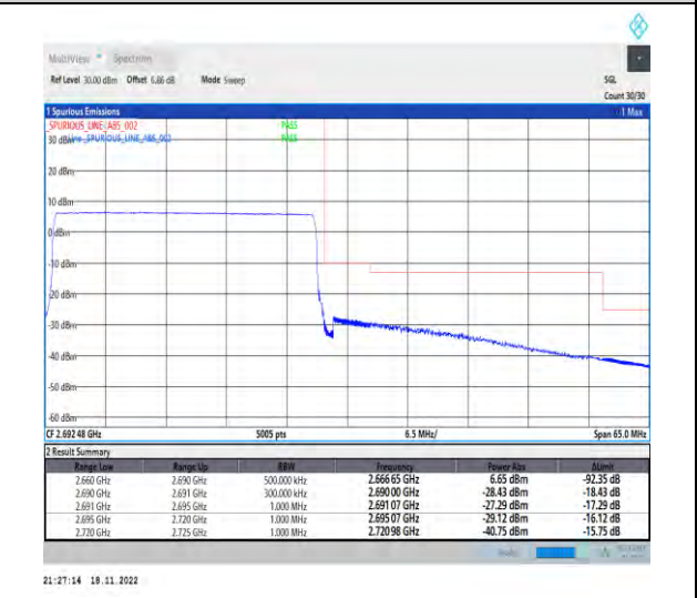
1-N41-PC2-30-30-H-6-CP-QPSK-Outer_Full-78@ 0-Ant1-1--PASS-see graph
