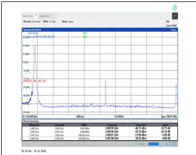
1-N41-PC2-30-100-L-4-CP-QPSK-Edge_1RB_Left-1@ 0-Ant1-1--PASS-see graph
