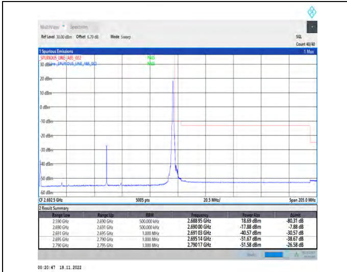
1-N41-PC2-30-100-H-2-DFT-PI2BPSK-Edge_1RB_Rig ht-1@272-Ant1-1--PASS-see graph
