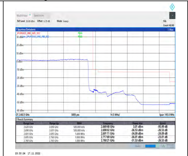
1-N41-PC2-30-70-H-3-DFT-PI2BPSK-Outer_Full-1 80@0-Ant1-1--PASS-see graph
