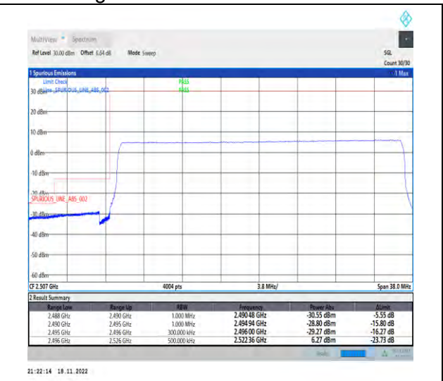
1-N41-PC2-30-30-L-6-CP-QPSK-Outer_Full-78@ 0-Ant1-1--PASS-see graph
