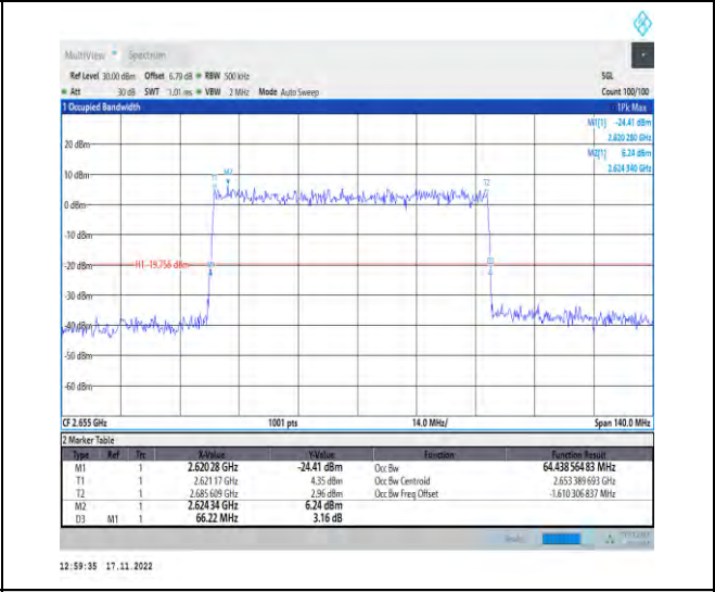
1-N41-PC2-30-70-H-5-DFT-256QAM-Outer_Full-180 @0-Ant1-64.439-66.220-≤70-PASS
