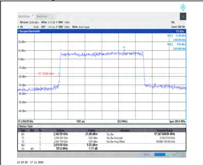
1-N41-PC2-30-100-M-7-CP-16QAM-Outer_Full-273@0-Ant1-97.368-101.000-≤100-PASS
