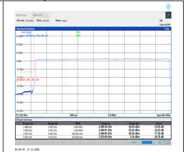
1-N41-PC2-30-60-L-3-DFT-PI2BPSK-Outer_Full-162@0-Ant1-1--PASS-see graph
