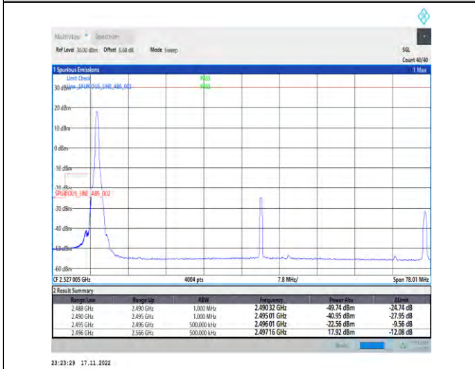
1-N41-PC2-30-70-L-4-CP-QPSK-Edge_1RB_Left-1@0-Ant1-1--PASS-see graph
