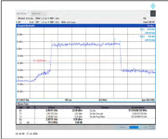
1-N41-PC2-30-100-L-7-CP-16QAM-Outer_Full-273 @0-Ant1-97.576-101.000-≤100-PASS
