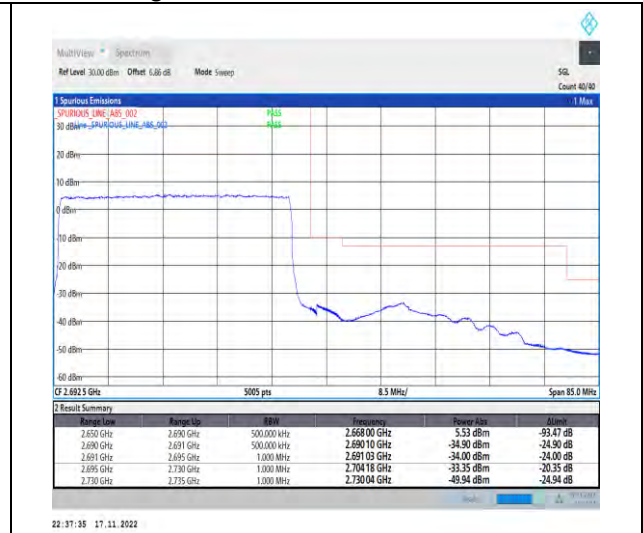
1-N41-PC2-30-40-H-3-DFT-PI2BPSK-Outer_Full-1 00@0-Ant1-1--PASS-see graph
