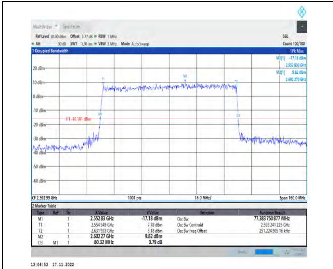
1-N41-PC2-30-80-M-8-CP-64QAM-Outer_Full-217@ 0-Ant1-77.384-80.320-<80-PASS
