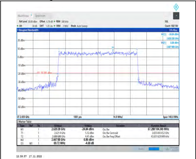
1-N41-PC2-30-70-H-7-CP-16QAM-Outer_Full-189@0-Ant1-67.288-69.720-≤70-PASS
