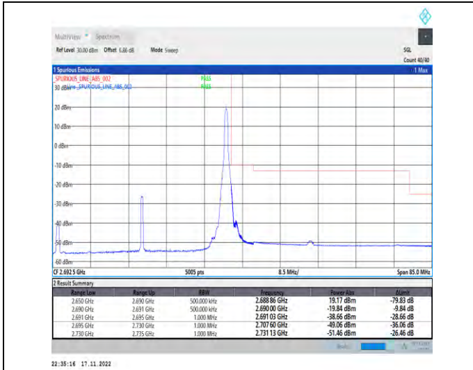
1-N41-PC2-30-40-H-2-DFT-PI2BPSK-Edge_1RB_Righ t-1@105-Ant1-1--PASS-see graph
