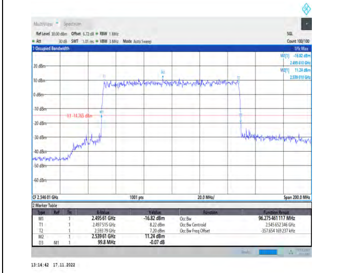
1-N41-PC2-30-100-L-1-DFT-QPSK-Outer_Full-270@ 0-Ant1-96.275-99.800-<=100-PASS
