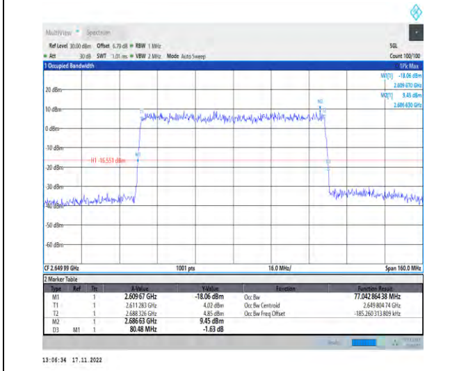
1-N41-PC2-30-80-H-5-DFT-256QAM-Outer_Full-216 @0-Ant1-77.043-80.480-≤80-PASS
