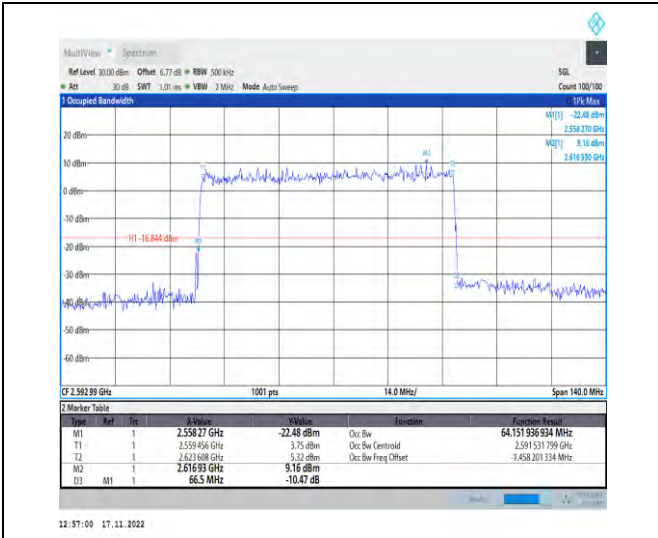
1-N41-PC2-30-70-M-3-DFT-16QAM-Outer_Full-180 @0-Ant1-64.152-66.500-≤70-PASS
