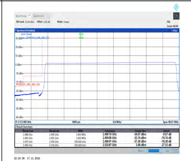
1-N41-PC2-30-40-L-6-CP-QPSK-Outer_Full-106@0-Ant1-1--PASS-see graph
