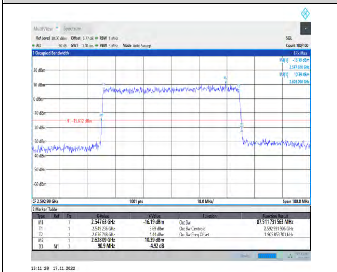
1-N41-PC2-30-90-M-7-CP-16QAM-Outer_Full-245@0-Ant1-87.512-90.900-≤90-PASS
