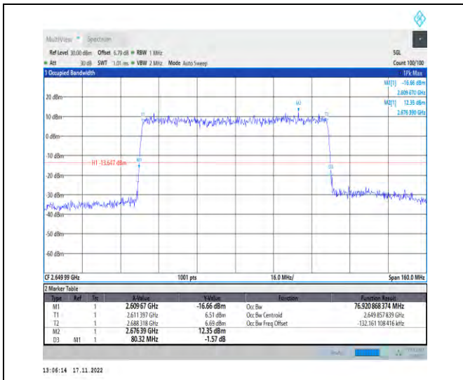
1-N41-PC2-30-80-H-3-DFT-16QAM-Outer_Full-216 @0-Ant1-76.921-80.320-≤80-PASS
