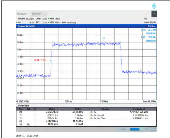
1-N41-PC2-30-80-M-4-DFT-64QAM-Outer_Full-216 @0-Ant1-76.921-80.320-≤80-PASS
