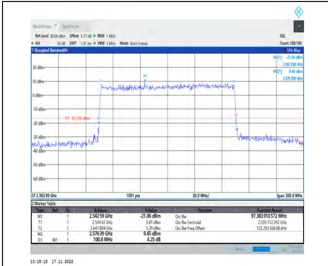
1-N41-PC2-30-100-M-6-CP-QPSK-Outer_Full-273@0-Ant1-97.384-100.800-≤100-PASS
