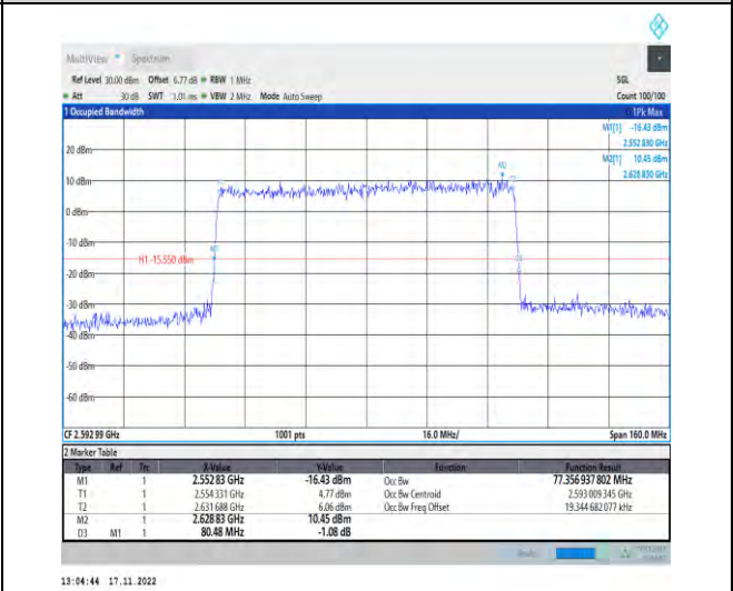
1-N41-PC2-30-80-M-7-CP-16QAM-Outer_Full-217@0-Ant1-77.357-80.480-≤80-PASS
