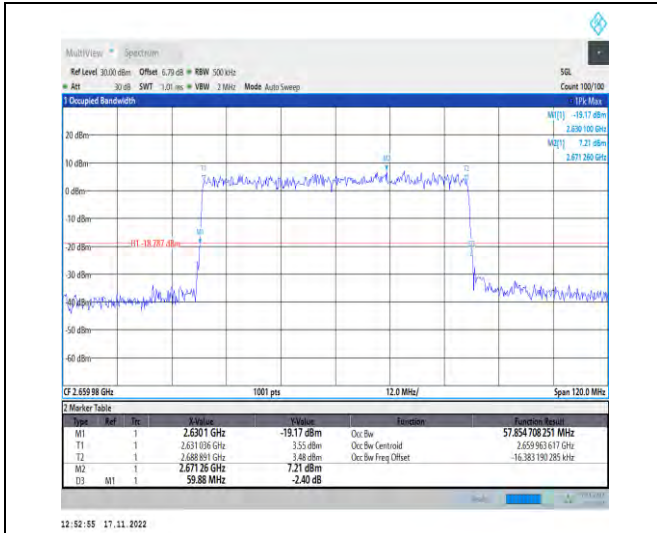
1-N41-PC2-30-60-H-5-DFT-256QAM-Outer_Full-162 @0-Ant1-57.855-59.880-≤60-PASS
