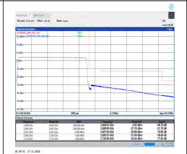
1-N41-PC2-30-30-H-6-CP-QPSK-Outer_Full-78@0-Ant1-1--PASS-see graph
