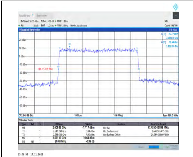
1-N41-PC2-30-80-H-7-CP-16QAM-Outer_Full-217@ 0-Ant1-77.436-80.480-≤80-PASS
