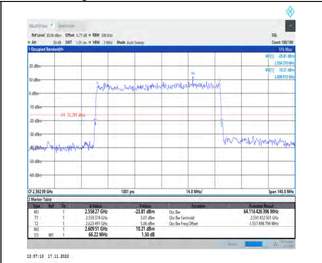
1-N41-PC2-30-70-M-4-DFT-64QAM-Outer_Full-180 @0-Ant1-64.116-66.220-≤70-PASS
