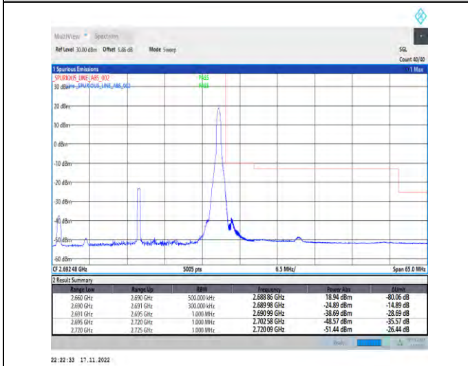
1-N41-PC2-30-30-H-5-CP-QPSK-Edge_1RB_Right-1@77-Ant1-1--PASS-see graph
