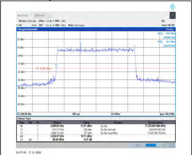
1-N41-PC2-30-80-H-8-CP-64QAM-Outer_Full-217@ 0-Ant1-77.356-80.640-≤80-PASS
