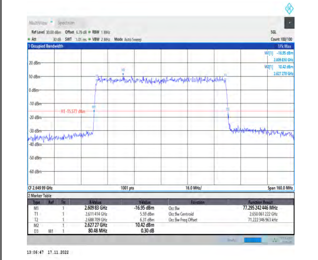
1-N41-PC2-30-80-H-6-CP-QPSK-Outer_Full-217@0-Ant1-77.295-80.480-≤80-PASS
