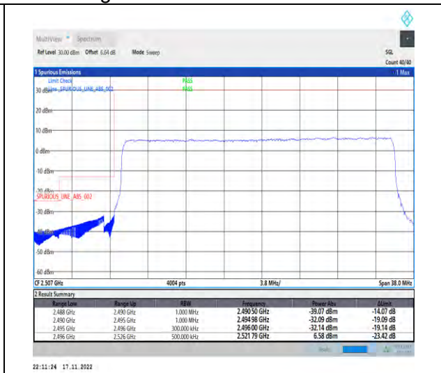
1-N41-PC2-30-30-L-3-DFT-PI2BPSK-Outer_Full-75@0-Ant1-1--PASS-see graph
