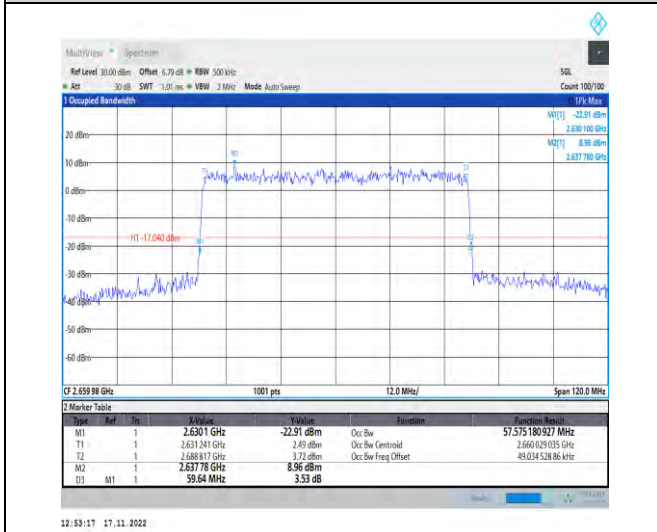
1-N41-PC2-30-60-H-7-CP-16QAM-Outer_Full-162@0-Ant1-57.575-59.640-≤60-PASS
