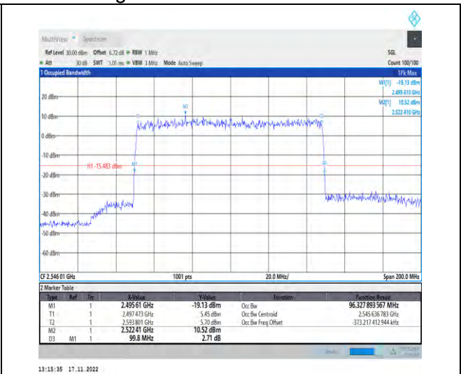
1-N41-PC2-30-100-L-4-DFT-64QAM-Outer_Full-270 @0-Ant1-96.328-99.800-≤100-PASS
