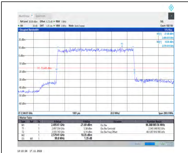
1-N41-PC2-30-100-L-3-DFT-16QAM-Outer_Full-270 @0-Ant1-96.389-99.800-≤100-PASS
