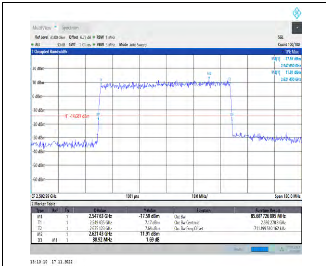
1-N41-PC2-30-90-M-1-DFT-QPSK-Outer_Full-240@0-Ant1-85.688-88.920-≤90-PASS
