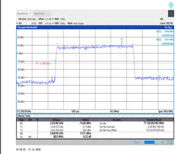
1-N41-PC2-30-80-M-3-DFT-16QAM-Outer_Full-216 @0-Ant1-77.12-80.000-<math>\leq 80</math>-PASS
