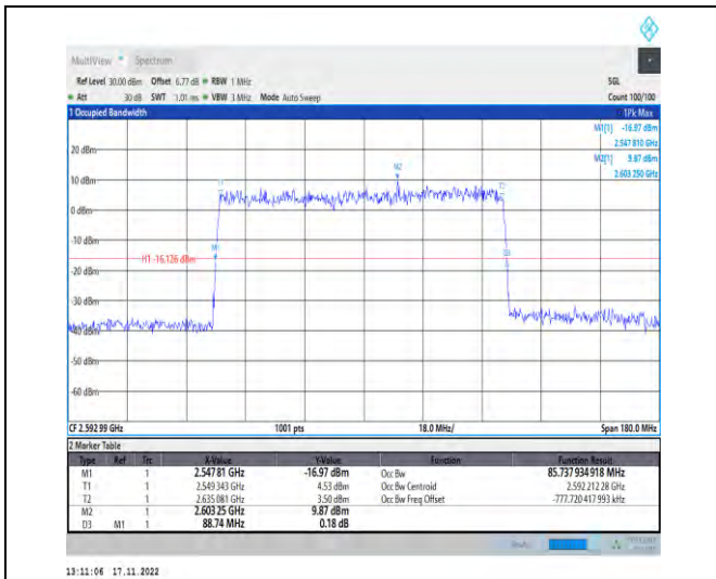
1-N41-PC2-30-90-M-5-DFT-256QAM-Outer_Full-240 @0-Ant1-85.738-88.740-≤90-PASS
