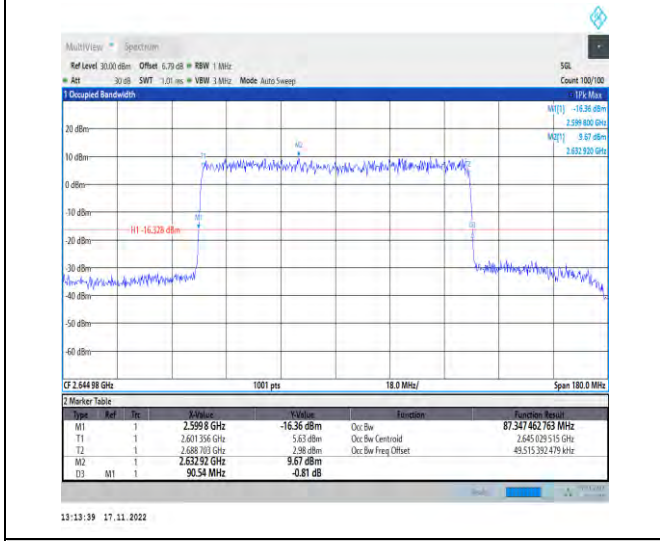
1-N41-PC2-30-90-H-6-CP-QPSK-Outer_Full-245@0-Ant1-87.347-90.540-≤90-PASS
