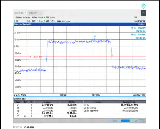
1-N41-PC2-30-90-M-4-DFT-64QAM-Outer_Full-240@0-Ant1-85.498-88.920-≤90-PASS
