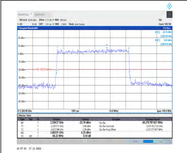
1-N41-PC2-30-70-M-5-DFT-256QAM-Outer_Full-180 @0-Ant1-64.271-66.220-≤70-PASS
