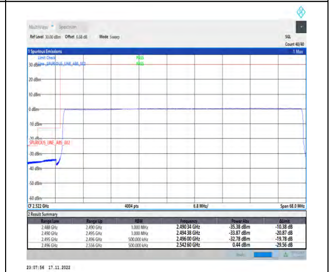
1-N41-PC2-30-60-L-6-CP-QPSK-Outer_Full-162@0-Ant1-1--PASS-see graph
