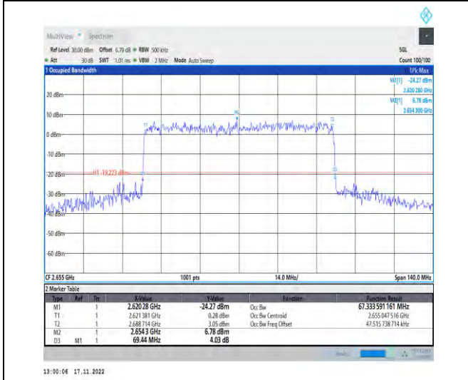
1-N41-PC2-30-70-H-8-CP-64QAM-Outer_Full-189@0-Ant1-67.334-69.440-≤70-PASS
