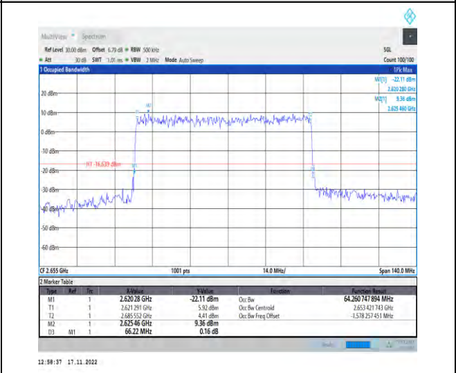
1-N41-PC2-30-70-H-1-DFT-QPSK-Outer_Full-180@ 0-Ant1-64.261-66.220-≤70-PASS
