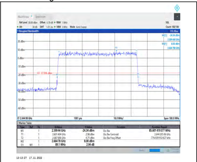
1-N41-PC2-30-90-H-5-DFT-256QAM-Outer_Full-240 @0-Ant1-85.601-89.100-≤90-PASS
