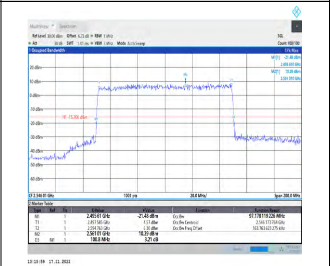
1-N41-PC2-30-100-L-6-CP-QPSK-Outer_Full-273 @0-Ant1-97.178-100.800-≤100-PASS
