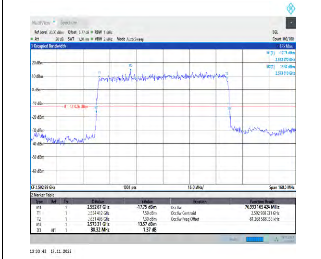
1-N41-PC2-30-80-M-2-DFT-PI2BPSK-Outer_Full-216 @0-Ant1-76.993-80.320-<math>\leq 80</math>-PASS
