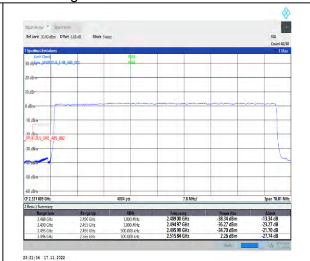
1-N41-PC2-30-70-L-3-DFT-PI2BPSK-Outer_Full-180@0-Ant1-1--PASS-see graph
