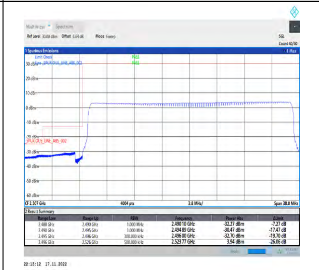
1-N41-PC2-30-30-L-6-CP-QPSK-Outer_Full-78@0-Ant1-1--PASS-see graph
