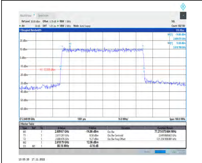
1-N41-PC2-30-80-H-1-DFT-QPSK-Outer_Full-216@ 0-Ant1-77.215-80.160-<80-PASS
