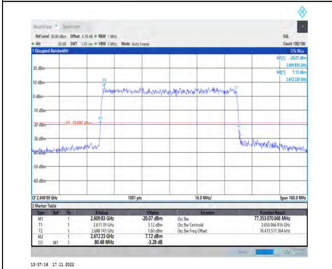
1-N41-PC2-30-80-H-9-CP-256QAM-Outer_Full-217 @0-Ant1-77.353-80.480-≤80-PASS
