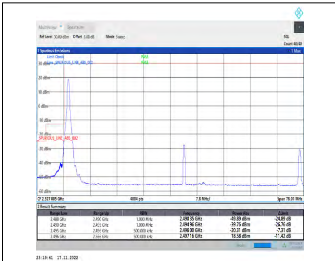
1-N41-PC2-30-70-L-1-DFT-PI2BPSK-Edge_1RB_Left-1@0-Ant1-1--PASS-see graph
