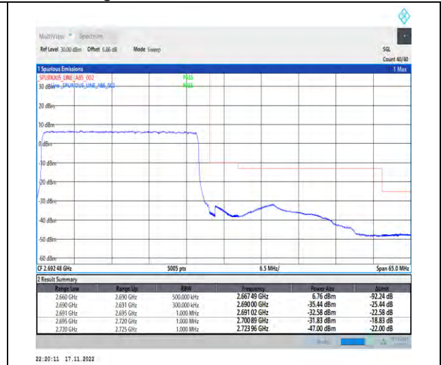
1-N41-PC2-30-30-H-3-DFT-PI2BPSK-Outer_Full-75@0-Ant1-1--PASS-see graph
