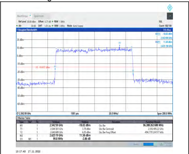
1-N41-PC2-30-100-M-3-DFT-16QAM-Outer_Full-270@0-Ant1-96.388-99.800-≤100-PASS
