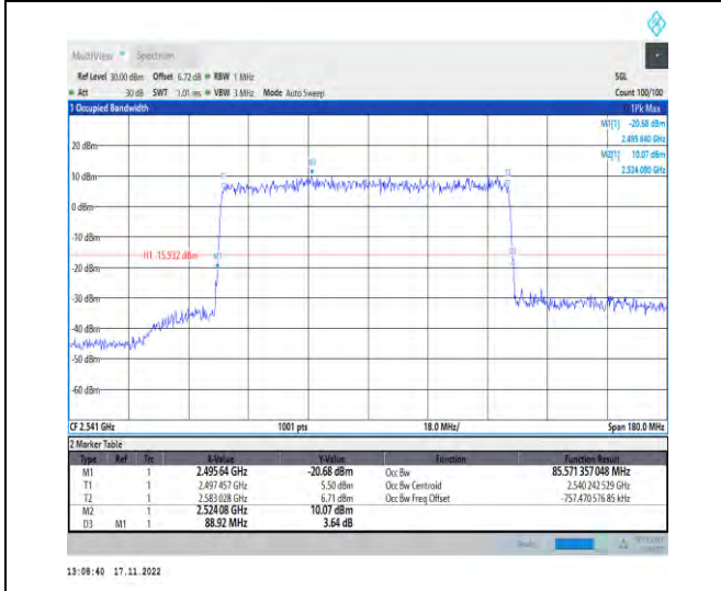
1-N41-PC2-30-90-L-4-DFT-64QAM-Outer_Full-240 @0-Ant1-85.571-88.920-≤90-PASS
