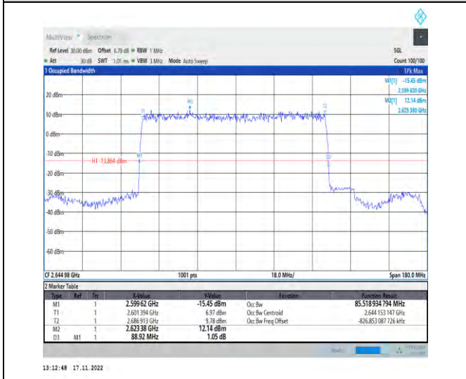
1-N41-PC2-30-90-H-2-DFT-PI2BPSK-Outer_Full-240 @0-Ant1-85.519-88.920-≤90-PASS
