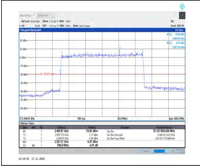
1-N41-PC2-30-100-L-9-CP-256QAM-Outer_Full-273 @0-Ant1-97.358-100.800-≤100-PASS
