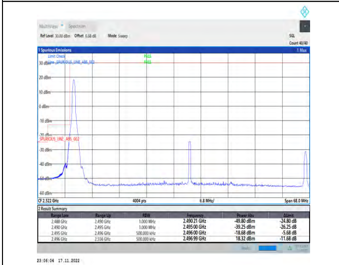
1-N41-PC2-30-60-L-4-CP-QPSK-Edge_1RB_Left-1@0-Ant1-1--PASS-see graph
