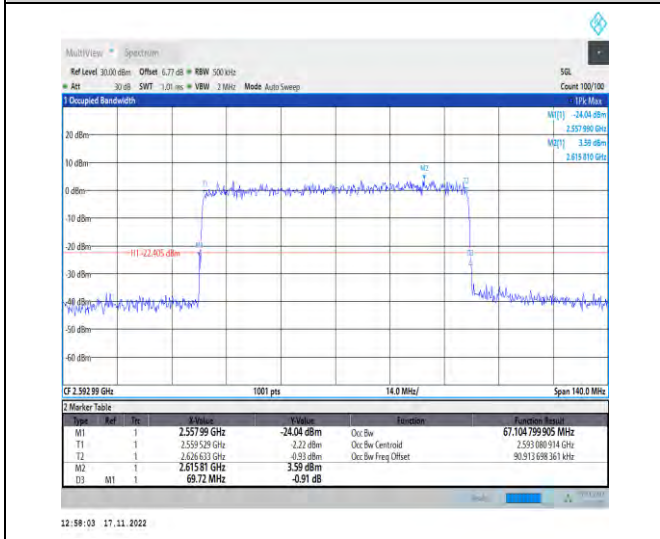
1-N41-PC2-30-70-M-9-CP-256QAM-Outer_Full-189 @0-Ant1-67.105-69.720-≤70-PASS
