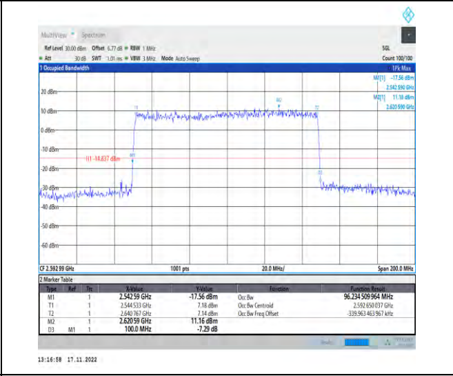
1-N41-PC2-30-100-M-1-DFT-QPSK-Outer_Full-270 @0-Ant1-96.235-100.000-≤100-PASS
