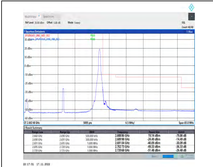
1-N41-PC2-30-30-H-2-DFT-PI2BPSK-Edge_1RB_Right-t-1@77-Ant1-1--PASS-see graph
