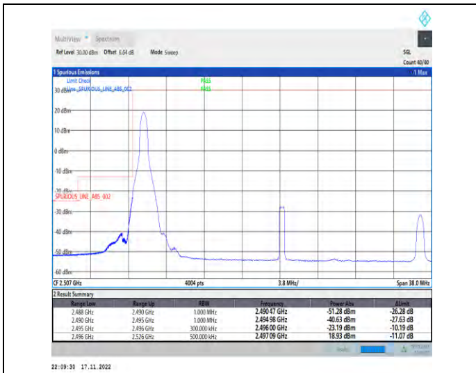
1-N41-PC2-30-30-L-1-DFT-PI2BPSK-Edge_1RB_Left-1@0-Ant1-1--PASS-see graph
