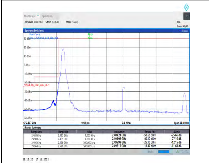
1-N41-PC2-30-30-L-4-CP-QPSK-Edge_1RB_Left-1@0-Ant1-1--PASS-see graph
