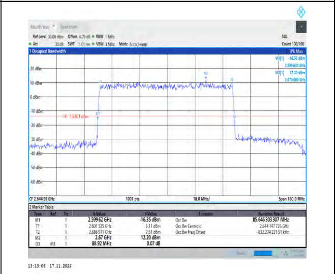
1-N41-PC2-30-90-H-3-DFT-16QAM-Outer_Full-240 @0-Ant1-85.646-88.920-≤90-PASS
