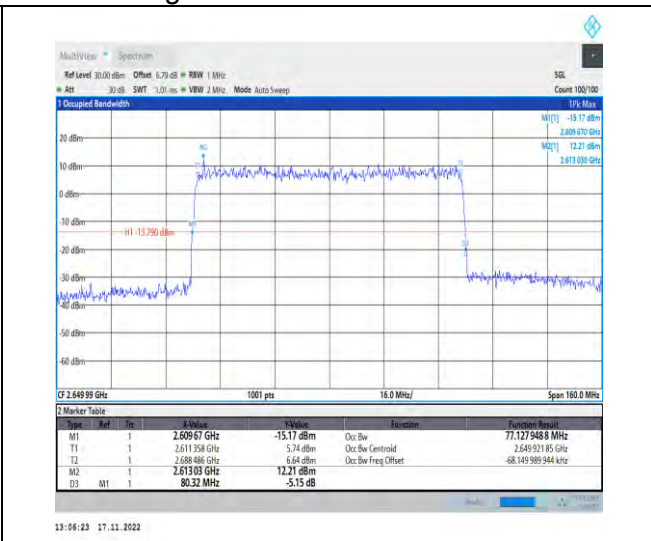
1-N41-PC2-30-80-H-4-DFT-64QAM-Outer_Full-216 @0-Ant1-77.128-80.320-≤80-PASS
