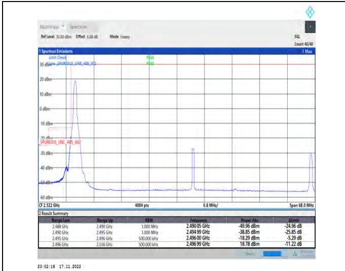
1-N41-PC2-30-60-L-1-DFT-PI2BPSK-Edge_1RB_Left-1@0-Ant1-1--PASS-see graph
