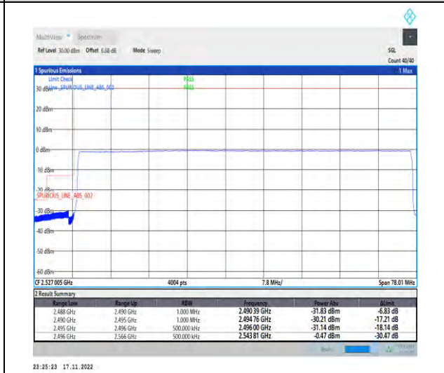
1-N41-PC2-30-70-L-6-CP-QPSK-Outer_Full-189@0-Ant1-1--PASS-see graph
