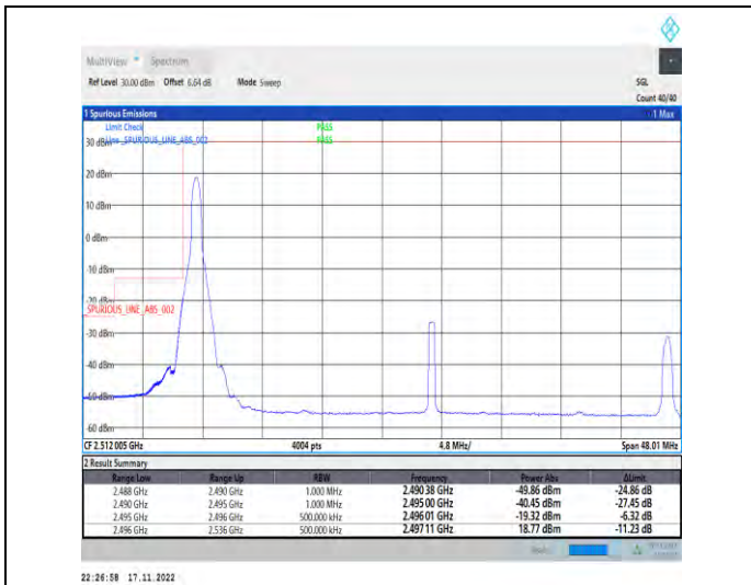
1-N41-PC2-30-40-L-1-DFT-PI2BPSK-Edge_1RB_Left-1@0-Ant1-1--PASS-see graph
