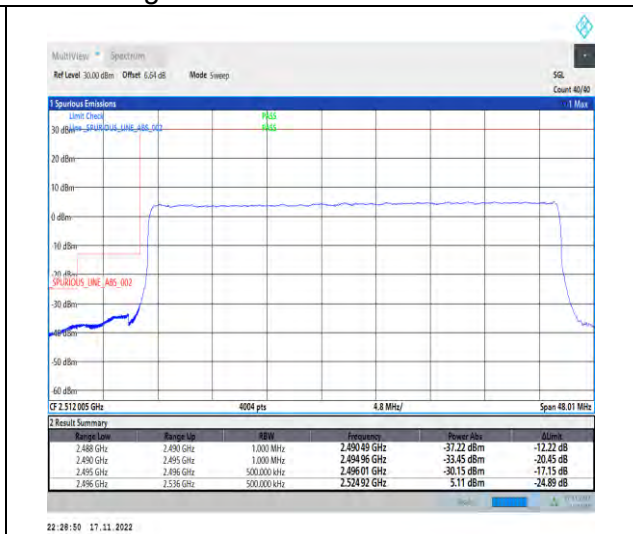
1-N41-PC2-30-40-L-3-DFT-PI2BPSK-Outer_Full-100@0-Ant1-1--PASS-see graph
