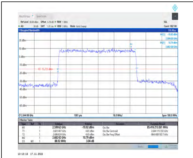
1-N41-PC2-30-90-H-4-DFT-64QAM-Outer_Full-240 @0-Ant1-85.416-88.920-≤90-PASS
