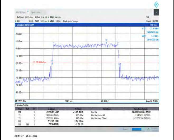
1-N41-PC2-30-30-L-5-DFT-256QAM-Outer_Full-75 @0-Ant1-26.829-27.960-≤30-PASS
