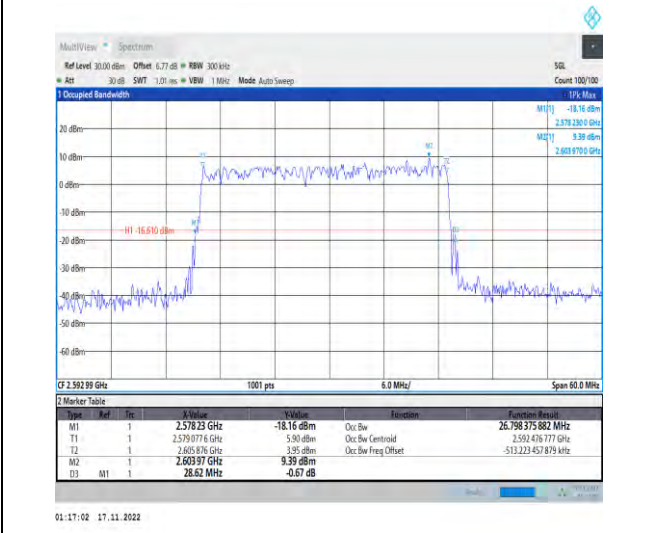
1-N41-PC2-30-30-M-5-DFT-256QAM-Outer_Full-75 @0-Ant1-26.798-28.620-≤30-PASS
