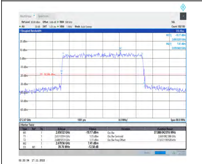
1-N41-PC2-30-40-H-9-CP-256QAM-Outer_Full-106 @0-Ant1-37.886-39.760-≤40-PASS
