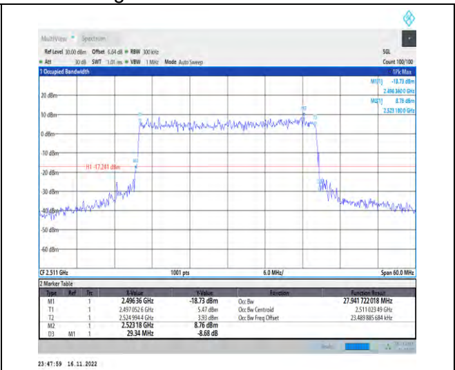
1-N41-PC2-30-30-L-7-CP-16QAM-Outer_Full-78@0-A Ant1-27.942-29.340-≤30-PASS
