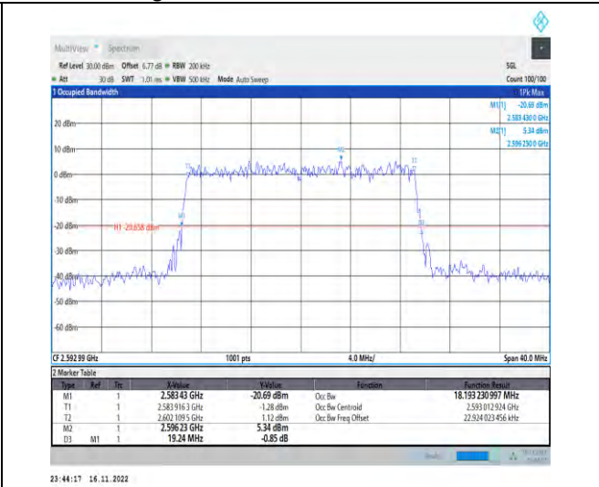
1-N41-PC2-30-20-M-9-CP-256QAM-Outer_Full-51@0 -Ant1-18.193-19.240-≤20-PASS
