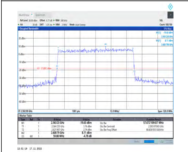
1-N41-PC2-30-60-M-8-CP-64QAM-Outer_Full-162@0 -Ant1-57.672-59.880-≤60-PASS
