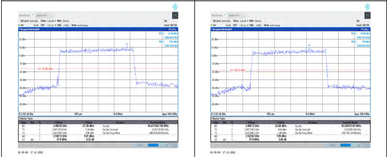
1-N41-PC2-30-50-L-4-DFT-64QAM-Outer_Full-128 @0-Ant1-45.614-47.800-≤50-PASS 1-N41-PC2-30-50-L-5-DFT-256QAM-Outer_Full-128 @0-Ant1-45.53-47.800-≤50-PASS
