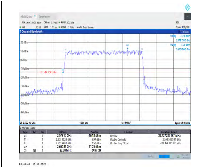
1-N41-PC2-30-30-M-1-DFT-QPSK-Outer_Full-75@0 -Ant1-26.727-28.380-≤30-PASS
