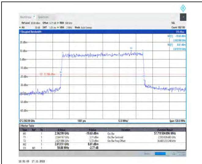
1-N41-PC2-30-60-M-6-CP-QPSK-Outer_Full-162@0 -Ant1-57.72-59.880-≤60-PASS
