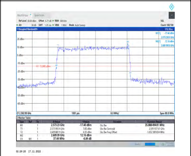
1-N41-PC2-30-40-M-3-DFT-16QAM-Outer_Full-100 @0-Ant1-35.888-37.440-<math>\leq 40</math>-PASS
