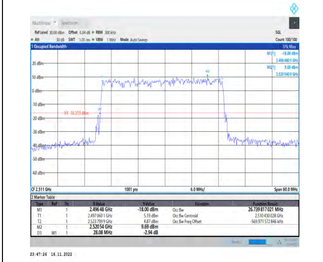
1-N41-PC2-30-30-L-4-DFT-64QAM-Outer_Full-75@ 0-Ant1-26.74-28.080-≤30-PASS
