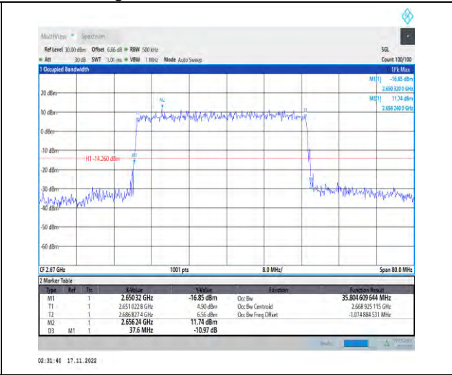
1-N41-PC2-30-40-H-4-DFT-64QAM-Outer_Full-100 @0-Ant1-35.805-37.600-≤40-PASS
