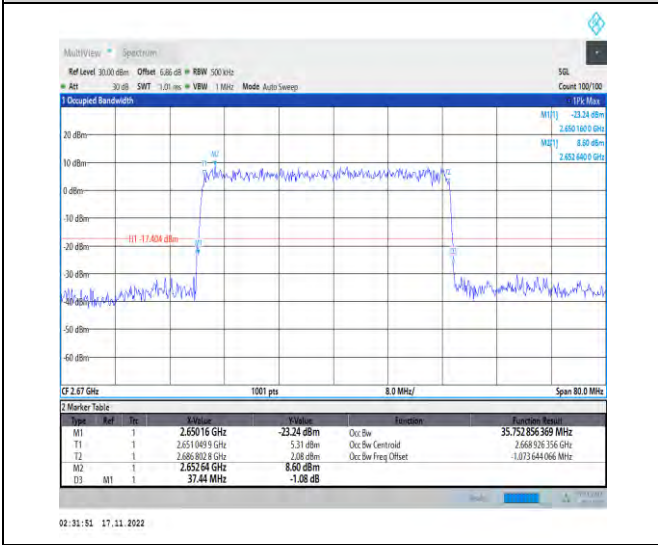
1-N41-PC2-30-40-H-5-DFT-256QAM-Outer_Full-100 @0-Ant1-35.753-37.440-≤40-PASS
