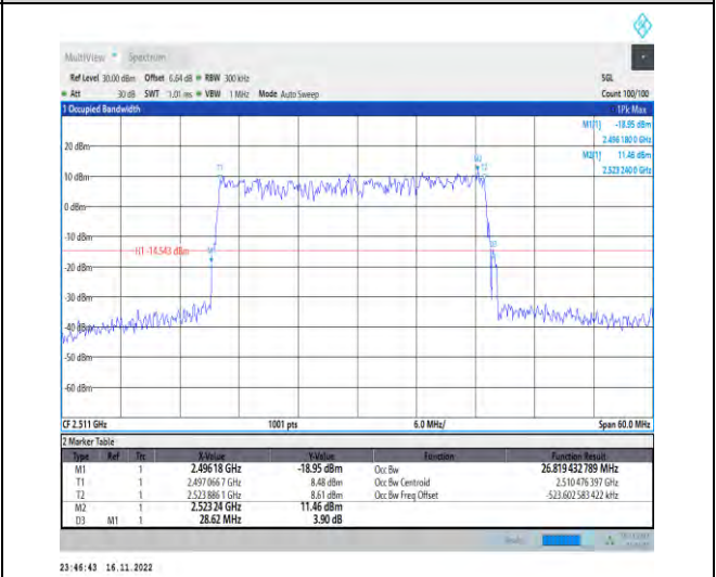
1-N41-PC2-30-30-L-1-DFT-QPSK-Outer_Full-75@0- Ant1-26.819-28.620-≤30-PASS
