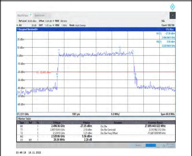
1-N41-PC2-30-30-L-9-CP-256QAM-Outer_Full-78@0-A Ant1-27.895-29.340-≤30-PASS
