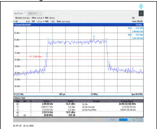
1-N41-PC2-30-30-L-3-DFT-16QAM-Outer_Full-75@ 0-Ant1-26.945-28.080-≤30-PASS
