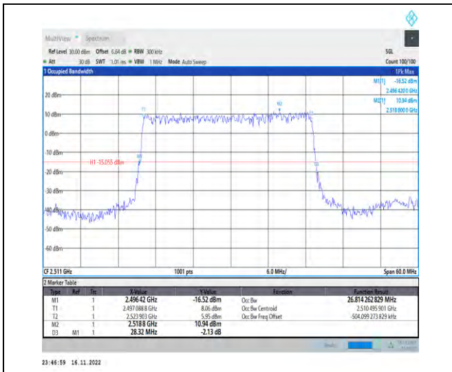
1-N41-PC2-30-30-L-2-DFT-PI2BPSK-Outer_Full-75 @0-Ant1-26.814-28.320-≤30-PASS
