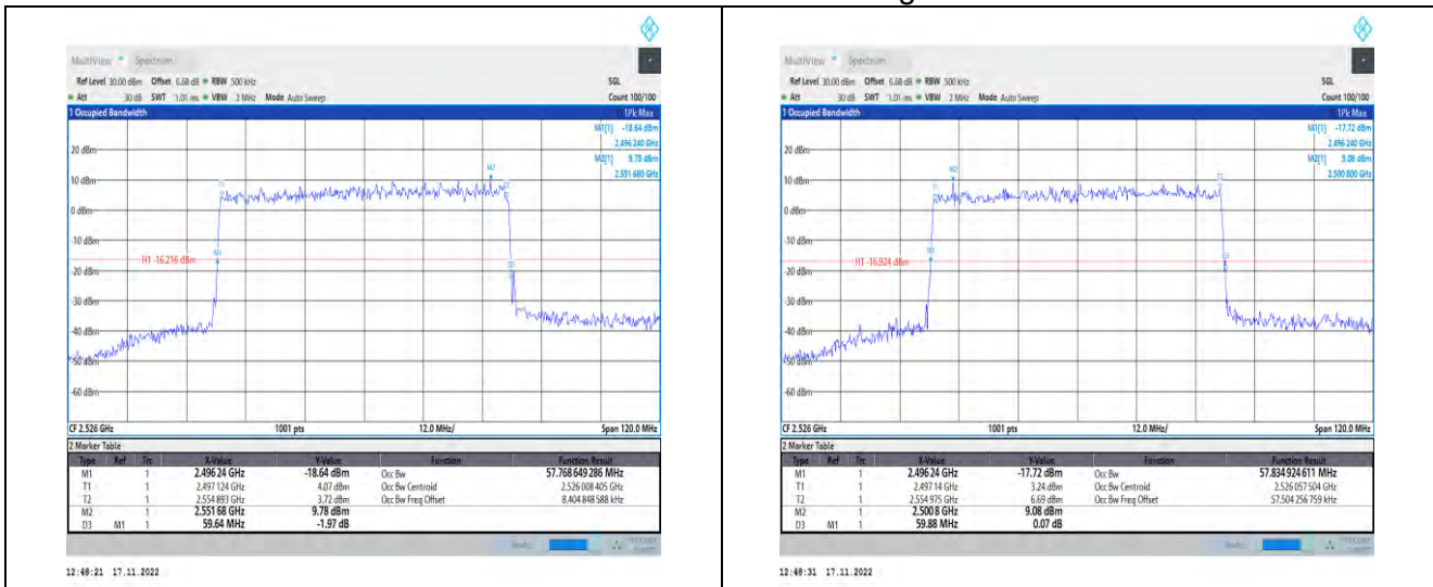
1-N41-PC2-30-60-L-3-DFT-16QAM-Outer_Full-162 @0-Ant1-57.769-59.640-≤60-PASS
