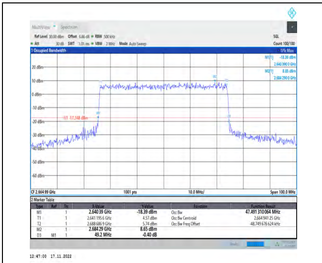
1-N41-PC2-30-50-H-8-CP-64QAM-Outer_Full-133@ 0-Ant1-47.491-49.200-≤50-PASS
