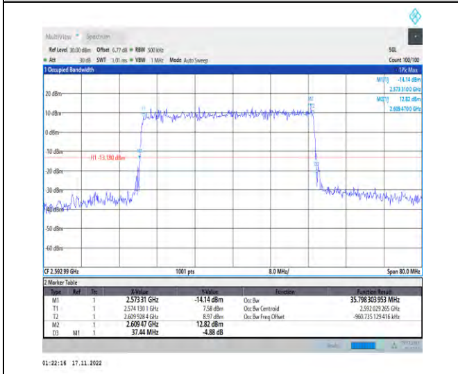
1-N41-PC2-30-40-M-1-DFT-QPSK-Outer_Full-100@ 0-Ant1-35.798-37.440-<math>\leq 40</math>-PASS
