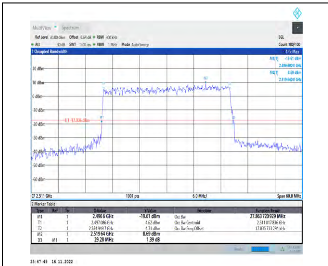
1-N41-PC2-30-30-L-6-CP-QPSK-Outer_Full-78@0-A Ant1-27.864-29.280-≤30-PASS
