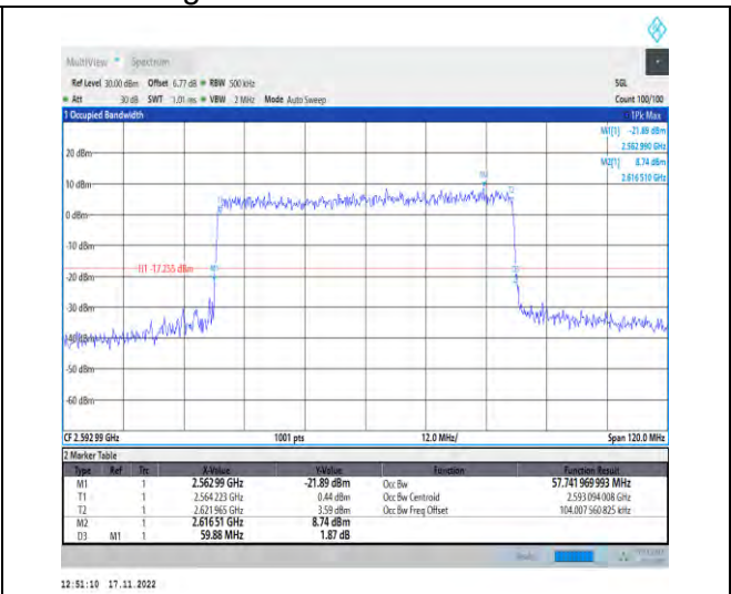
1-N41-PC2-30-60-M-7-CP-16QAM-Outer_Full-162@0 -Ant1-57.742-59.880-≤60-PASS
