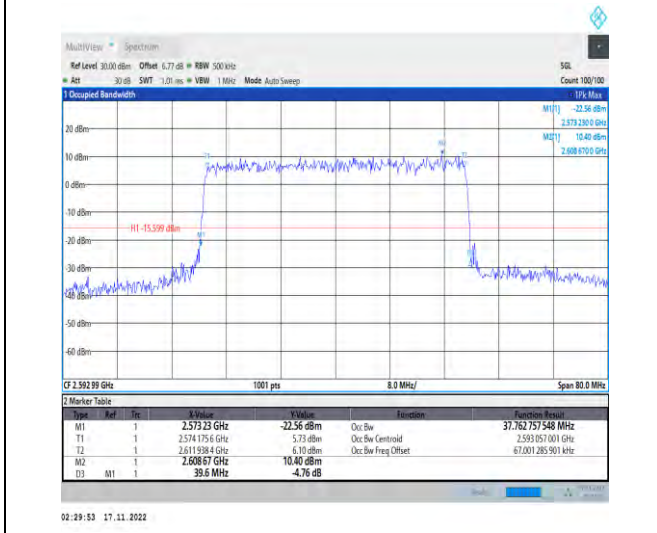
1-N41-PC2-30-40-M-6-CP-QPSK-Outer_Full-106@0 -Ant1-37.763-39.600-≤40-PASS
