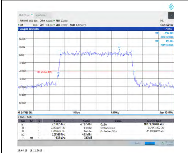
1-N41-PC2-30-20-H-9-CP-256QAM-Outer_Full-51@0 0-Ant1-18.174-19.320-≤20-PASS
