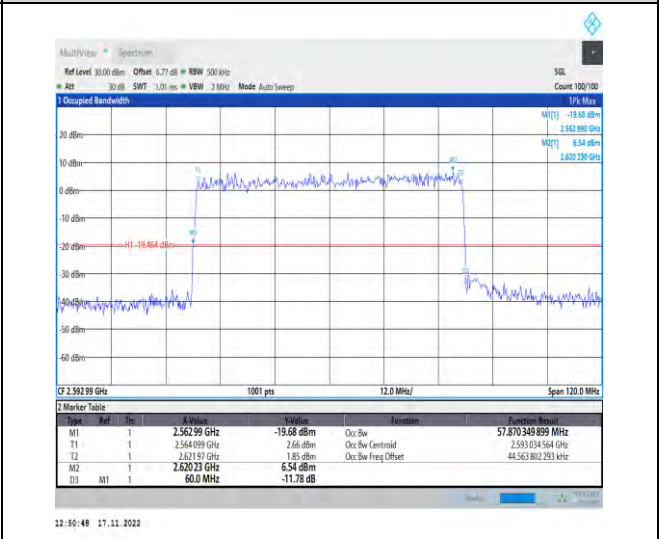
1-N41-PC2-30-60-M-5-DFT-256QAM-Outer_Full-162 @0-Ant1-57.87-60.000-≤60-PASS
