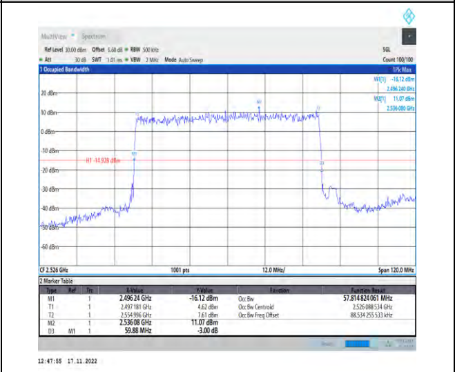
1-N41-PC2-30-60-L-2-DFT-PI2BPSK-Outer_Full-162 @0-Ant1-57.815-59.880-≤60-PASS
