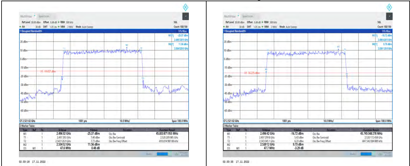
1-N41-PC2-30-50-L-2-DFT-PI2BPSK-Outer_Full-128 @0-Ant1-45.834-47.600-≤50-PASS 1-N41-PC2-30-50-L-3-DFT-16QAM-Outer_Full-128 @0-Ant1-45.745-47.700-≤50-PASS
