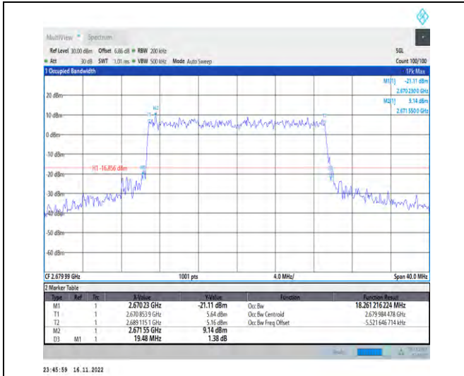
1-N41-PC2-30-20-H-7-CP-16QAM-Outer_Full-51@0 -Ant1-18.261-19.480-≤20-PASS
