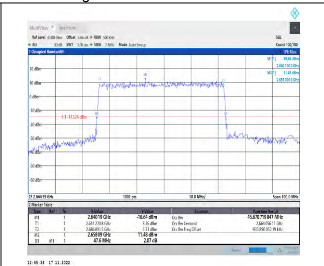
1-N41-PC2-30-50-H-1-DFT-QPSK-Outer_Full-128 @0-Ant1-45.671-47.600-≤50-PASS
