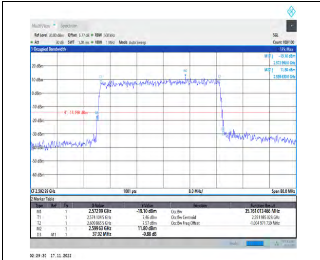
1-N41-PC2-30-40-M-4-DFT-64QAM-Outer_Full-100 @0-Ant1-35.761-37.920-≤40-PASS
