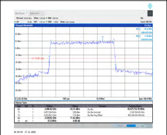
1-N41-PC2-30-50-L-1-DFT-QPSK-Outer_Full-128@ 0-Ant1-45.676-47.800-≤50-PASS
