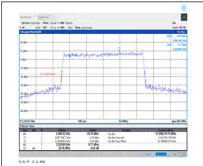
1-N41-PC2-30-40-L-8-CP-64QAM-Outer_Full-106@ 0-Ant1-37.698-39.760-<math>\leq 40</math>-PASS
