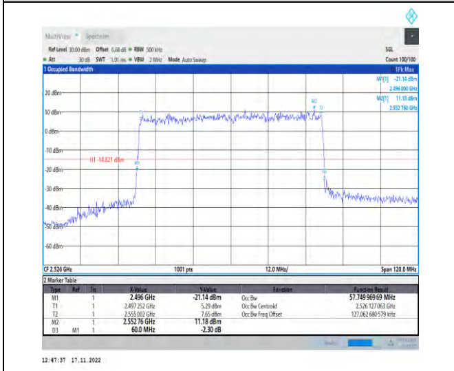
1-N41-PC2-30-60-L-1-DFT-QPSK-Outer_Full-162@0 -Ant1-57.75-60.000-≤60-PASS
