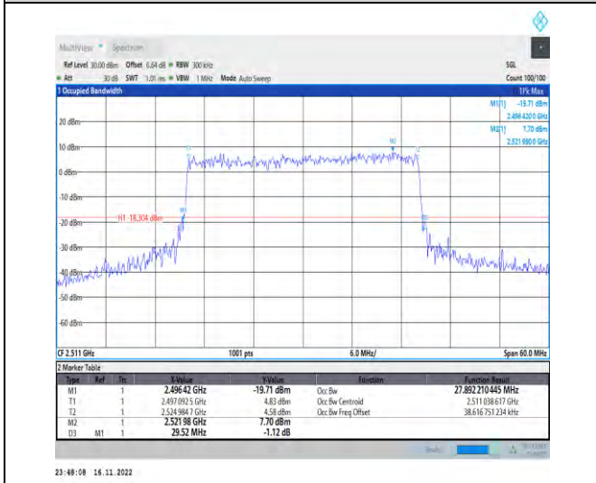
1-N41-PC2-30-30-L-8-CP-64QAM-Outer_Full-78@0-A Ant1-27.892-29.520-≤30-PASS
