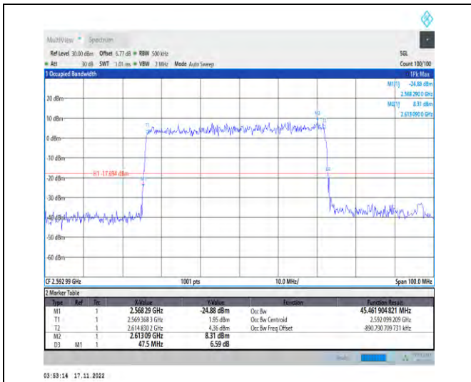
1-N41-PC2-30-50-M-5-DFT-256QAM-Outer_Full-128 @0-Ant1-45.462-47.500-≤50-PASS
