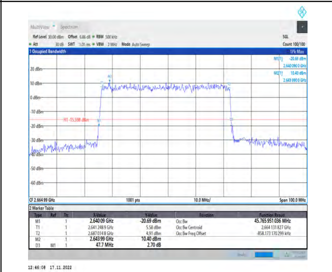
1-N41-PC2-30-50-H-3-DFT-16QAM-Outer_Full-128 @0-Ant1-45.766-47.700-≤50-PASS
