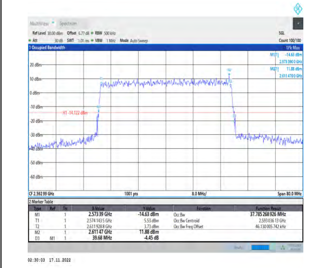
1-N41-PC2-30-40-M-7-CP-16QAM-Outer_Full-106@0 -Ant1-37.785-39.680-≤40-PASS
