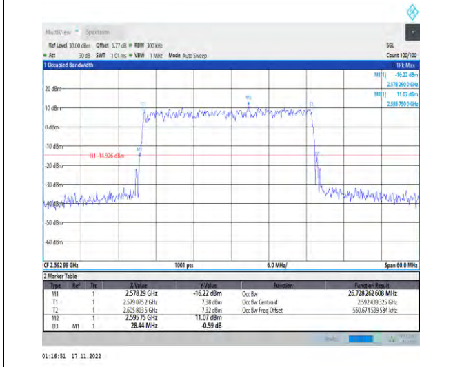
1-N41-PC2-30-30-M-4-DFT-64QAM-Outer_Full-75@ 0-Ant1-26.728-28.440-≤30-PASS
