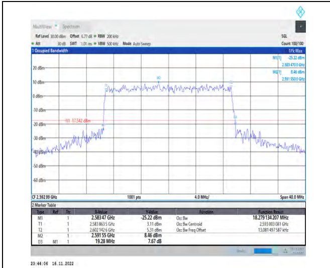
1-N41-PC2-30-20-M-8-CP-64QAM-Outer_Full-51@0 -Ant1-18.279-19.280-≤20-PASS
