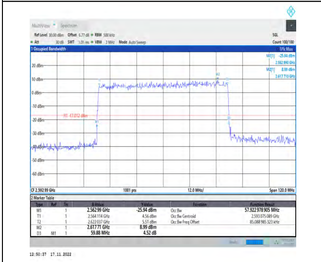
1-N41-PC2-30-60-M-4-DFT-64QAM-Outer_Full-162 @0-Ant1-57.923-59.880-≤60-PASS
