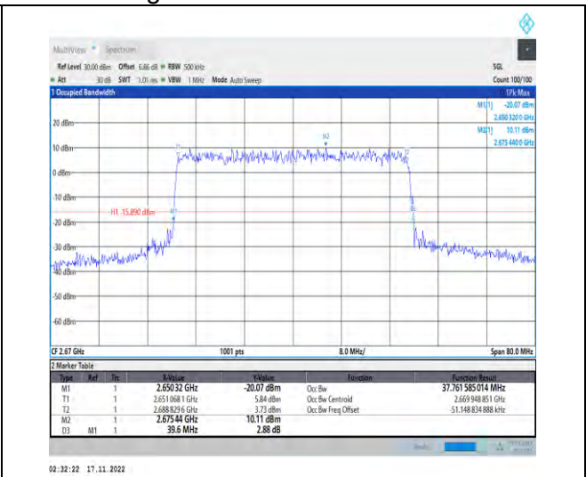
1-N41-PC2-30-40-H-8-CP-64QAM-Outer_Full-106@ 0-Ant1-37.762-39.600-≤40-PASS
