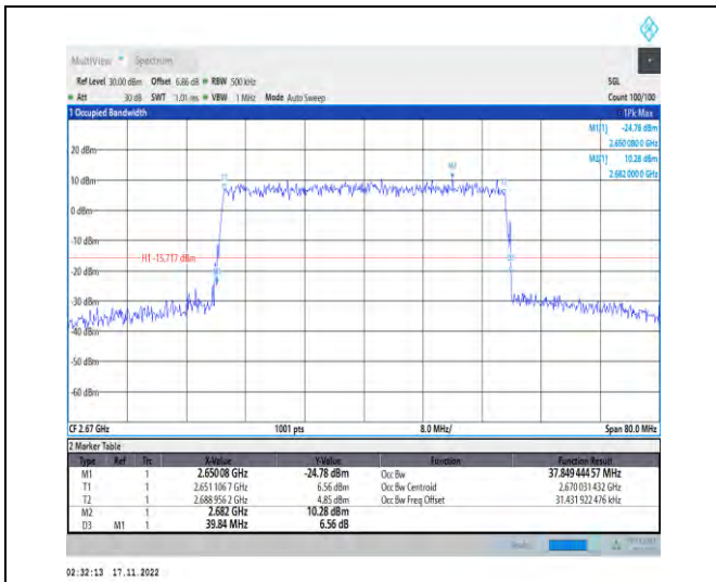
1-N41-PC2-30-40-H-7-CP-16QAM-Outer_Full-106@ 0-Ant1-37.849-39.840-≤40-PASS
