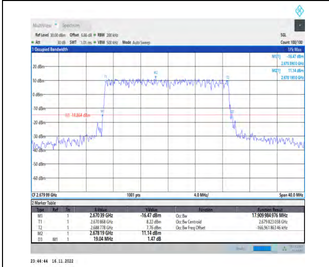
1-N41-PC2-30-20-H-1-DFT-QPSK-Outer_Full-50@0- Ant1-17.91-19.040-≤20-PASS
