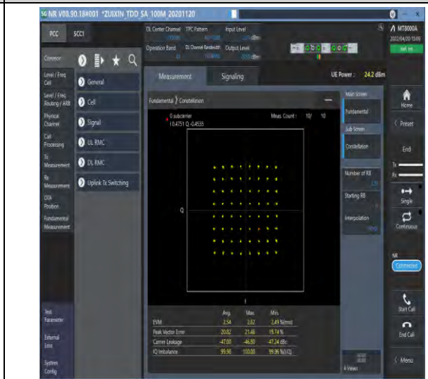
1-N41--30-100-M-4-DFT-64QAM-Outer_Full-270@0-Ant1-see graph-PASS
