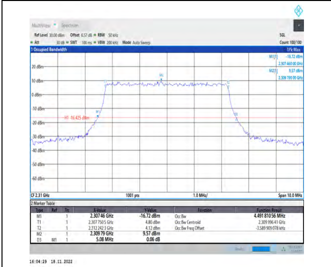
1-N30-PC3-15-5-M-6-CP-QPSK-Outer_Full-25@0-Ant1-4.492-5.080-≤5-PASS
