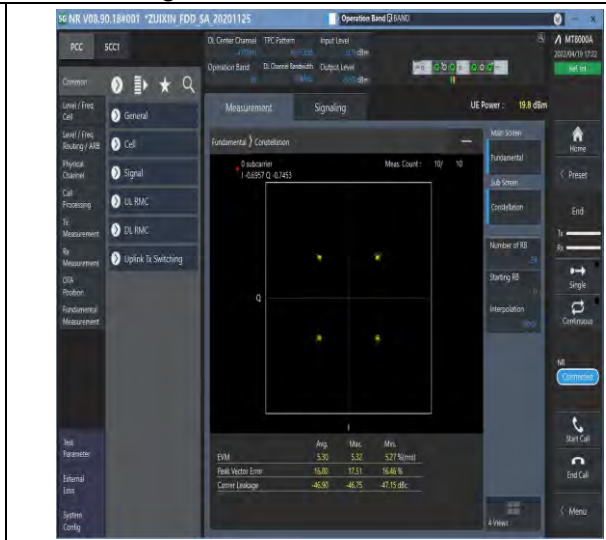
1-N30--30-10-M-6-CP-QPSK-Outer_Full-24@0-Ant 1-see graph-PASS
