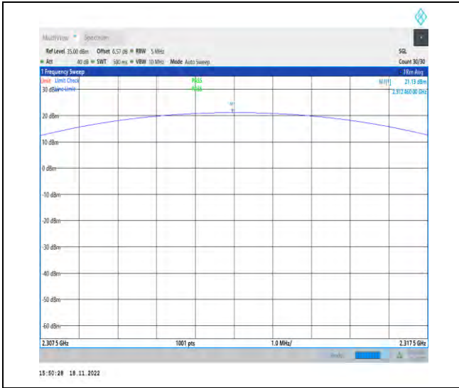
1-N30-PC3-15-5-H-3-DFT-PI2BPSK-Outter_Full-25 @0-2307.5-2317.5-Ant1-2312.46-21.13-99-PASS
