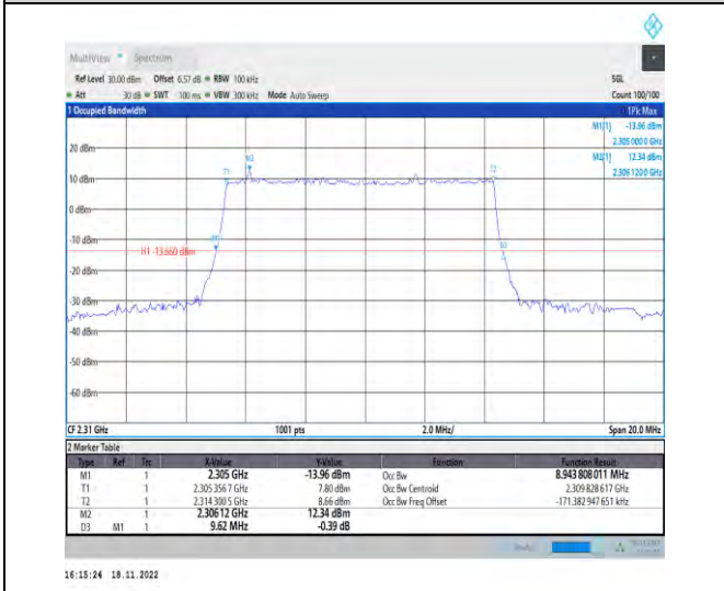
1-N30-PC3-15-10-M-4-DFT-64QAM-Outer_Full-50 @0-Ant1-8.944-9.620-≤10-PASS
