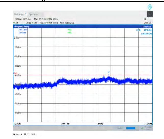
1-N30-PC3-15-10-H-1-DFT-PI2BPSK-Inner_1RB_Lef t-1@1-12000-27000-Ant1-22312.50--40.14--40-PASS
