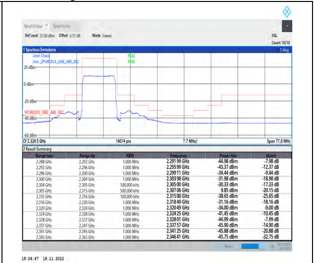
1-N30-PC3-15-10-L-3-DFT-PI2BPSK-Outer_Full-50@0-Ant1-1--PASS-see graph
