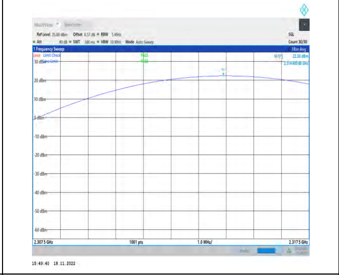
1-N30-PC3-15-5-H-2-DFT-PI2BPSK-Inner_1RB_Righ t-1@23-2307.5-2317.5-Ant1-2314.40-22.33-99-PASS
