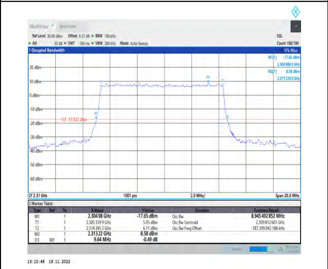
1-N30-PC3-15-10-M-5-DFT-256QAM-Outer_Full-50 @0-Ant1-8.945-9.640-≤10-PASS
