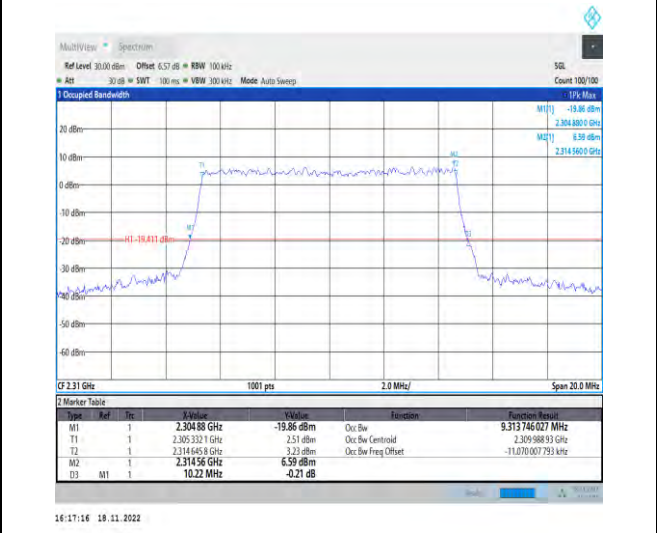
1-N30-PC3-15-10-M-9-CP-256QAM-Outer_Full-52@0-Ant1-9.314-10.220-≤10-PASS
