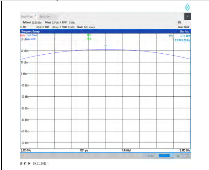
1-N30-PC3-15-5-M-3-DFT-PI2BPSK-Outer_Full-25@ 0-2305-2315-Ant1-2310.01-21.14-99-PASS
