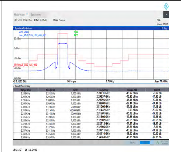
1-N30-PC3-15-5-H-6-CP-QPSK-Outer_Full-25@0-Ant1-1--PASS-see graph
