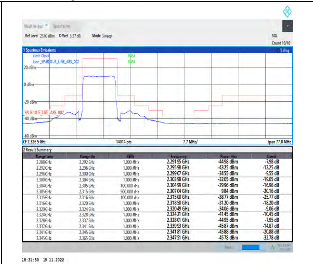
1-N30-PC3-15-10-H-3-DFT-PI2BPSK-Outer_Full-50@0-Ant1-1--PASS-see graph
