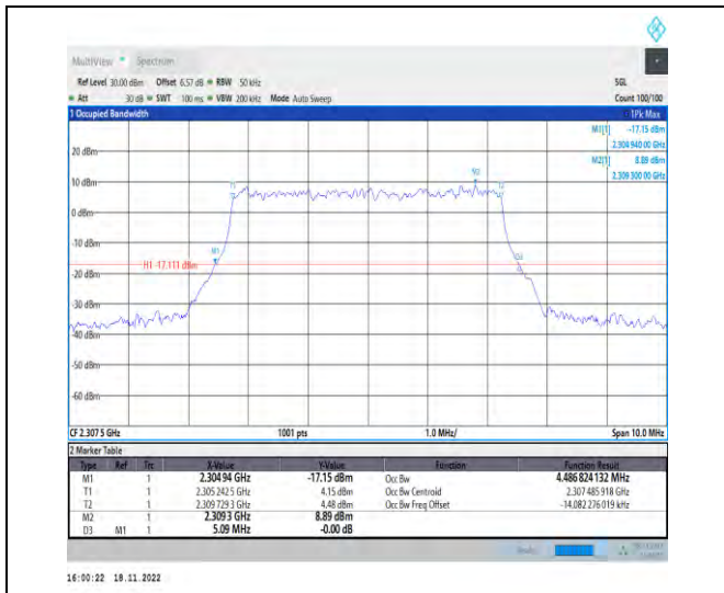
1-N30-PC3-15-5-L-5-DFT-256QAM-Outer_Full-25@0-Ant1-4.487-5.090-≤5-PASS
