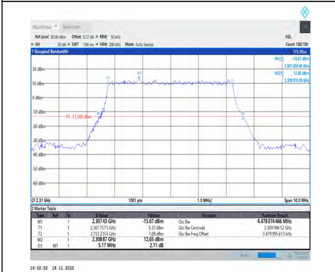
1-N30-PC3-15-5-M-2-DFT-PI2BPSK-Outer_Full-25@0-Ant1-4.478-5.170-≤5-PASS
