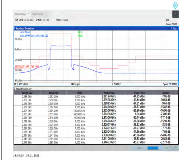
1-N30-PC3-15-10-H-6-CP-QPSK-Outer_Full-52@0-Ant1-1--PASS-see graph
