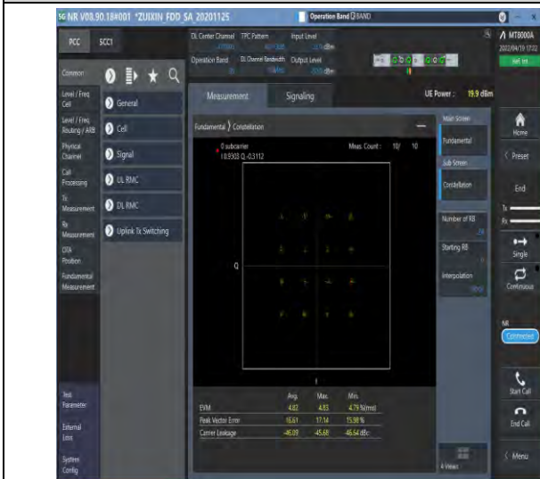
1-N30--30-10-M-7-CP-16QAM-Outer_Full-24@0-Ant1 -see graph-PASS
