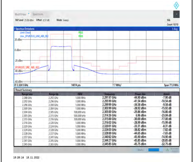
1-N30-PC3-15-10-L-6-CP-QPSK-Outer_Full-52@0-Ant1-1--PASS-see graph
