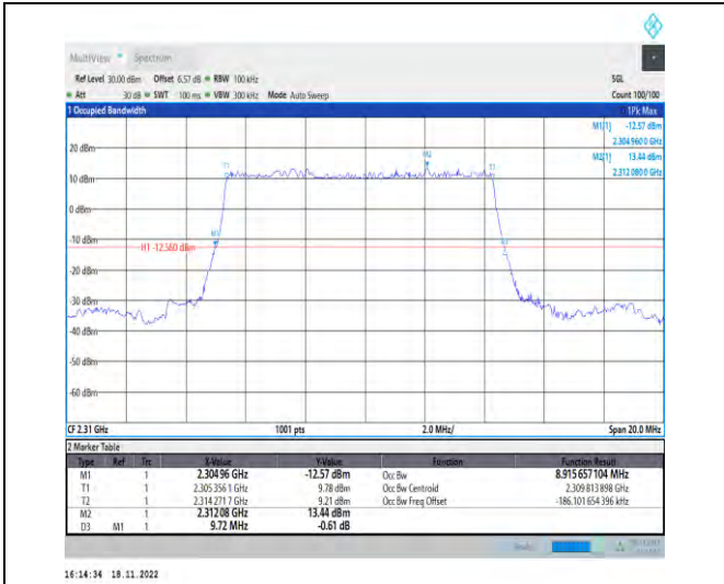
1-N30-PC3-15-10-M-2-DFT-PI2BPSK-Outer_Full-50 @0-Ant1-8.916-9.720-≤10-PASS
