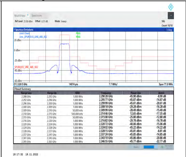
1-N30-PC3-15-5-H-3-DFT-PI2BPSK-Outer_Full-25@0-Ant1-1--PASS-see graph
