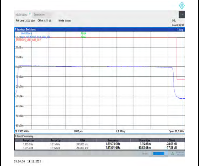
1-N25-PC3-15-20-H-6-CP-QPSK-Outer_Full-106@0-Ant1-1-seegraph-PASS-see graph
