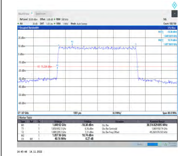
1-N25-PC3-15-40-L-5-DFT-256QAM-Outer_Full-216 @0-Ant1-38.517-40.160-≤40-PASS
