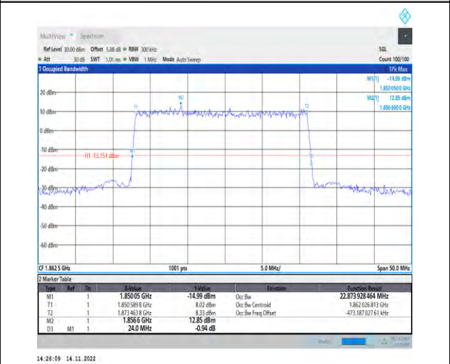
1-N25-PC3-15-25-L-4-DFT-64QAM-Outer_Full-128 @0-Ant1-22.874-24.000-≤25-PASS
