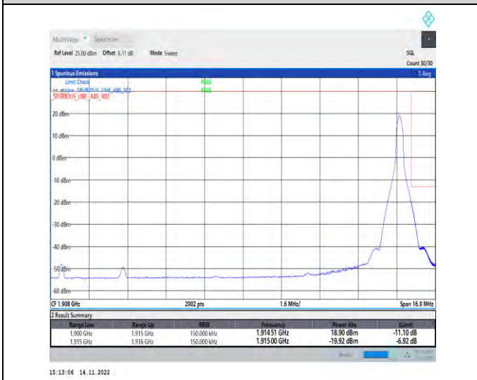
1-N25-PC3-15-15-H-5-CP-QPSK-Edge_1RB_Right-1@78-Ant1-1-seegraph-PASS-see graph
