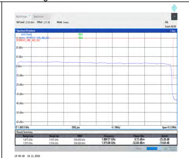
1-N25-PC3-15-40-H-3-DFT-PI2BPSK-Outer_Full-216@0-Ant1-1-seegraph-PASS-see graph
