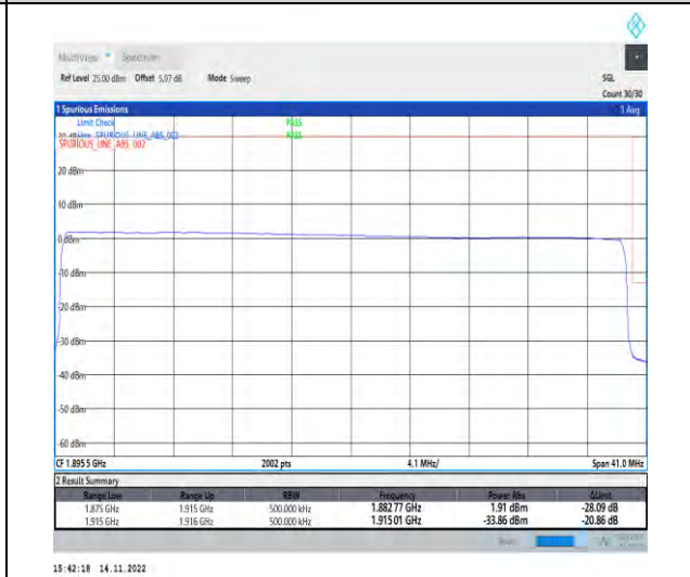
1-N25-PC3-15-40-H-6-CP-QPSK-Outer_Full-216@0-Ant1-1-seegraph-PASS-see graph
