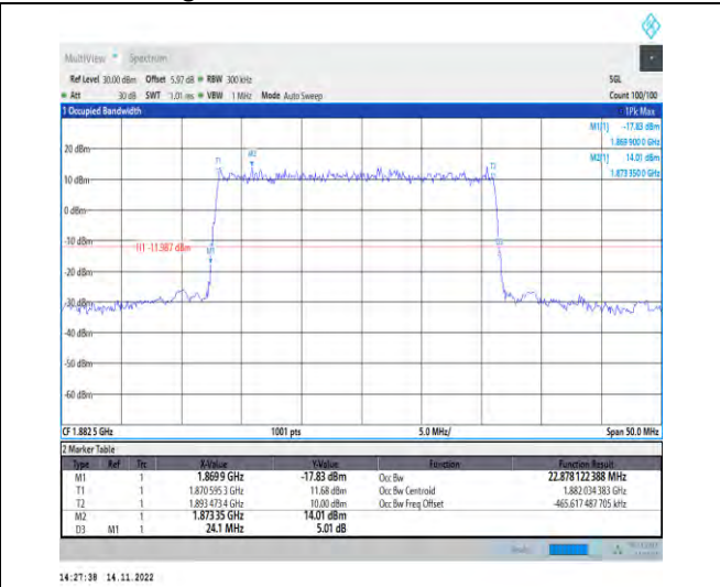
1-N25-PC3-15-25-M-1-DFT-QPSK-Outer_Full-128 @0-Ant1-22.878-24.100-≤25-PASS
