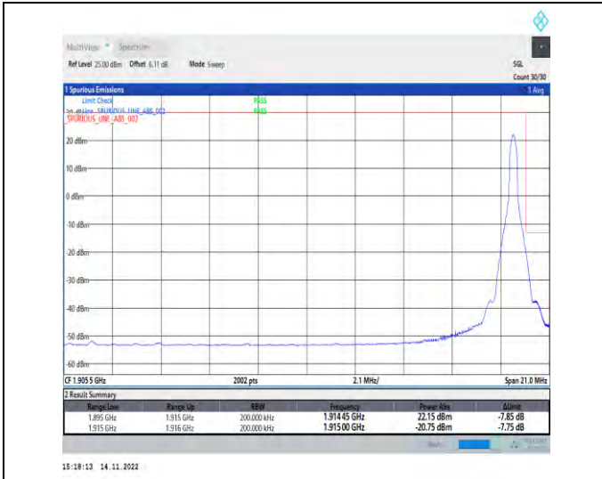
1-N25-PC3-15-20-H-2-DFT-PI2BPSK-Edge_1RB_Right-1@105-Ant1-1-seegraph-PASS-see graph
