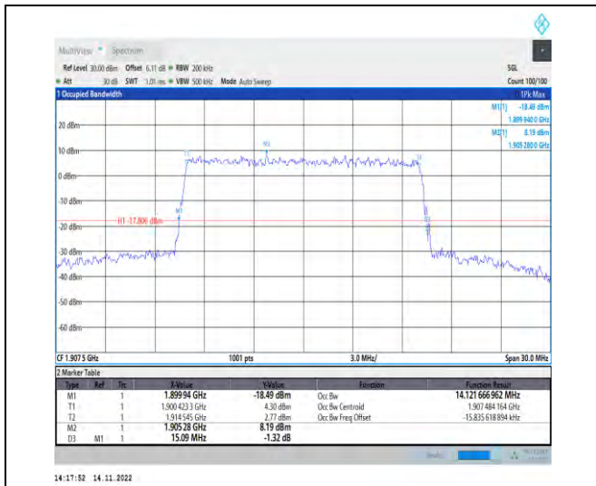
1-N25-PC3-15-15-H-9-CP-256QAM-Outer_Full-79@ 0-Ant1-14.122-15.090-≤15-PASS
