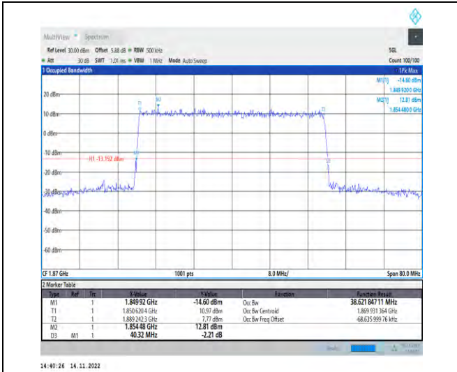
1-N25-PC3-15-40-L-3-DFT-16QAM-Outer_Full-216 @0-Ant1-38.622-40.320-≤40-PASS
