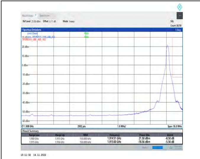
1-N25-PC3-15-15-H-2-DFT-PI2BPSK-Edge_1RB_Right-t1@78-Ant1-1-seegraph-PASS-see graph
