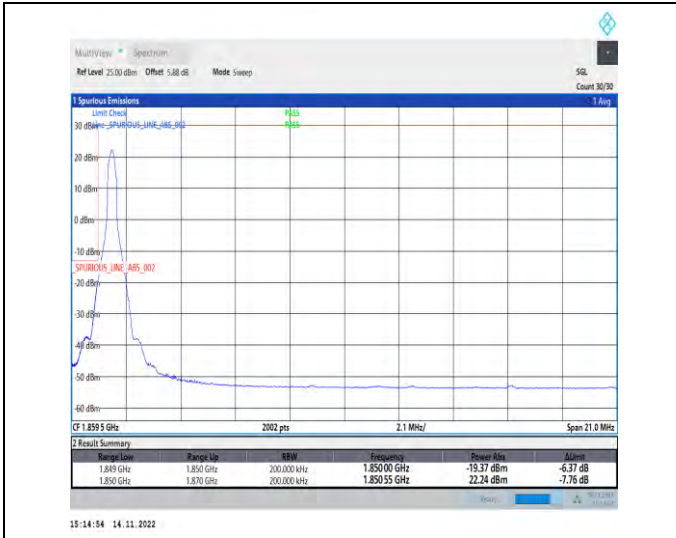
1-N25-PC3-15-20-L-1-DFT-PI2BPSK-Edge_1RB_Left-1@0-Ant1-1-seegraph-PASS-see graph
