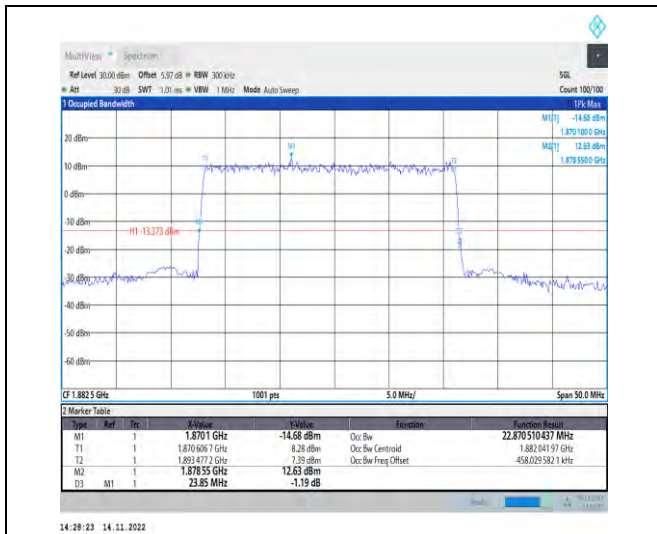
1-N25-PC3-15-25-M-4-DFT-64QAM-Outer_Full-128 @0-Ant1-22.871-23.850-≤25-PASS
