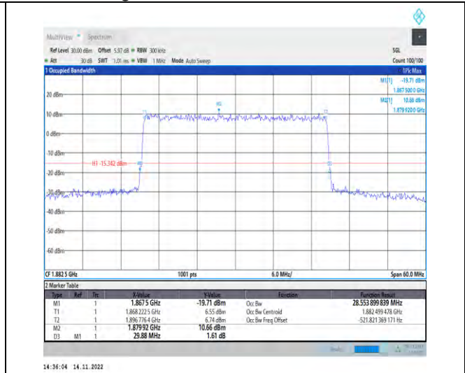
1-N25-PC3-15-30-M-6-CP-QPSK-Outer_Full-160@0 -Ant1-28.554-29.880-≤30-PASS
