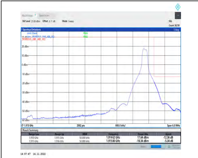
1-N25-PC3-15-5-H-2-DFT-PI2BPSK-Edge_1RB_Right-1@24-Ant1-1-seegraph-PASS-see graph
