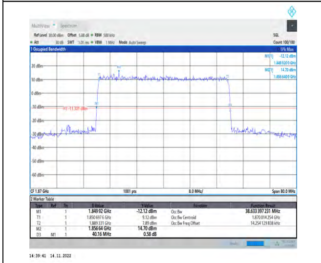
1-N25-PC3-15-40-L-1-DFT-QPSK-Outer_Full-216@ 0-Ant1-38.633-40.160-≤40-PASS
