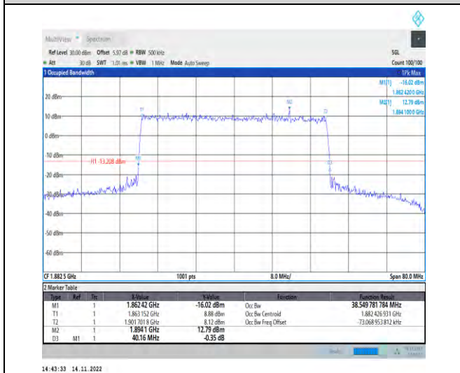
1-N25-PC3-15-40-M-8-CP-64QAM-Outer_Full-216@0 -Ant1-38.55-40.160-≤40-PASS
