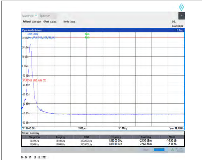
1-N25-PC3-15-30-L-1-DFT-PI2BPSK-Edge_1RB_Left-1@0-Ant1-1-seegraph-PASS-see graph
