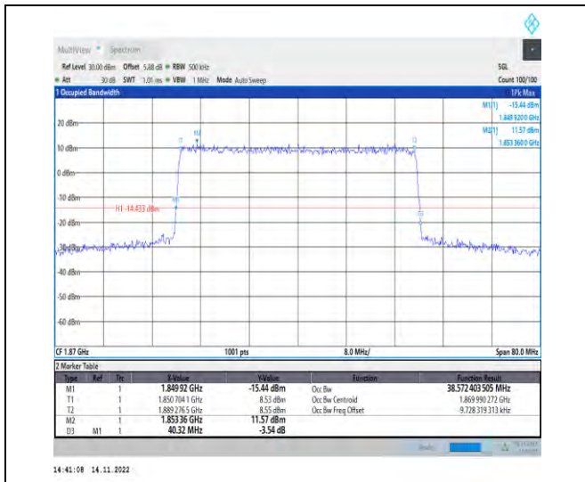
1-N25-PC3-15-40-L-7-CP-16QAM-Outer_Full-216@ 0-Ant1-38.572-40.320-≤40-PASS
