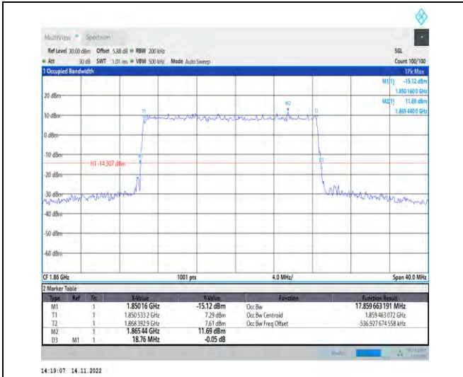
1-N25-PC3-15-20-L-4-DFT-64QAM-Outer_Full-100 @0-Ant1-17.86-18.760-<math>\leq 20</math>-PASS
