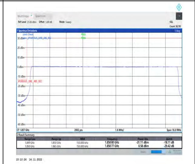
1-N25-PC3-15-15-L-6-CP-QPSK-Outer_Full-79@0-Ant1-1-seegraph-PASS-see graph
