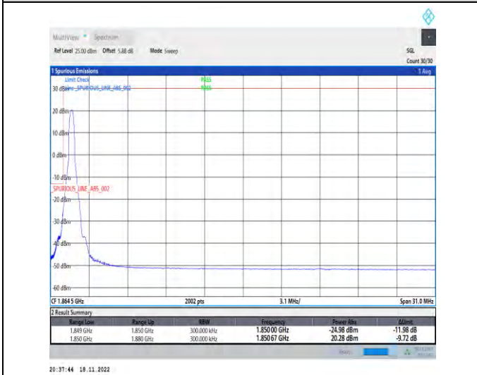
1-N25-PC3-15-30-L-4-CP-QPSK-Edge_1RB_Left-1@0-Ant1-1-seegraph-PASS-see graph
