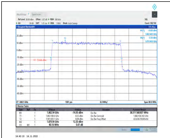
1-N25-PC3-15-40-M-6-CP-QPSK-Outer_Full-216@0 -Ant1-38.512-40.160-≤40-PASS
