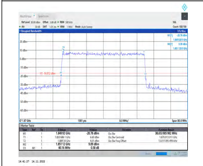
1-N25-PC3-15-40-L-9-CP-256QAM-Outer_Full-216 @0-Ant1-38.654-40.160-≤40-PASS
