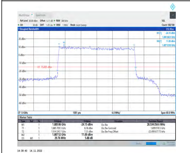
1-N25-PC3-15-30-H-6-CP-QPSK-Outer_Full-160@0 -Ant1-28.534-29.760-≤30-PASS
