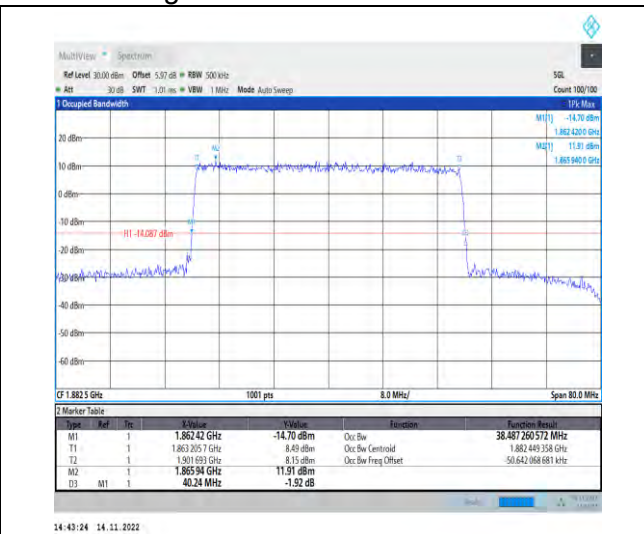
1-N25-PC3-15-40-M-7-CP-16QAM-Outer_Full-216@0 -Ant1-38.487-40.240-≤40-PASS
