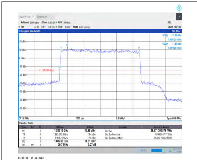
1-N25-PC3-15-30-H-4-DFT-64QAM-Outer_Full-160 @0-Ant1-28.572-29.700-≤30-PASS
