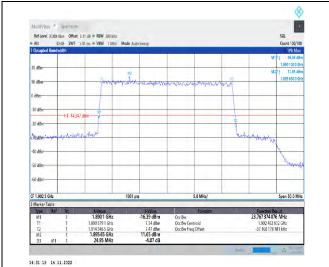
1-N25-PC3-15-25-H-7-CP-16QAM-Outer_Full-133@ 0-Ant1-23.767-24.950-≤25-PASS
