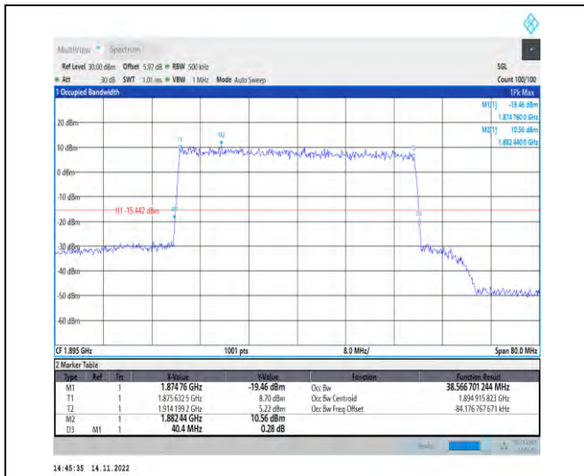
1-N25-PC3-15-40-H-5-DFT-256QAM-Outer_Full-216 @0-Ant1-38.567-40.400-≤40-PASS
