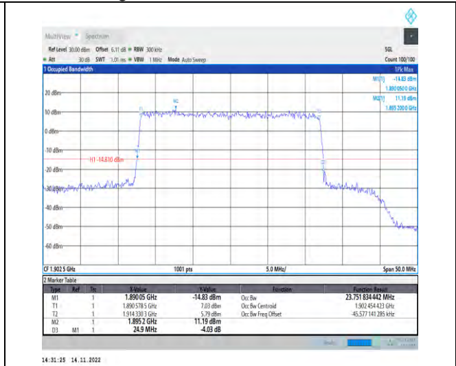
1-N25-PC3-15-25-H-8-CP-64QAM-Outer_Full-133@ 0-Ant1-23.752-24.900-≤25-PASS
