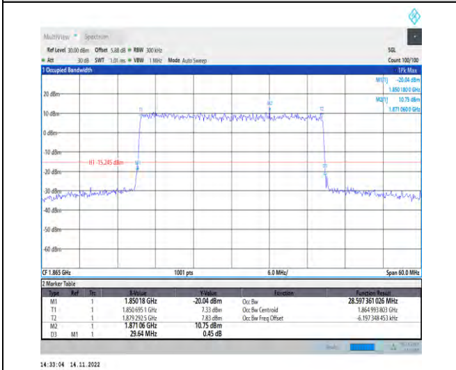
1-N25-PC3-15-30-L-4-DFT-64QAM-Outer_Full-160 @0-Ant1-28.597-29.640-≤30-PASS
