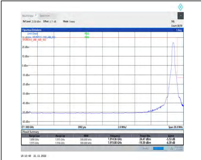
1-N25-PC3-15-25-H-2-DFT-PI2BPSK-Edge_1RB_Right-t-1@132-Ant1-1-seegraph-PASS-see graph
