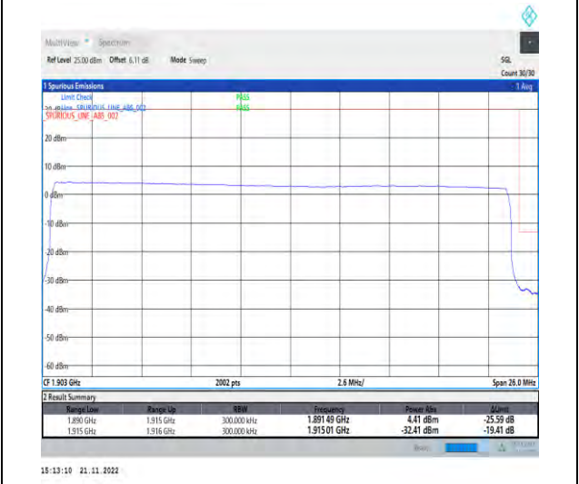
1-N25-PC3-15-25-H-6-CP-QPSK-Outer_Full-133@0-Ant1-1-seegraph-PASS-see graph
