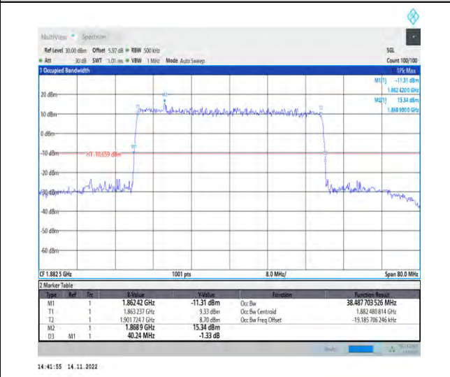
1-N25-PC3-15-40-M-1-DFT-QPSK-Outer_Full-216@ 0-Ant1-38.488-40.240-≤40-PASS
