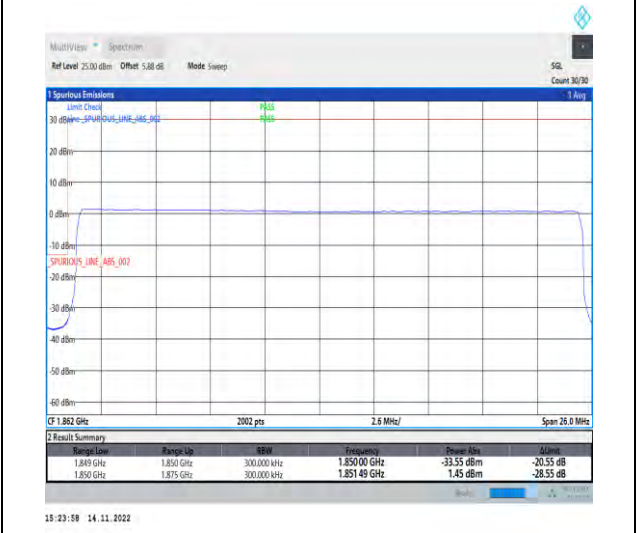
1-N25-PC3-15-25-L-6-CP-QPSK-Outer_Full-133@0-Ant1-1-seegraph-PASS-see graph
