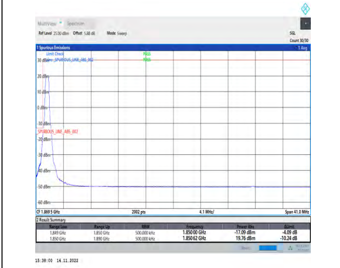
1-N25-PC3-15-40-L-4-CP-QPSK-Edge_1RB_Left-1@0-Ant1-1-seegraph-PASS-see graph
