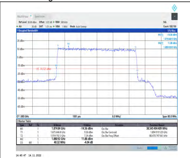
1-N25-PC3-15-40-H-6-CP-QPSK-Outer_Full-216@0 -Ant1-38.545-40.320-≤40-PASS
