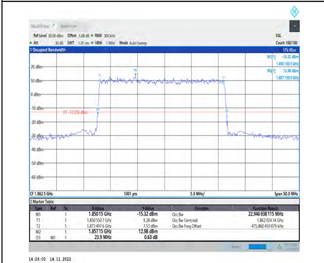
1-N25-PC3-15-25-L-3-DFT-16QAM-Outer_Full-128 @0-Ant1-22.947-23.900-≤25-PASS
