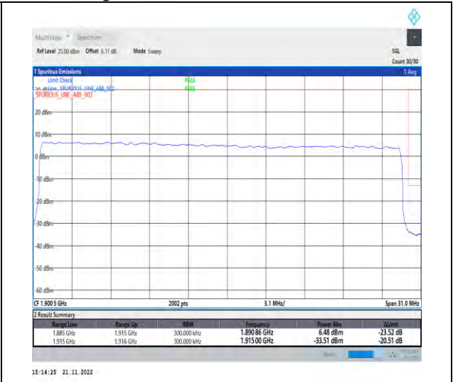
1-N25-PC3-15-30-H-3-DFT-PI2BPSK-Outer_Full-160@0-Ant1-1-seegraph-PASS-see graph
