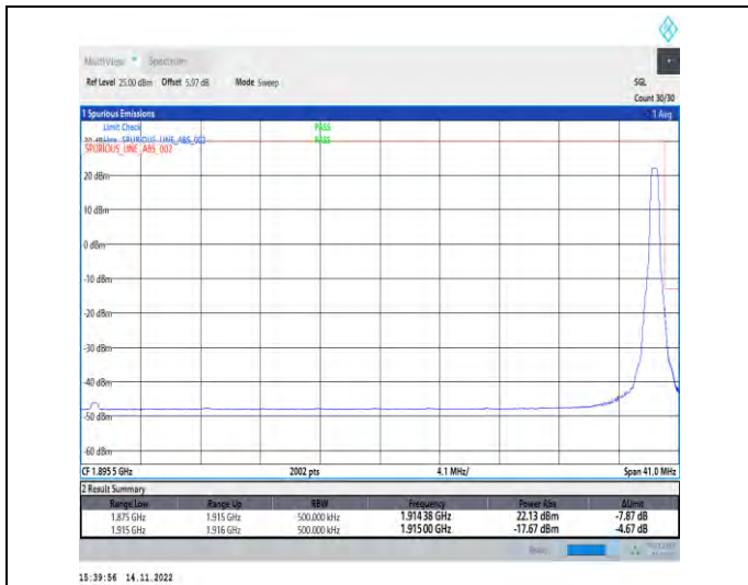
1-N25-PC3-15-40-H-2-DFT-PI2BPSK-Edge_1RB_Right-t-1@215-Ant1-1-seegraph-PASS-see graph
