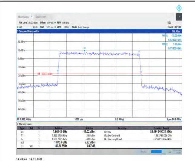
1-N25-PC3-15-40-M-9-CP-256QAM-Outer_Full-216@0 -Ant1-38.485-40.240-≤40-PASS
