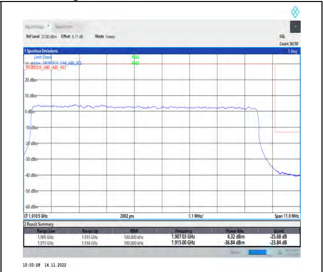
1-N25-PC3-15-10-H-3-DFT-PI2BPSK-Outer_Full-50@0-Ant1-1-seegraph-PASS-see graph
