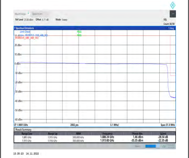
1-N25-PC3-15-30-H-6-CP-QPSK-Outer_Full-160@0-Ant1-1-seegraph-PASS-see graph
