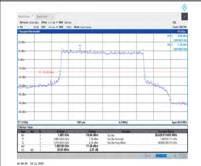
1-N25-PC3-15-30-H-7-CP-16QAM-Outer_Full-160@0 -Ant1-28.629-29.940-≤30-PASS
