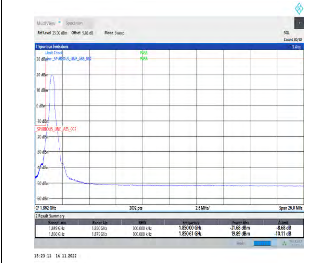
1-N25-PC3-15-25-L-4-CP-QPSK-Edge_1RB_Left-1@0-Ant1-1-seegraph-PASS-see graph
