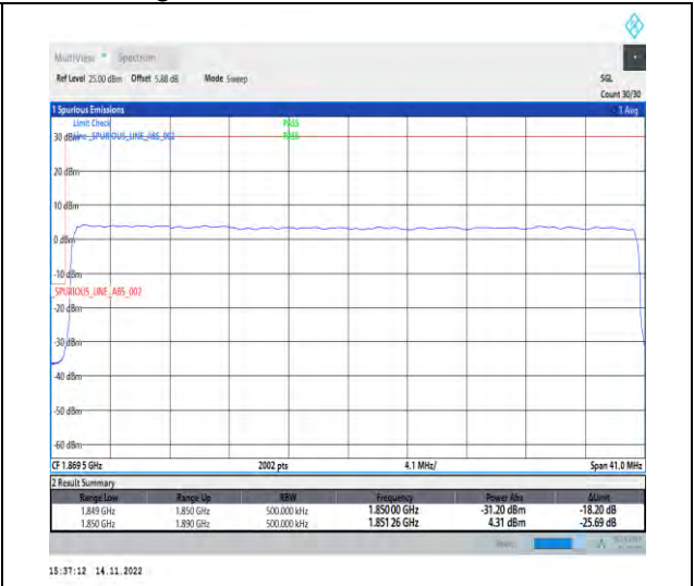
1-N25-PC3-15-40-L-3-DFT-PI2BPSK-Outer_Full-216@0-Ant1-1-seegraph-PASS-see graph
