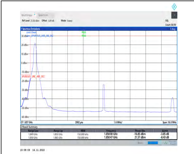
1-N25-PC3-15-15-L-1-DFT-PI2BPSK-Edge_1RB_Left-1@0-Ant1-1-seegraph-PASS-see graph
