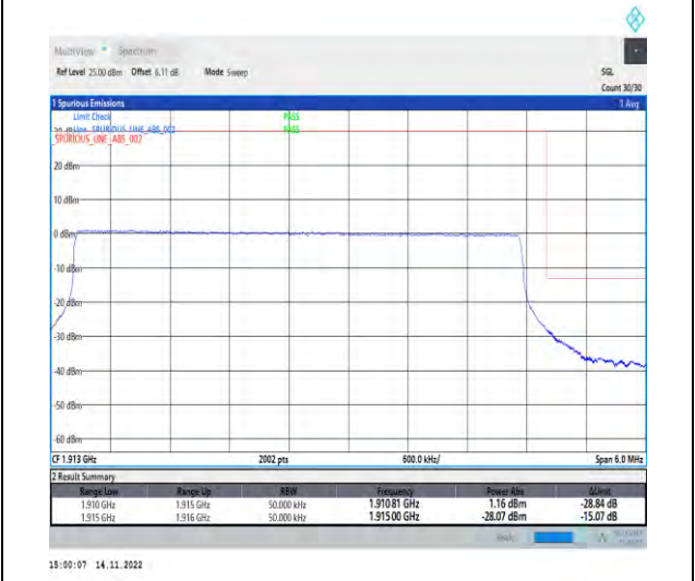
1-N25-PC3-15-5-H-6-CP-QPSK-Outer_Full-25@0-Ant1-1-seegraph-PASS-see graph
