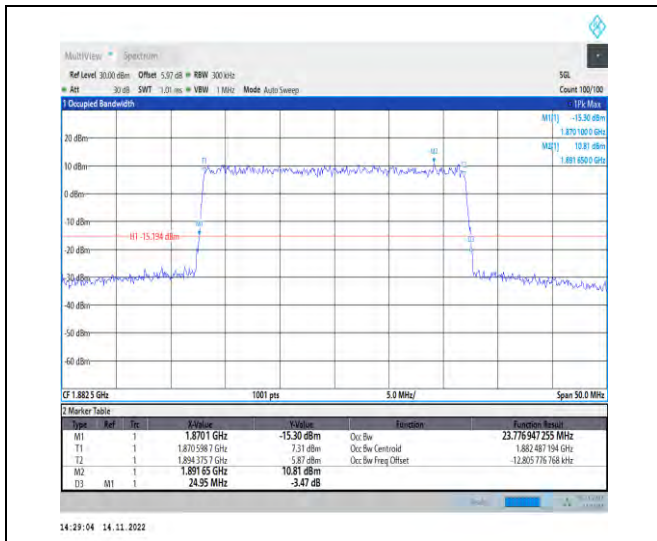
1-N25-PC3-15-25-M-8-CP-64QAM-Outer_Full-133@ 0-Ant1-23.777-24.950-≤25-PASS
