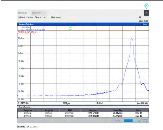
1-N25-PC3-15-10-H-2-DFT-PI2BPSK-Edge_1RB_Right-t@51-Ant1-1-seegraph-PASS-see graph
