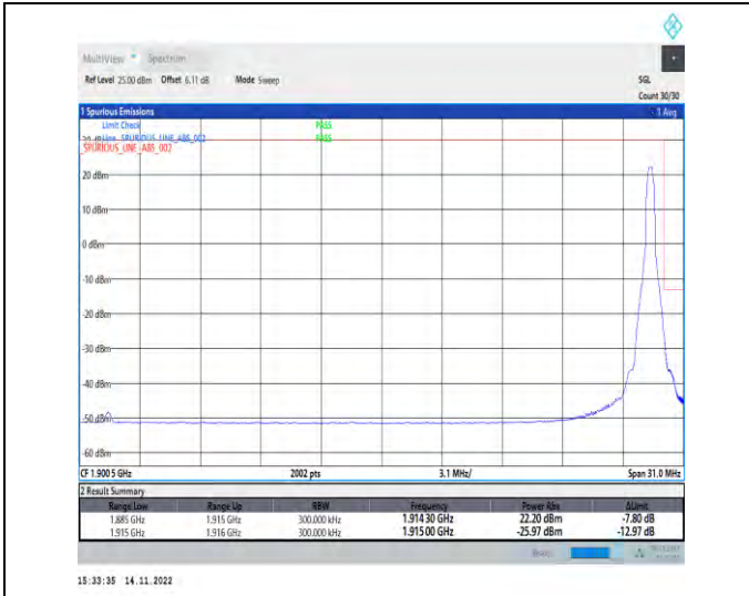
1-N25-PC3-15-30-H-2-DFT-PI2BPSK-Edge_1RB_Right-t-1@159-Ant1-1-seegraph-PASS-see graph
