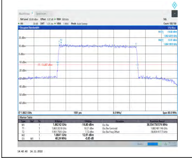
1-N25-PC3-15-40-M-4-DFT-64QAM-Outer_Full-216 @0-Ant1-38.555-40.240-≤40-PASS
