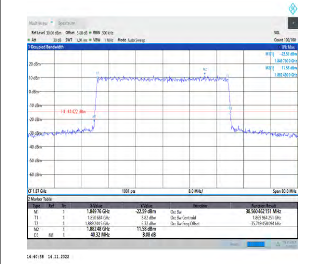
1-N25-PC3-15-40-L-6-CP-QPSK-Outer_Full-216 @0-Ant1-38.56-40.320-≤40-PASS
