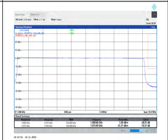
1-N25-PC3-15-15-H-6-CP-QPSK-Outer_Full-79@0-Ant1-1-seegraph-PASS-see graph
