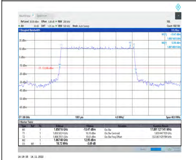
1-N25-PC3-15-20-L-2-DFT-PI2BPSK-Outer_Full-100 @0-Ant1-17.891-18.720-≤20-PASS
