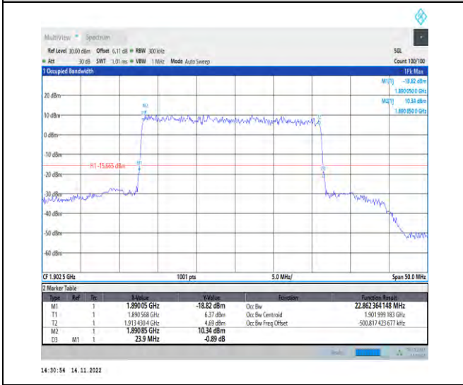
1-N25-PC3-15-25-H-5-DFT-256QAM-Outer_Full-128 @0-Ant1-22.862-23.900-≤25-PASS
