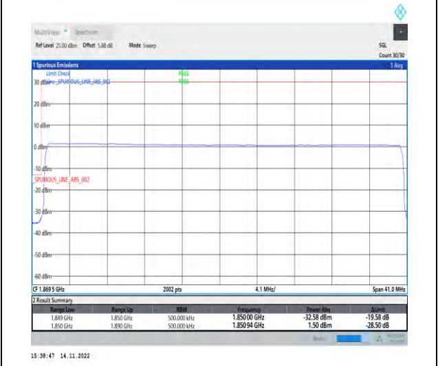
1-N25-PC3-15-40-L-6-CP-QPSK-Outer_Full-216@0-Ant1-1-seegraph-PASS-see graph
