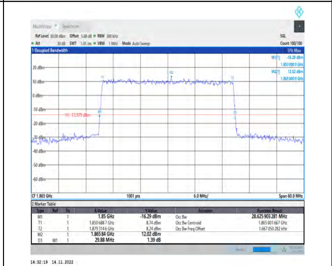
1-N25-PC3-15-30-L-1-DFT-QPSK-Outer_Full-160@ 0-Ant1-28.626-29.880-≤30-PASS
