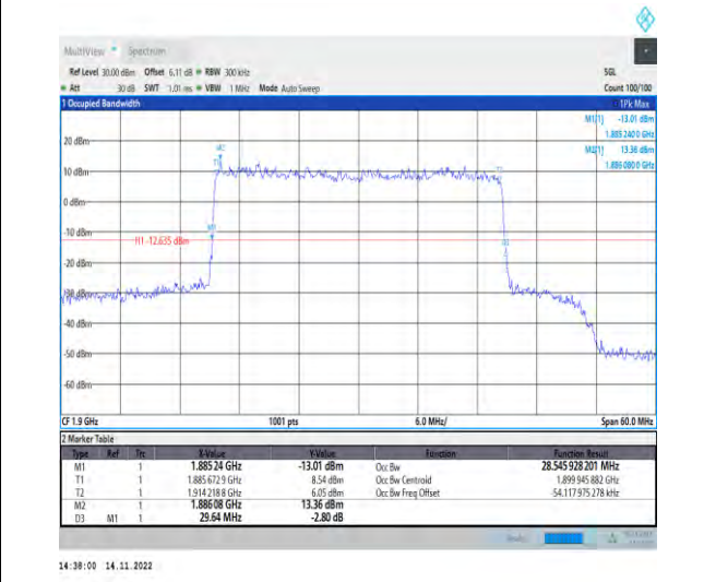
1-N25-PC3-15-30-H-3-DFT-16QAM-Outer_Full-160 @0-Ant1-28.546-29.640-≤30-PASS
