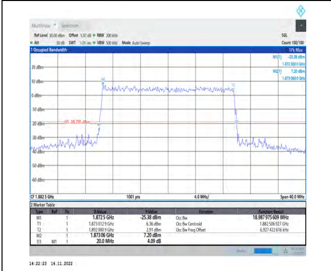
1-N25-PC3-15-20-M-9-CP-256QAM-Outer_Full-106 @0-Ant1-18.988-20.000-≤20-PASS
