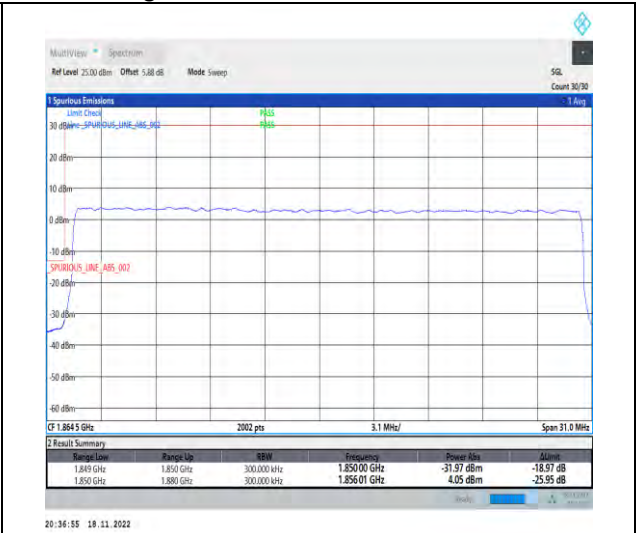
1-N25-PC3-15-30-L-3-DFT-PI2BPSK-Outer_Full-160@0-Ant1-1-seegraph-PASS-see graph
