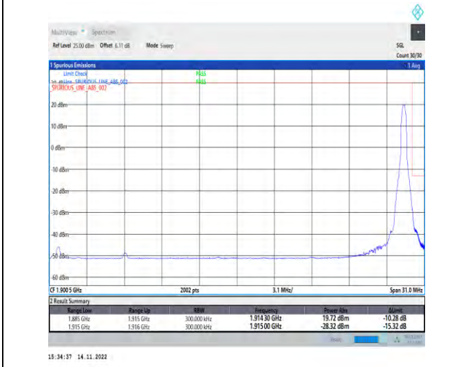
1-N25-PC3-15-30-H-5-CP-QPSK-Edge_1RB_Right-1@159-Ant1-1-seegraph-PASS-see graph
