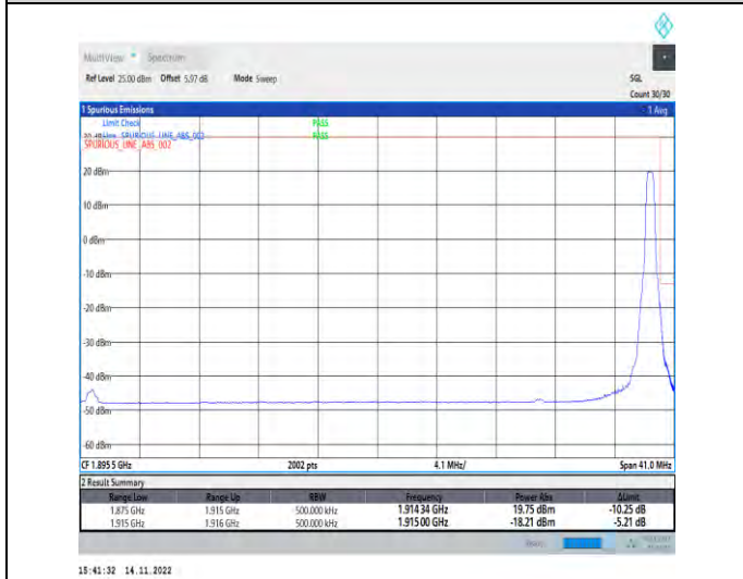
1-N25-PC3-15-40-H-5-CP-QPSK-Edge_1RB_Right-1@215-Ant1-1-seegraph-PASS-see graph
