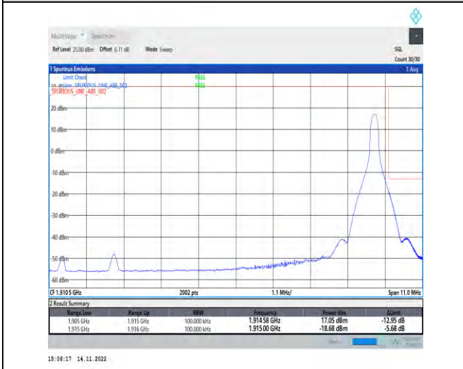
1-N25-PC3-15-10-H-5-CP-QPSK-Edge_1RB_Right-1@51-Ant1-1-seegraph-PASS-see graph
