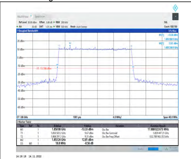
1-N25-PC3-15-20-L-1-DFT-QPSK-Outer_Full-100@ 0-Ant1-17.888-18.800-≤20-PASS
