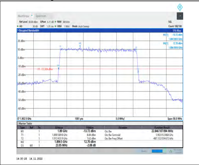
1-N25-PC3-15-25-H-4-DFT-64QAM-Outer_Full-128 @0-Ant1-22.846-23.950-≤25-PASS
