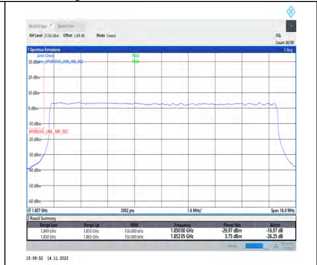
1-N25-PC3-15-15-L-3-DFT-PI2BPSK-Outer_Full-75@0-Ant1-1-seegraph-PASS-see graph
