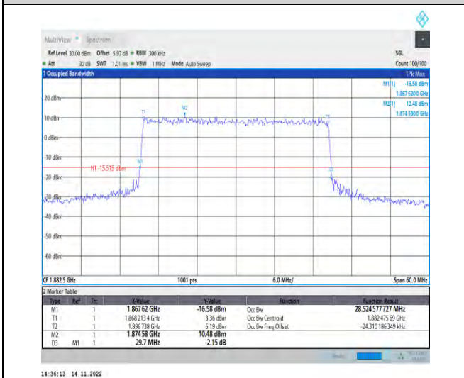
1-N25-PC3-15-30-M-7-CP-16QAM-Outer_Full-160@0-Ant1-28.525-29.700-≤30-PASS
