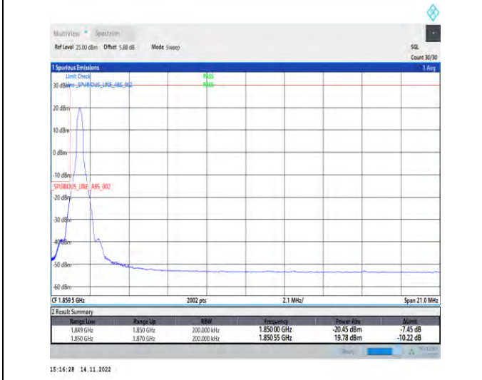
1-N25-PC3-15-20-L-4-CP-QPSK-Edge_1RB_Left-1@0-Ant1-1-seegraph-PASS-see graph
