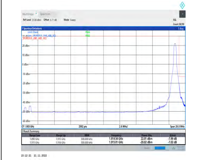
1-N25-PC3-15-25-H-5-CP-QPSK-Edge_1RB_Right-1@132-Ant1-1-seegraph-PASS-see graph
