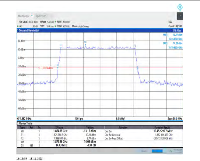
1-N25-PC3-15-15-M-1-DFT-QPSK-Outer_Full-75@0-Ant1-13.452-14.430-≤15-PASS
