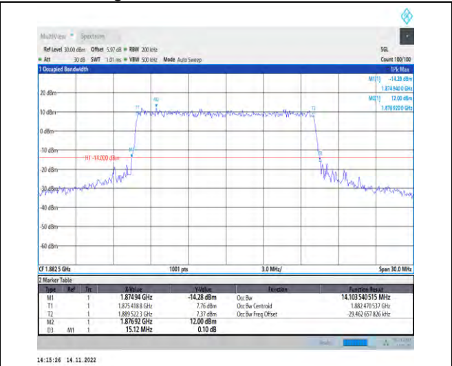
1-N25-PC3-15-15-M-7-CP-16QAM-Outer_Full-79@0-Ant1-14.104-15.120-≤15-PASS
