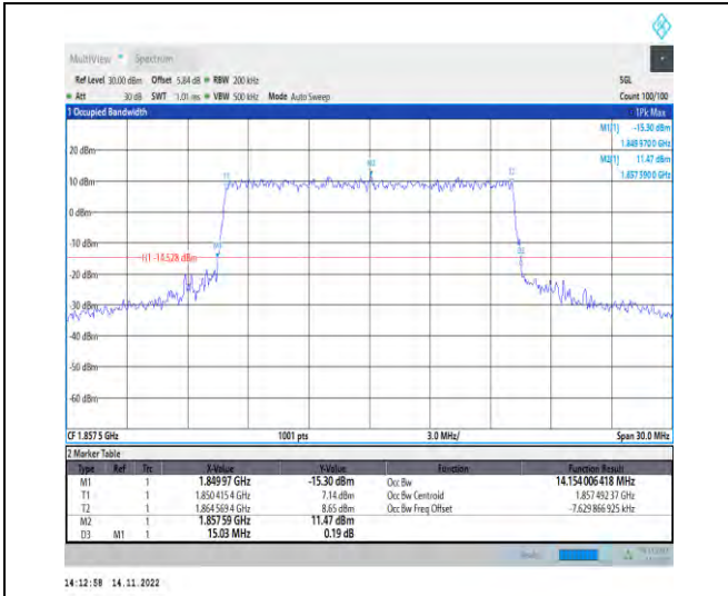
1-N25-PC3-15-15-L-7-CP-16QAM-Outer_Full-79@0-Ant1-14.154-15.030-≤15-PASS
