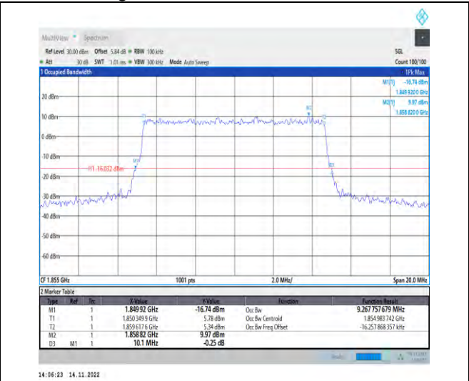
1-N25-PC3-15-10-L-7-CP-16QAM-Outer_Full-52@0-A Ant1-9.268-10.100-≤10-PASS
