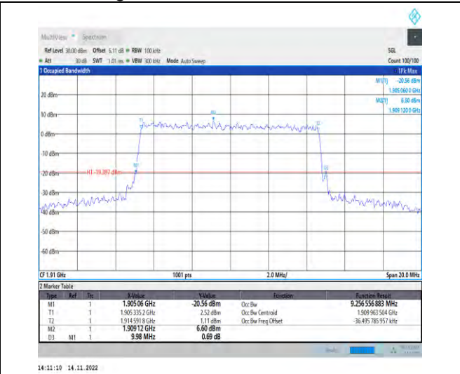
1-N25-PC3-15-10-H-9-CP-256QAM-Outer_Full-52@0 -Ant1-9.257-9.980-≤10-PASS
