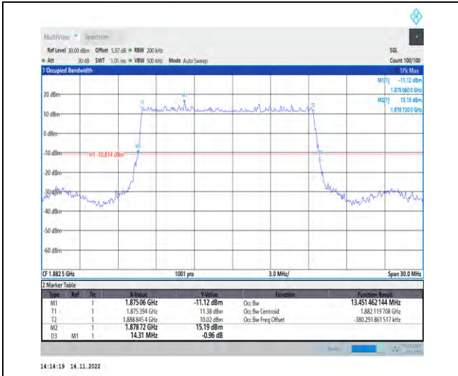
1-N25-PC3-15-15-M-2-DFT-PI2BPSK-Outer_Full-75 @0-Ant1-13.451-14.310-≤15-PASS
