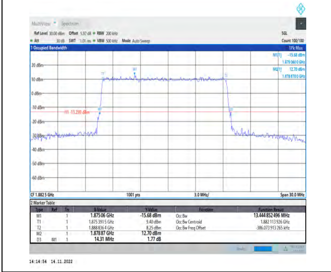
1-N25-PC3-15-15-M-4-DFT-64QAM-Outer_Full-75 @0-Ant1-13.445-14.310-≤15-PASS
