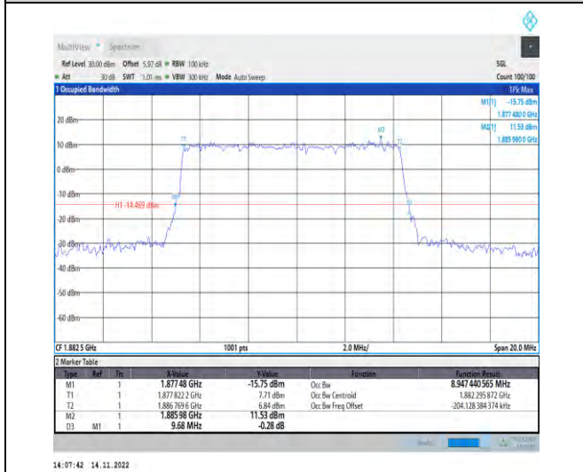
1-N25-PC3-15-10-M-3-DFT-16QAM-Outer_Full-50@0 0-Ant1-8.947-9.680-≤10-PASS
