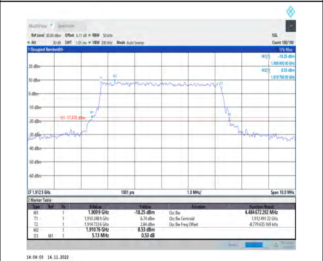
1-N25-PC3-15-5-H-6-CP-QPSK-Outer_Full-25@0-A nt1-4.485-5.130-≤5-PASS
