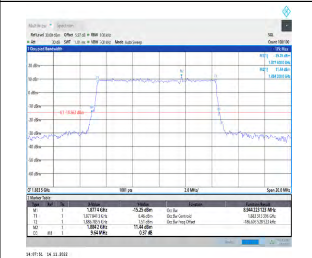
1-N25-PC3-15-10-M-4-DFT-64QAM-Outer_Full-50@0 0-Ant1-8.944-9.640-≤10-PASS
