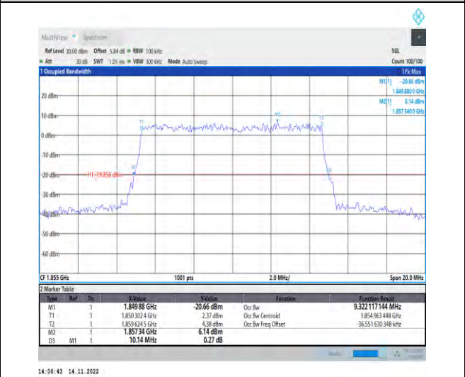
1-N25-PC3-15-10-L-9-CP-256QAM-Outer_Full-52@0-A Ant1-9.322-10.140-≤10-PASS
