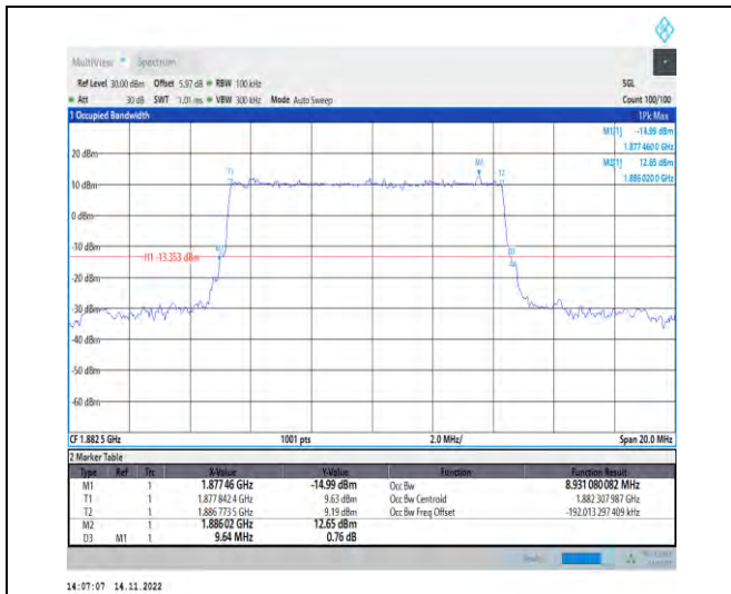
1-N25-PC3-15-10-M-1-DFT-QPSK-Outer_Full-50@0 -Ant1-8.931-9.640-≤10-PASS
