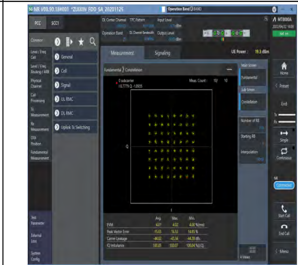
1-N25--15-40-M-8-CP-64QAM-Outer_Full-216@0-Ant1-see graph-PASS
