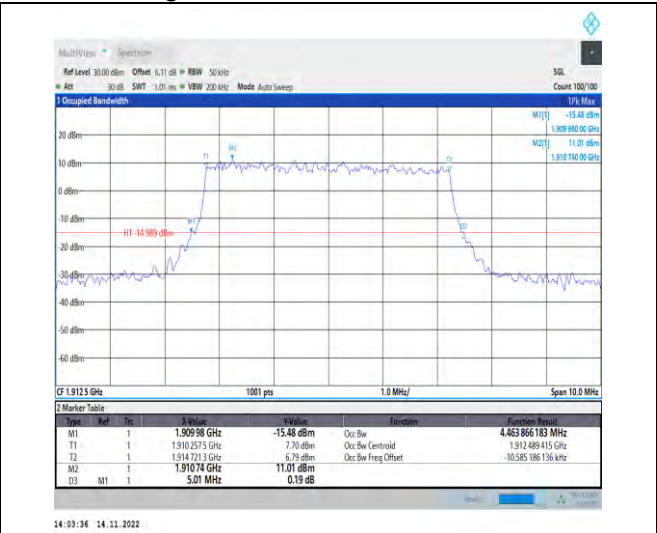
1-N25-PC3-15-5-H-4-DFT-64QAM-Outer_Full-25@0 -Ant1-4.464-5.010-≤5-PASS
