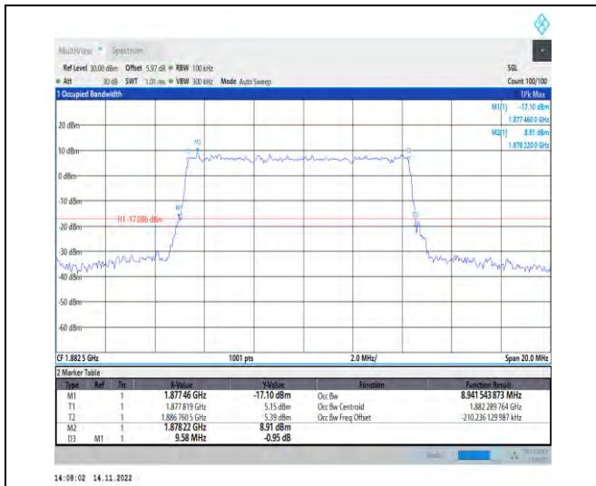
1-N25-PC3-15-10-M-5-DFT-256QAM-Outer_Full-50@0-Ant1-8.942-9.580-≤10-PASS
