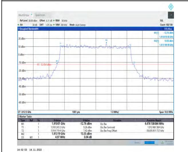
1-N25-PC3-15-5-H-1-DFT-QPSK-Outer_Full-25@0-Ant1-4.476-4.970-≤5-PASS
