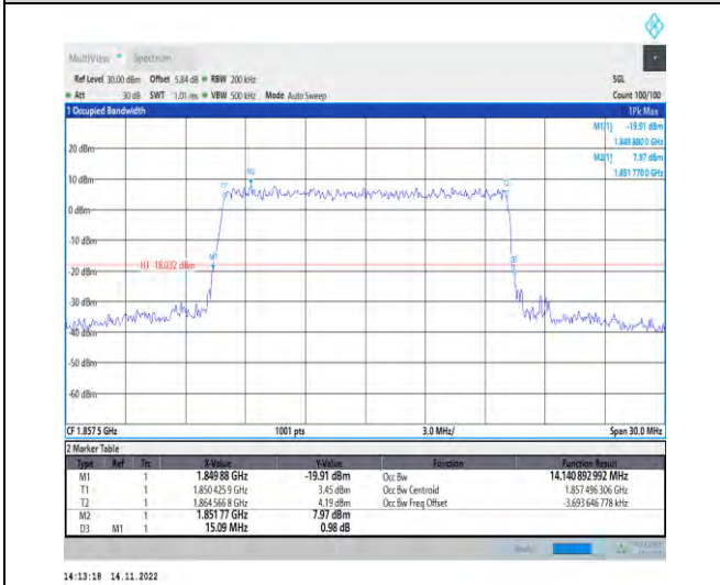
1-N25-PC3-15-15-L-9-CP-256QAM-Outer_Full-79@0-Ant1-14.141-15.090-≤15-PASS
