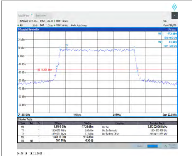
1-N25-PC3-15-10-L-6-CP-QPSK-Outer_Full-52@0-A nt1-9.312-10.100-≤10-PASS
